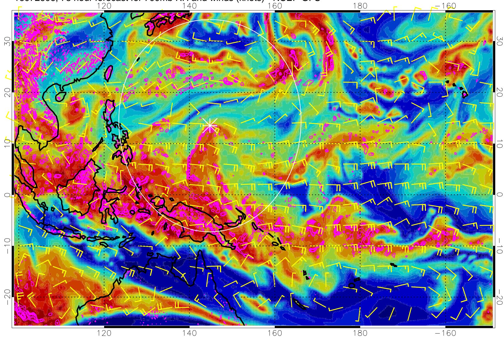
16072606, 78 hour forecast for 700mb RH and winds (knots) - NCEP GFS
