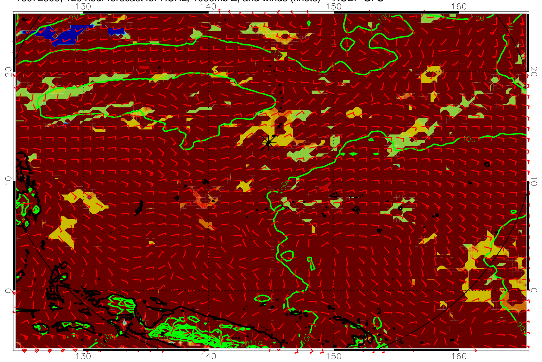
16072800, 120 hour forecast for HCAL, 1000mb Z, and winds (knots) -- NCEP GFS
