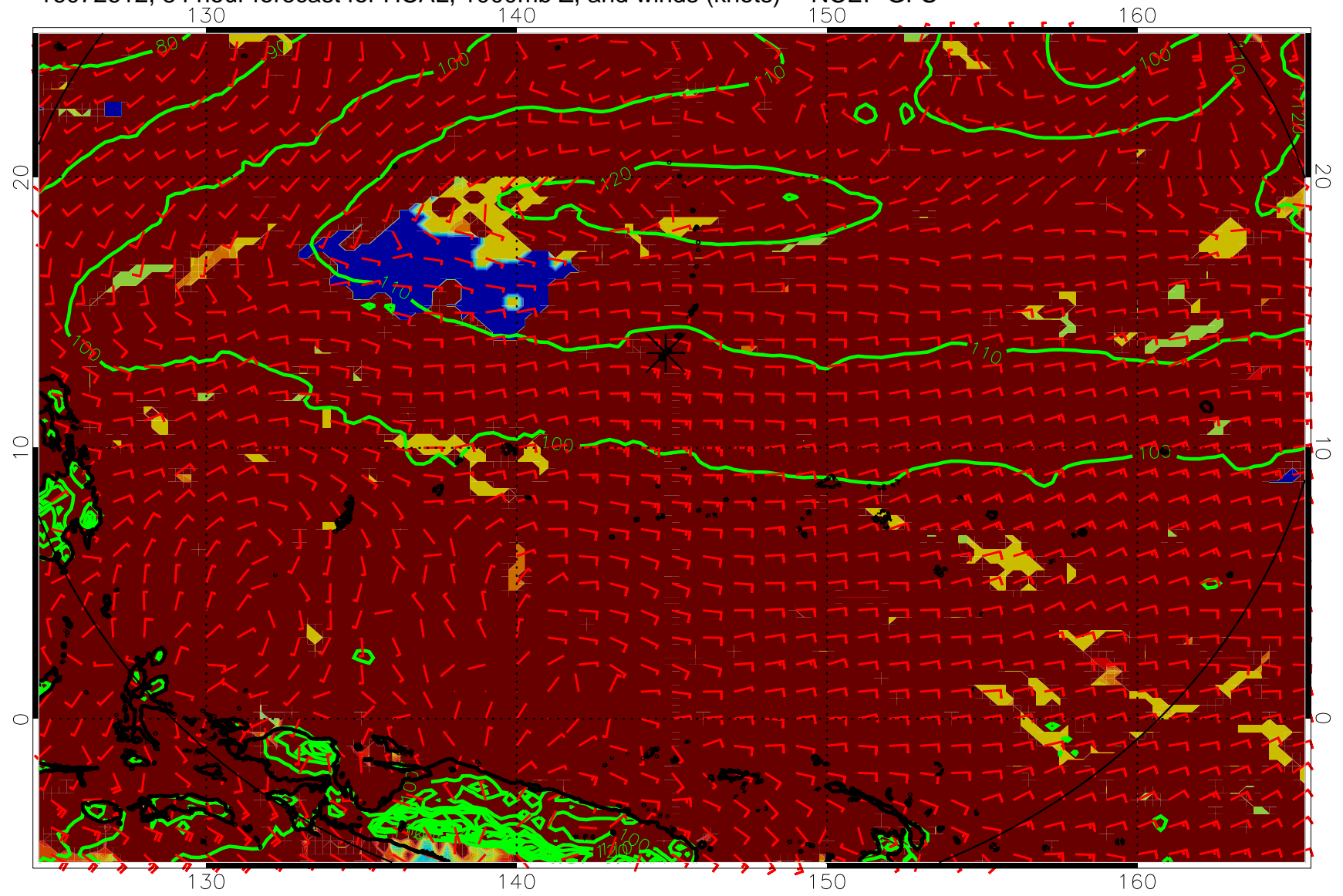
16072612, 84 hour forecast for HCAL, 1000mb Z, and winds (knots) -- NCEP GFS
