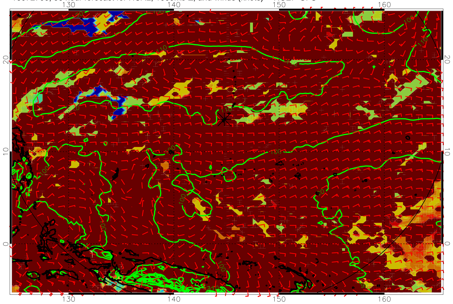
16072700, 96 hour forecast for HCAL, 1000mb Z, and winds (knots) -- NCEP GFS
