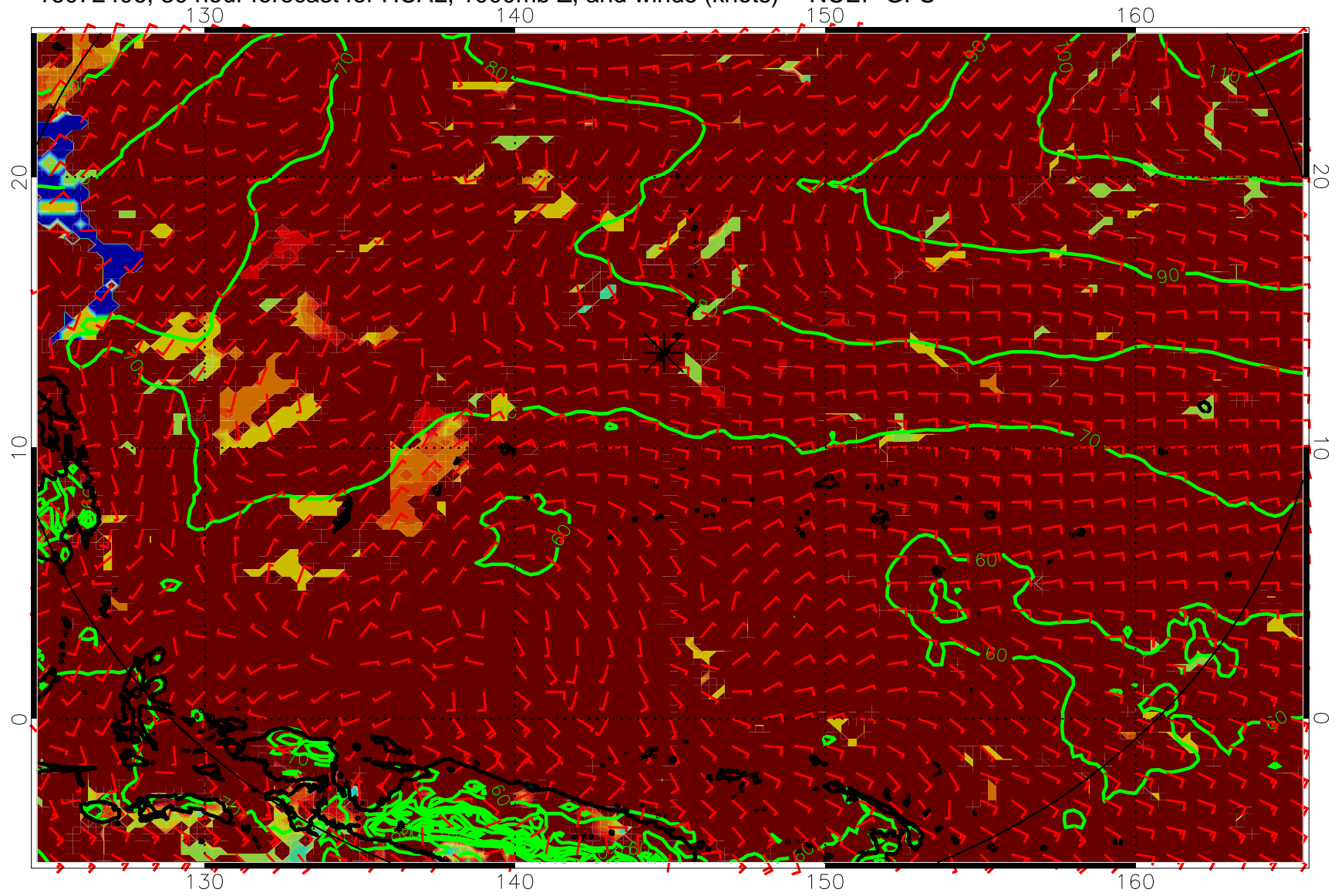
16072406, 30 hour forecast for HCAL, 1000mb Z, and winds (knots) -- NCEP GFS
