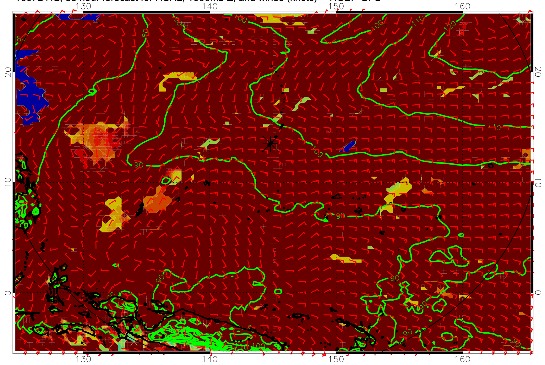
16072412, 36 hour forecast for HCAL, 1000mb Z, and winds (knots) -- NCEP GFS
