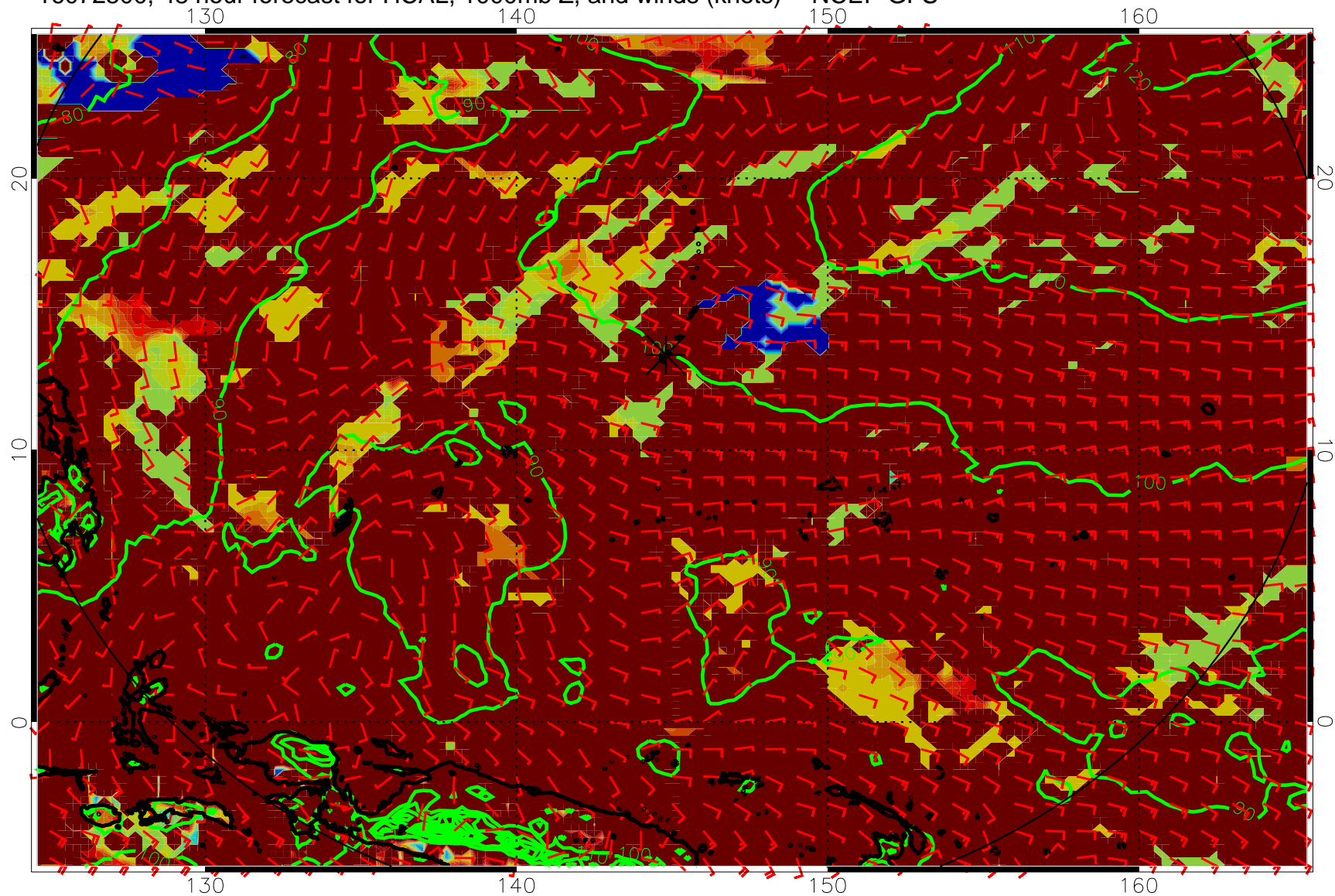
16072500, 48 hour forecast for HCAL, 1000mb Z, and winds (knots) -- NCEP GFS
