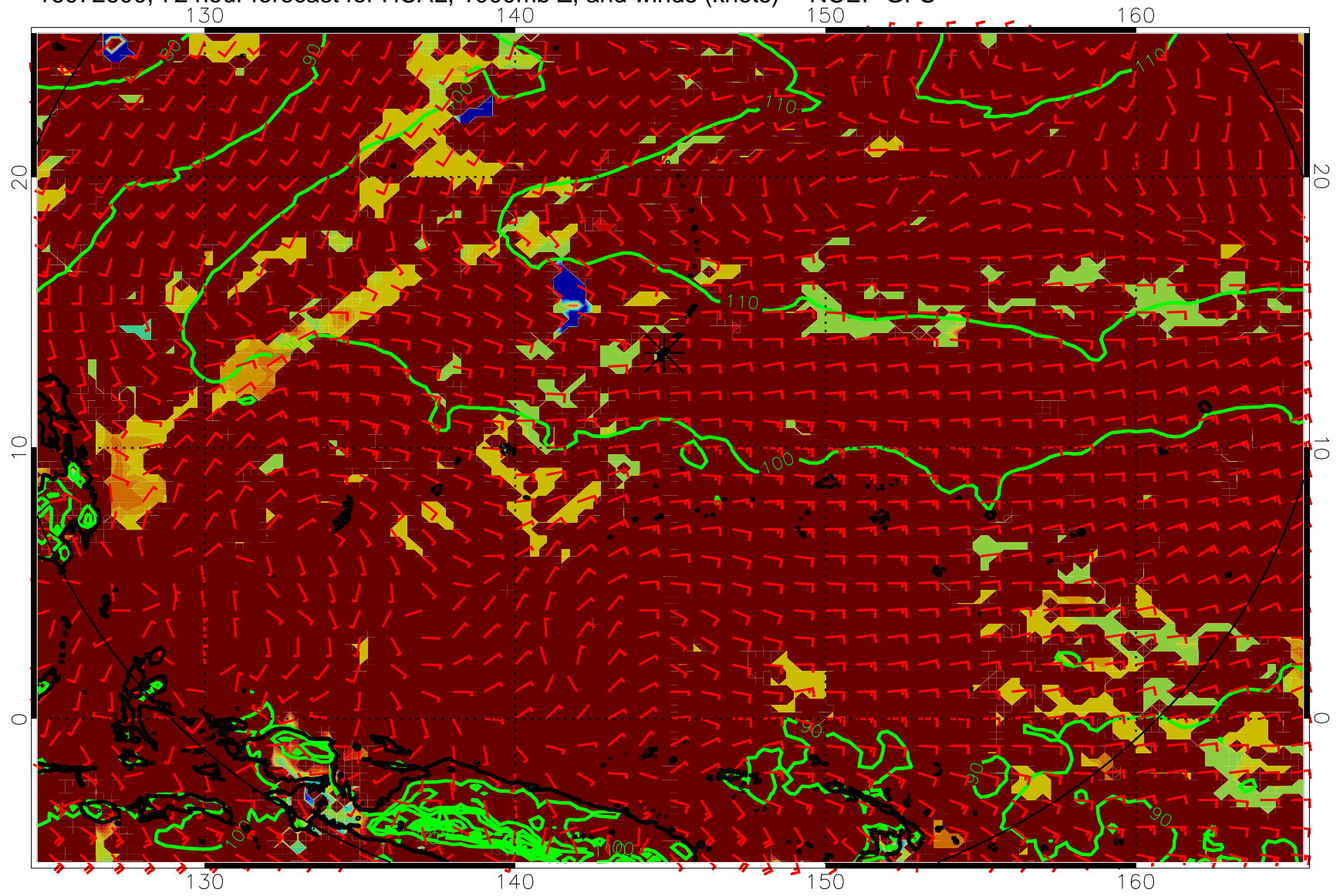
16072600, 72 hour forecast for HCAL, 1000mb Z, and winds (knots) -- NCEP GFS
