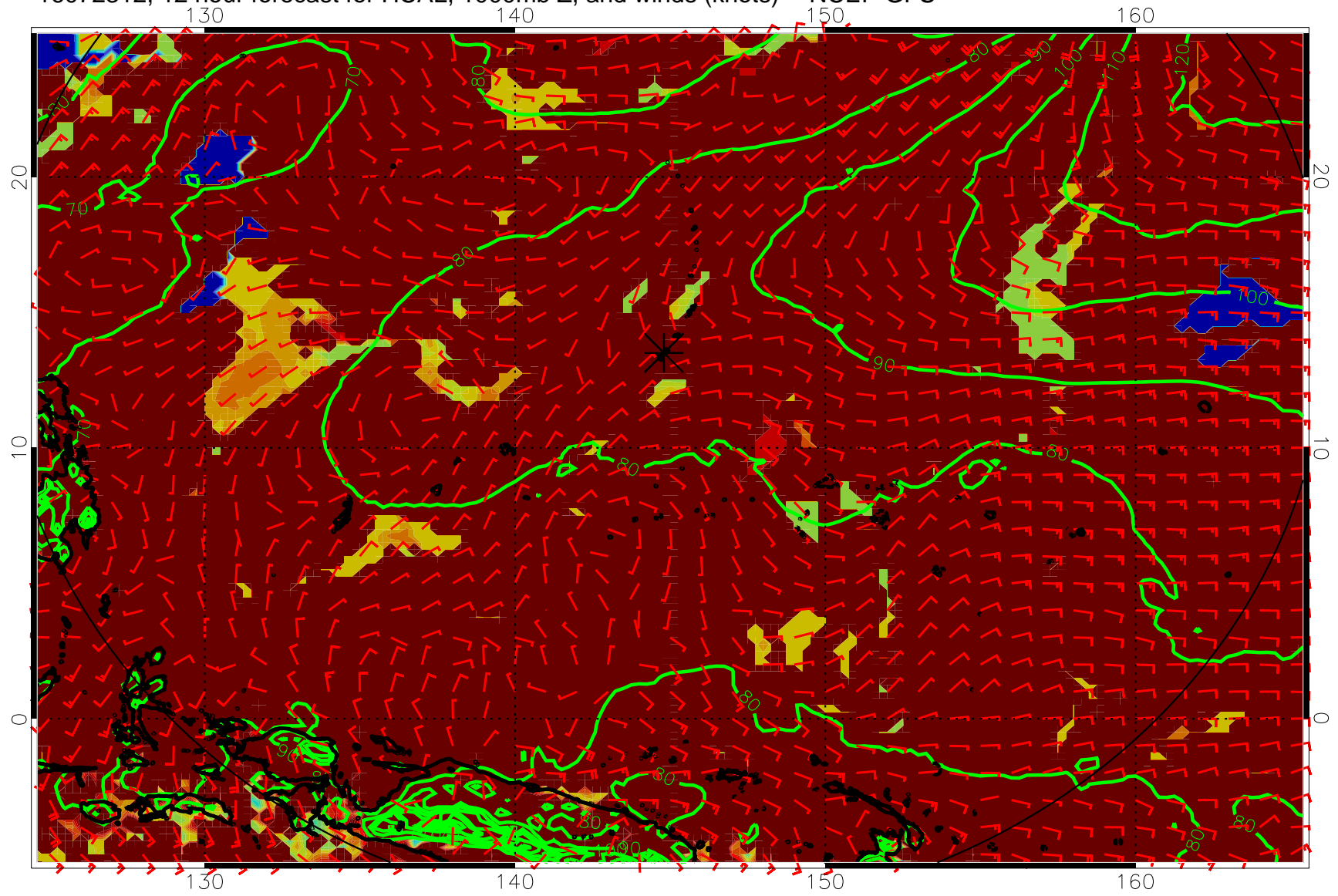
16072312, 12 hour forecast for HCAL, 1000mb Z, and winds (knots) -- NCEP GFS
