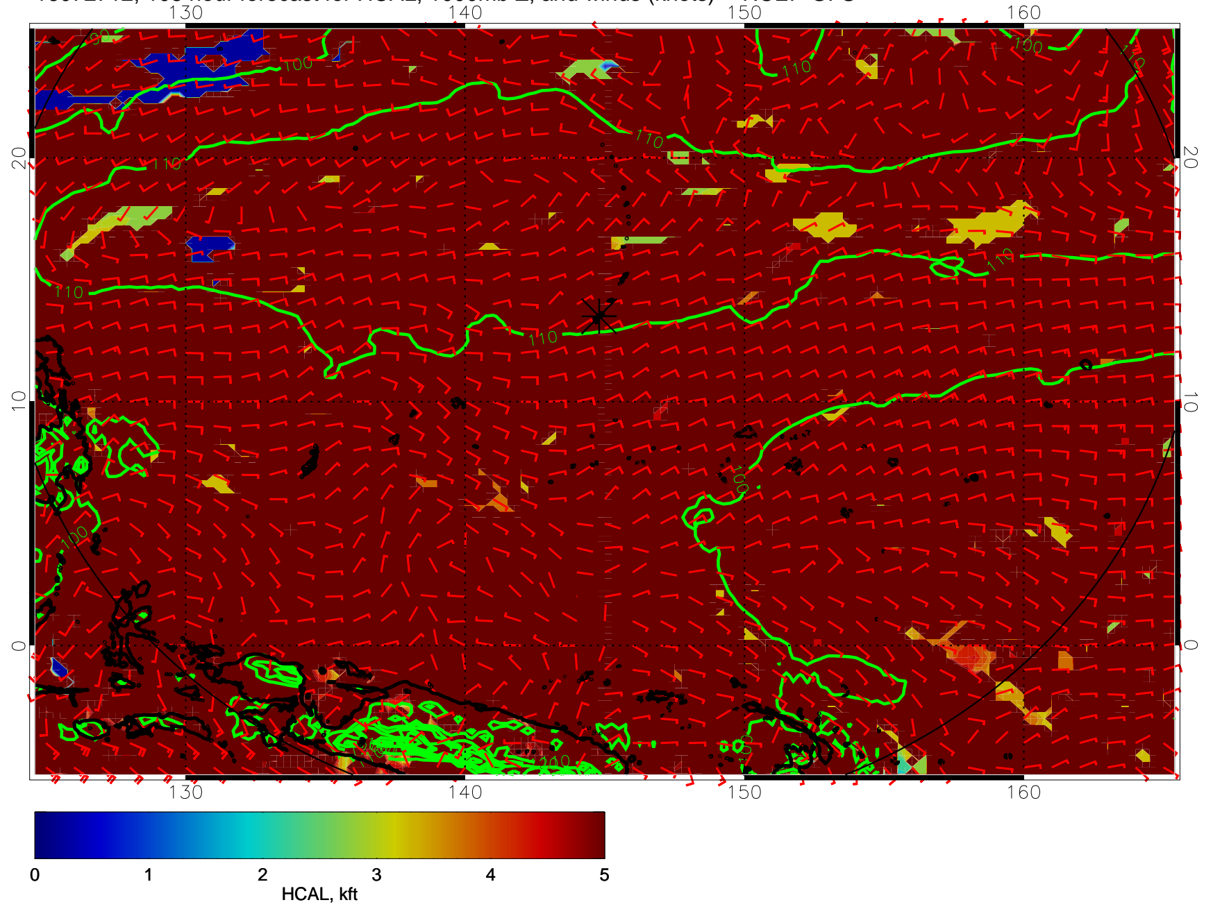
16072712, 108 hour forecast for HCAL, 1000mb Z, and winds (knots) -- NCEP GFS
