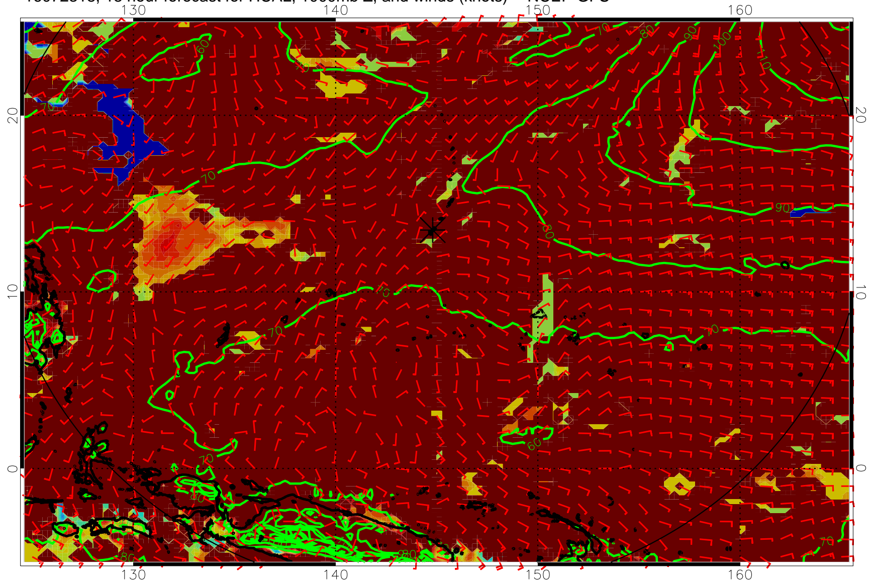
16072318, 18 hour forecast for HCAL, 1000mb Z, and winds (knots) -- NCEP GFS
