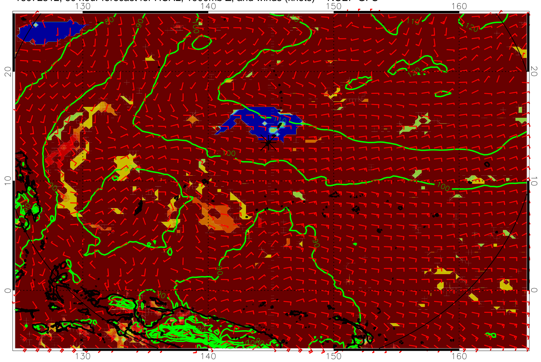
16072512, 60 hour forecast for HCAL, 1000mb Z, and winds (knots) -- NCEP GFS
