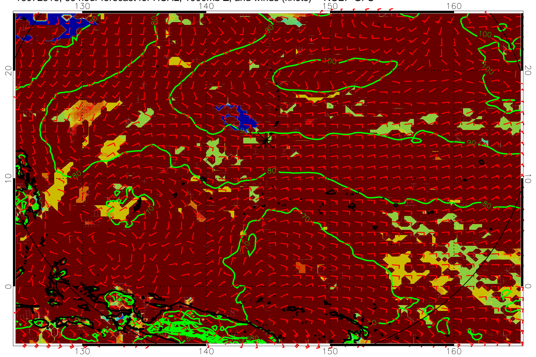
16072518, 66 hour forecast for HCAL, 1000mb Z, and winds (knots) -- NCEP GFS
