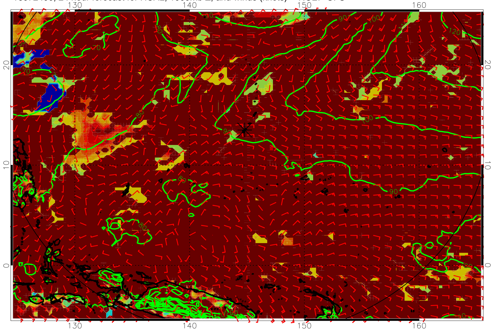
16072400, 24 hour forecast for HCAL, 1000mb Z, and winds (knots) -- NCEP GFS
