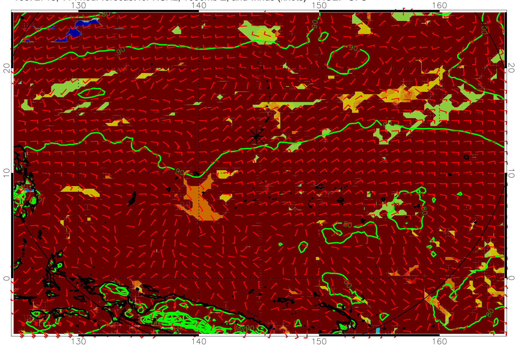
16072718, 114 hour forecast for HCAL, 1000mb Z, and winds (knots) -- NCEP GFS
