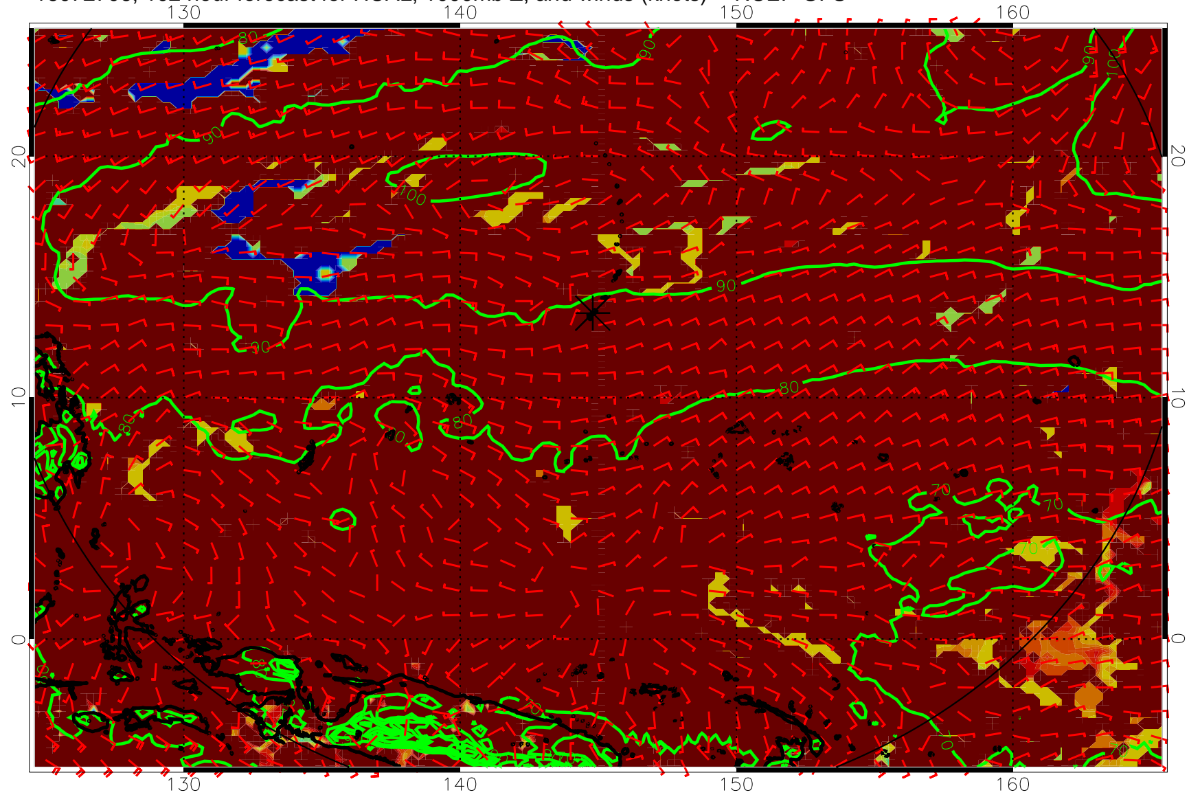
16072706, 102 hour forecast for HCAL, 1000mb Z, and winds (knots) -- NCEP GFS
