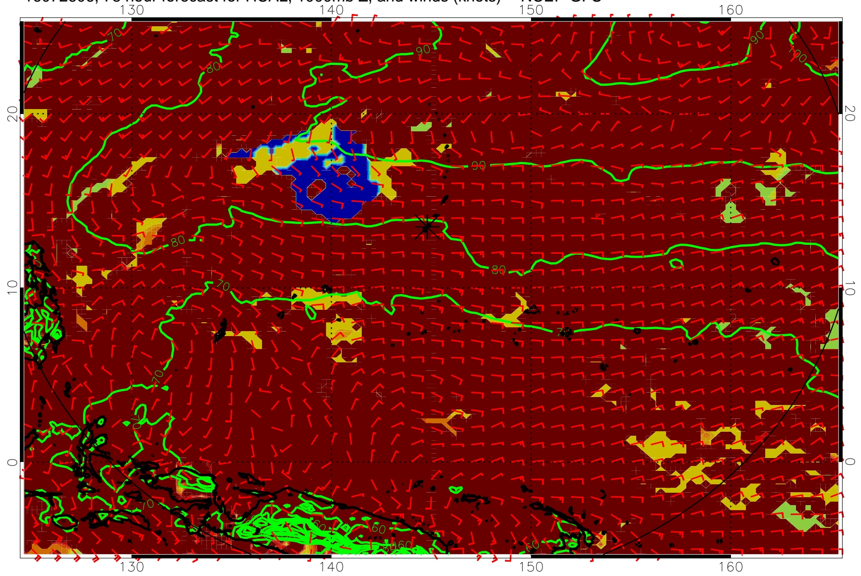
16072606, 78 hour forecast for HCAL, 1000mb Z, and winds (knots) -- NCEP GFS
