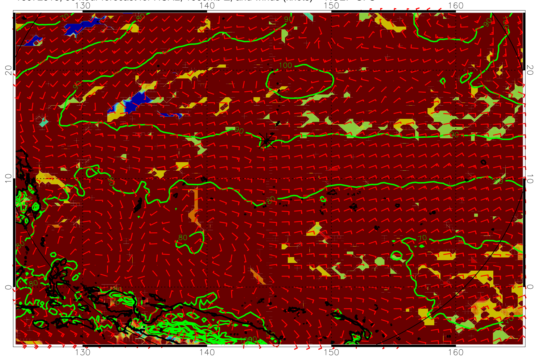
16072618, 90 hour forecast for HCAL, 1000mb Z, and winds (knots) -- NCEP GFS
