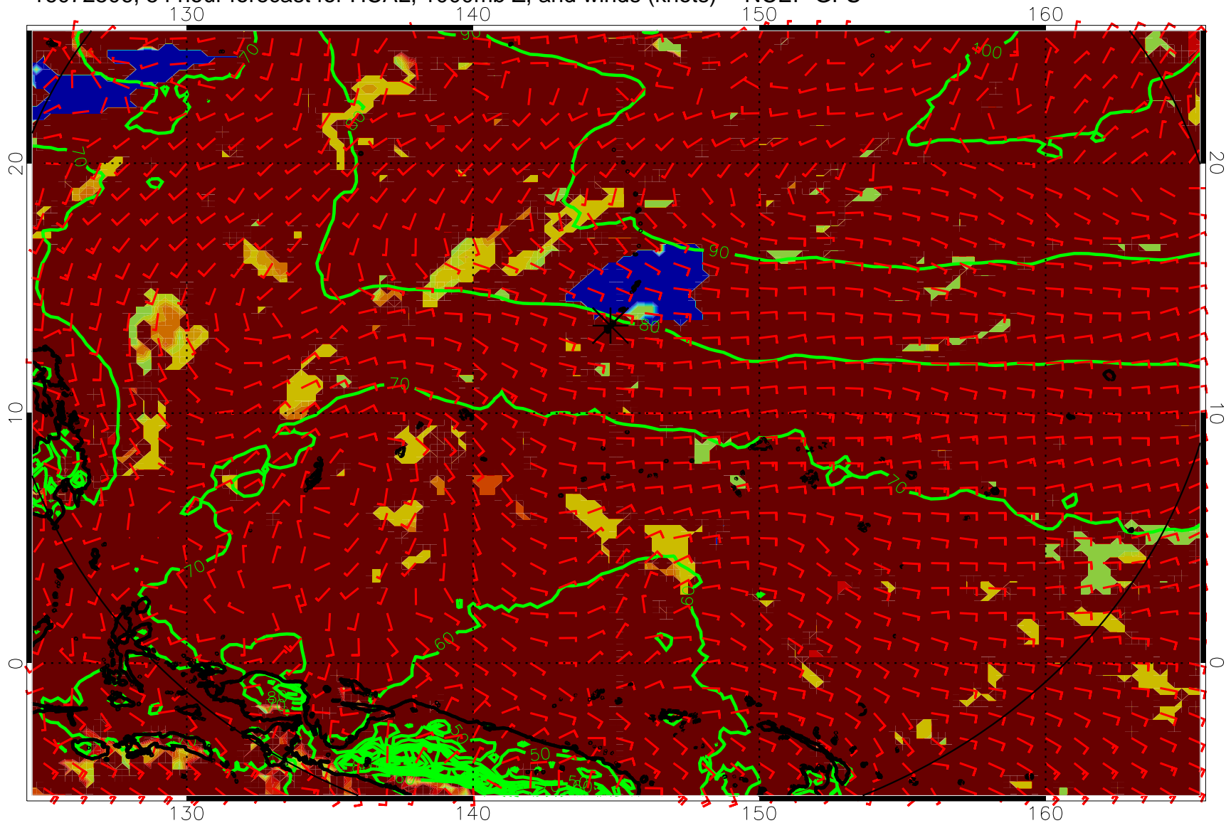
16072506, 54 hour forecast for HCAL, 1000mb Z, and winds (knots) -- NCEP GFS
