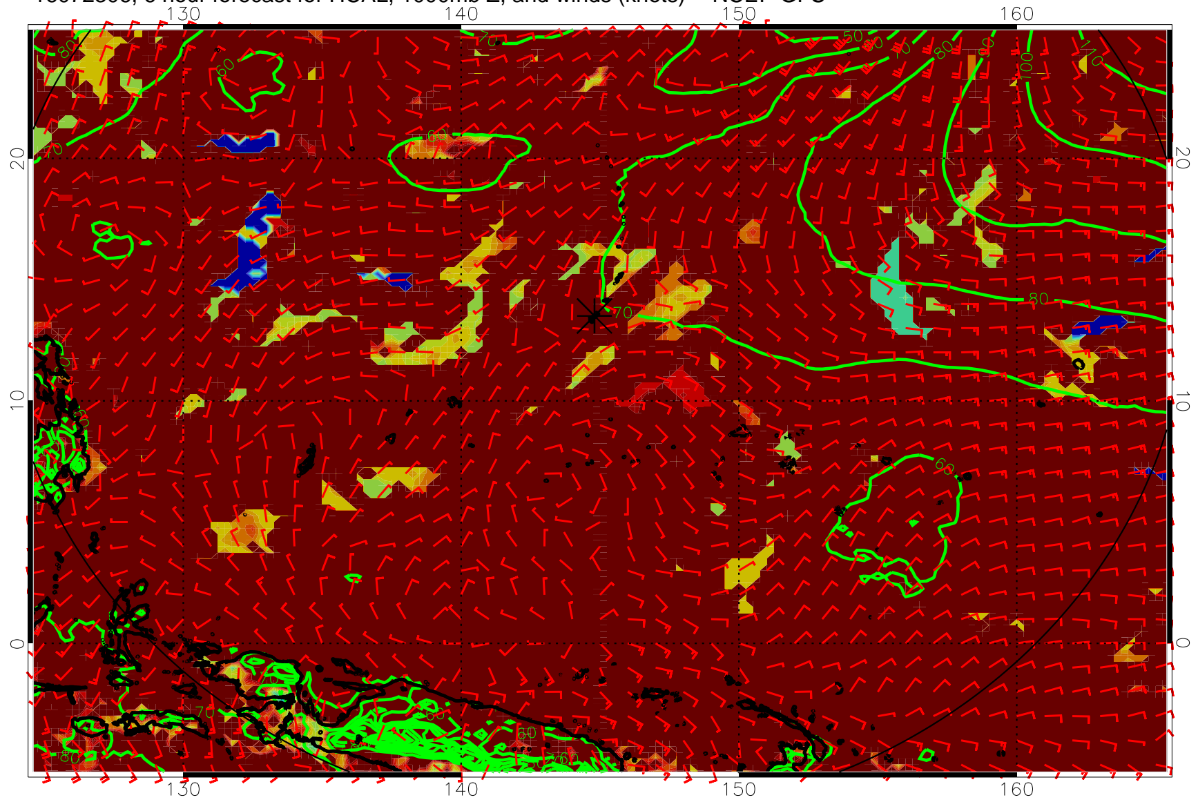
16072306, 6 hour forecast for HCAL, 1000mb Z, and winds (knots) -- NCEP GFS
