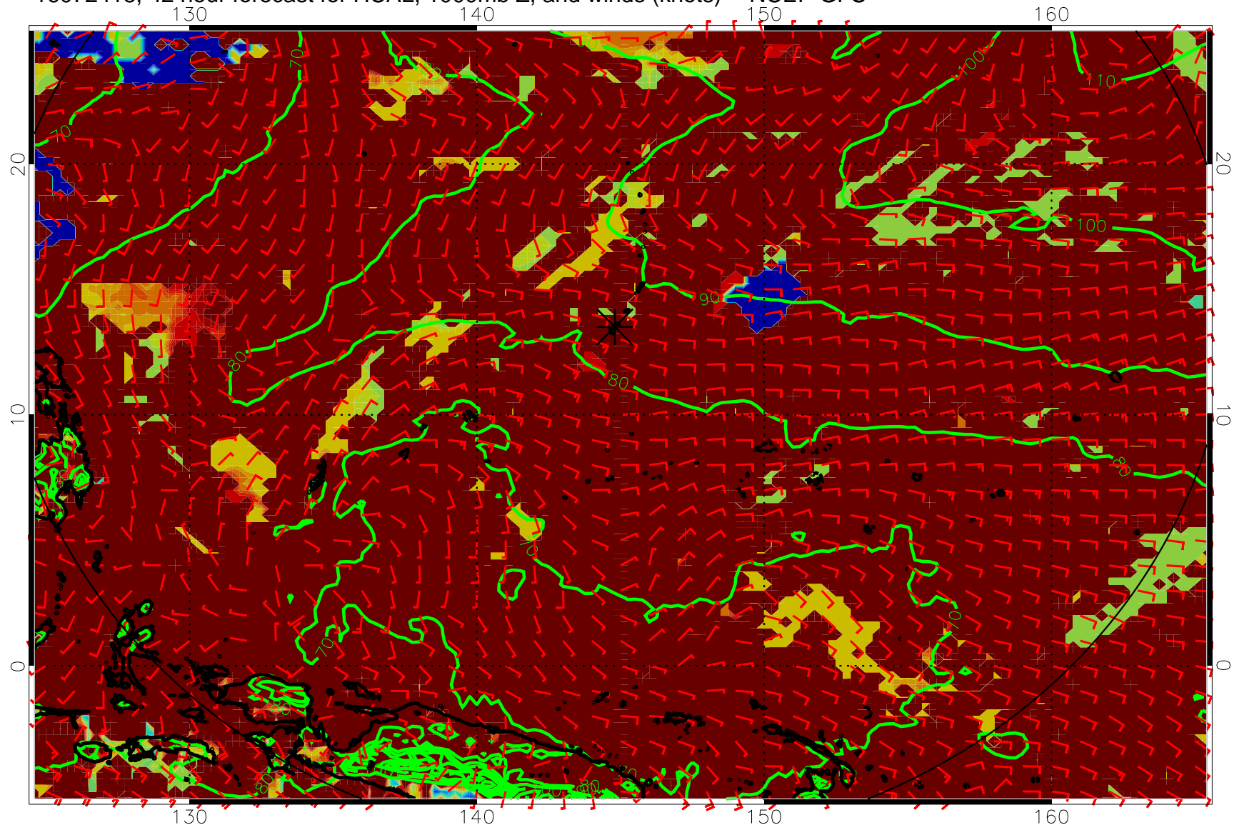
16072418, 42 hour forecast for HCAL, 1000mb Z, and winds (knots) -- NCEP GFS
