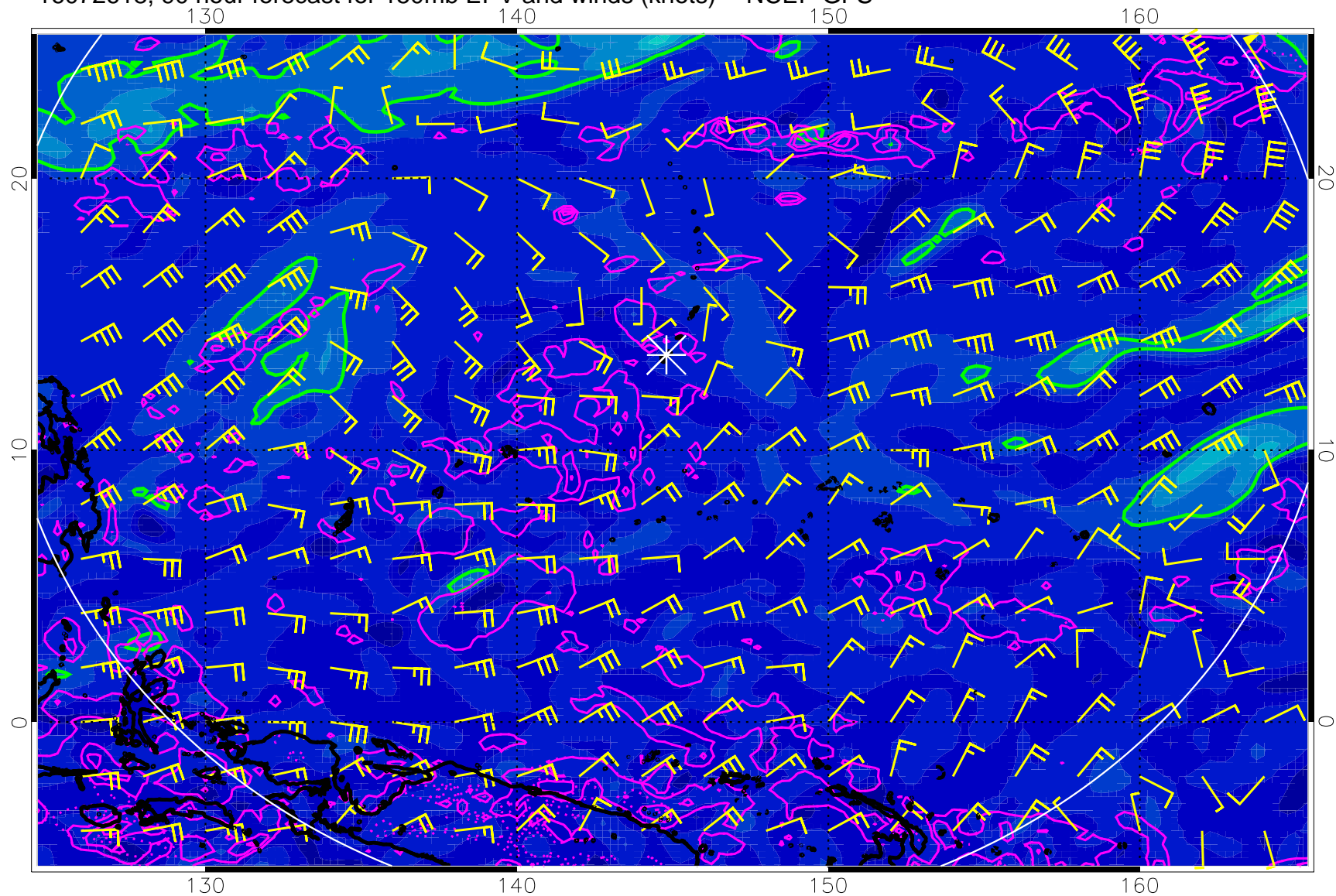
16072618, 90 hour forecast for 150mb EPV and winds (knots) -- NCEP GFS
