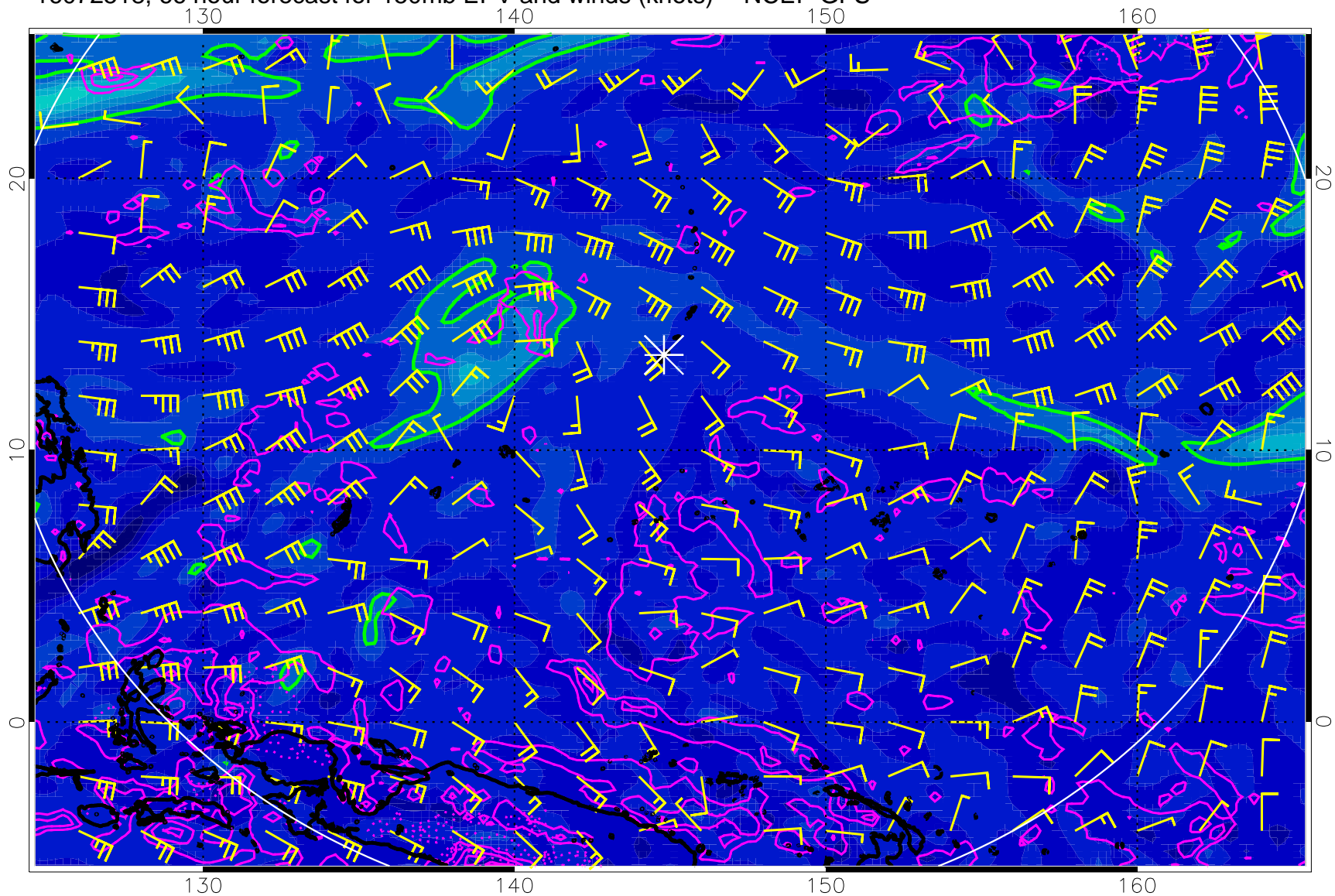
16072518, 66 hour forecast for 150mb EPV and winds (knots) -- NCEP GFS
