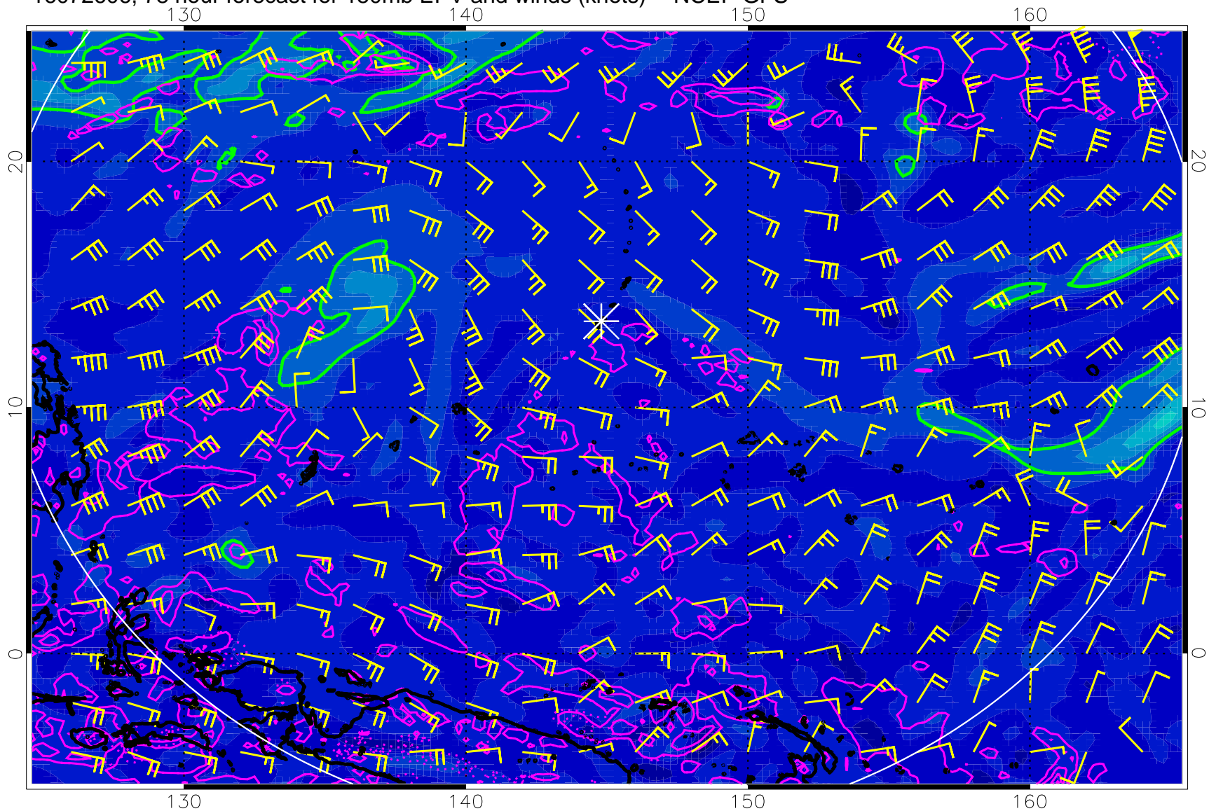
16072606, 78 hour forecast for 150mb EPV and winds (knots) -- NCEP GFS
