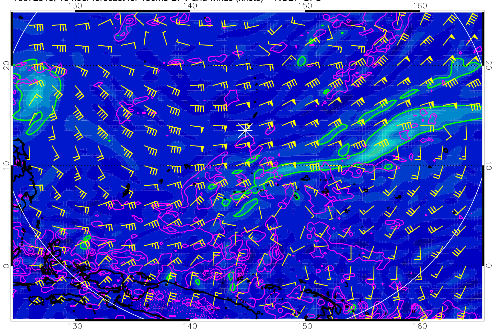
16072318, 18 hour forecast for 150mb EPV and winds (knots) -- NCEP GFS
