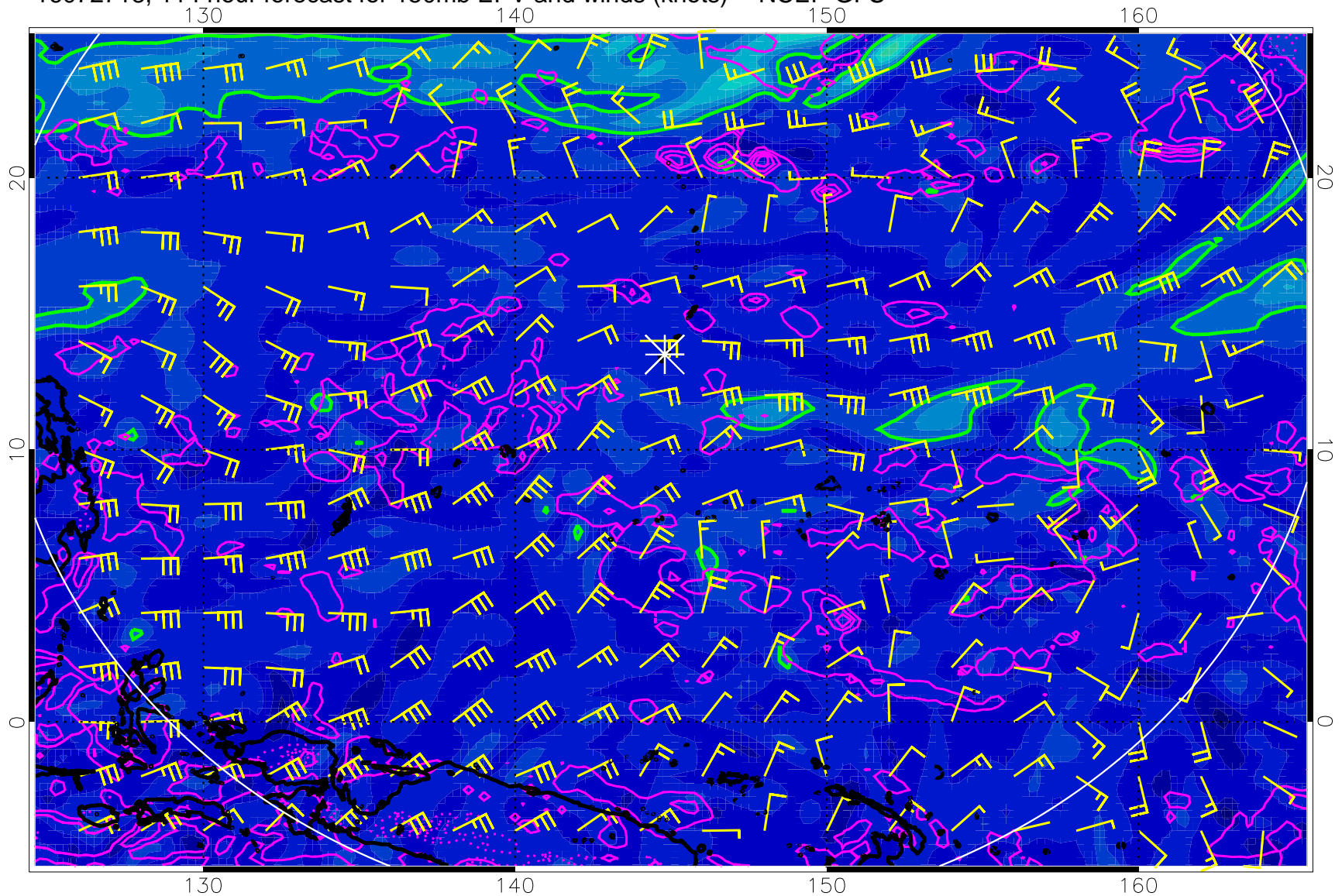
16072718, 114 hour forecast for 150mb EPV and winds (knots) -- NCEP GFS
