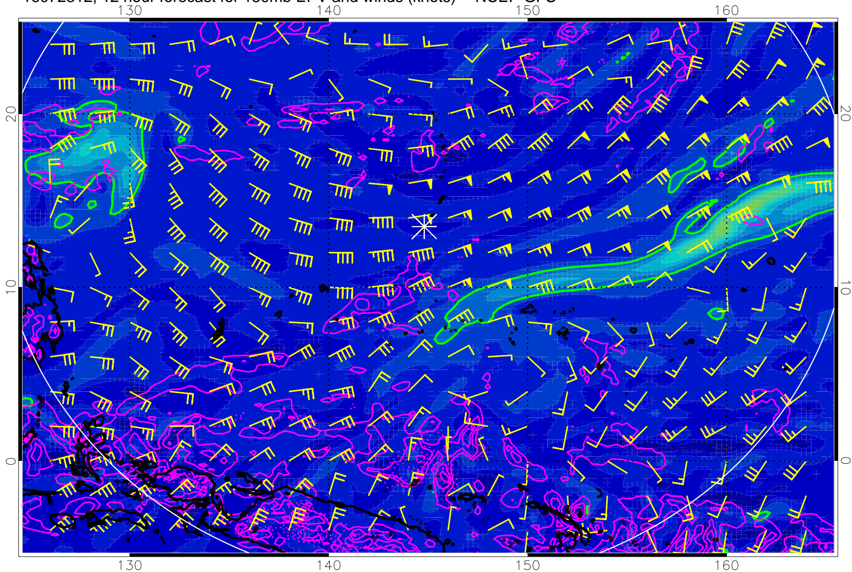
16072312, 12 hour forecast for 150mb EPV and winds (knots) -- NCEP GFS
