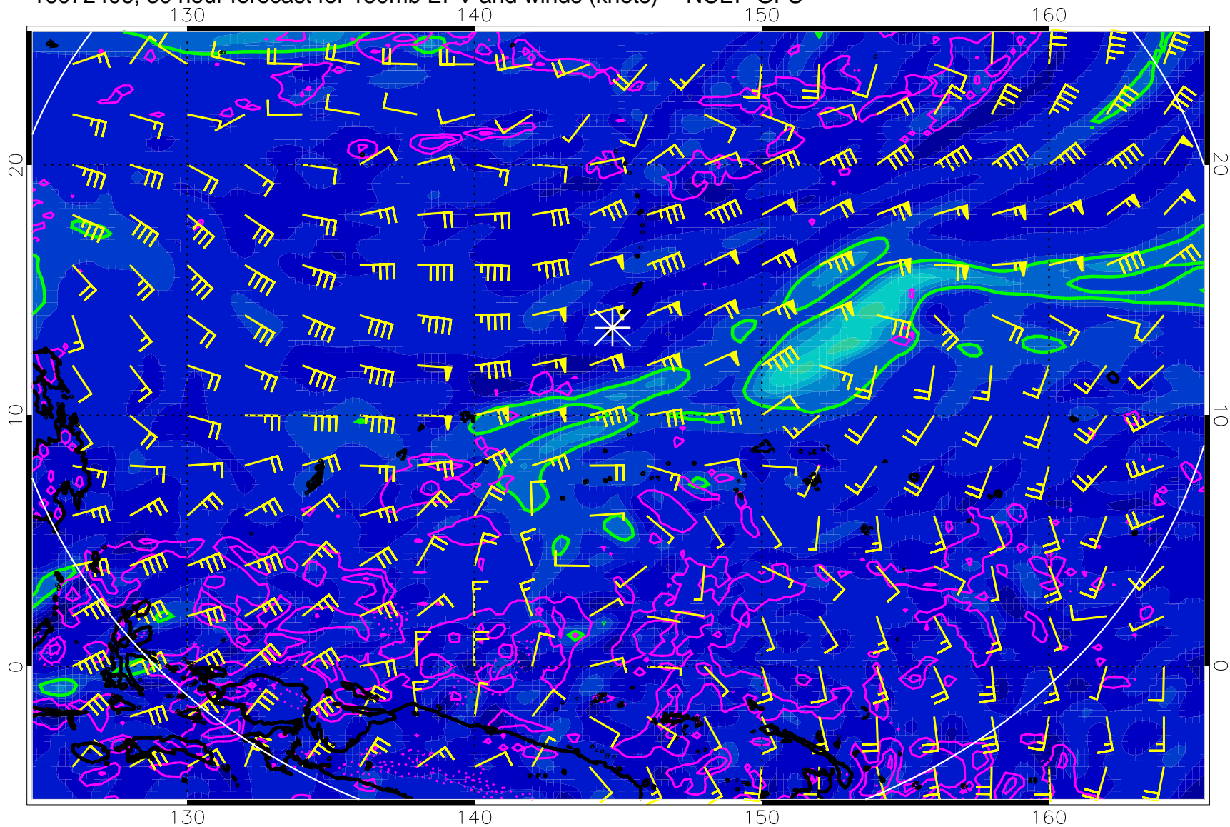
16072406, 30 hour forecast for 150mb EPV and winds (knots) -- NCEP GFS
