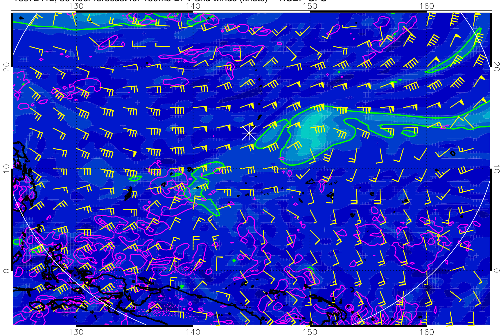
16072412, 36 hour forecast for 150mb EPV and winds (knots) -- NCEP GFS
