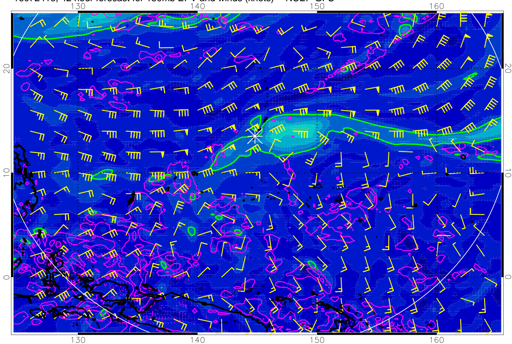
16072418, 42 hour forecast for 150mb EPV and winds (knots) -- NCEP GFS
