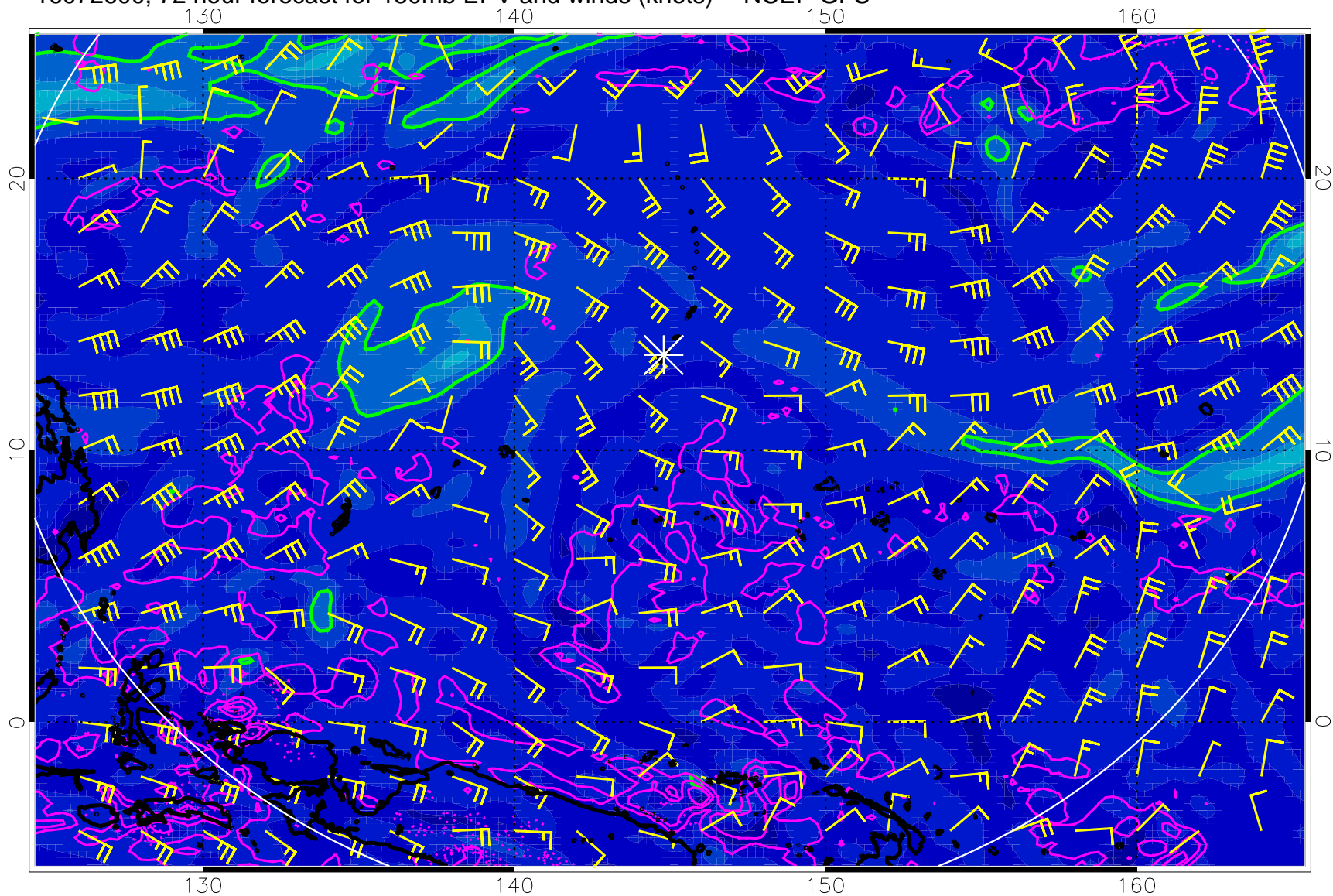
16072600, 72 hour forecast for 150mb EPV and winds (knots) -- NCEP GFS
