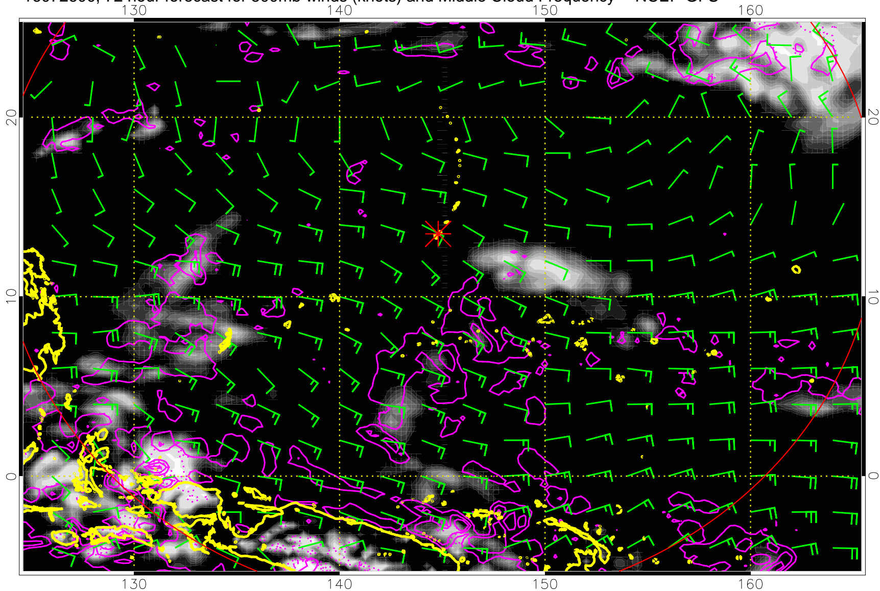
16072600, 72 hour forecast for 500mb winds (knots) and Middle Cloud Frequency -- NCEP GFS
