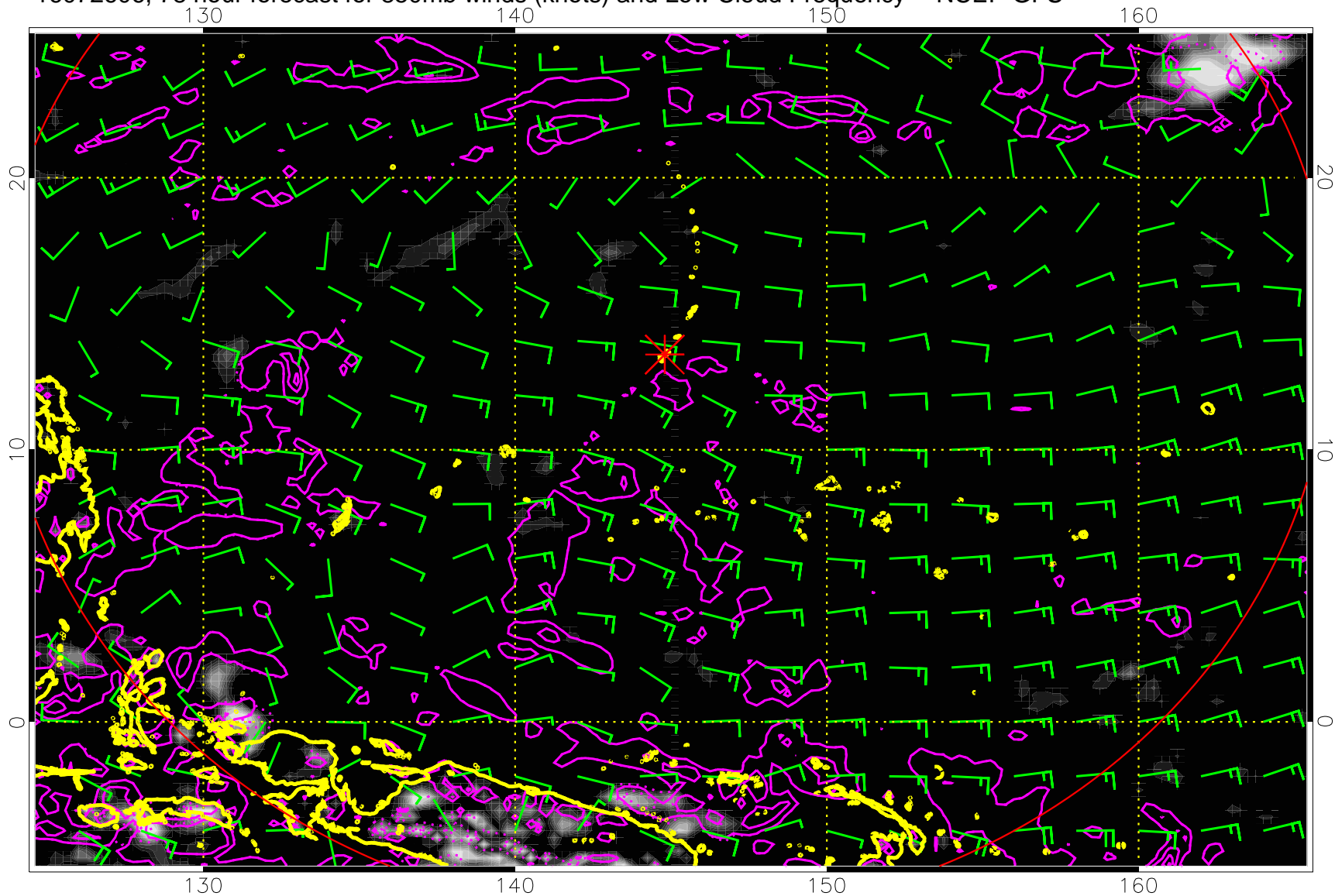
16072606, 78 hour forecast for 850mb winds (knots) and Low Cloud Frequency -- NCEP GFS
