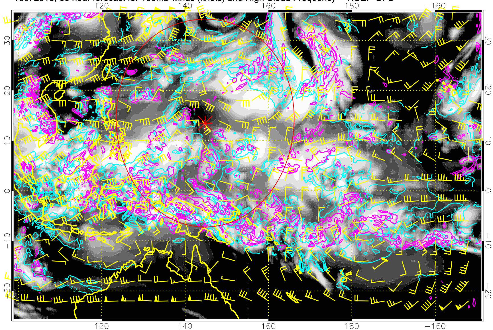
16072518, 66 hour forecast for 150mb winds (knots) and High Cloud Frequency -- NCEP GFS
