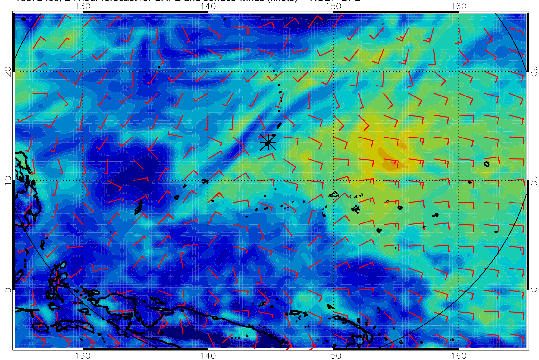
16072400, 24 hour forecast for CAPE and surface winds (knots) -- NCEP GFS
