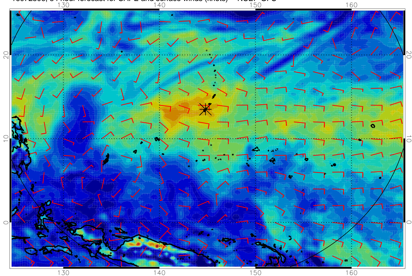
16072506, 54 hour forecast for CAPE and surface winds (knots) -- NCEP GFS
