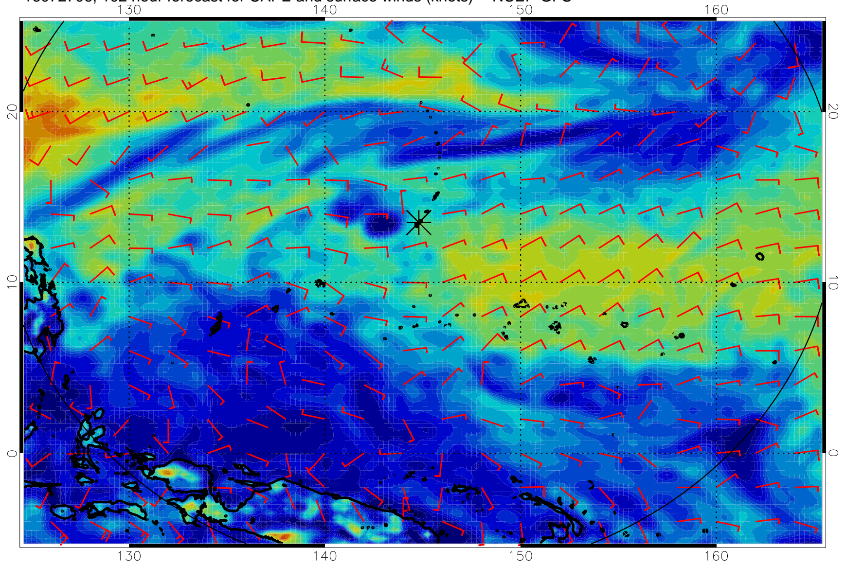
16072706, 102 hour forecast for CAPE and surface winds (knots) -- NCEP GFS
