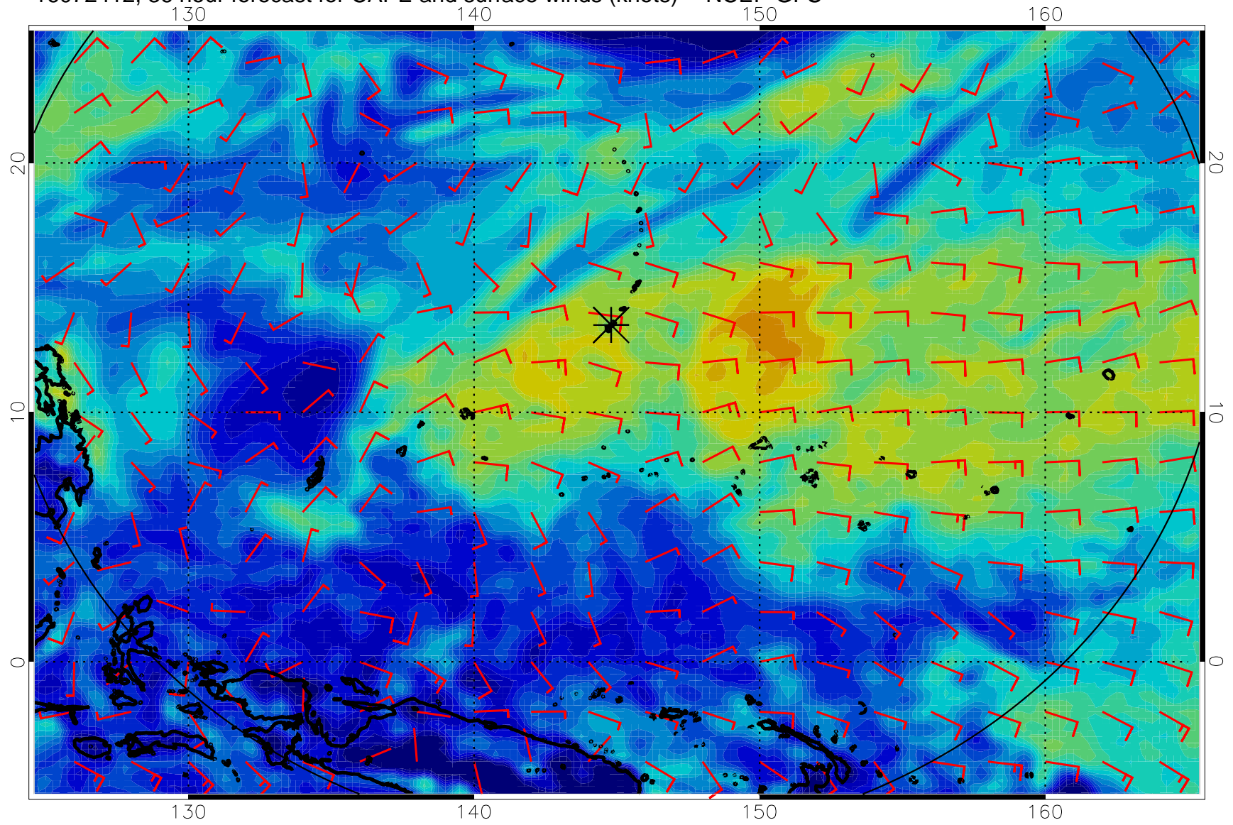
16072412, 36 hour forecast for CAPE and surface winds (knots) -- NCEP GFS
