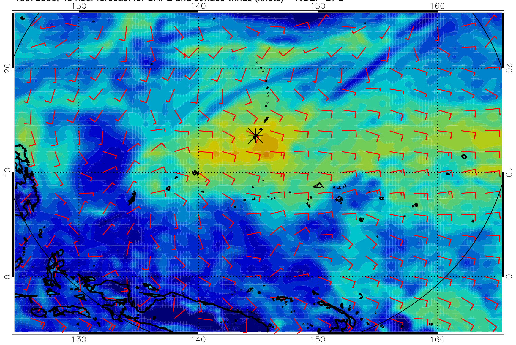
16072500, 48 hour forecast for CAPE and surface winds (knots) -- NCEP GFS
