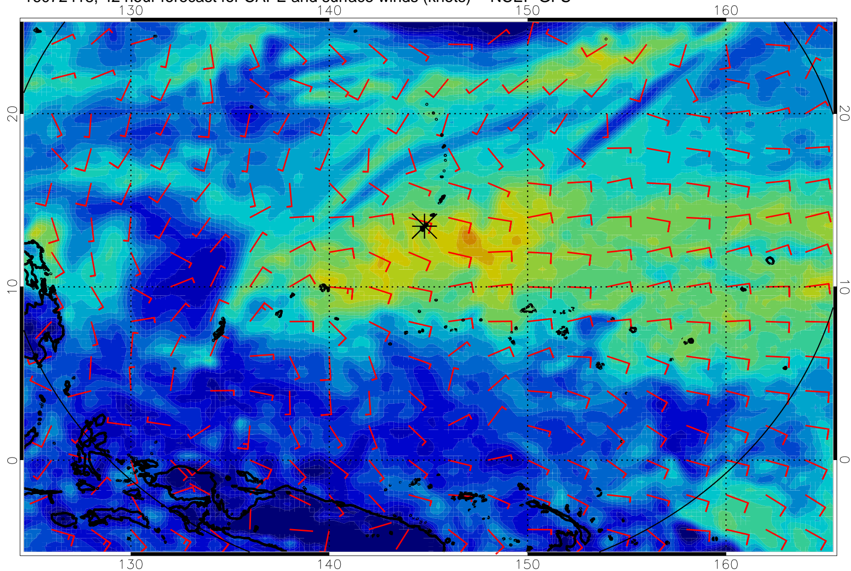
16072418, 42 hour forecast for CAPE and surface winds (knots) -- NCEP GFS
