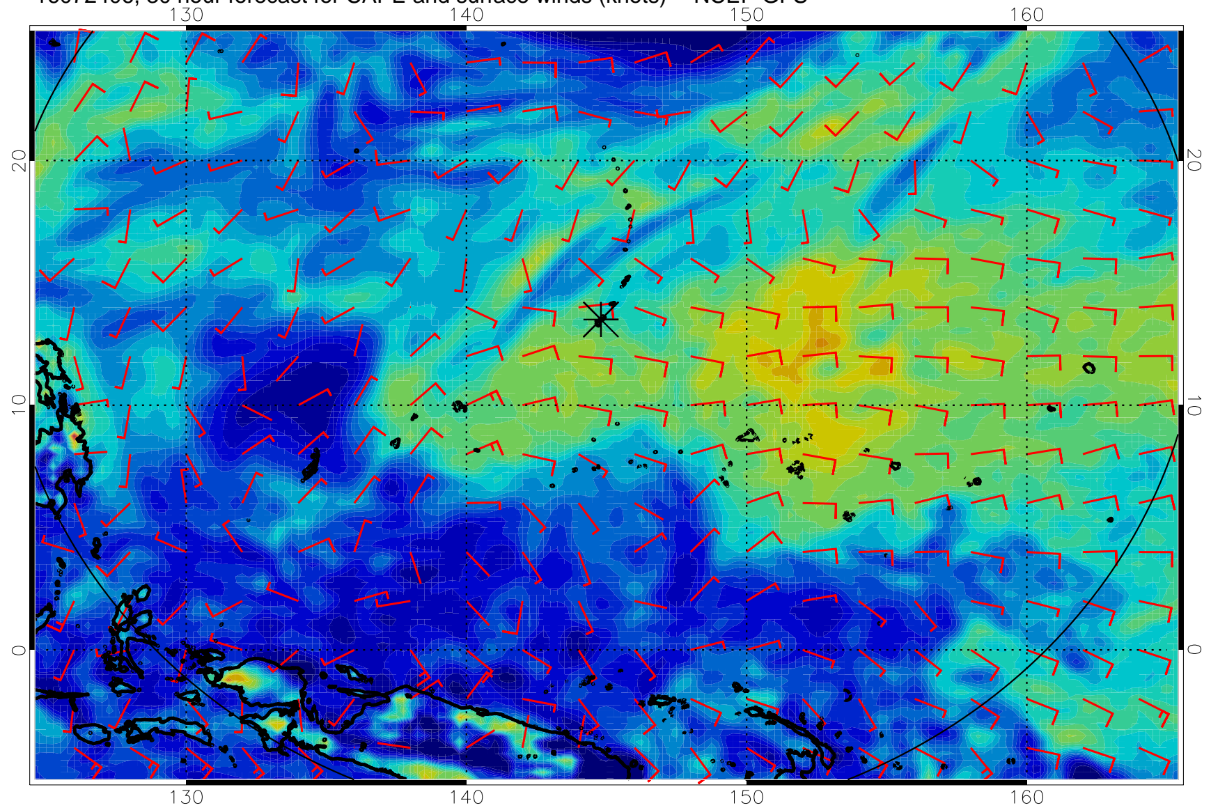
16072406, 30 hour forecast for CAPE and surface winds (knots) -- NCEP GFS
