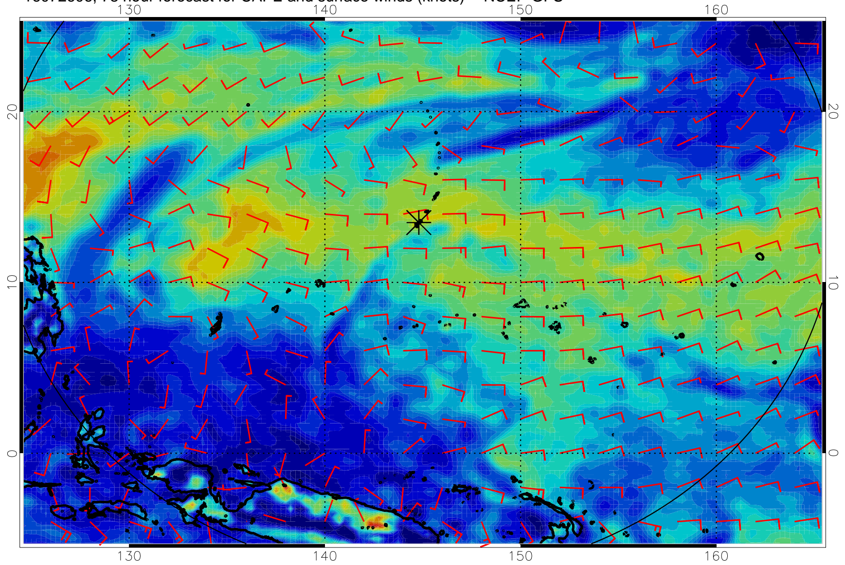
16072606, 78 hour forecast for CAPE and surface winds (knots) -- NCEP GFS
