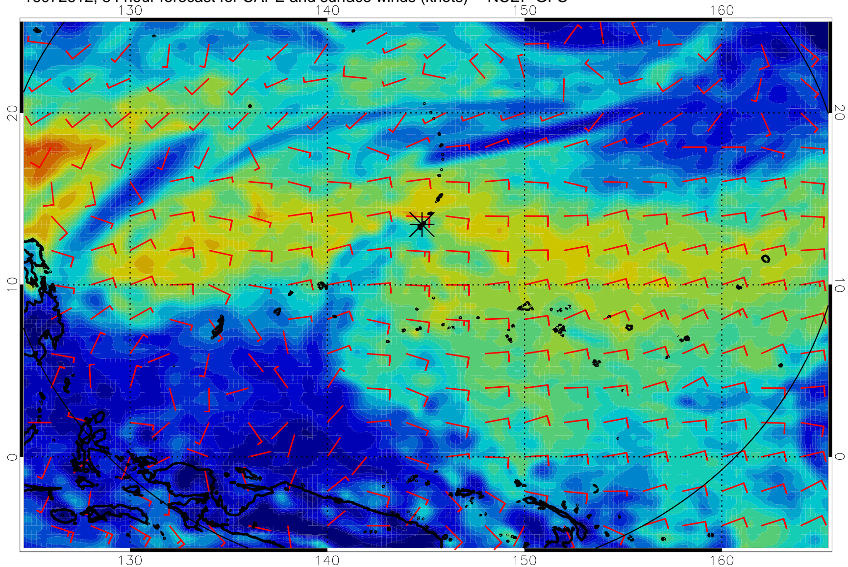
16072612, 84 hour forecast for CAPE and surface winds (knots) -- NCEP GFS
