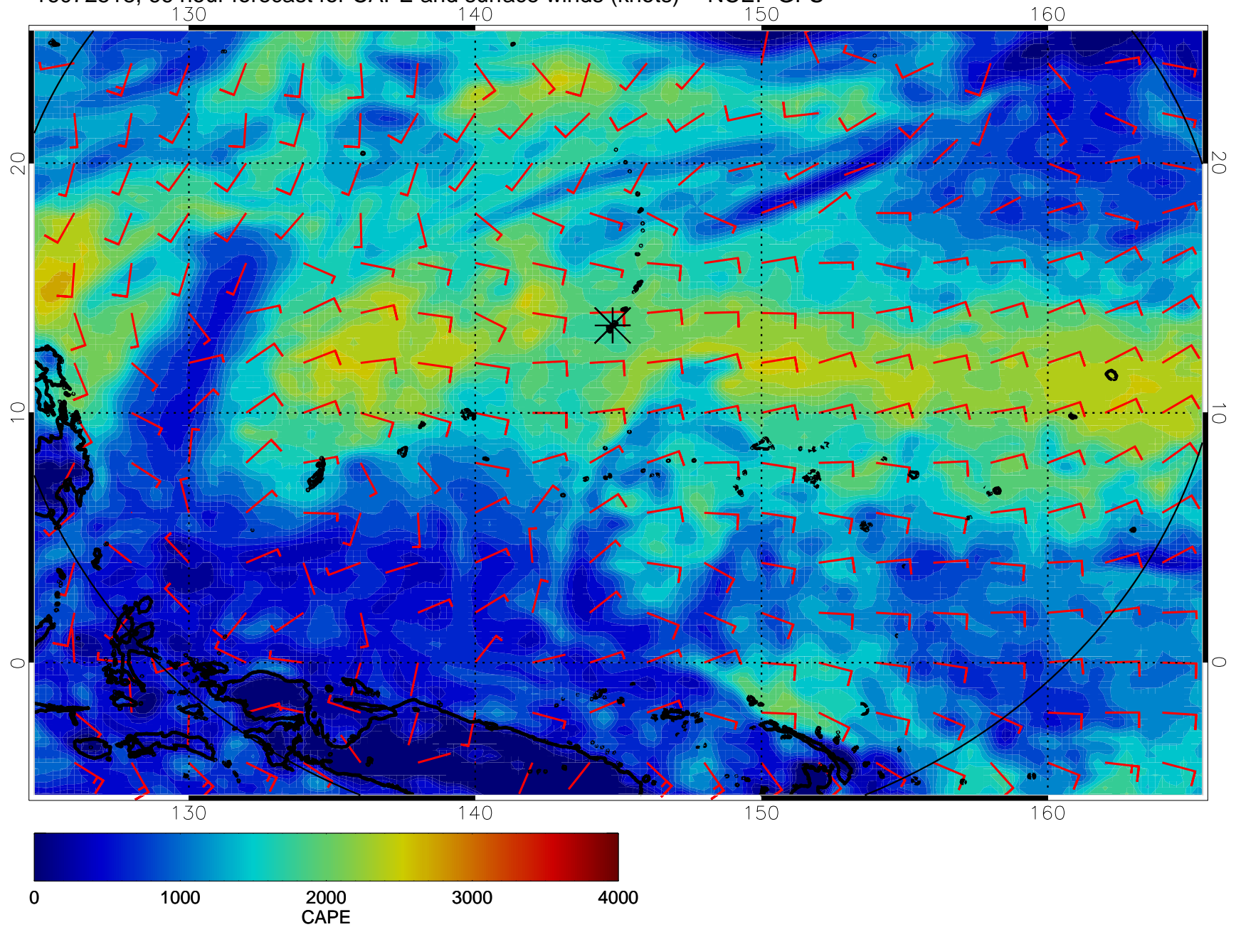
16072518, 66 hour forecast for CAPE and surface winds (knots) -- NCEP GFS
