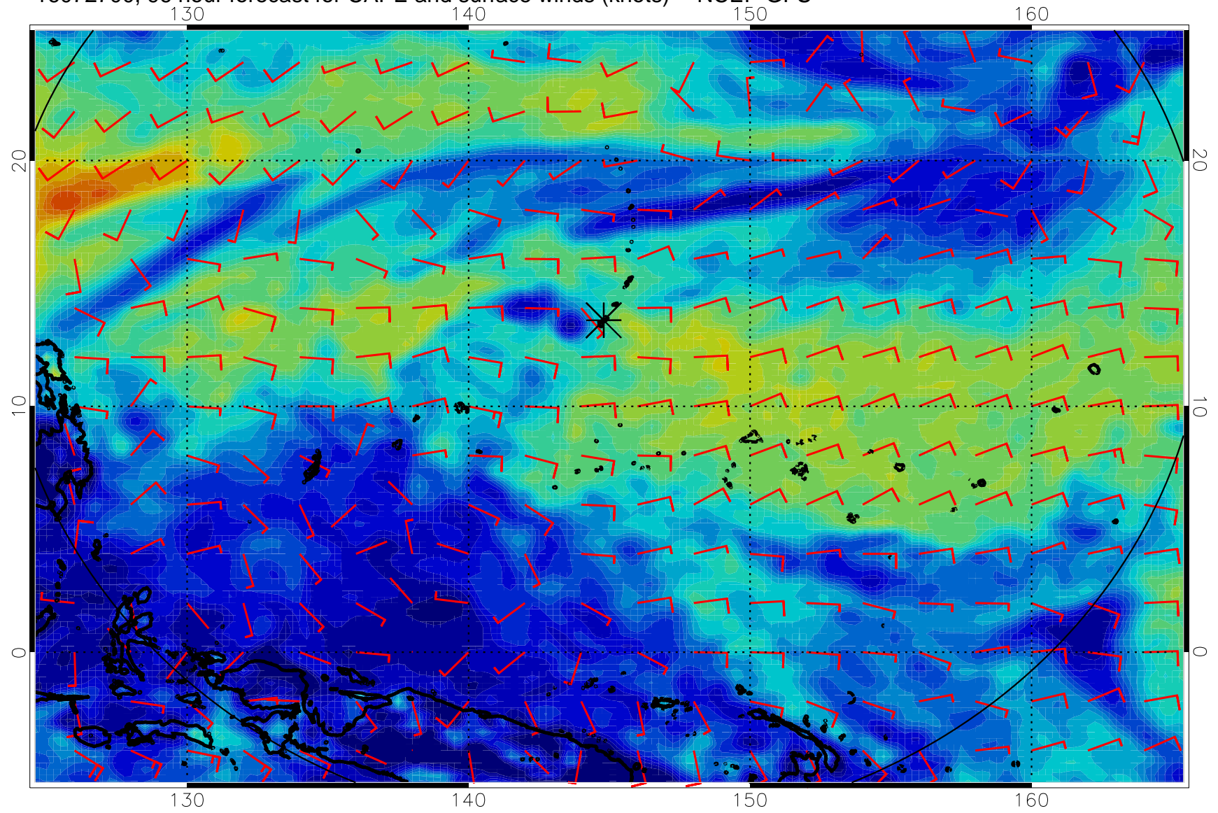
16072700, 96 hour forecast for CAPE and surface winds (knots) -- NCEP GFS
