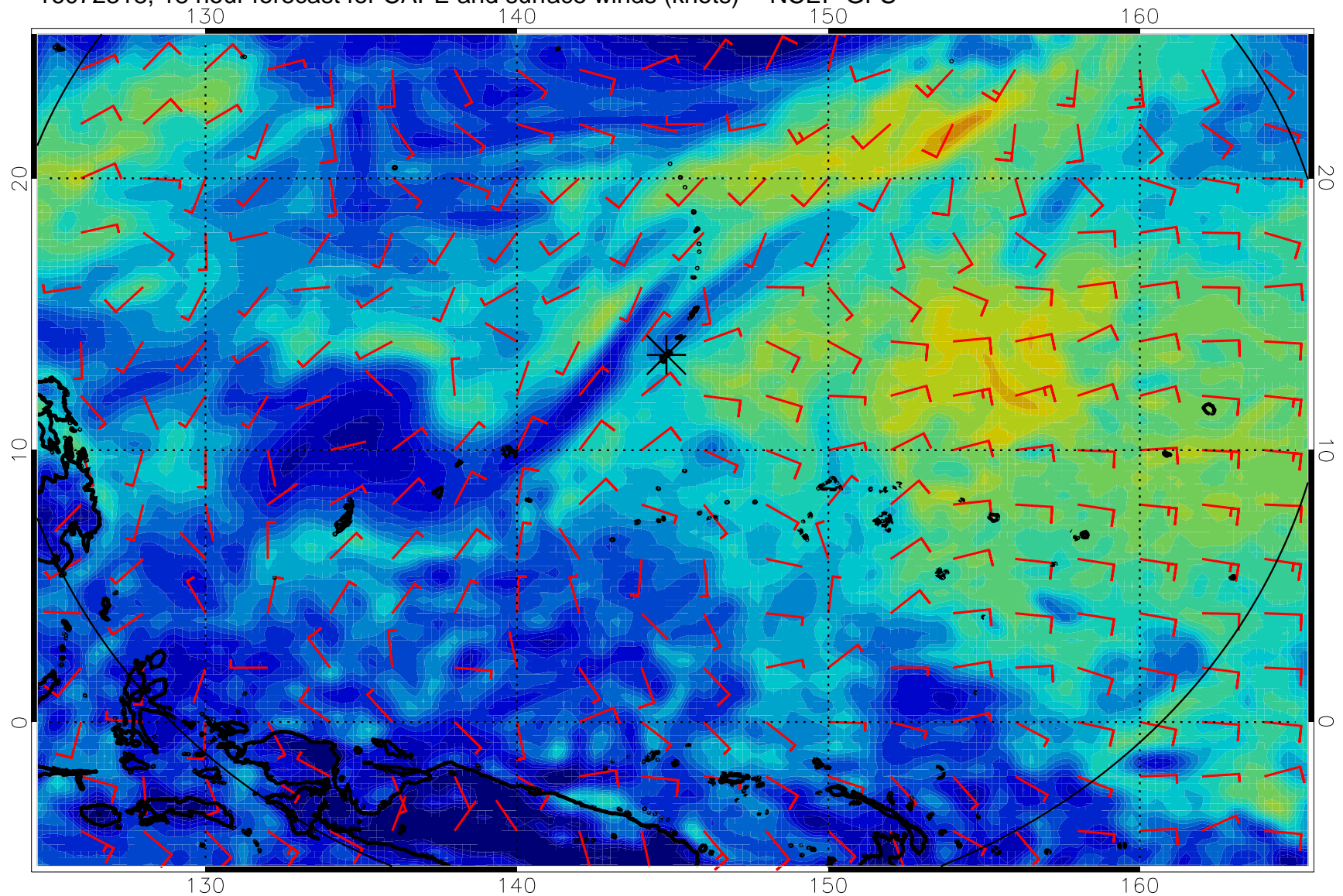
16072318, 18 hour forecast for CAPE and surface winds (knots) -- NCEP GFS
