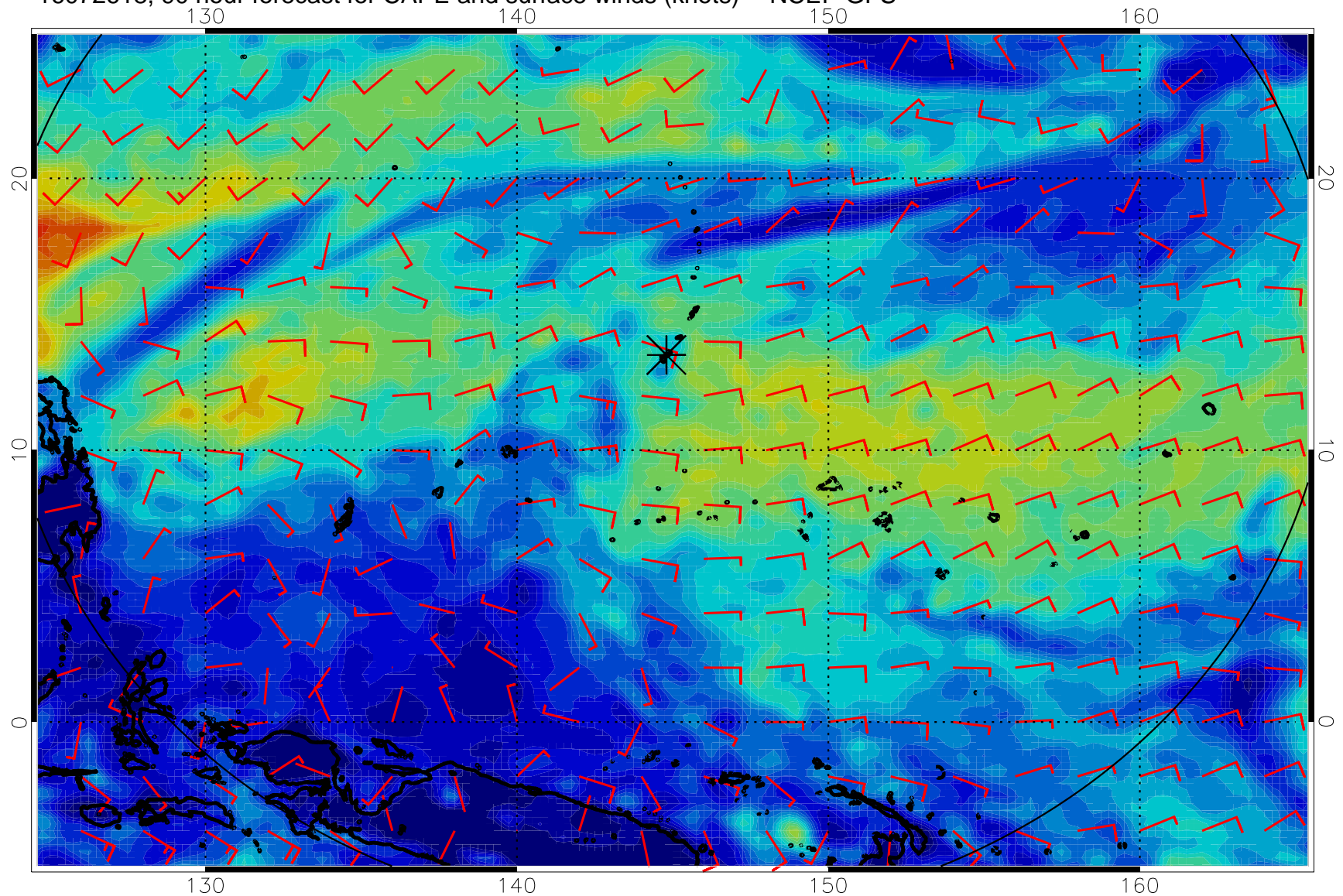
16072618, 90 hour forecast for CAPE and surface winds (knots) -- NCEP GFS
