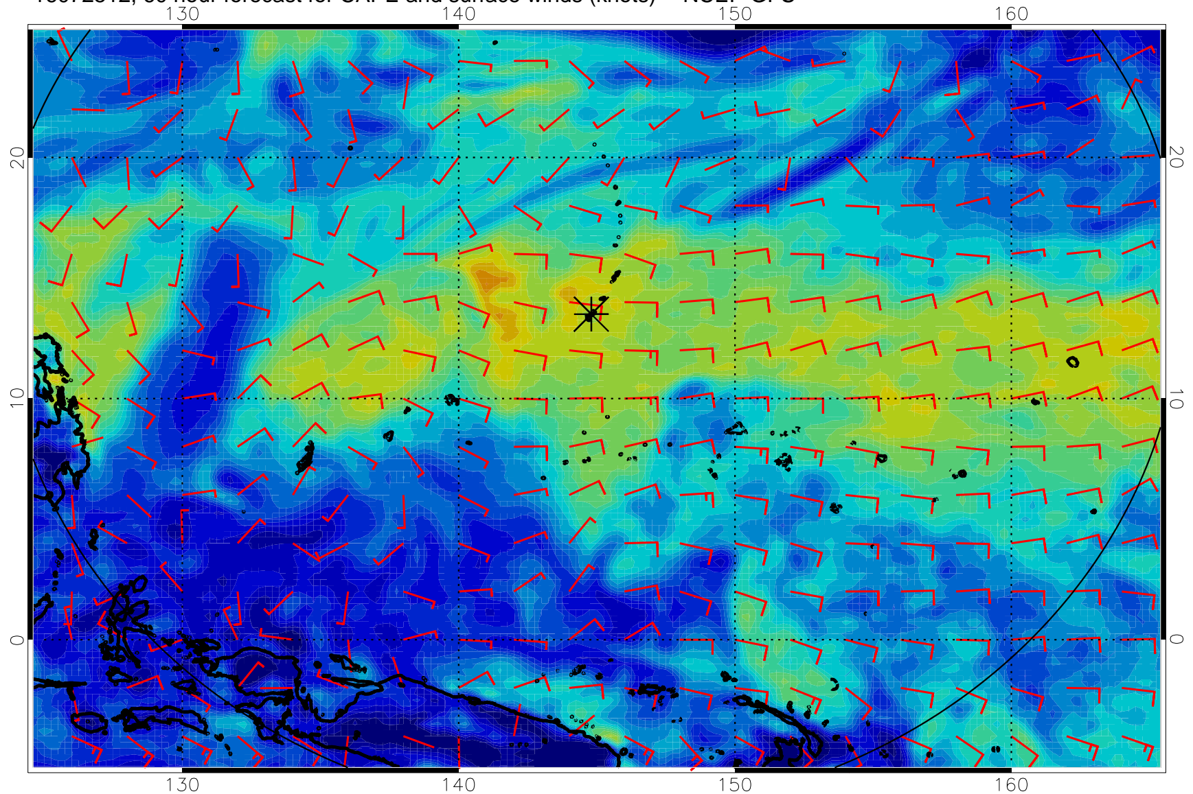
16072512, 60 hour forecast for CAPE and surface winds (knots) -- NCEP GFS
