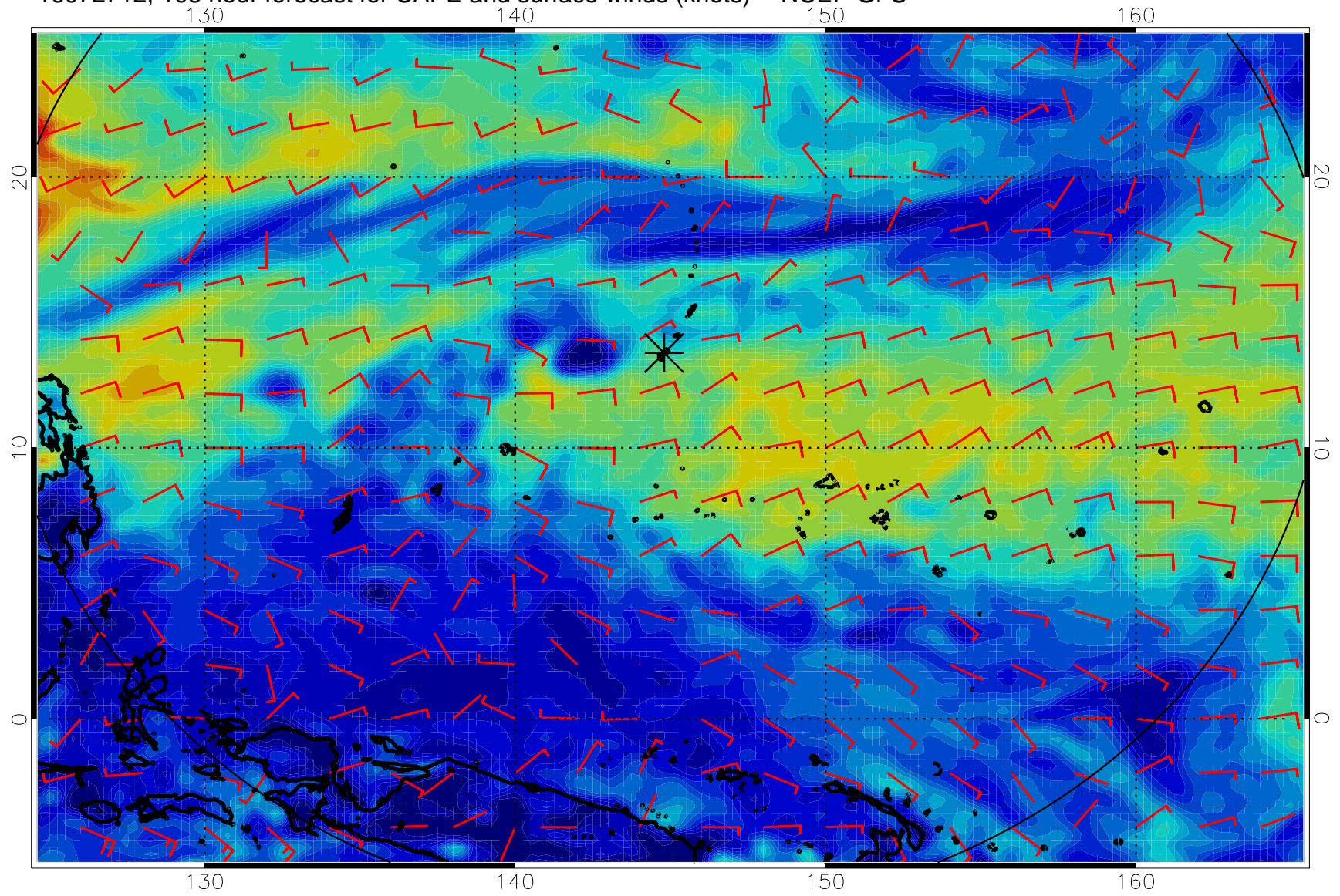
16072712, 108 hour forecast for CAPE and surface winds (knots) -- NCEP GFS
