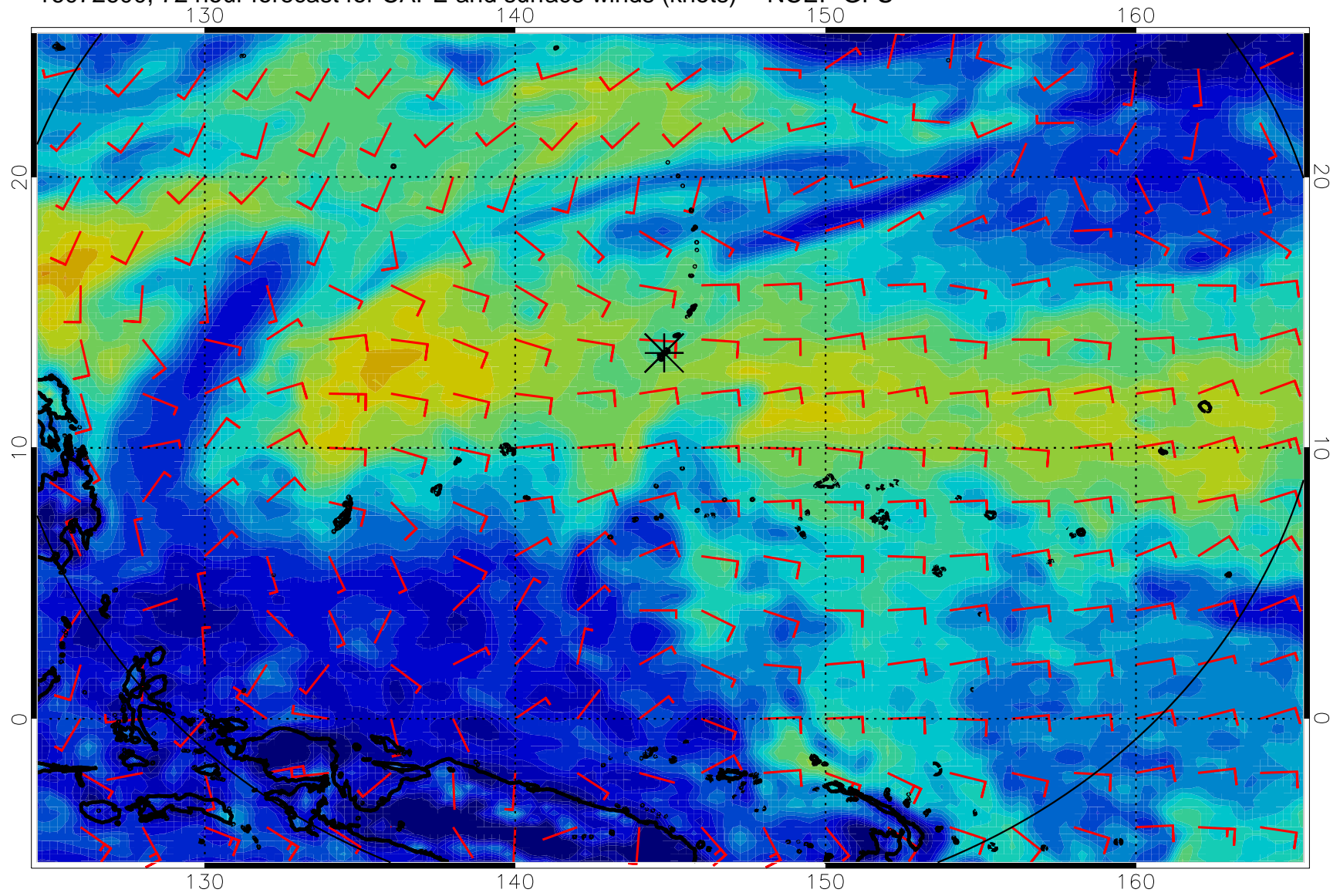
16072600, 72 hour forecast for CAPE and surface winds (knots) -- NCEP GFS
