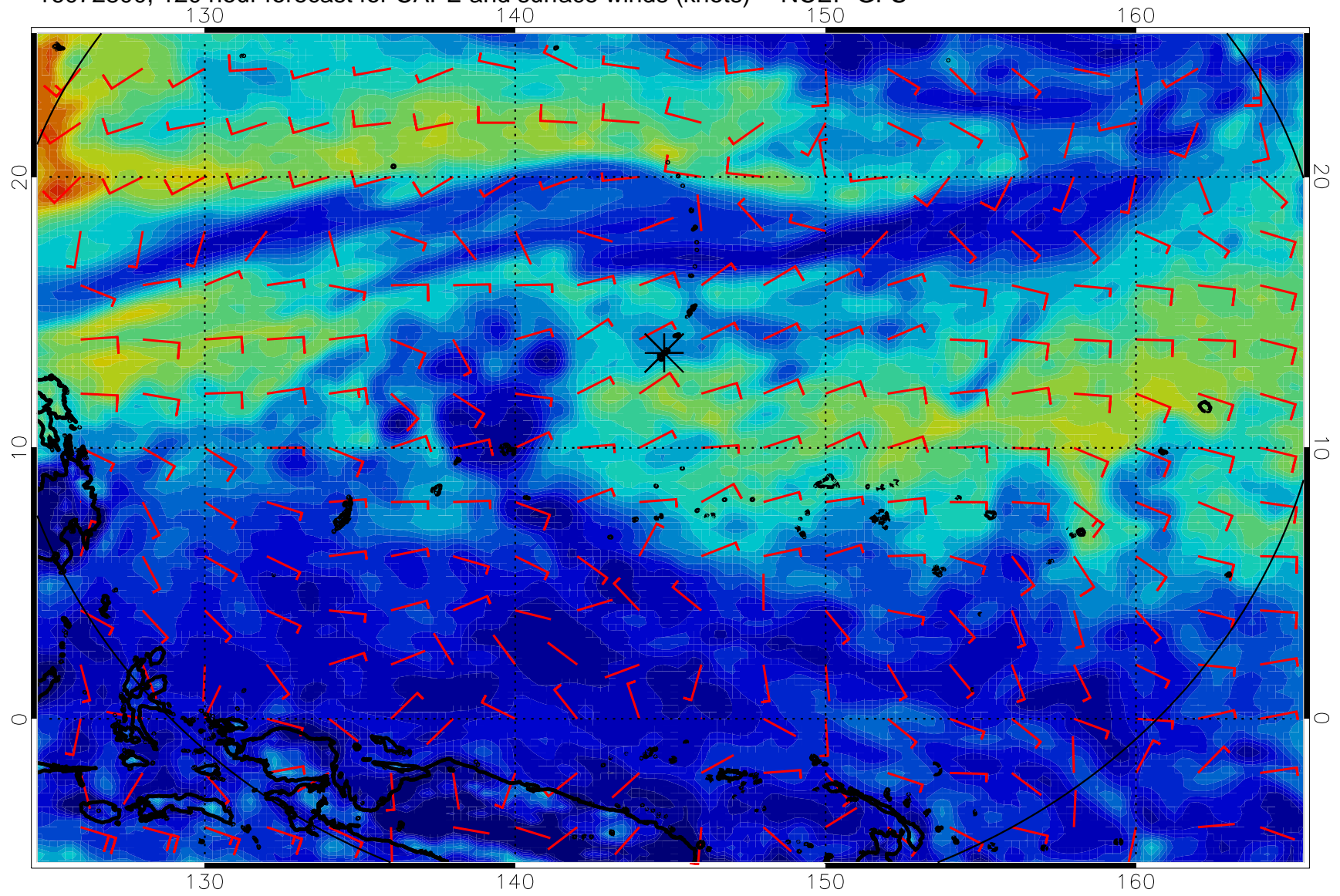
16072800, 120 hour forecast for CAPE and surface winds (knots) -- NCEP GFS
