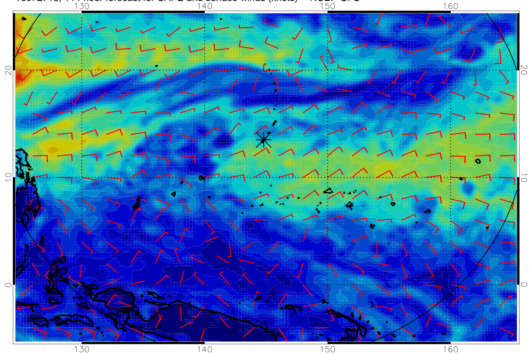
16072718, 114 hour forecast for CAPE and surface winds (knots) -- NCEP GFS
