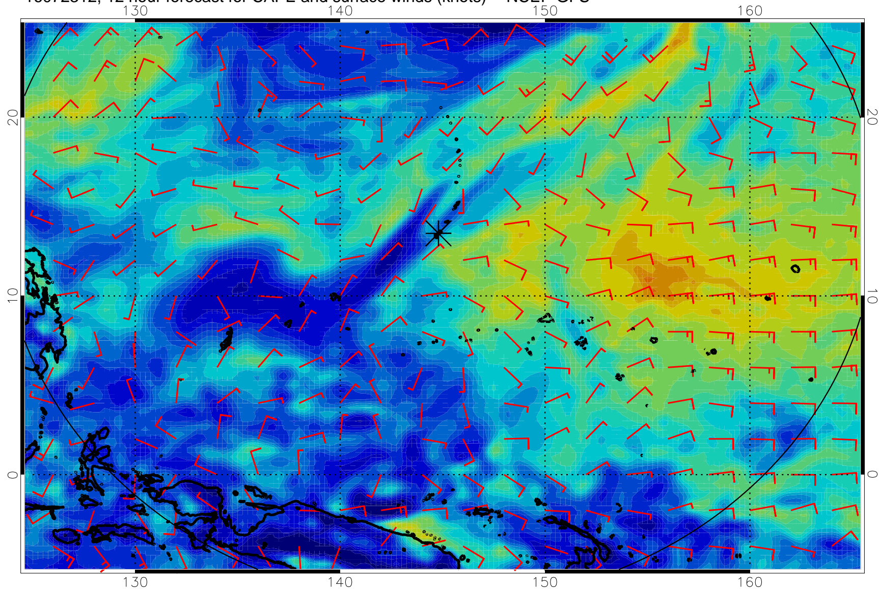
16072312, 12 hour forecast for CAPE and surface winds (knots) -- NCEP GFS
