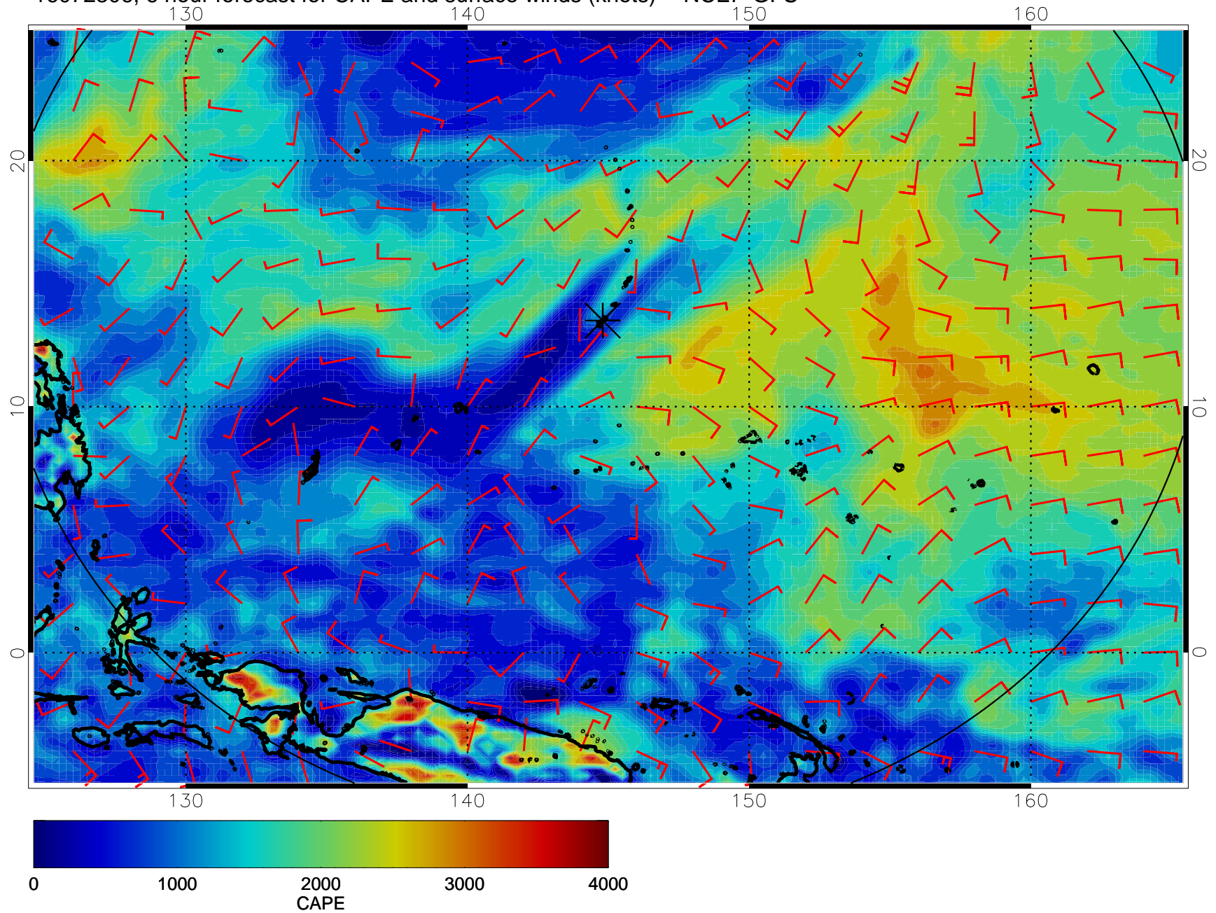
16072306, 6 hour forecast for CAPE and surface winds (knots) -- NCEP GFS
