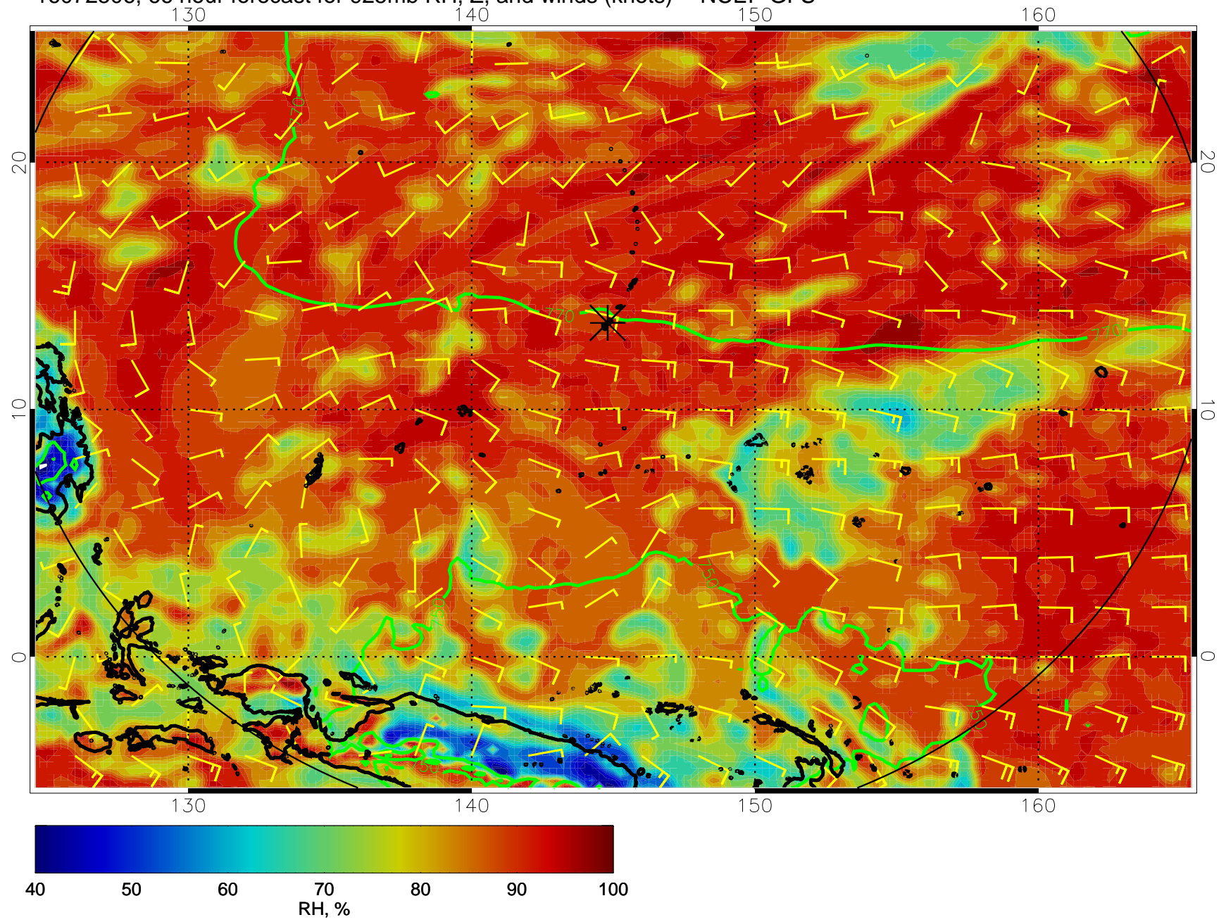
16072506, 66 hour forecast for 925mb RH, Z, and winds (knots) -- NCEP GFS
