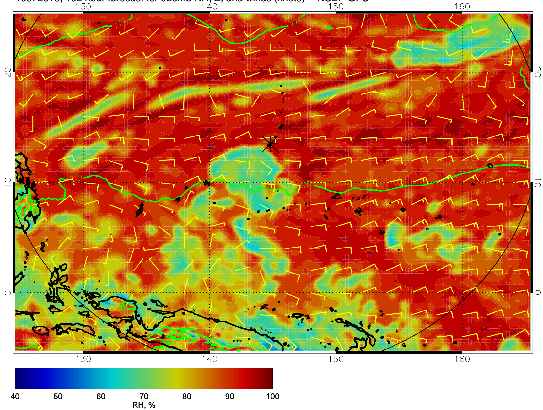
16072618, 102 hour forecast for 925mb RH, Z, and winds (knots) -- NCEP GFS
