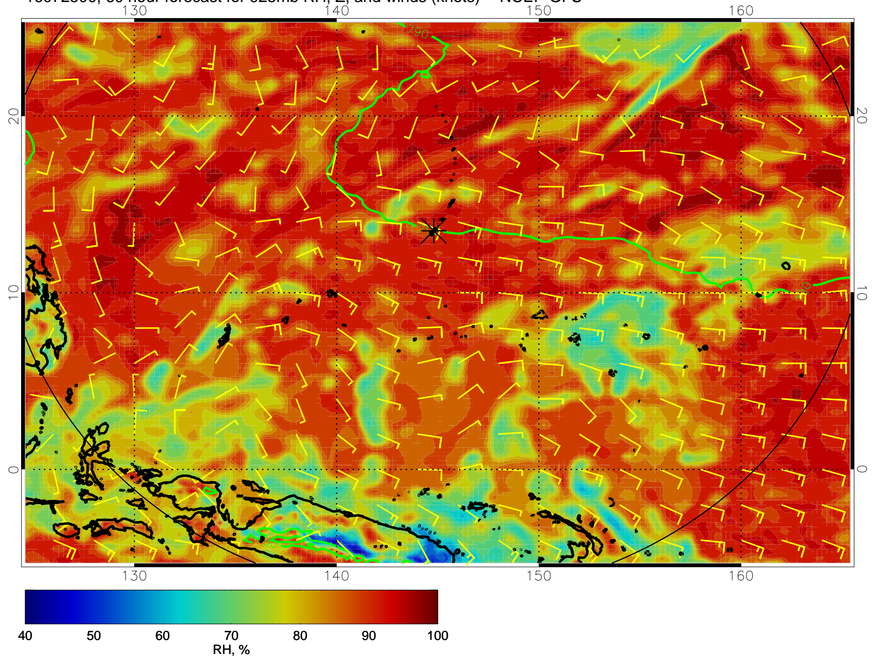
16072500, 60 hour forecast for 925mb RH, Z, and winds (knots) -- NCEP GFS
