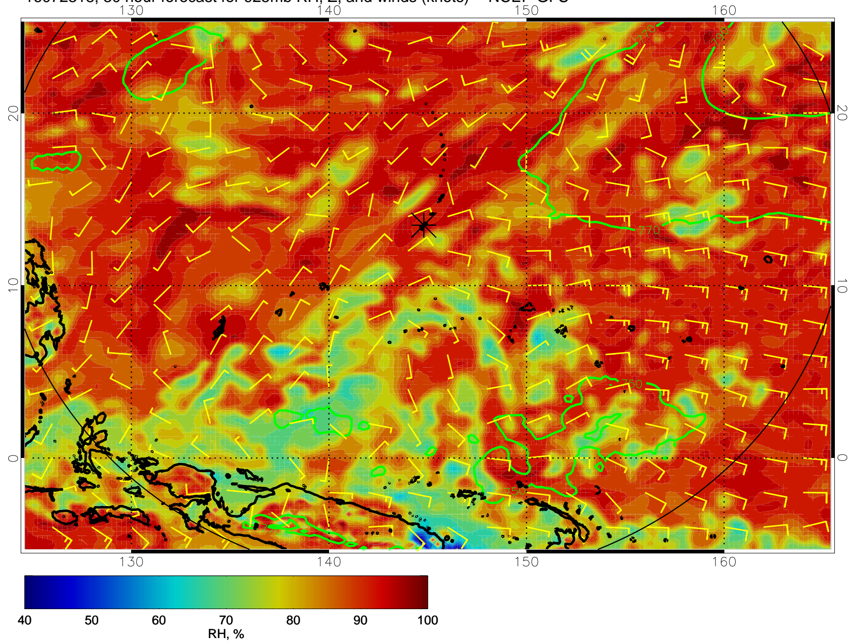
16072318, 30 hour forecast for 925mb RH, Z, and winds (knots) -- NCEP GFS
