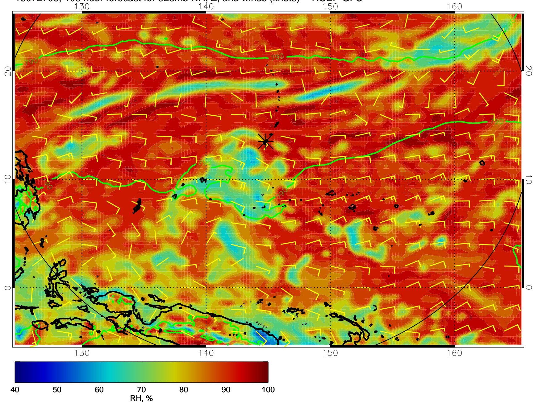
16072700, 108 hour forecast for 925mb RH, Z, and winds (knots) -- NCEP GFS
