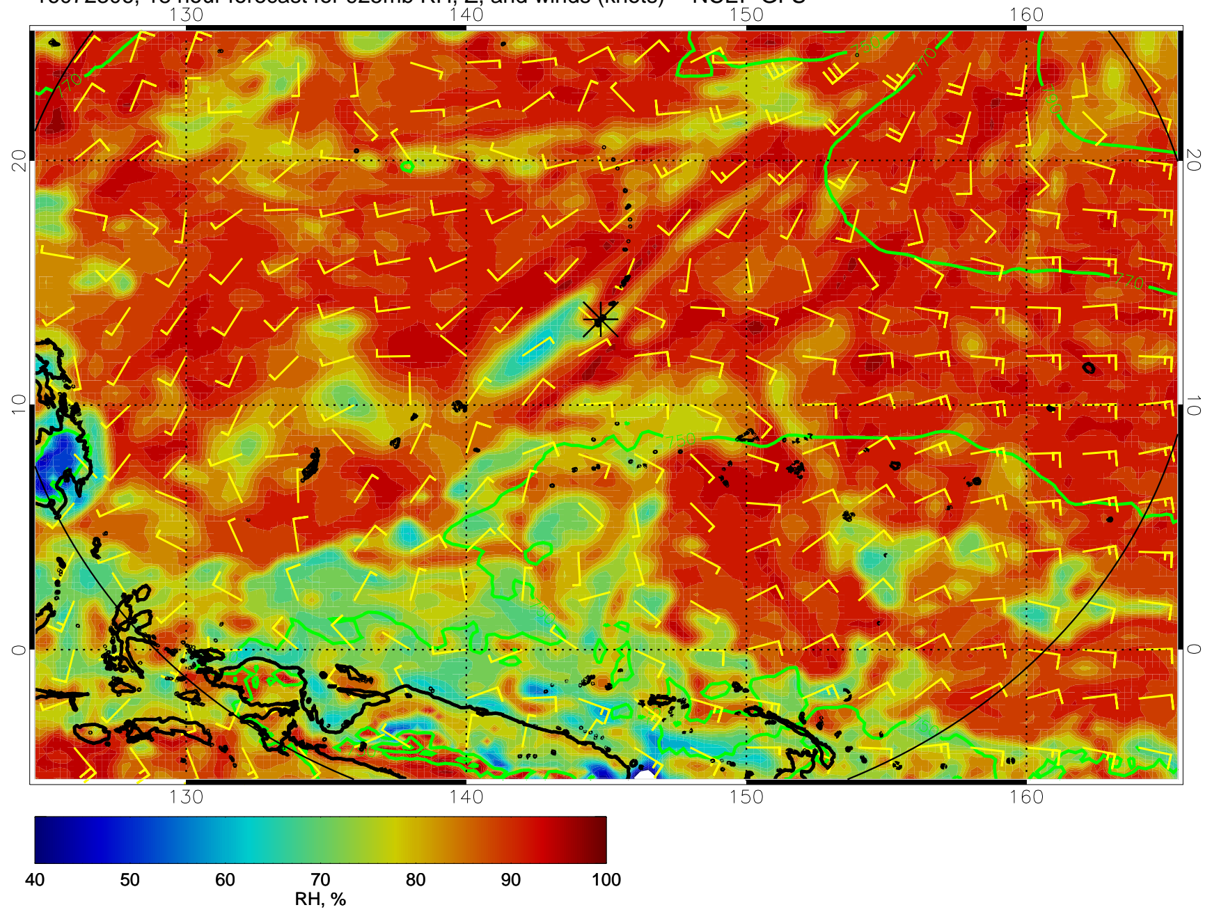
16072306, 18 hour forecast for 925mb RH, Z, and winds (knots) -- NCEP GFS
