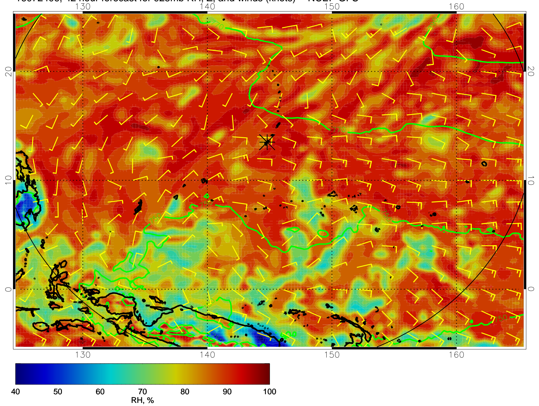
16072406, 42 hour forecast for 925mb RH, Z, and winds (knots) -- NCEP GFS
