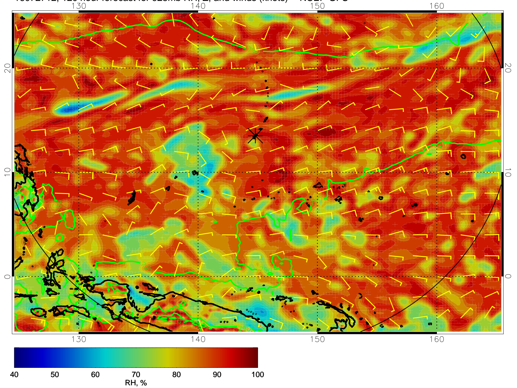
16072712, 120 hour forecast for 925mb RH, Z, and winds (knots) -- NCEP GFS
