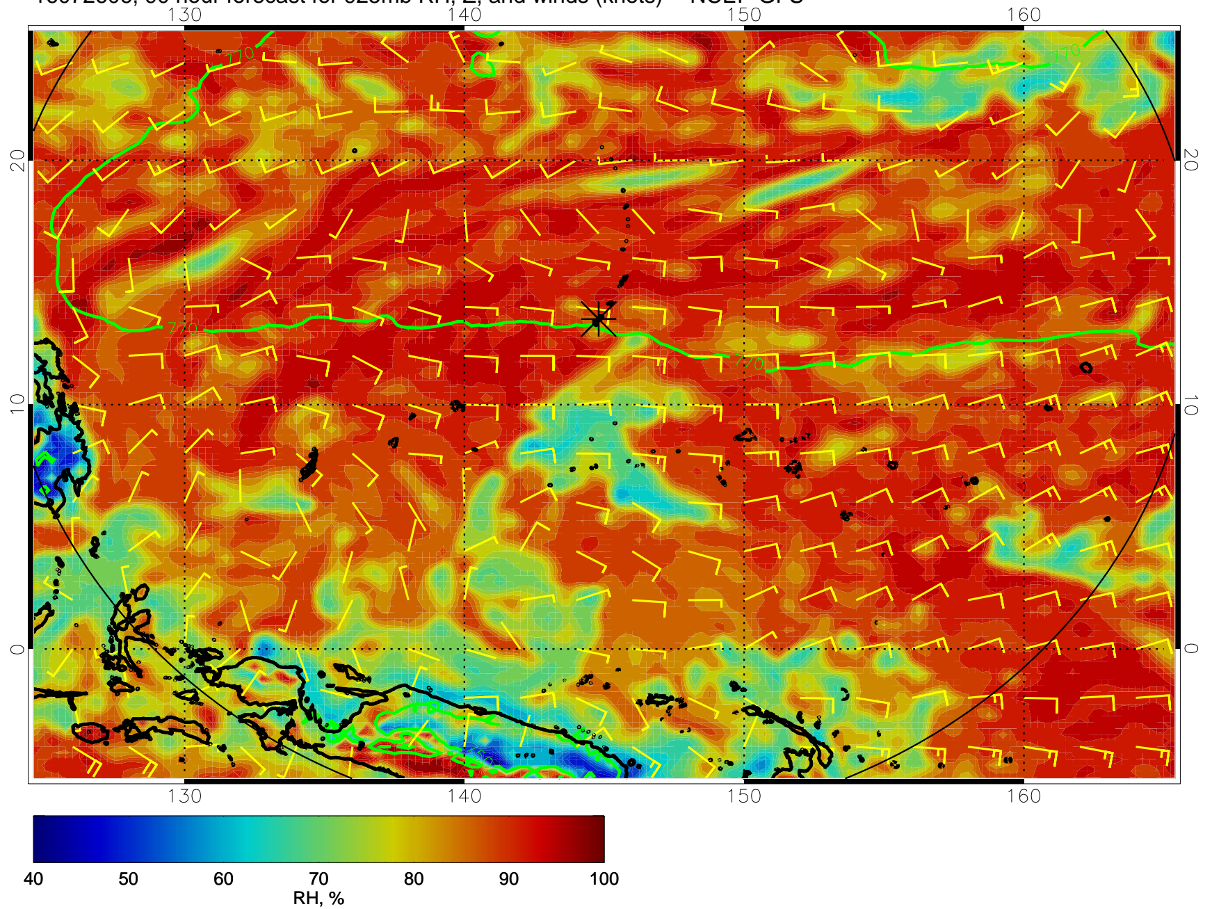
16072606, 90 hour forecast for 925mb RH, Z, and winds (knots) -- NCEP GFS
