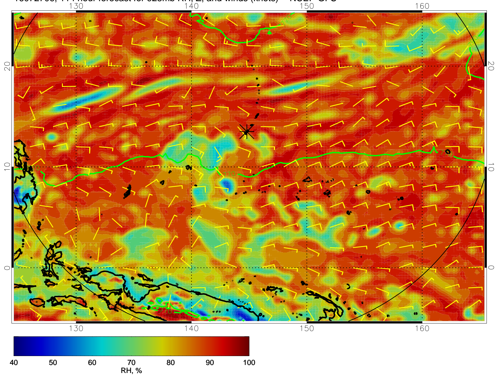
16072706, 114 hour forecast for 925mb RH, Z, and winds (knots) -- NCEP GFS
