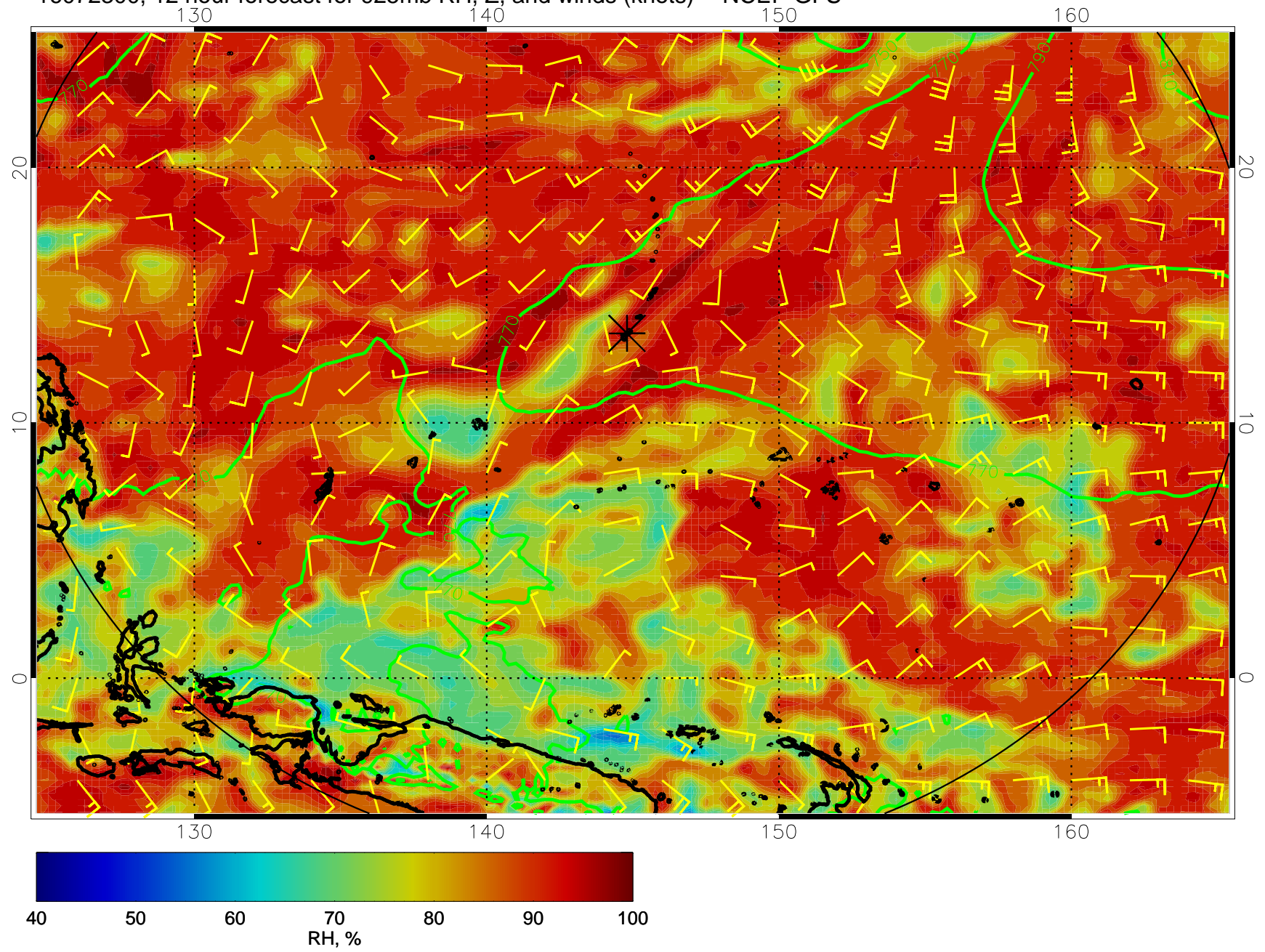
16072300, 12 hour forecast for 925mb RH, Z, and winds (knots) -- NCEP GFS
