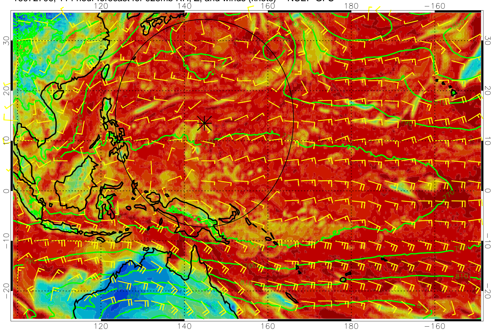
16072706, 114 hour forecast for 925mb RH, Z, and winds (knots) -- NCEP GFS
