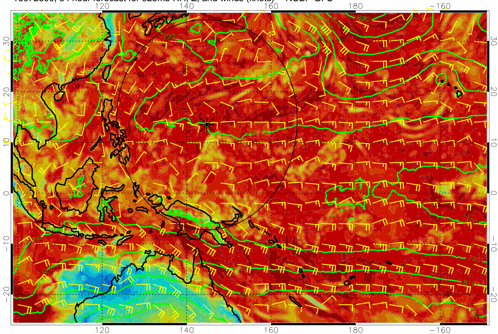
16072600, 84 hour forecast for 925mb RH, Z, and winds (knots) -- NCEP GFS
