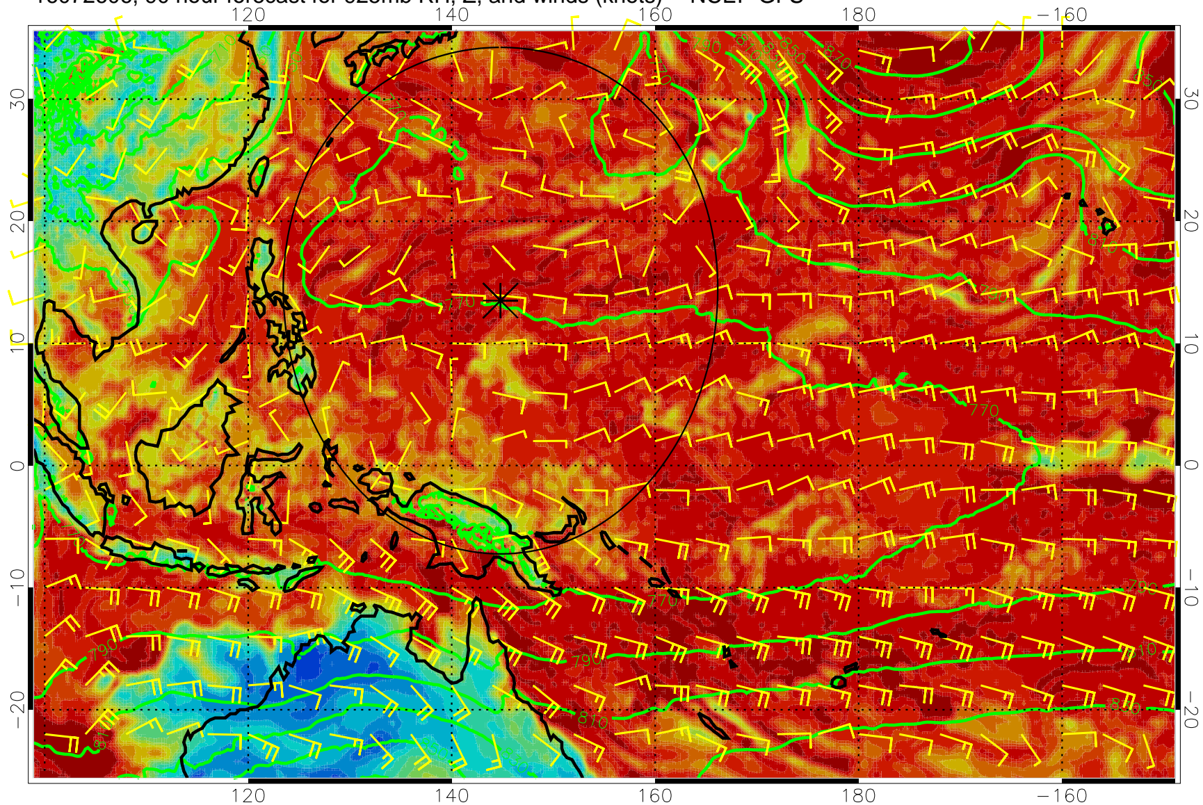
16072606, 90 hour forecast for 925mb RH, Z, and winds (knots) -- NCEP GFS
