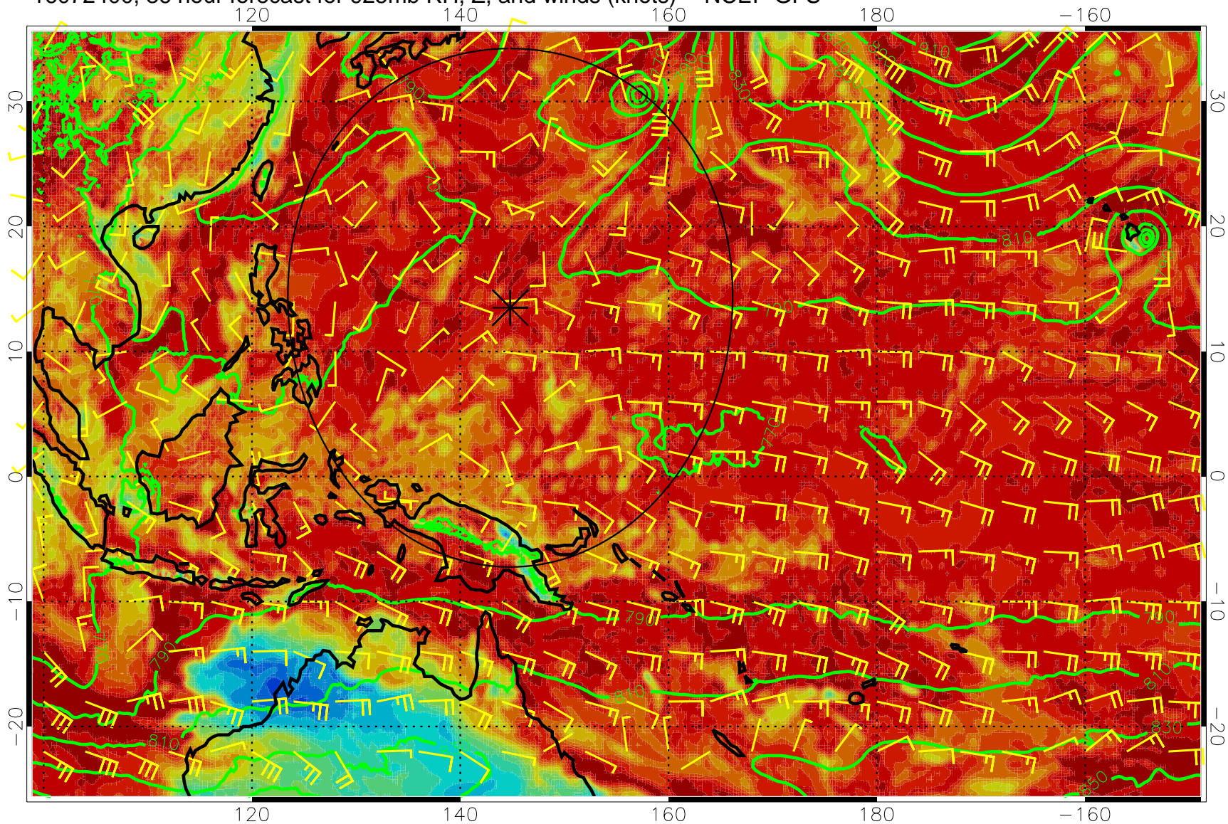
16072400, 36 hour forecast for 925mb RH, Z, and winds (knots) -- NCEP GFS
