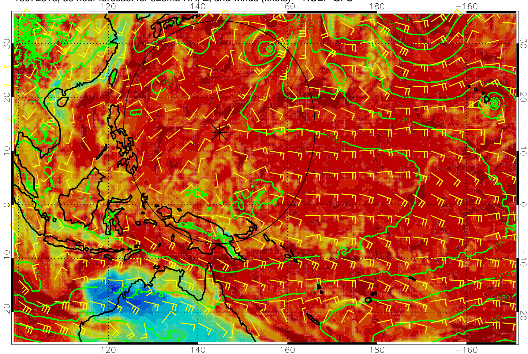
16072318, 30 hour forecast for 925mb RH, Z, and winds (knots) -- NCEP GFS
