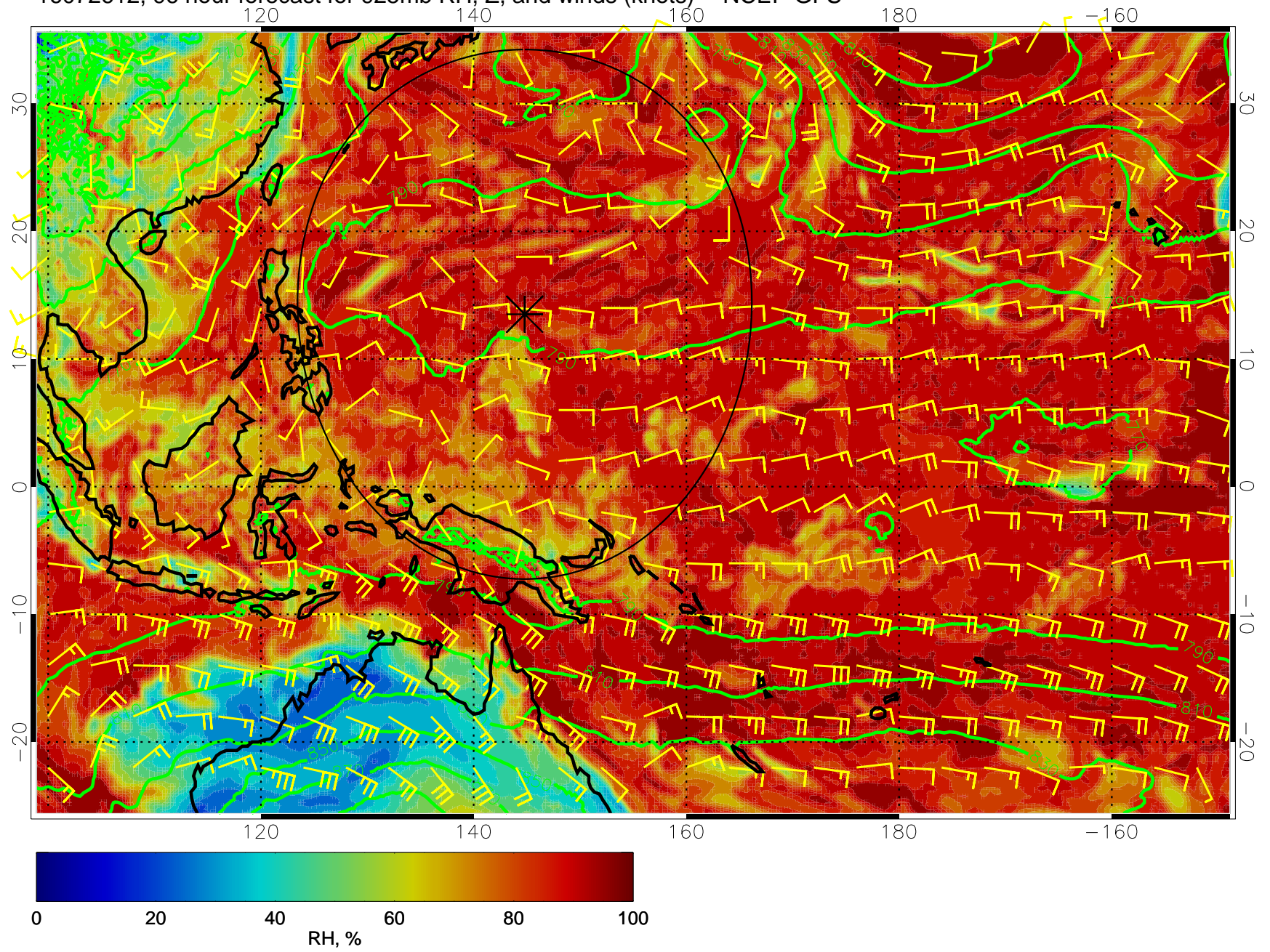
16072612, 96 hour forecast for 925mb RH, Z, and winds (knots) -- NCEP GFS
