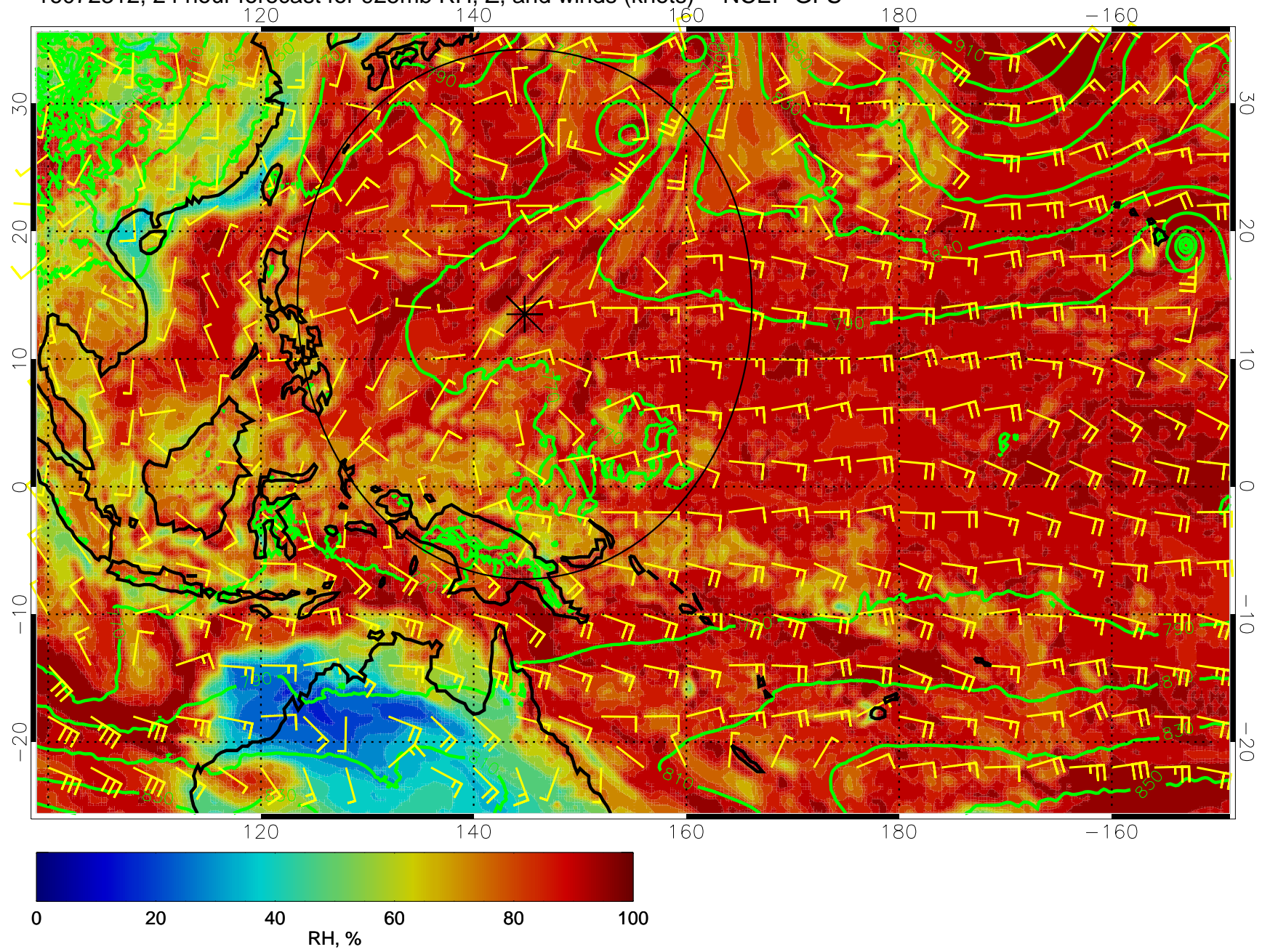
16072312, 24 hour forecast for 925mb RH, Z, and winds (knots) -- NCEP GFS
