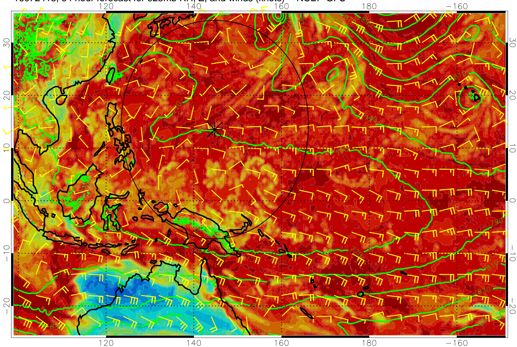
16072418, 54 hour forecast for 925mb RH, Z, and winds (knots) -- NCEP GFS
