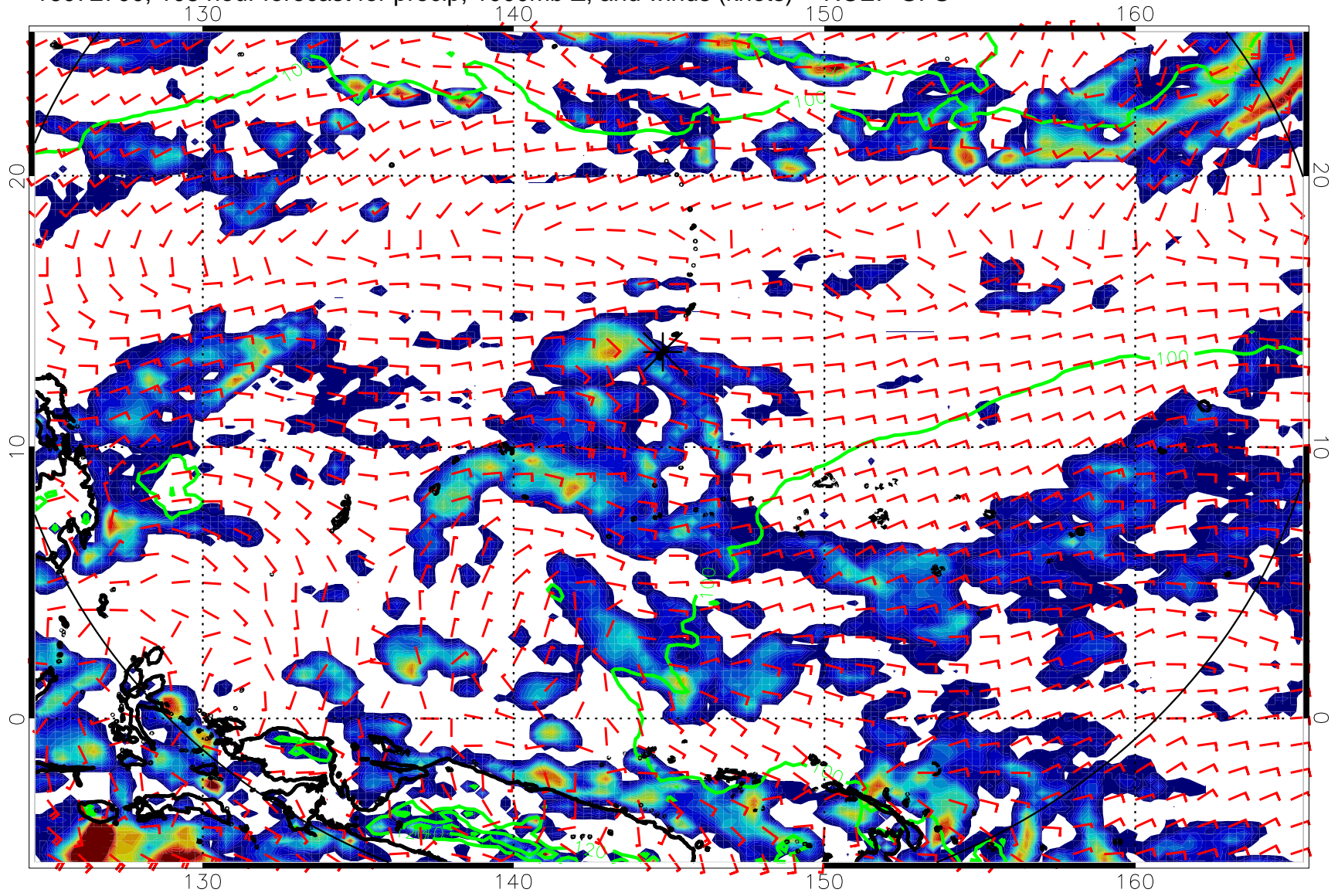
16072700, 108 hour forecast for precip, 1000mb Z, and winds (knots) -- NCEP GFS
