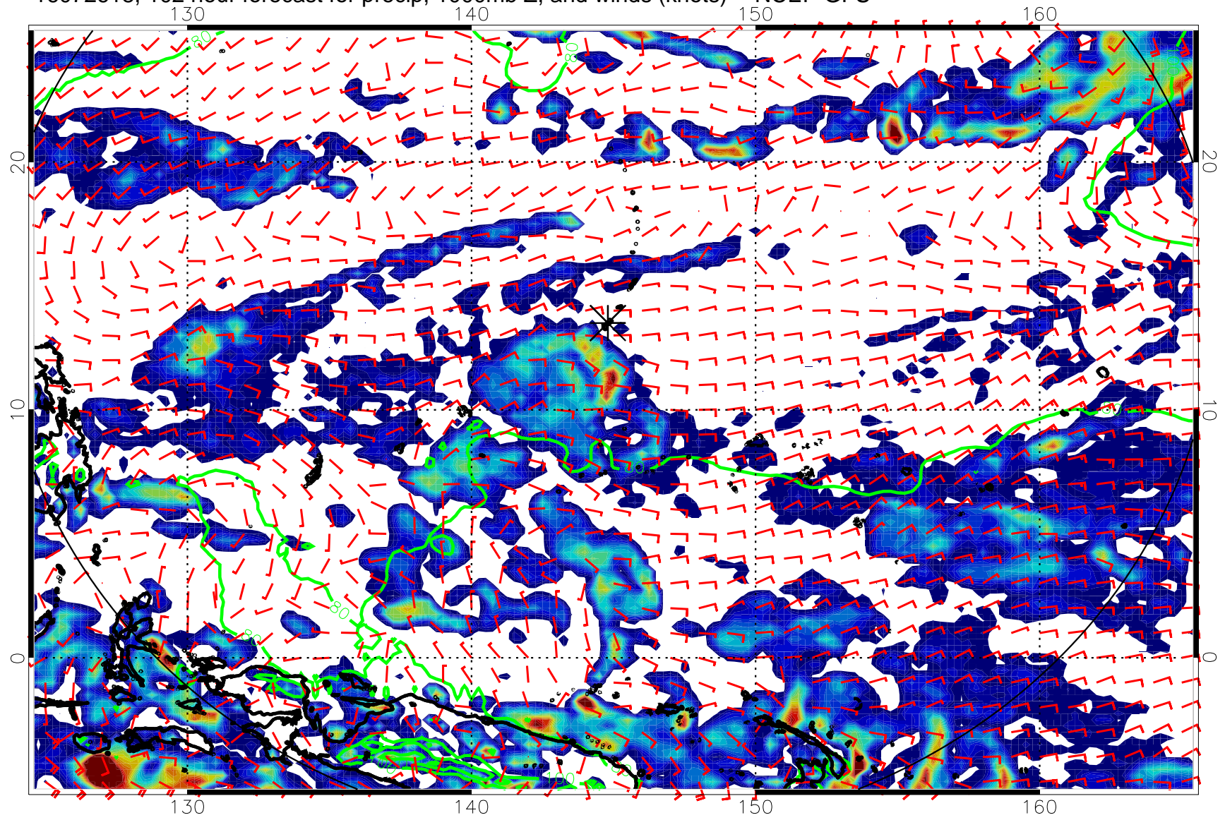
16072618, 102 hour forecast for precip, 1000mb Z, and winds (knots) -- NCEP GFS
