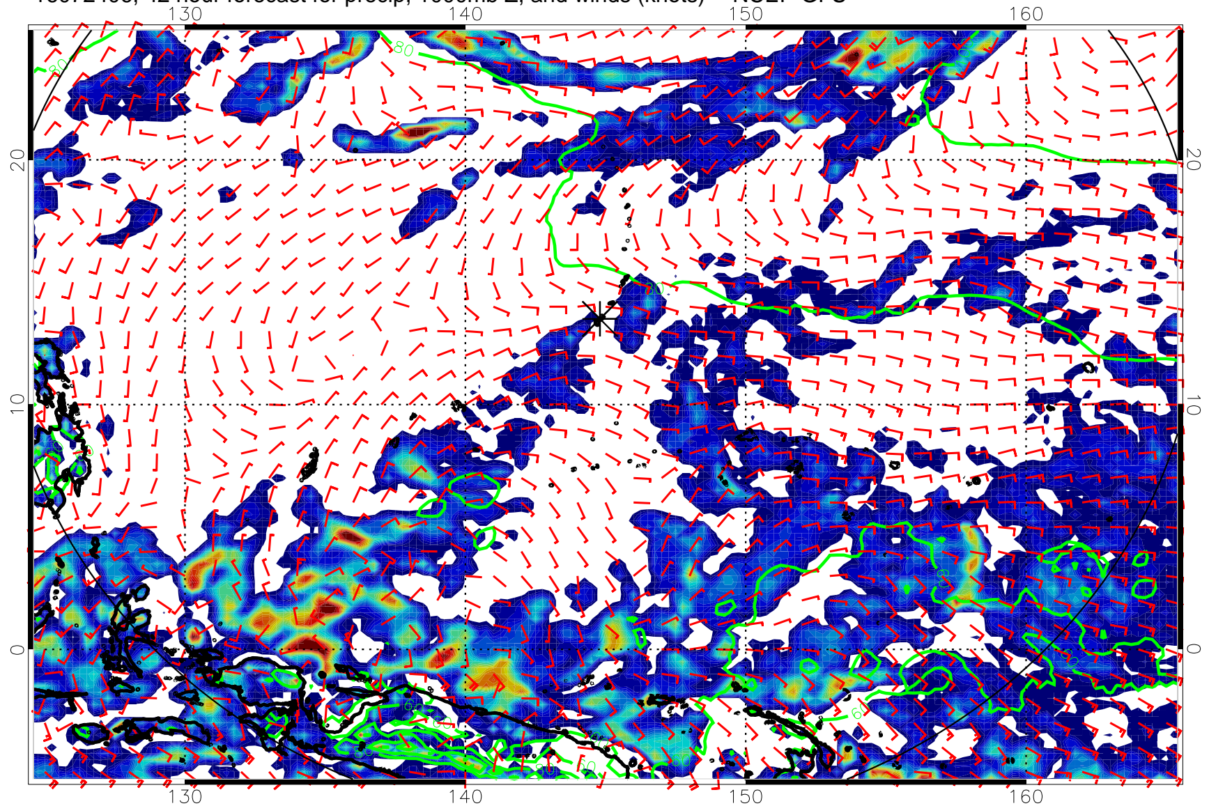
16072406, 42 hour forecast for precip, 1000mb Z, and winds (knots) -- NCEP GFS
