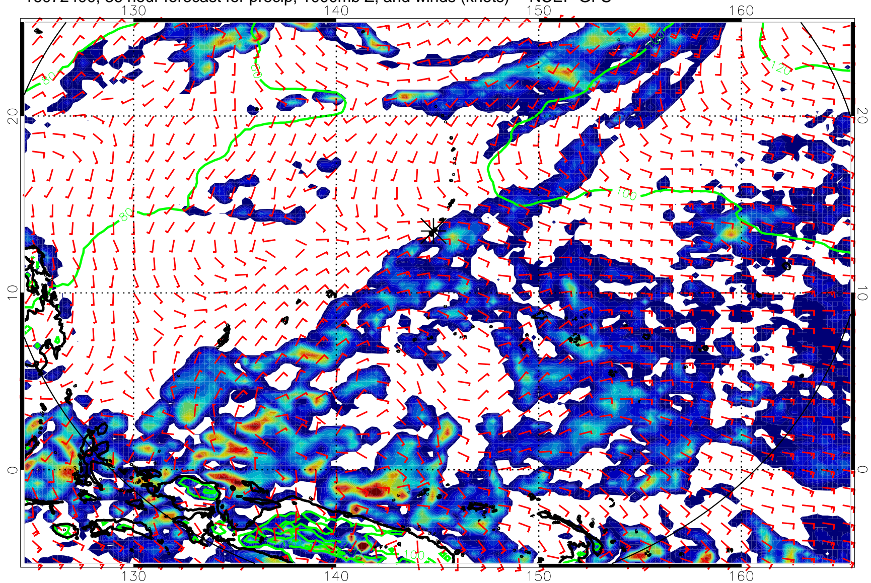
16072400, 36 hour forecast for precip, 1000mb Z, and winds (knots) -- NCEP GFS
