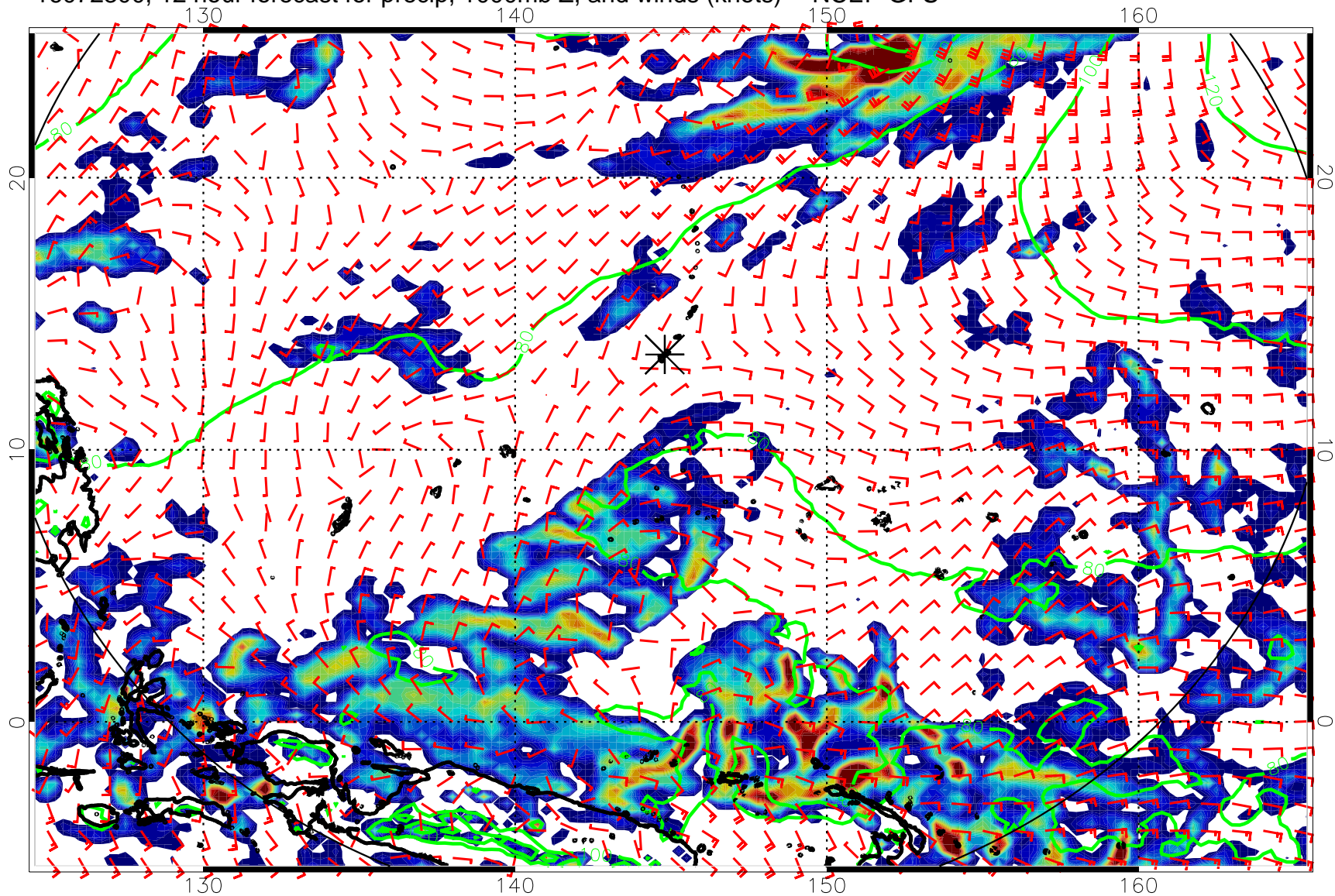
16072300, 12 hour forecast for precip, 1000mb Z, and winds (knots) -- NCEP GFS
