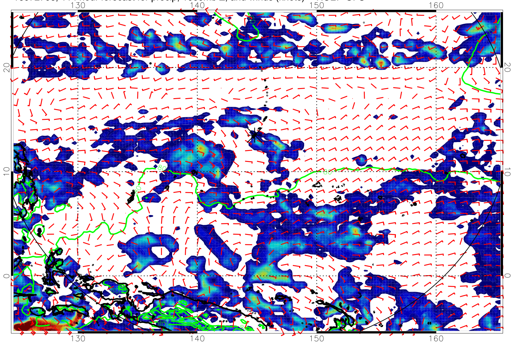
16072706, 114 hour forecast for precip, 1000mb Z, and winds (knots) -- NCEP GFS
