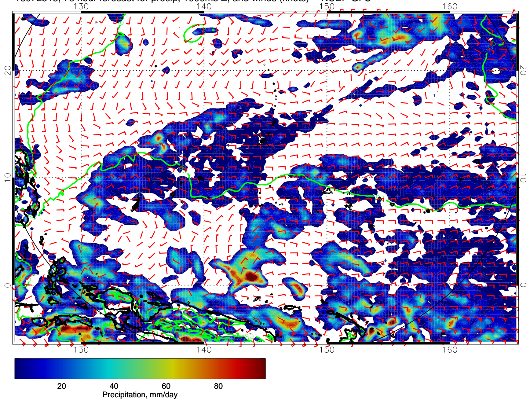
16072518, 78 hour forecast for precip, 1000mb Z, and winds (knots) -- NCEP GFS
