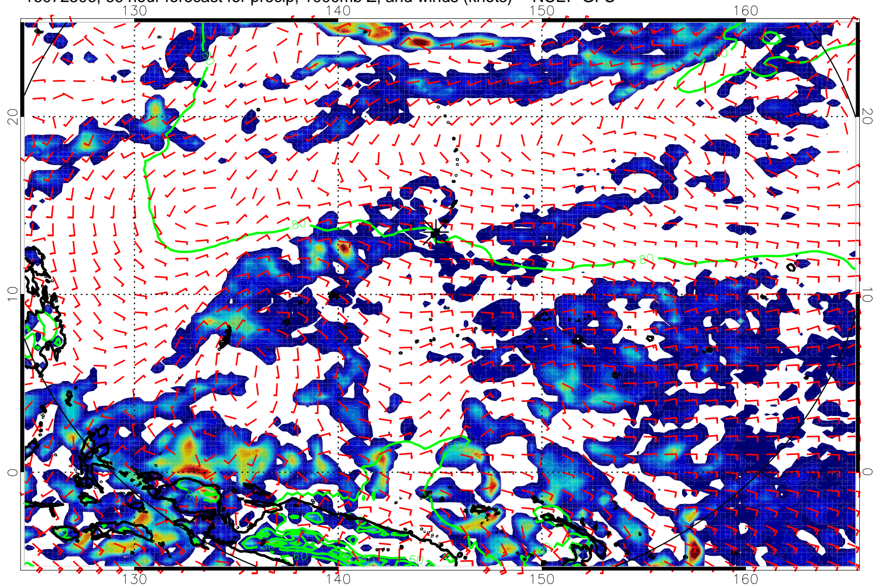
16072506, 66 hour forecast for precip, 1000mb Z, and winds (knots) -- NCEP GFS
