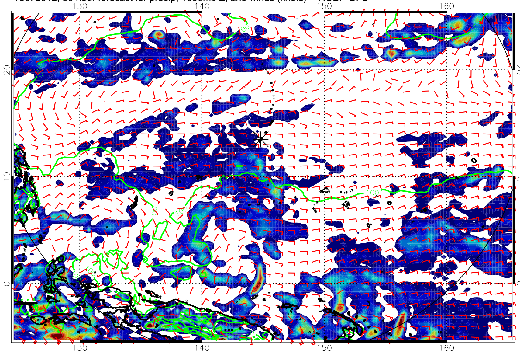
16072612, 96 hour forecast for precip, 1000mb Z, and winds (knots) -- NCEP GFS
