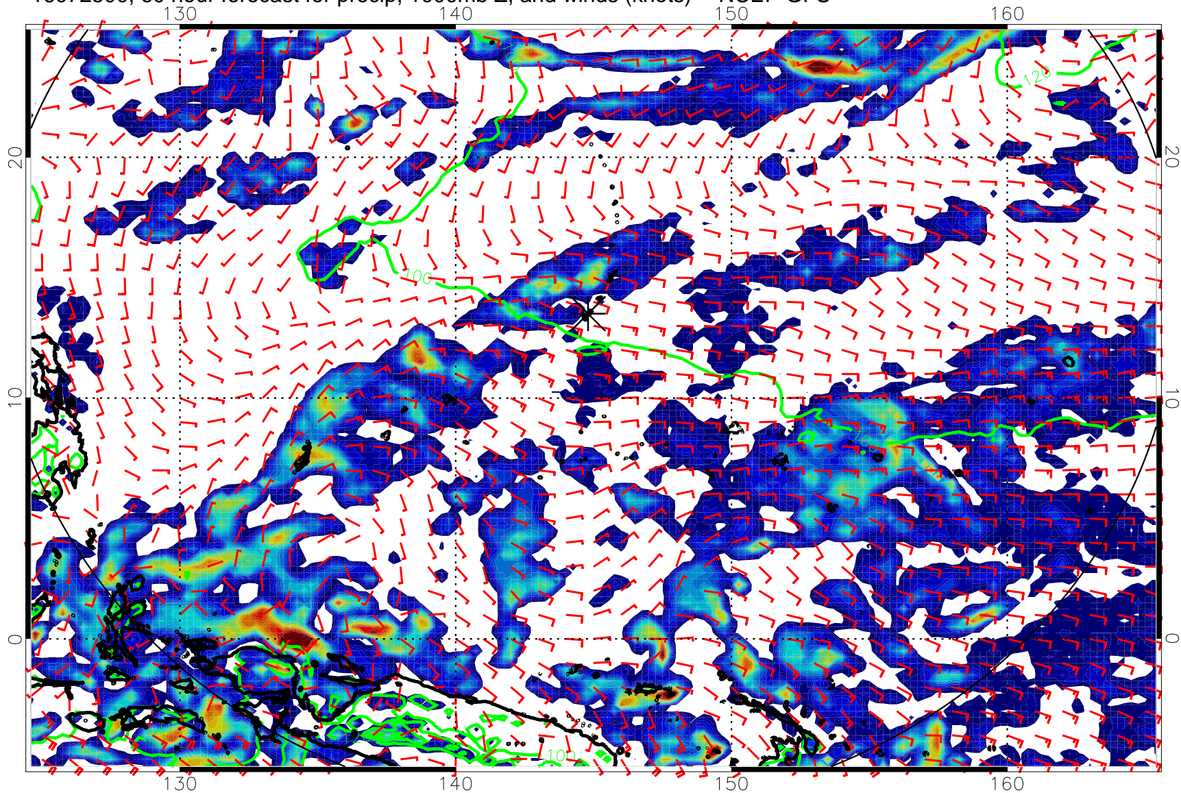
16072500, 60 hour forecast for precip, 1000mb Z, and winds (knots) -- NCEP GFS
