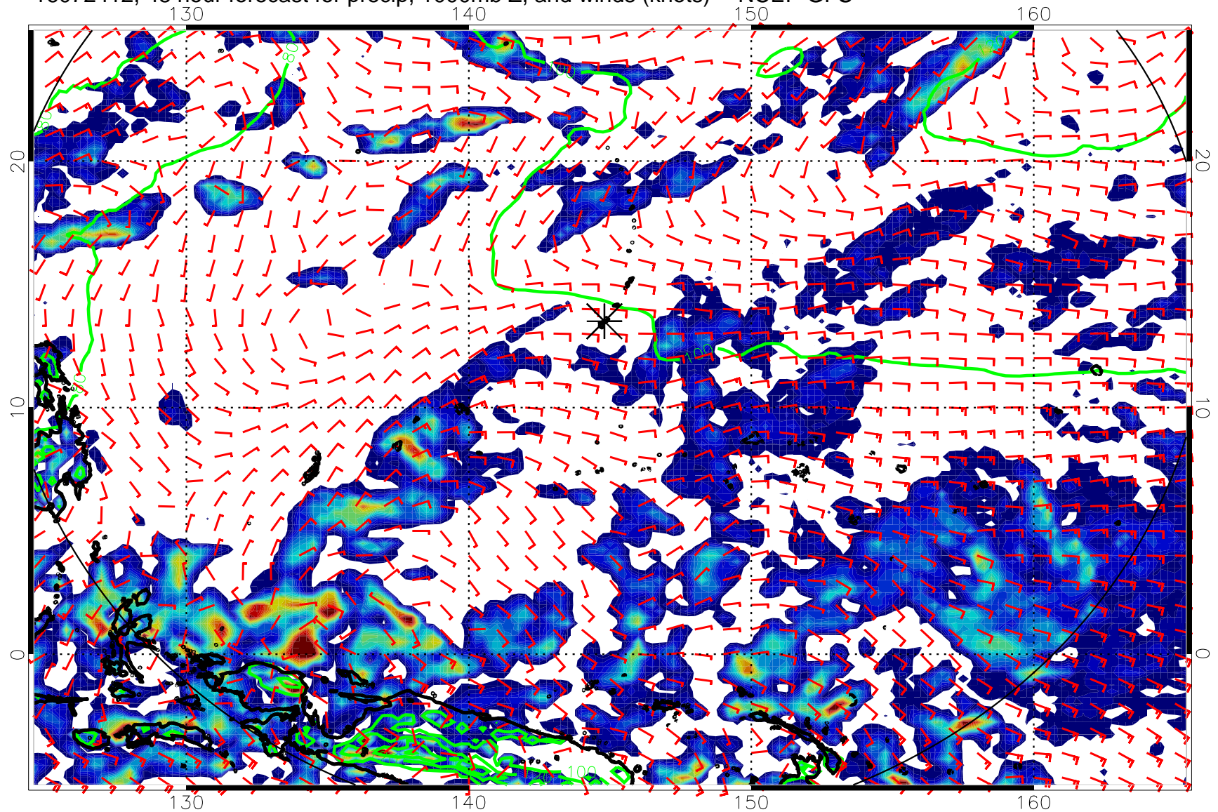
16072412, 48 hour forecast for precip, 1000mb Z, and winds (knots) -- NCEP GFS
