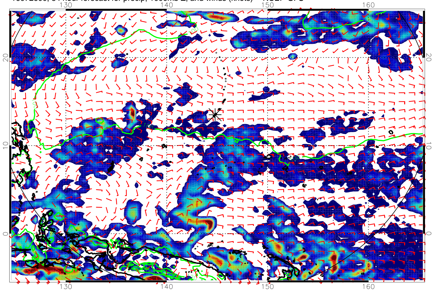
16072600, 84 hour forecast for precip, 1000mb Z, and winds (knots) -- NCEP GFS
