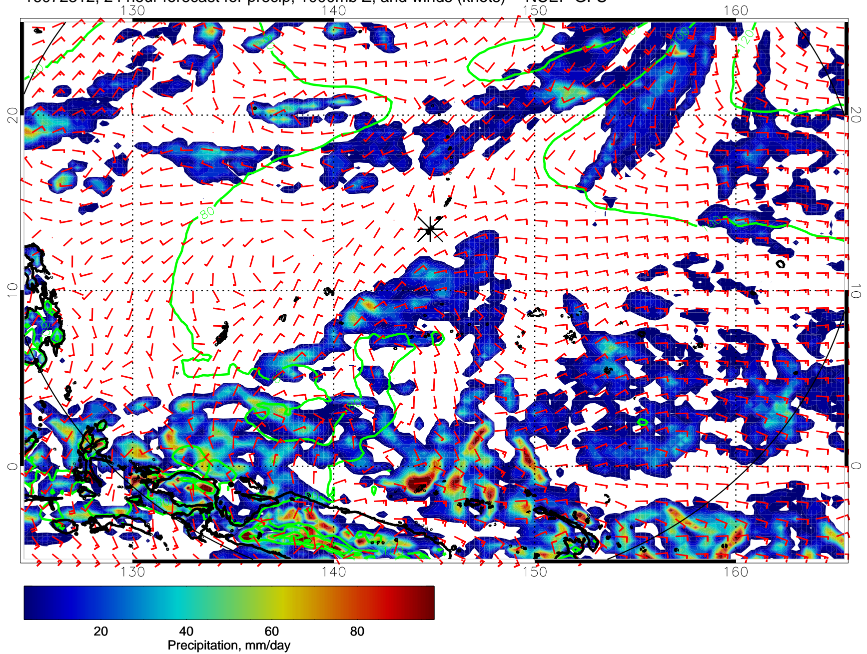
16072312, 24 hour forecast for precip, 1000mb Z, and winds (knots) -- NCEP GFS
