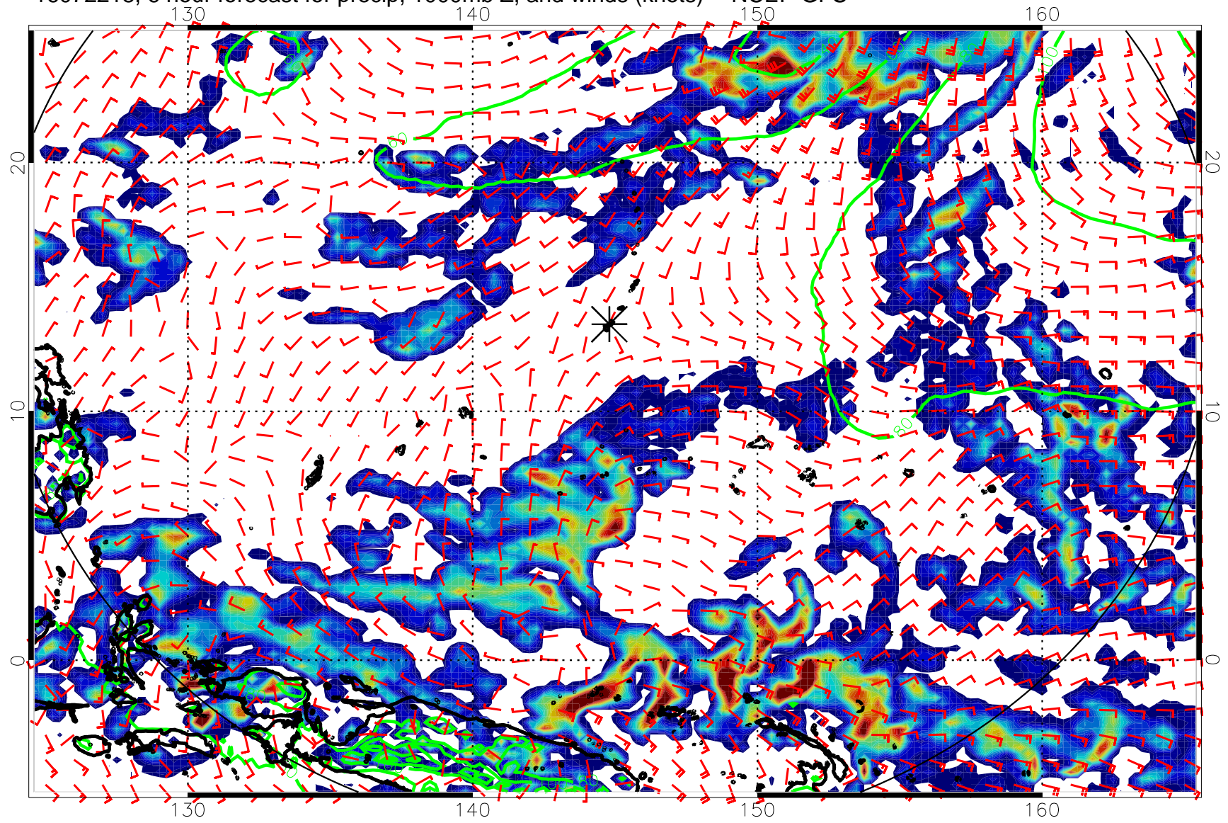
16072218, 6 hour forecast for precip, 1000mb Z, and winds (knots) -- NCEP GFS
