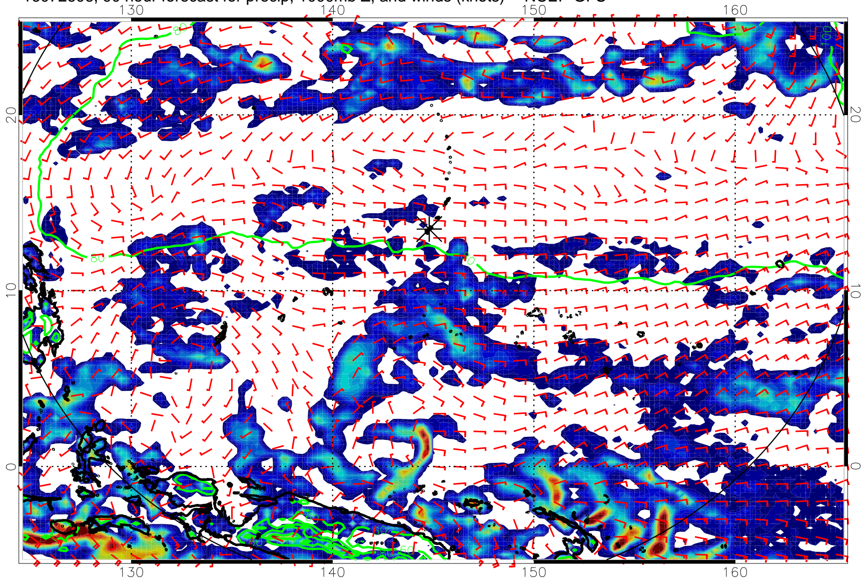
16072606, 90 hour forecast for precip, 1000mb Z, and winds (knots) -- NCEP GFS
