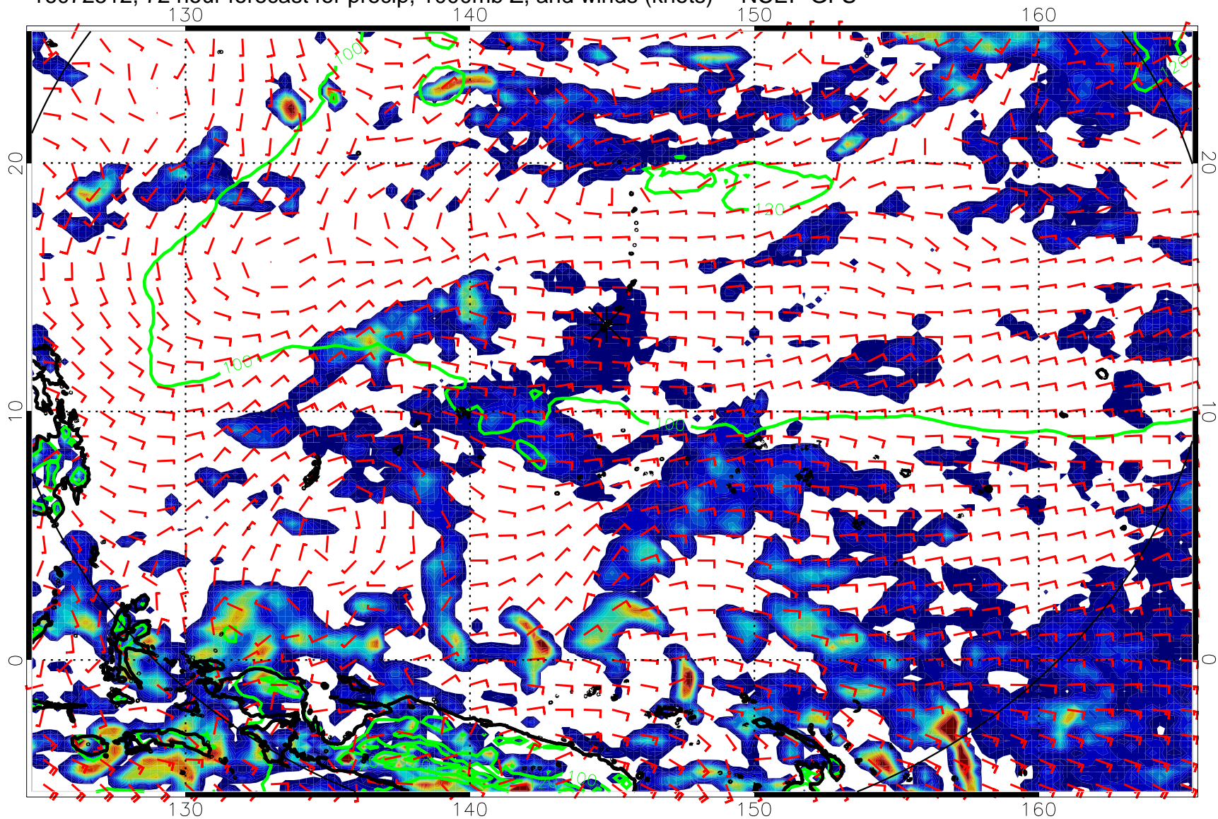
16072512, 72 hour forecast for precip, 1000mb Z, and winds (knots) -- NCEP GFS
