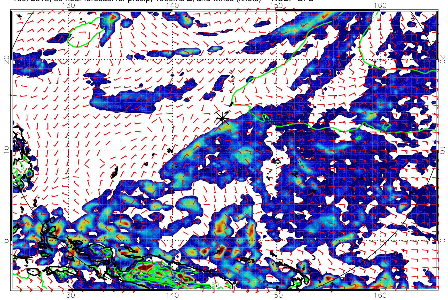
16072318, 30 hour forecast for precip, 1000mb Z, and winds (knots) -- NCEP GFS
