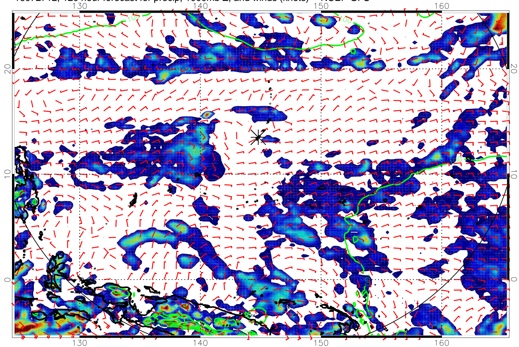
16072712, 120 hour forecast for precip, 1000mb Z, and winds (knots) -- NCEP GFS
