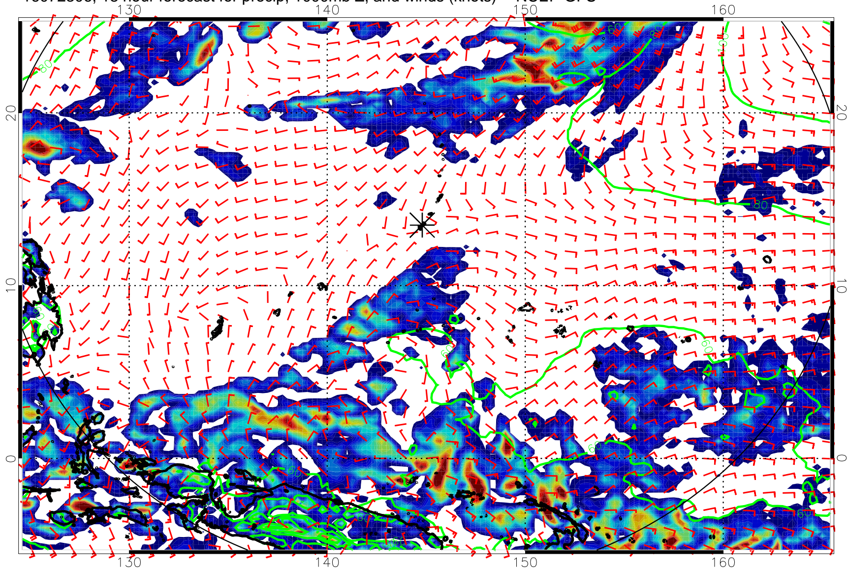
16072306, 18 hour forecast for precip, 1000mb Z, and winds (knots) -- NCEP GFS
