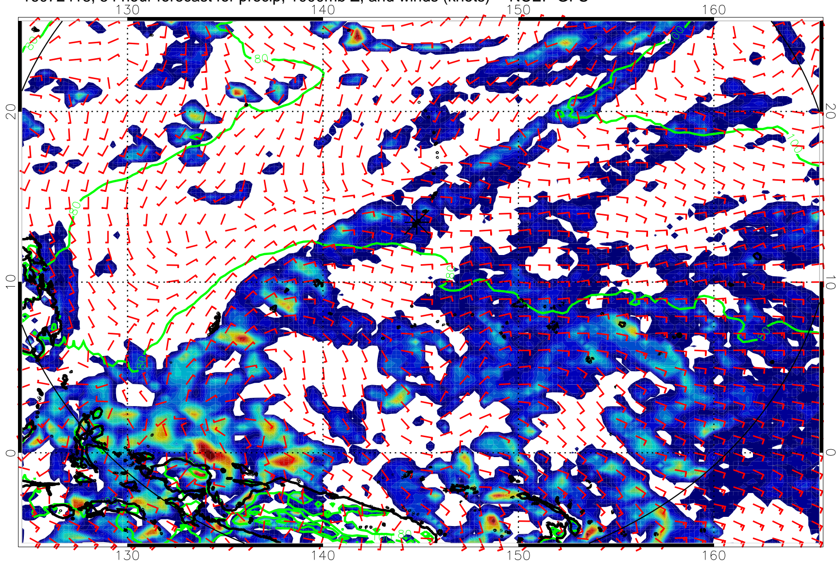
16072418, 54 hour forecast for precip, 1000mb Z, and winds (knots) -- NCEP GFS
