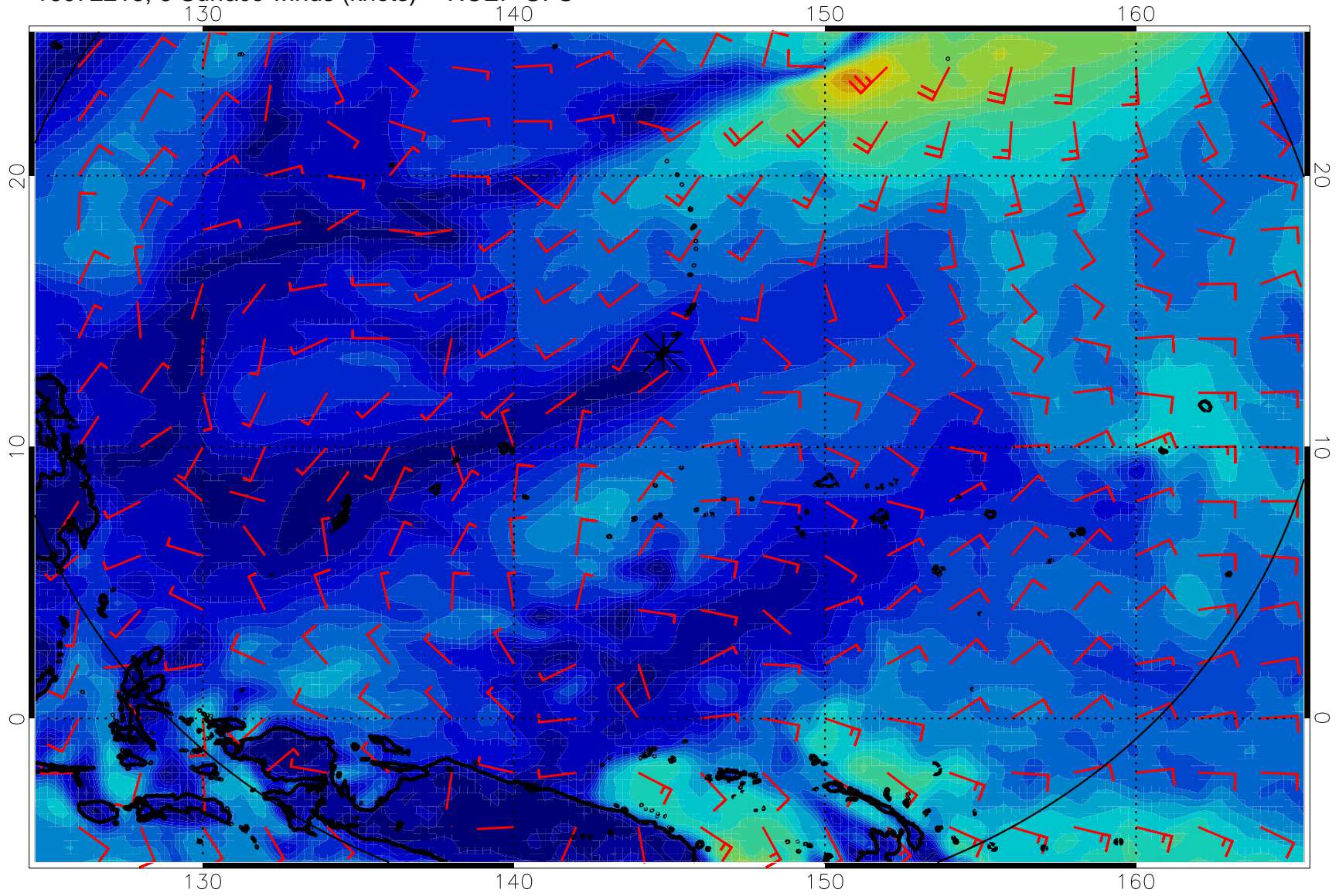
16072218, 6 Surface winds (knots) -- NCEP GFS
