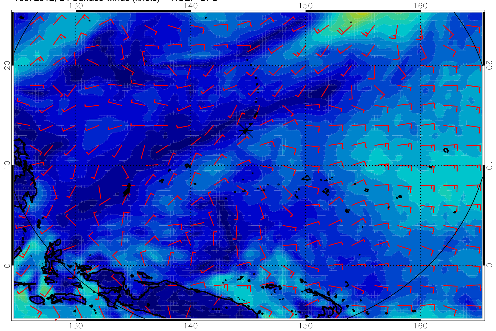
16072312, 24 Surface winds (knots) -- NCEP GFS
