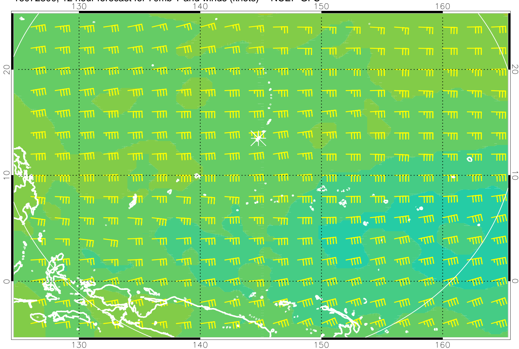
16072300, 12 hour forecast for 70mb T and winds (knots) -- NCEP GFS
