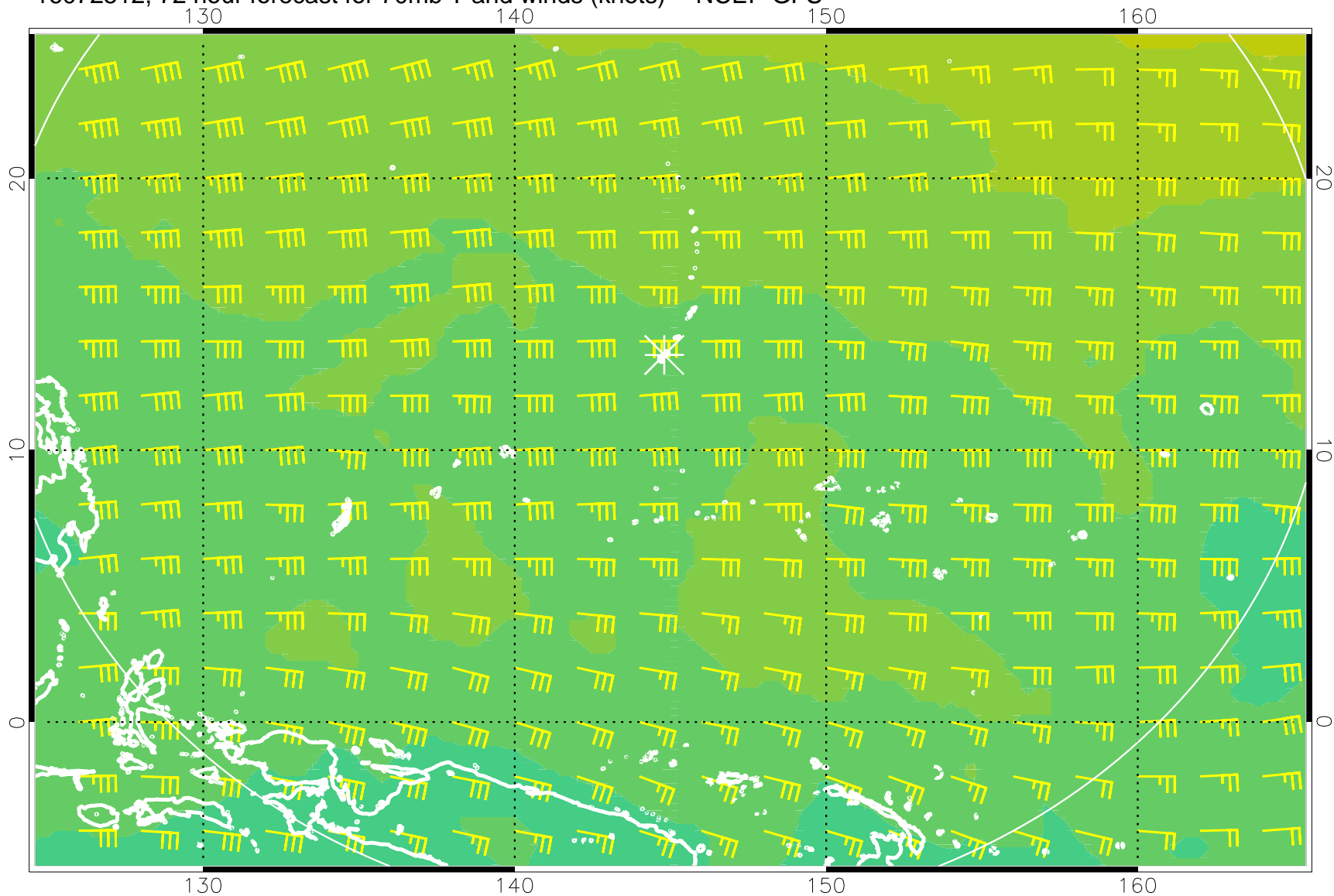
16072512, 72 hour forecast for 70mb T and winds (knots) -- NCEP GFS
