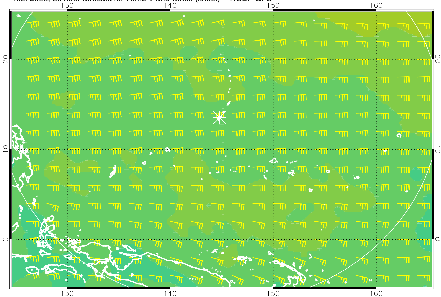
16072506, 66 hour forecast for 70mb T and winds (knots) -- NCEP GFS
