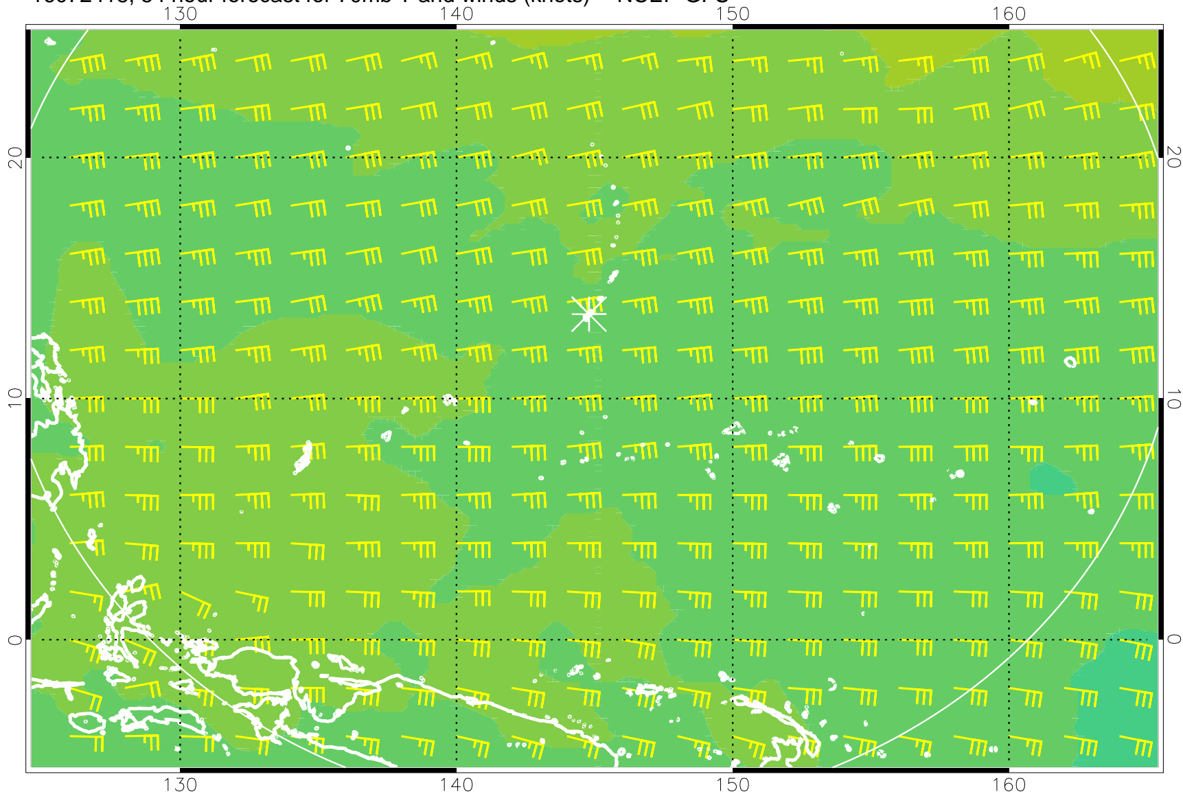
16072418, 54 hour forecast for 70mb T and winds (knots) -- NCEP GFS
