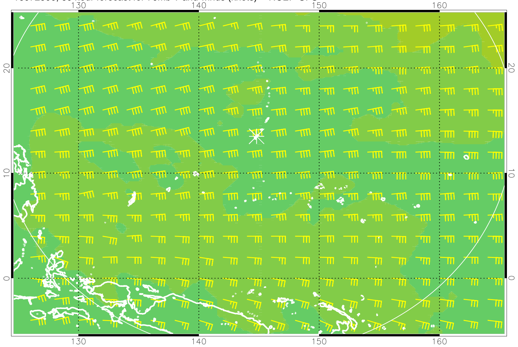
16072500, 60 hour forecast for 70mb T and winds (knots) -- NCEP GFS
