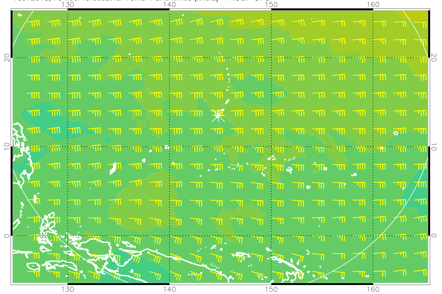
16072518, 78 hour forecast for 70mb T and winds (knots) -- NCEP GFS
