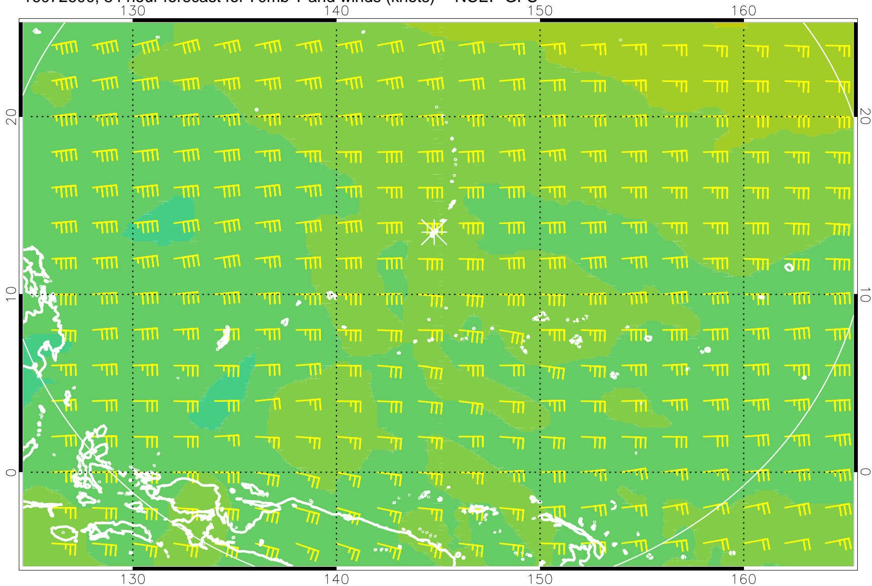
16072600, 84 hour forecast for 70mb T and winds (knots) -- NCEP GFS
