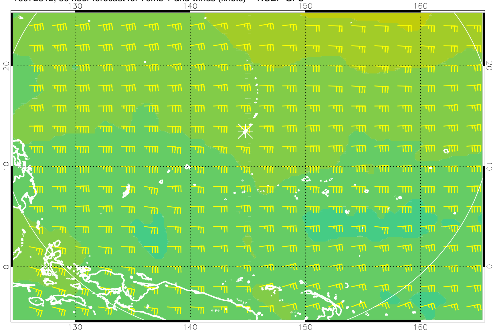
16072612, 96 hour forecast for 70mb T and winds (knots) -- NCEP GFS
