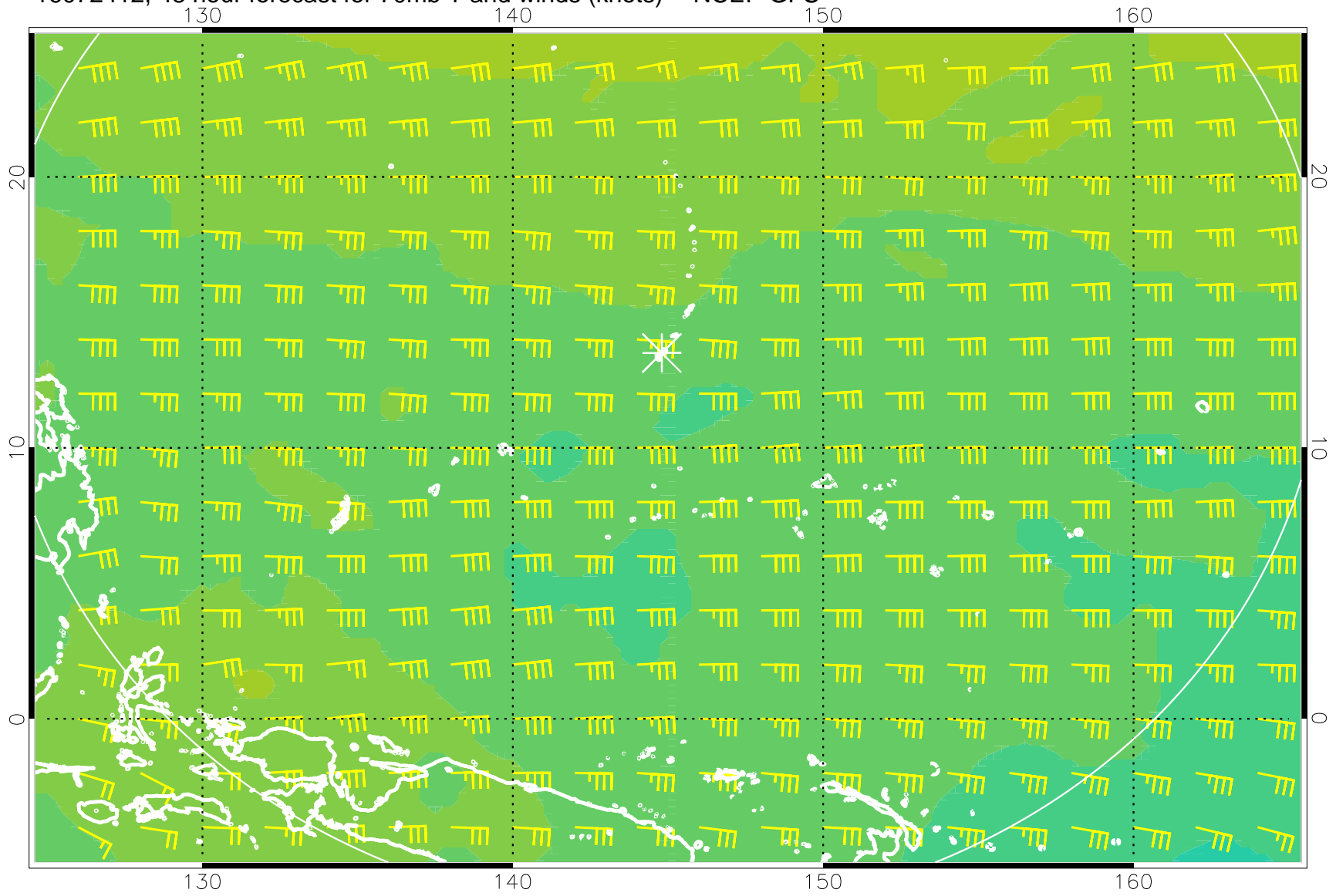
16072412, 48 hour forecast for 70mb T and winds (knots) -- NCEP GFS
