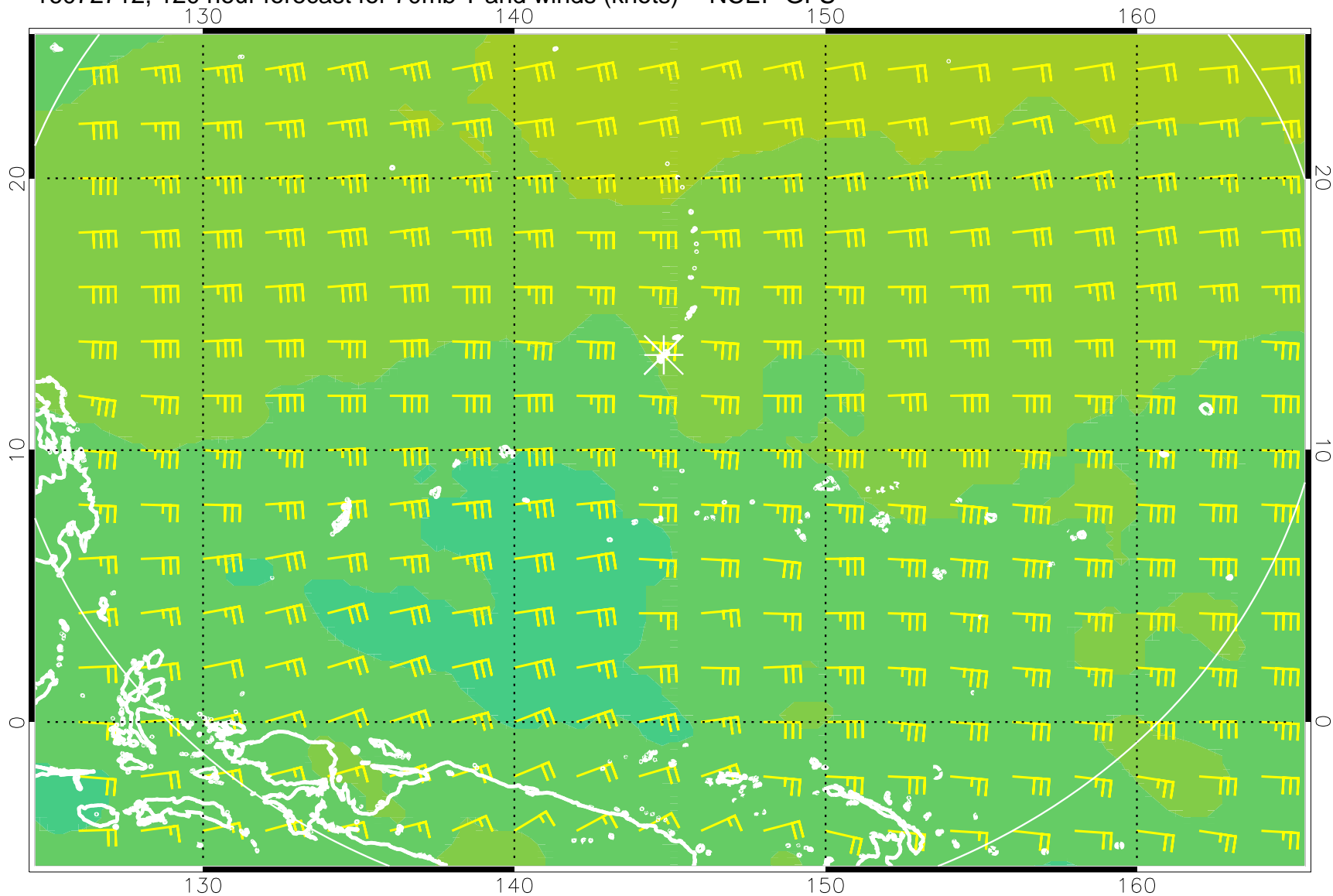
16072712, 120 hour forecast for 70mb T and winds (knots) -- NCEP GFS
