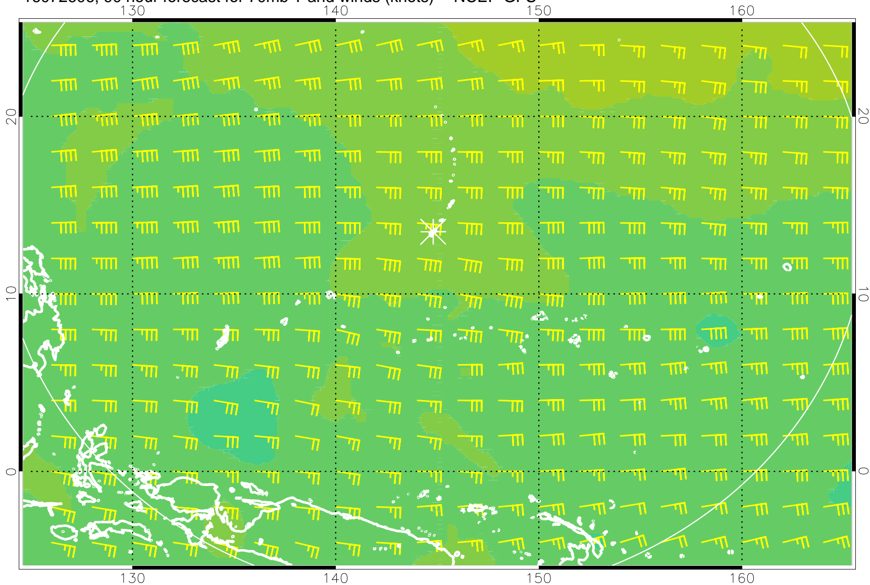
16072606, 90 hour forecast for 70mb T and winds (knots) -- NCEP GFS
