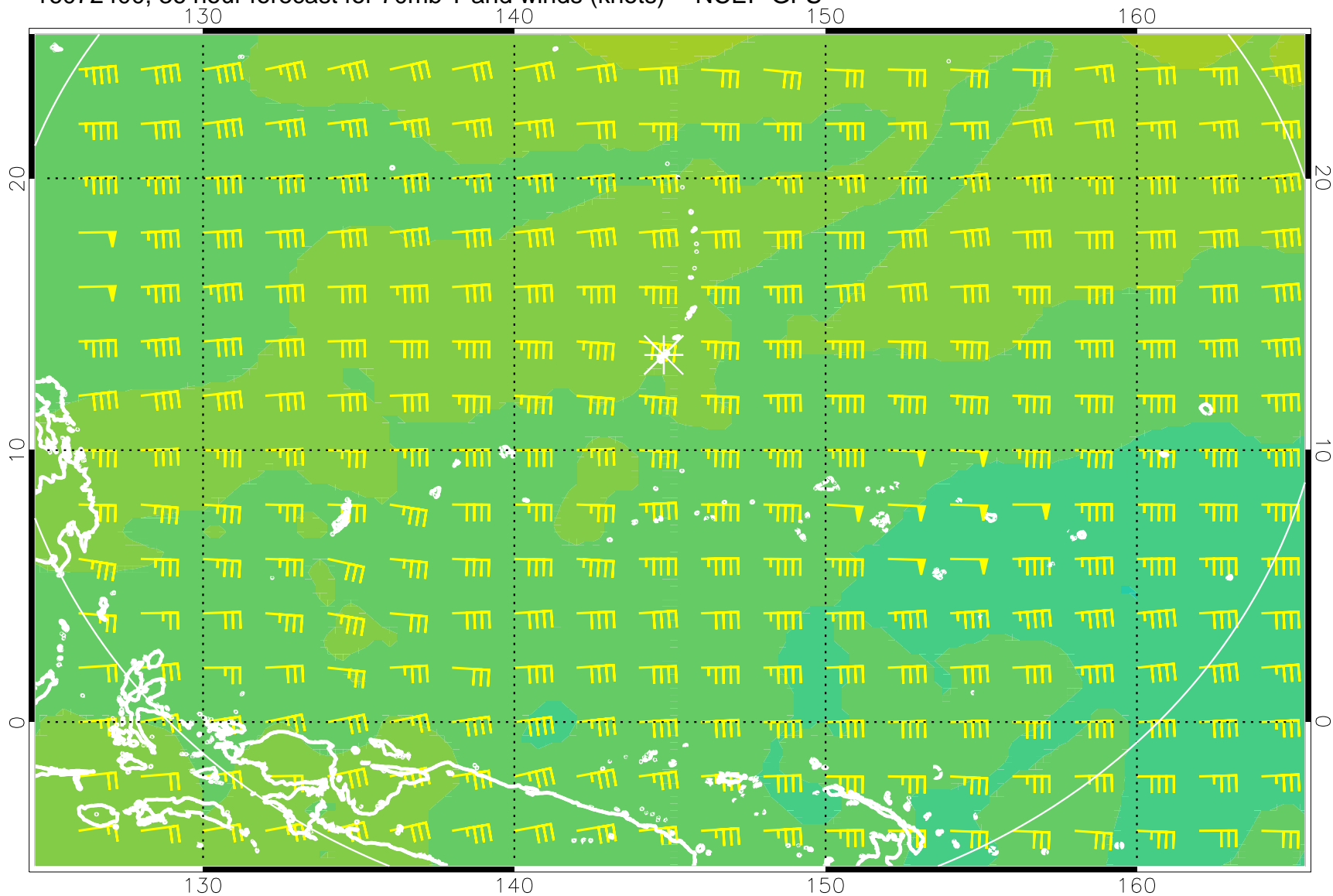
16072400, 36 hour forecast for 70mb T and winds (knots) -- NCEP GFS
