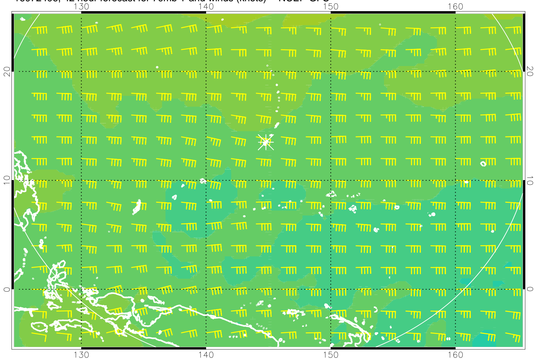
16072406, 42 hour forecast for 70mb T and winds (knots) -- NCEP GFS
