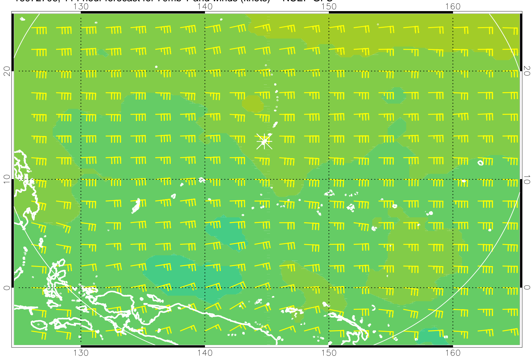
16072706, 114 hour forecast for 70mb T and winds (knots) -- NCEP GFS
