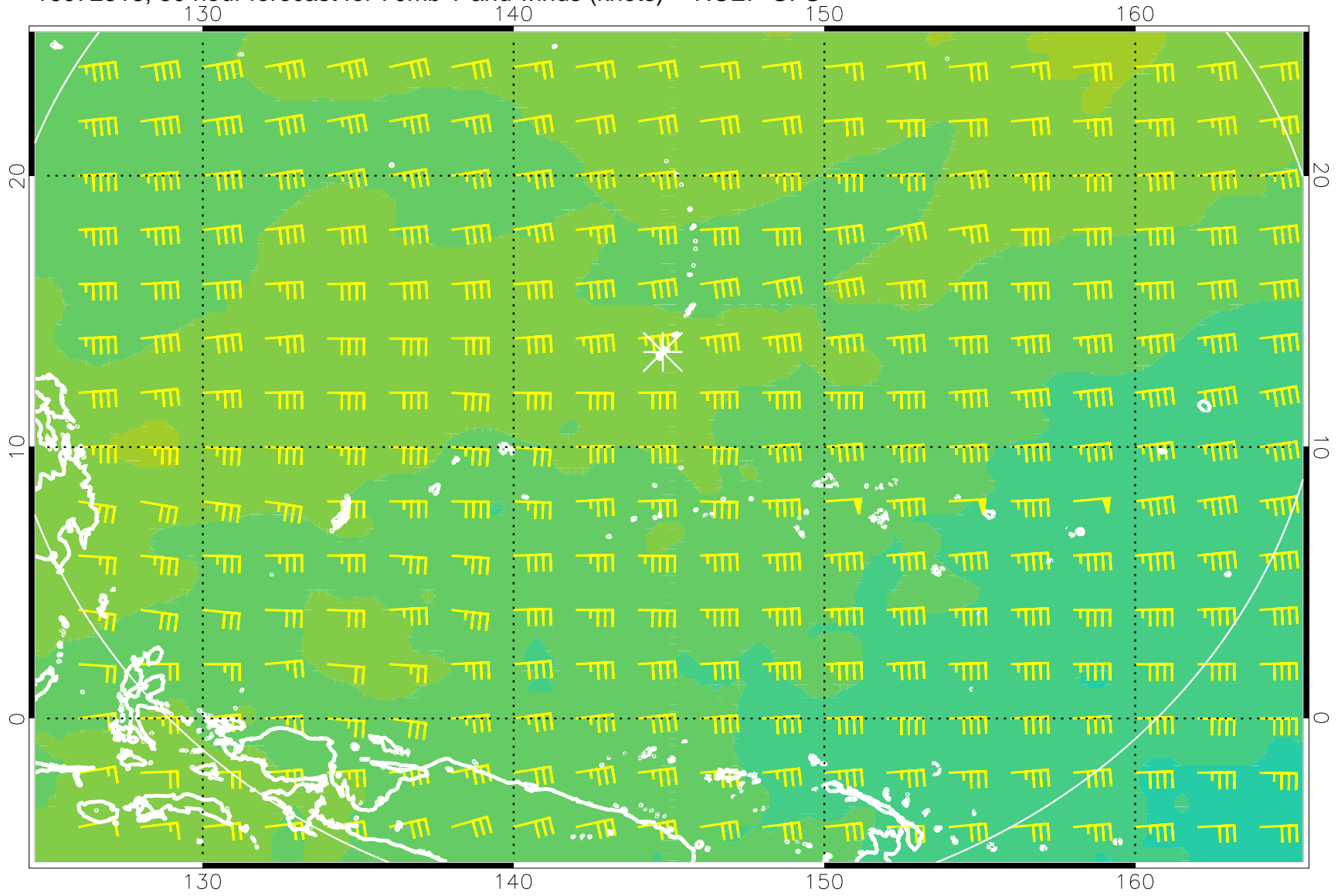
16072318, 30 hour forecast for 70mb T and winds (knots) -- NCEP GFS
