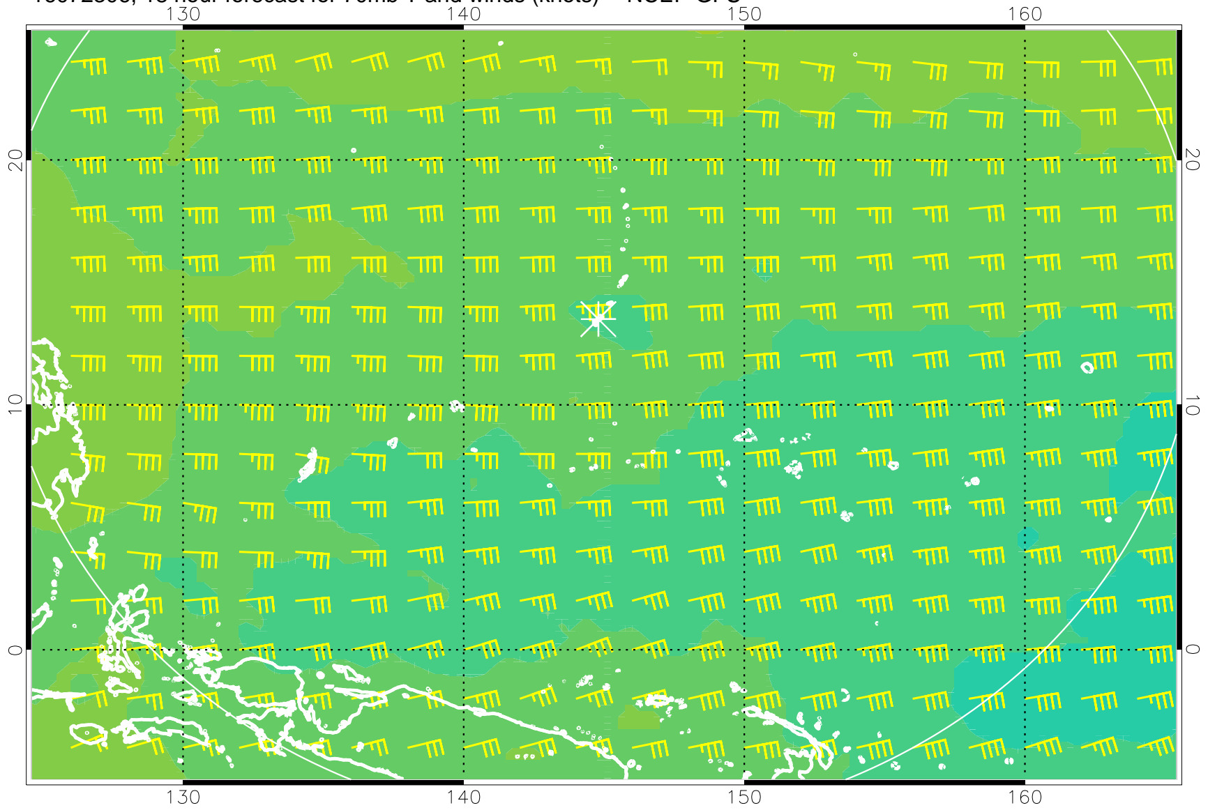
16072306, 18 hour forecast for 70mb T and winds (knots) -- NCEP GFS
