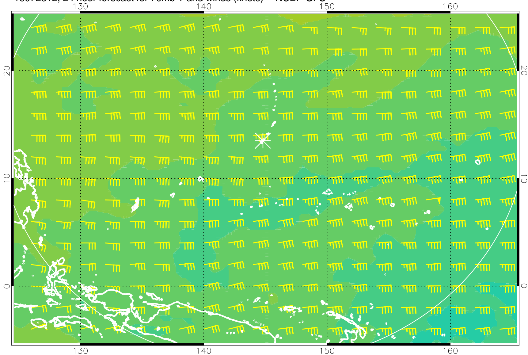
16072312, 24 hour forecast for 70mb T and winds (knots) -- NCEP GFS
