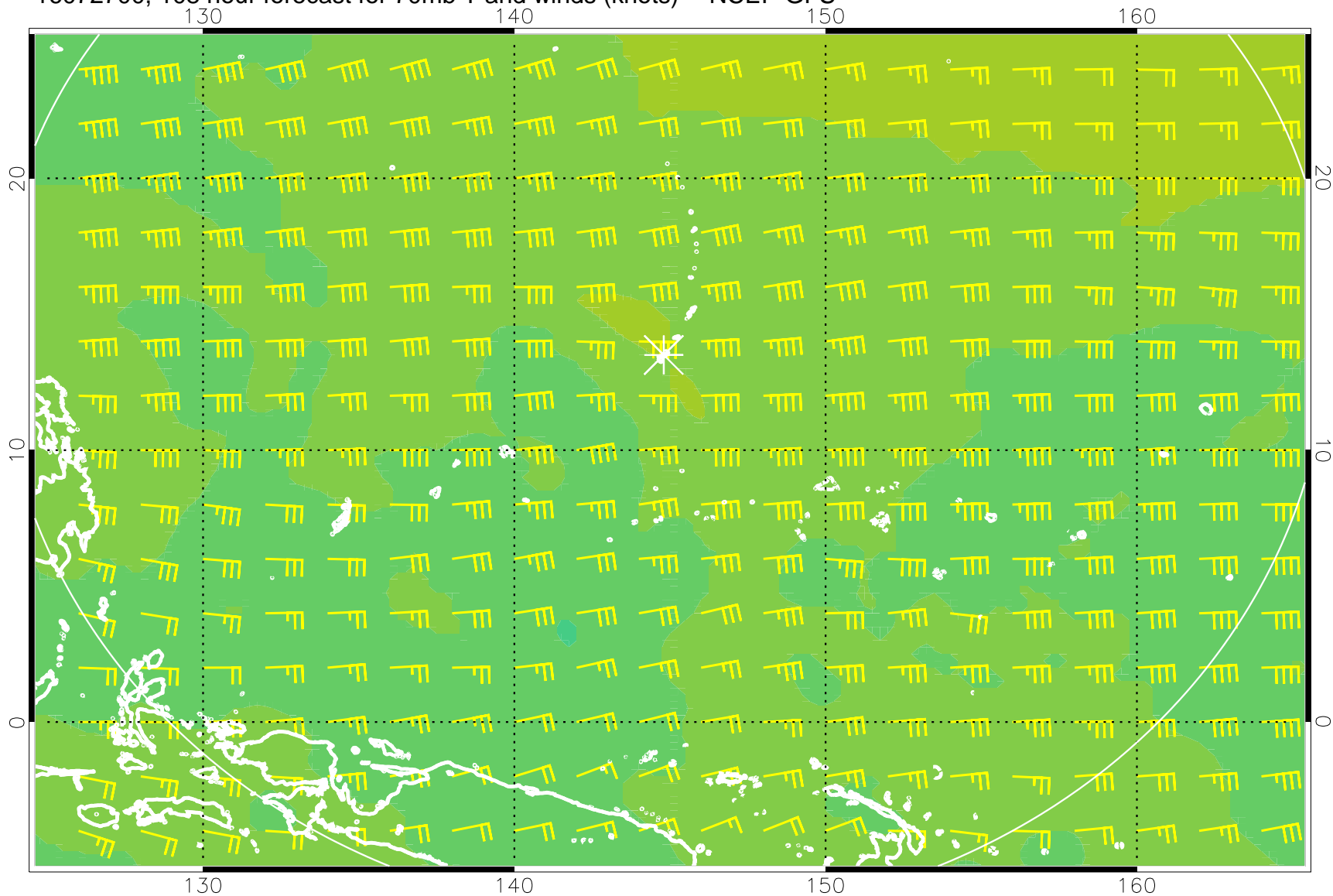
16072700, 108 hour forecast for 70mb T and winds (knots) -- NCEP GFS
