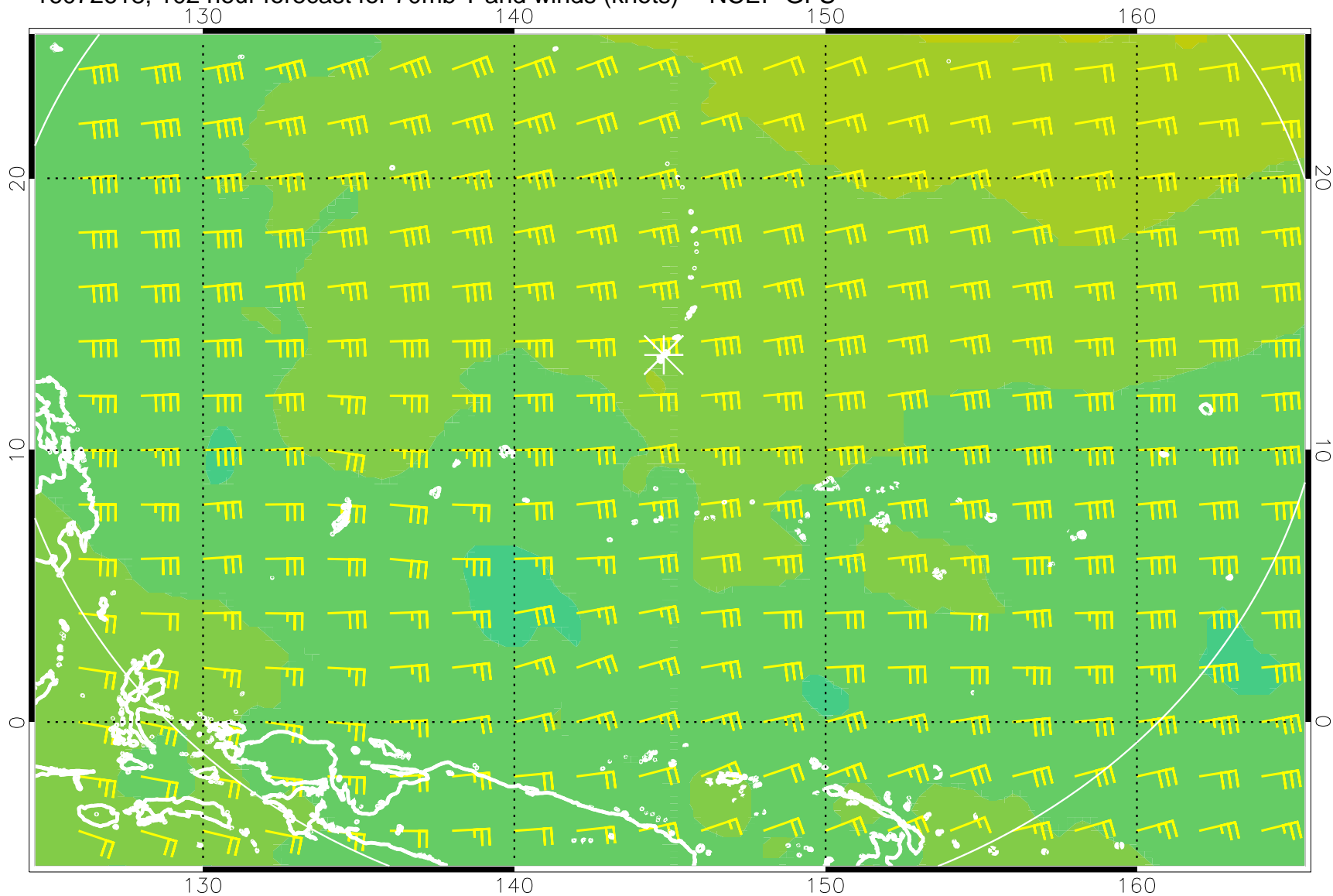
16072618, 102 hour forecast for 70mb T and winds (knots) -- NCEP GFS
