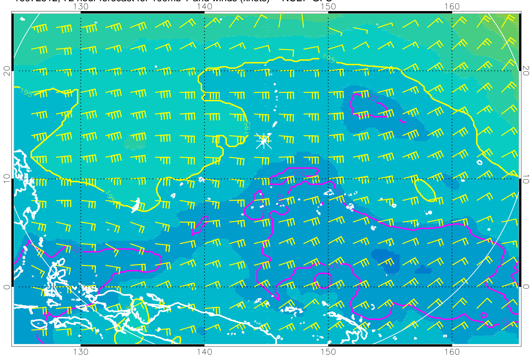
16072512, 72 hour forecast for 100mb T and winds (knots) -- NCEP GFS
