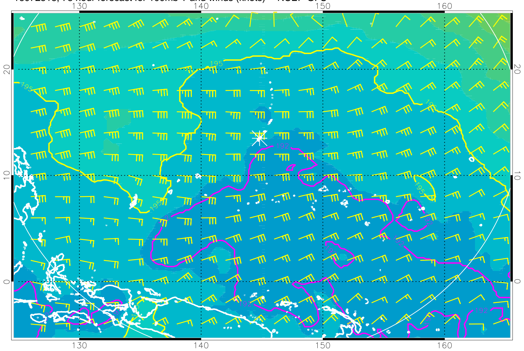
16072518, 78 hour forecast for 100mb T and winds (knots) -- NCEP GFS
