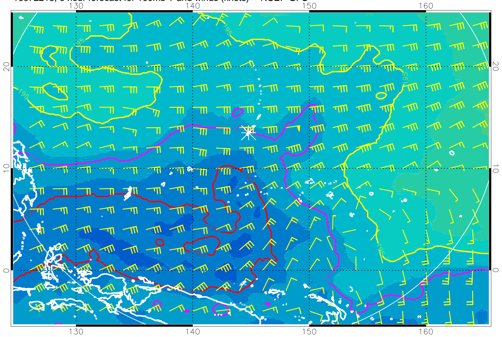
16072218, 6 hour forecast for 100mb T and winds (knots) -- NCEP GFS
