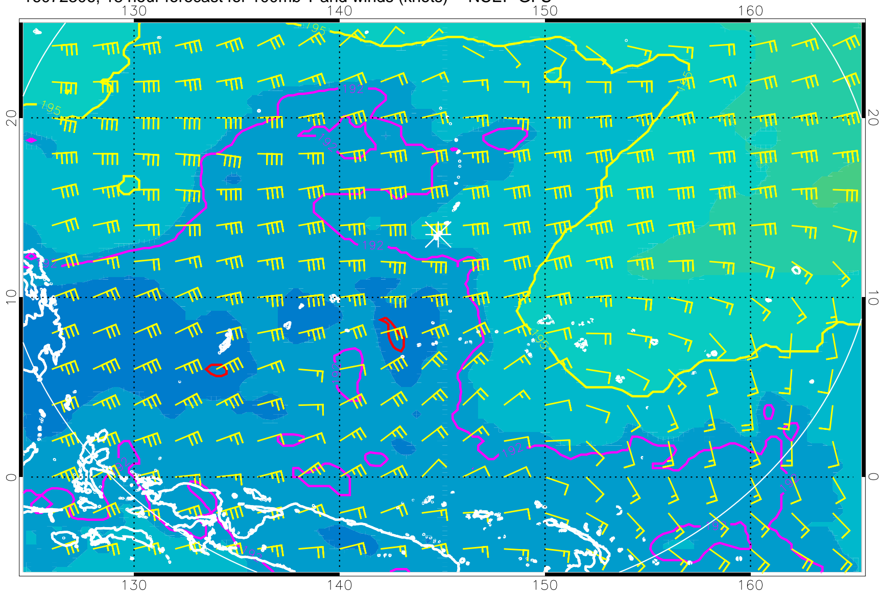
16072306, 18 hour forecast for 100mb T and winds (knots) -- NCEP GFS
