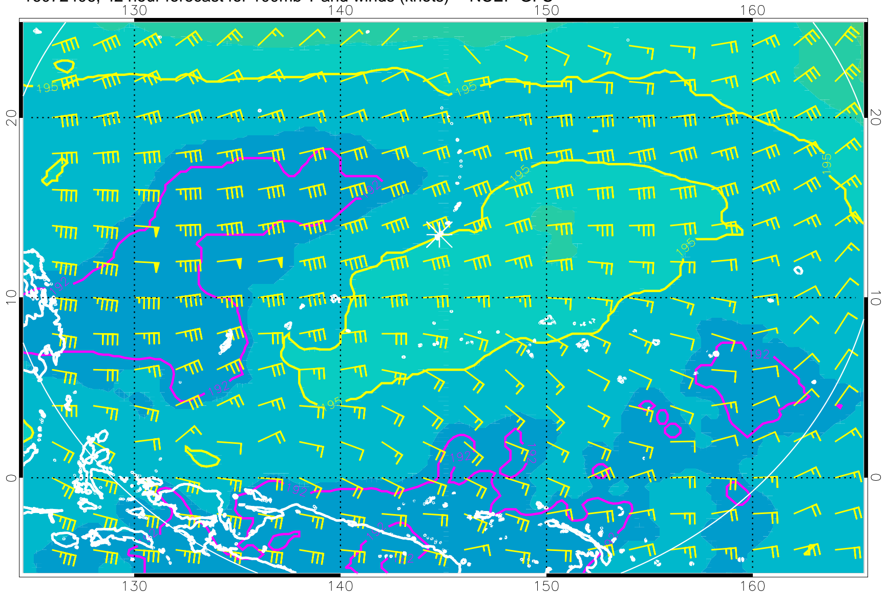
16072406, 42 hour forecast for 100mb T and winds (knots) -- NCEP GFS
