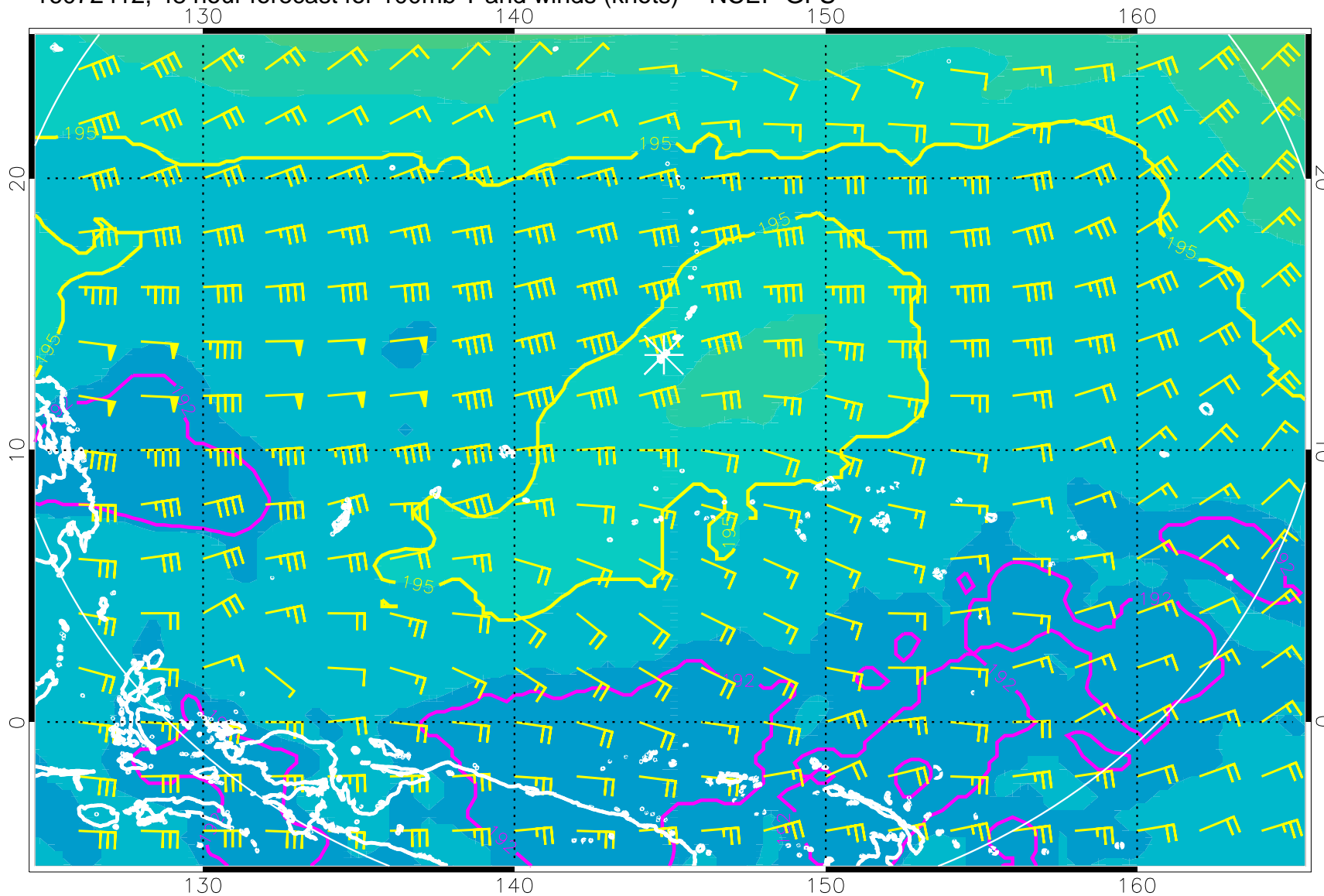
16072412, 48 hour forecast for 100mb T and winds (knots) -- NCEP GFS
