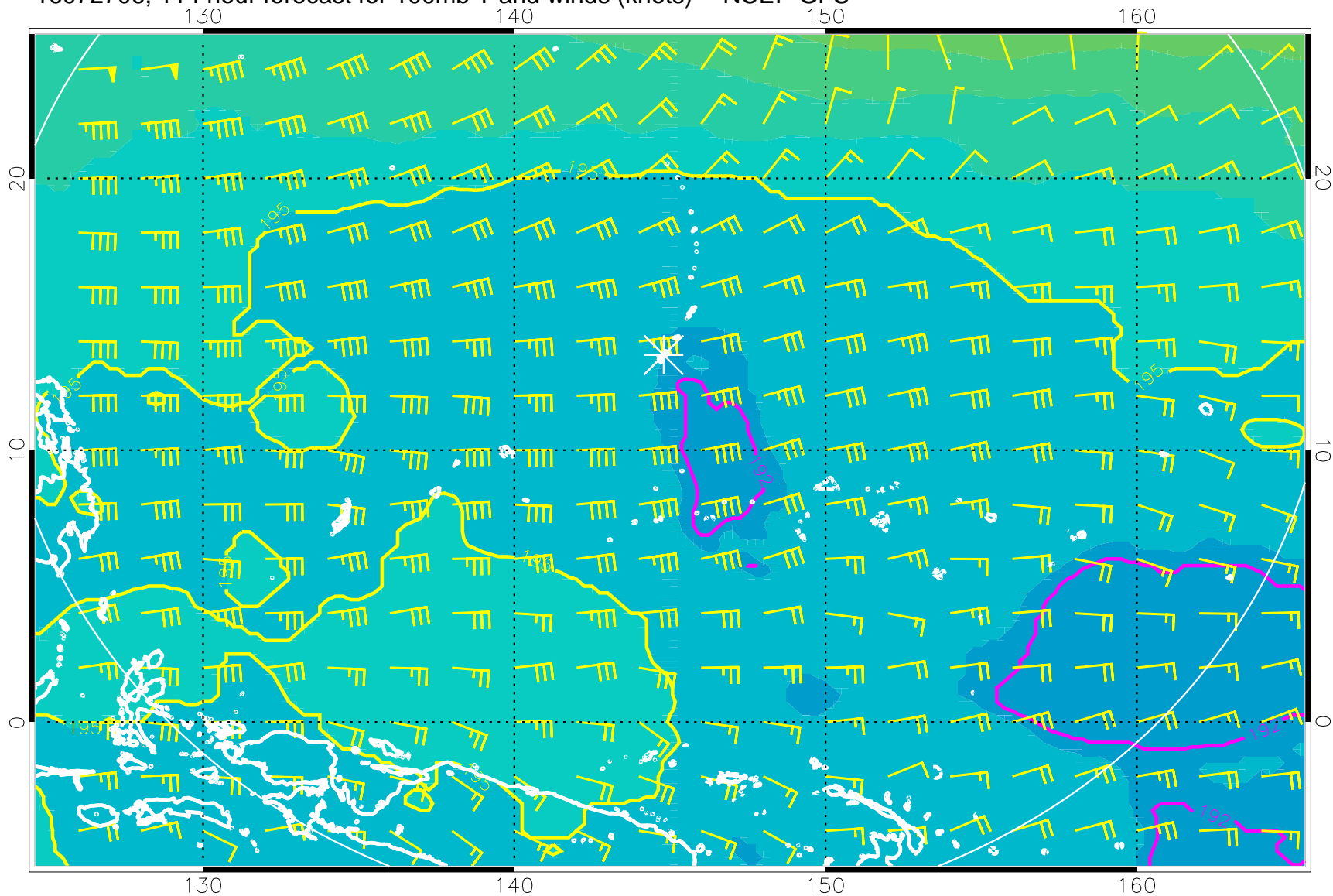
16072706, 114 hour forecast for 100mb T and winds (knots) -- NCEP GFS
