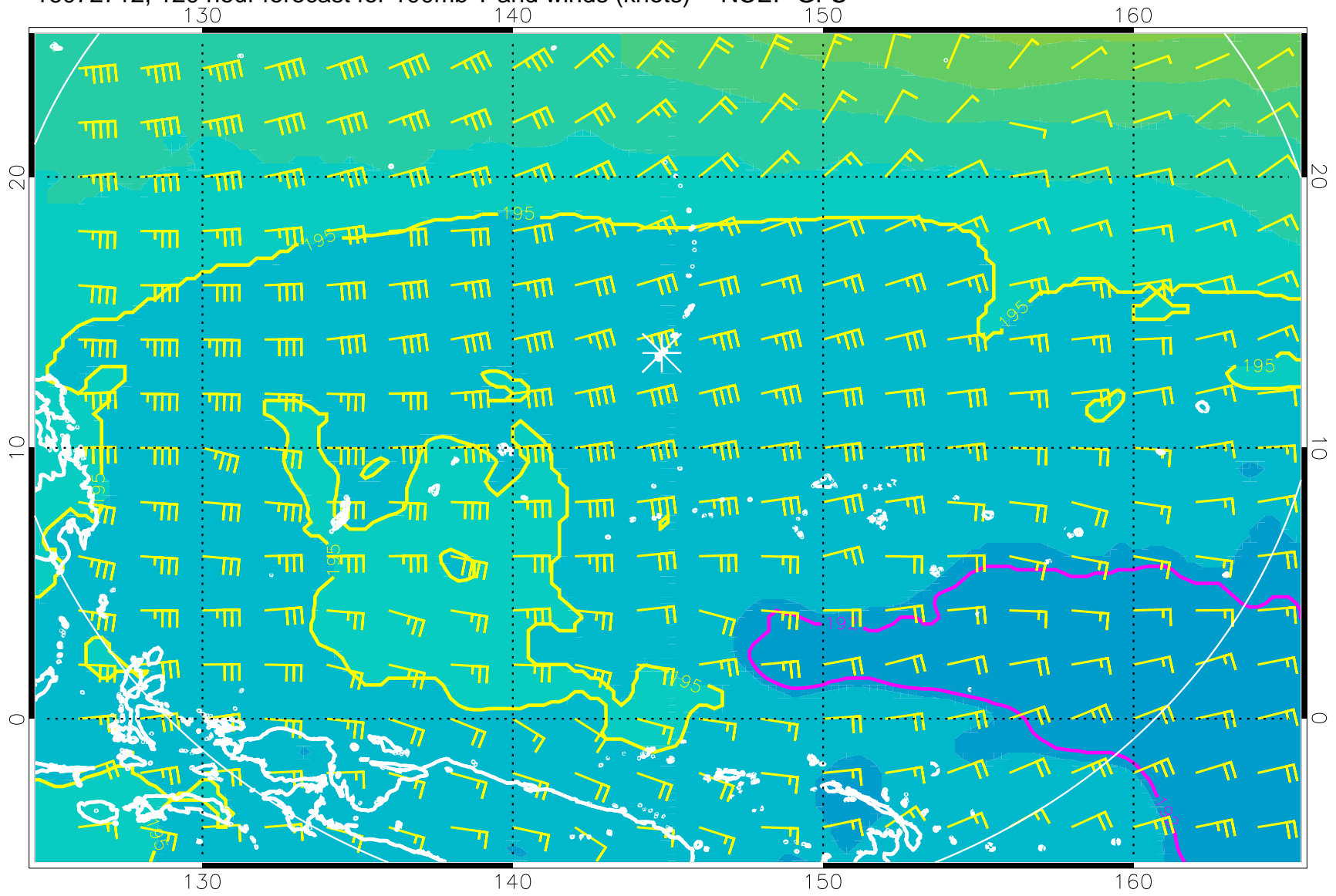
16072712, 120 hour forecast for 100mb T and winds (knots) -- NCEP GFS
