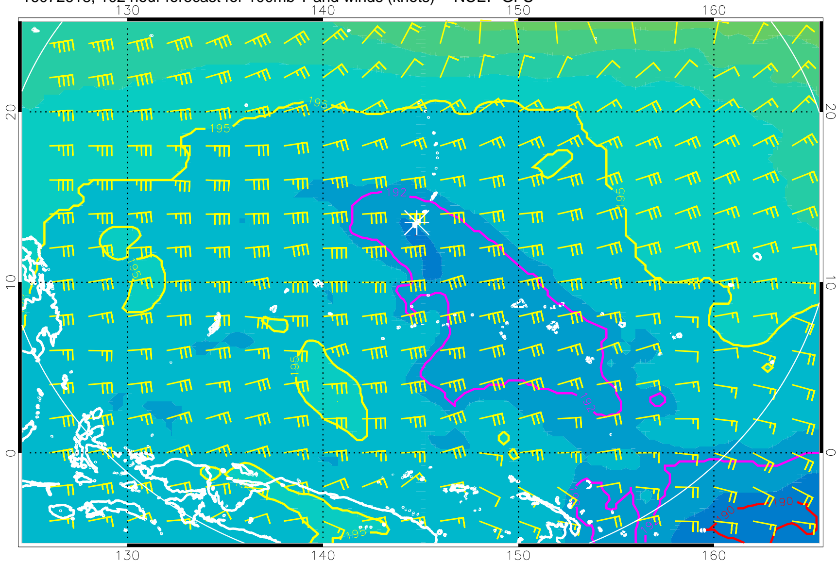
16072618, 102 hour forecast for 100mb T and winds (knots) -- NCEP GFS
