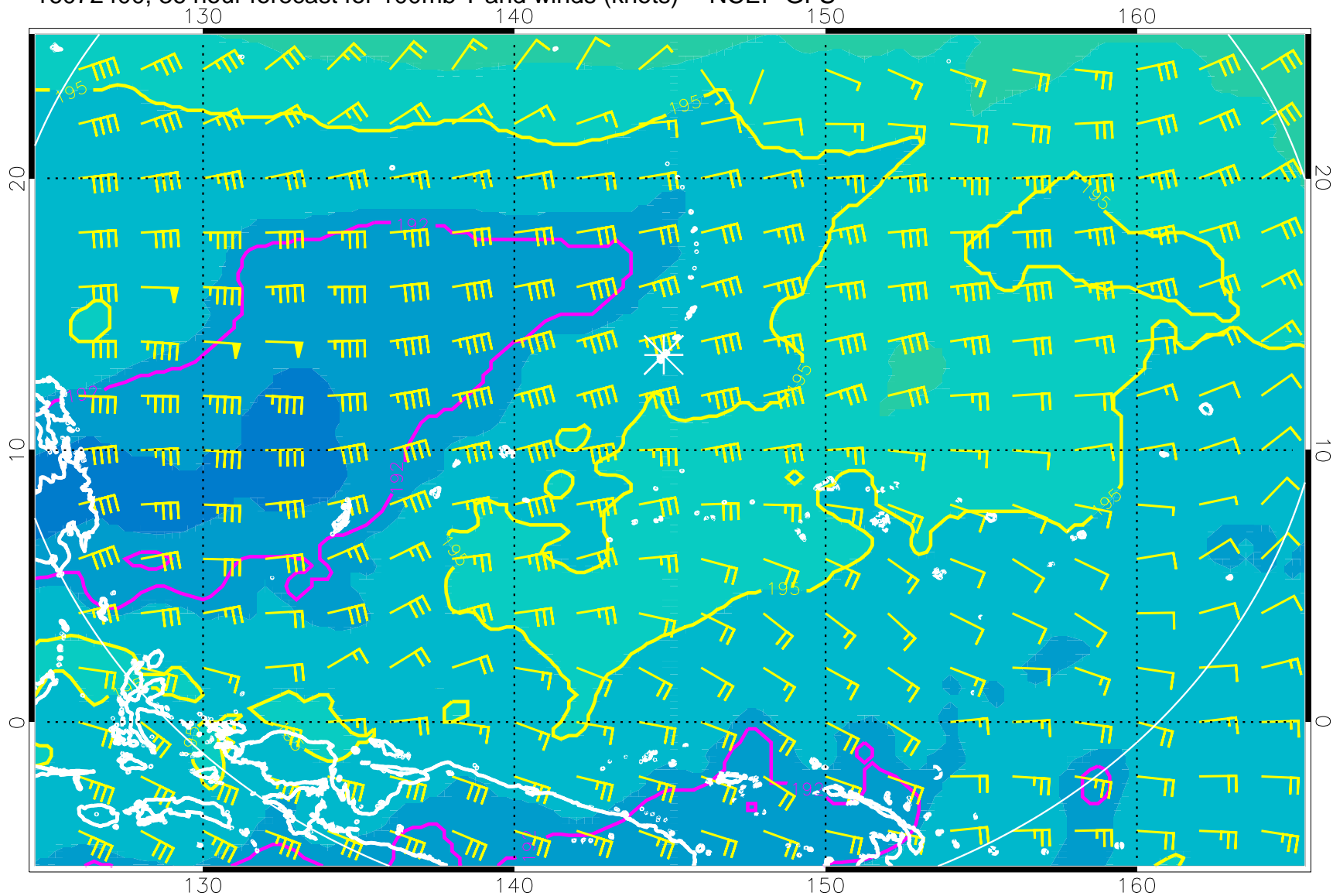
16072400, 36 hour forecast for 100mb T and winds (knots) -- NCEP GFS
