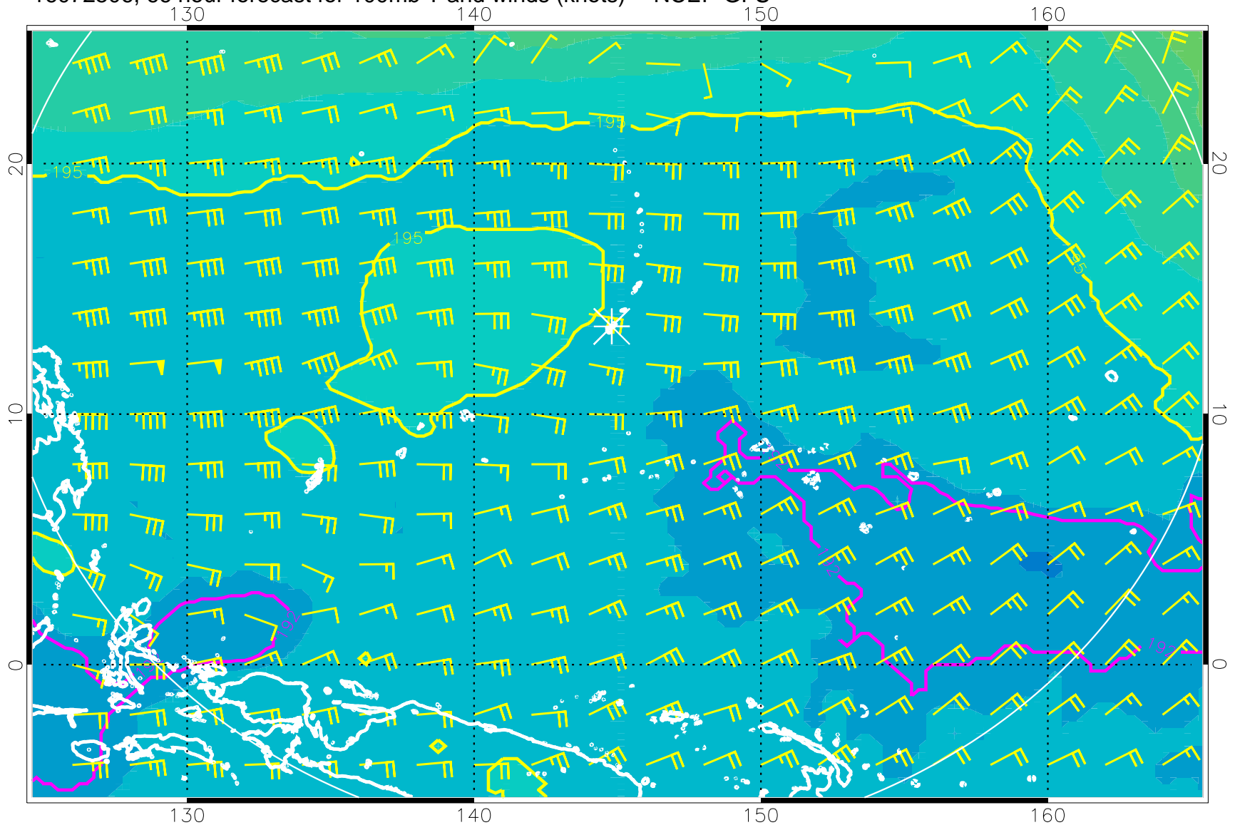
16072506, 66 hour forecast for 100mb T and winds (knots) -- NCEP GFS
