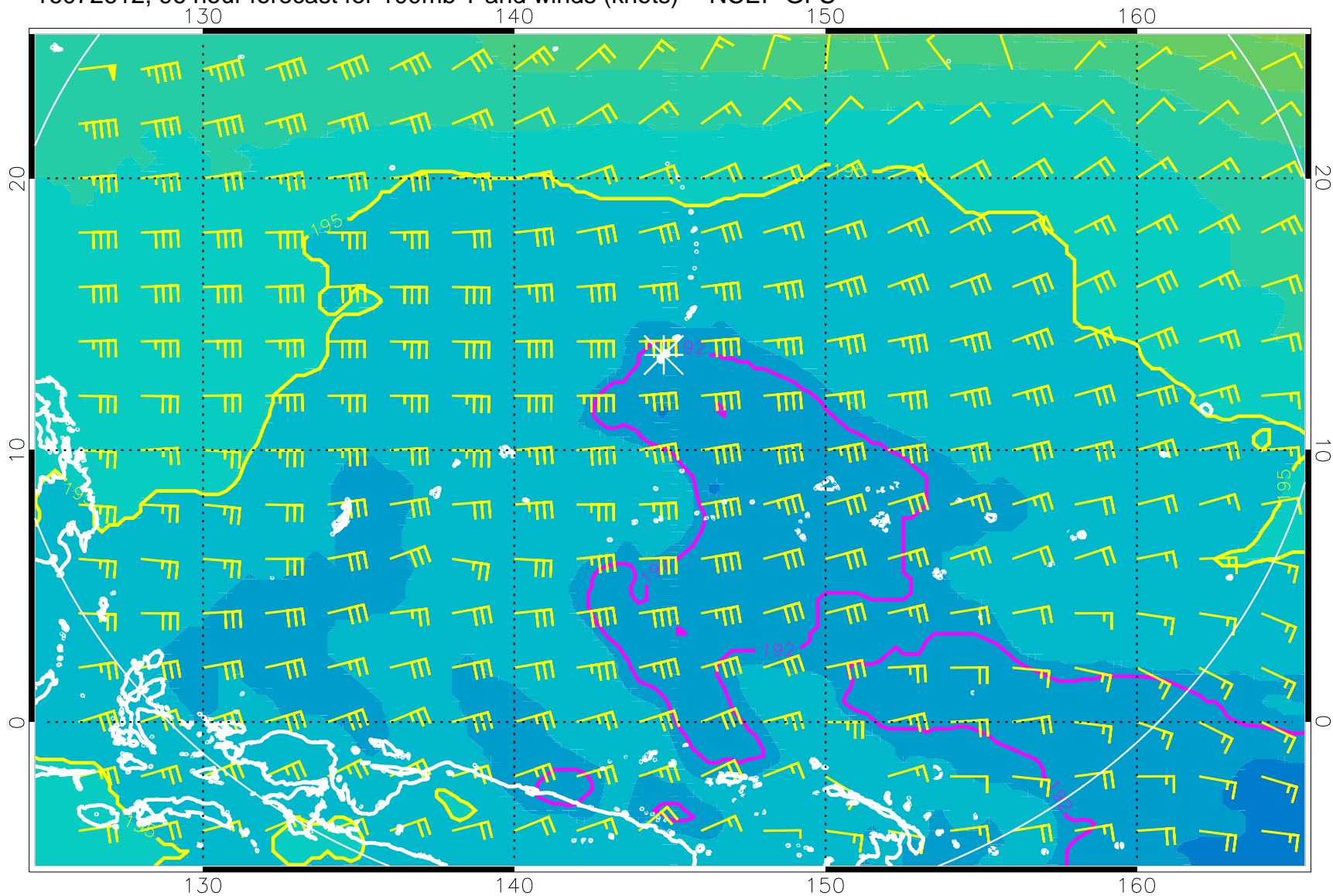
16072612, 96 hour forecast for 100mb T and winds (knots) -- NCEP GFS
