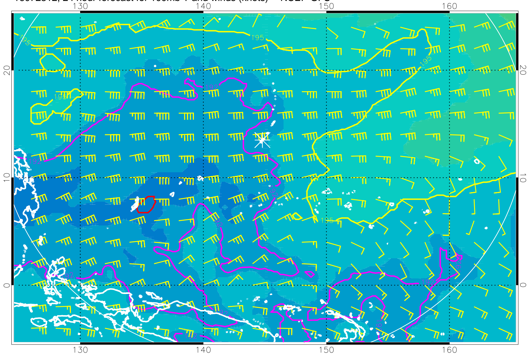
16072312, 24 hour forecast for 100mb T and winds (knots) -- NCEP GFS
