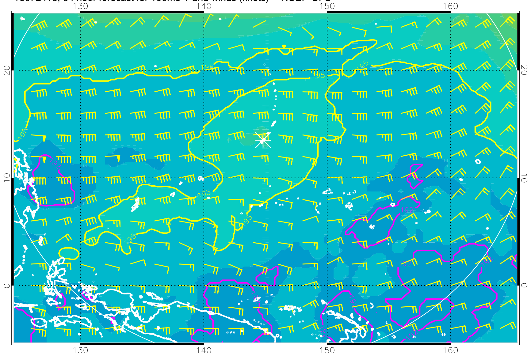
16072418, 54 hour forecast for 100mb T and winds (knots) -- NCEP GFS
