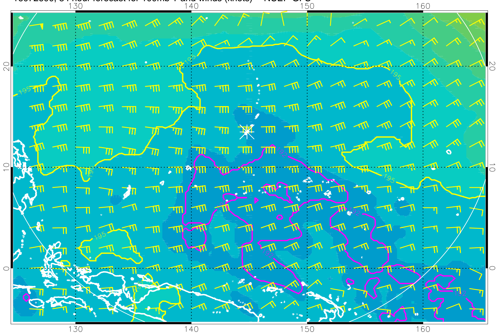
16072600, 84 hour forecast for 100mb T and winds (knots) -- NCEP GFS
