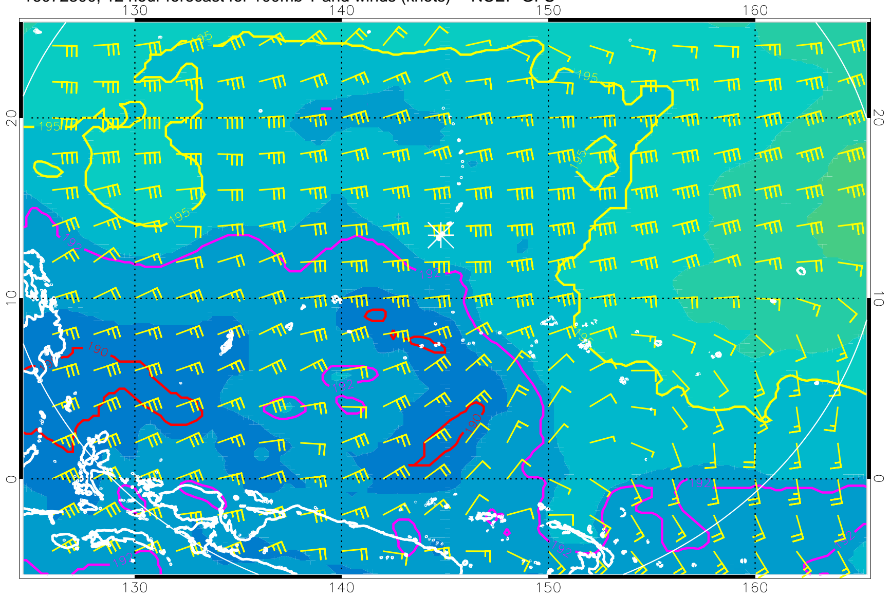
16072300, 12 hour forecast for 100mb T and winds (knots) -- NCEP GFS
