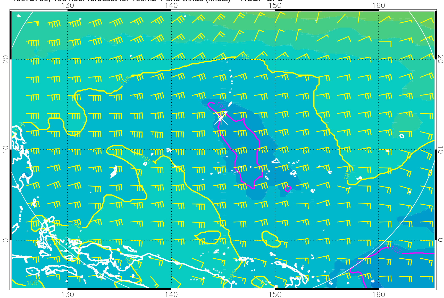
16072700, 108 hour forecast for 100mb T and winds (knots) -- NCEP GFS
