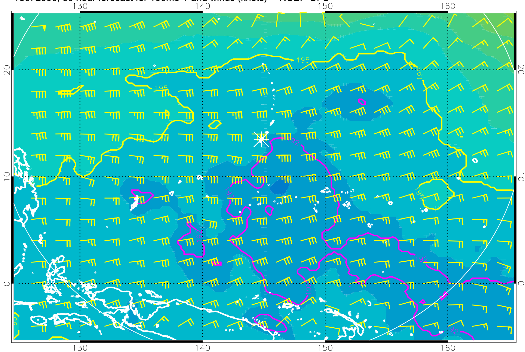
16072606, 90 hour forecast for 100mb T and winds (knots) -- NCEP GFS
