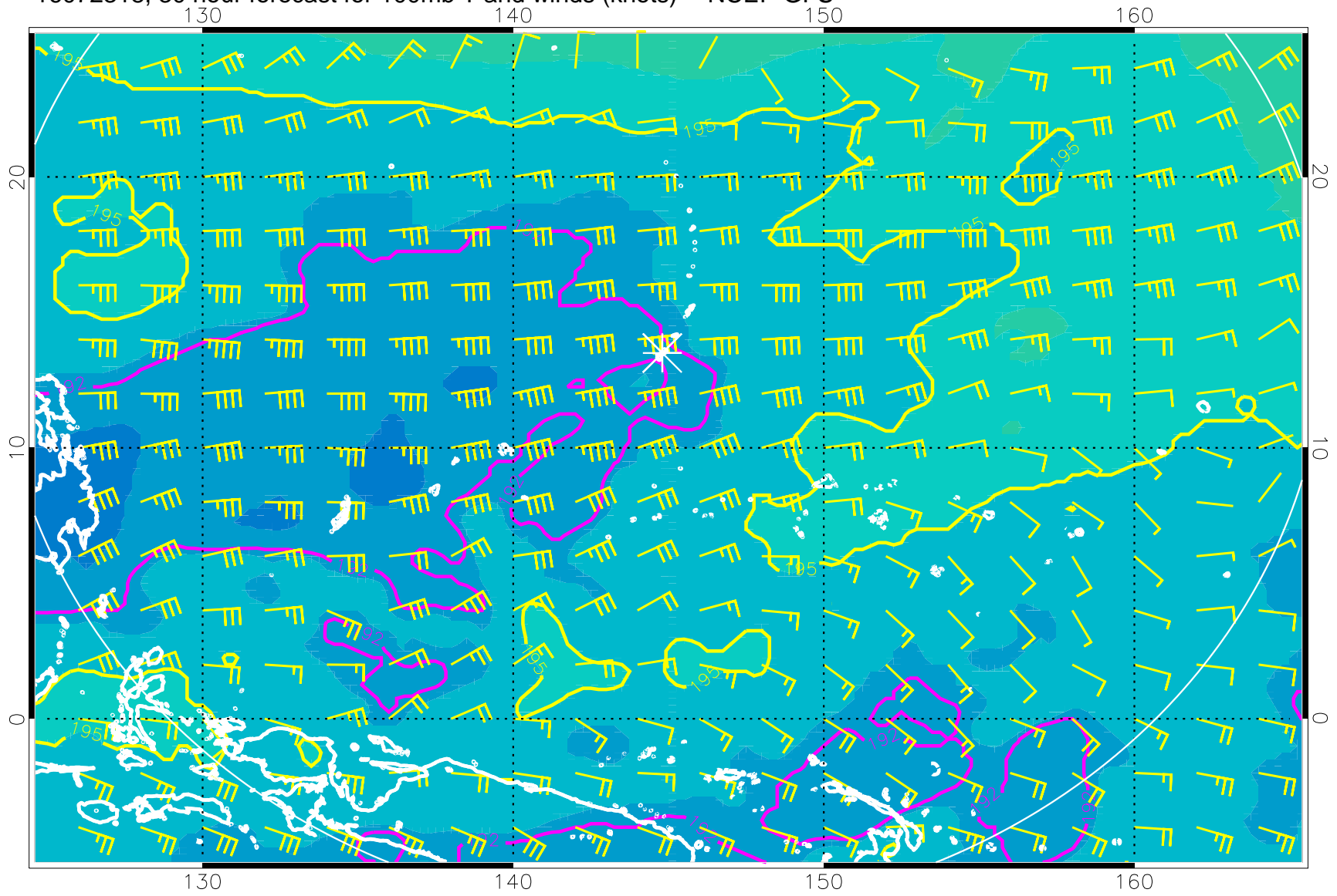
16072318, 30 hour forecast for 100mb T and winds (knots) -- NCEP GFS
