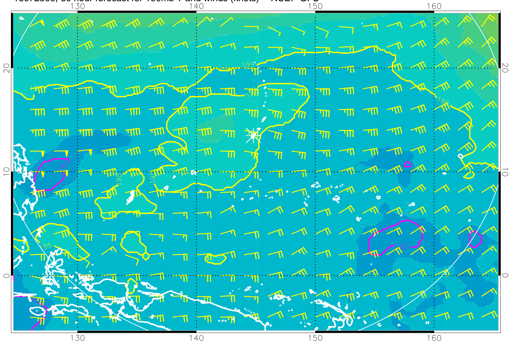
16072500, 60 hour forecast for 100mb T and winds (knots) -- NCEP GFS
