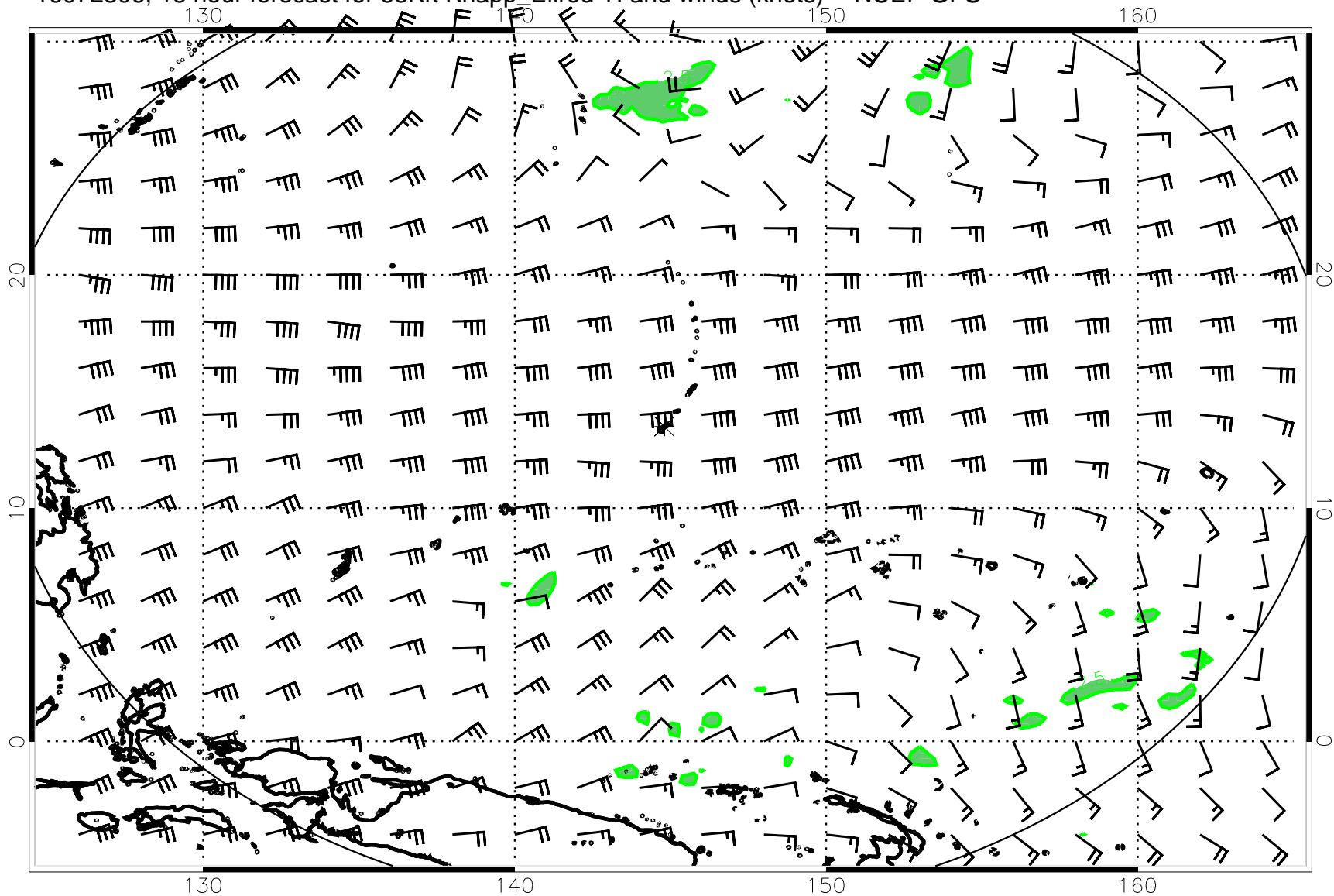
16072306, 18 hour forecast for 53Kft Knapp_Ellrod TI and winds (knots) -- NCEP GFS
