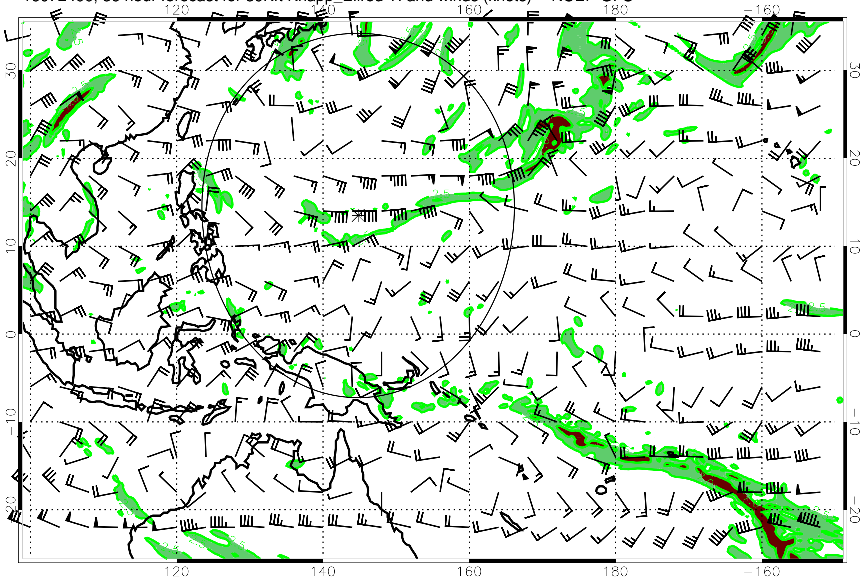
16072400, 36 hour forecast for 39Kft Knapp_Ellrod TI and winds (knots) -- NCEP GFS
