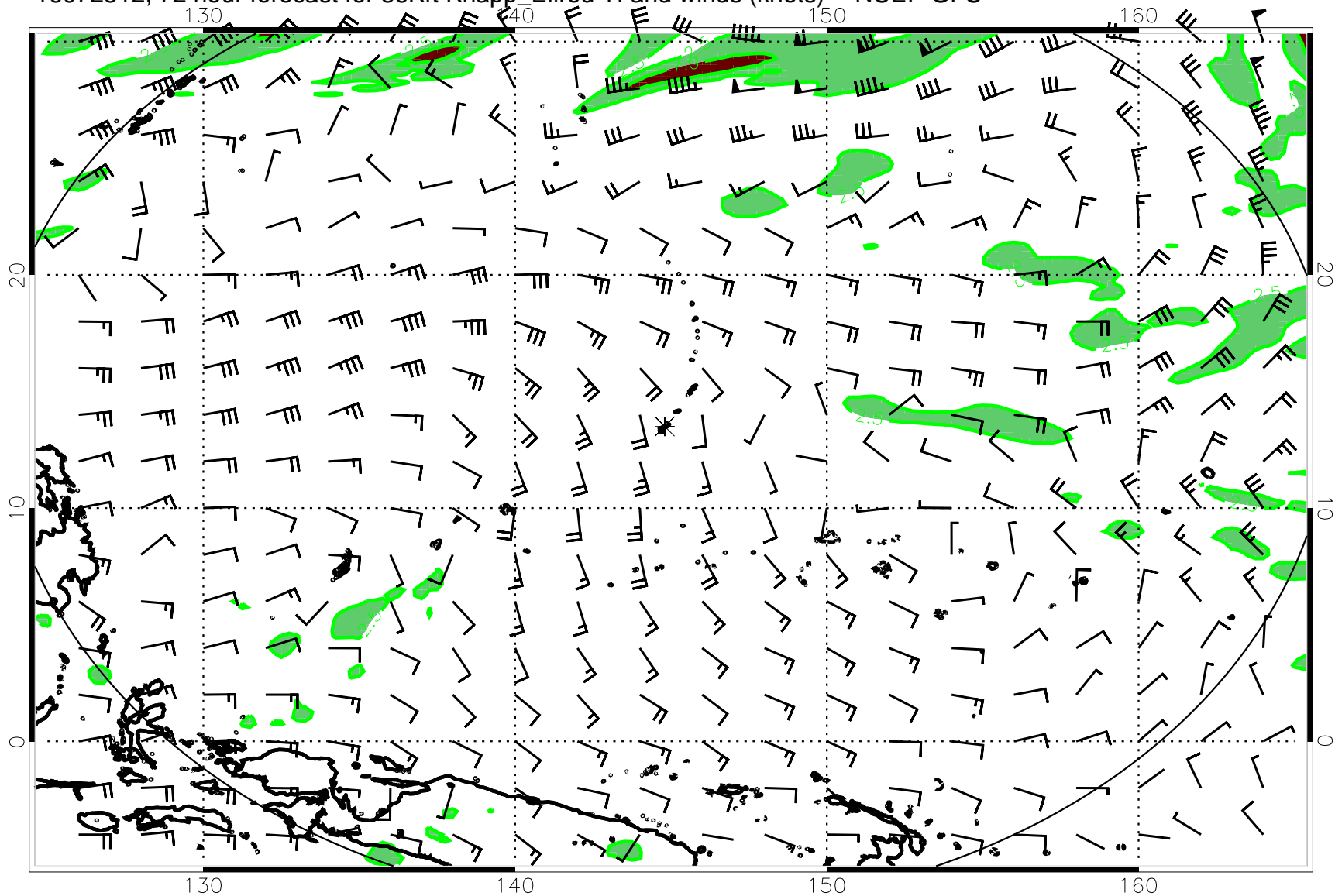
16072512, 72 hour forecast for 36Kft Knapp_Ellrod TI and winds (knots) -- NCEP GFS
