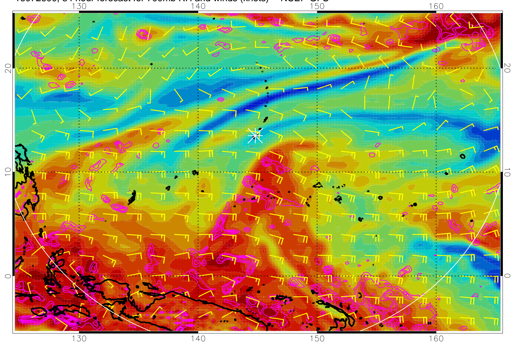
16072600, 84 hour forecast for 700mb RH and winds (knots) -- NCEP GFS
