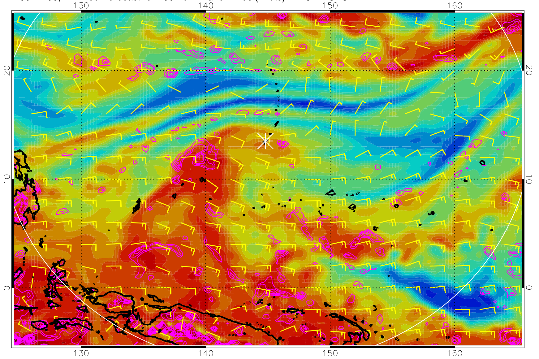
16072706, 114 hour forecast for 700mb RH and winds (knots) -- NCEP GFS
