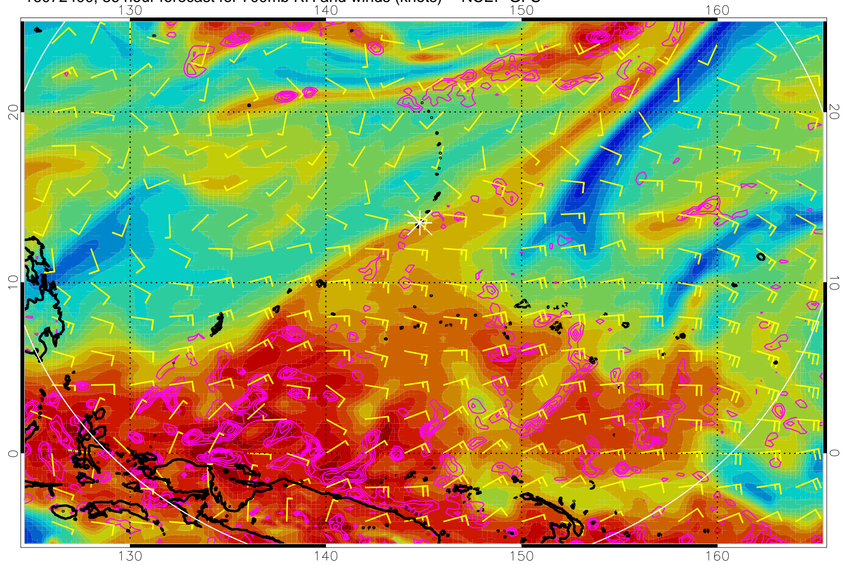
16072400, 36 hour forecast for 700mb RH and winds (knots) -- NCEP GFS
