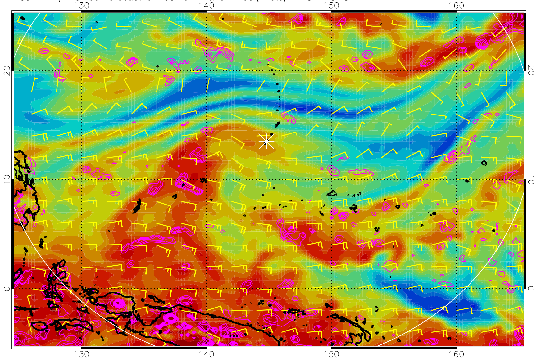
16072712, 120 hour forecast for 700mb RH and winds (knots) -- NCEP GFS
