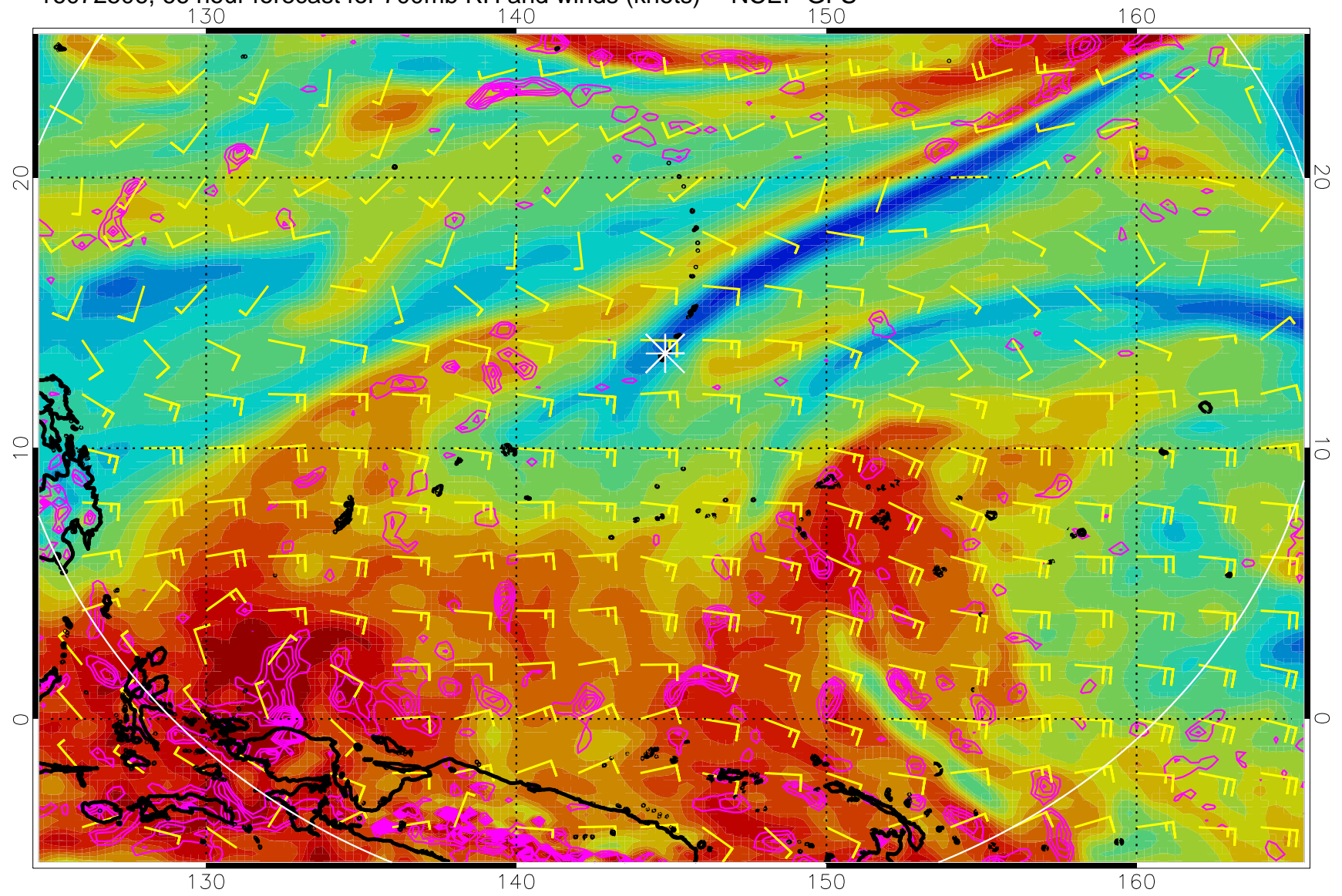
16072506, 66 hour forecast for 700mb RH and winds (knots) -- NCEP GFS
