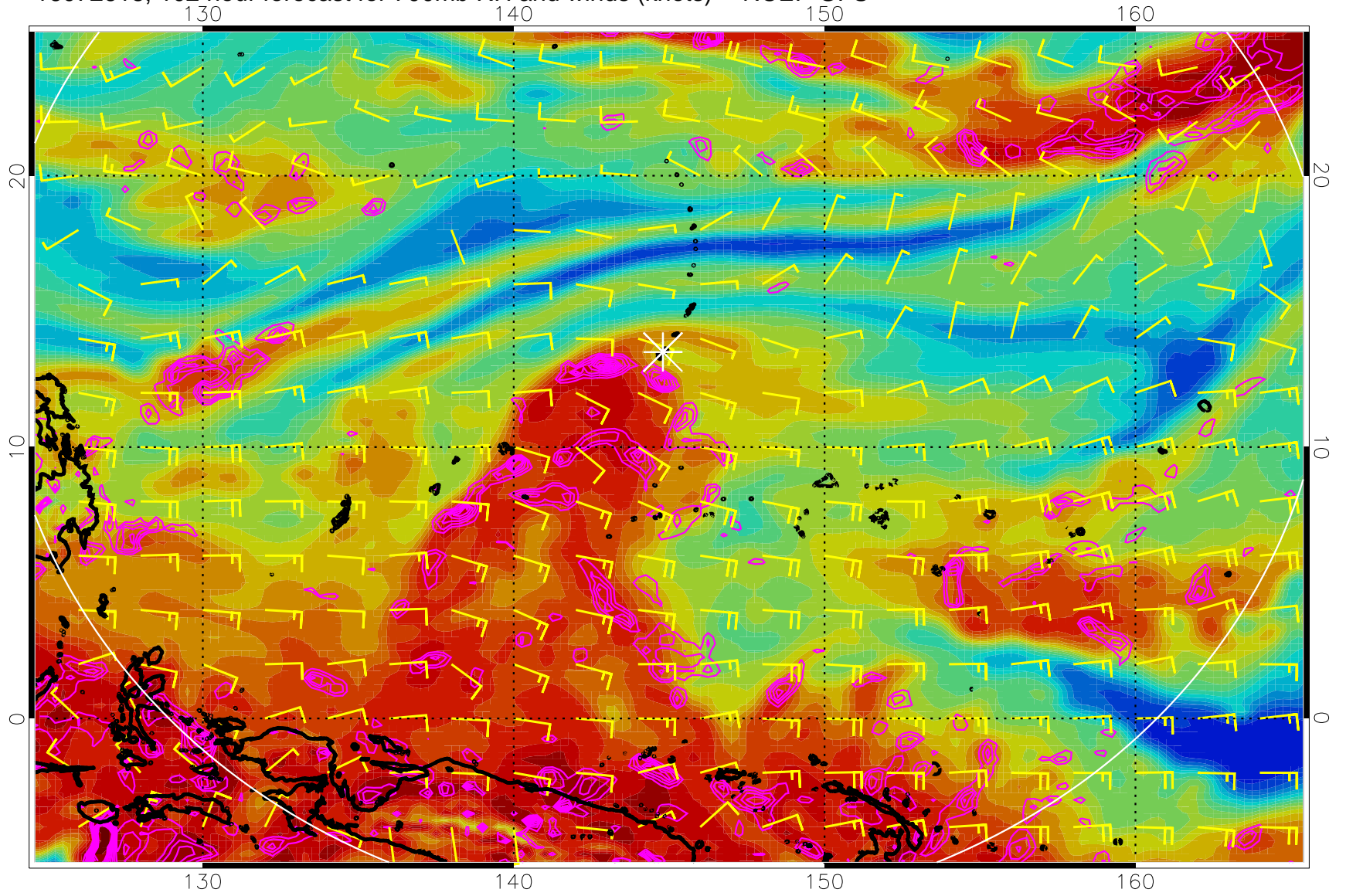
16072618, 102 hour forecast for 700mb RH and winds (knots) -- NCEP GFS
