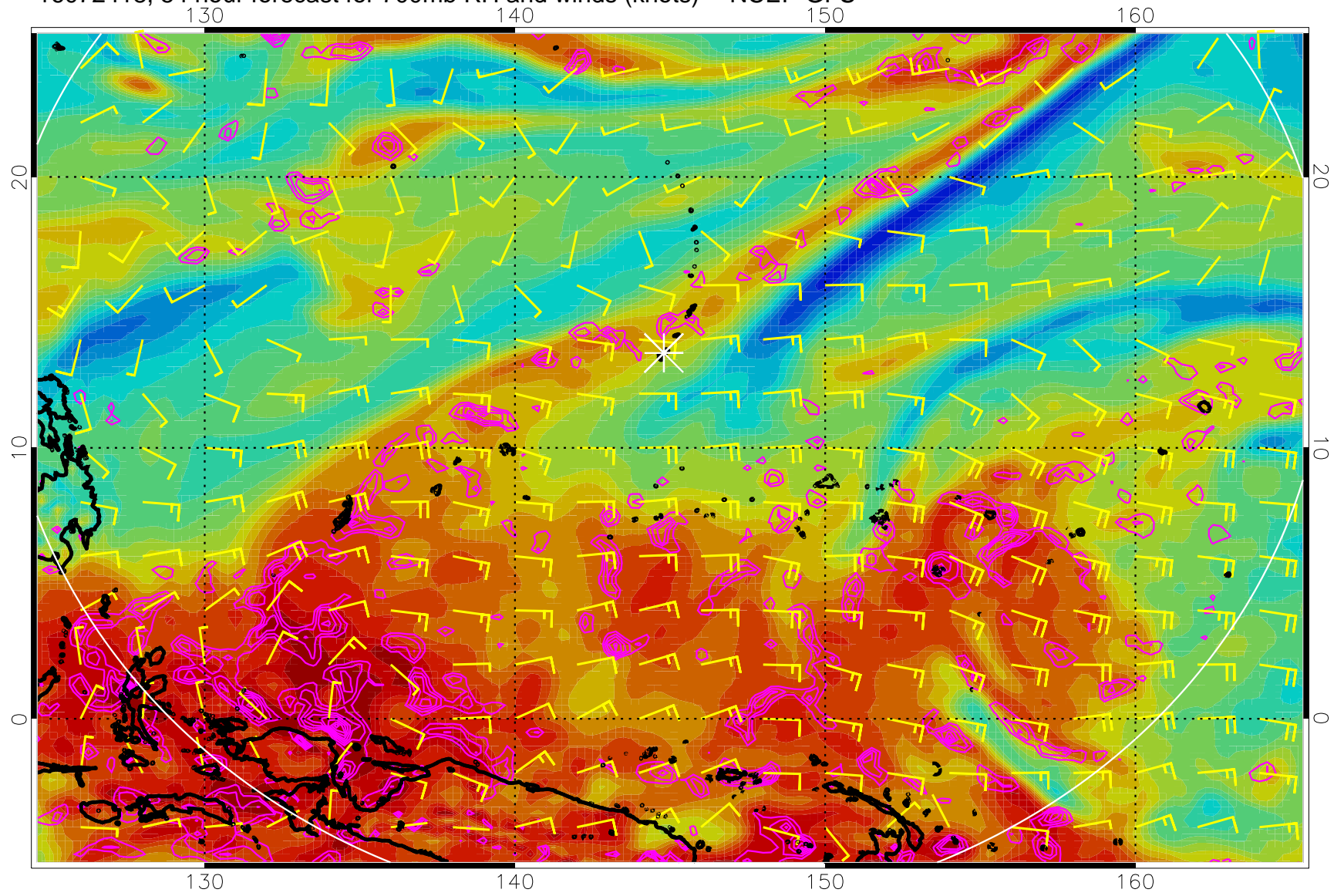
16072418, 54 hour forecast for 700mb RH and winds (knots) -- NCEP GFS
