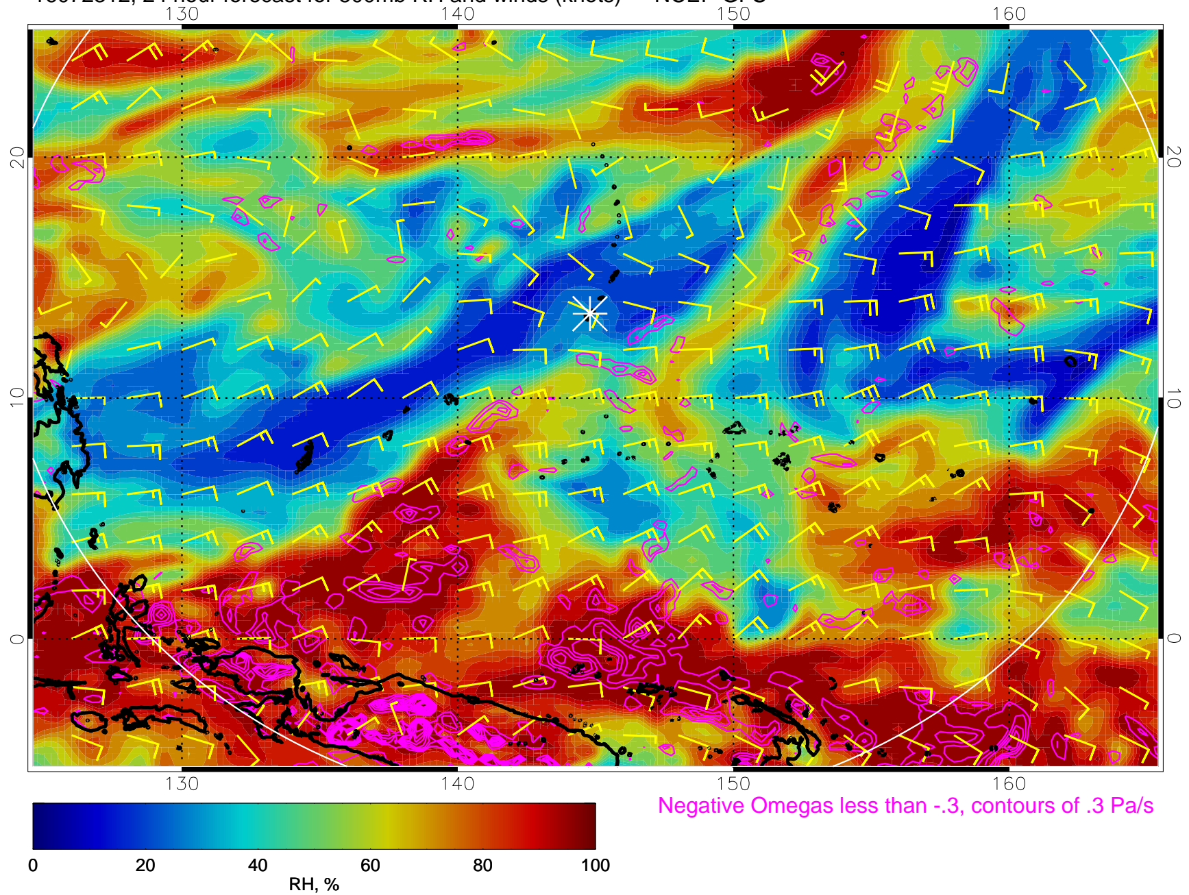
16072312, 24 hour forecast for 500mb RH and winds (knots) -- NCEP GFS
