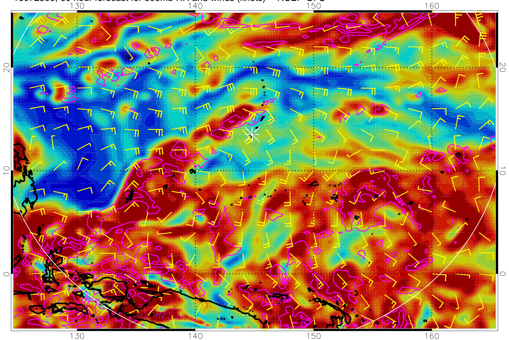
16072500, 60 hour forecast for 300mb RH and winds (knots) -- NCEP GFS
