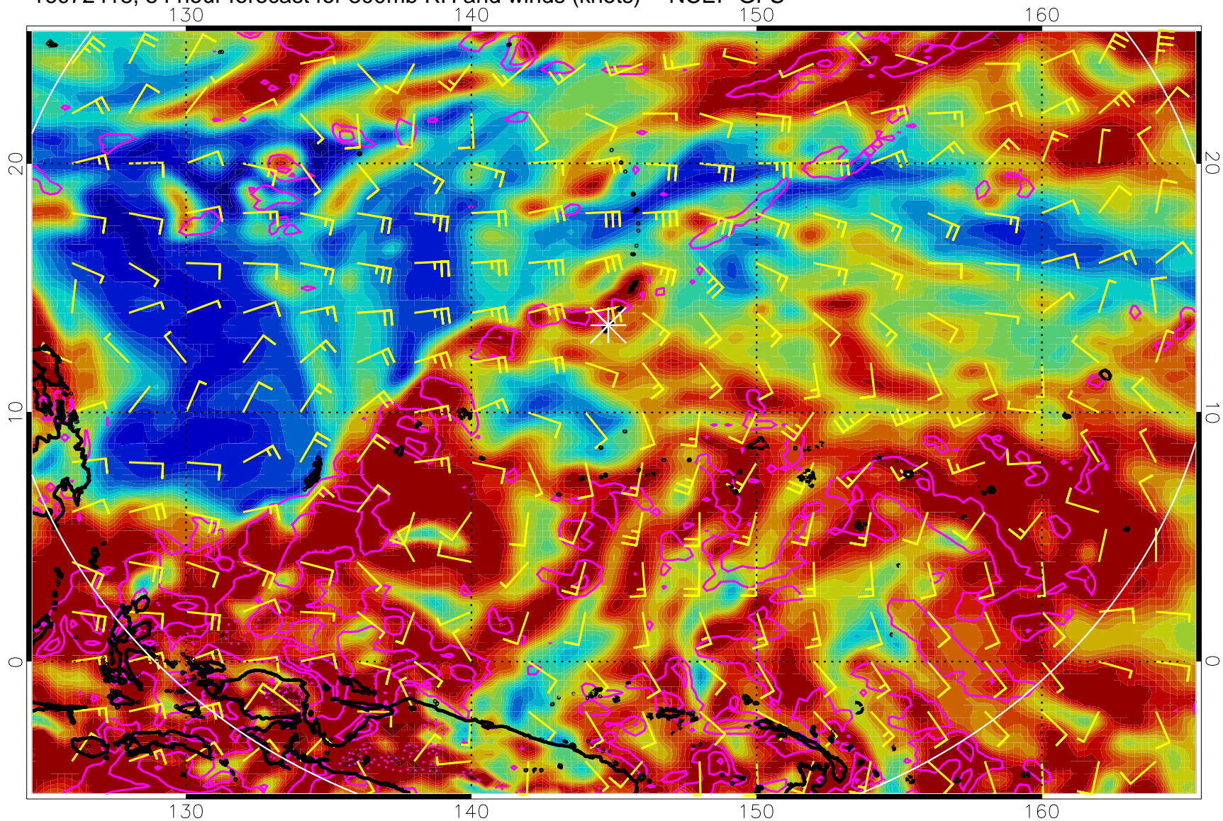
16072418, 54 hour forecast for 300mb RH and winds (knots) -- NCEP GFS
