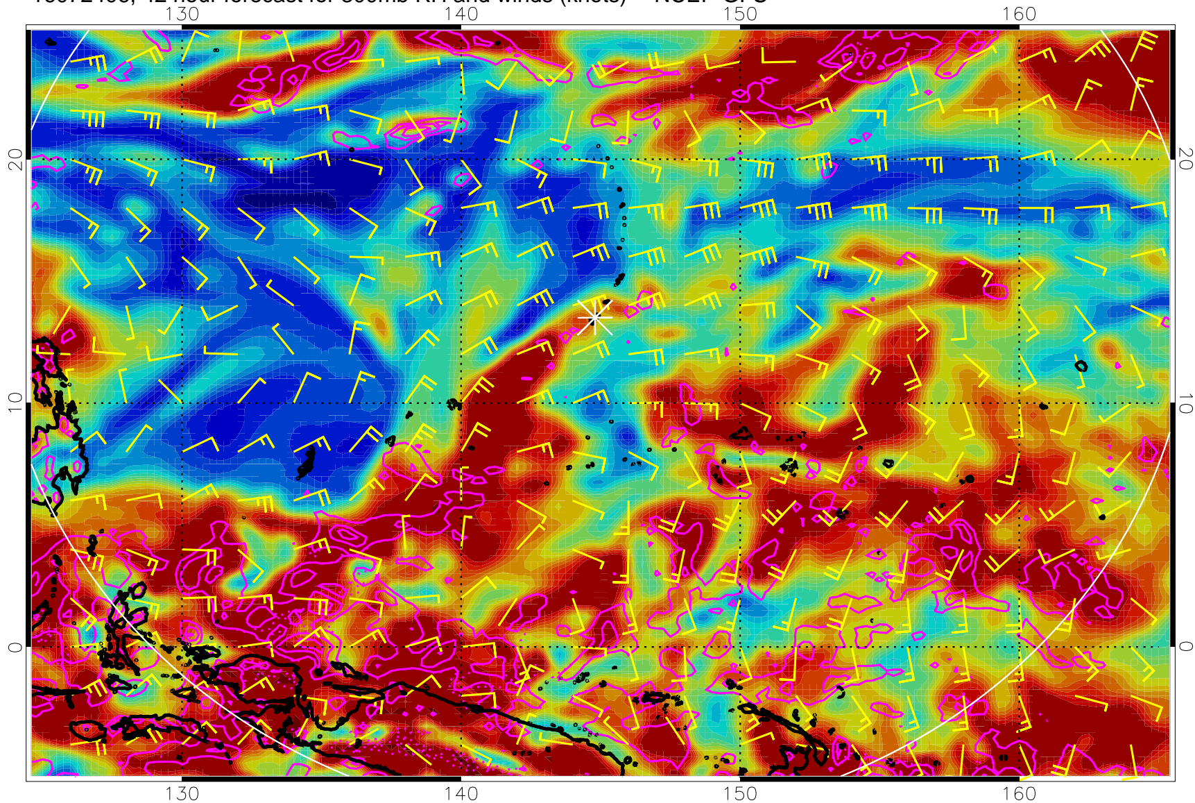
16072406, 42 hour forecast for 300mb RH and winds (knots) -- NCEP GFS
