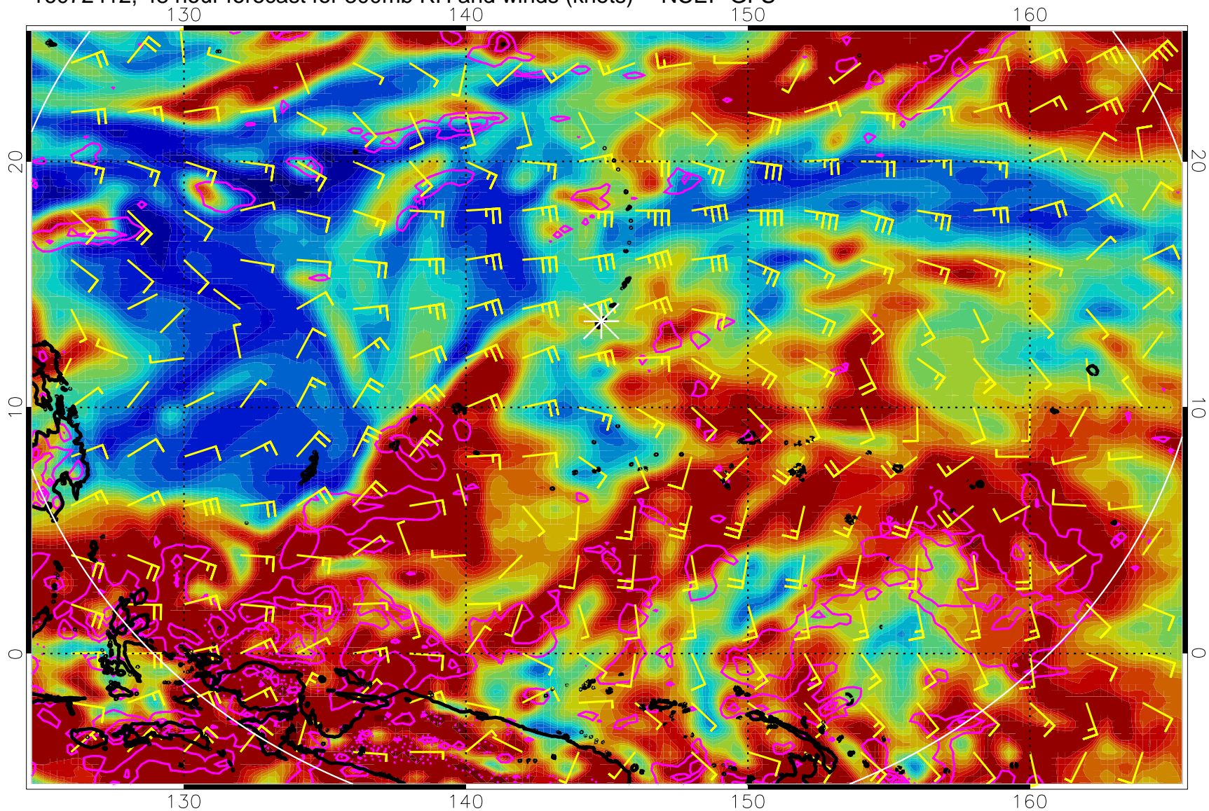
16072412, 48 hour forecast for 300mb RH and winds (knots) -- NCEP GFS
