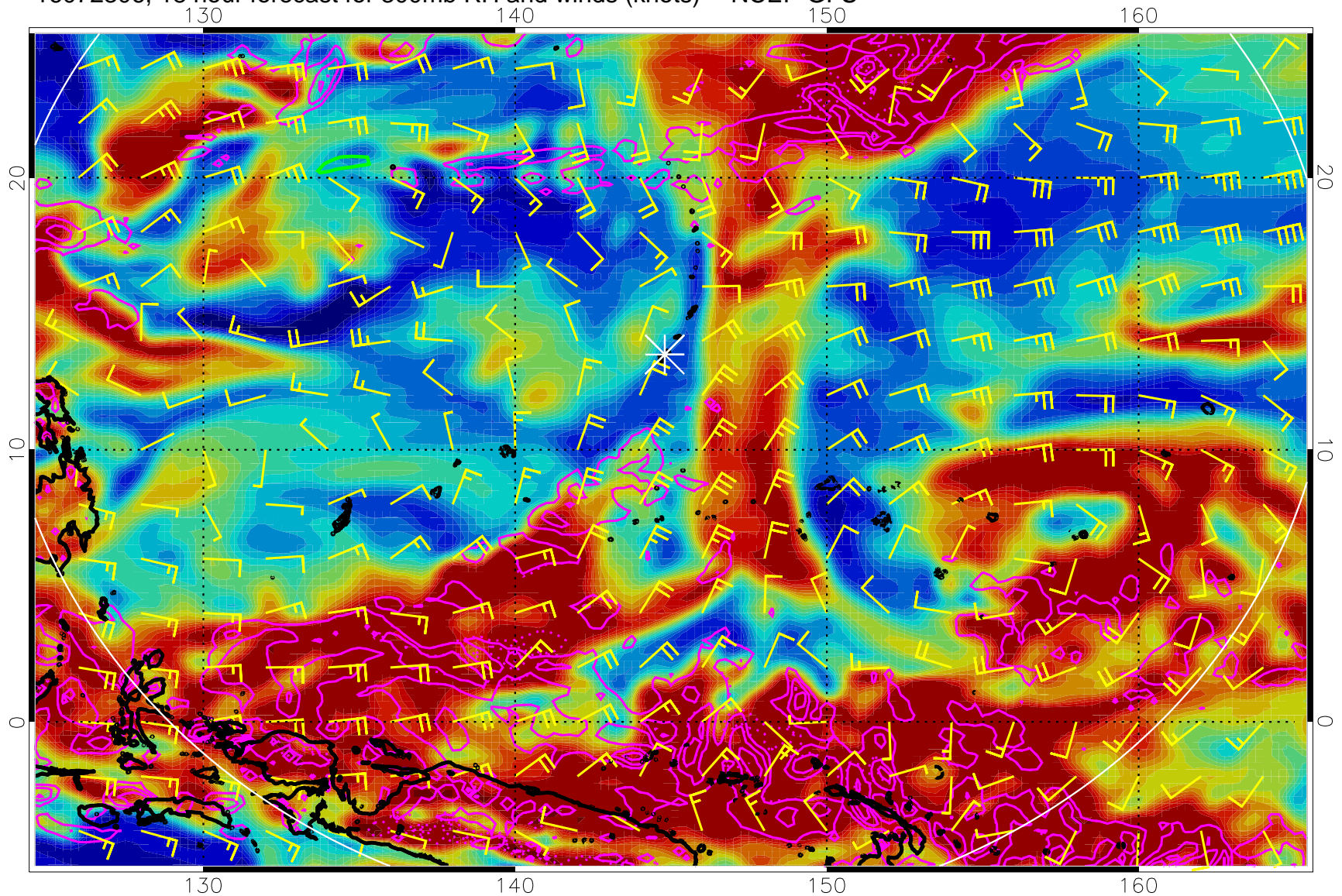
16072306, 18 hour forecast for 300mb RH and winds (knots) -- NCEP GFS
