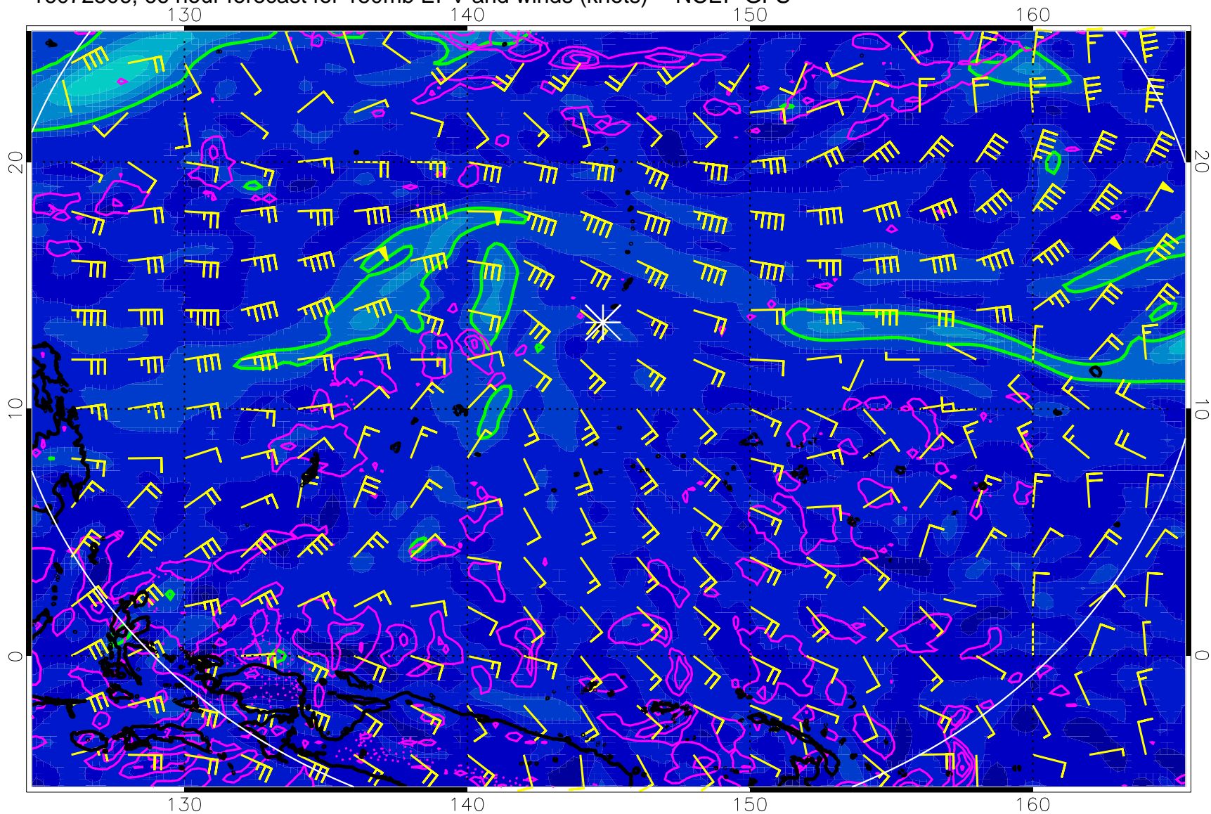
16072506, 66 hour forecast for 150mb EPV and winds (knots) -- NCEP GFS
