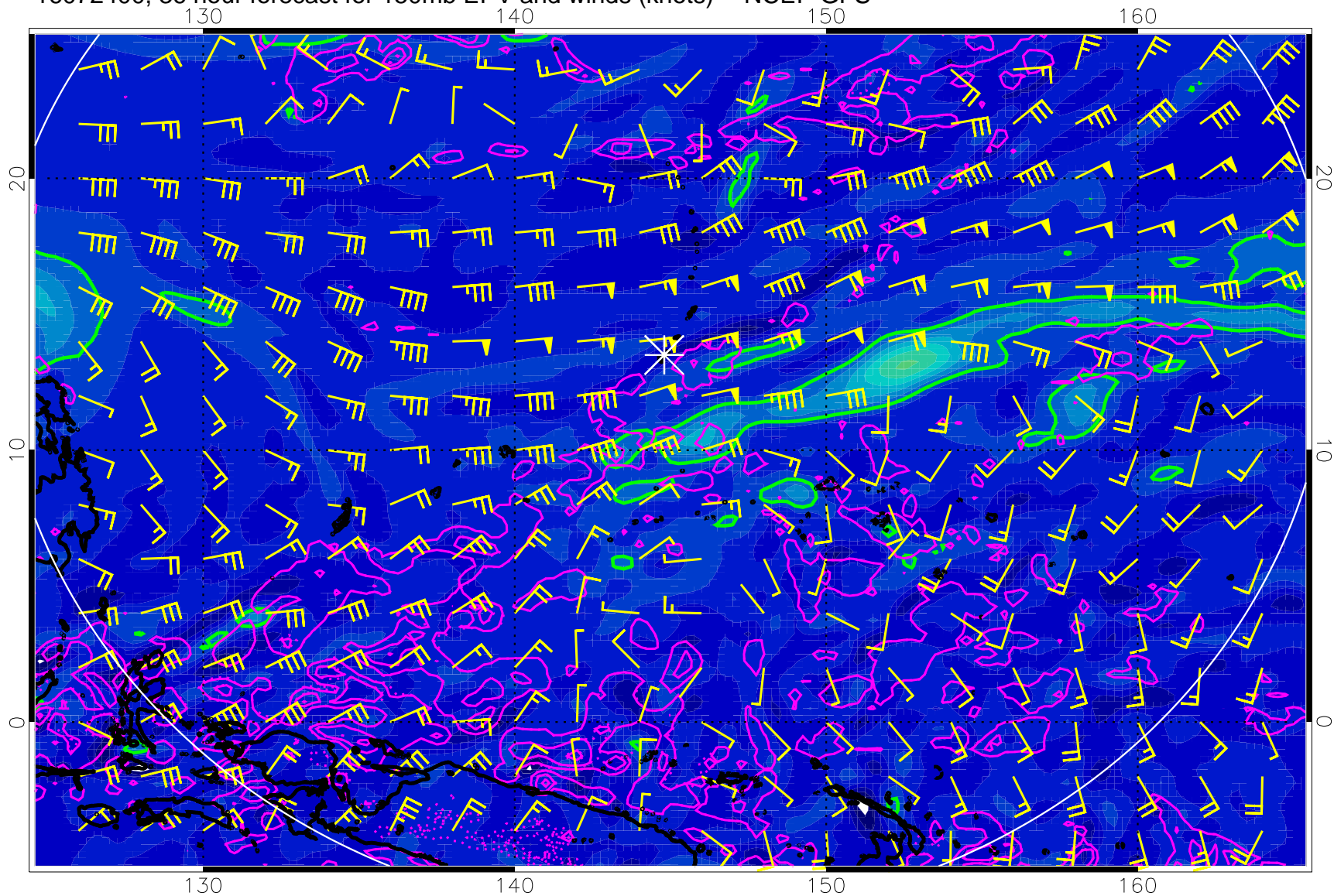
16072400, 36 hour forecast for 150mb EPV and winds (knots) -- NCEP GFS
