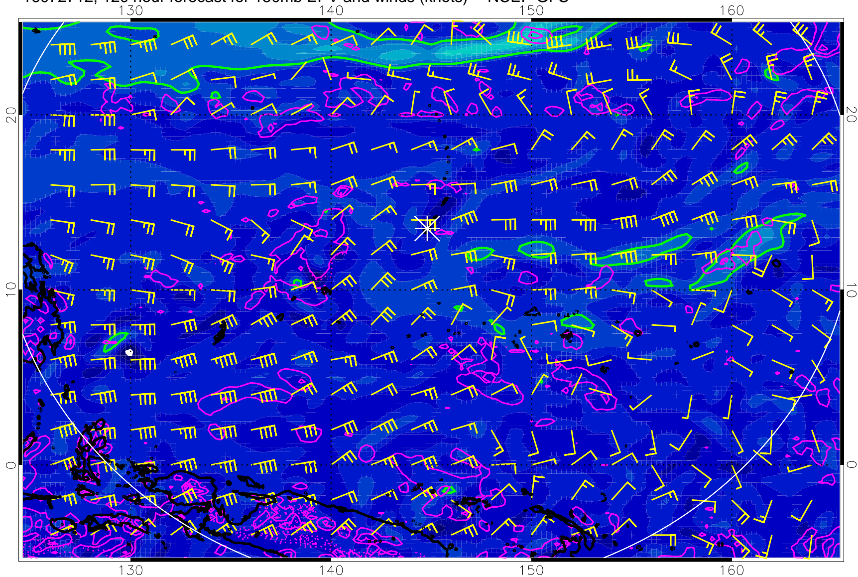
16072712, 120 hour forecast for 150mb EPV and winds (knots) -- NCEP GFS
