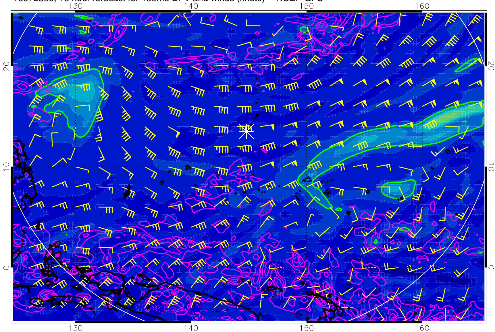
16072306, 18 hour forecast for 150mb EPV and winds (knots) -- NCEP GFS
