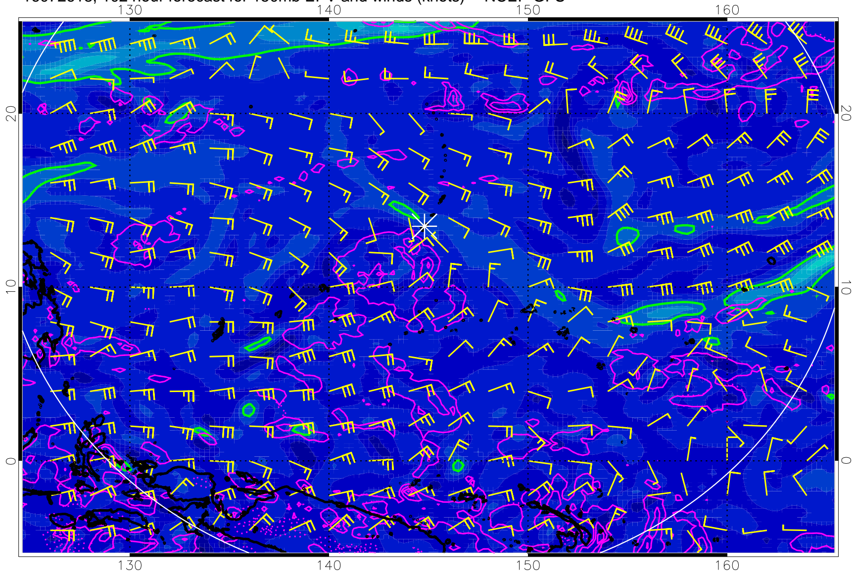
16072618, 102 hour forecast for 150mb EPV and winds (knots) -- NCEP GFS
