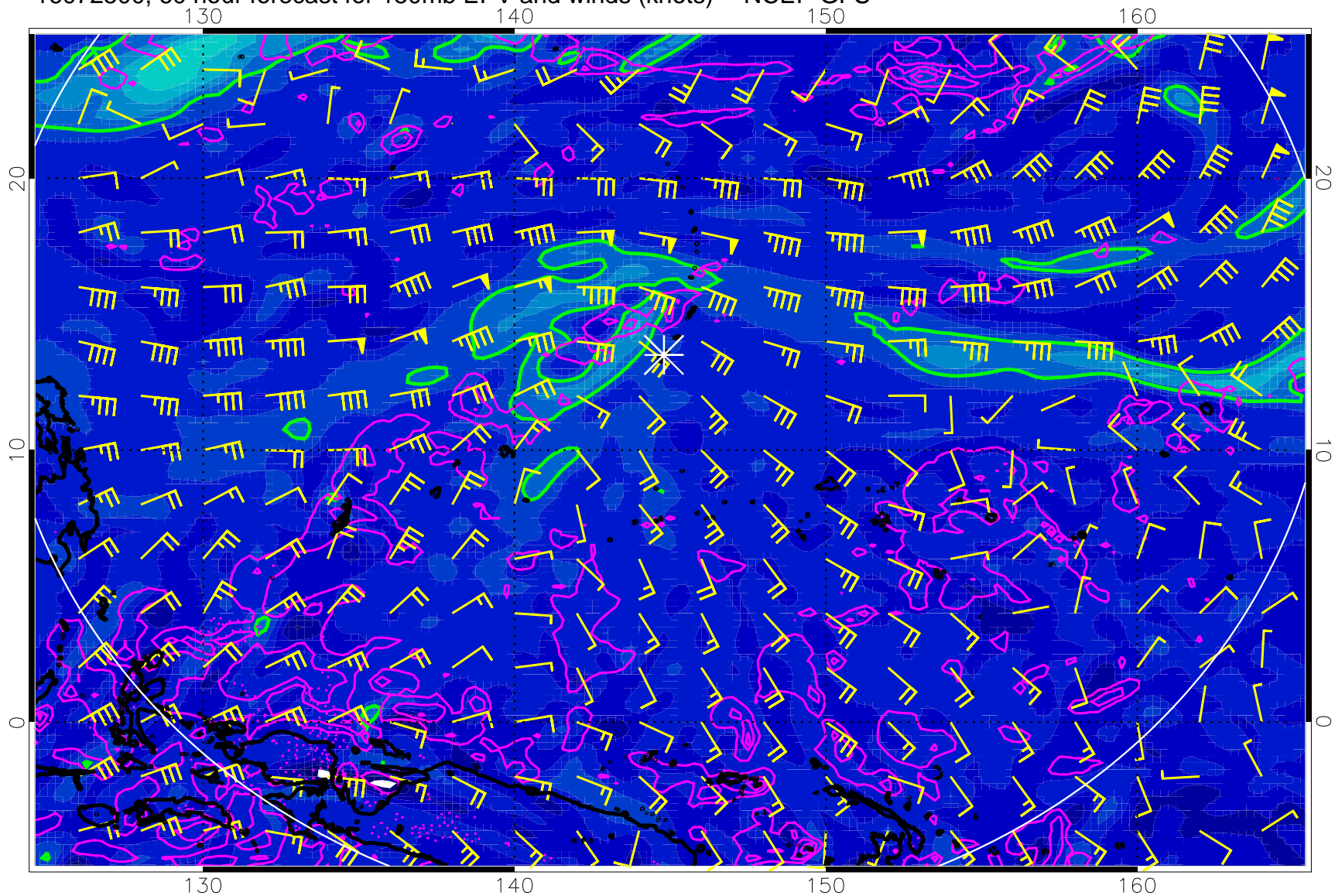
16072500, 60 hour forecast for 150mb EPV and winds (knots) -- NCEP GFS
