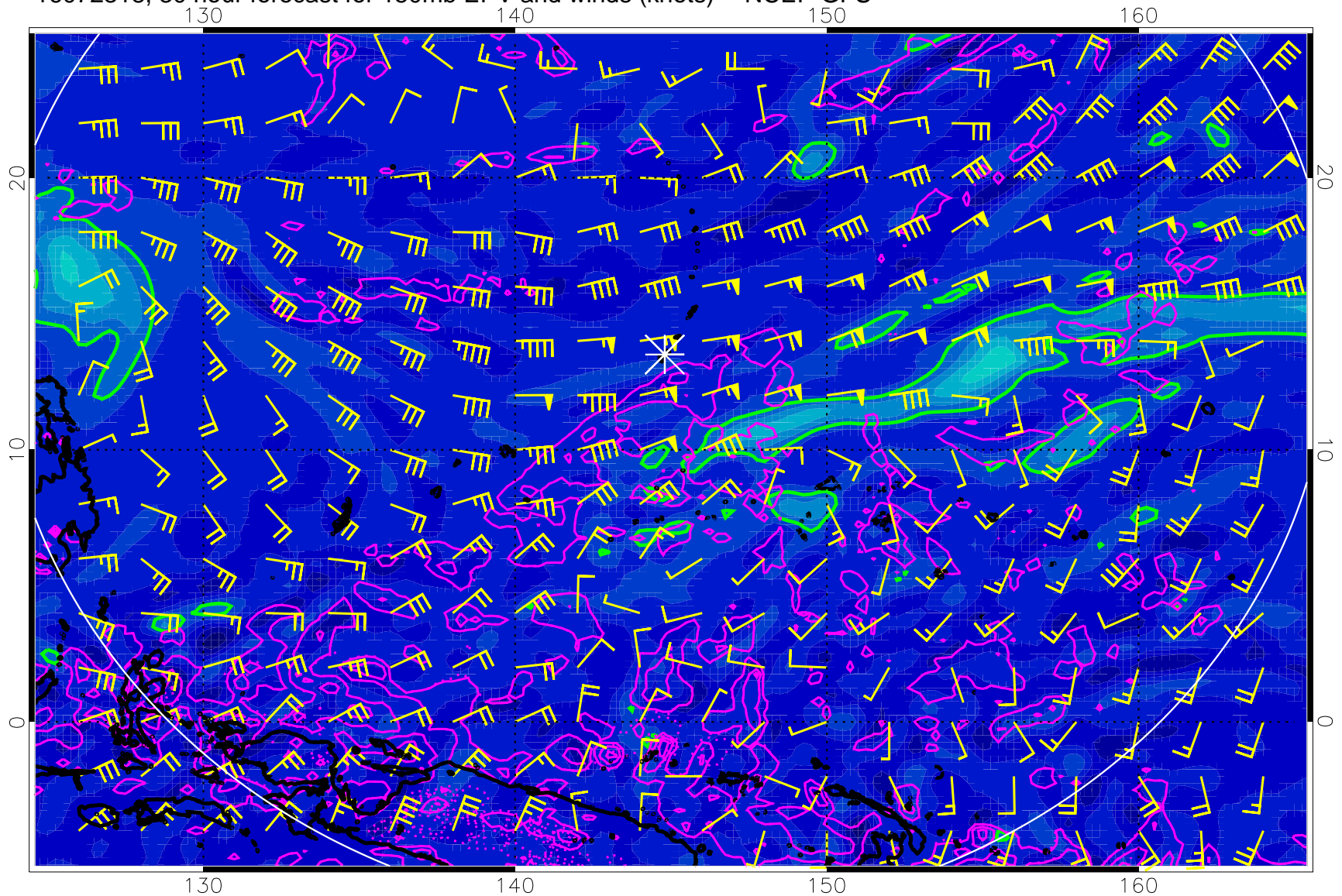
16072318, 30 hour forecast for 150mb EPV and winds (knots) -- NCEP GFS
