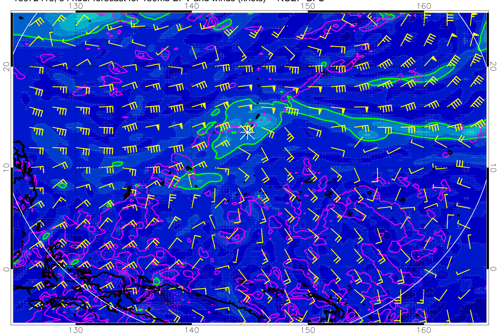
16072418, 54 hour forecast for 150mb EPV and winds (knots) -- NCEP GFS
