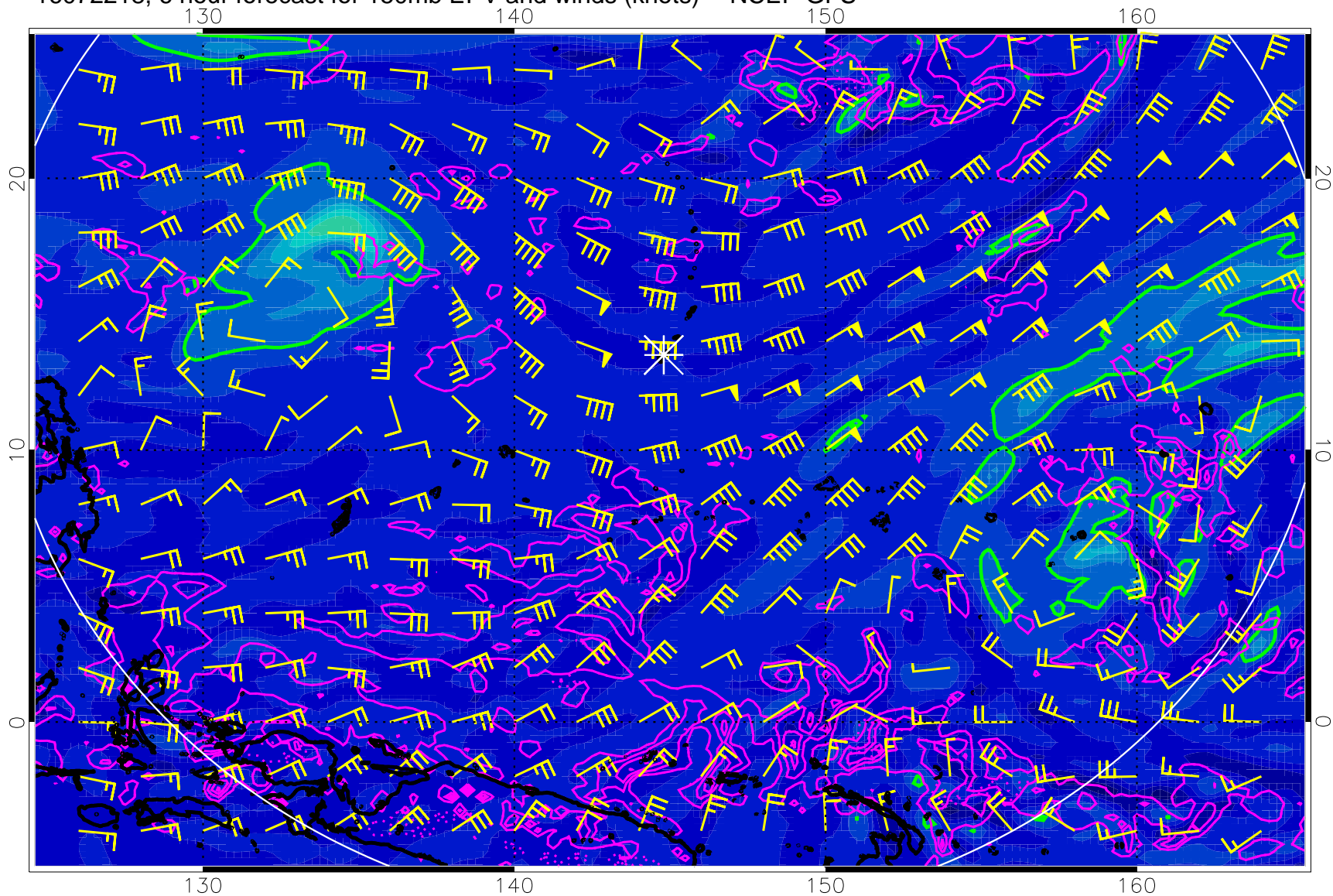
16072218, 6 hour forecast for 150mb EPV and winds (knots) -- NCEP GFS
