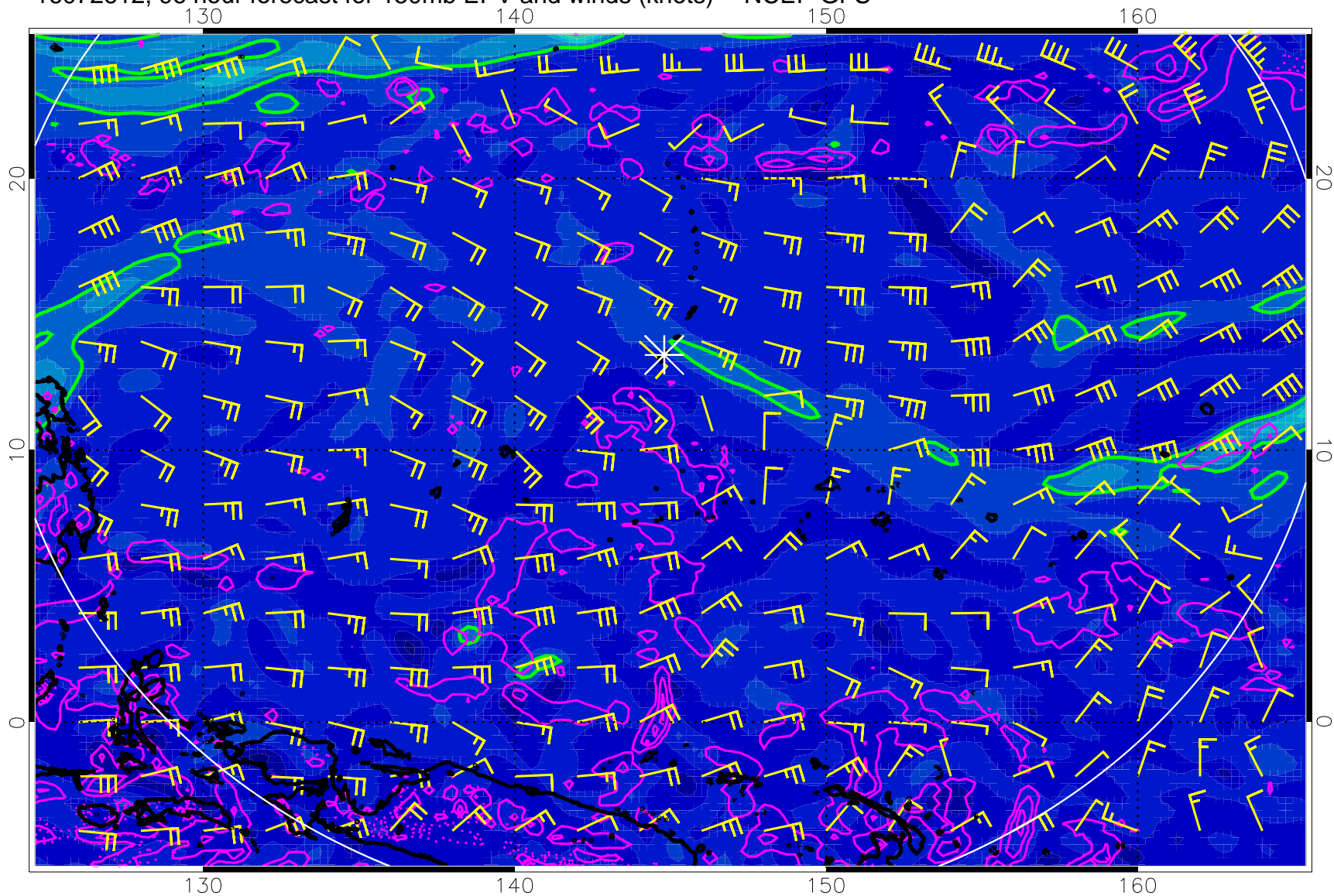
16072612, 96 hour forecast for 150mb EPV and winds (knots) -- NCEP GFS
