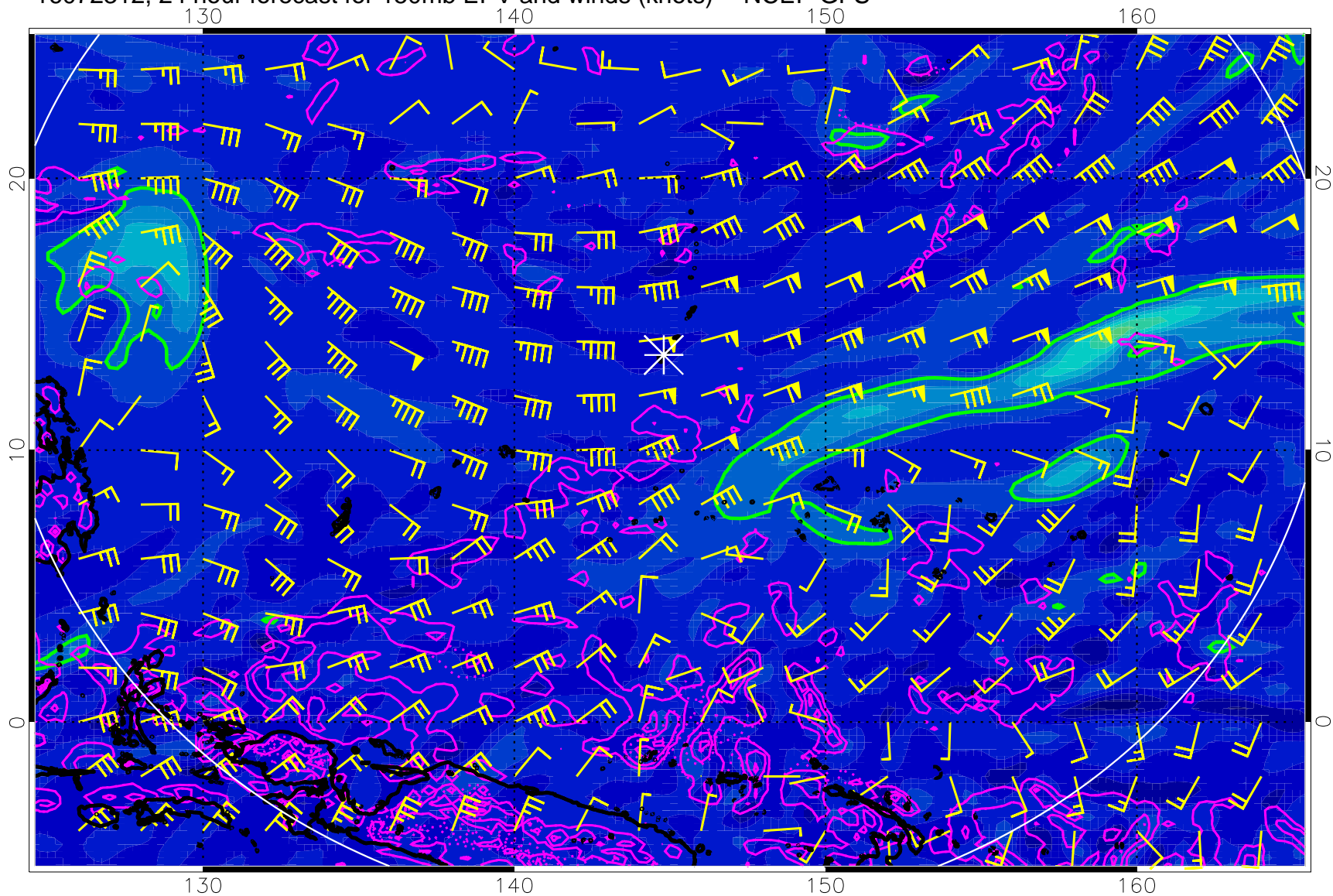
16072312, 24 hour forecast for 150mb EPV and winds (knots) -- NCEP GFS
