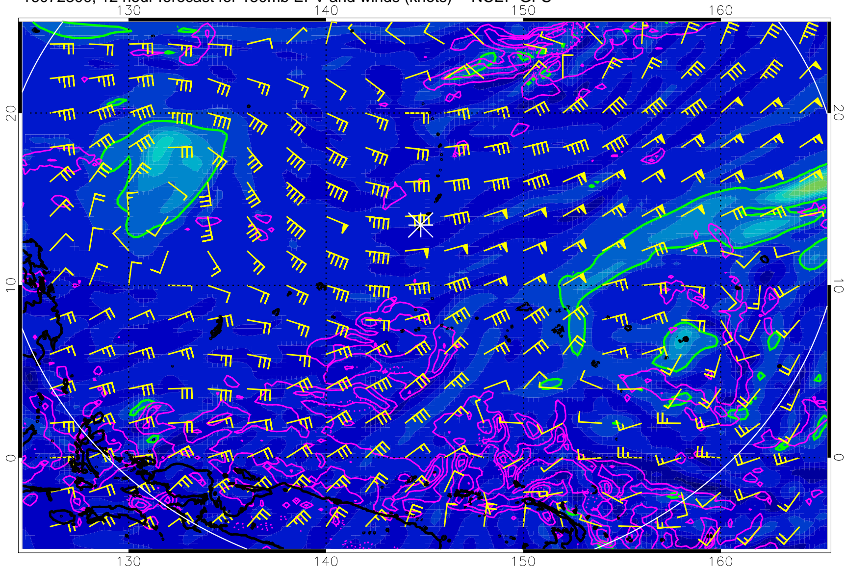
16072300, 12 hour forecast for 150mb EPV and winds (knots) -- NCEP GFS
