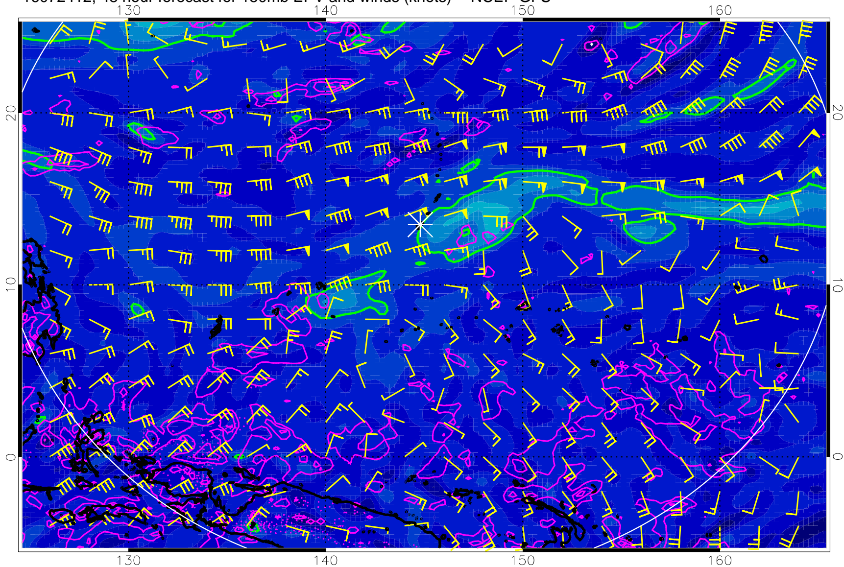
16072412, 48 hour forecast for 150mb EPV and winds (knots) -- NCEP GFS
