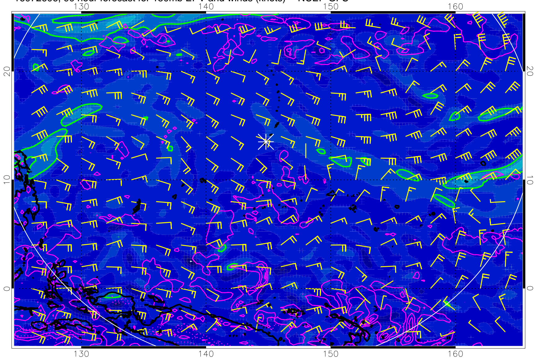
16072606, 90 hour forecast for 150mb EPV and winds (knots) -- NCEP GFS
