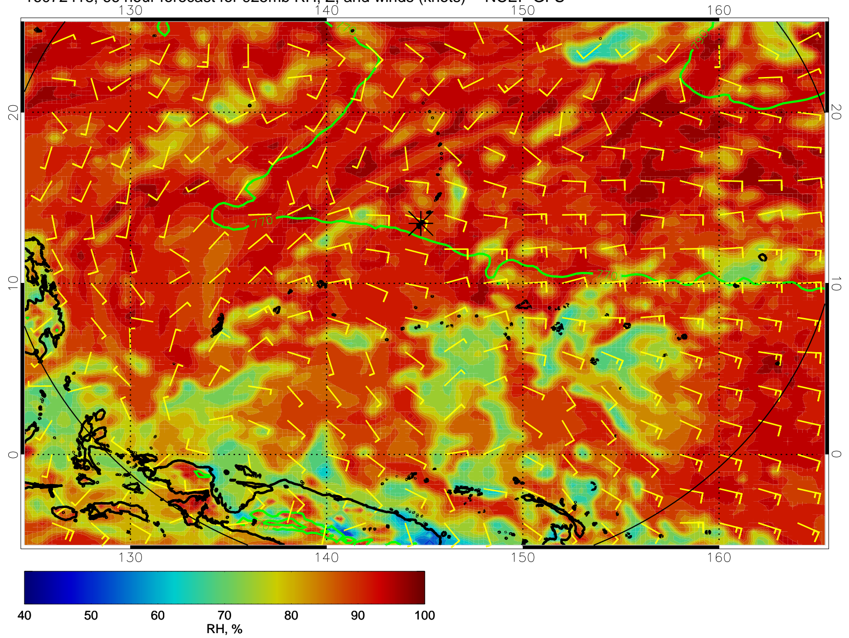
16072418, 66 hour forecast for 925mb RH, Z, and winds (knots) -- NCEP GFS
