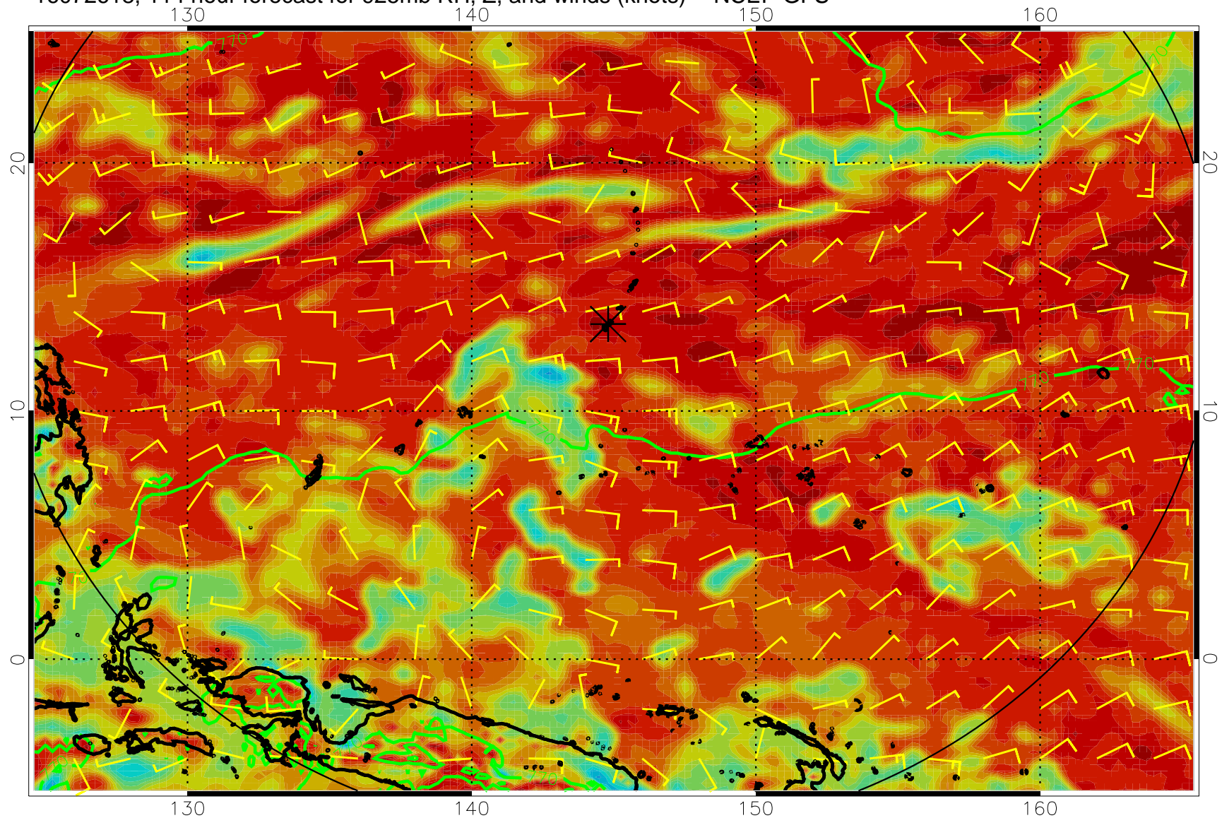
16072618, 114 hour forecast for 925mb RH, Z, and winds (knots) -- NCEP GFS
