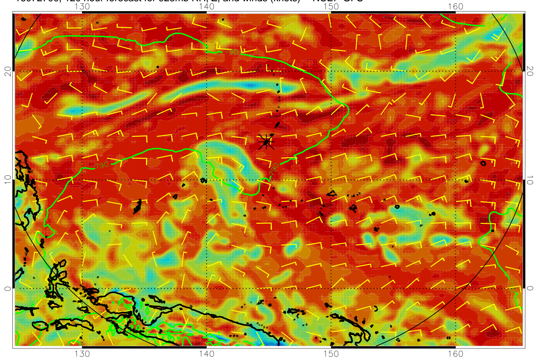
16072700, 120 hour forecast for 925mb RH, Z, and winds (knots) -- NCEP GFS
