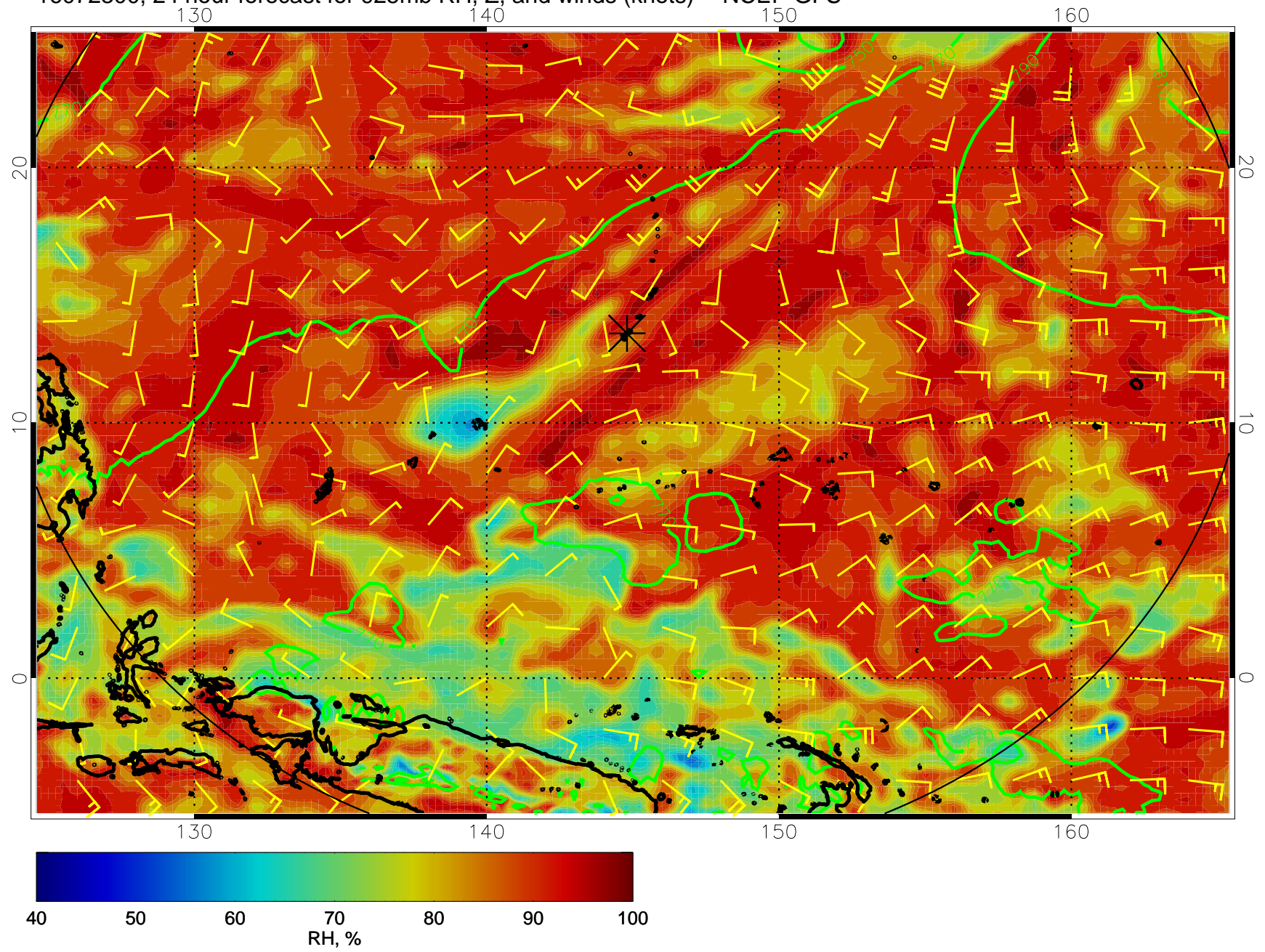
16072300, 24 hour forecast for 925mb RH, Z, and winds (knots) -- NCEP GFS
