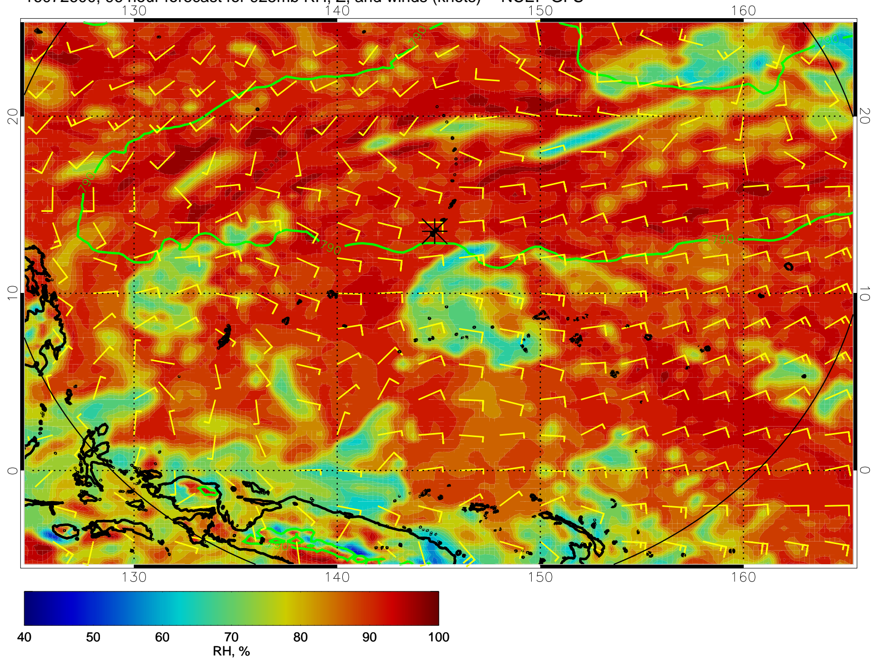
16072600, 96 hour forecast for 925mb RH, Z, and winds (knots) -- NCEP GFS
