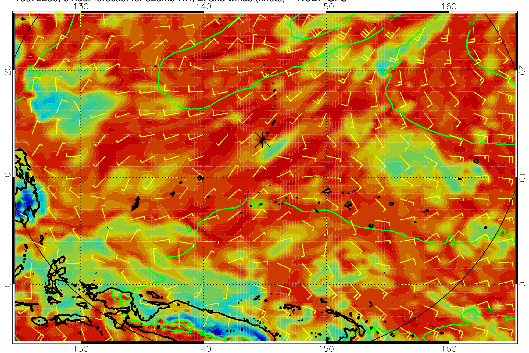
16072206, 6 hour forecast for 925mb RH, Z, and winds (knots) -- NCEP GFS
