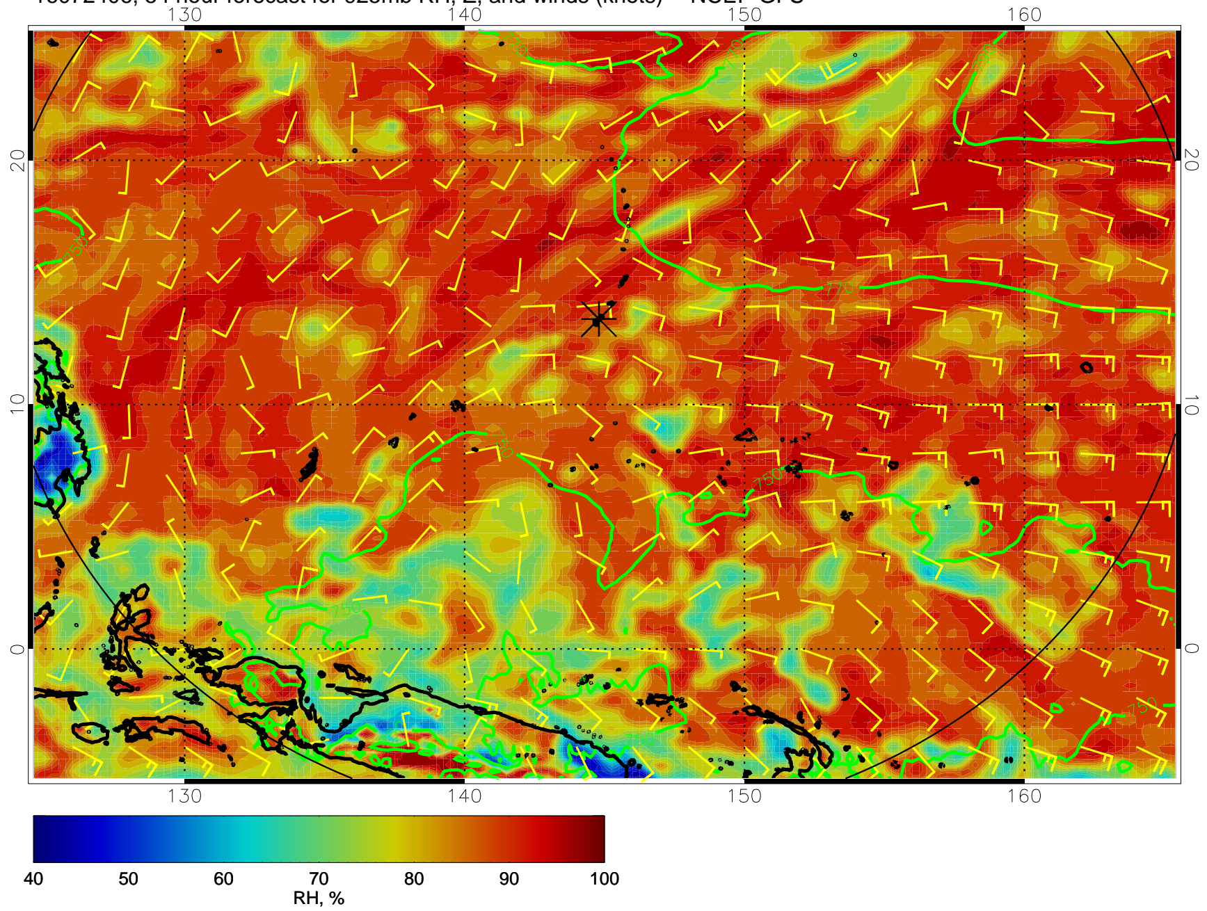
16072406, 54 hour forecast for 925mb RH, Z, and winds (knots) -- NCEP GFS
