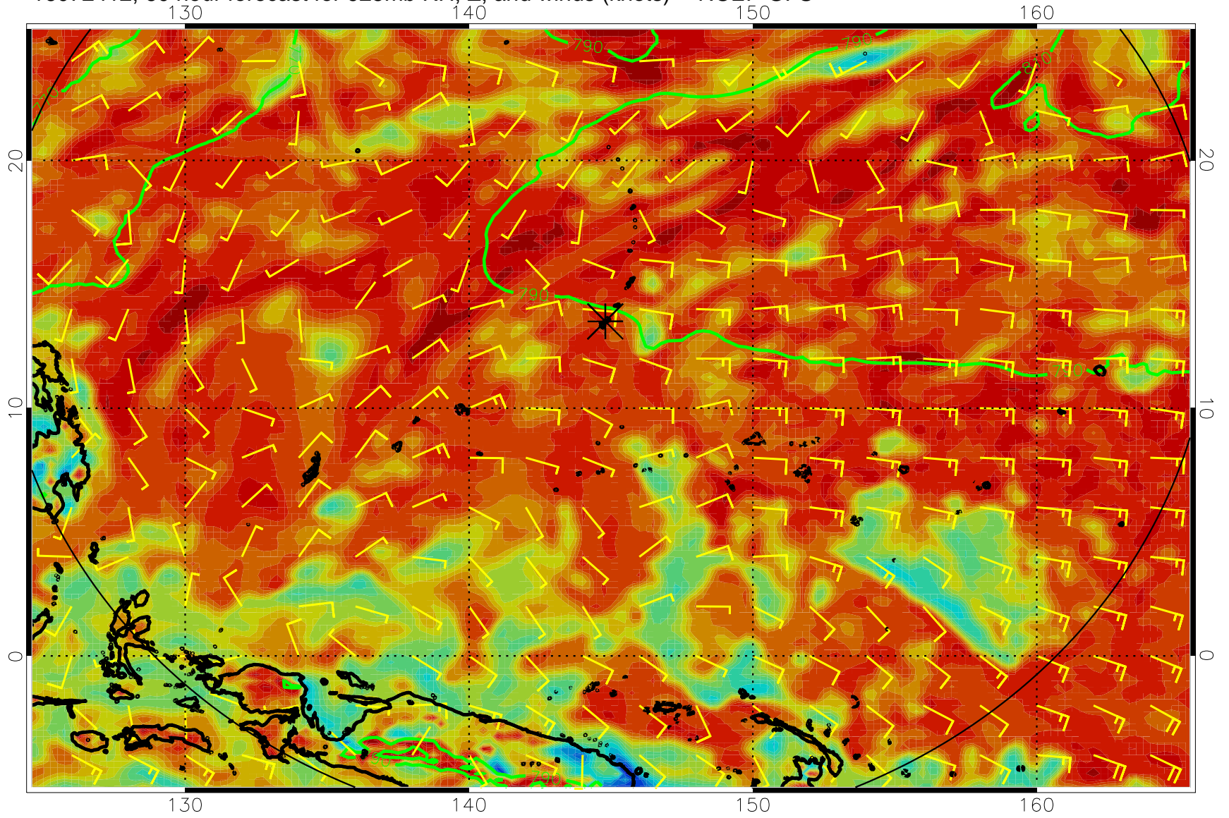
16072412, 60 hour forecast for 925mb RH, Z, and winds (knots) -- NCEP GFS
