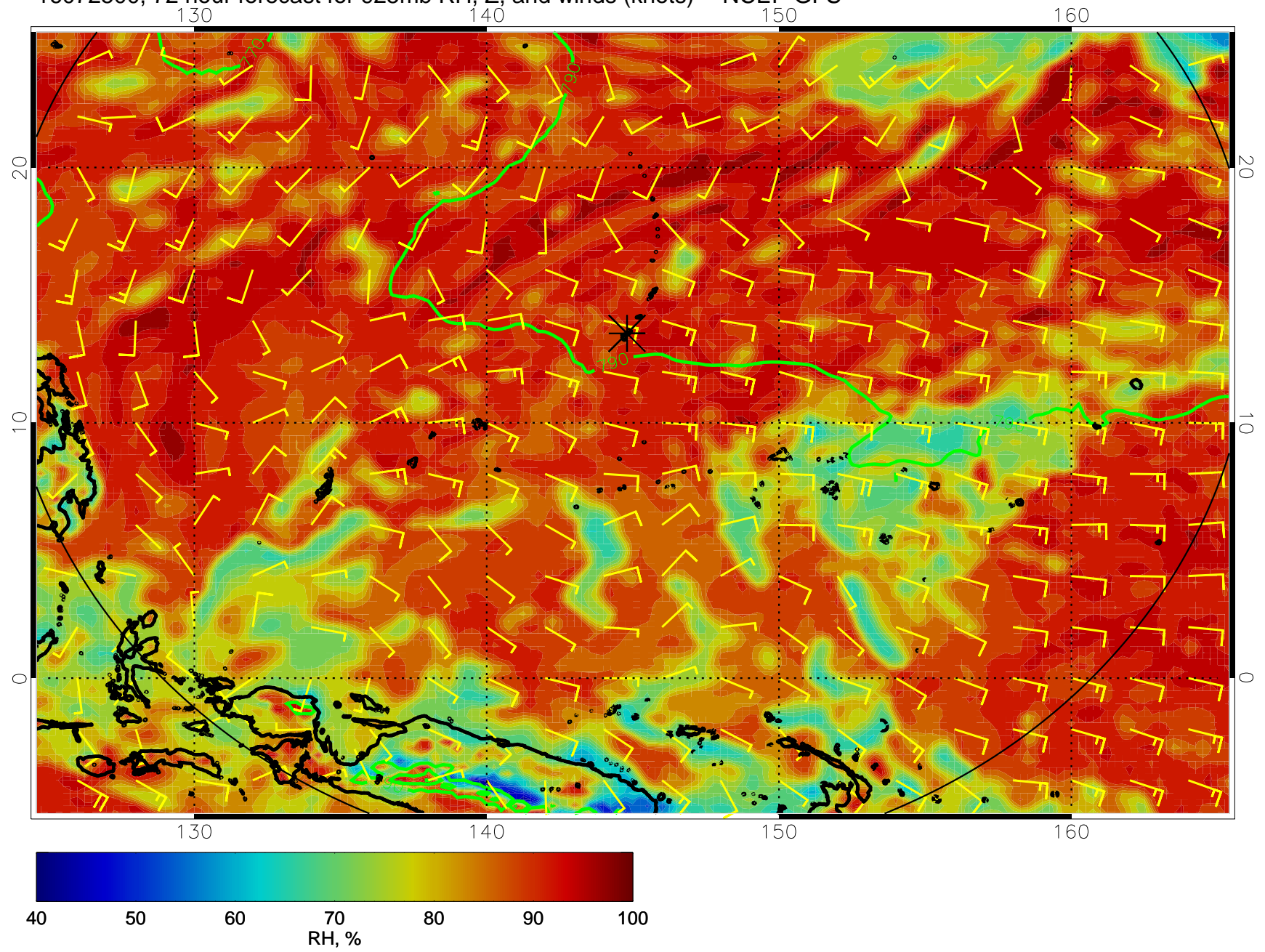
16072500, 72 hour forecast for 925mb RH, Z, and winds (knots) -- NCEP GFS
