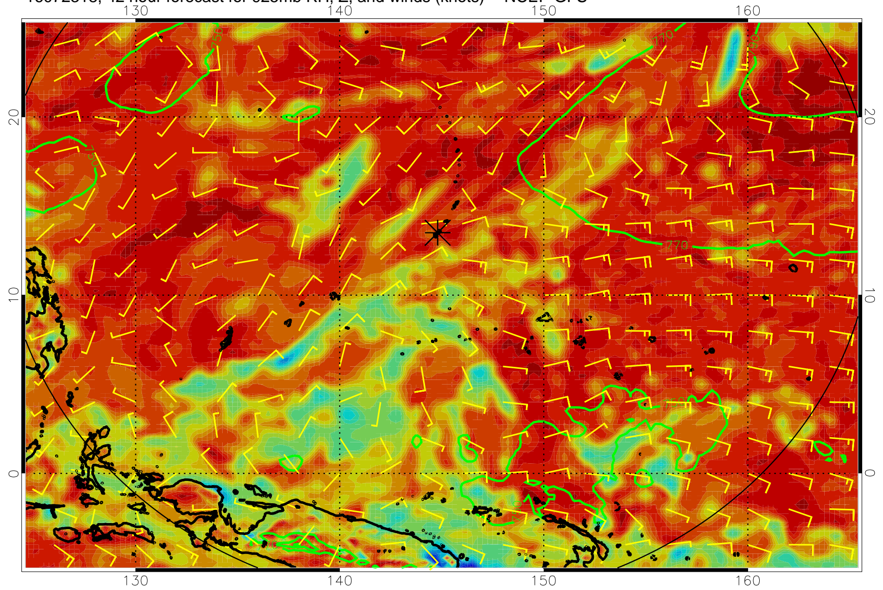
16072318, 42 hour forecast for 925mb RH, Z, and winds (knots) -- NCEP GFS
