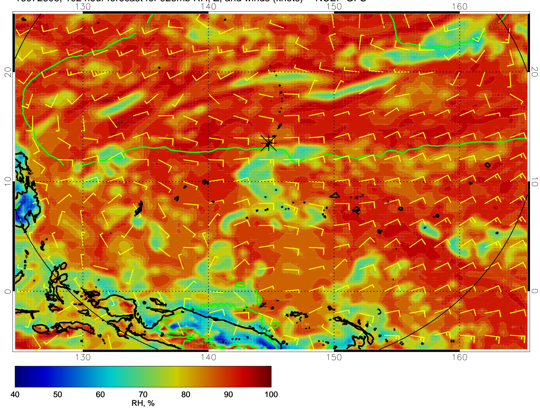
16072606, 102 hour forecast for 925mb RH, Z, and winds (knots) -- NCEP GFS
