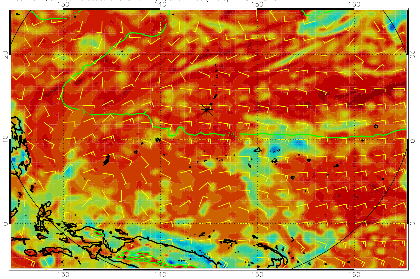
16072512, 84 hour forecast for 925mb RH, Z, and winds (knots) -- NCEP GFS
