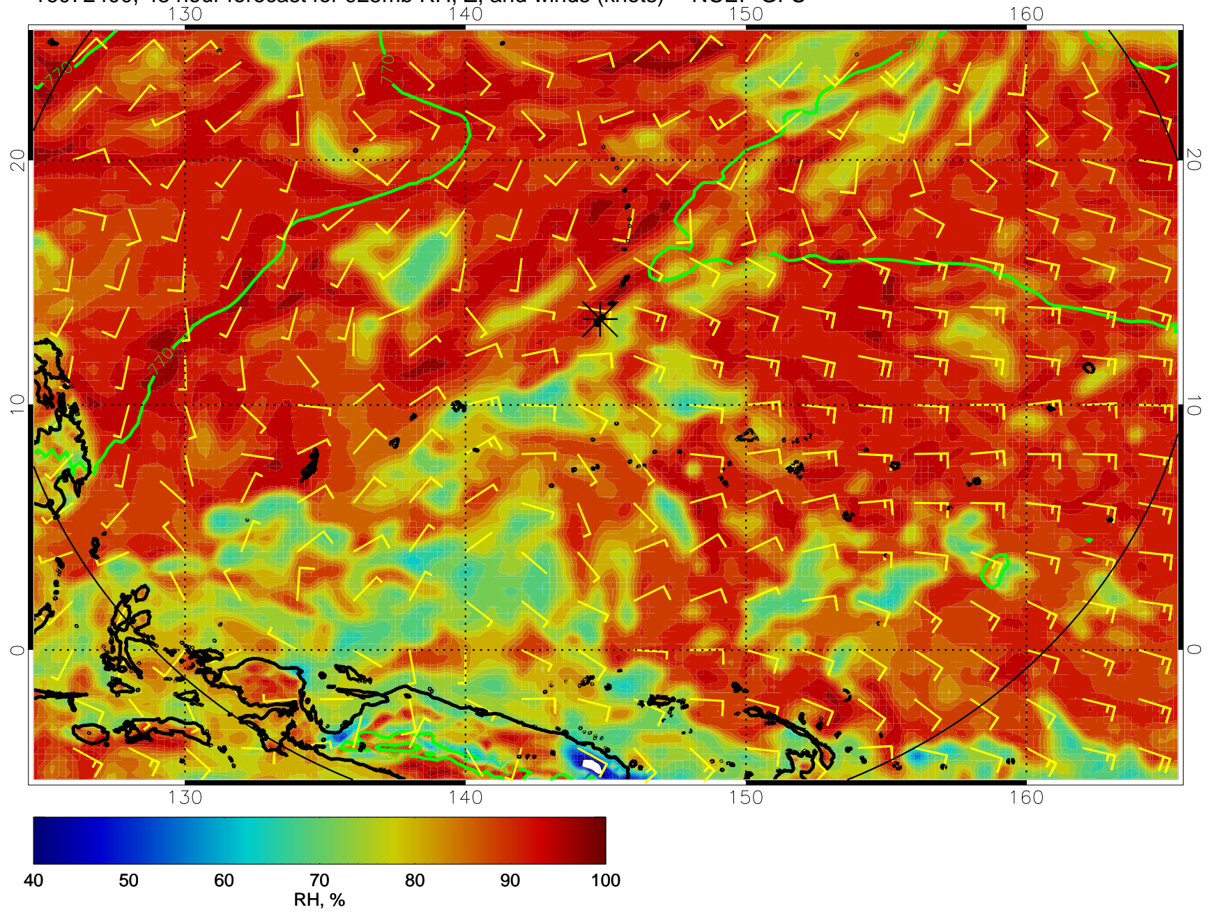
16072400, 48 hour forecast for 925mb RH, Z, and winds (knots) -- NCEP GFS
