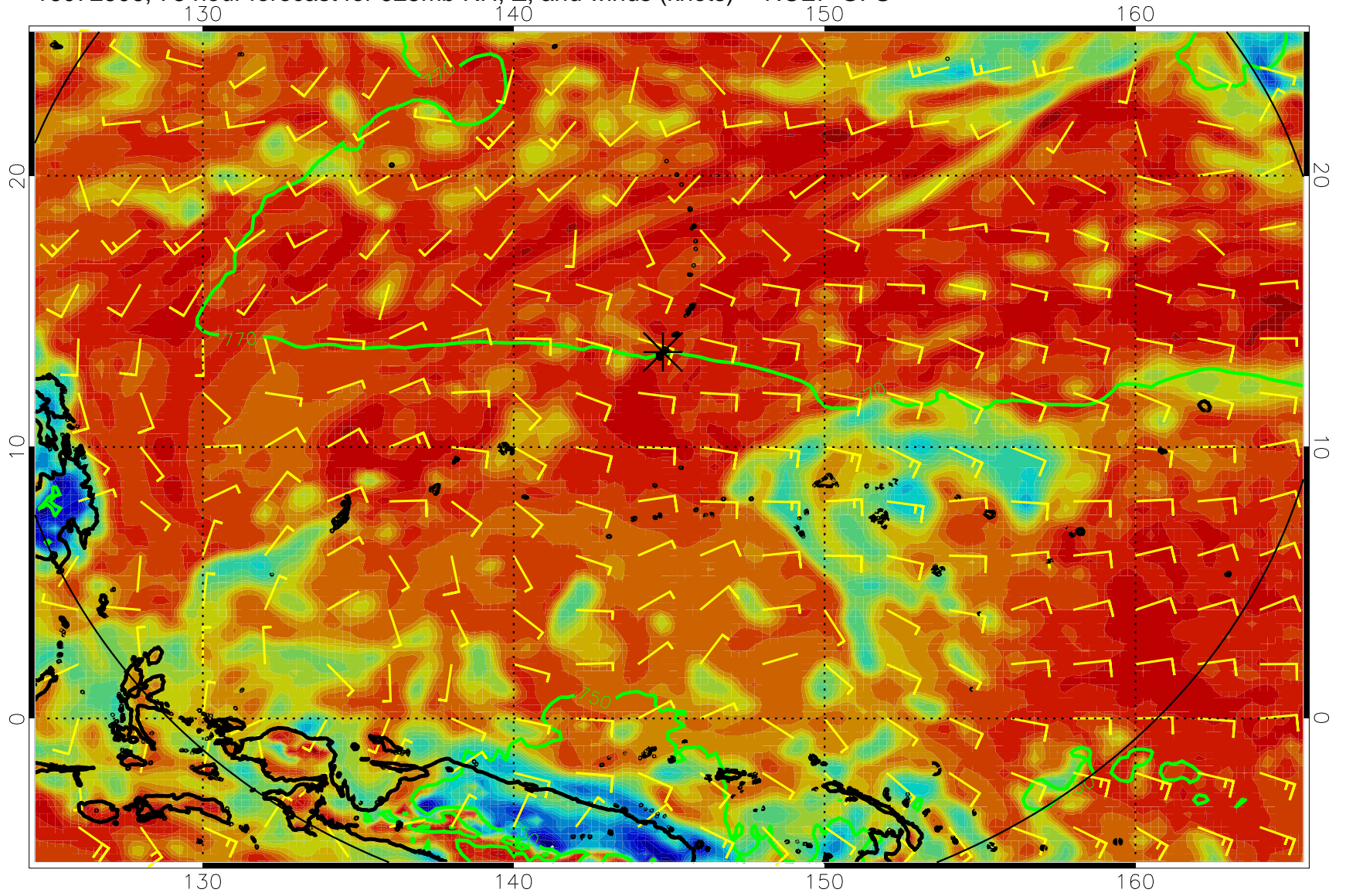
16072506, 78 hour forecast for 925mb RH, Z, and winds (knots) -- NCEP GFS
