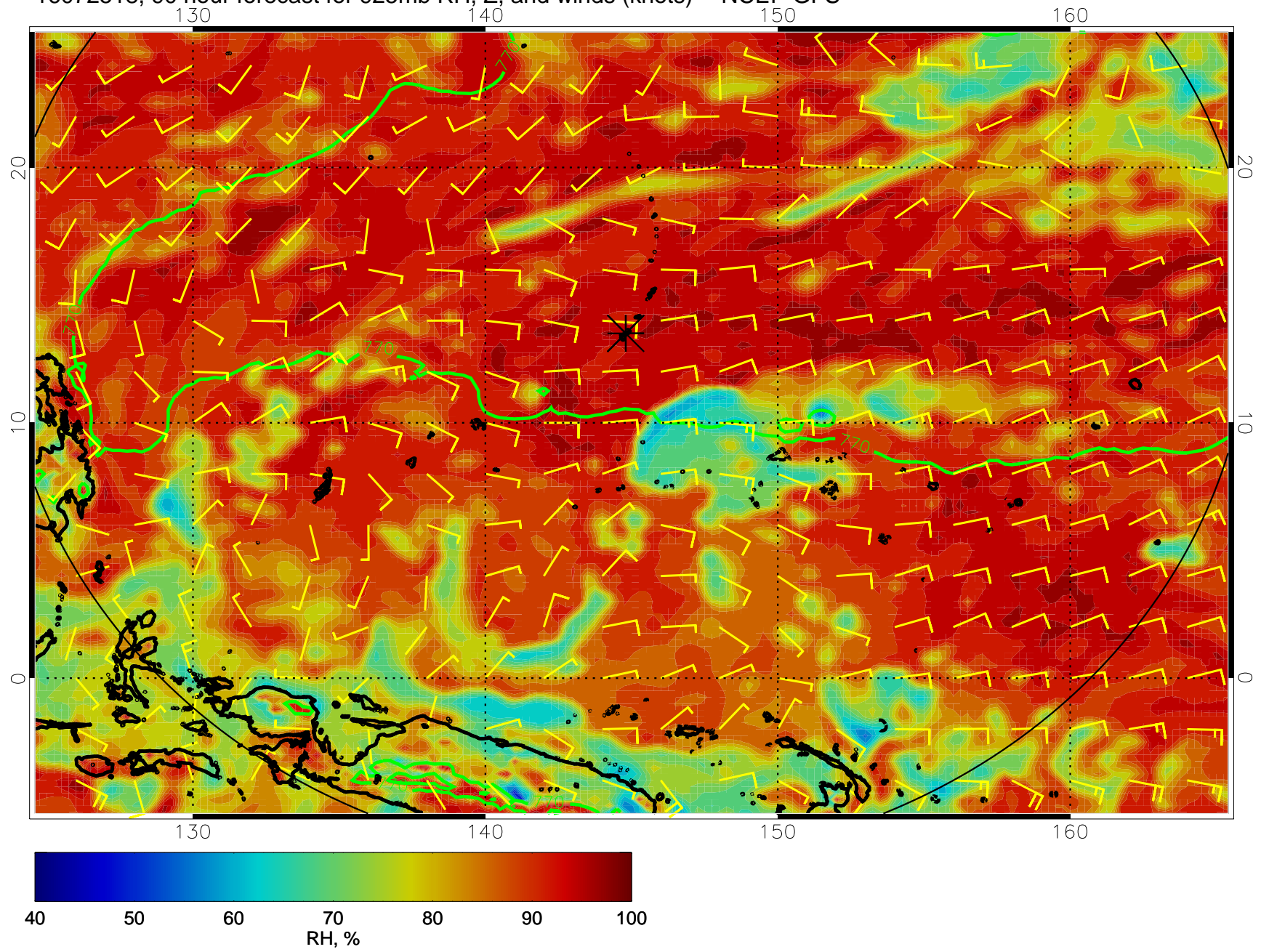
16072518, 90 hour forecast for 925mb RH, Z, and winds (knots) -- NCEP GFS
