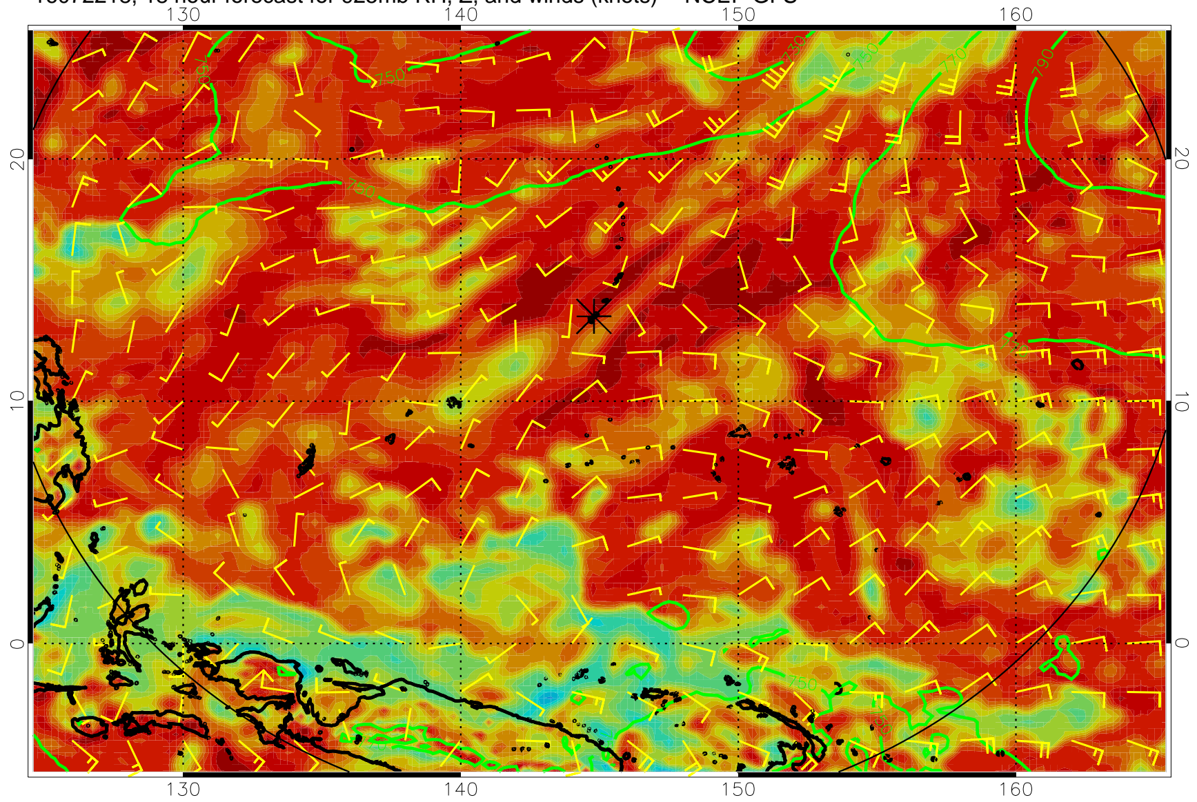
16072218, 18 hour forecast for 925mb RH, Z, and winds (knots) -- NCEP GFS
