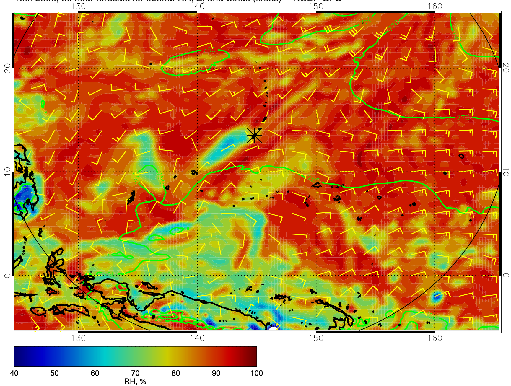
16072306, 30 hour forecast for 925mb RH, Z, and winds (knots) -- NCEP GFS
