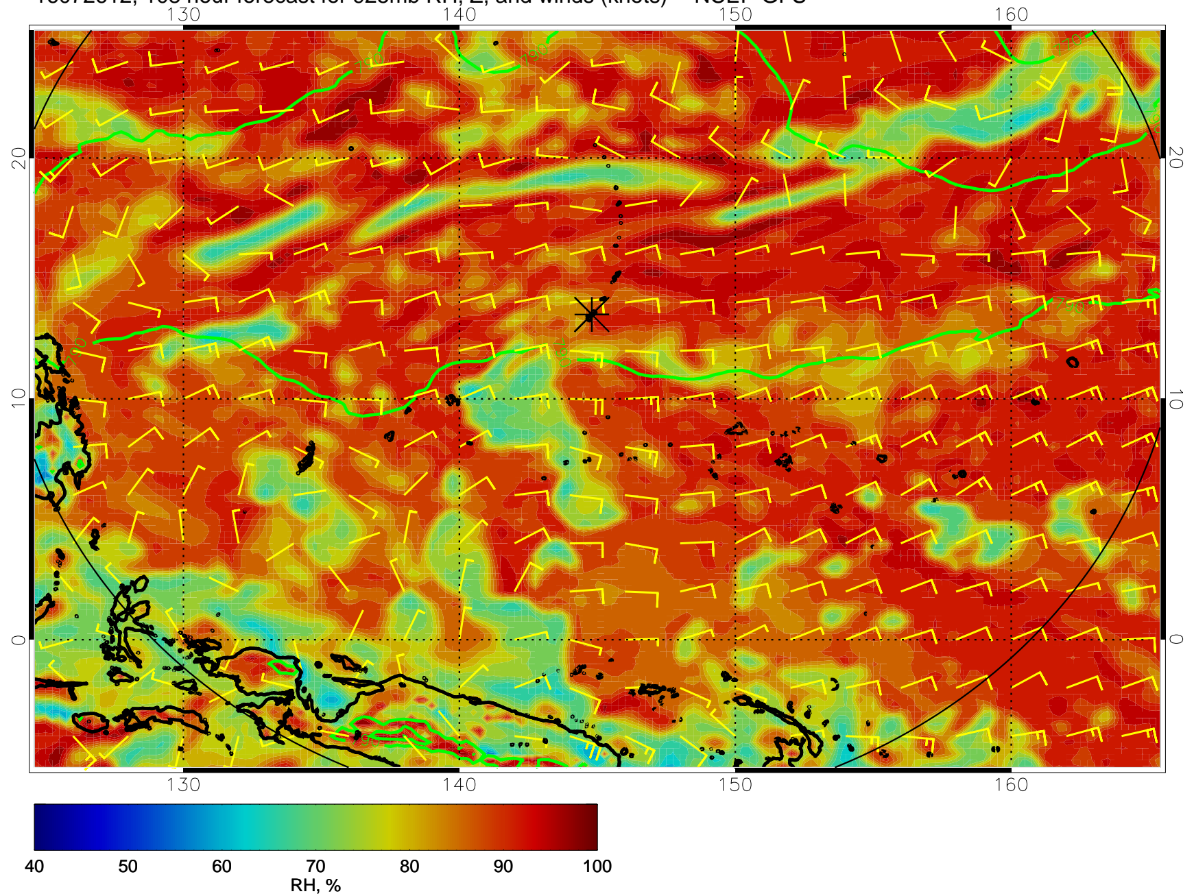
16072612, 108 hour forecast for 925mb RH, Z, and winds (knots) -- NCEP GFS
