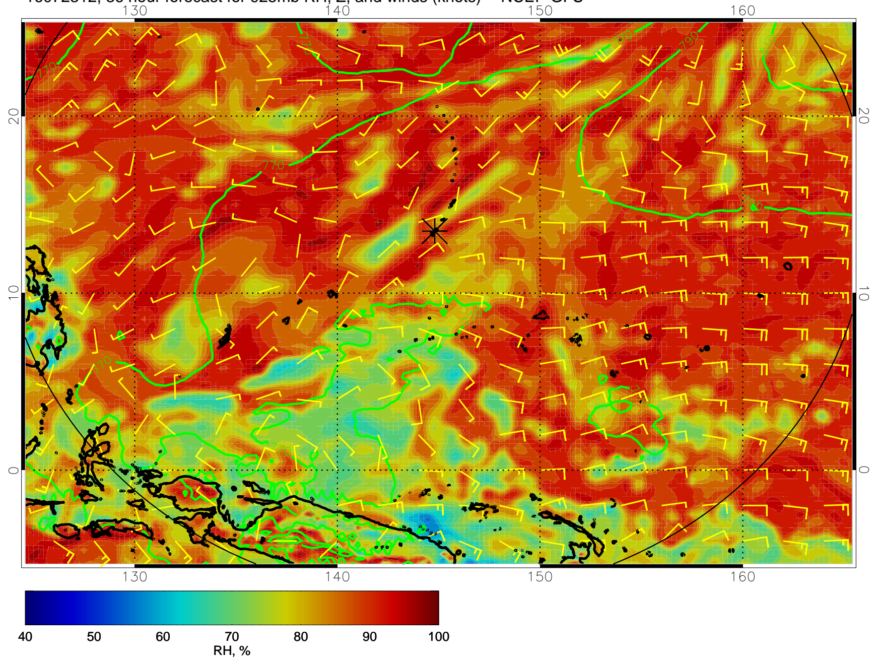
16072312, 36 hour forecast for 925mb RH, Z, and winds (knots) -- NCEP GFS
