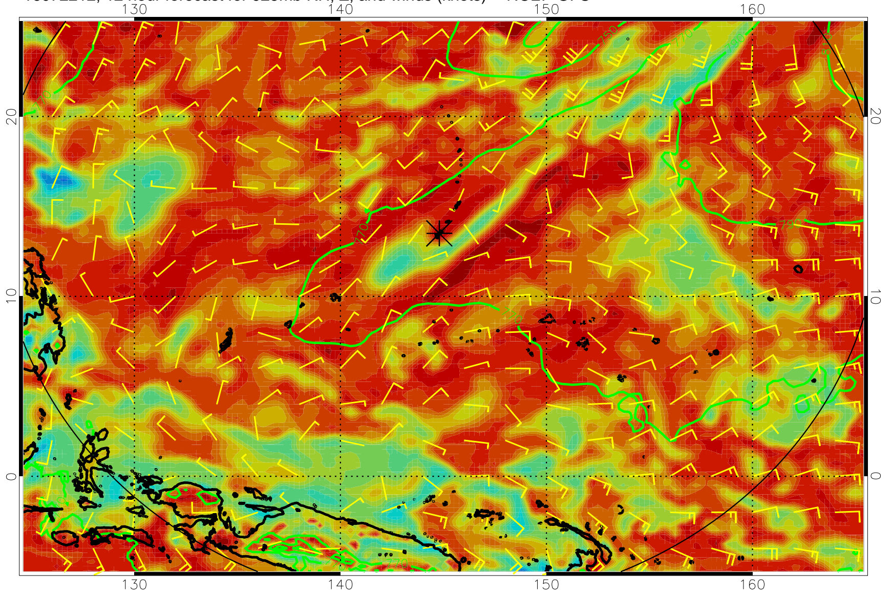
16072212, 12 hour forecast for 925mb RH, Z, and winds (knots) -- NCEP GFS
