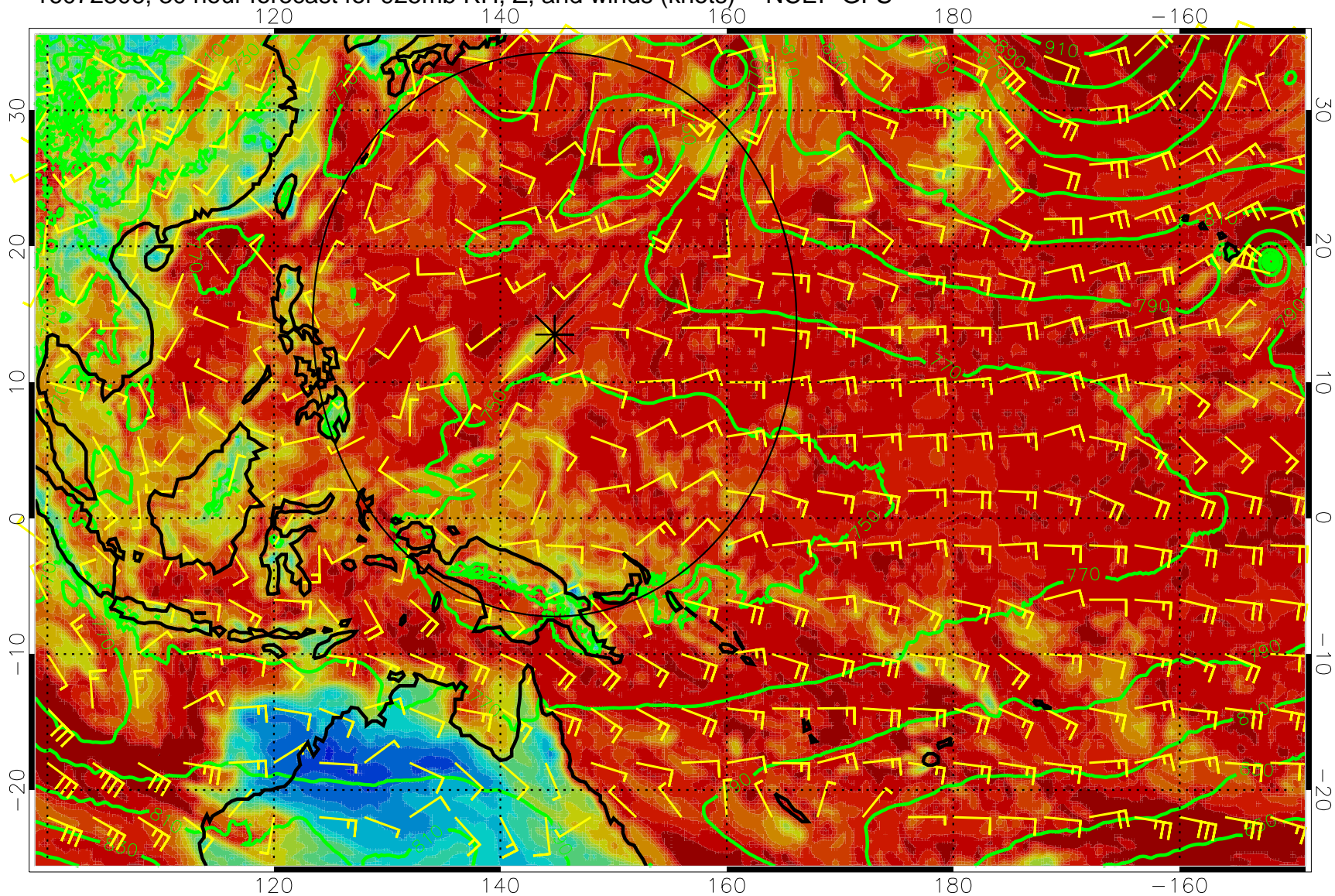
16072306, 30 hour forecast for 925mb RH, Z, and winds (knots) -- NCEP GFS
