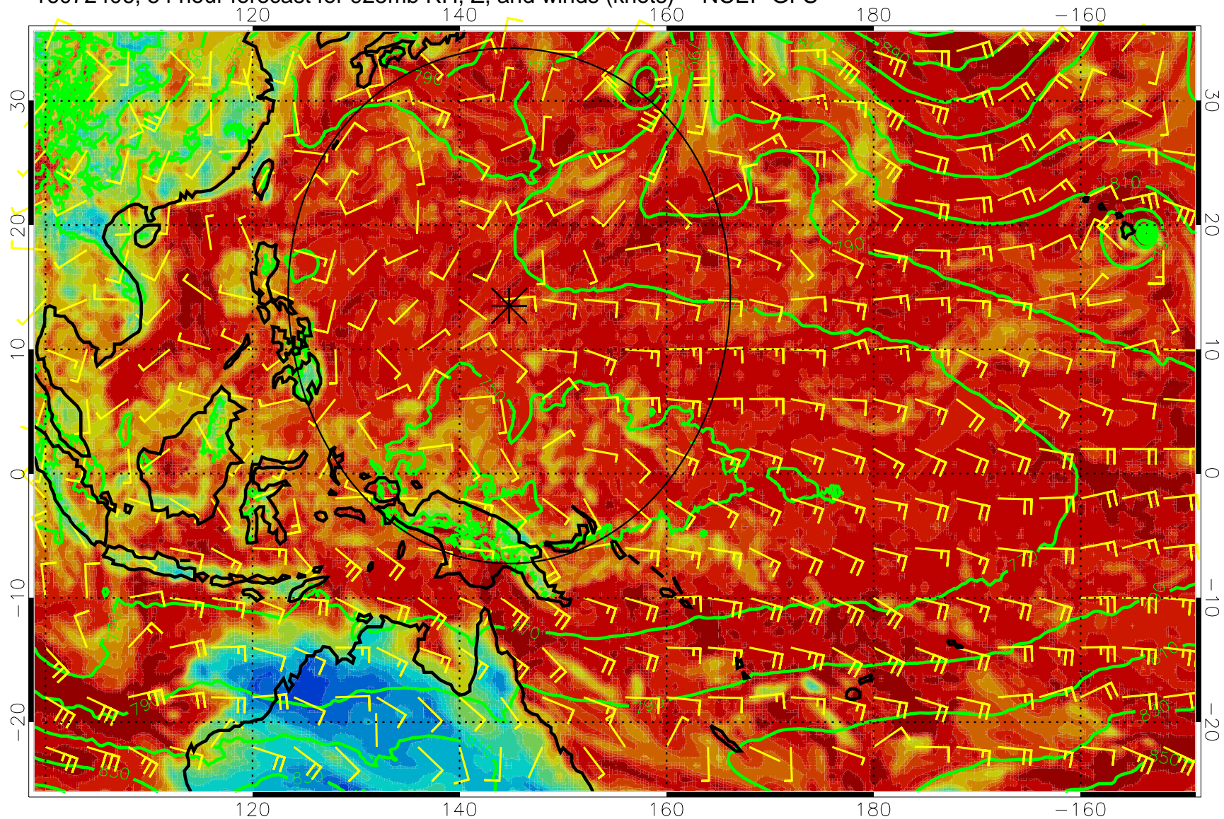
16072406, 54 hour forecast for 925mb RH, Z, and winds (knots) -- NCEP GFS
