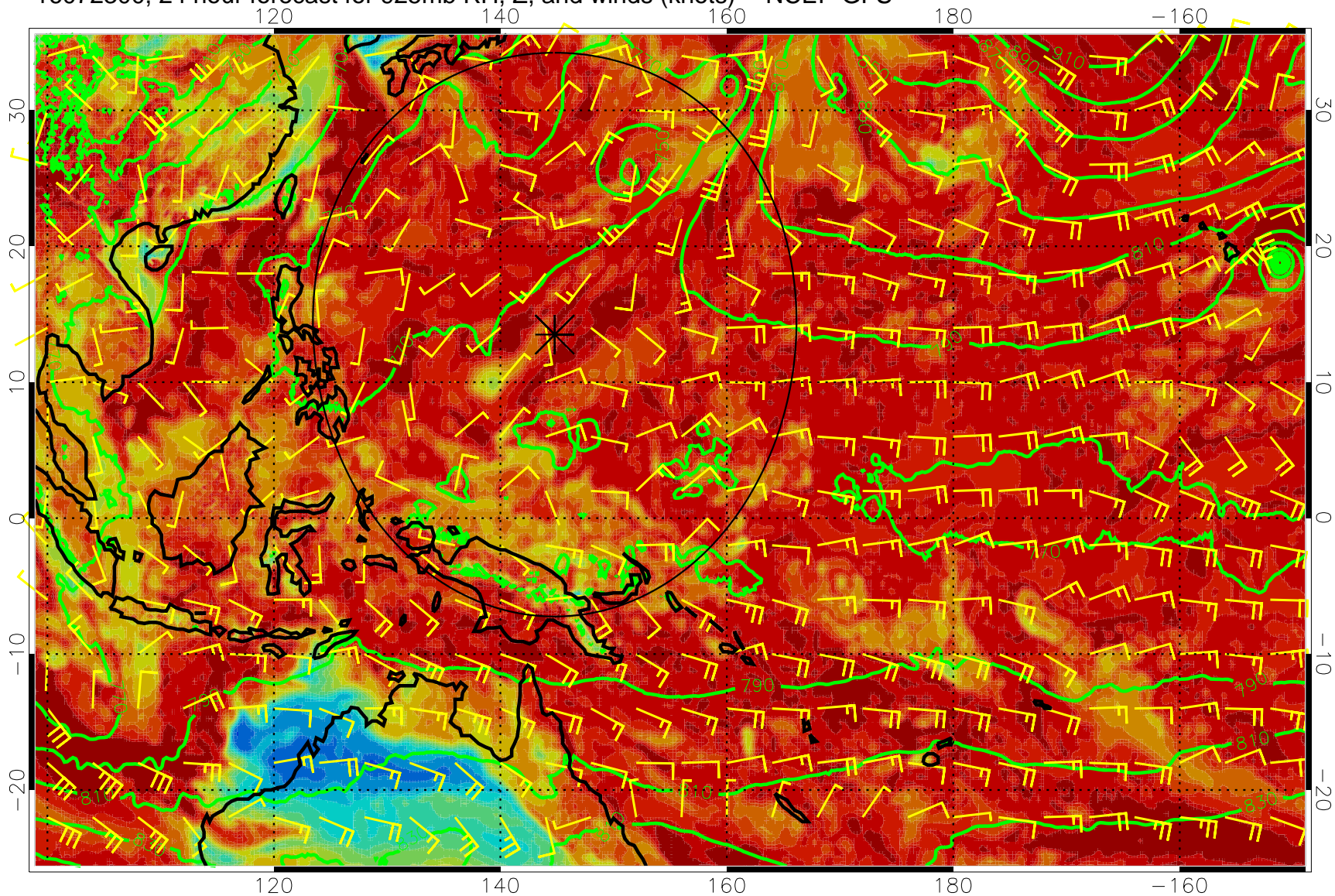
16072300, 24 hour forecast for 925mb RH, Z, and winds (knots) -- NCEP GFS
