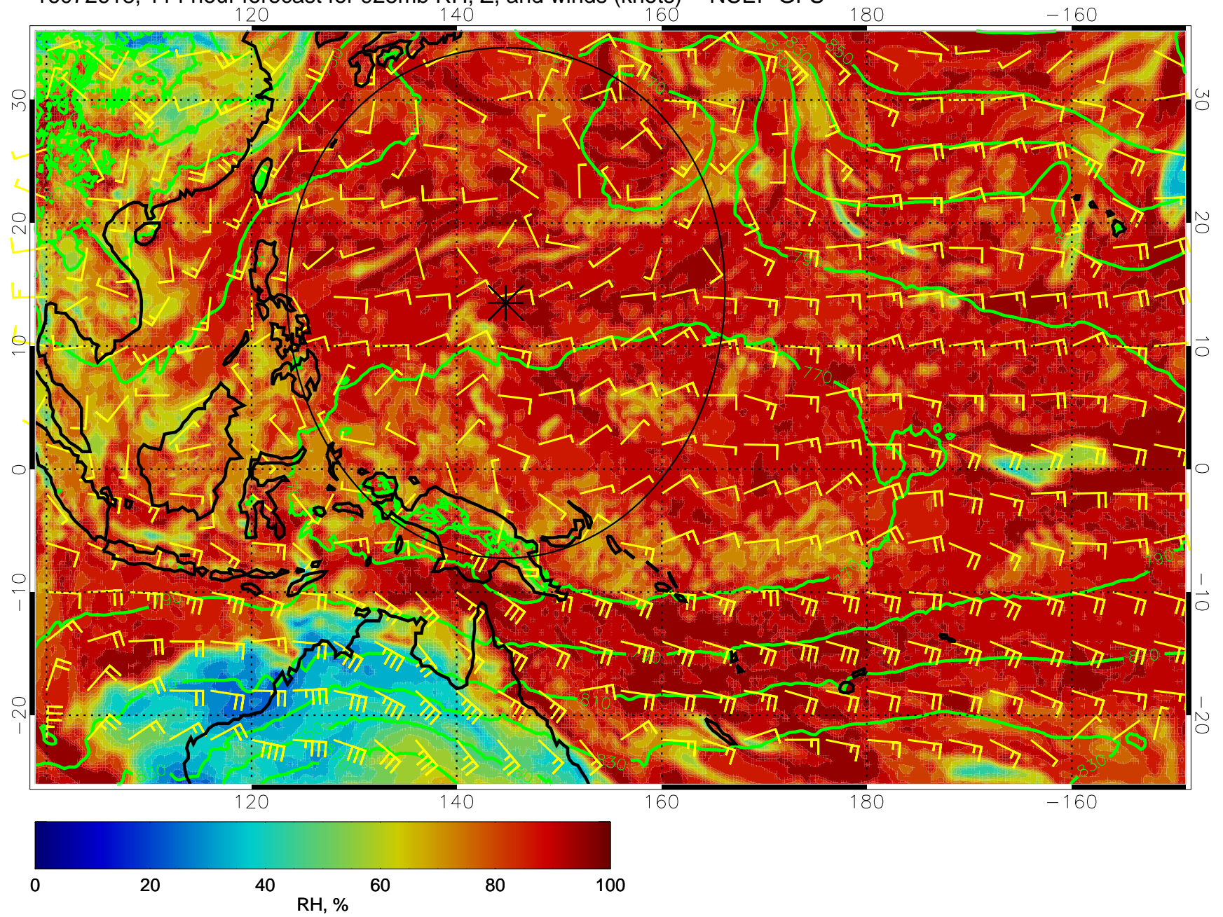
16072618, 114 hour forecast for 925mb RH, Z, and winds (knots) -- NCEP GFS
