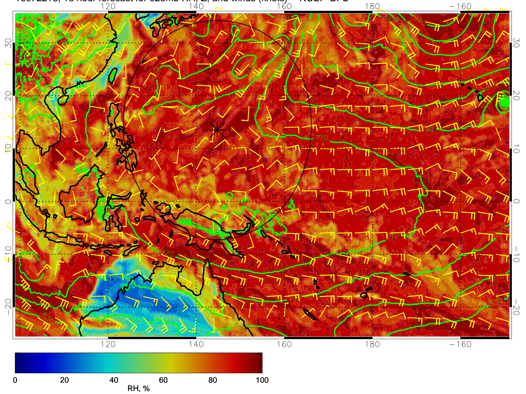
16072218, 18 hour forecast for 925mb RH, Z, and winds (knots) -- NCEP GFS
