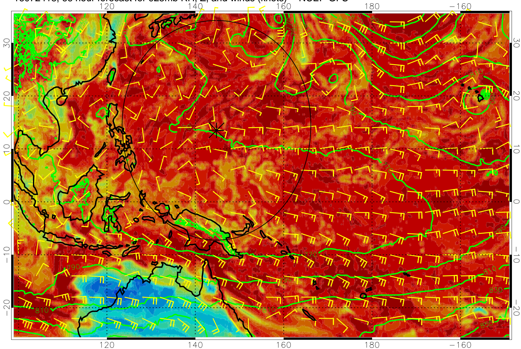
16072418, 66 hour forecast for 925mb RH, Z, and winds (knots) -- NCEP GFS
