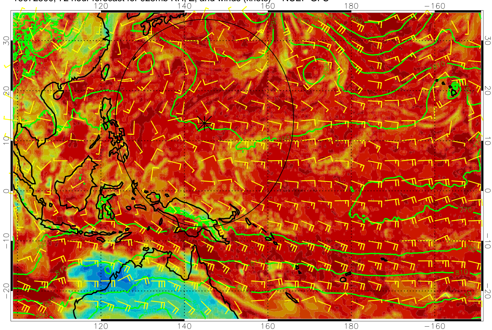
16072500, 72 hour forecast for 925mb RH, Z, and winds (knots) -- NCEP GFS
