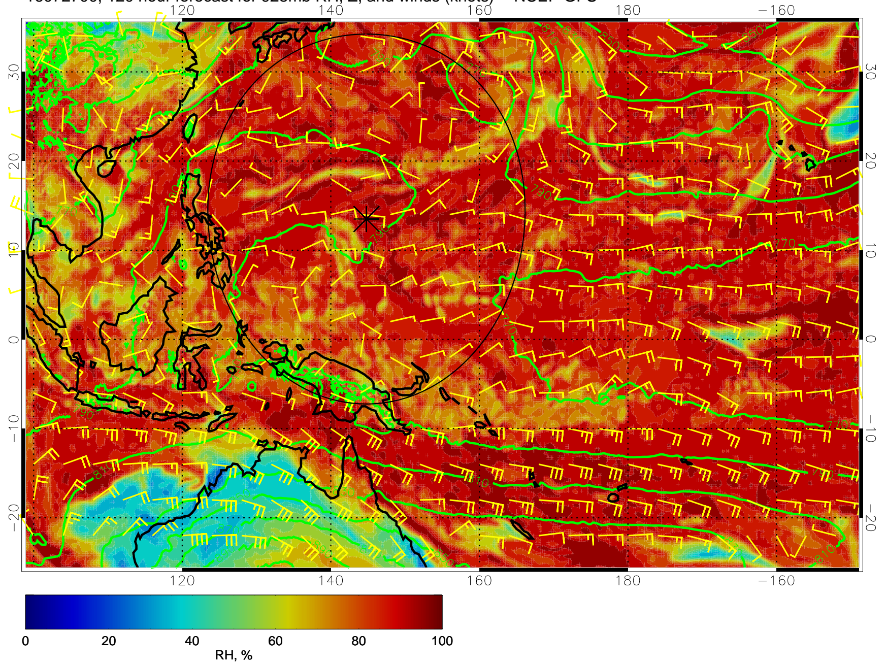
16072700, 120 hour forecast for 925mb RH, Z, and winds (knots) -- NCEP GFS
