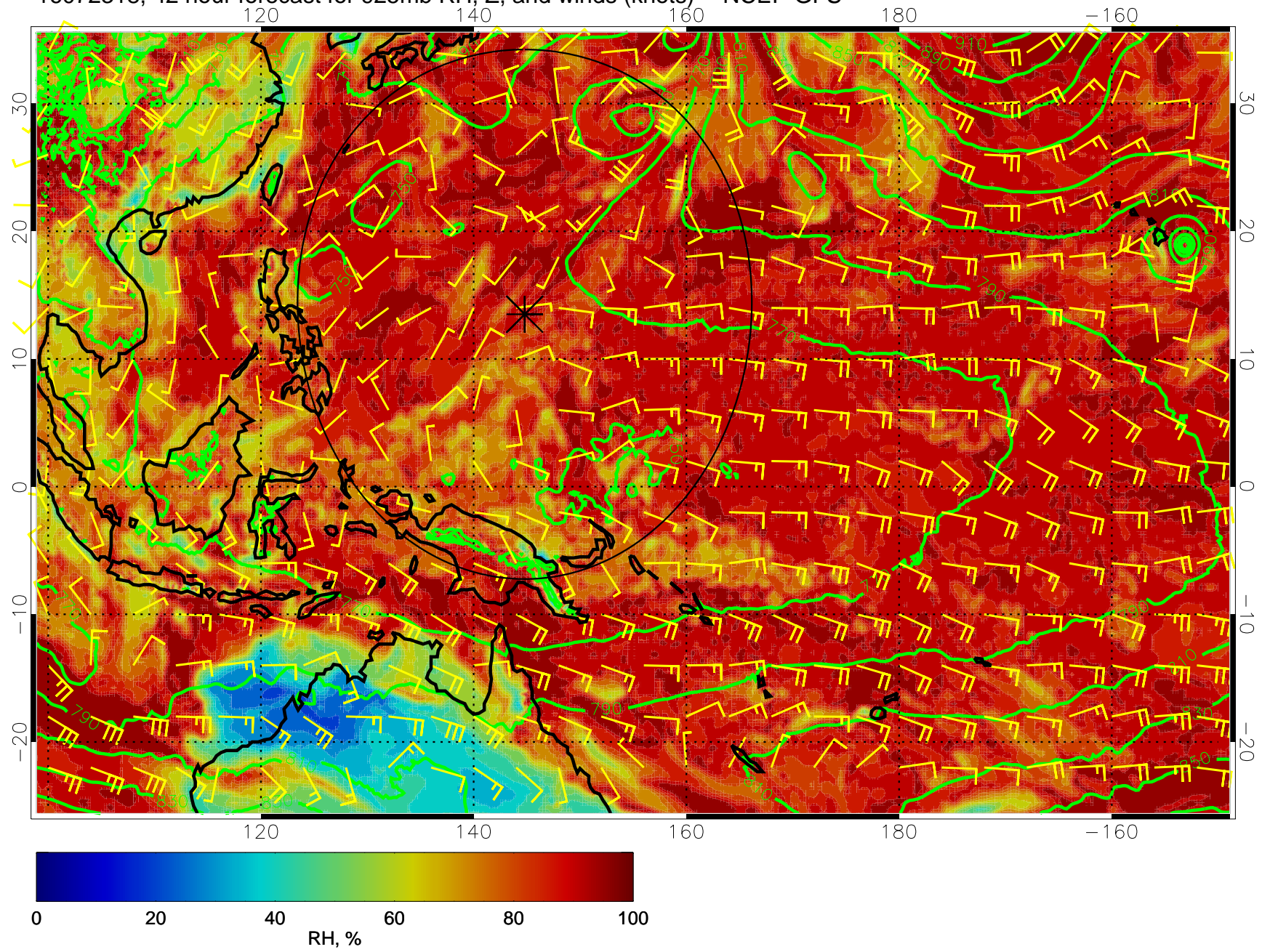
16072318, 42 hour forecast for 925mb RH, Z, and winds (knots) -- NCEP GFS
