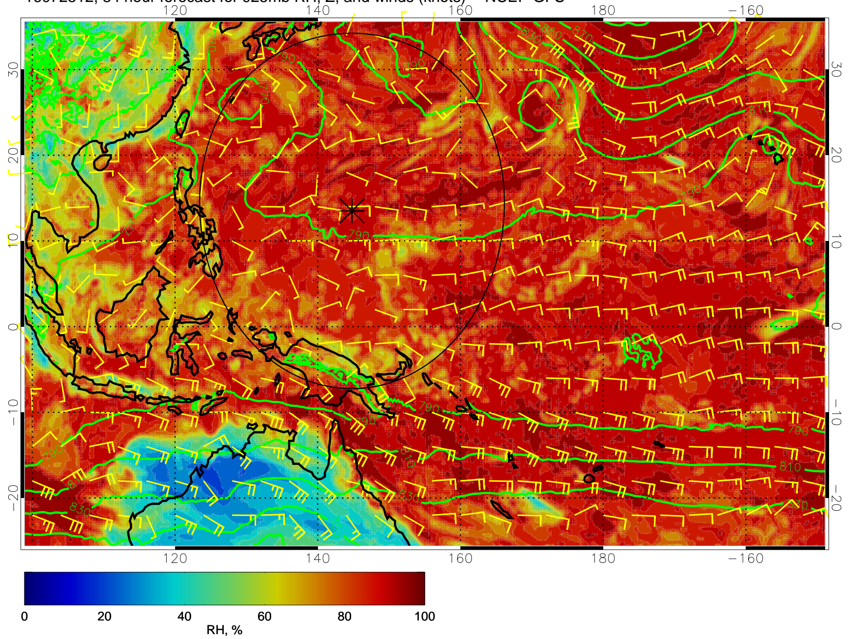
16072512, 84 hour forecast for 925mb RH, Z, and winds (knots) -- NCEP GFS
