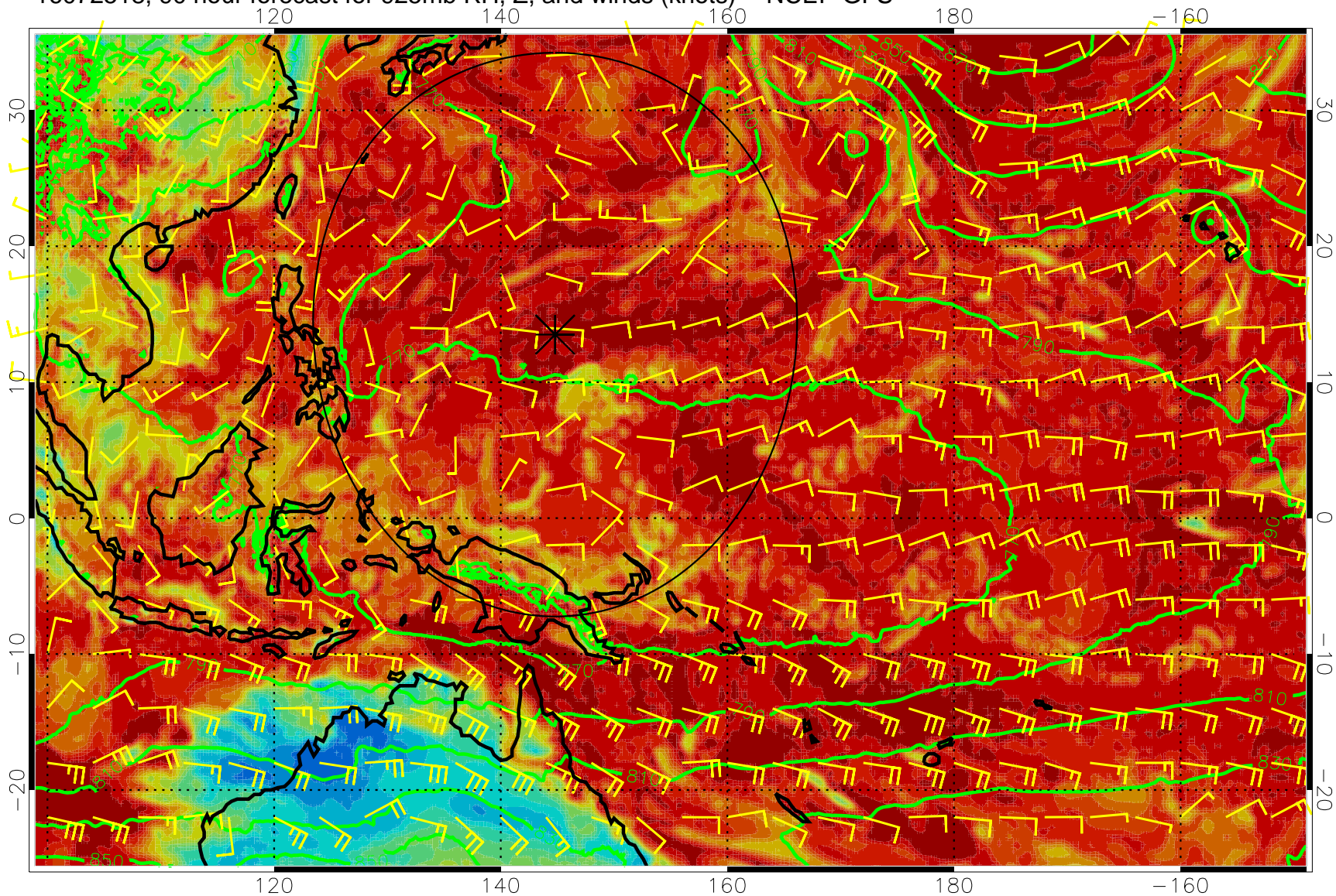
16072518, 90 hour forecast for 925mb RH, Z, and winds (knots) -- NCEP GFS
