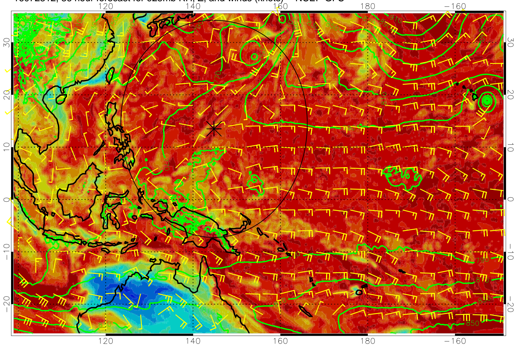
16072312, 36 hour forecast for 925mb RH, Z, and winds (knots) -- NCEP GFS
