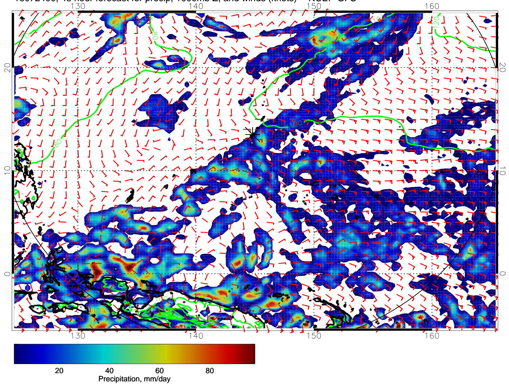
16072400, 48 hour forecast for precip, 1000mb Z, and winds (knots) -- NCEP GFS
