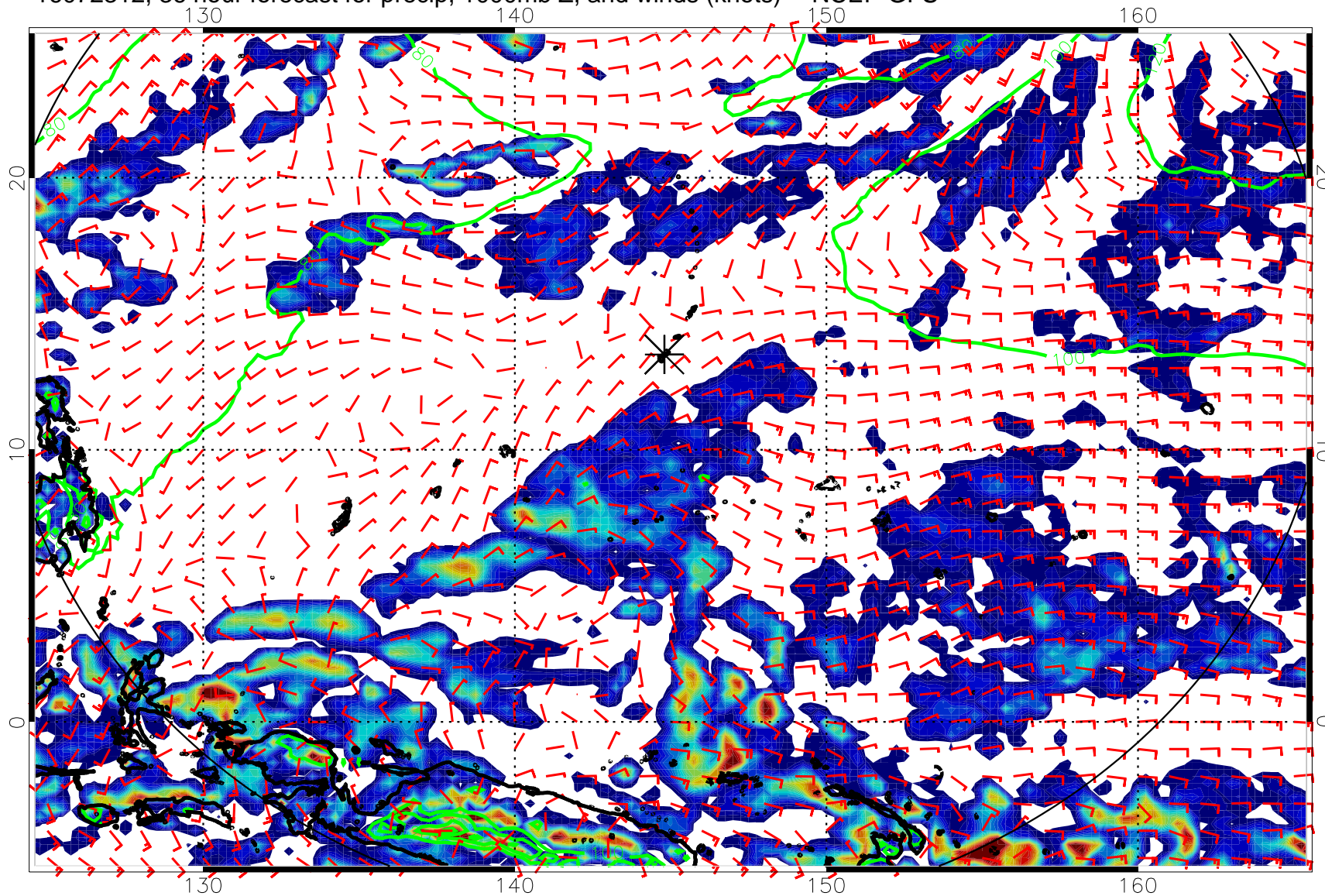
16072312, 36 hour forecast for precip, 1000mb Z, and winds (knots) -- NCEP GFS
