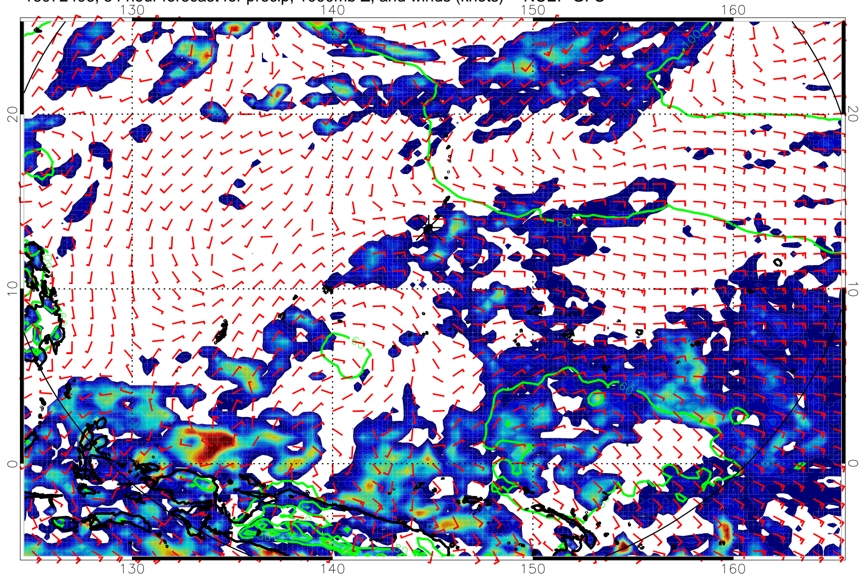
16072406, 54 hour forecast for precip, 1000mb Z, and winds (knots) -- NCEP GFS
