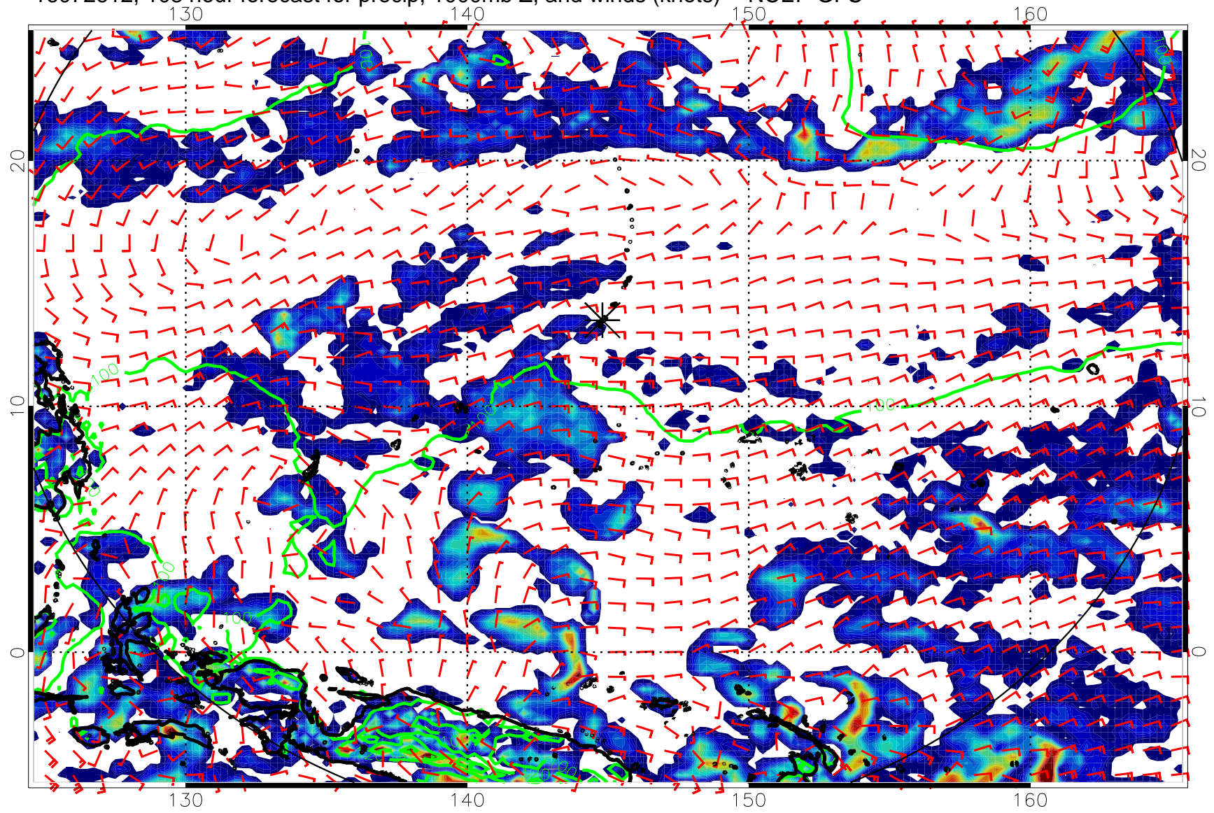
16072612, 108 hour forecast for precip, 1000mb Z, and winds (knots) -- NCEP GFS
