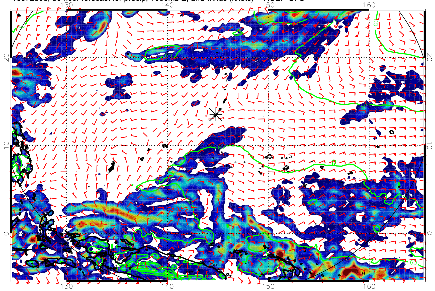
16072306, 30 hour forecast for precip, 1000mb Z, and winds (knots) -- NCEP GFS
