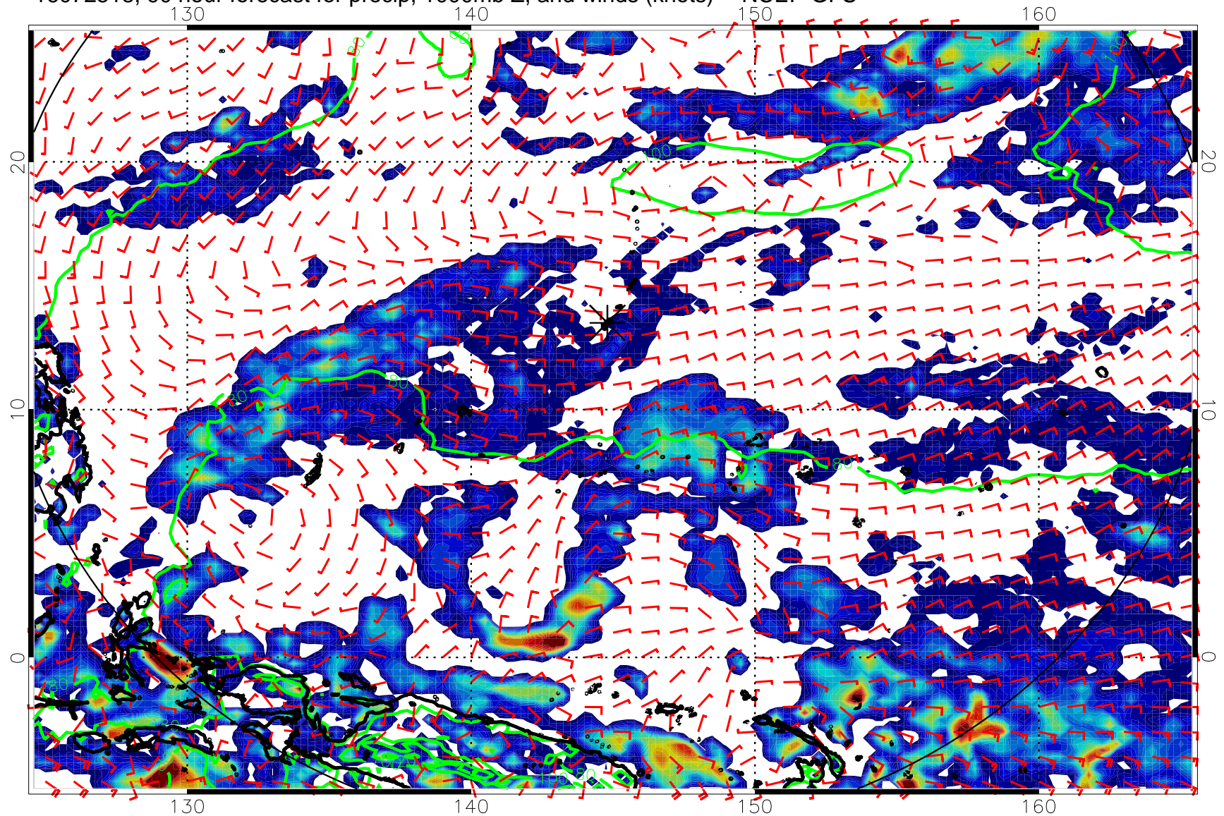
16072518, 90 hour forecast for precip, 1000mb Z, and winds (knots) -- NCEP GFS
