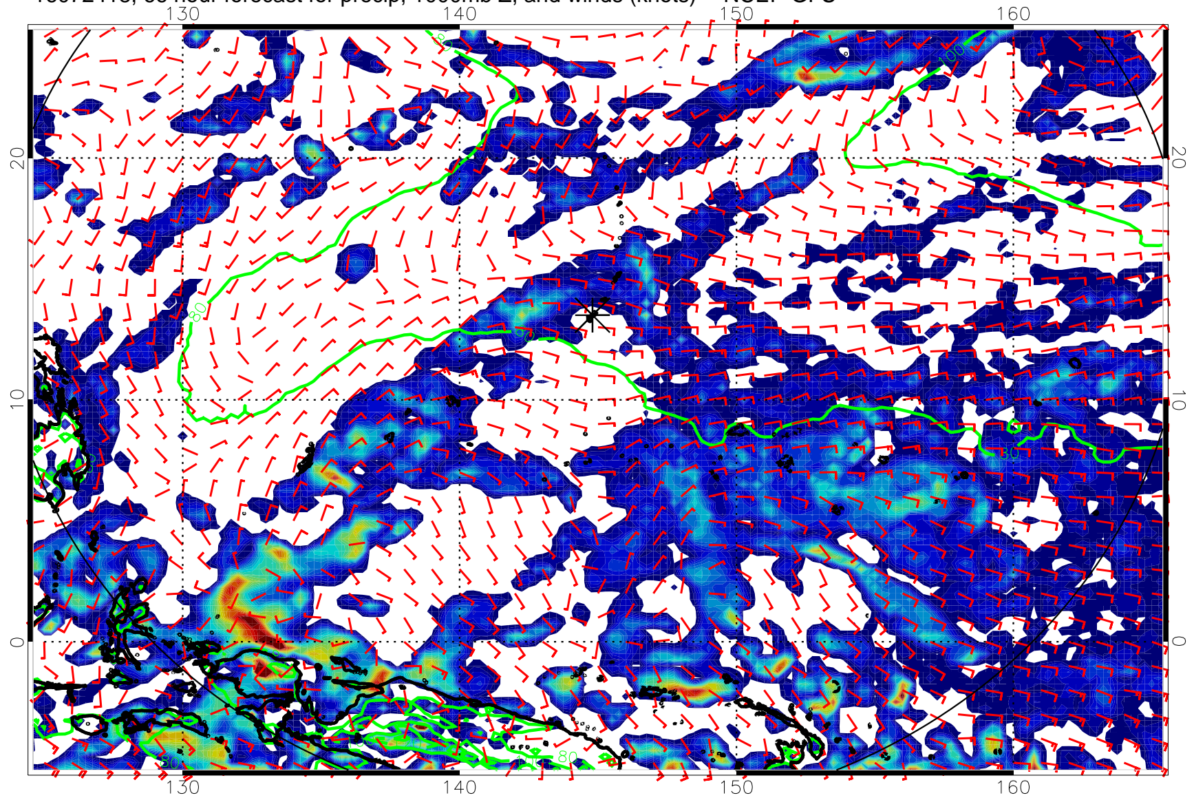
16072418, 66 hour forecast for precip, 1000mb Z, and winds (knots) -- NCEP GFS
