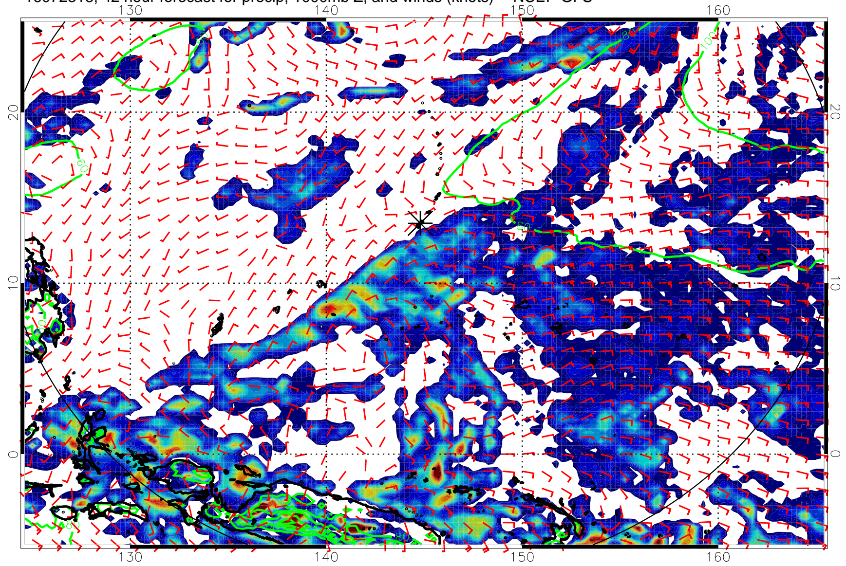
16072318, 42 hour forecast for precip, 1000mb Z, and winds (knots) -- NCEP GFS
