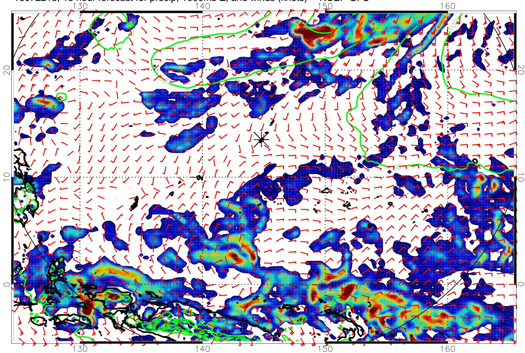
16072218, 18 hour forecast for precip, 1000mb Z, and winds (knots) -- NCEP GFS
