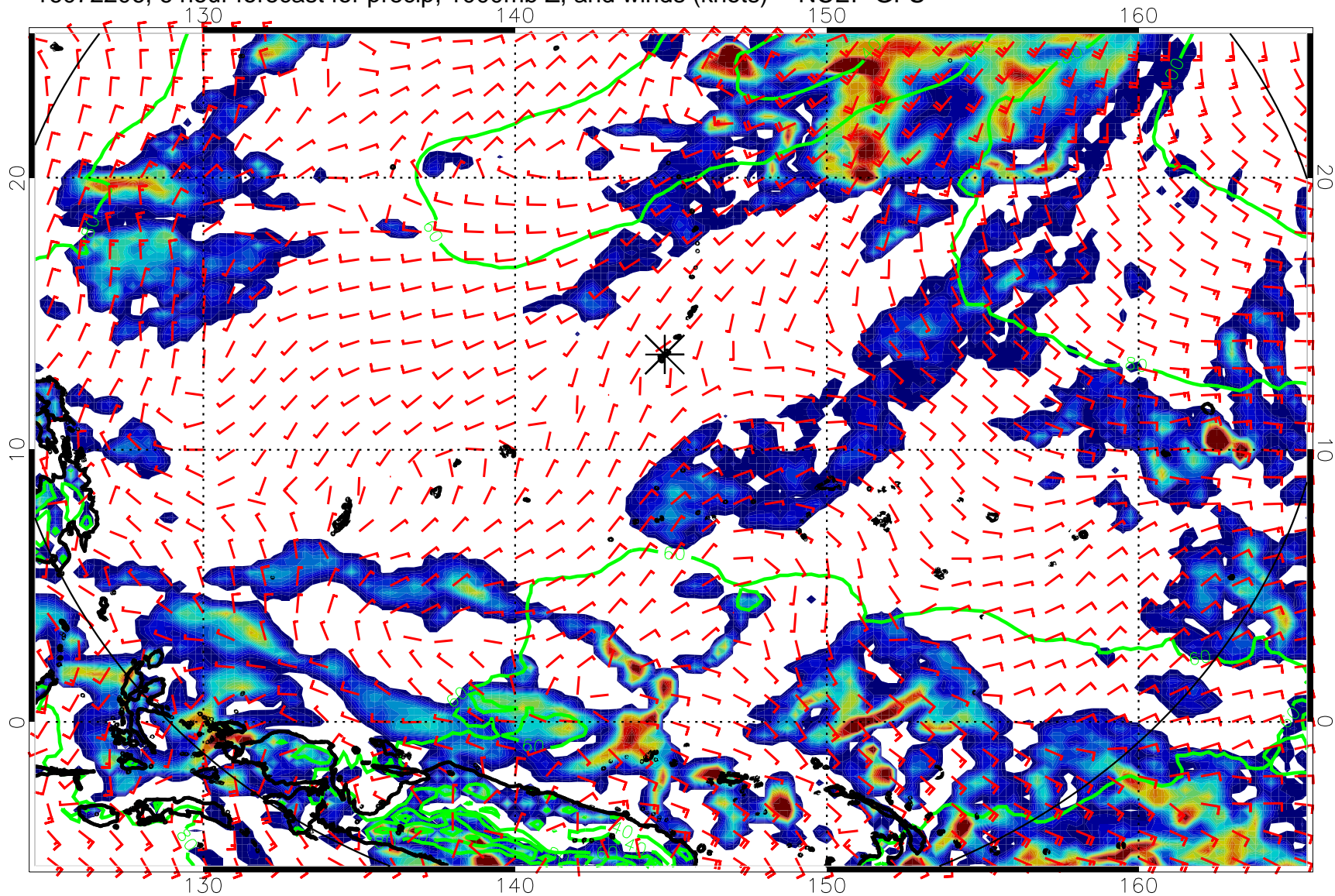
16072206, 6 hour forecast for precip, 1000mb Z, and winds (knots) -- NCEP GFS
