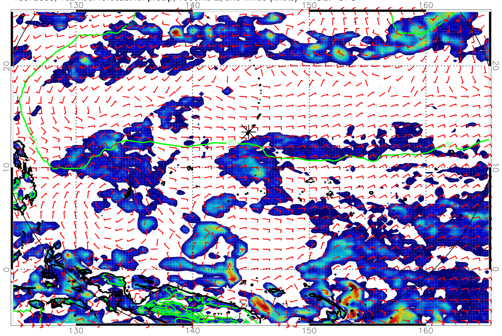
16072606, 102 hour forecast for precip, 1000mb Z, and winds (knots) -- NCEP GFS
