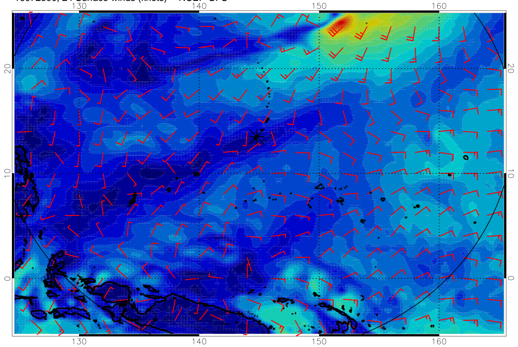
16072300, 24 Surface winds (knots) -- NCEP GFS
