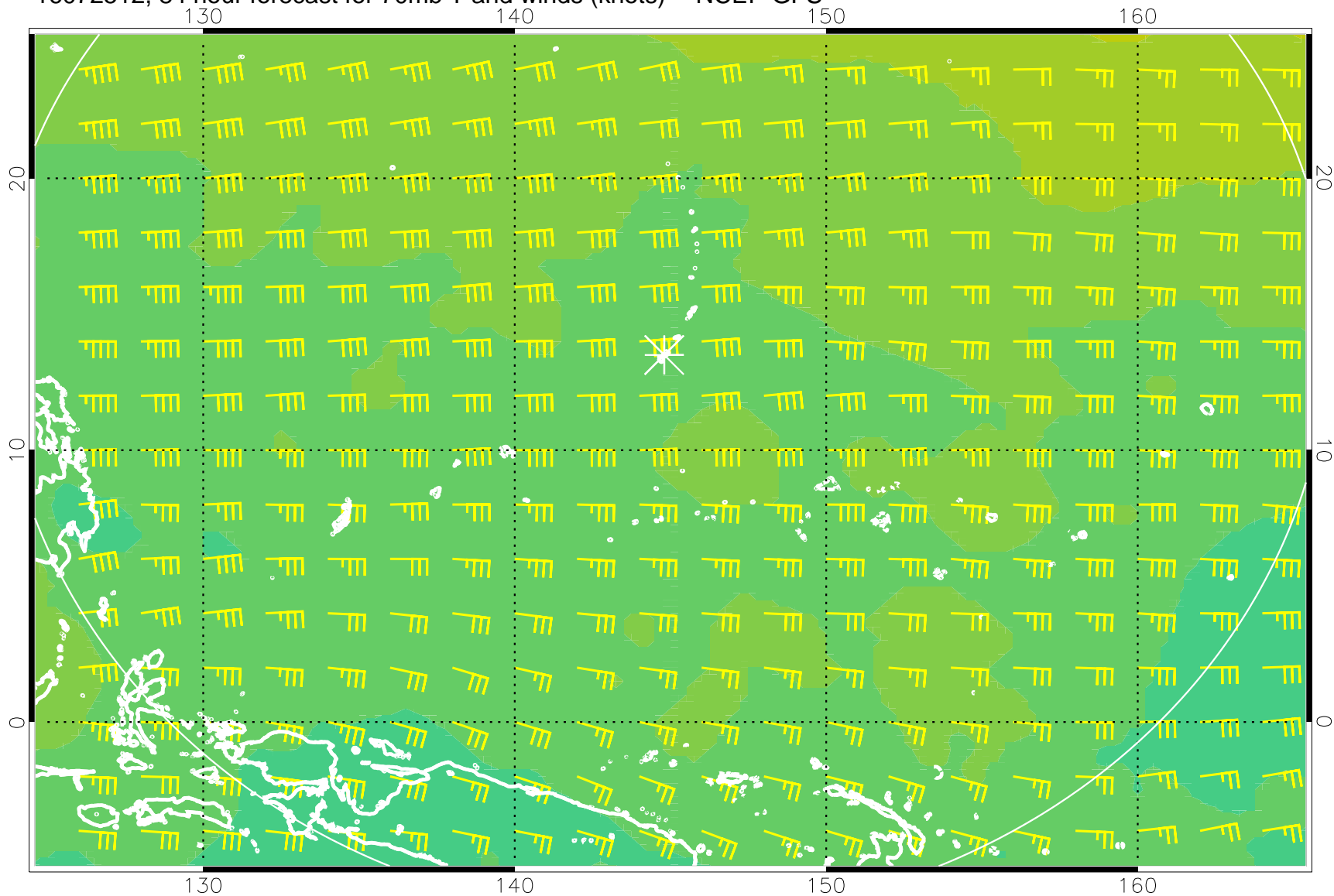
16072512, 84 hour forecast for 70mb T and winds (knots) -- NCEP GFS
