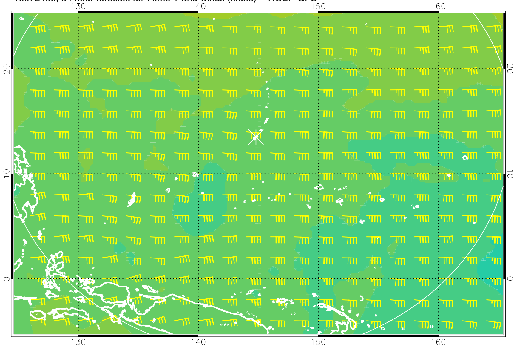
16072406, 54 hour forecast for 70mb T and winds (knots) -- NCEP GFS
