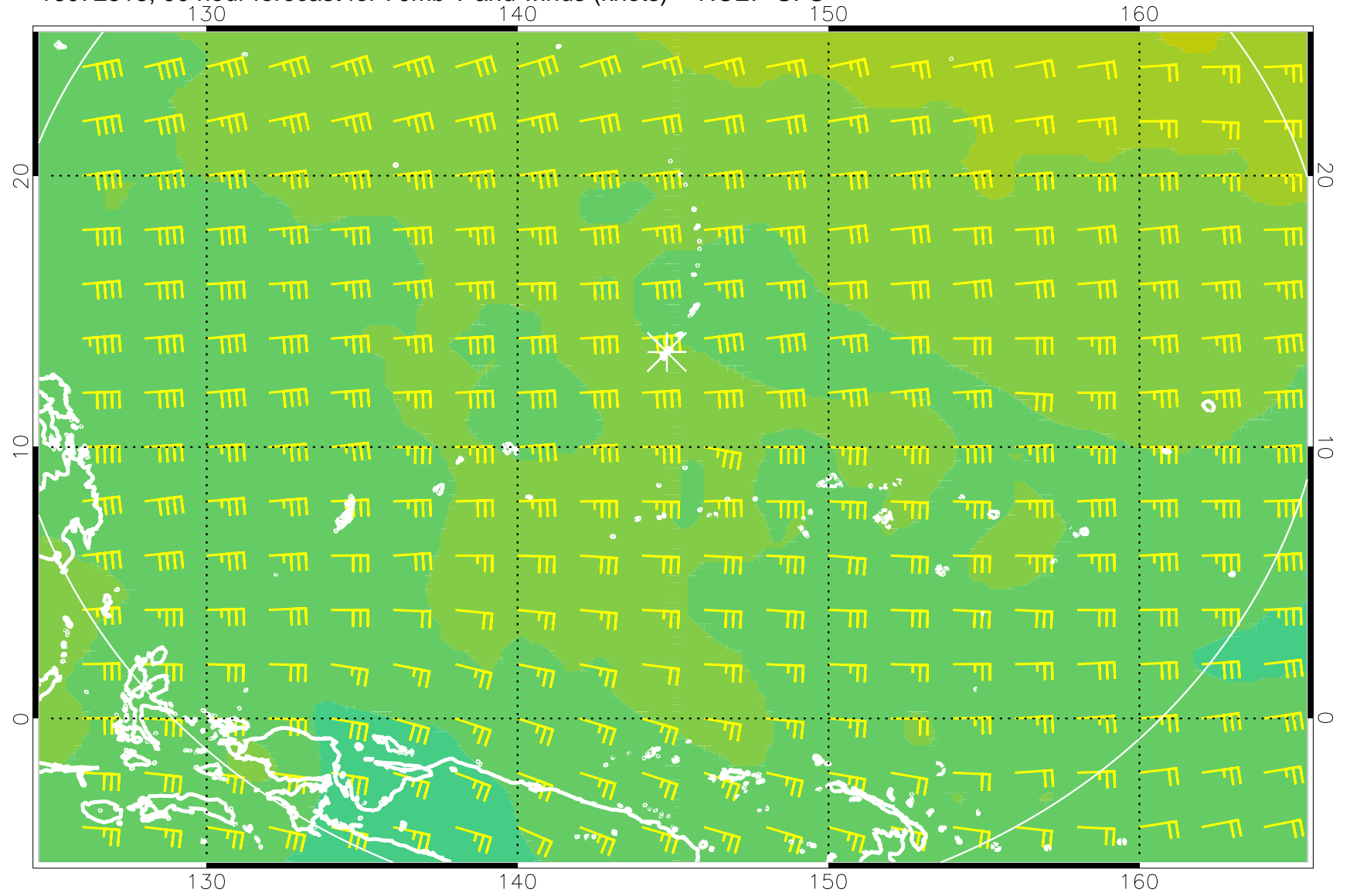
16072518, 90 hour forecast for 70mb T and winds (knots) -- NCEP GFS
