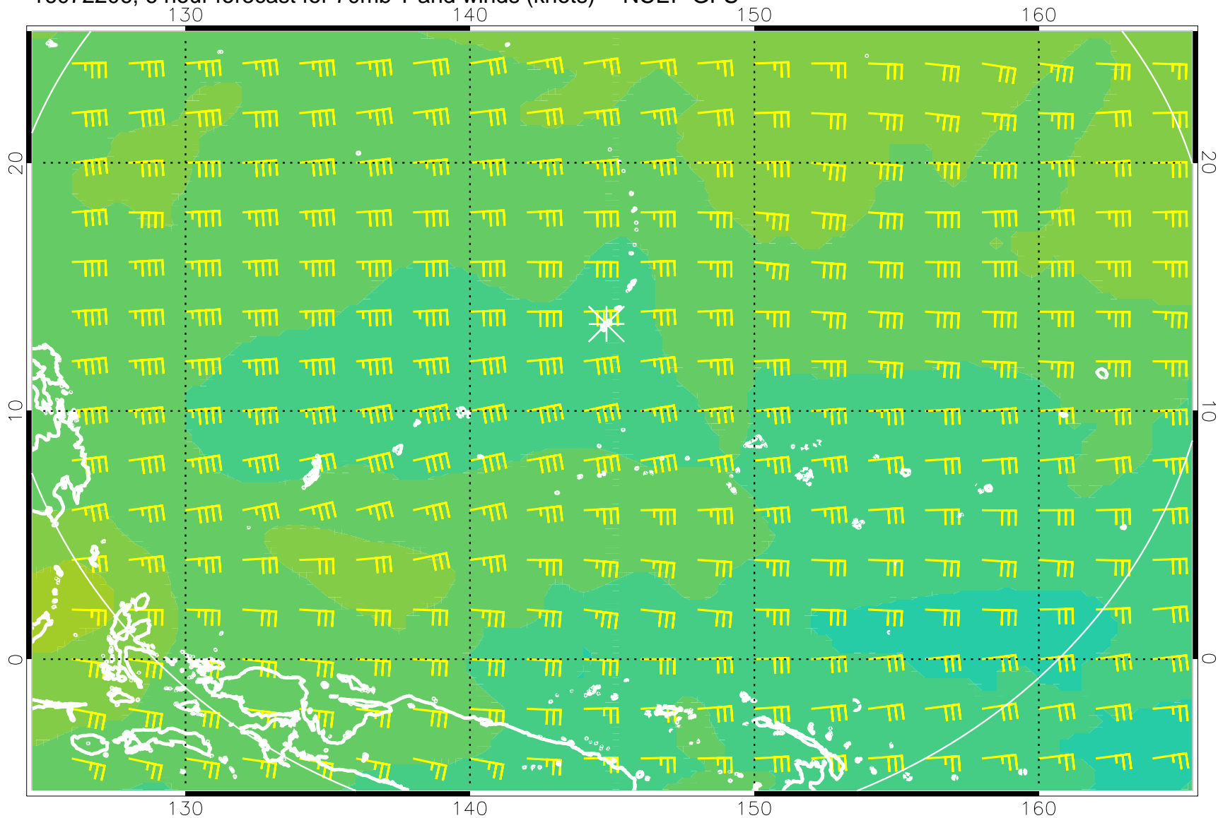
16072206, 6 hour forecast for 70mb T and winds (knots) -- NCEP GFS
