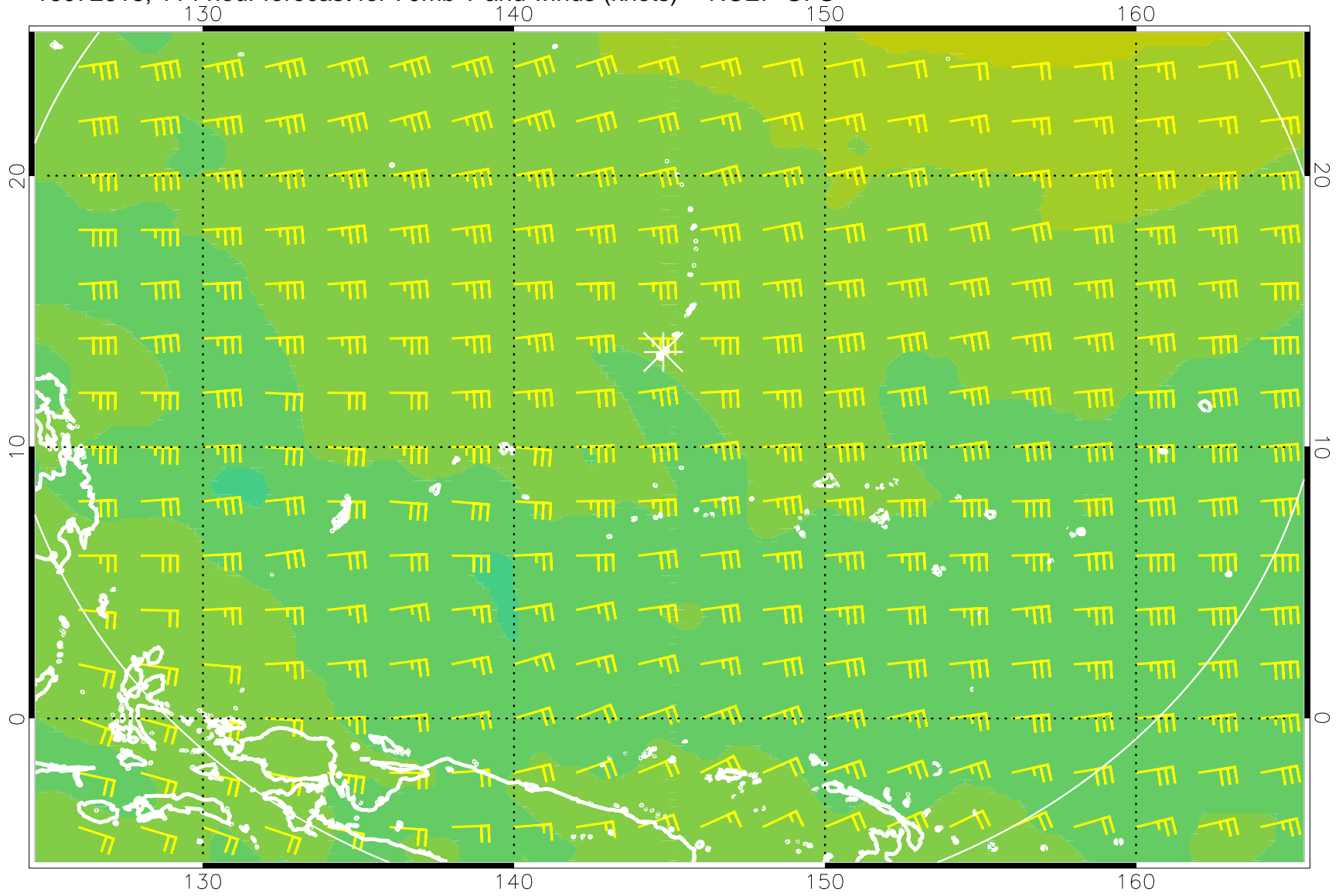
16072618, 114 hour forecast for 70mb T and winds (knots) -- NCEP GFS
