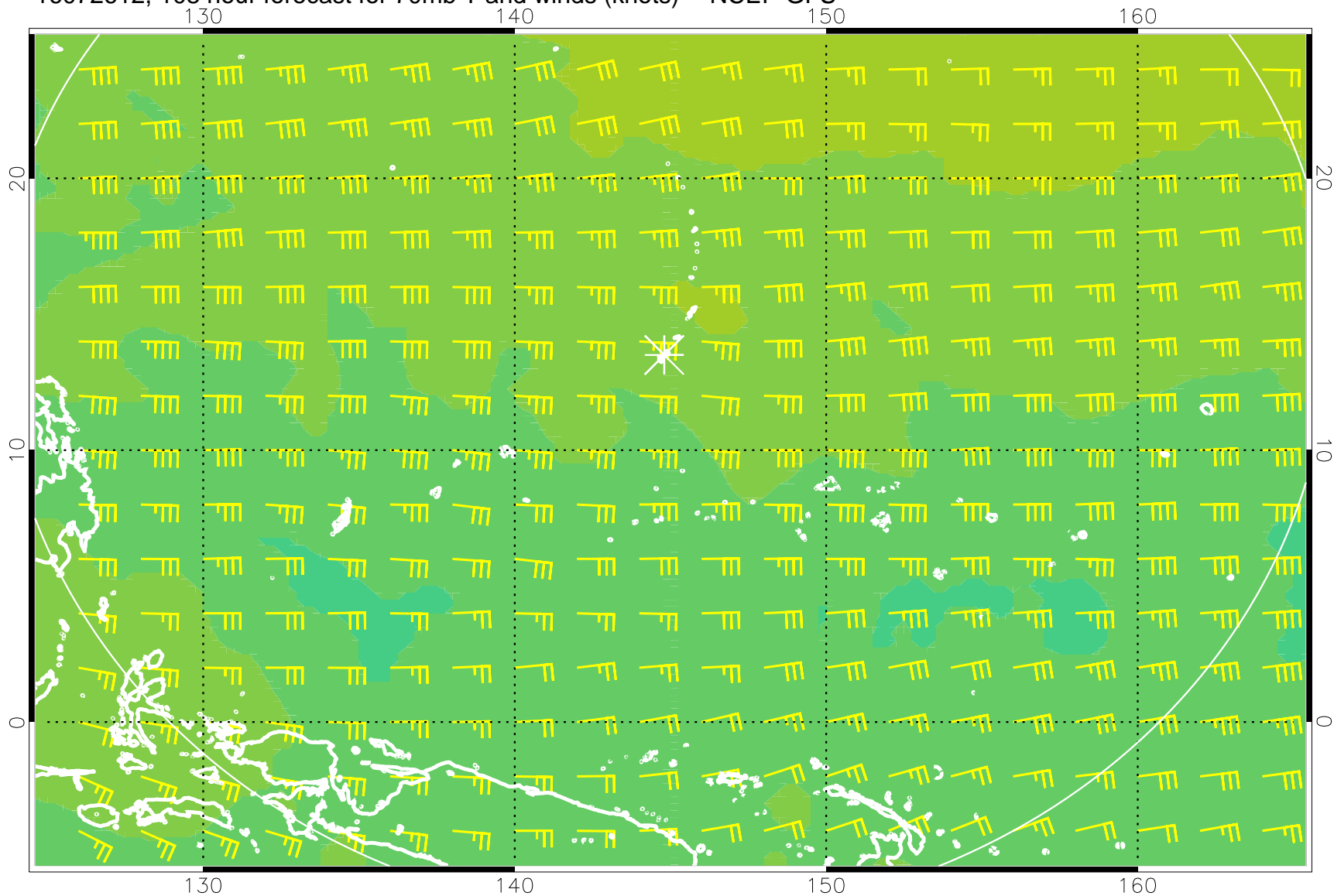
16072612, 108 hour forecast for 70mb T and winds (knots) -- NCEP GFS
