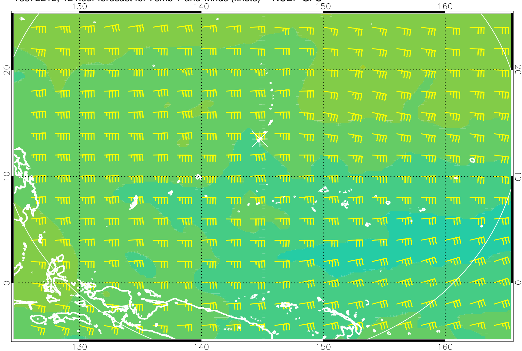
16072212, 12 hour forecast for 70mb T and winds (knots) -- NCEP GFS
