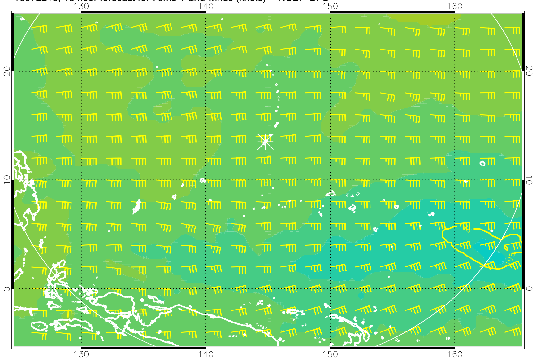
16072218, 18 hour forecast for 70mb T and winds (knots) -- NCEP GFS
