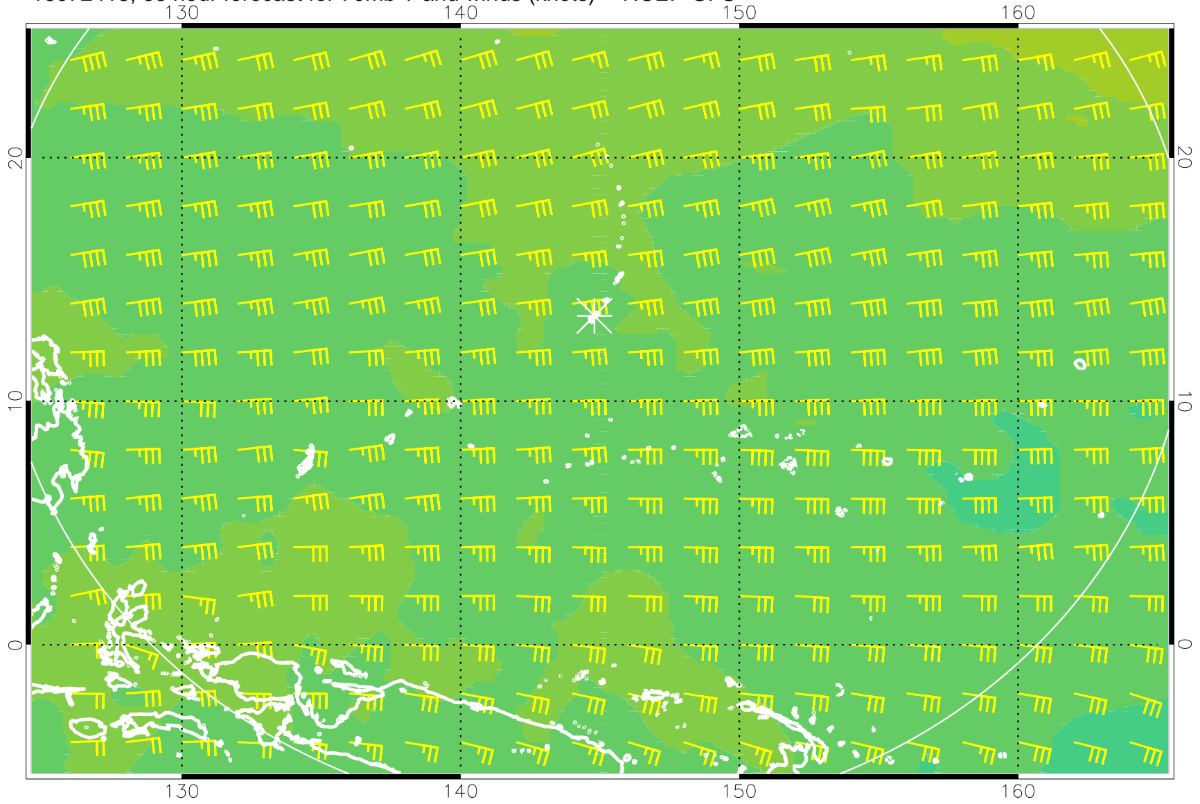
16072418, 66 hour forecast for 70mb T and winds (knots) -- NCEP GFS
