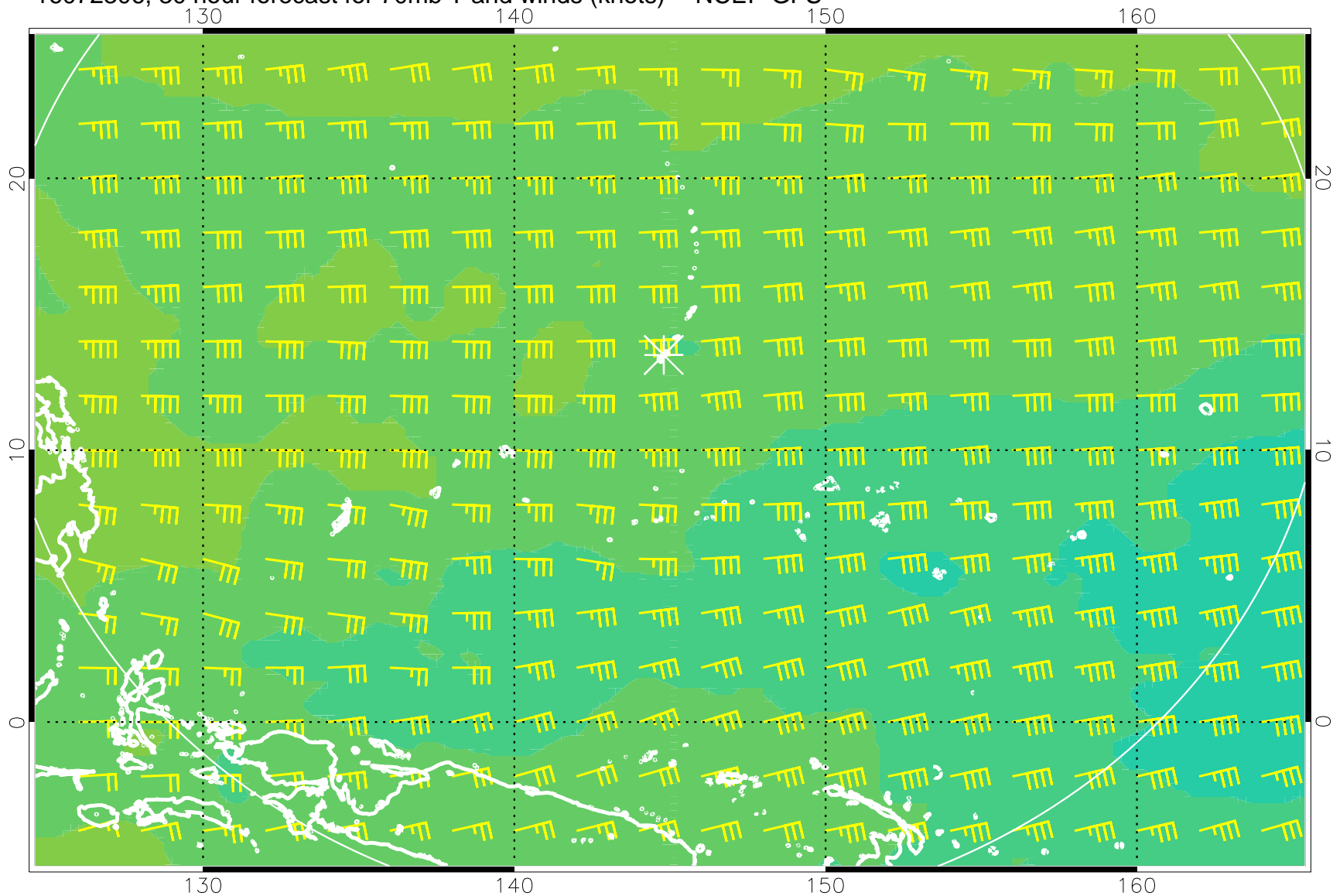
16072306, 30 hour forecast for 70mb T and winds (knots) -- NCEP GFS
