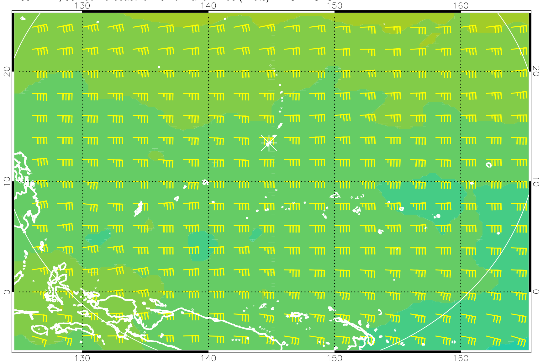
16072412, 60 hour forecast for 70mb T and winds (knots) -- NCEP GFS
