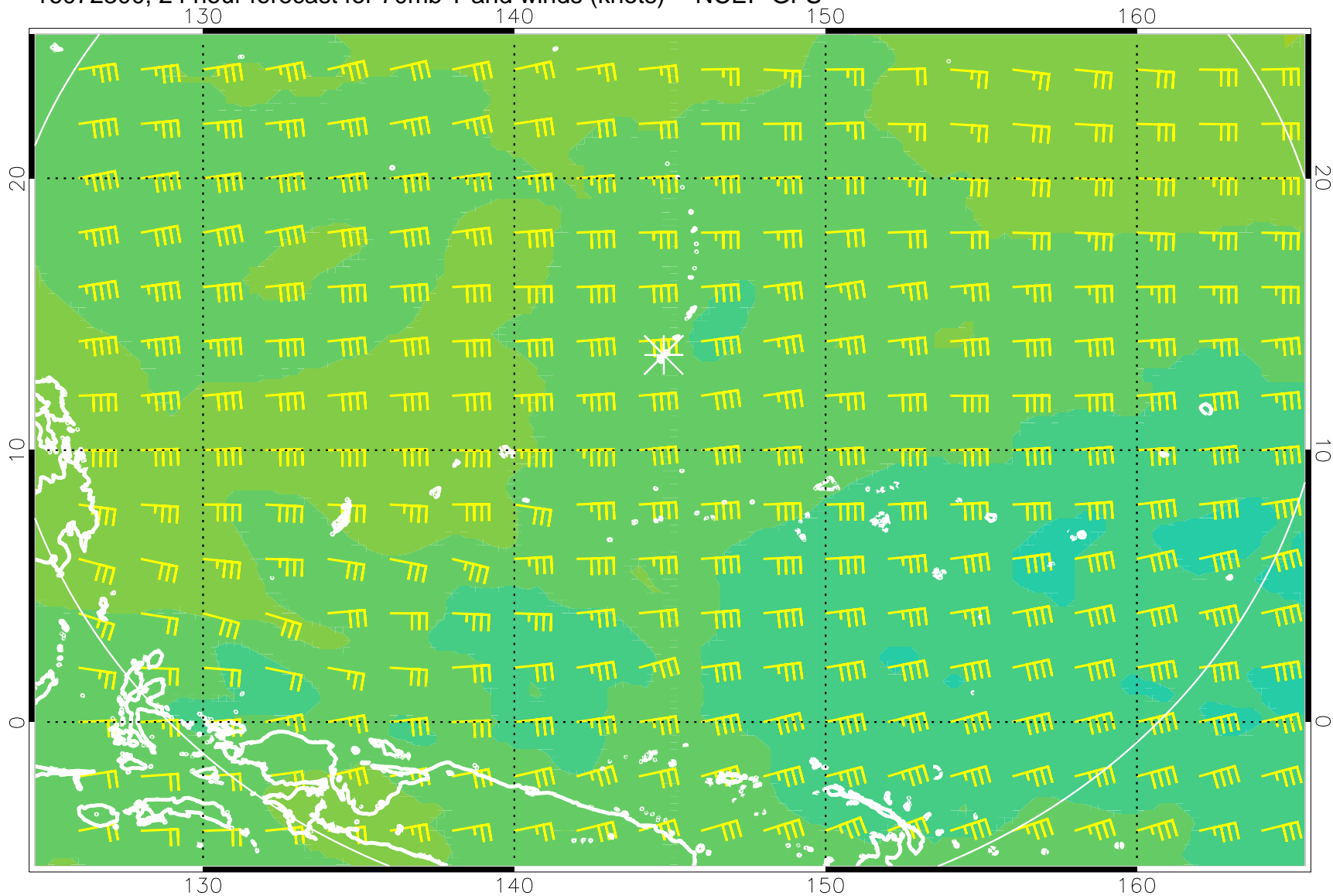
16072300, 24 hour forecast for 70mb T and winds (knots) -- NCEP GFS
