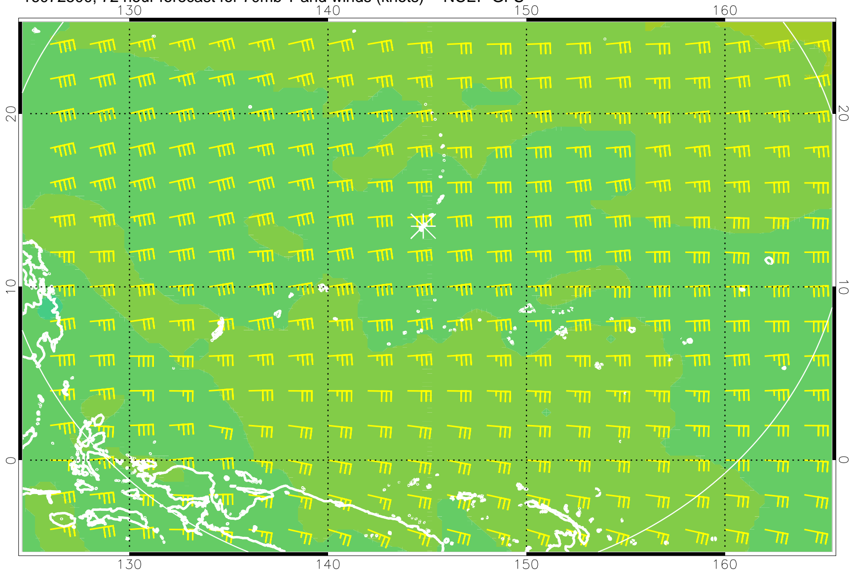
16072500, 72 hour forecast for 70mb T and winds (knots) -- NCEP GFS
