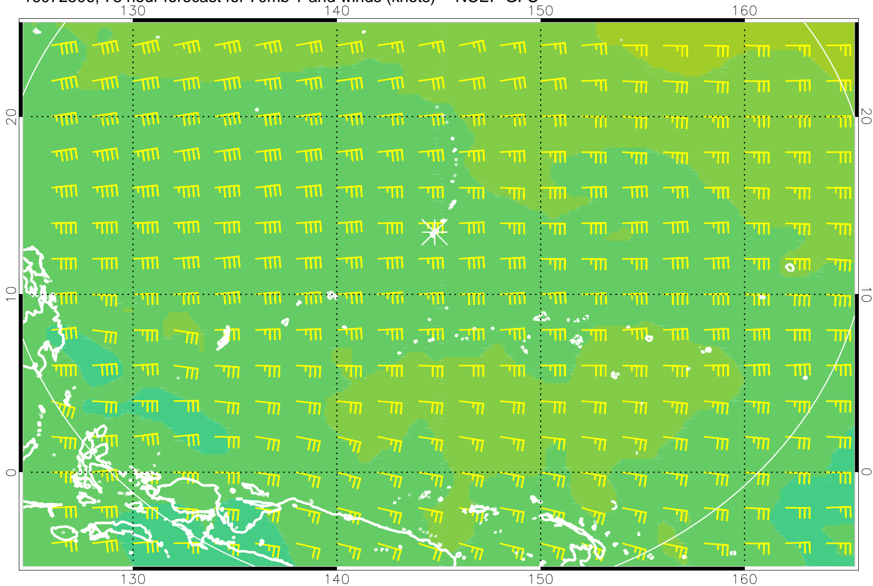
16072506, 78 hour forecast for 70mb T and winds (knots) -- NCEP GFS
