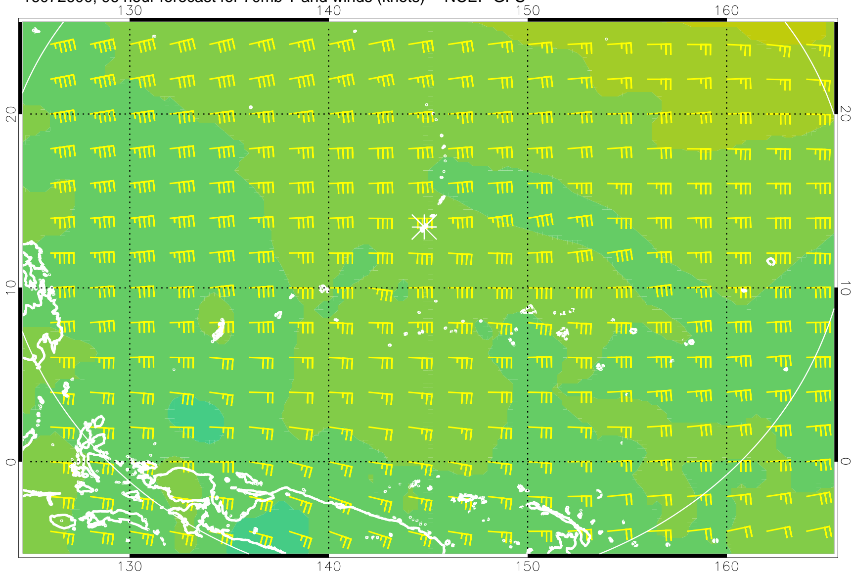
16072600, 96 hour forecast for 70mb T and winds (knots) -- NCEP GFS
