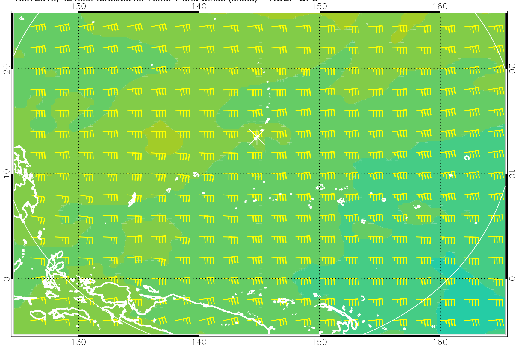
16072318, 42 hour forecast for 70mb T and winds (knots) -- NCEP GFS
