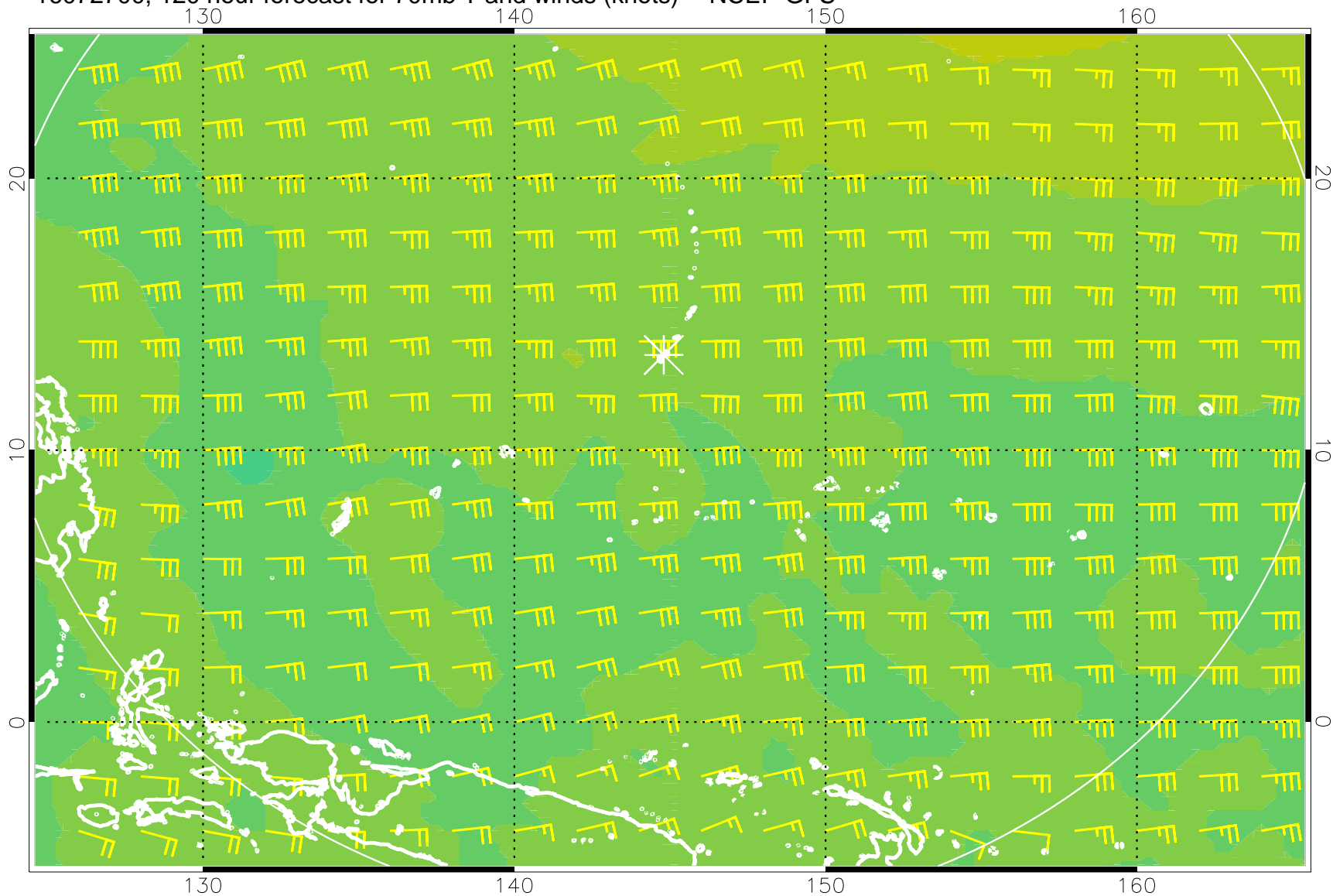
16072700, 120 hour forecast for 70mb T and winds (knots) -- NCEP GFS
