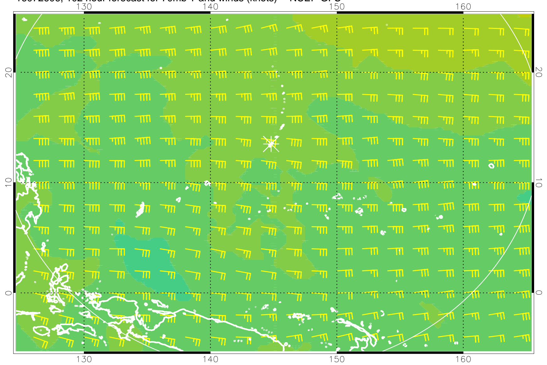
16072606, 102 hour forecast for 70mb T and winds (knots) -- NCEP GFS
