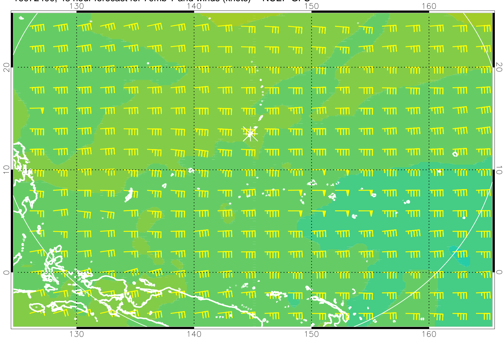
16072400, 48 hour forecast for 70mb T and winds (knots) -- NCEP GFS
