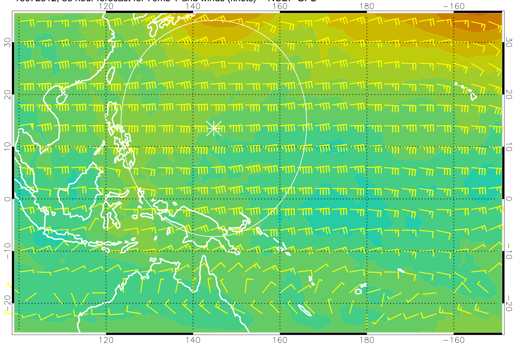
16072312, 36 hour forecast for 70mb T and winds (knots) -- NCEP GFS
