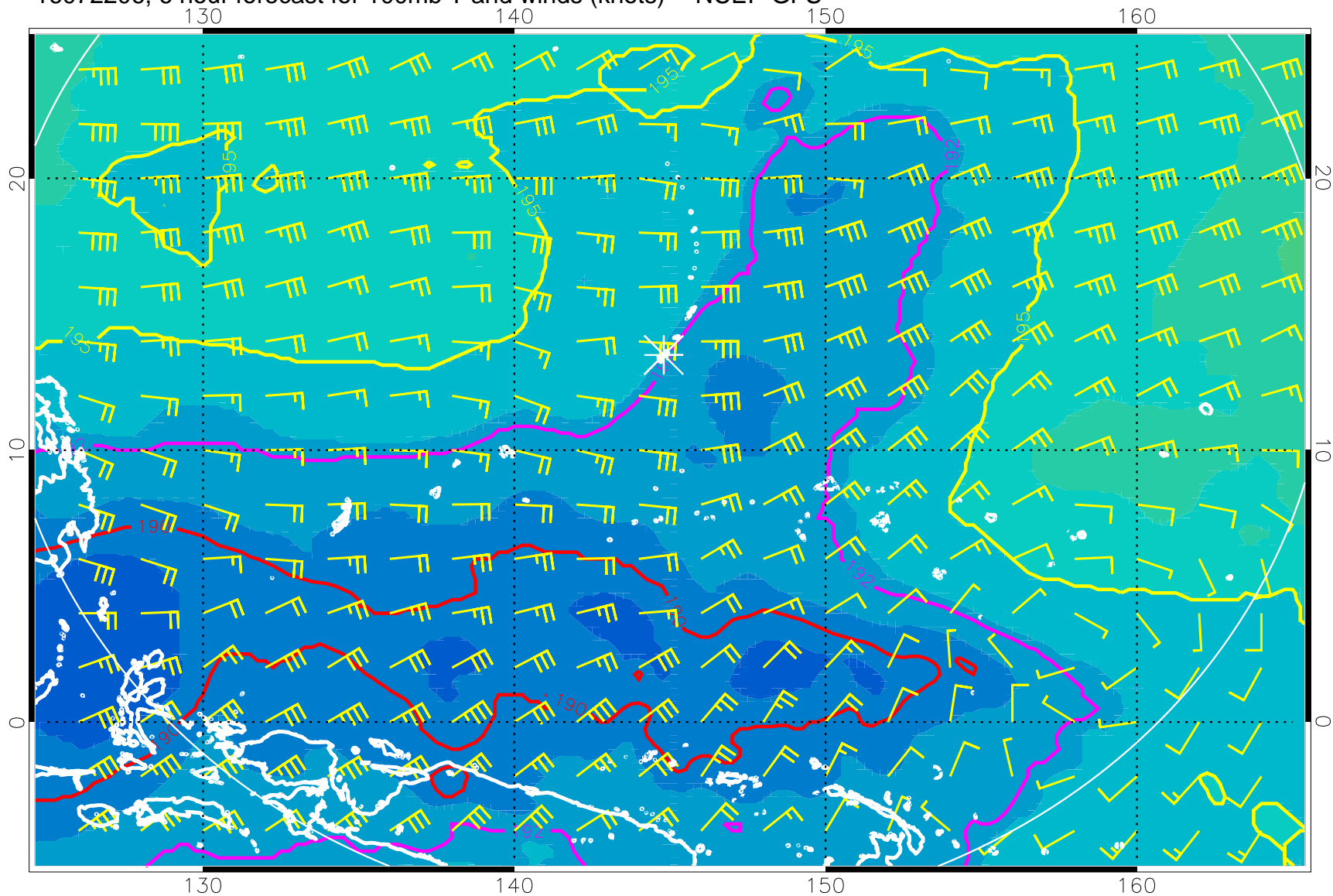
16072206, 6 hour forecast for 100mb T and winds (knots) -- NCEP GFS
