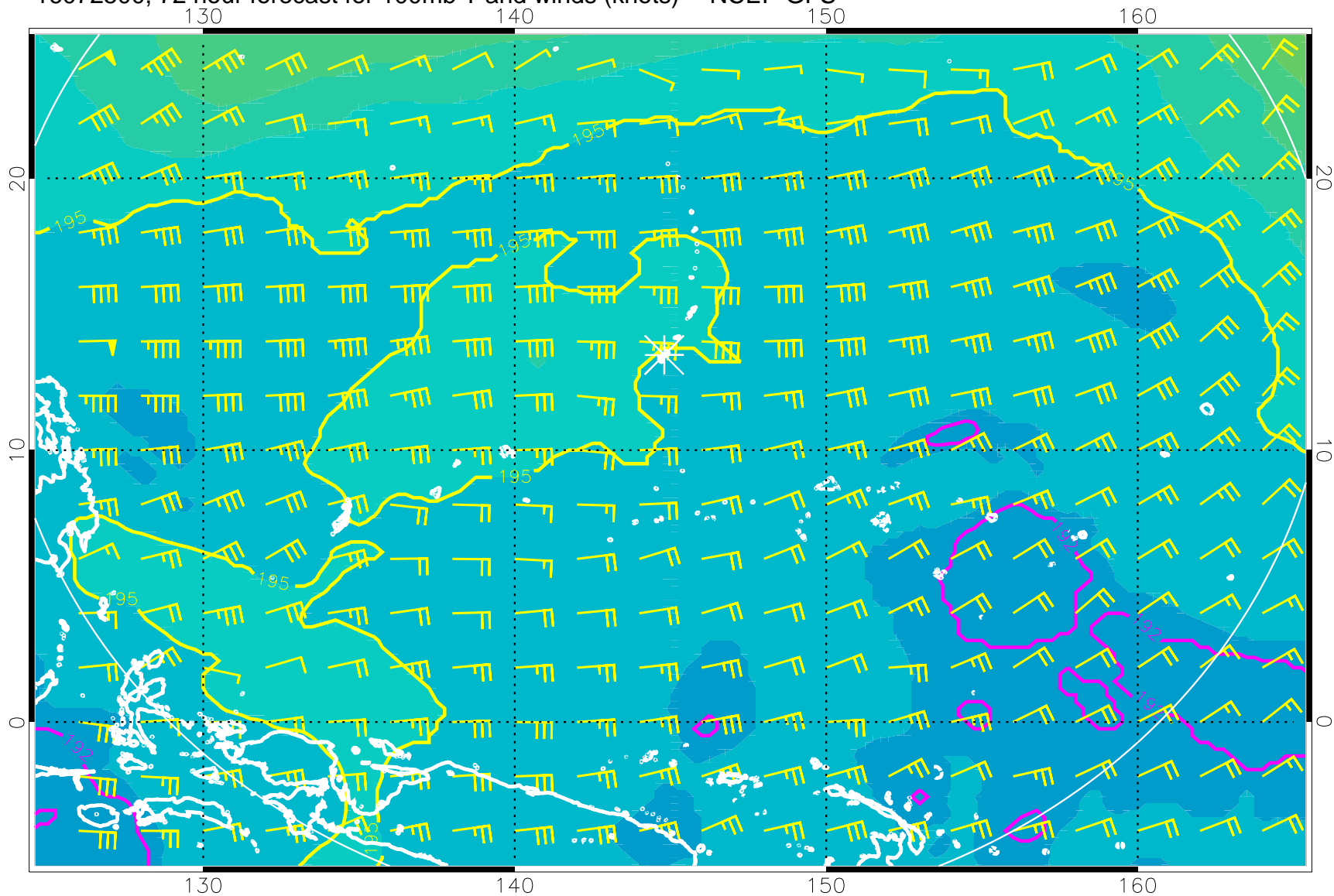
16072500, 72 hour forecast for 100mb T and winds (knots) -- NCEP GFS
