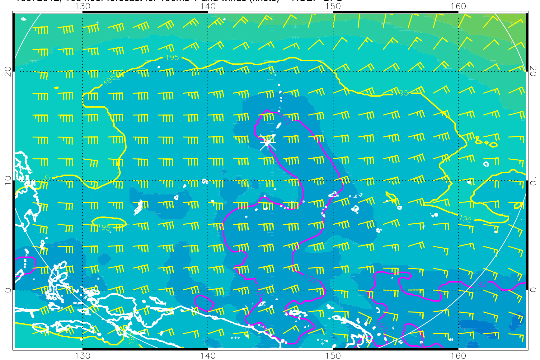
16072612, 108 hour forecast for 100mb T and winds (knots) -- NCEP GFS
