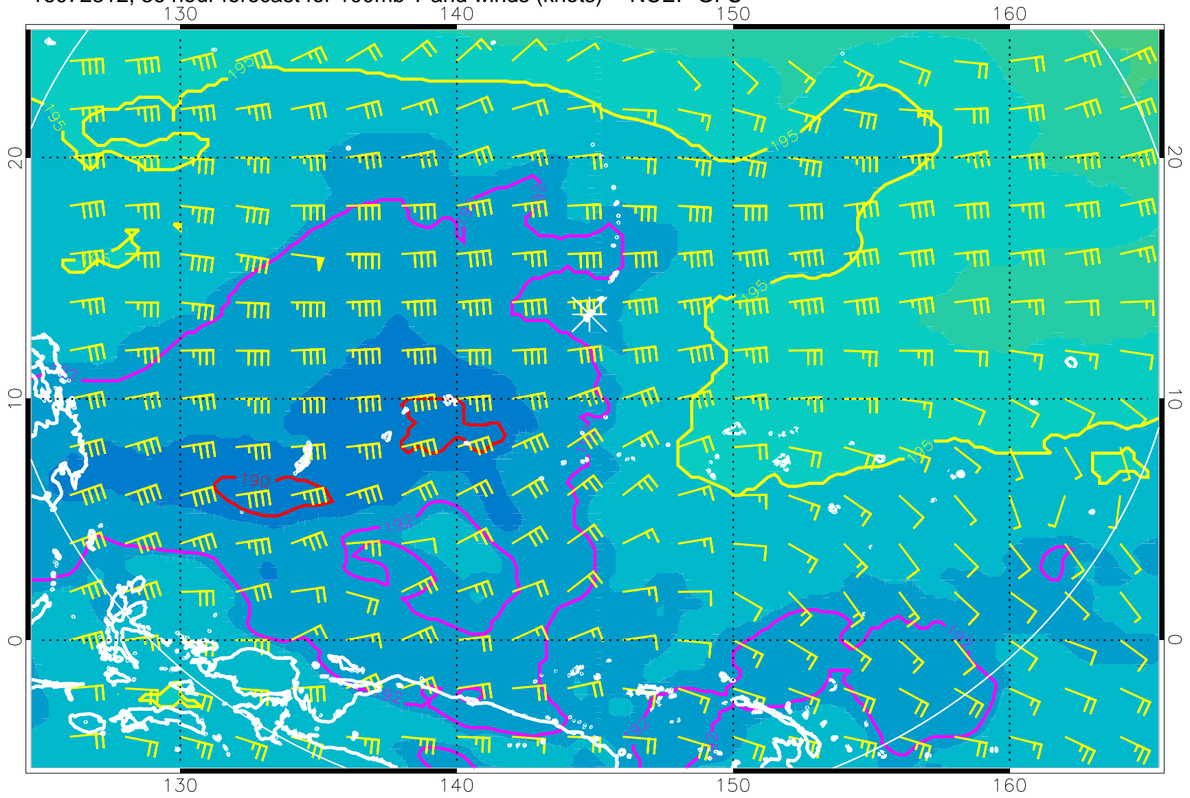
16072312, 36 hour forecast for 100mb T and winds (knots) -- NCEP GFS
