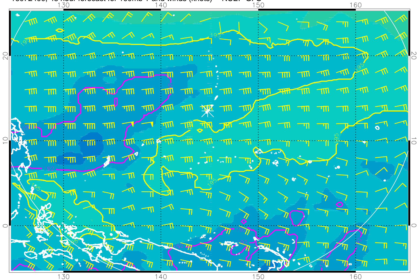
16072400, 48 hour forecast for 100mb T and winds (knots) -- NCEP GFS
