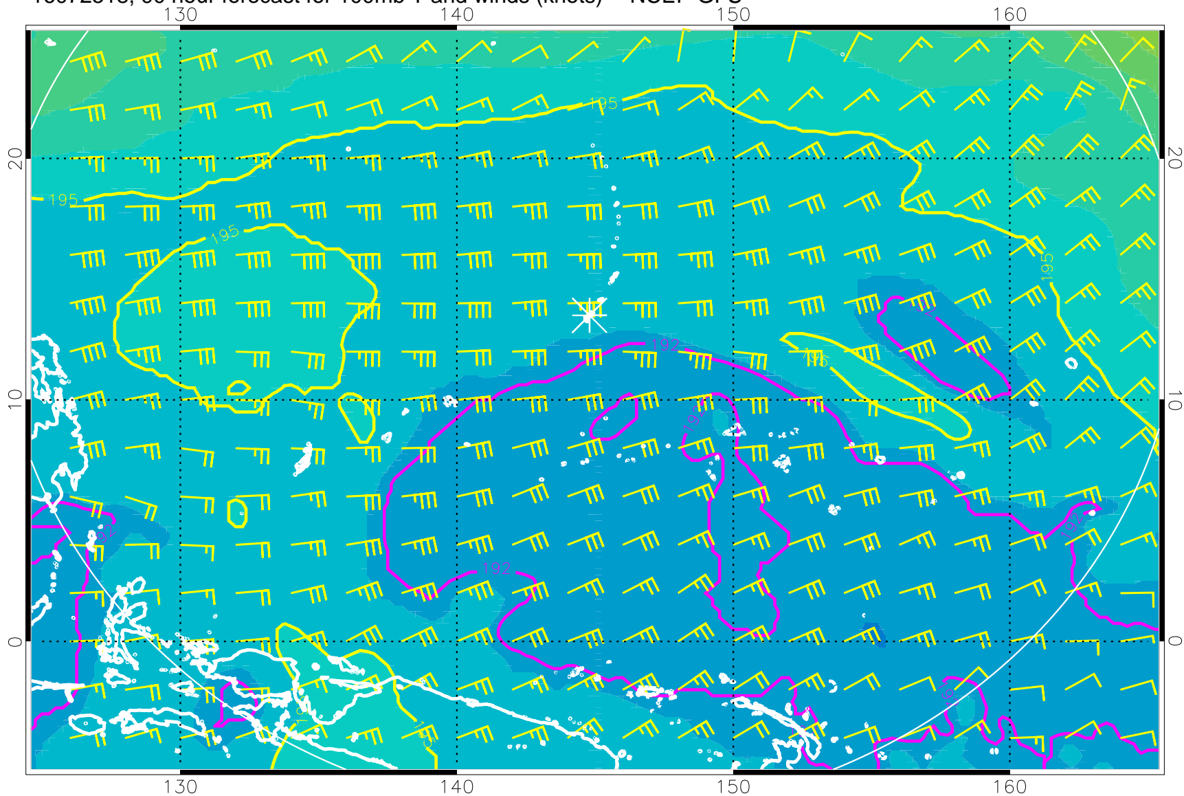
16072518, 90 hour forecast for 100mb T and winds (knots) -- NCEP GFS
