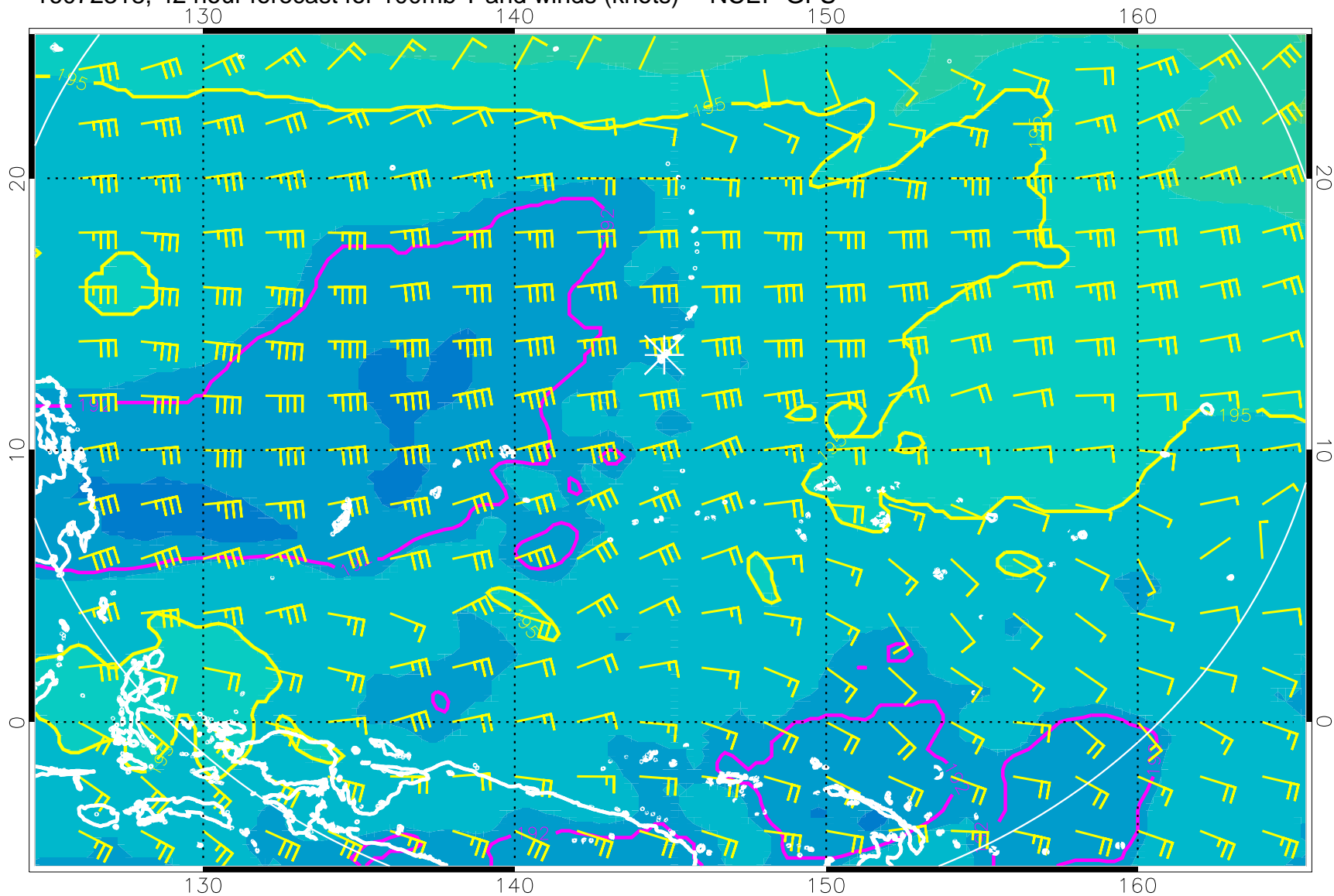
16072318, 42 hour forecast for 100mb T and winds (knots) -- NCEP GFS
