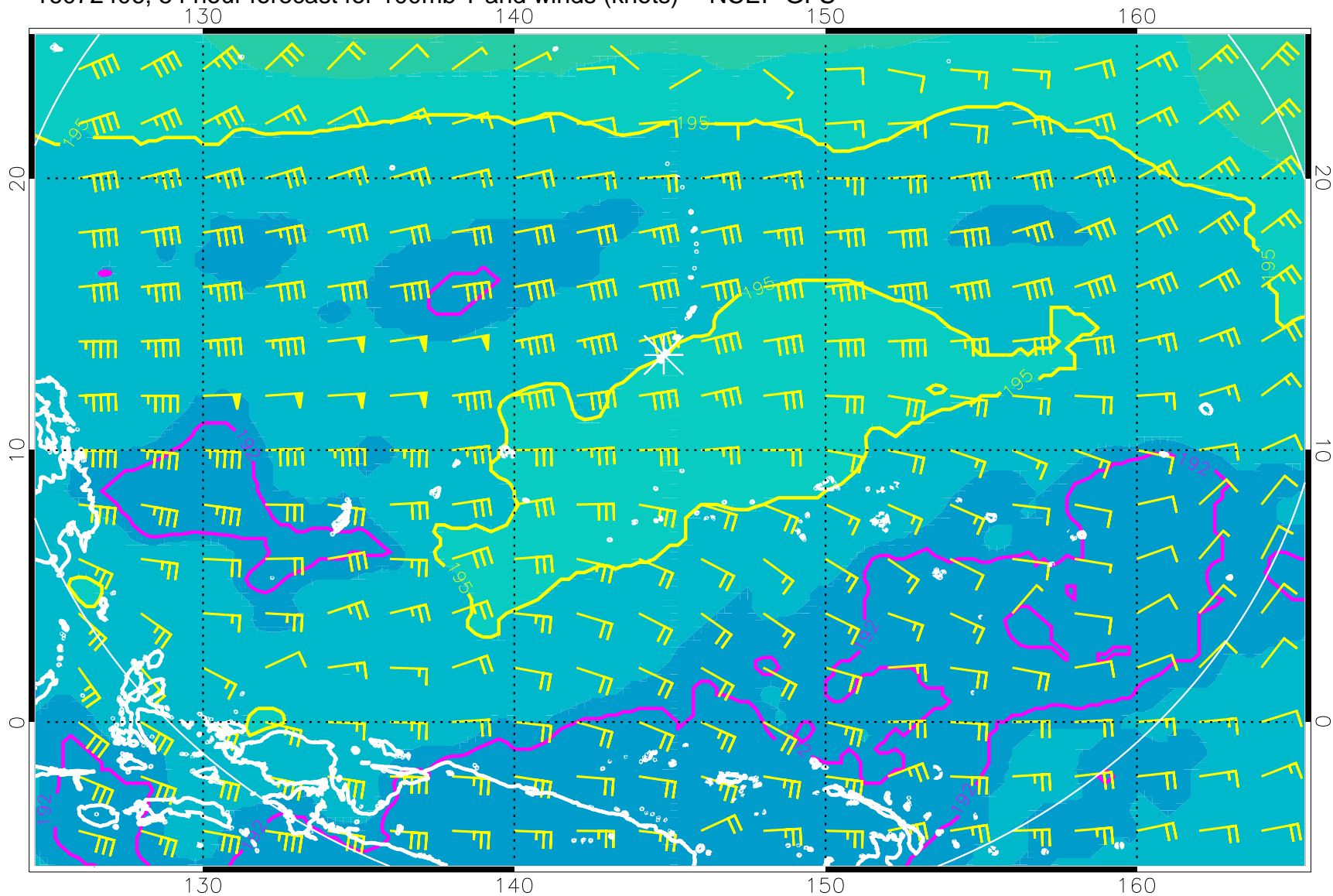
16072406, 54 hour forecast for 100mb T and winds (knots) -- NCEP GFS
