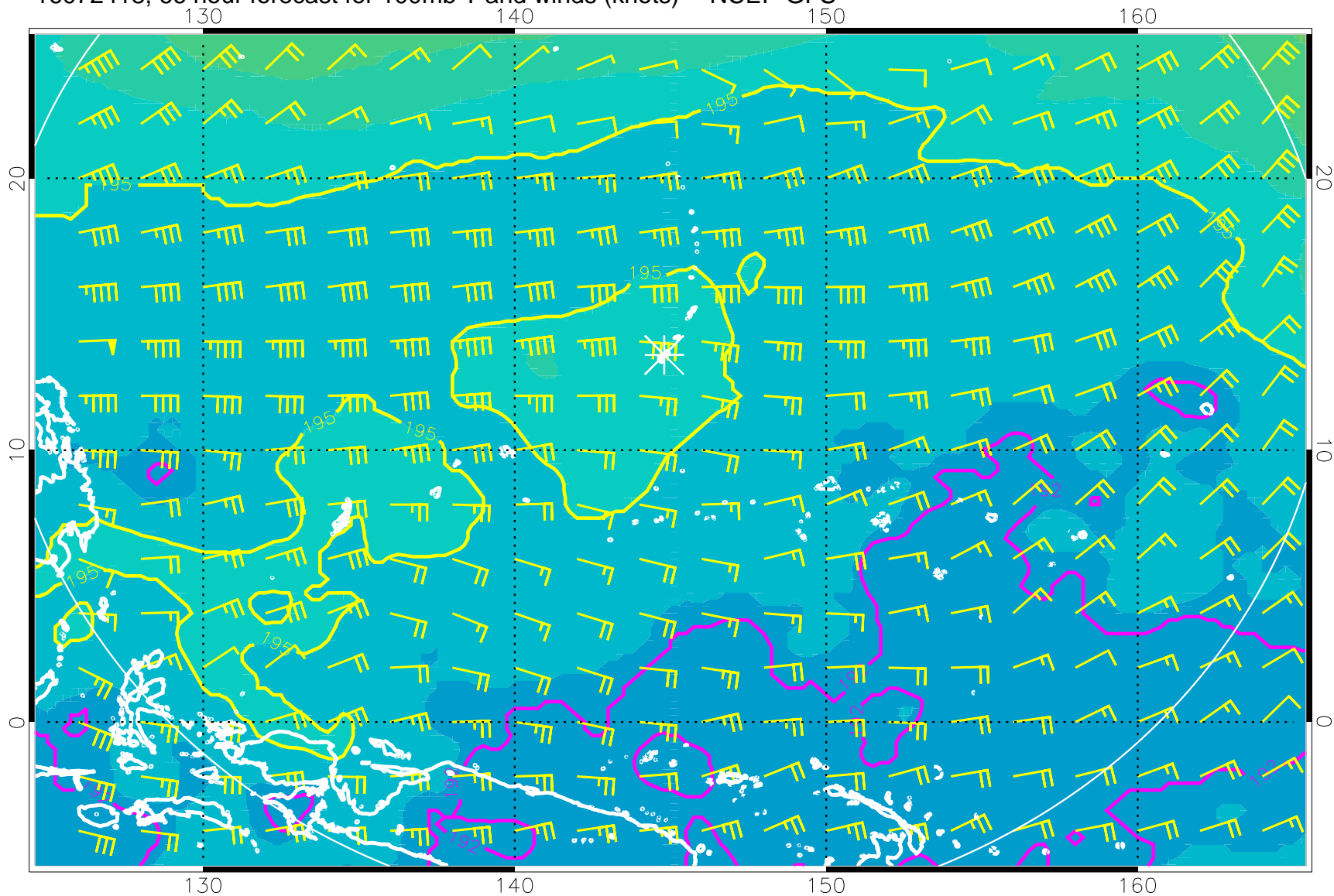
16072418, 66 hour forecast for 100mb T and winds (knots) -- NCEP GFS
