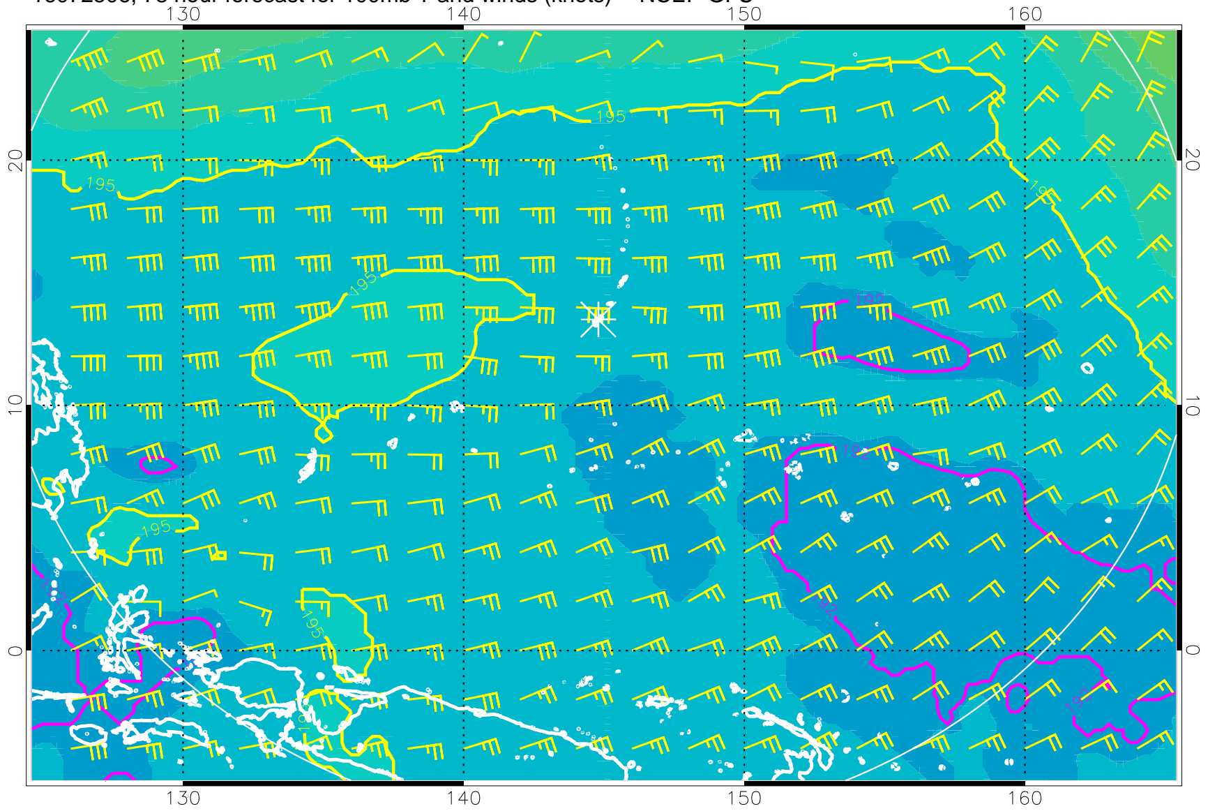
16072506, 78 hour forecast for 100mb T and winds (knots) -- NCEP GFS
