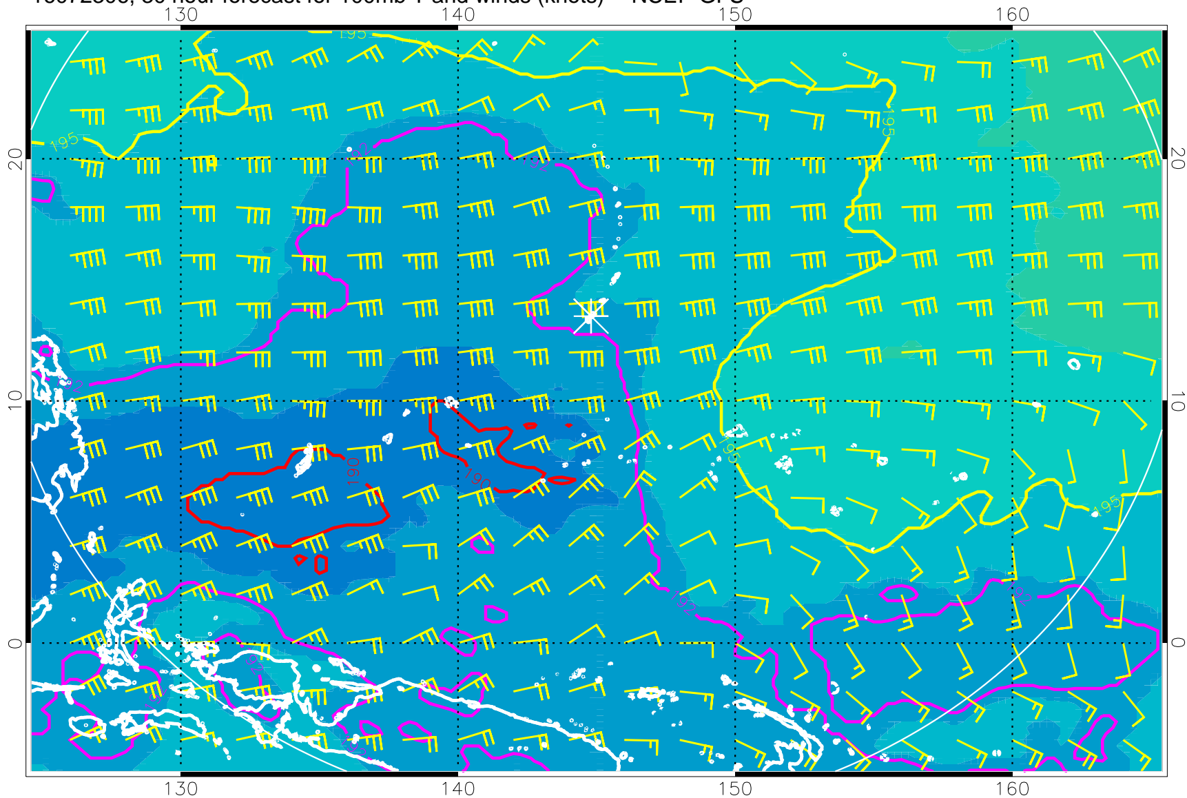
16072306, 30 hour forecast for 100mb T and winds (knots) -- NCEP GFS
