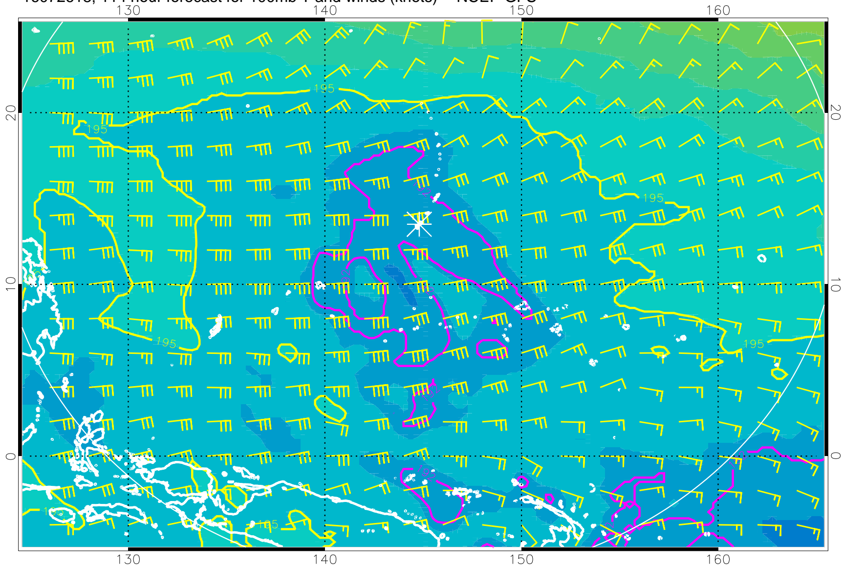
16072618, 114 hour forecast for 100mb T and winds (knots) -- NCEP GFS
