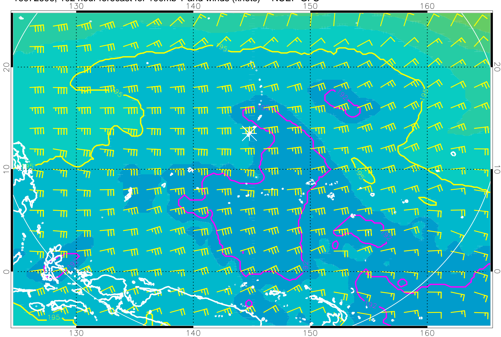
16072606, 102 hour forecast for 100mb T and winds (knots) -- NCEP GFS
