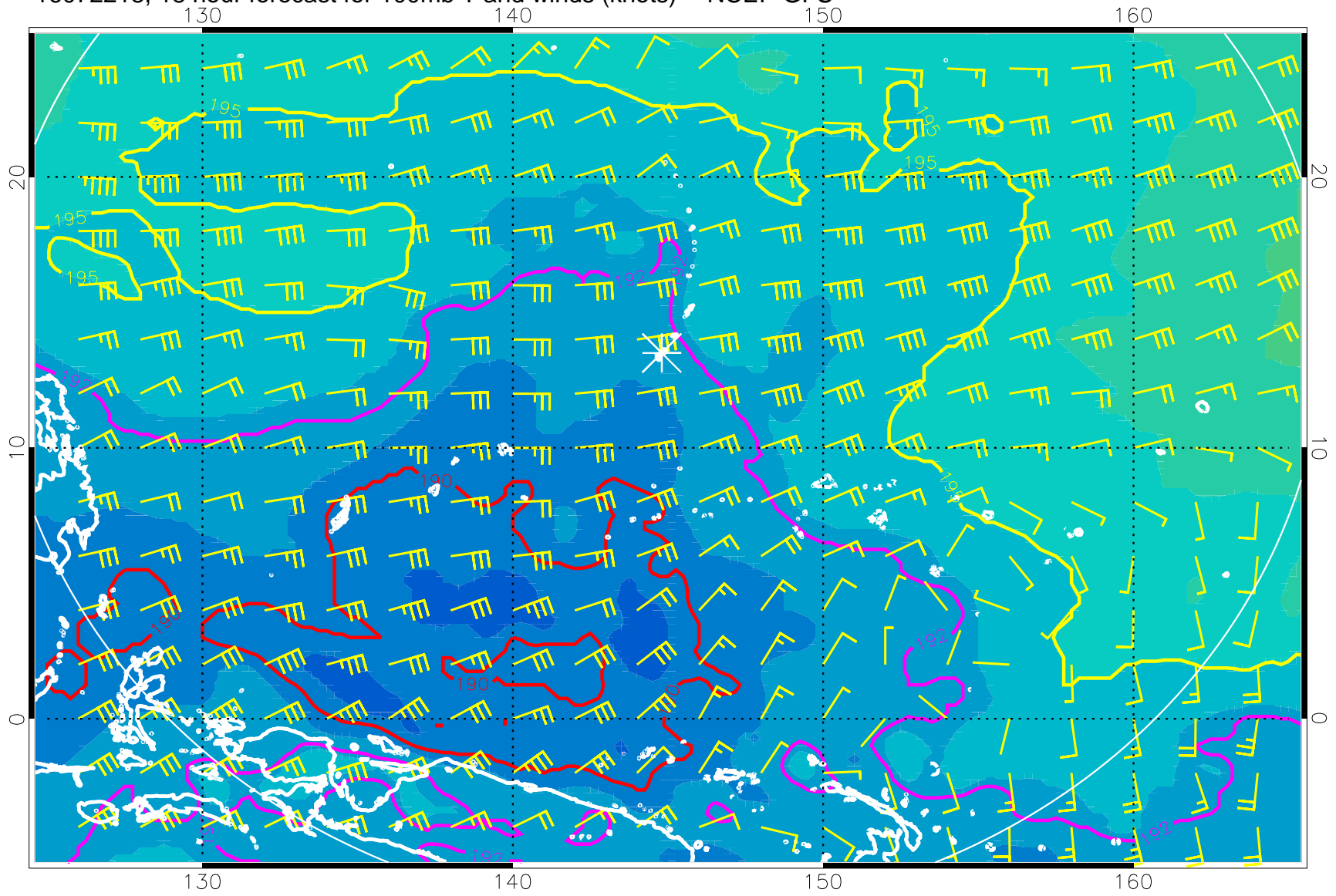
16072218, 18 hour forecast for 100mb T and winds (knots) -- NCEP GFS
