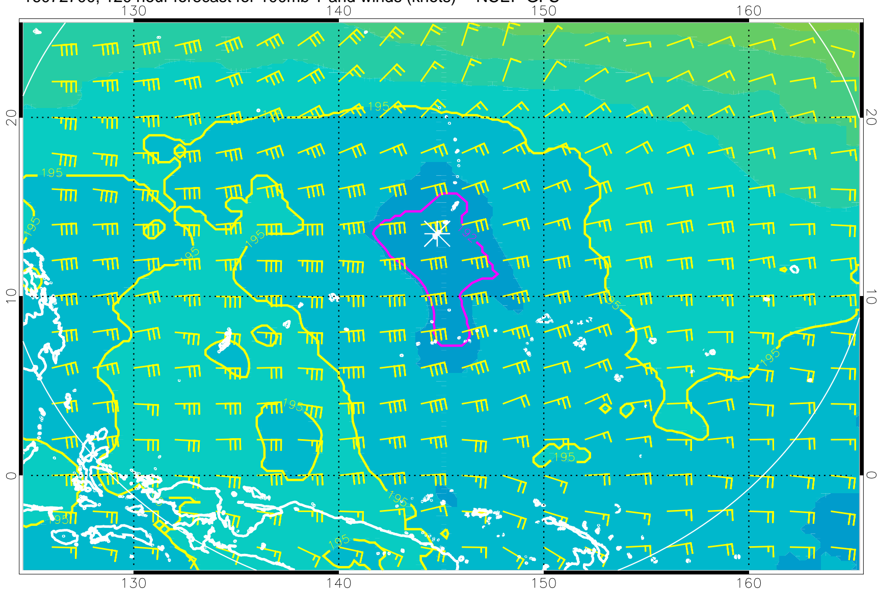
16072700, 120 hour forecast for 100mb T and winds (knots) -- NCEP GFS
