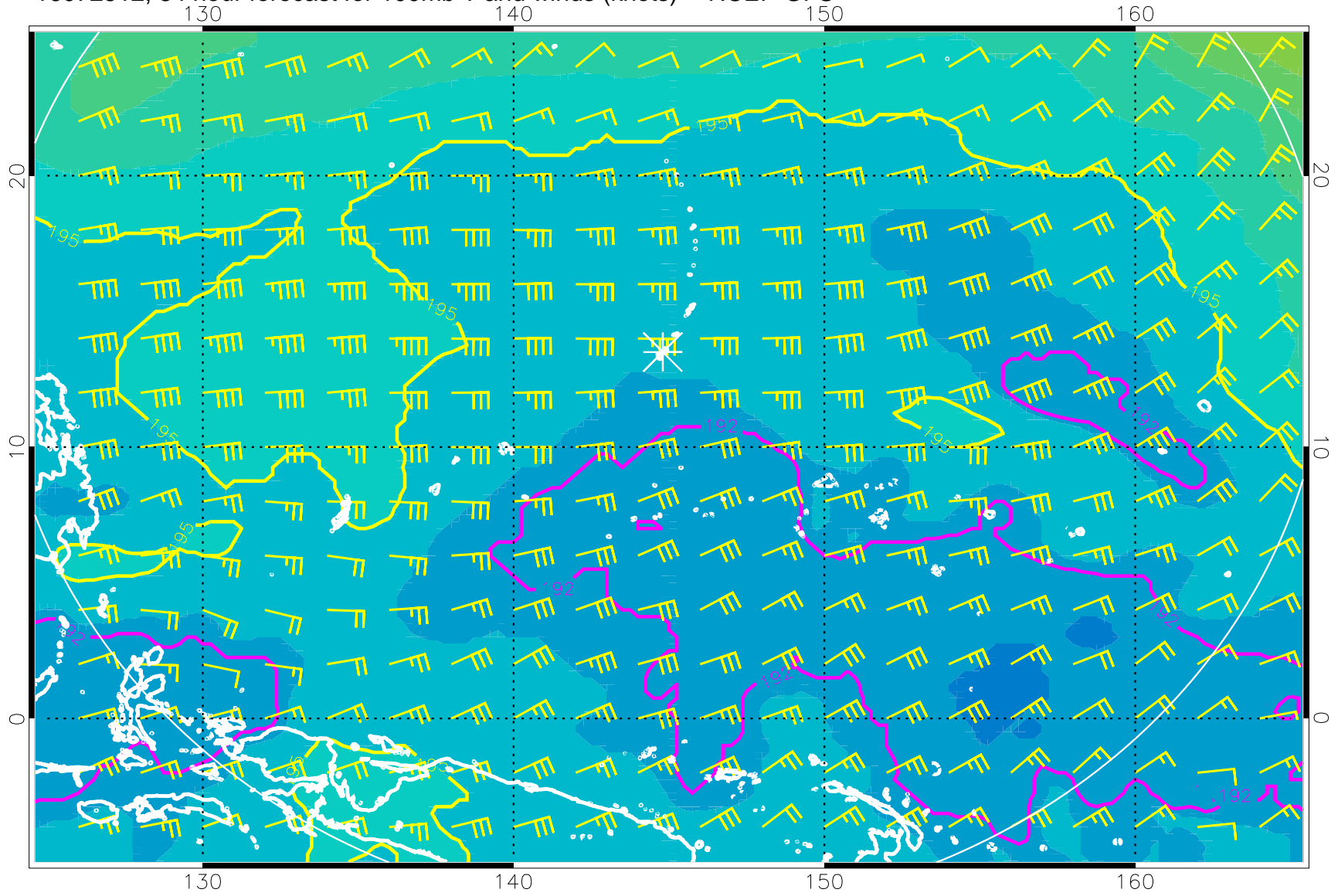
16072512, 84 hour forecast for 100mb T and winds (knots) -- NCEP GFS
