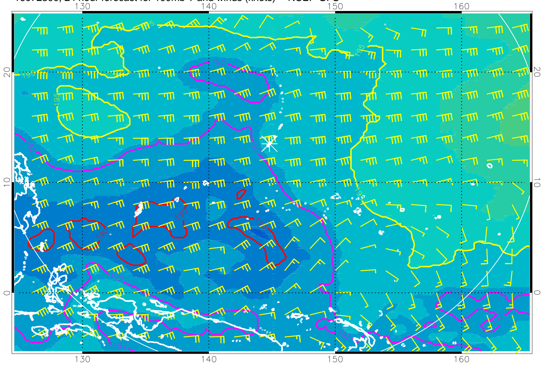
16072300, 24 hour forecast for 100mb T and winds (knots) -- NCEP GFS
