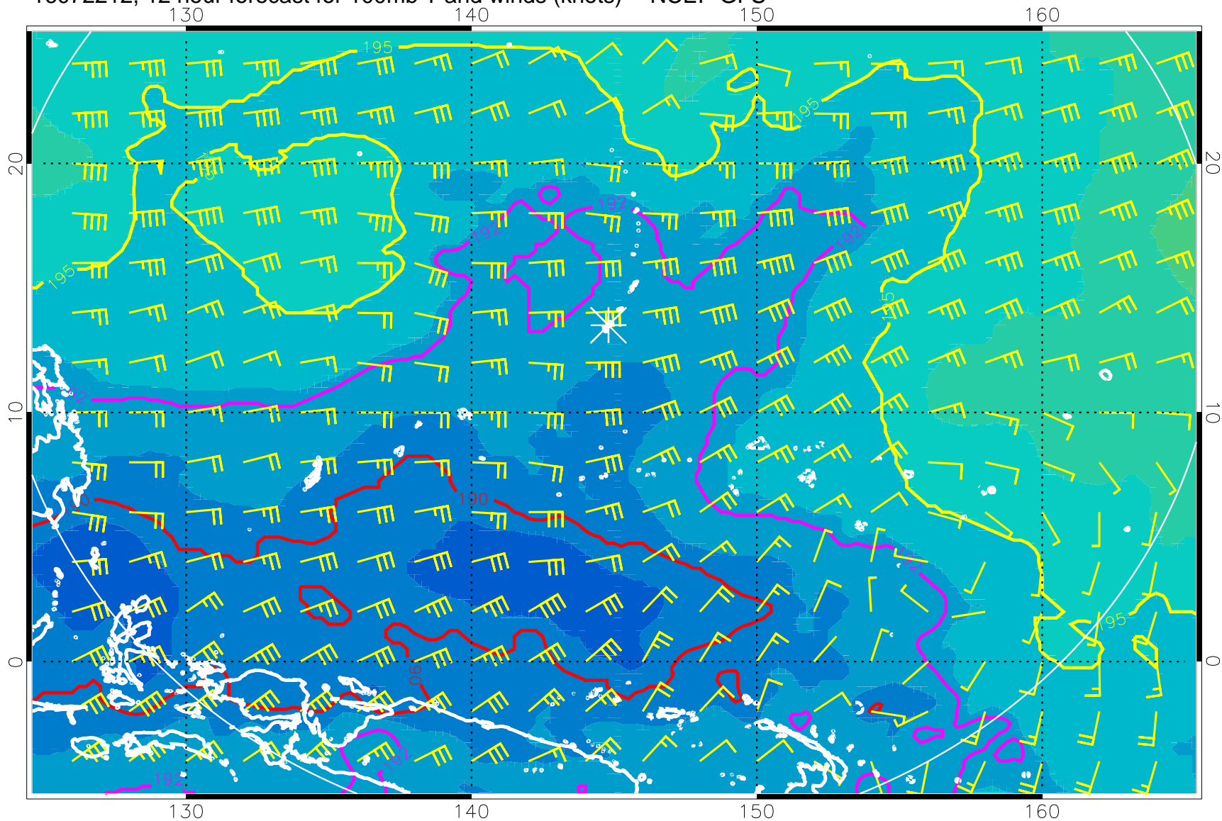
16072212, 12 hour forecast for 100mb T and winds (knots) -- NCEP GFS
