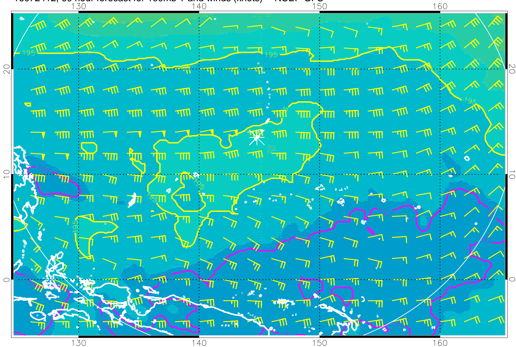
16072412, 60 hour forecast for 100mb T and winds (knots) -- NCEP GFS
