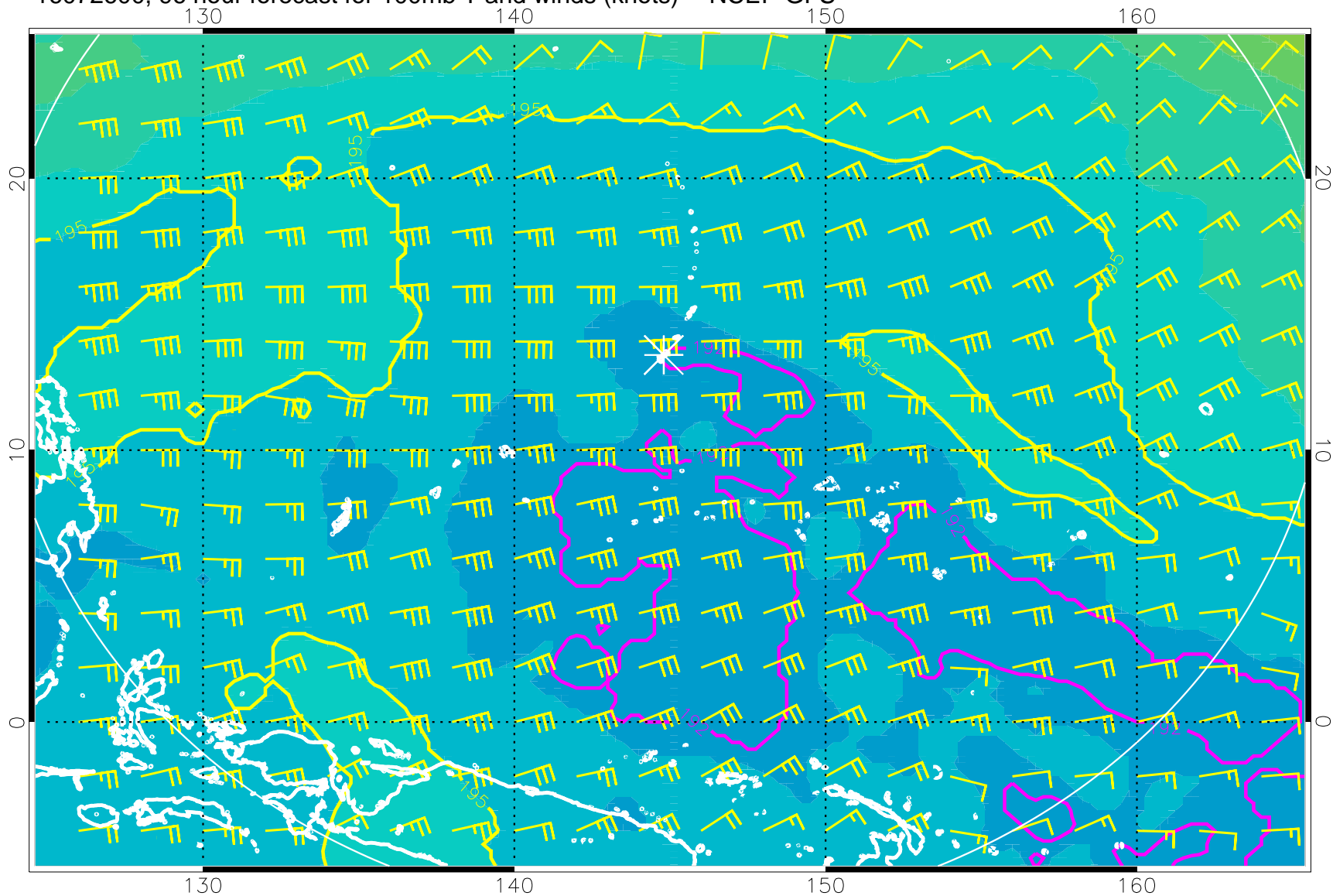
16072600, 96 hour forecast for 100mb T and winds (knots) -- NCEP GFS
