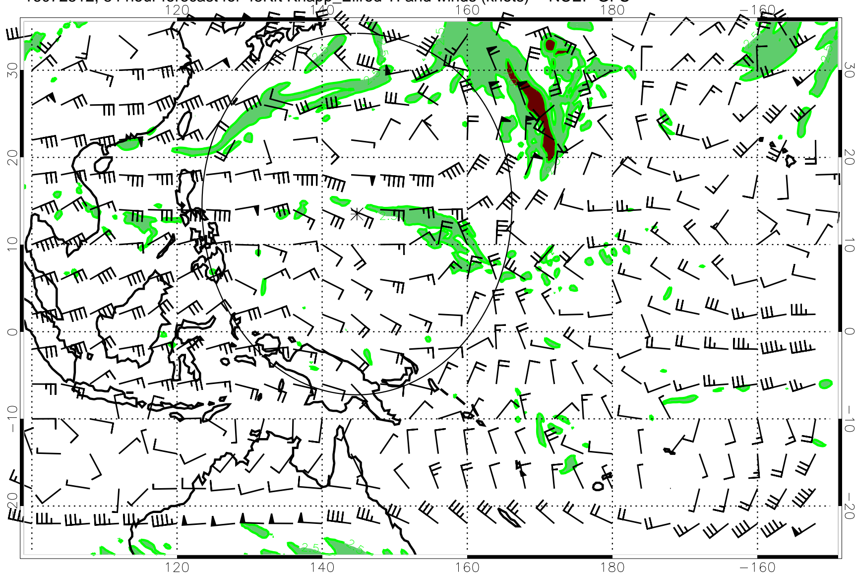
16072512, 84 hour forecast for 45Kft Knapp_Ellrod TI and winds (knots) -- NCEP GFS
