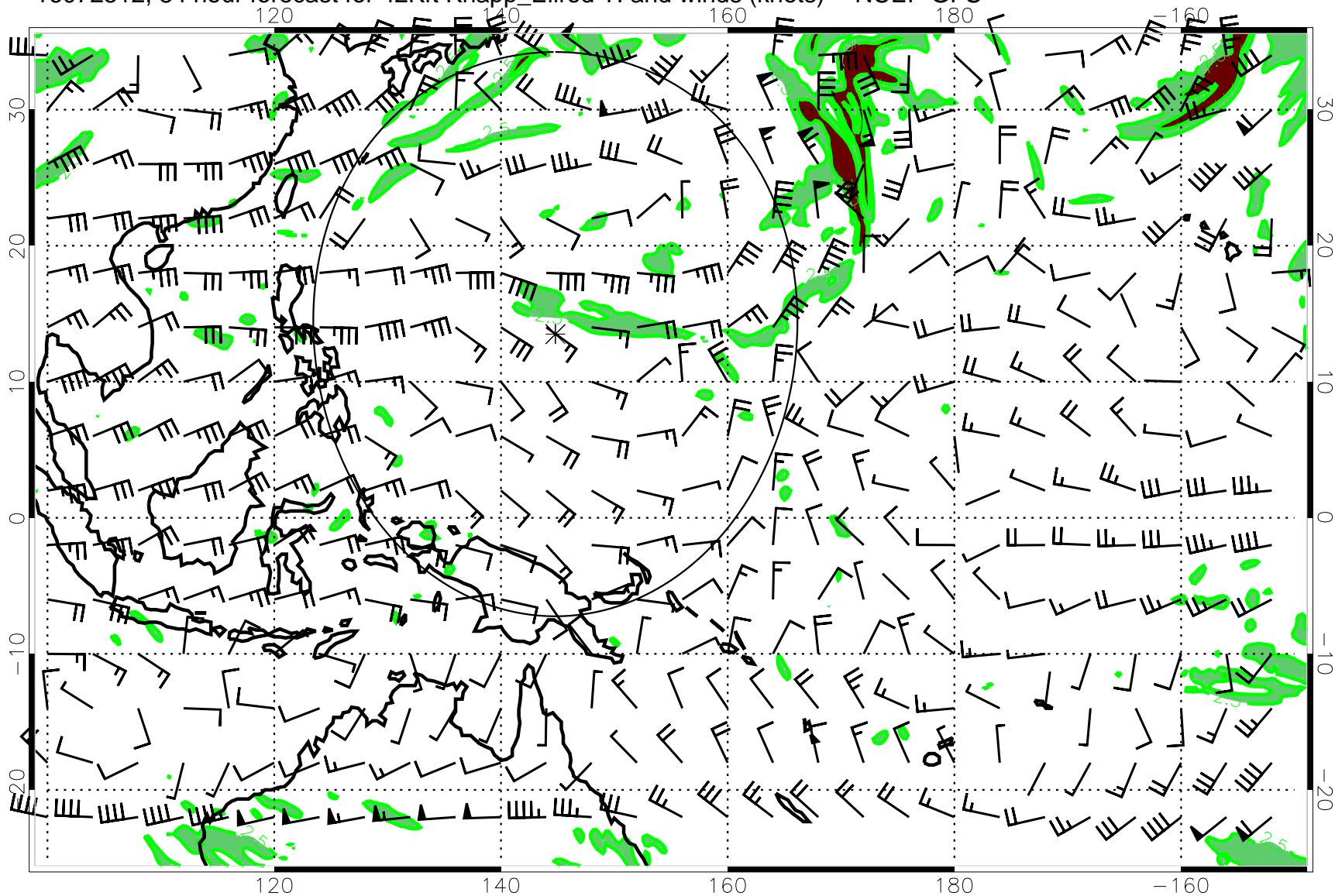
16072512, 84 hour forecast for 42Kft Knapp_Ellrod TI and winds (knots) -- NCEP GFS
