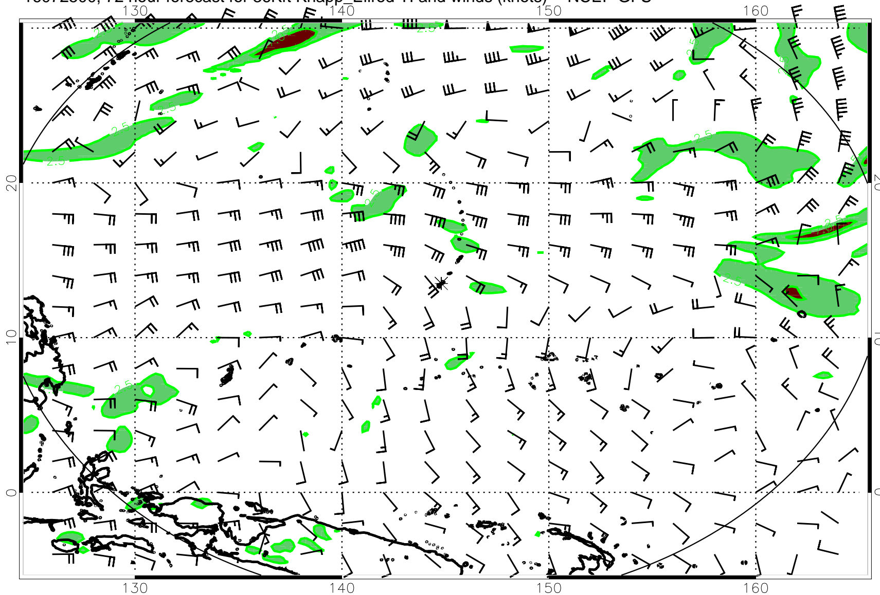
16072500, 72 hour forecast for 36Kft Knapp_Ellrod TI and winds (knots) -- NCEP GFS
