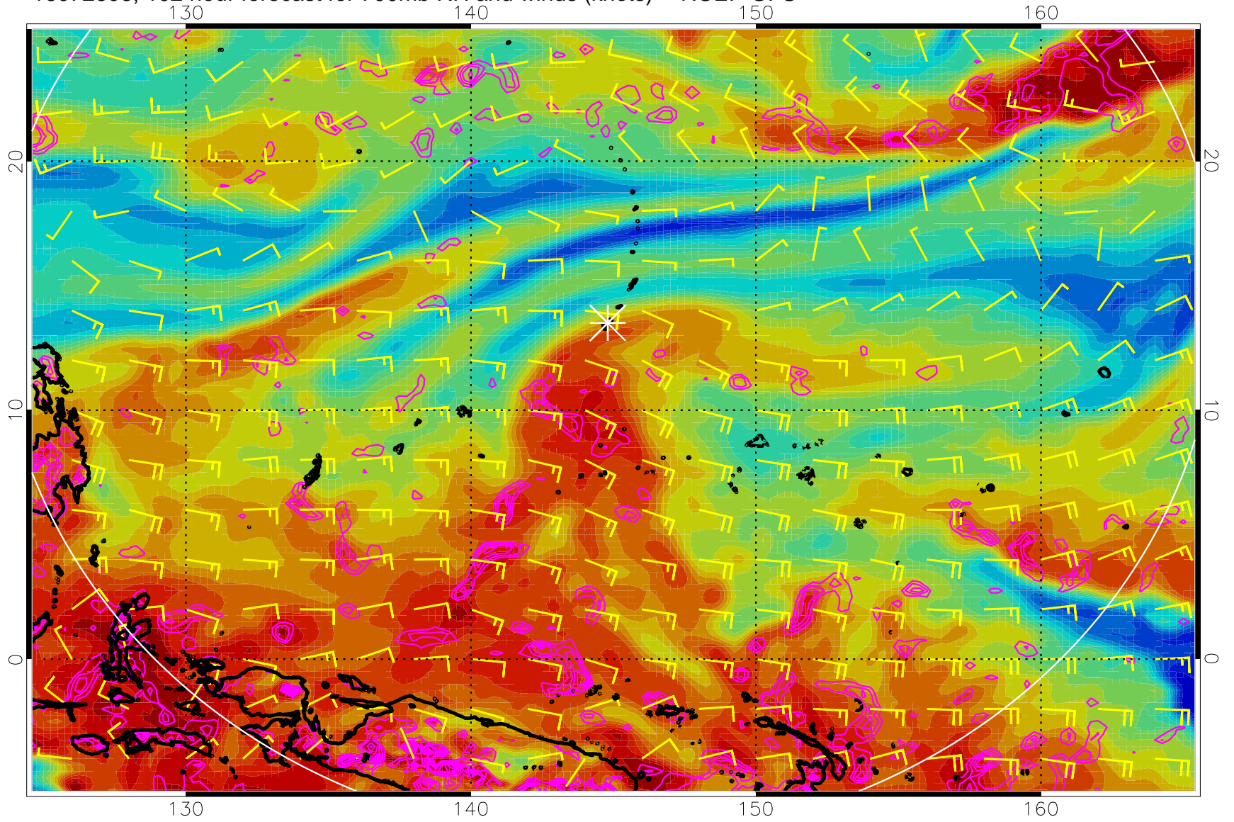
16072606, 102 hour forecast for 700mb RH and winds (knots) -- NCEP GFS
