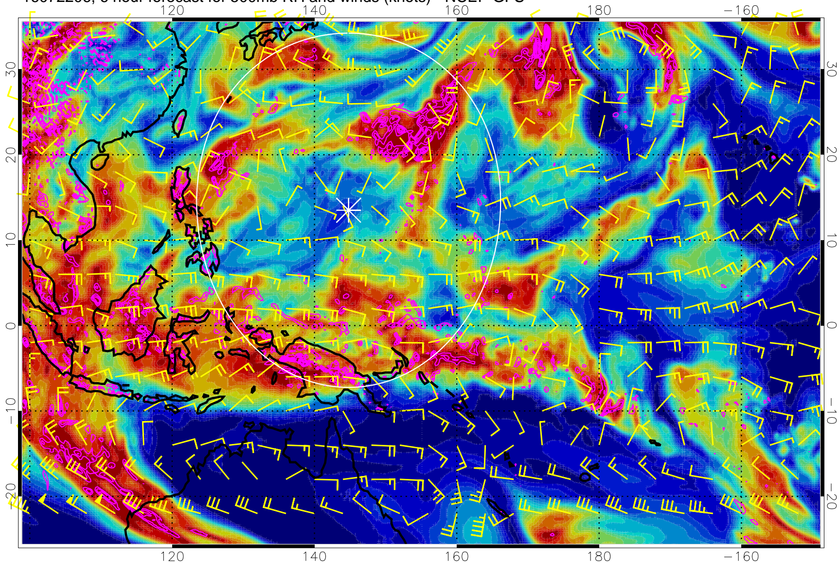
16072206, 6 hour forecast for 500mb RH and winds (knots) - NCEP GFS
