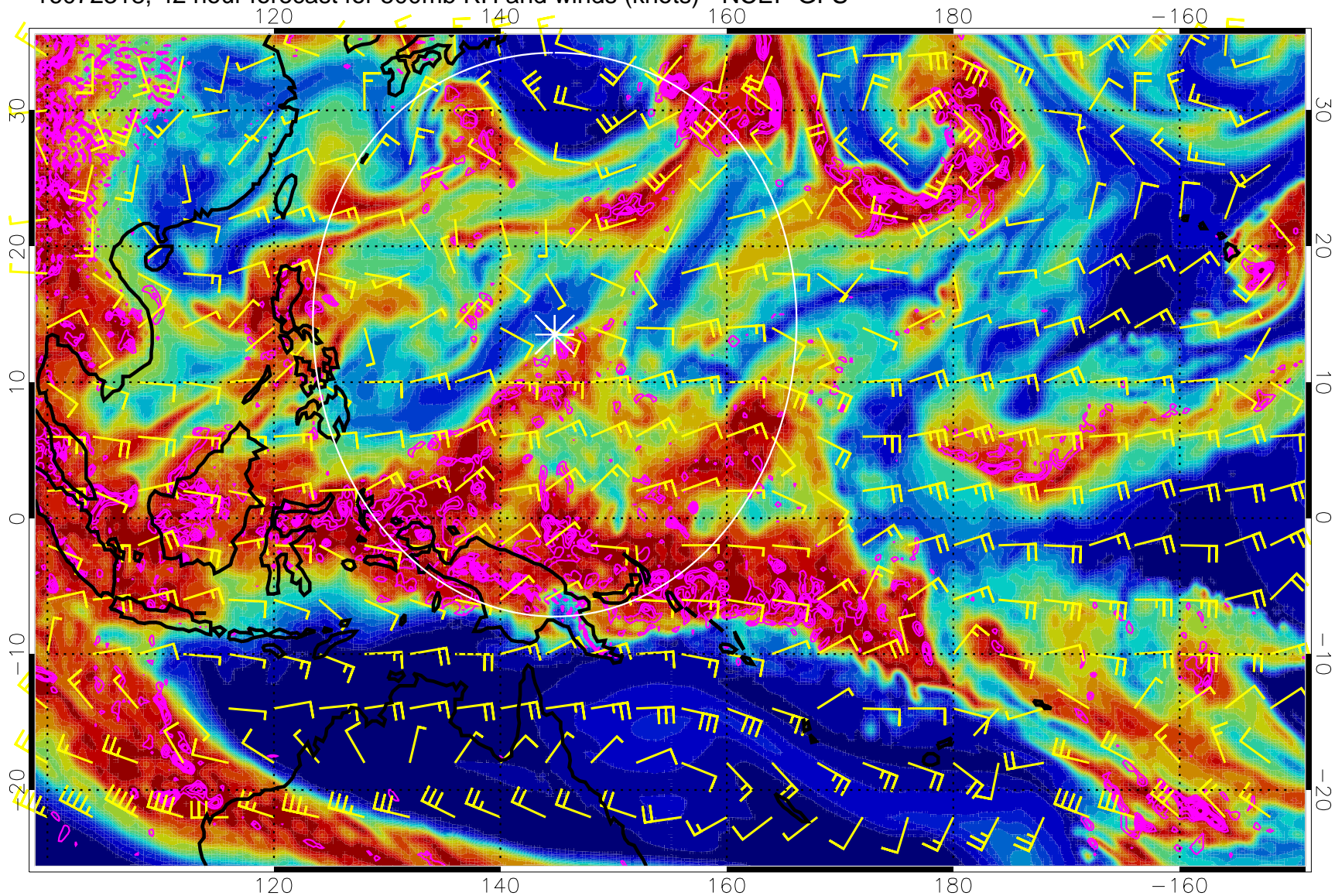
16072318, 42 hour forecast for 500mb RH and winds (knots) - NCEP GFS
