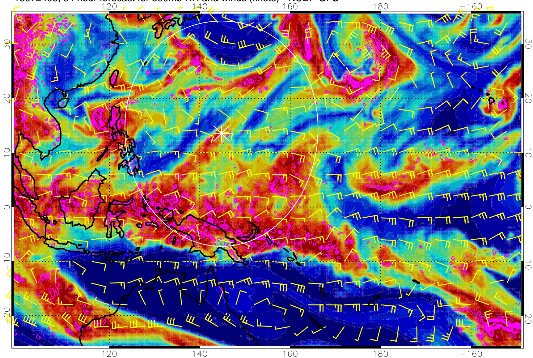
16072406, 54 hour forecast for 500mb RH and winds (knots) - NCEP GFS
