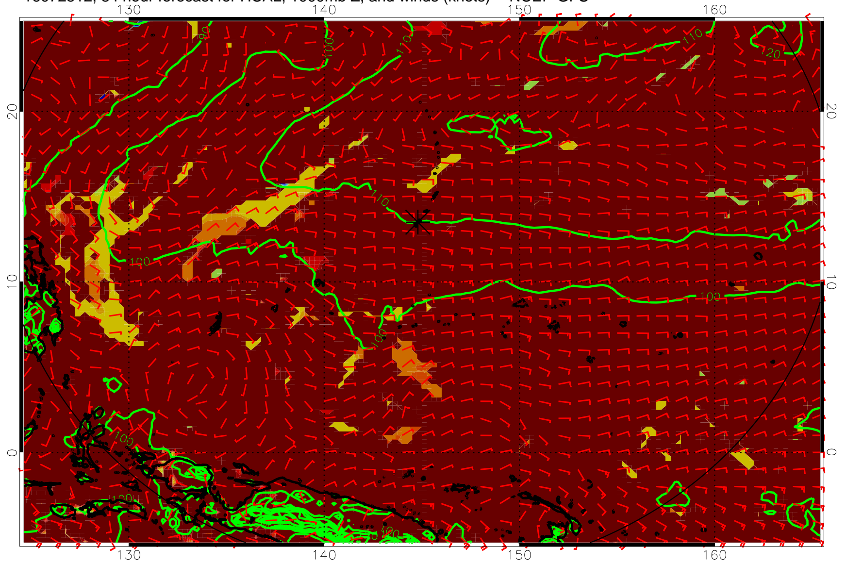
16072512, 84 hour forecast for HCAL, 1000mb Z, and winds (knots) -- NCEP GFS
