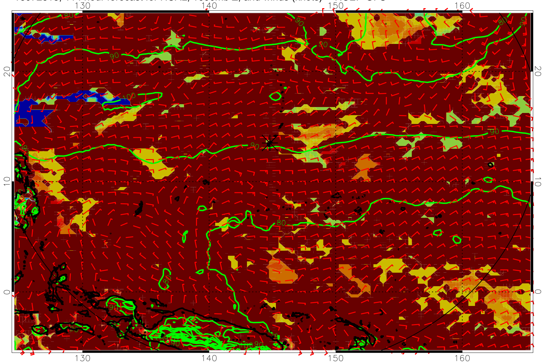
16072618, 114 hour forecast for HCAL, 1000mb Z, and winds (knots) -- NCEP GFS
