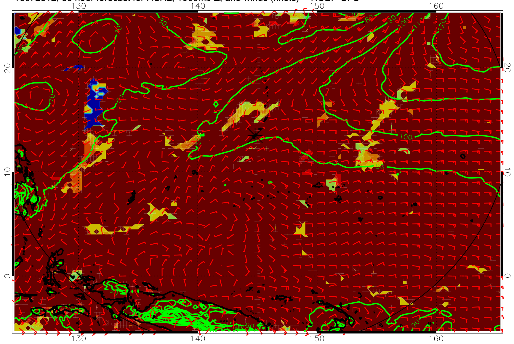
16072312, 36 hour forecast for HCAL, 1000mb Z, and winds (knots) -- NCEP GFS
