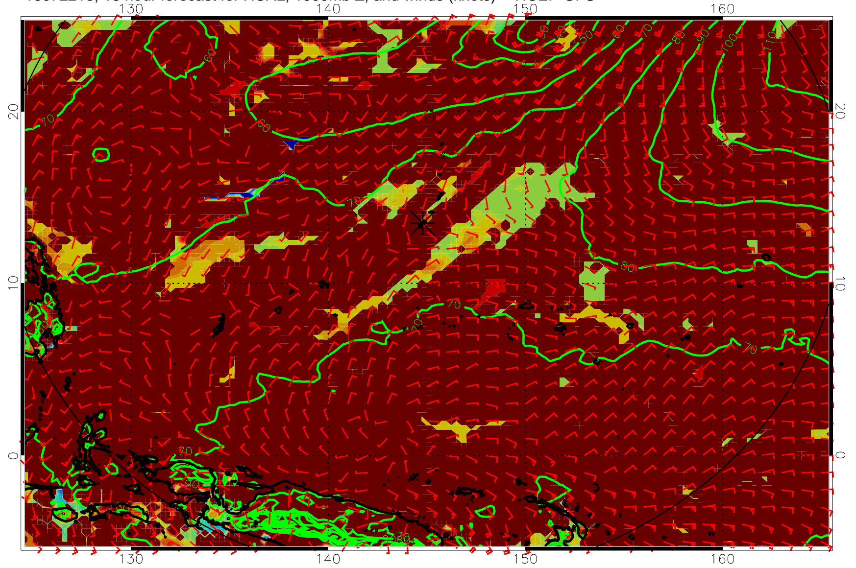
16072218, 18 hour forecast for HCAL, 1000mb Z, and winds (knots) -- NCEP GFS
