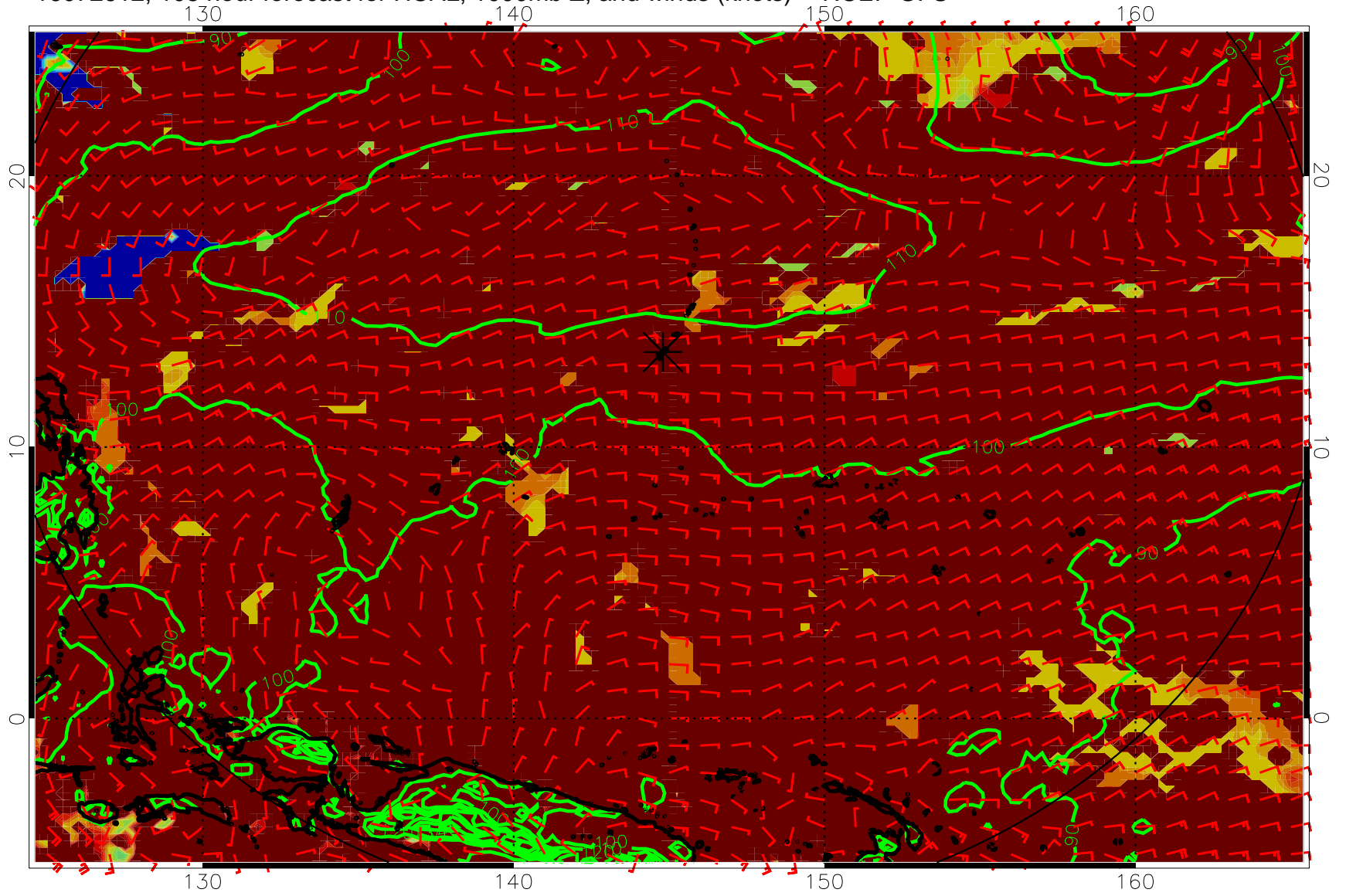
16072612, 108 hour forecast for HCAL, 1000mb Z, and winds (knots) -- NCEP GFS
