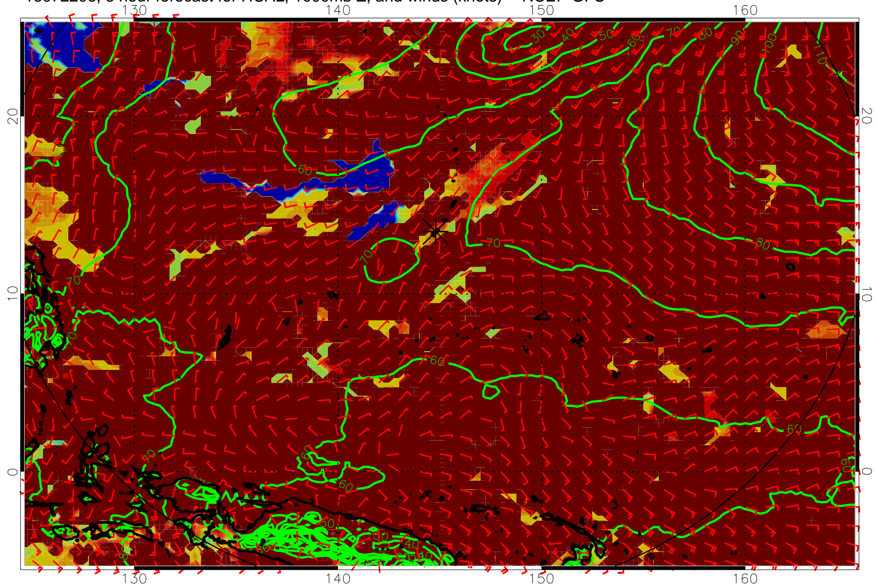
16072206, 6 hour forecast for HCAL, 1000mb Z, and winds (knots) -- NCEP GFS
