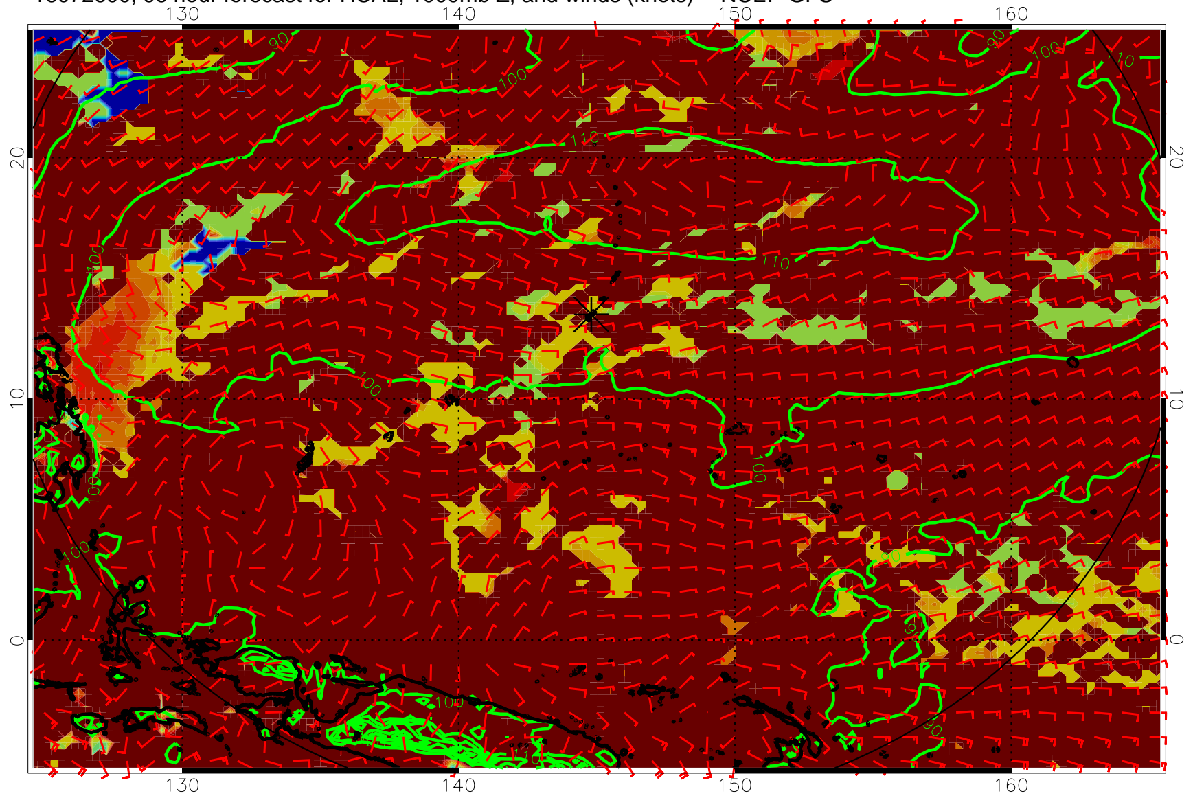
16072600, 96 hour forecast for HCAL, 1000mb Z, and winds (knots) -- NCEP GFS
