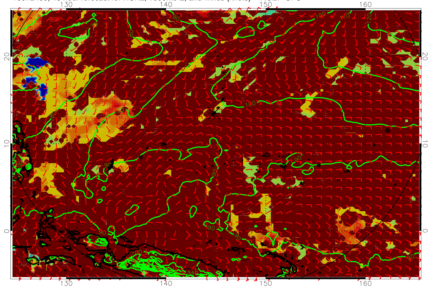
16072400, 48 hour forecast for HCAL, 1000mb Z, and winds (knots) -- NCEP GFS
