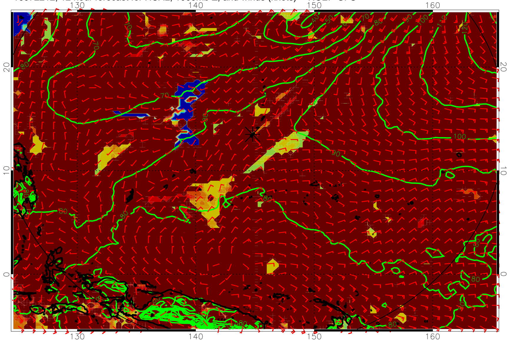
16072212, 12 hour forecast for HCAL, 1000mb Z, and winds (knots) -- NCEP GFS
