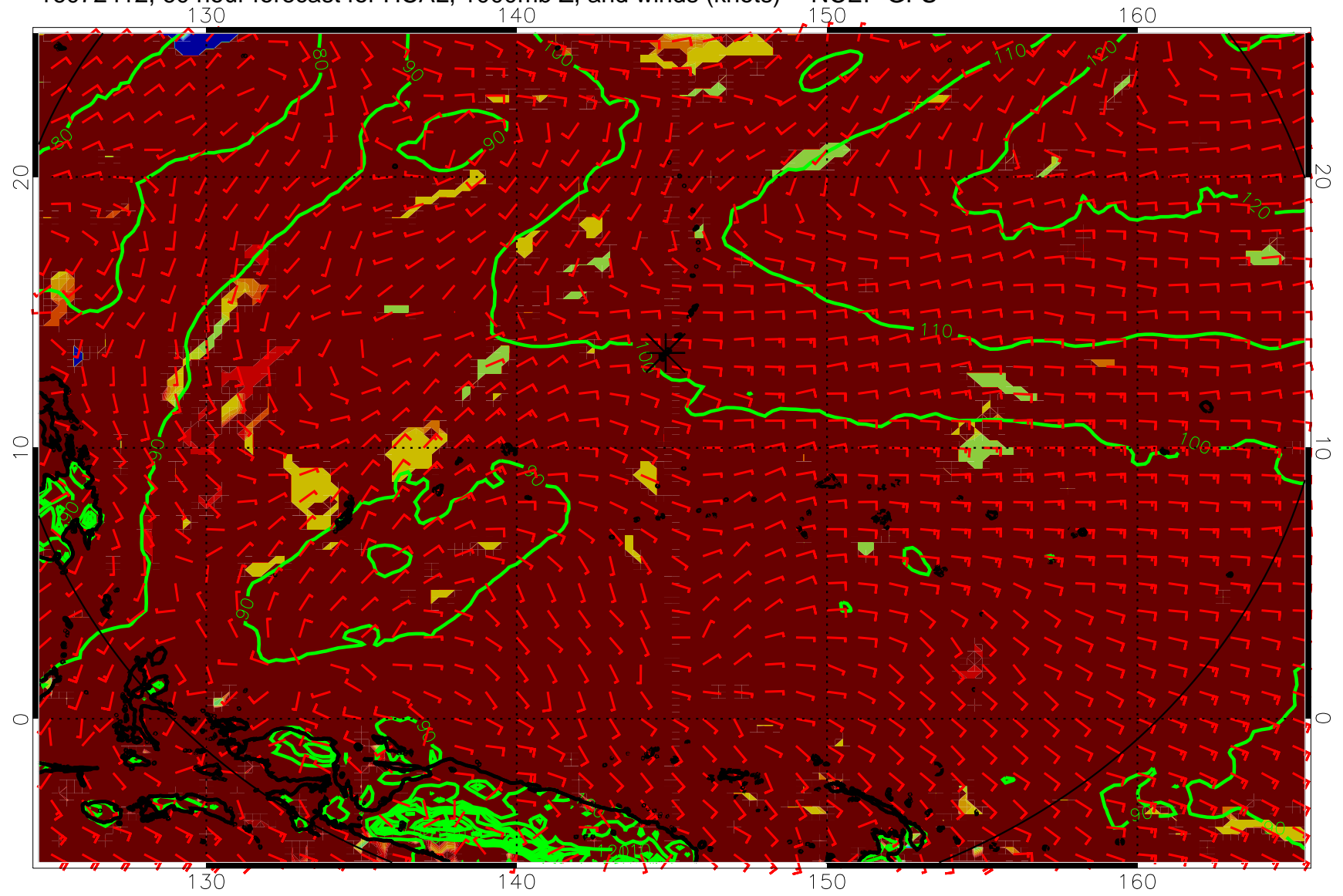
16072412, 60 hour forecast for HCAL, 1000mb Z, and winds (knots) -- NCEP GFS
