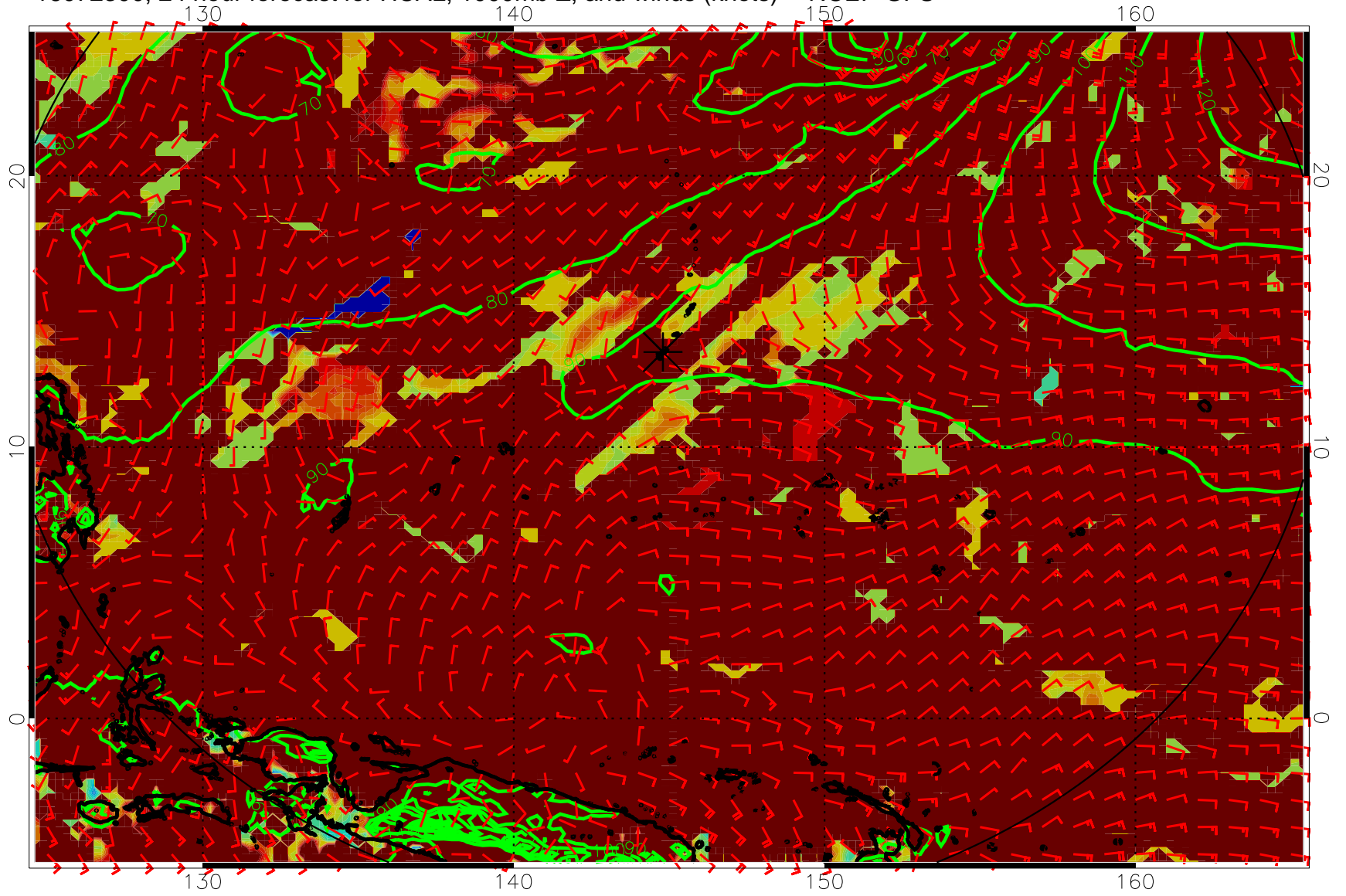
16072300, 24 hour forecast for HCAL, 1000mb Z, and winds (knots) -- NCEP GFS
