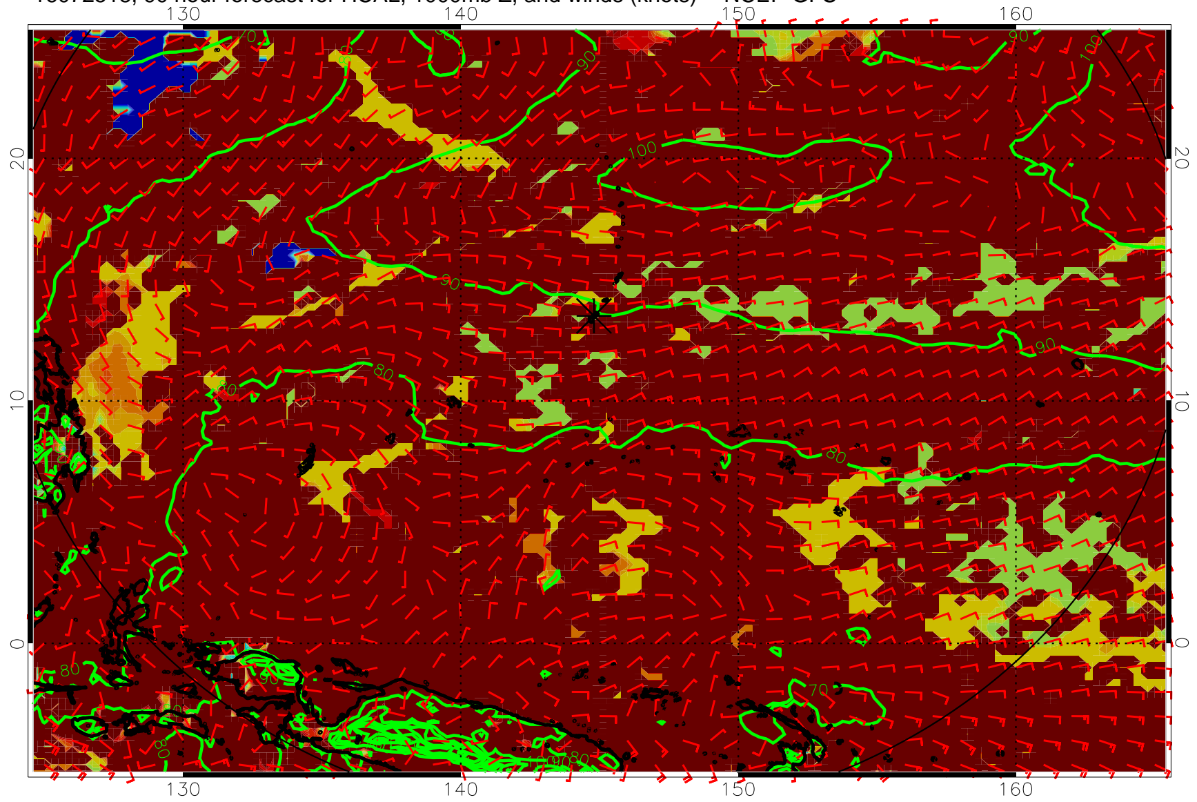
16072518, 90 hour forecast for HCAL, 1000mb Z, and winds (knots) -- NCEP GFS
