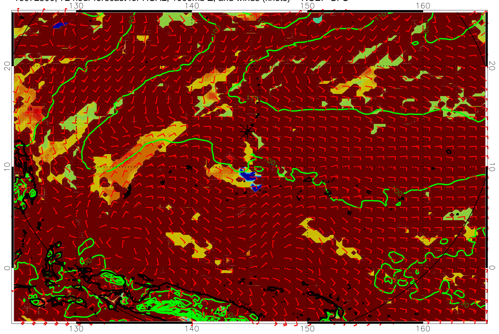
16072500, 72 hour forecast for HCAL, 1000mb Z, and winds (knots) -- NCEP GFS
