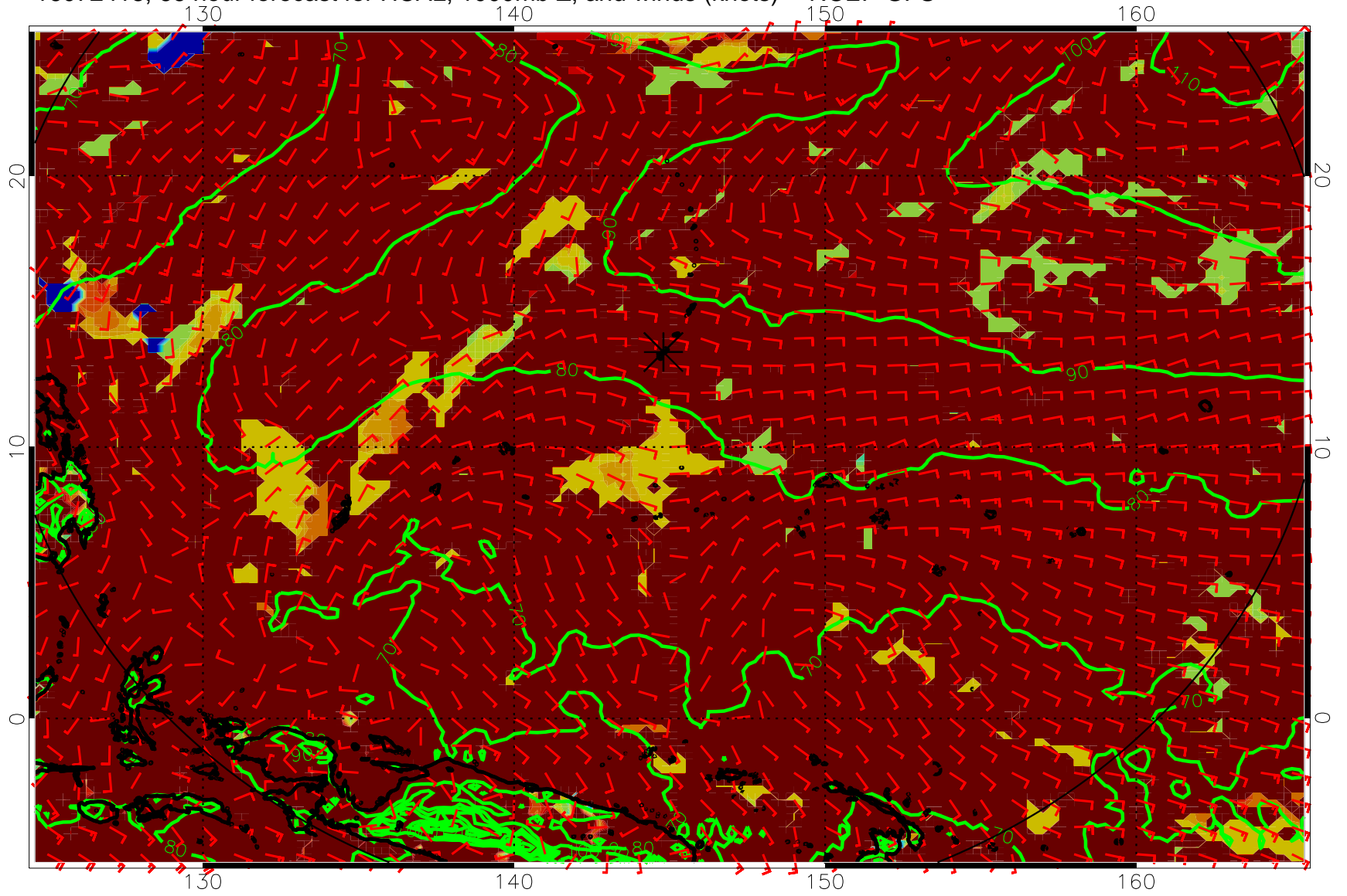
16072418, 66 hour forecast for HCAL, 1000mb Z, and winds (knots) -- NCEP GFS
