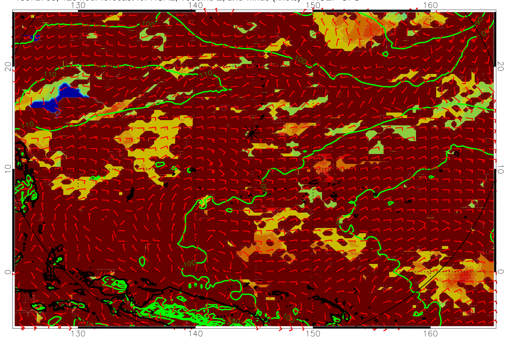
16072700, 120 hour forecast for HCAL, 1000mb Z, and winds (knots) -- NCEP GFS
