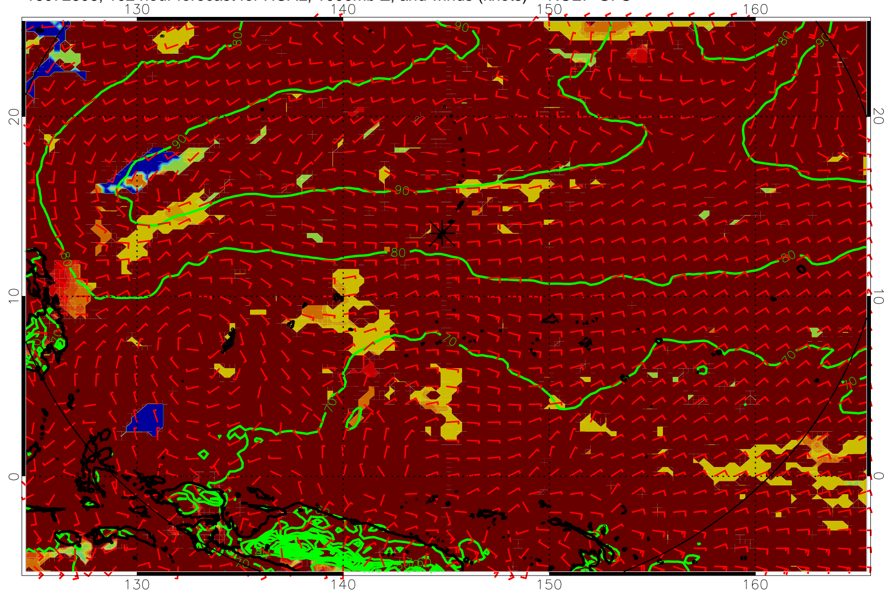
16072606, 102 hour forecast for HCAL, 1000mb Z, and winds (knots) -- NCEP GFS
