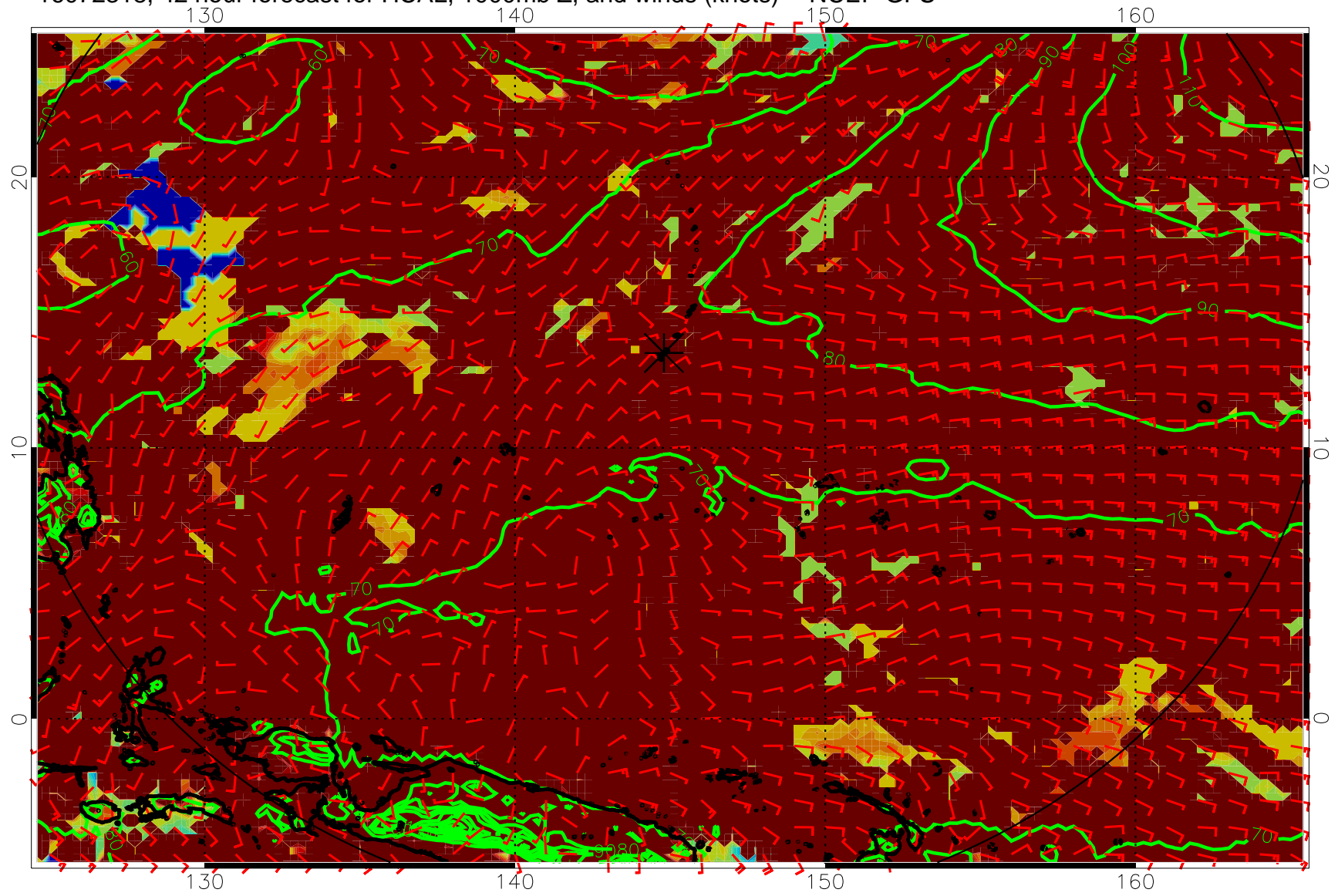
16072318, 42 hour forecast for HCAL, 1000mb Z, and winds (knots) -- NCEP GFS
