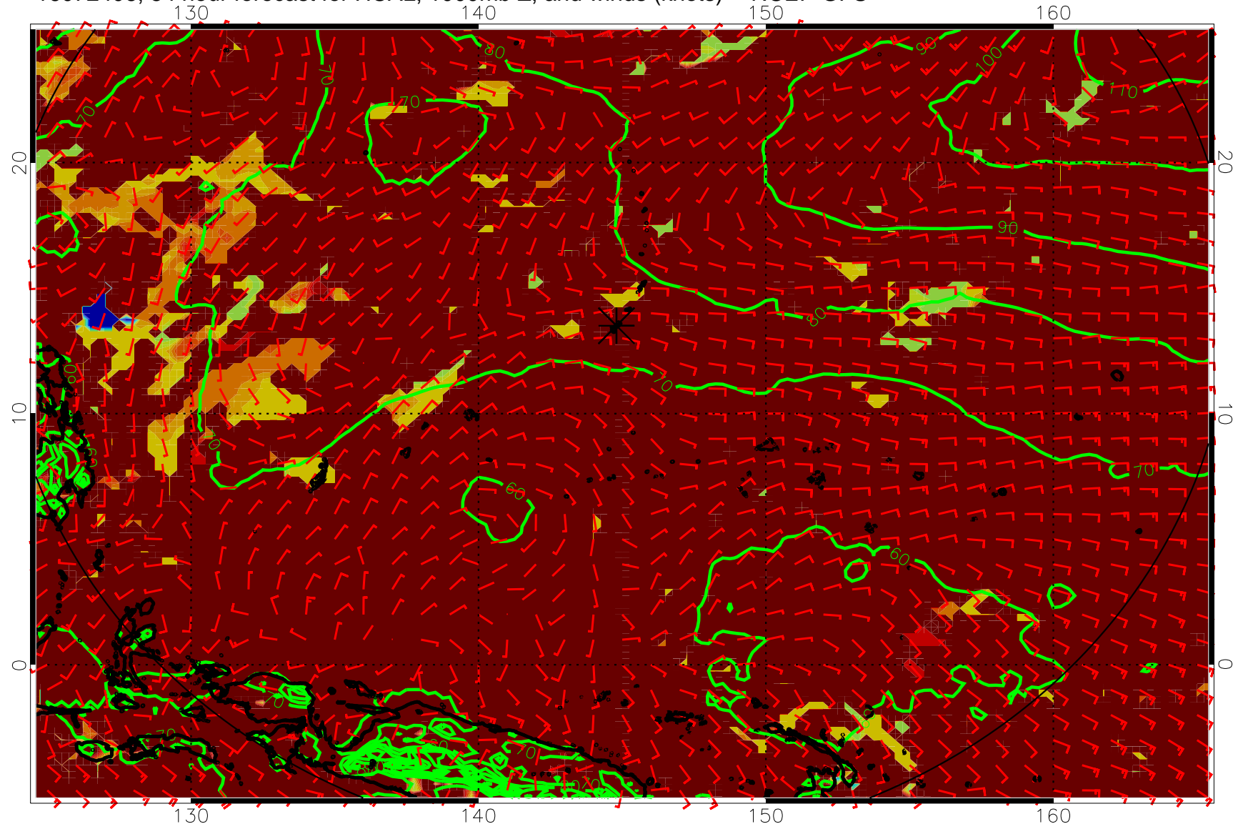
16072406, 54 hour forecast for HCAL, 1000mb Z, and winds (knots) -- NCEP GFS
