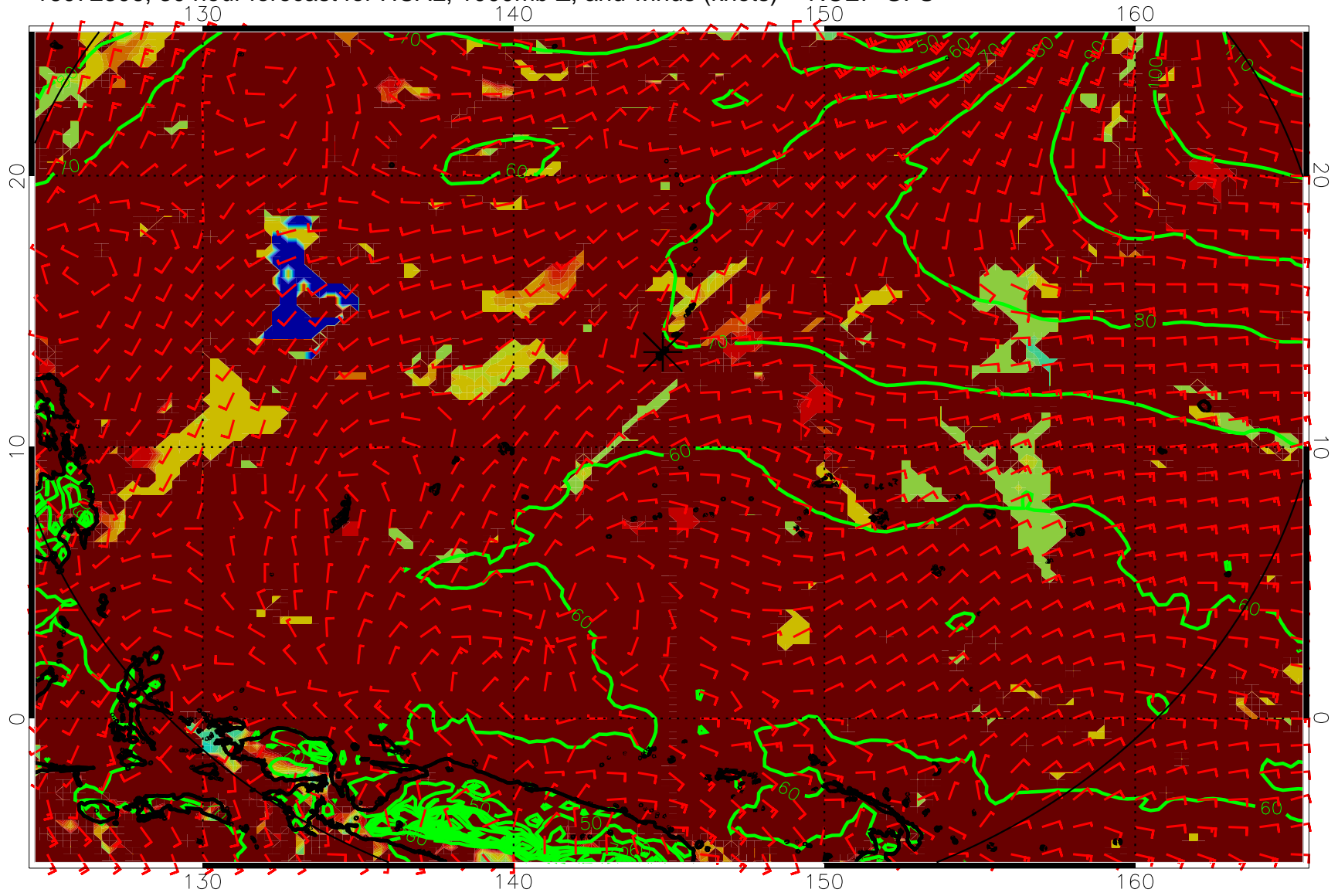
16072306, 30 hour forecast for HCAL, 1000mb Z, and winds (knots) -- NCEP GFS
