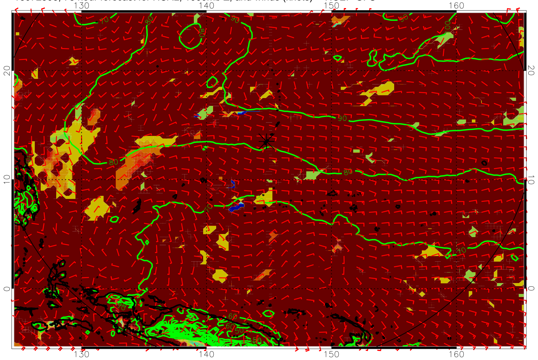
16072506, 78 hour forecast for HCAL, 1000mb Z, and winds (knots) -- NCEP GFS
