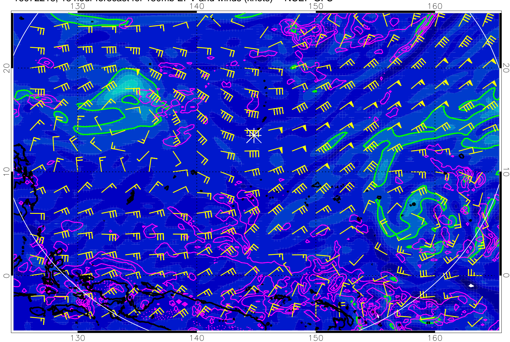
16072218, 18 hour forecast for 150mb EPV and winds (knots) -- NCEP GFS
