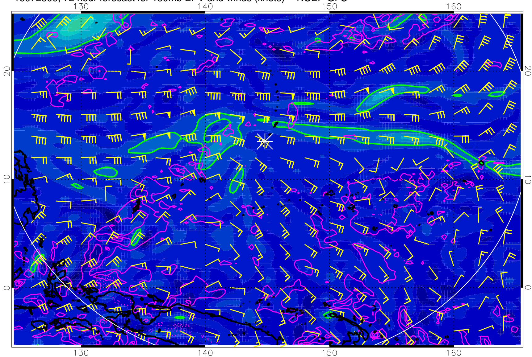
16072500, 72 hour forecast for 150mb EPV and winds (knots) -- NCEP GFS
