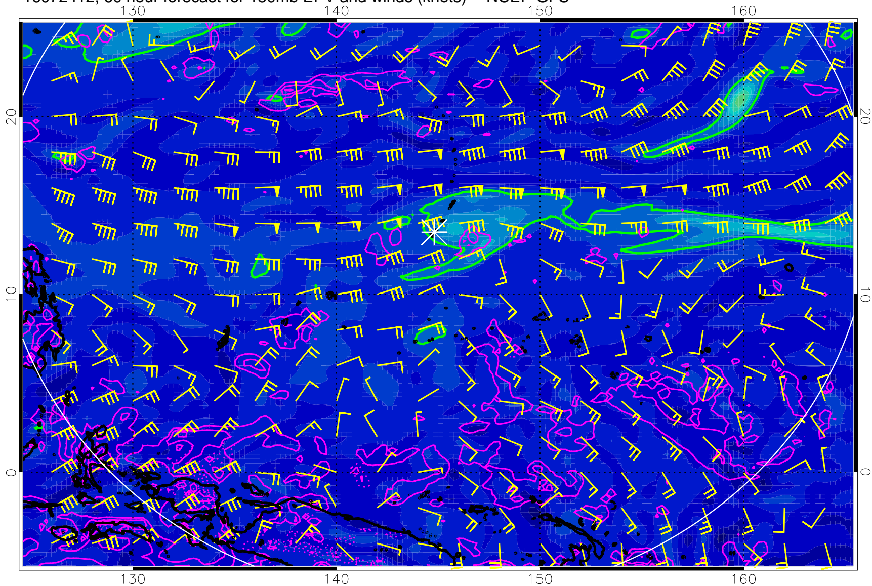
16072412, 60 hour forecast for 150mb EPV and winds (knots) -- NCEP GFS
