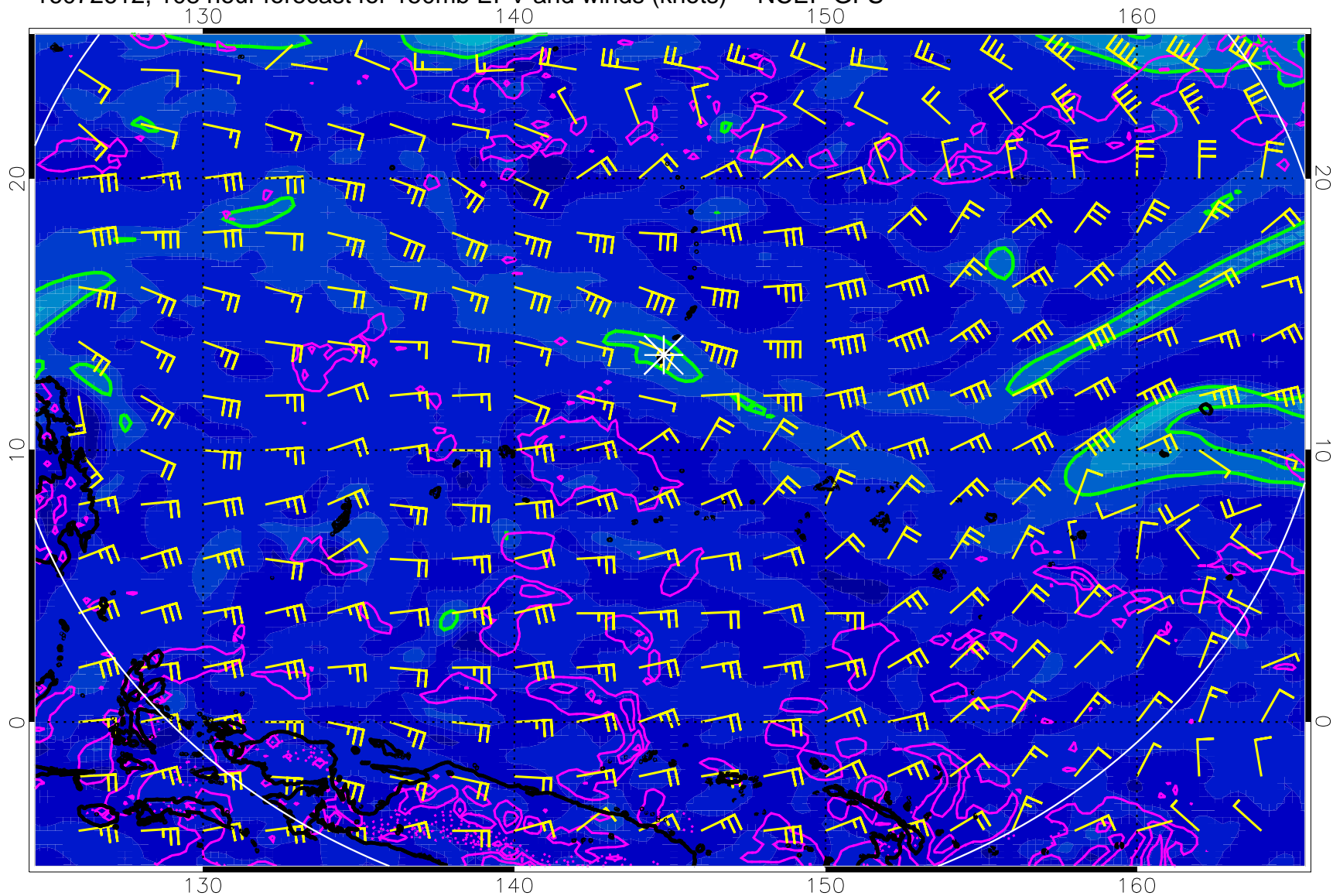
16072612, 108 hour forecast for 150mb EPV and winds (knots) -- NCEP GFS
