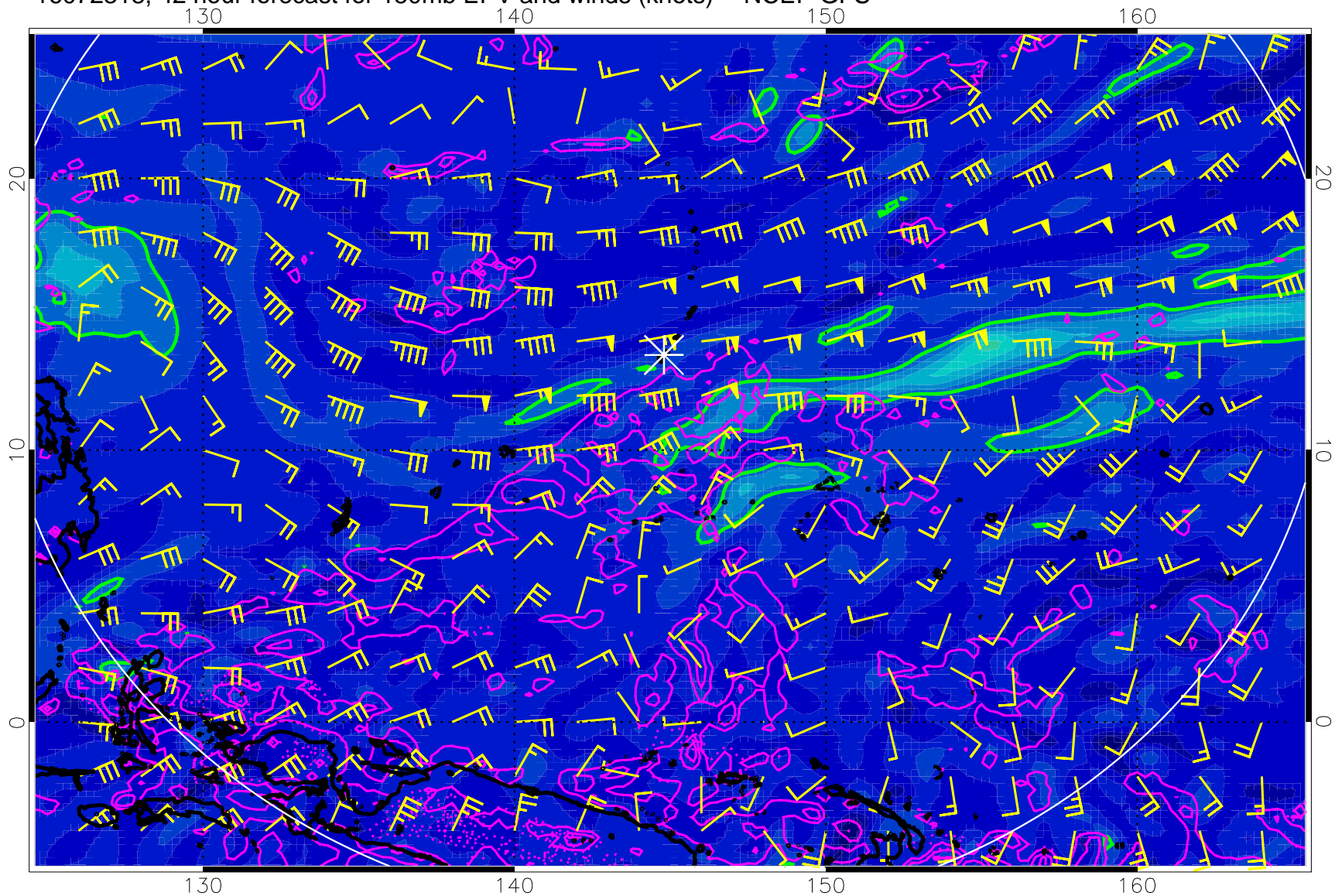
16072318, 42 hour forecast for 150mb EPV and winds (knots) -- NCEP GFS
