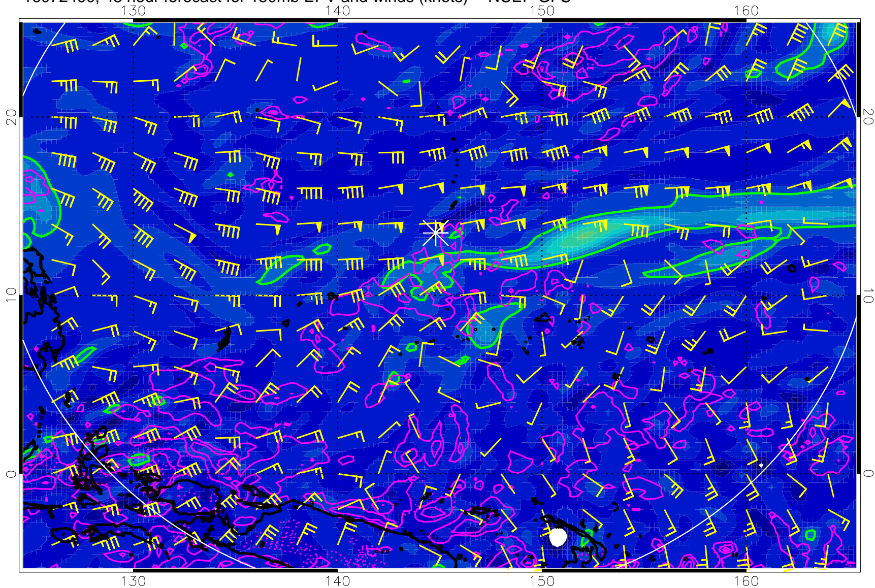
16072400, 48 hour forecast for 150mb EPV and winds (knots) -- NCEP GFS
