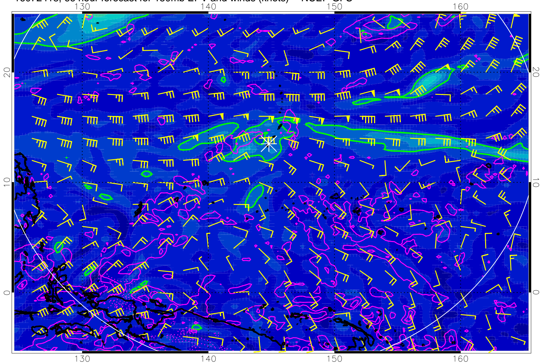
16072418, 66 hour forecast for 150mb EPV and winds (knots) -- NCEP GFS
