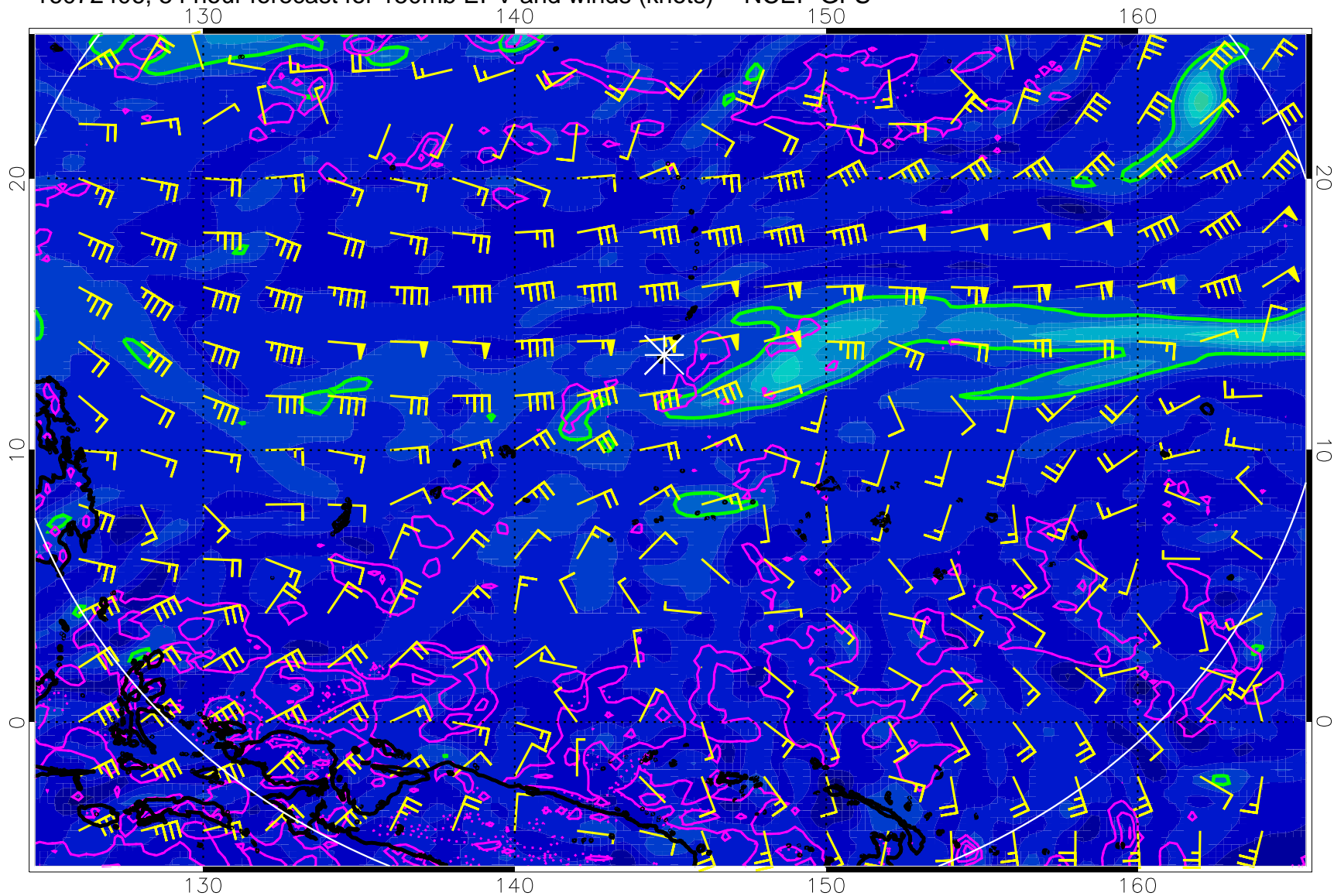
16072406, 54 hour forecast for 150mb EPV and winds (knots) -- NCEP GFS
