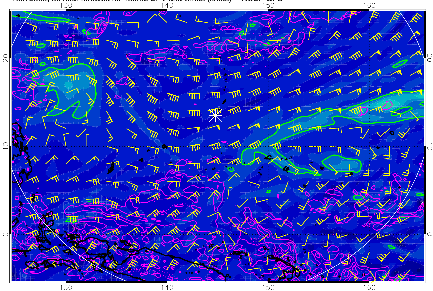
16072306, 30 hour forecast for 150mb EPV and winds (knots) -- NCEP GFS
