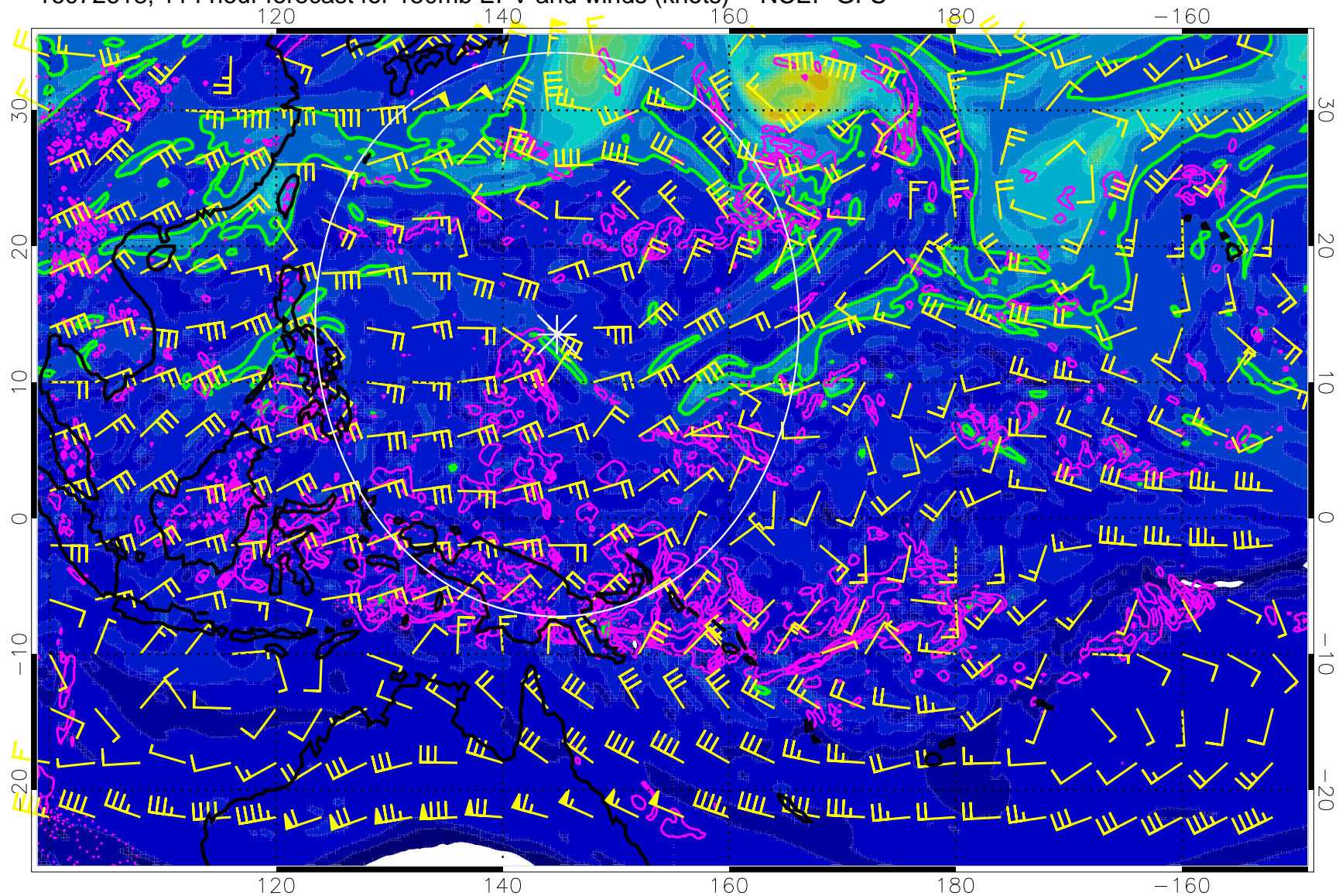
16072618, 114 hour forecast for 150mb EPV and winds (knots) -- NCEP GFS
