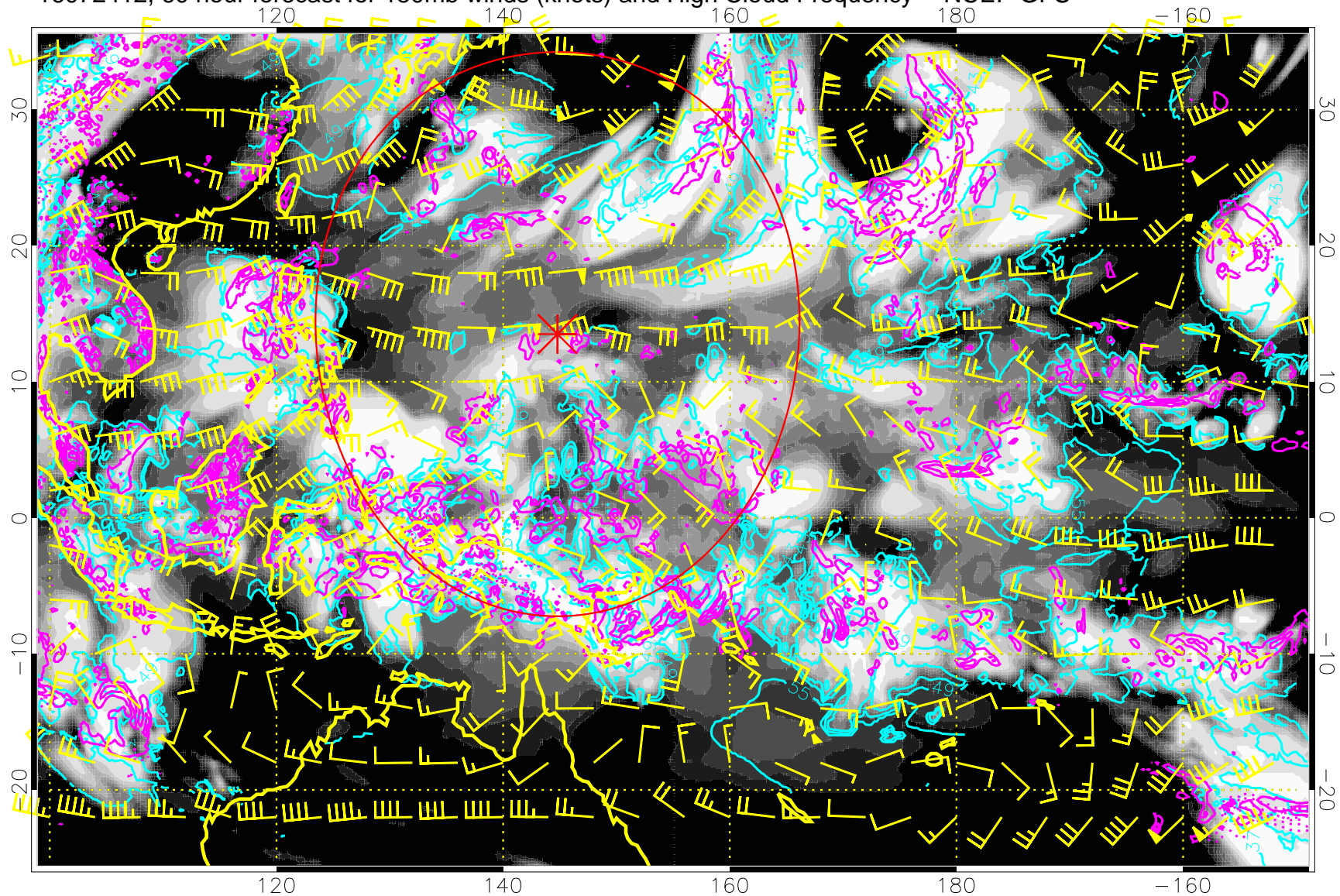
16072412, 60 hour forecast for 150mb winds (knots) and High Cloud Frequency -- NCEP GFS
