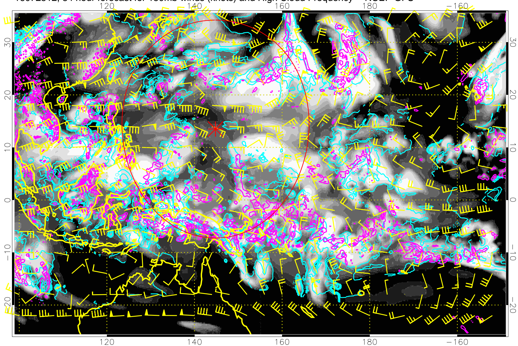
16072512, 84 hour forecast for 150mb winds (knots) and High Cloud Frequency -- NCEP GFS
