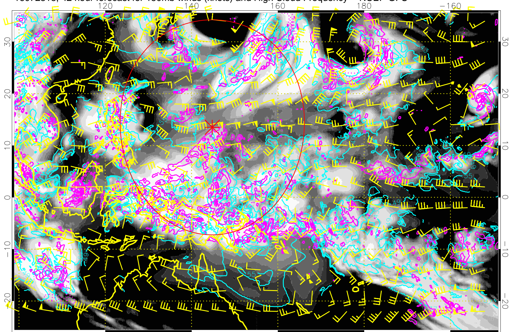
16072318, 42 hour forecast for 150mb winds (knots) and High Cloud Frequency -- NCEP GFS
