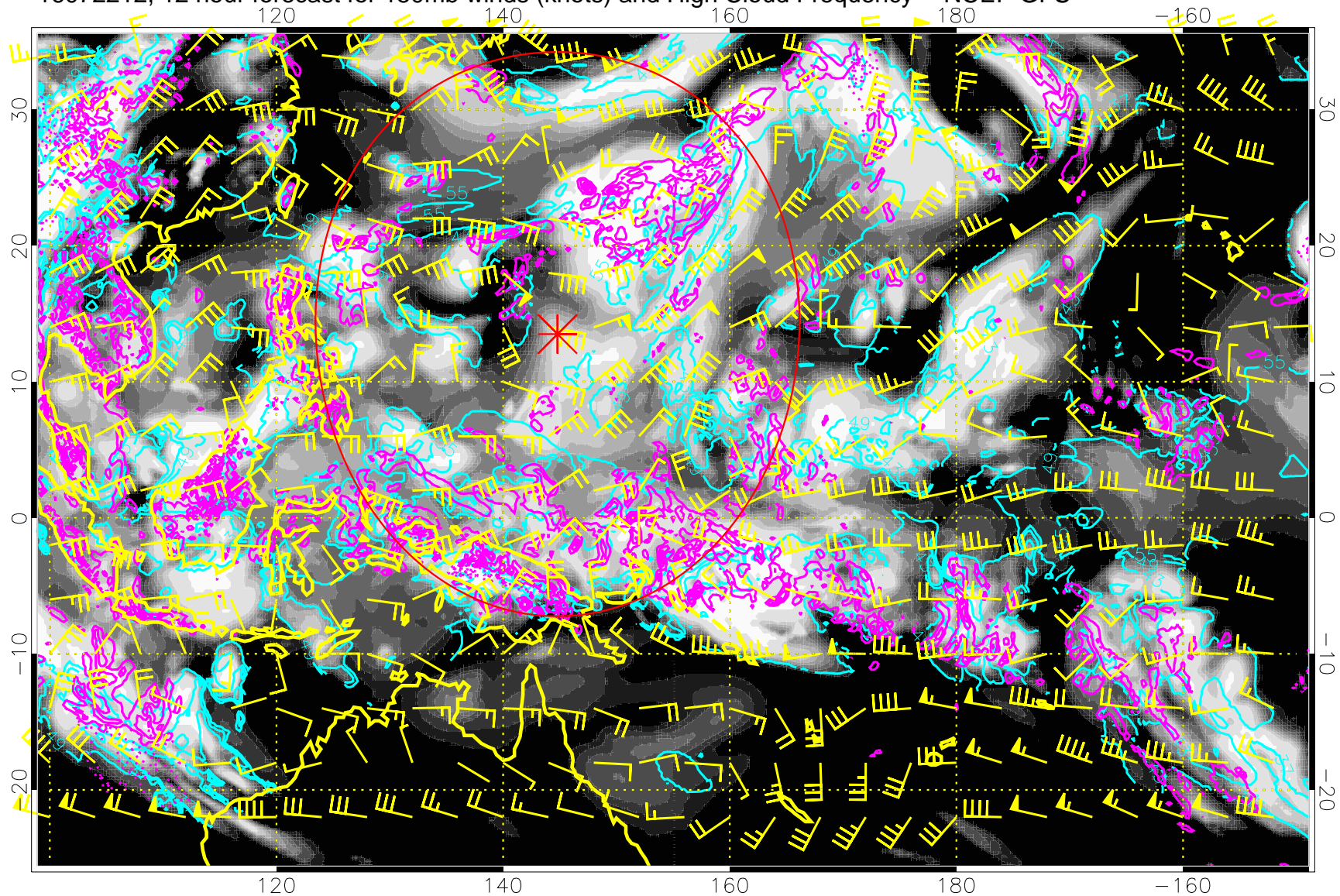
16072212, 12 hour forecast for 150mb winds (knots) and High Cloud Frequency -- NCEP GFS
