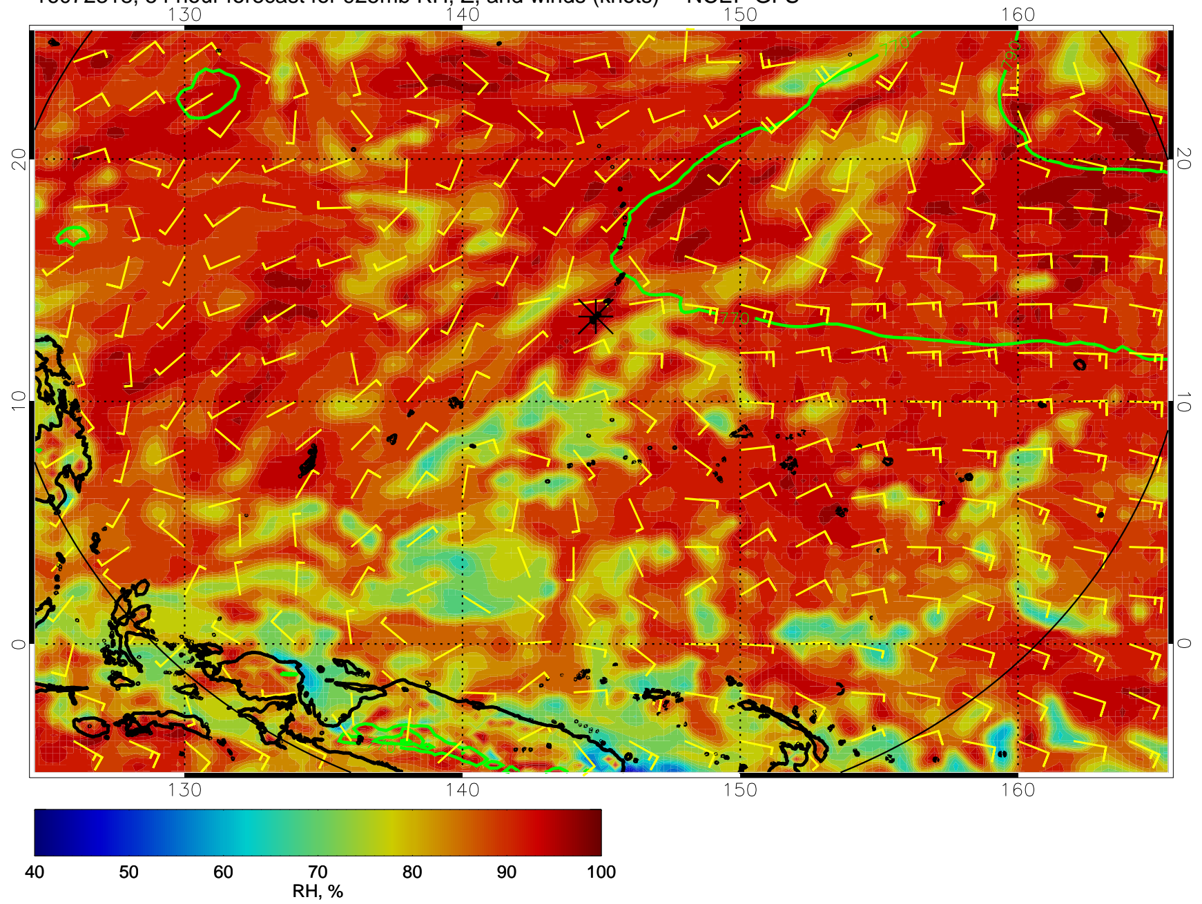
16072318, 54 hour forecast for 925mb RH, Z, and winds (knots) -- NCEP GFS
