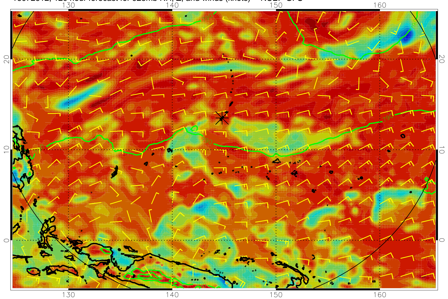
16072612, 120 hour forecast for 925mb RH, Z, and winds (knots) -- NCEP GFS
