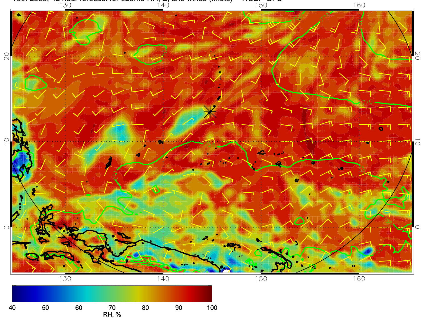
16072306, 42 hour forecast for 925mb RH, Z, and winds (knots) -- NCEP GFS
