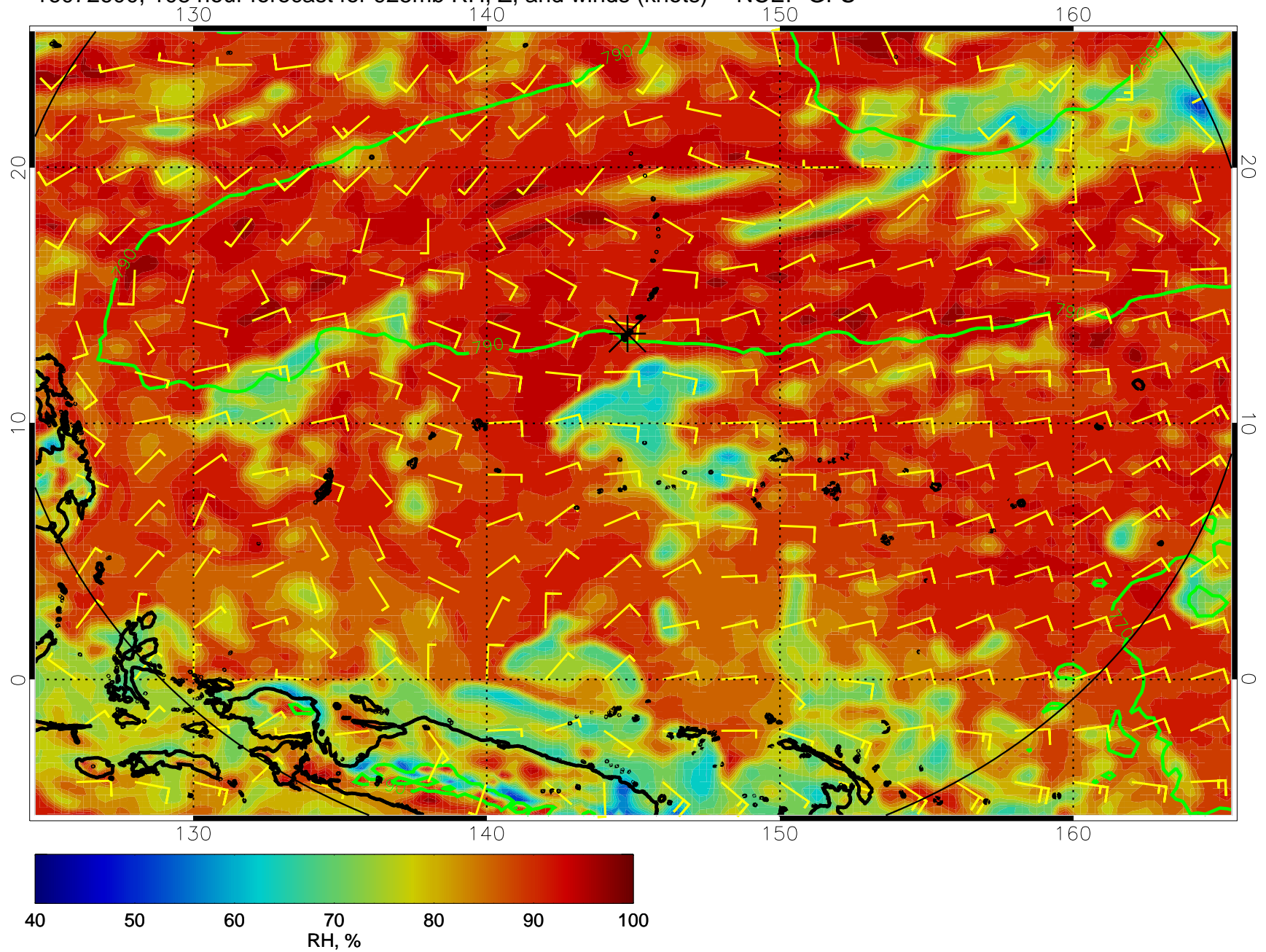
16072600, 108 hour forecast for 925mb RH, Z, and winds (knots) -- NCEP GFS
