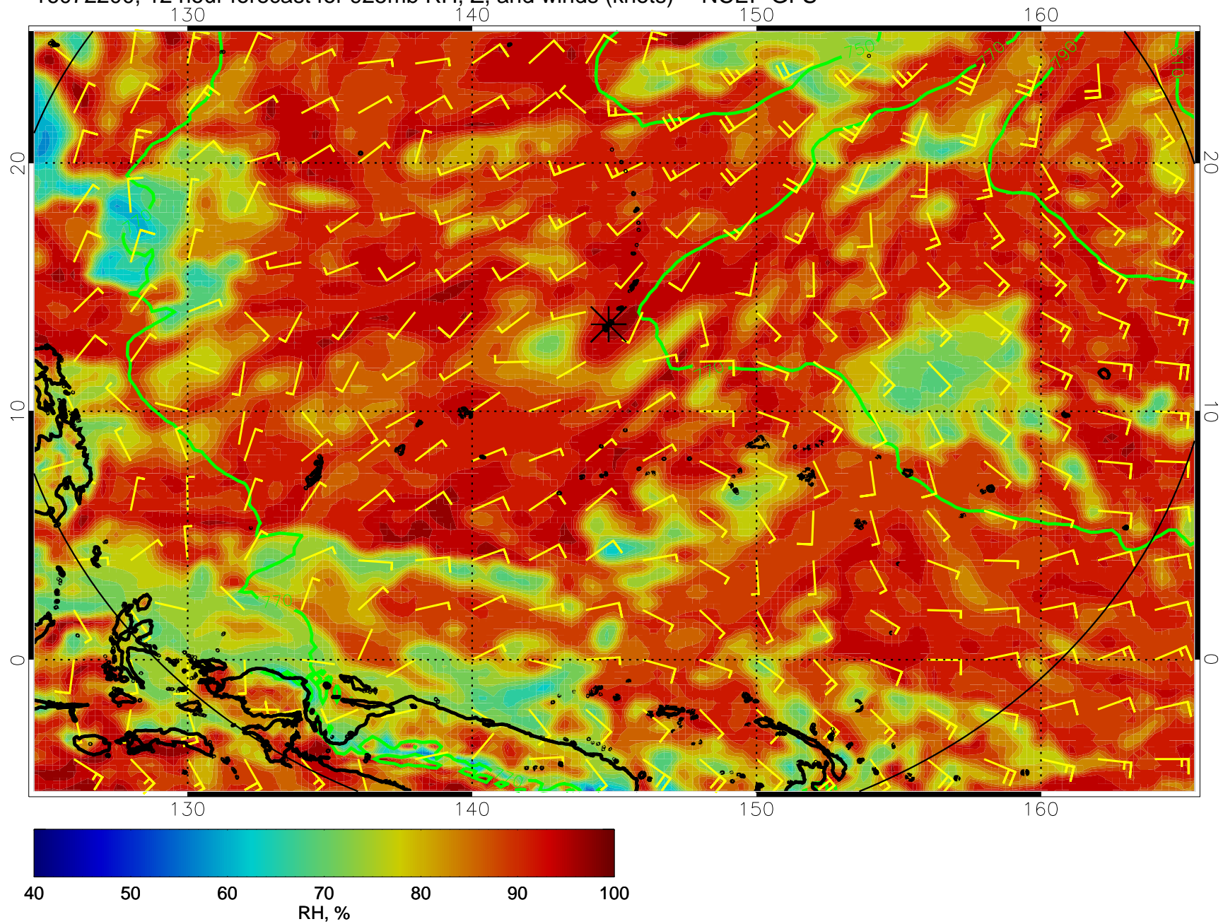
16072200, 12 hour forecast for 925mb RH, Z, and winds (knots) -- NCEP GFS
