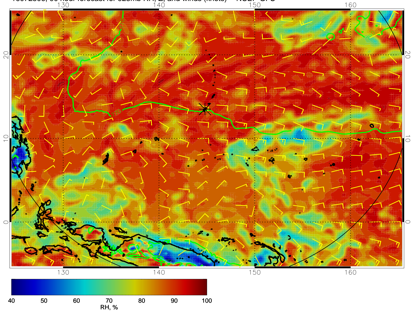
16072506, 90 hour forecast for 925mb RH, Z, and winds (knots) -- NCEP GFS
