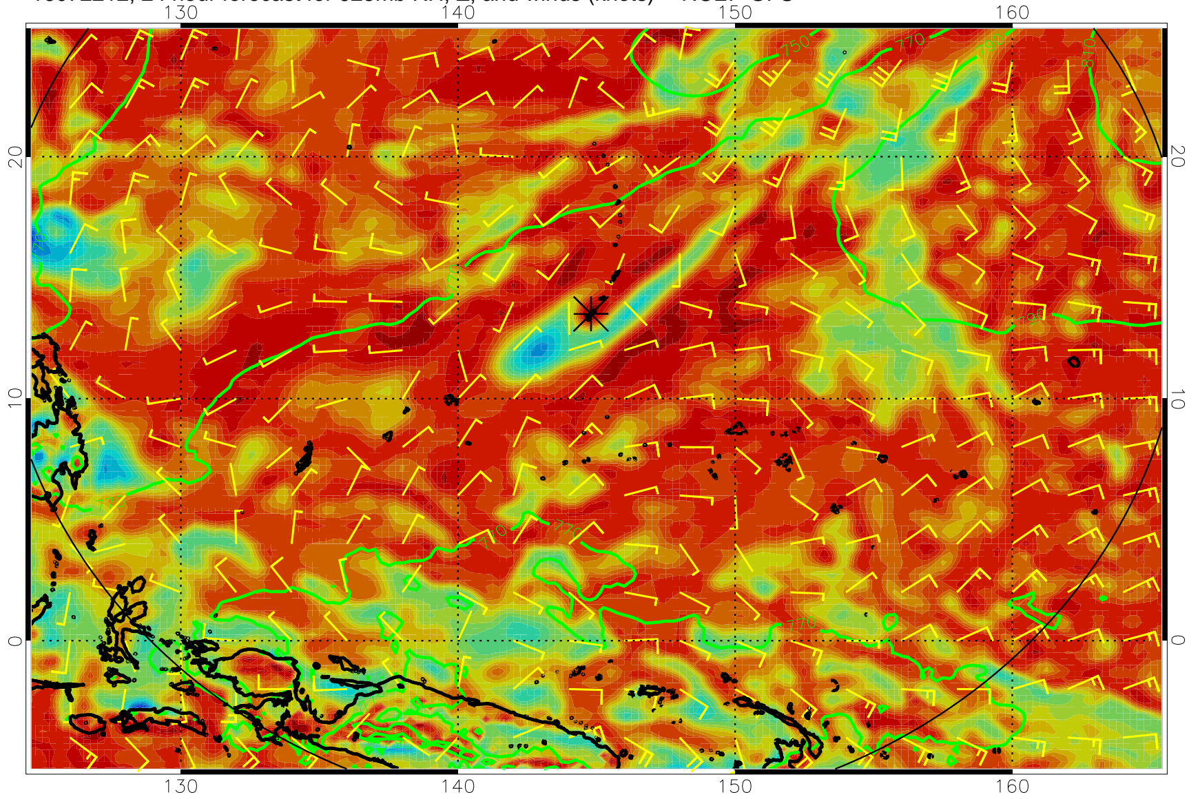
16072212, 24 hour forecast for 925mb RH, Z, and winds (knots) -- NCEP GFS
