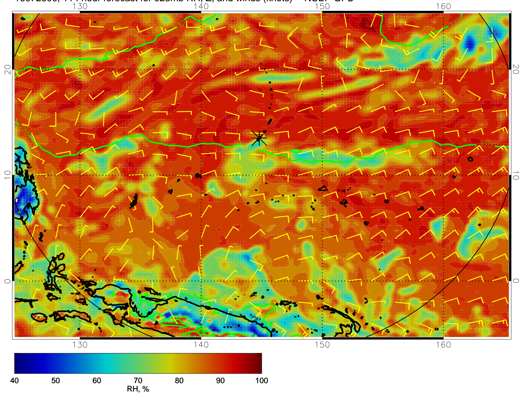
16072606, 114 hour forecast for 925mb RH, Z, and winds (knots) -- NCEP GFS
