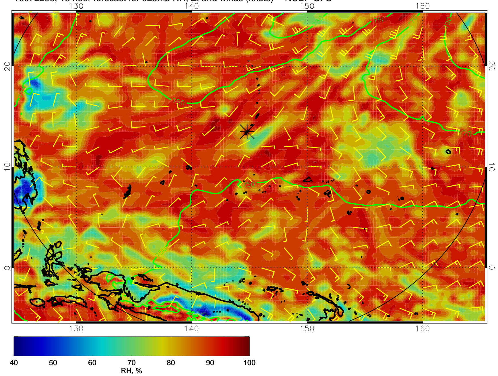
16072206, 18 hour forecast for 925mb RH, Z, and winds (knots) -- NCEP GFS
