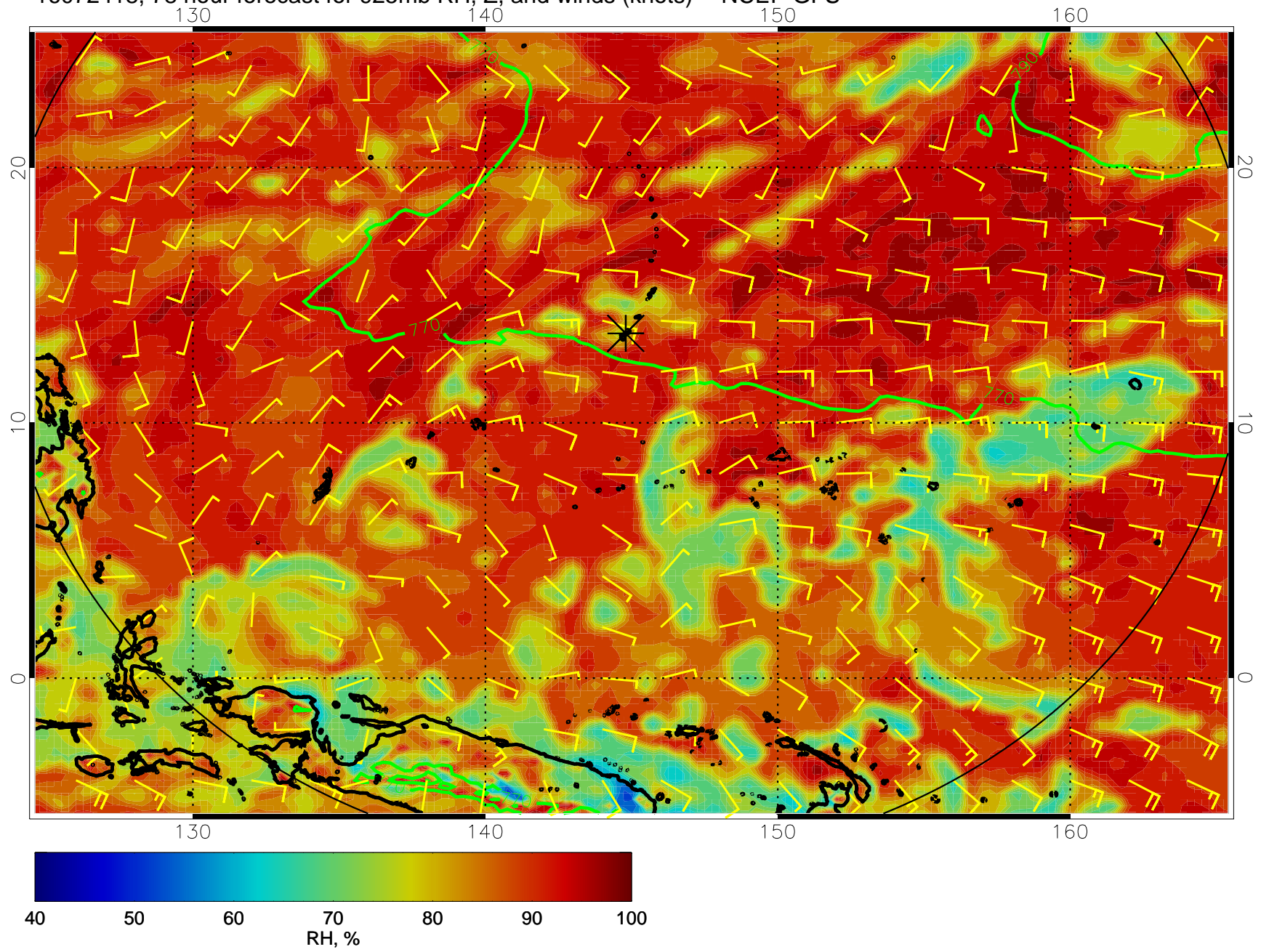
16072418, 78 hour forecast for 925mb RH, Z, and winds (knots) -- NCEP GFS
