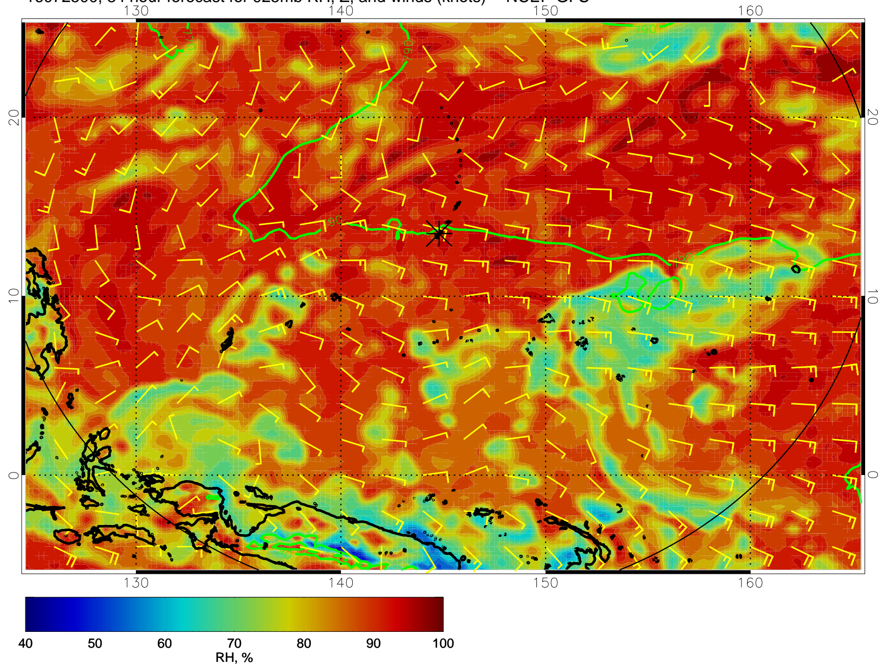
16072500, 84 hour forecast for 925mb RH, Z, and winds (knots) -- NCEP GFS
