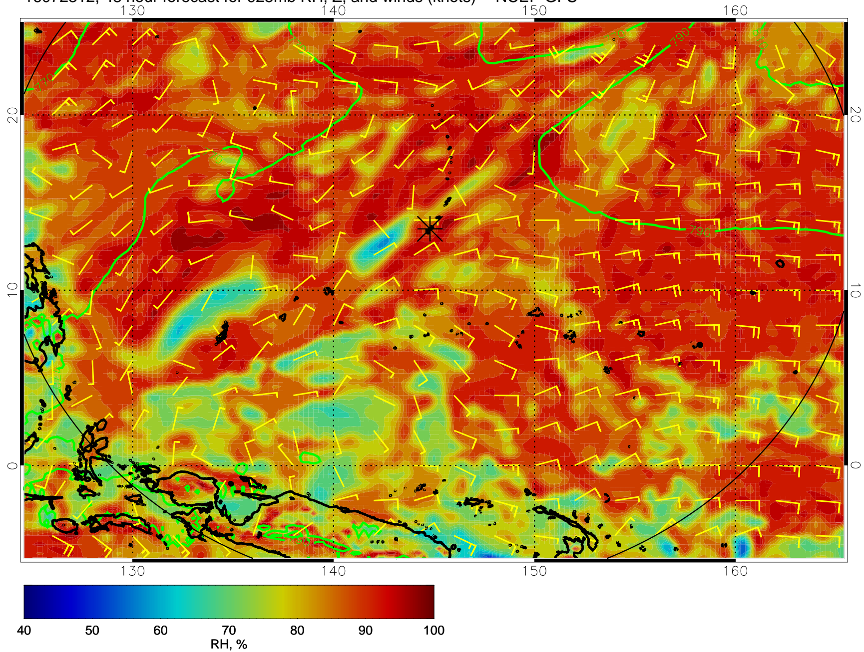
16072312, 48 hour forecast for 925mb RH, Z, and winds (knots) -- NCEP GFS
