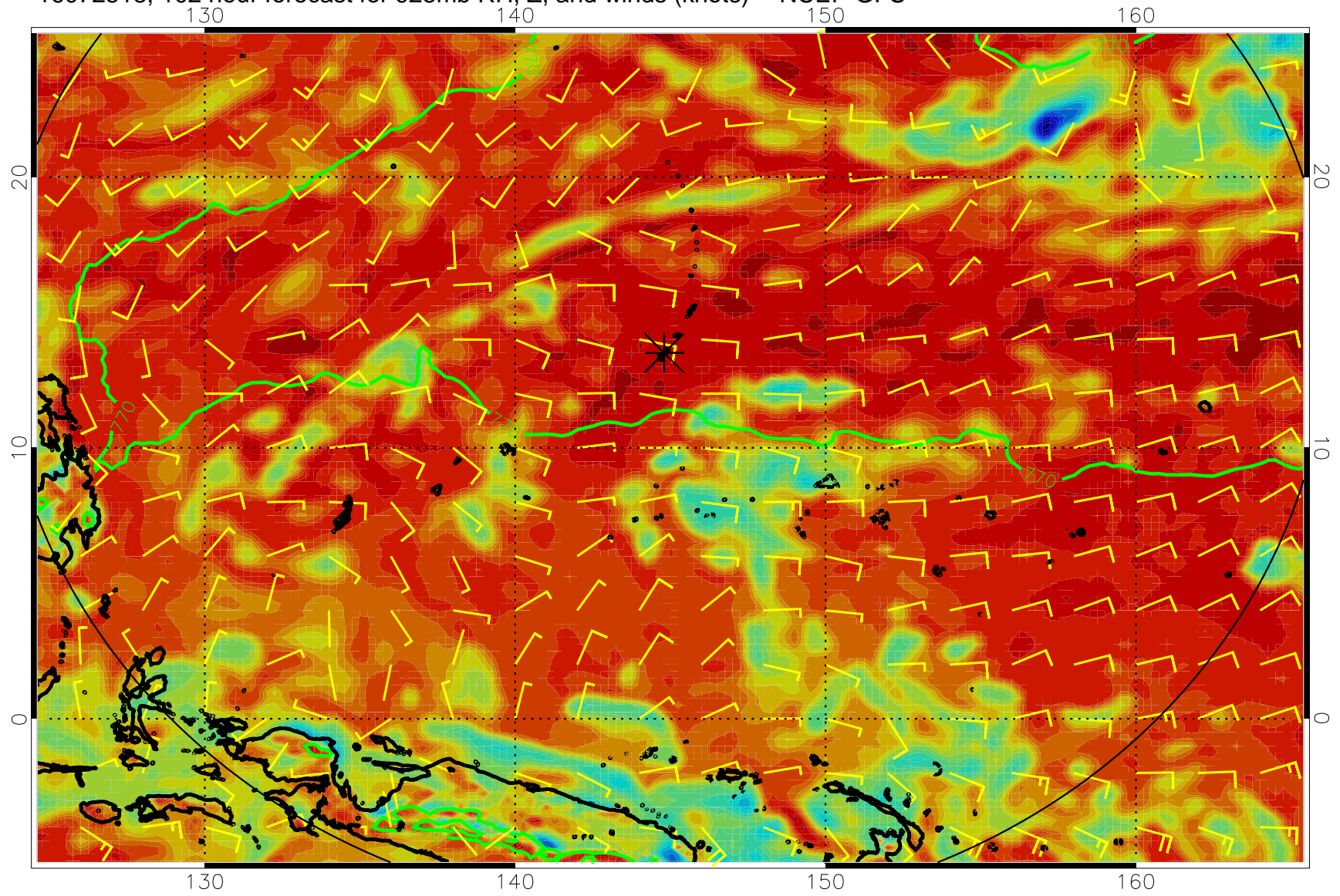
16072518, 102 hour forecast for 925mb RH, Z, and winds (knots) -- NCEP GFS
