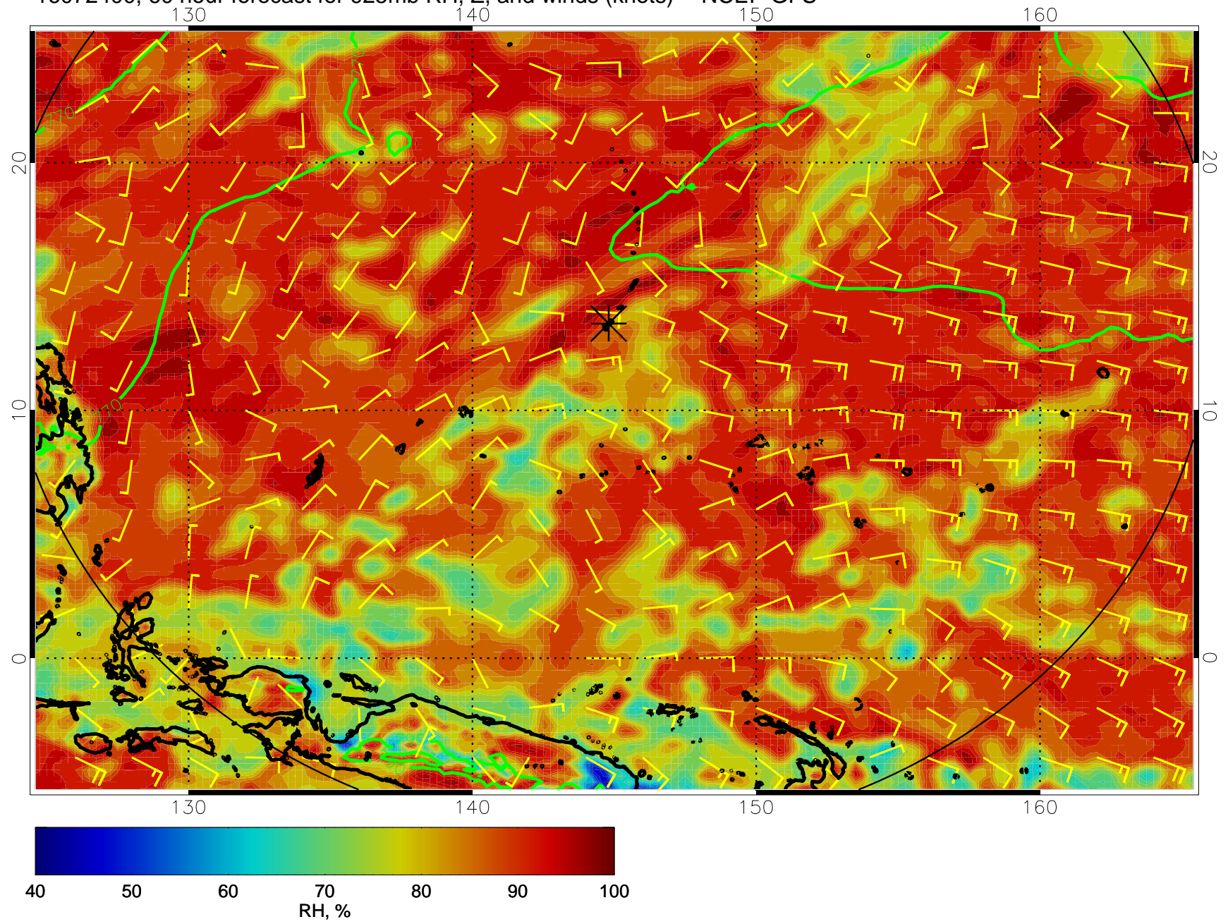
16072400, 60 hour forecast for 925mb RH, Z, and winds (knots) -- NCEP GFS
