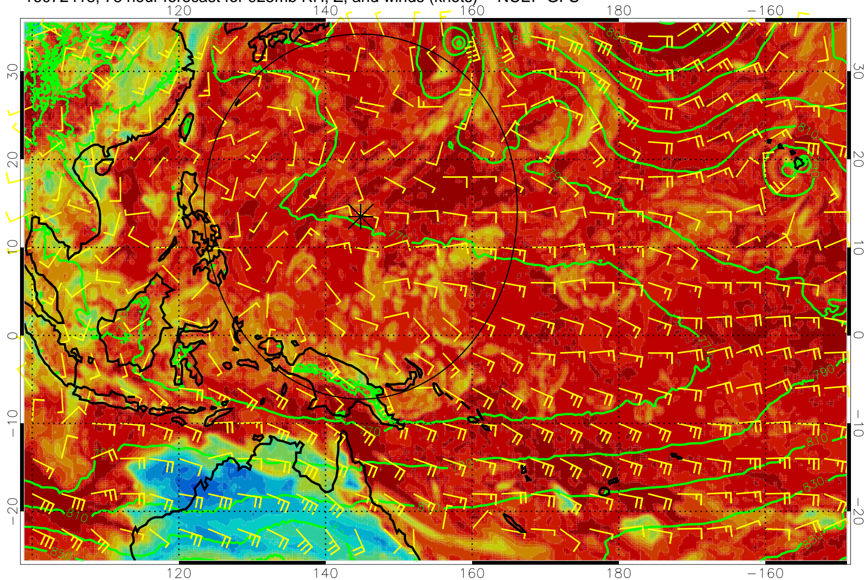
16072418, 78 hour forecast for 925mb RH, Z, and winds (knots) -- NCEP GFS
