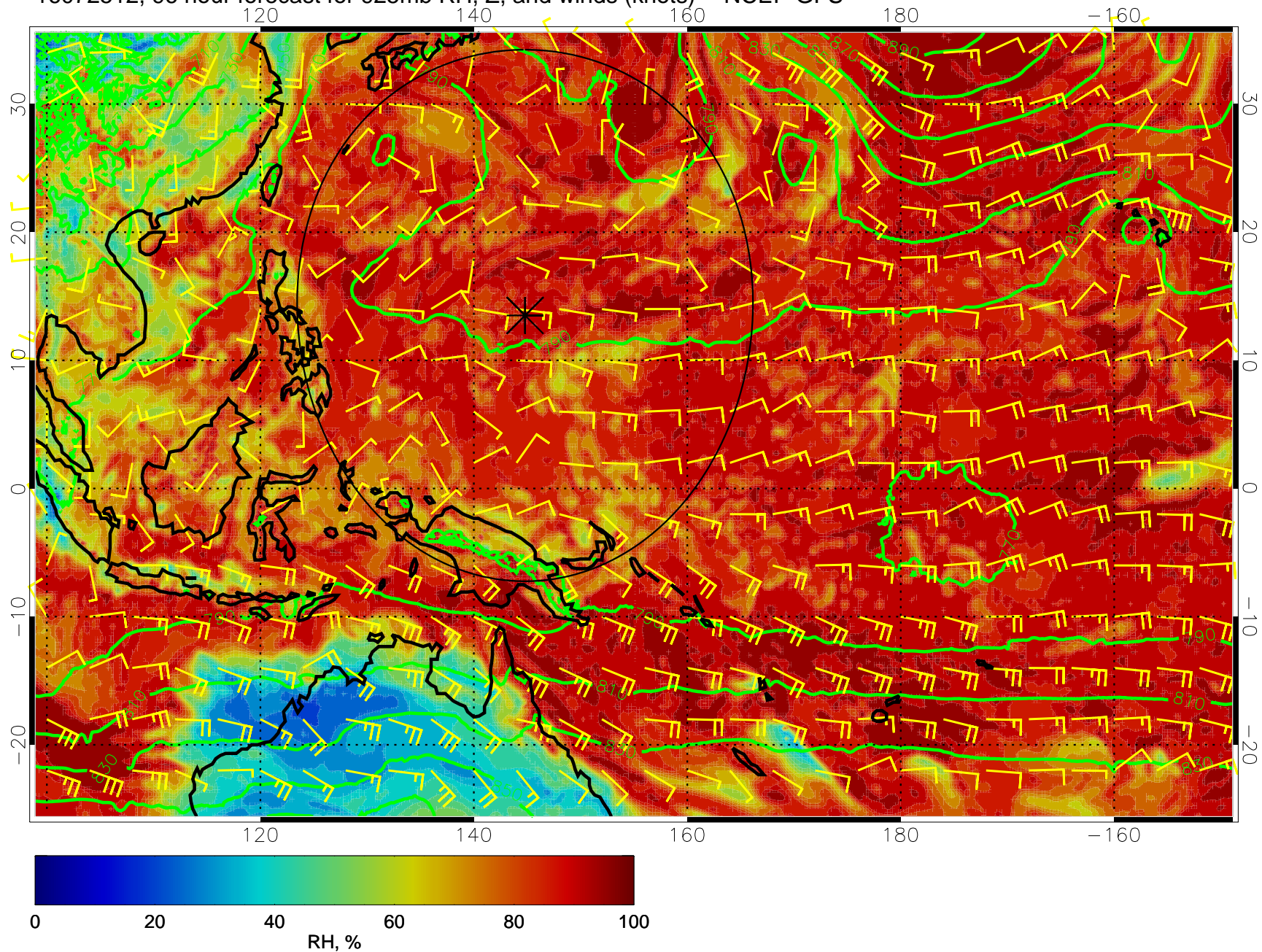
16072512, 96 hour forecast for 925mb RH, Z, and winds (knots) -- NCEP GFS
