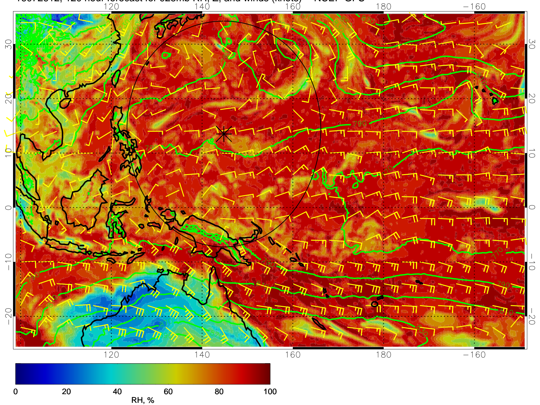
16072612, 120 hour forecast for 925mb RH, Z, and winds (knots) -- NCEP GFS
