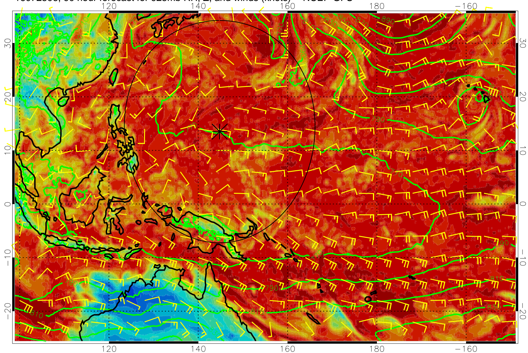
16072506, 90 hour forecast for 925mb RH, Z, and winds (knots) -- NCEP GFS
