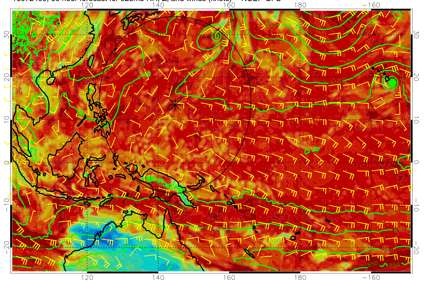
16072400, 60 hour forecast for 925mb RH, Z, and winds (knots) -- NCEP GFS
