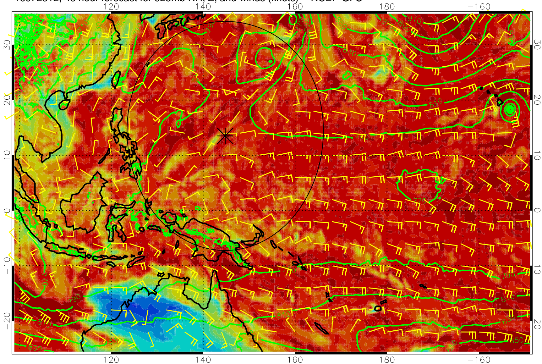
16072312, 48 hour forecast for 925mb RH, Z, and winds (knots) -- NCEP GFS
