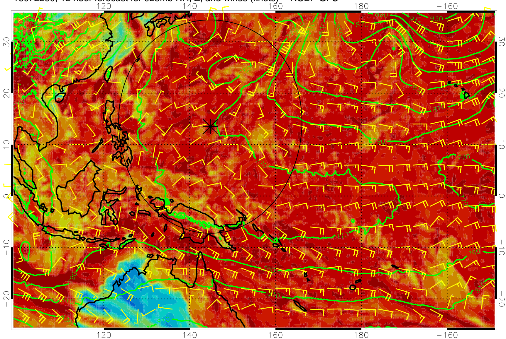
16072200, 12 hour forecast for 925mb RH, Z, and winds (knots) -- NCEP GFS
