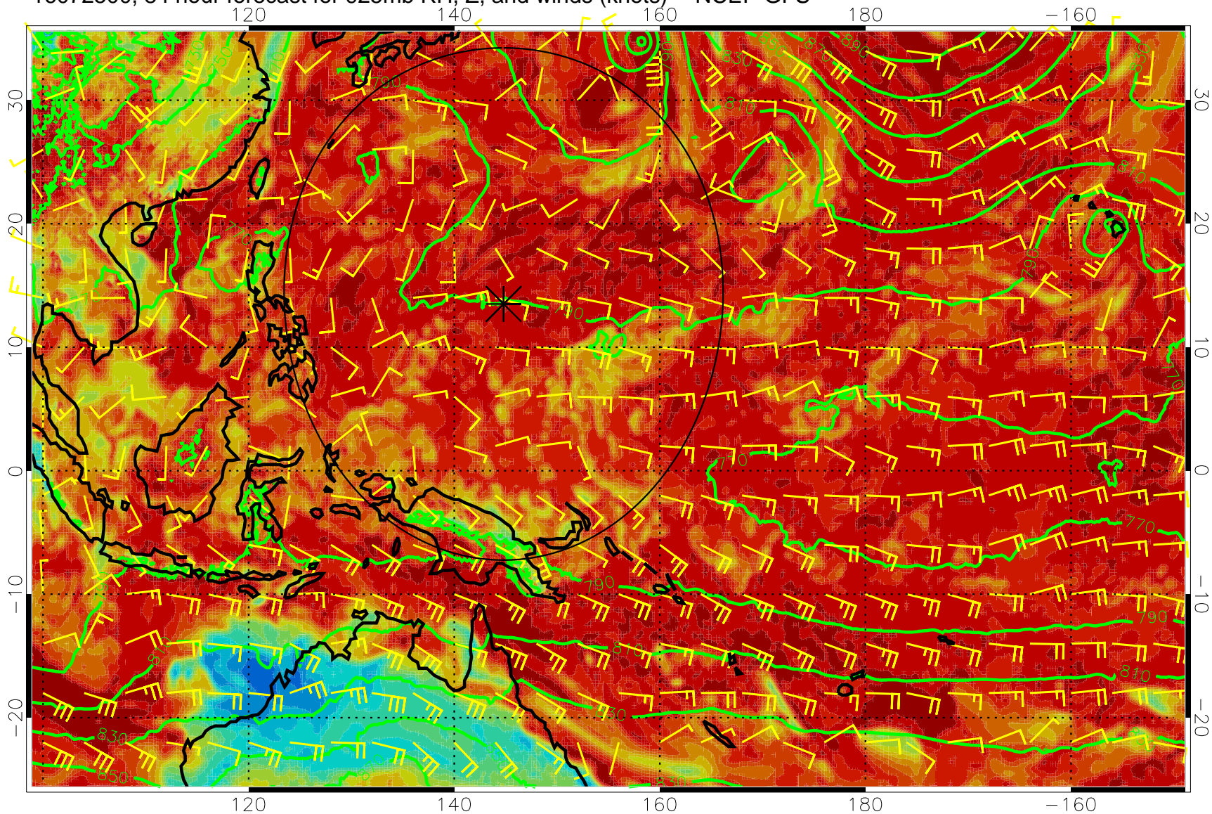
16072500, 84 hour forecast for 925mb RH, Z, and winds (knots) -- NCEP GFS
