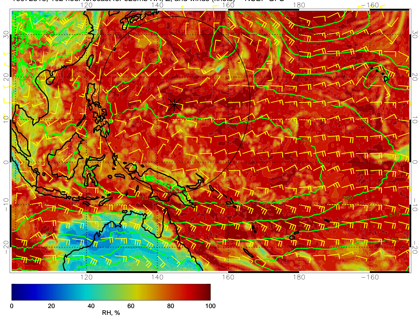
16072518, 102 hour forecast for 925mb RH, Z, and winds (knots) -- NCEP GFS
