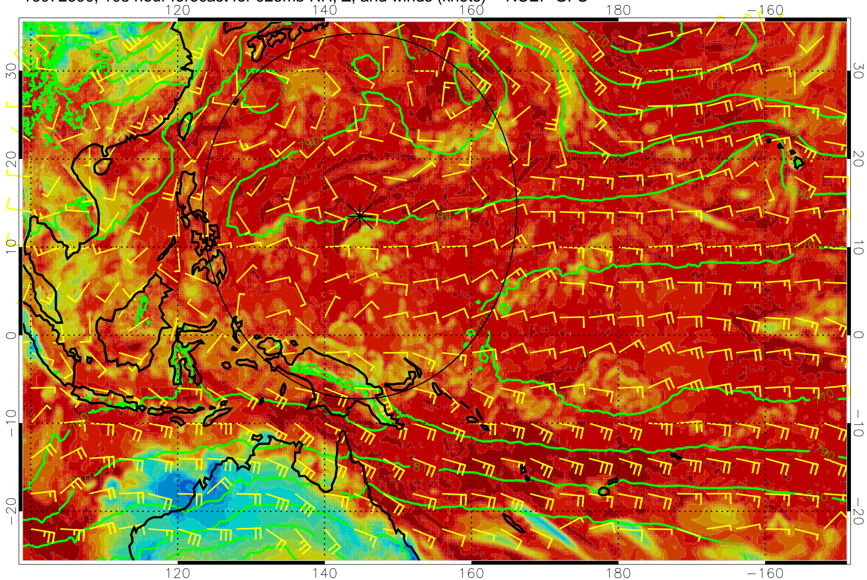
16072600, 108 hour forecast for 925mb RH, Z, and winds (knots) -- NCEP GFS
