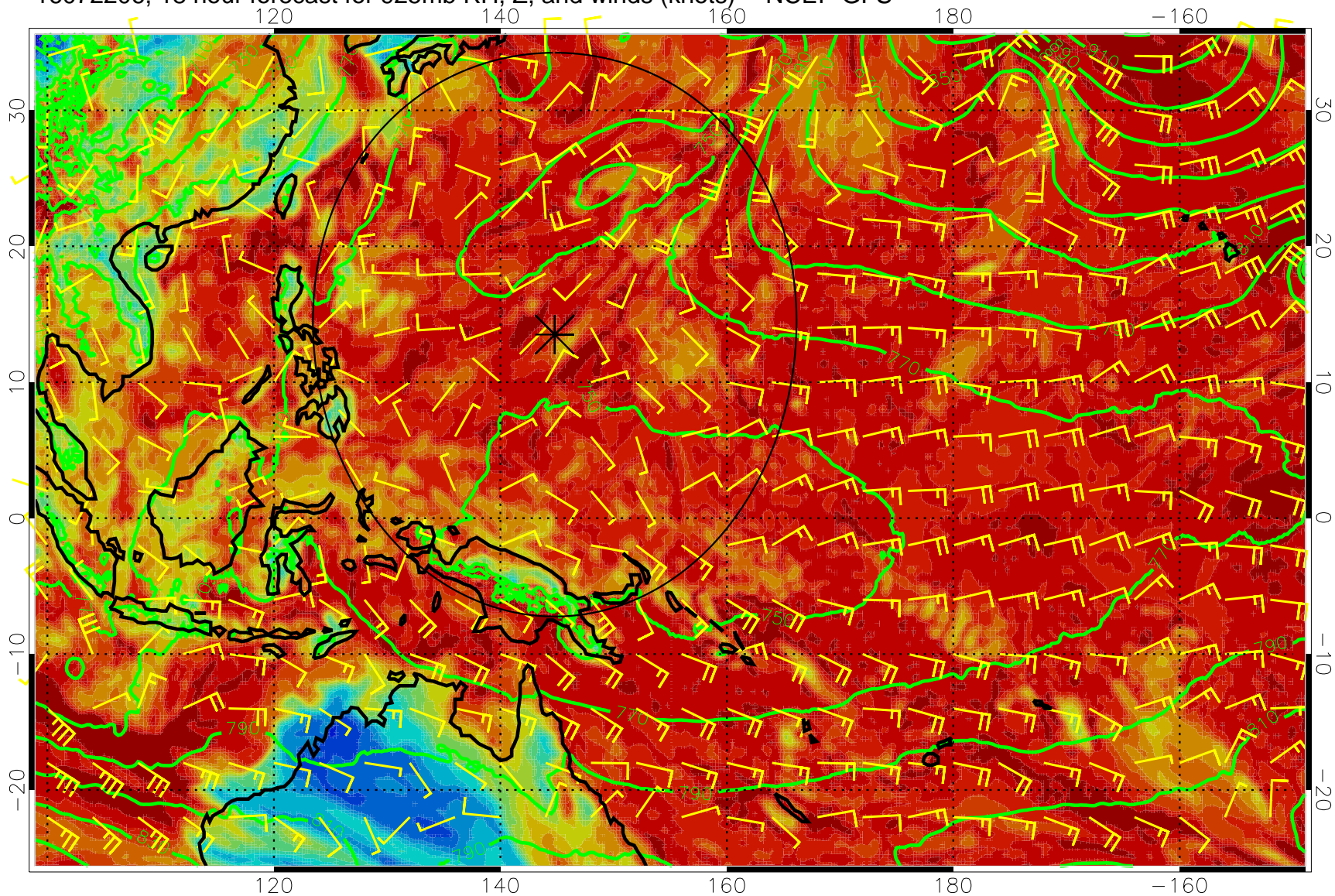
16072206, 18 hour forecast for 925mb RH, Z, and winds (knots) -- NCEP GFS
