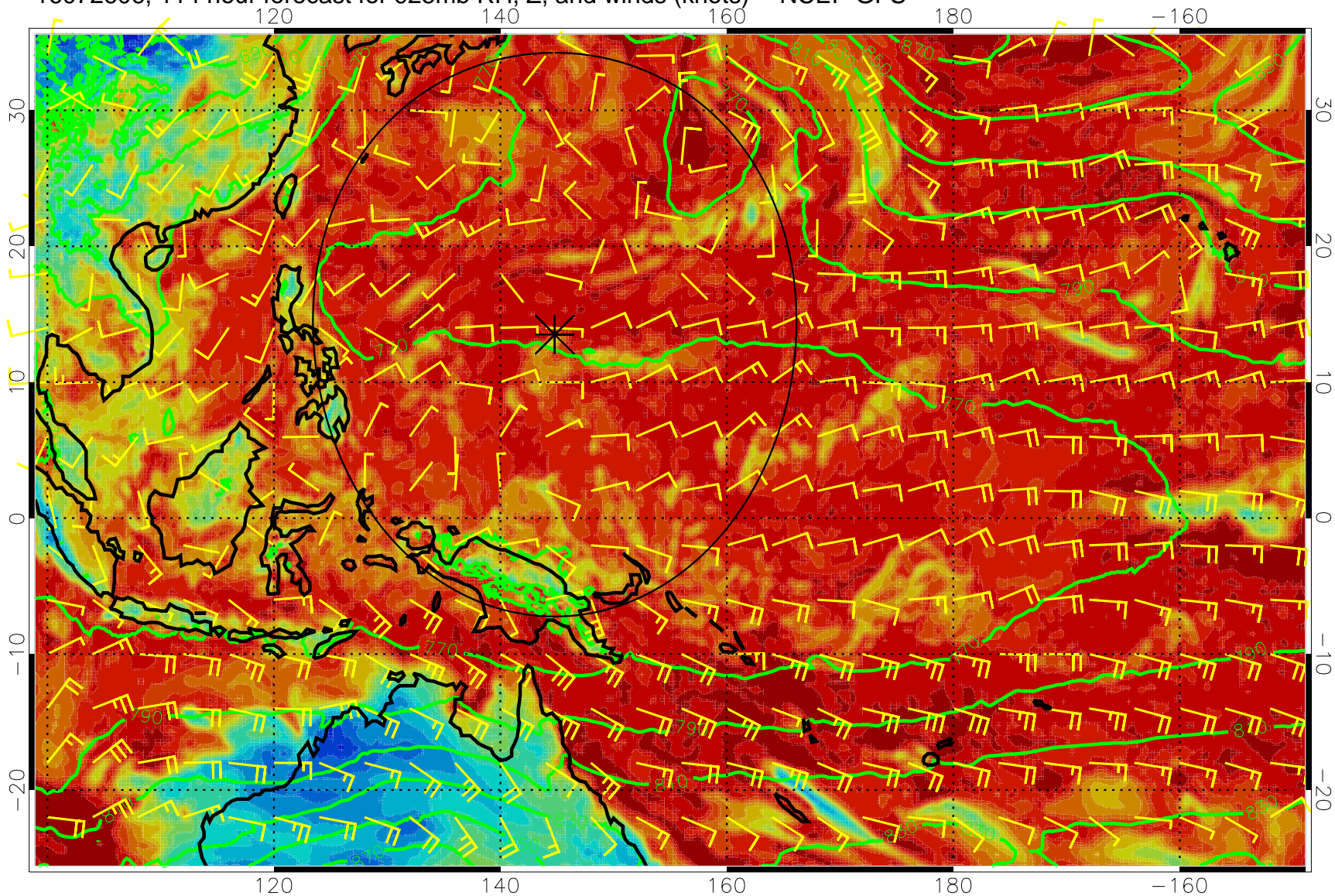
16072606, 114 hour forecast for 925mb RH, Z, and winds (knots) -- NCEP GFS
