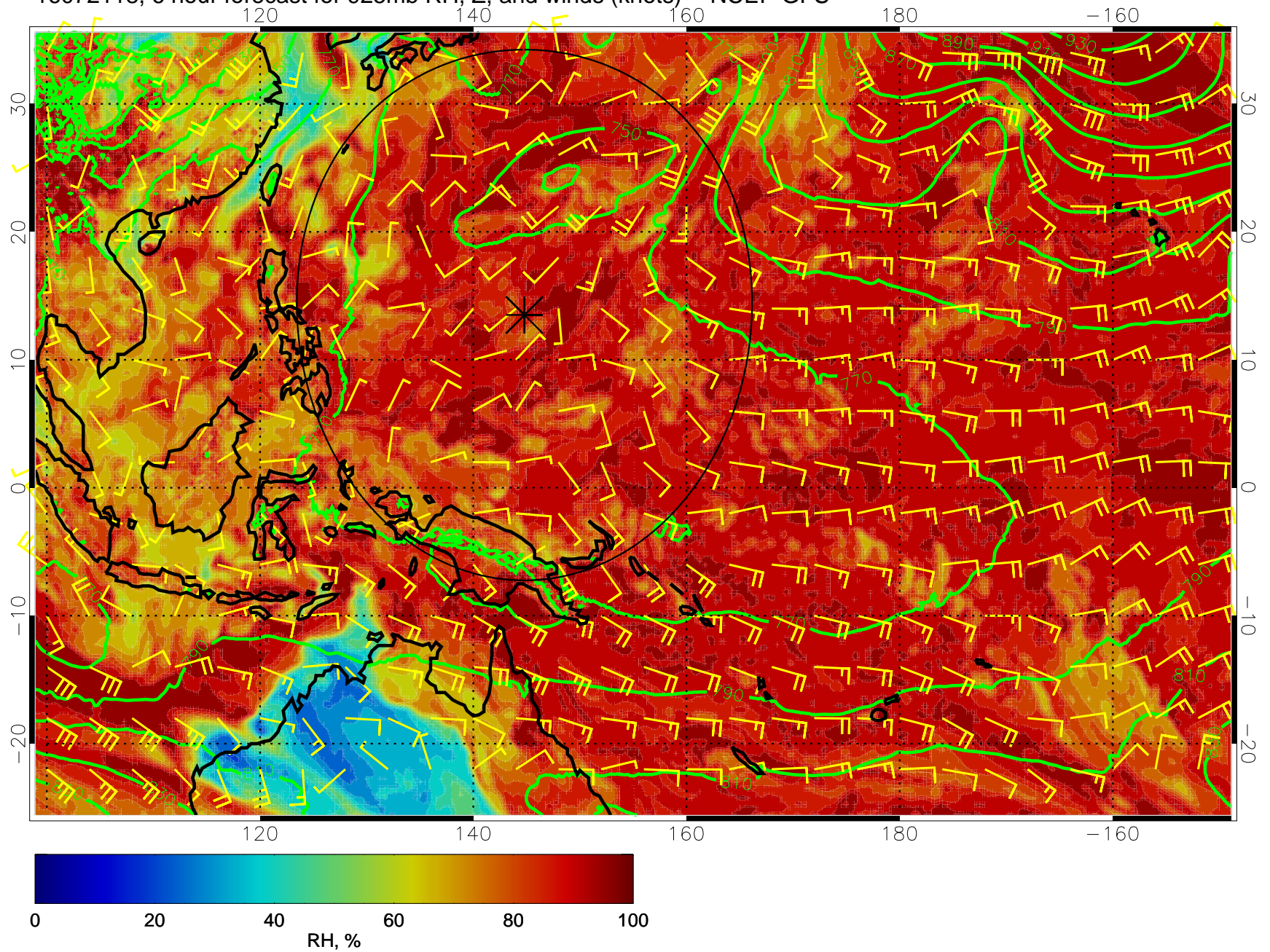
16072118, 6 hour forecast for 925mb RH, Z, and winds (knots) -- NCEP GFS
