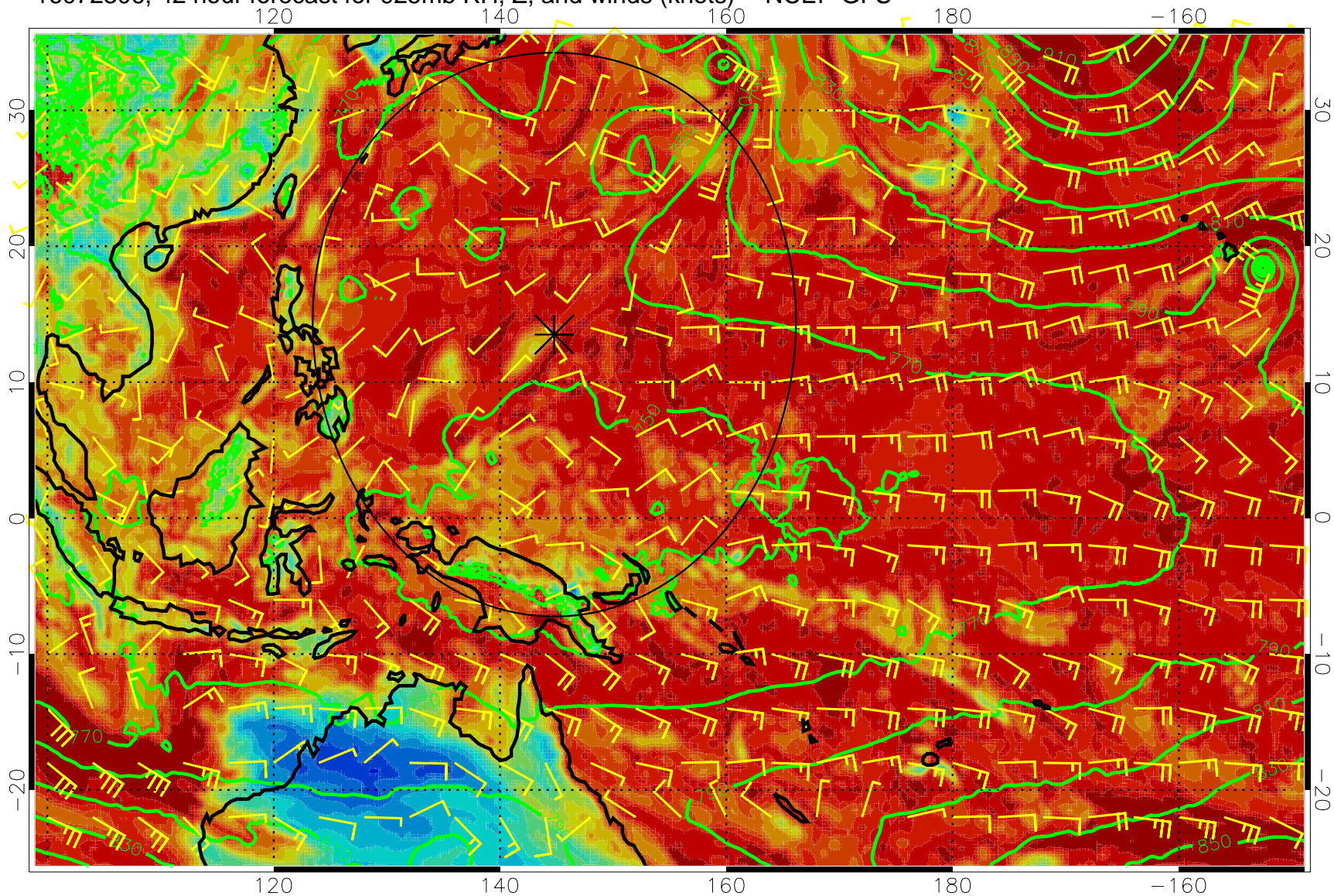
16072306, 42 hour forecast for 925mb RH, Z, and winds (knots) -- NCEP GFS
