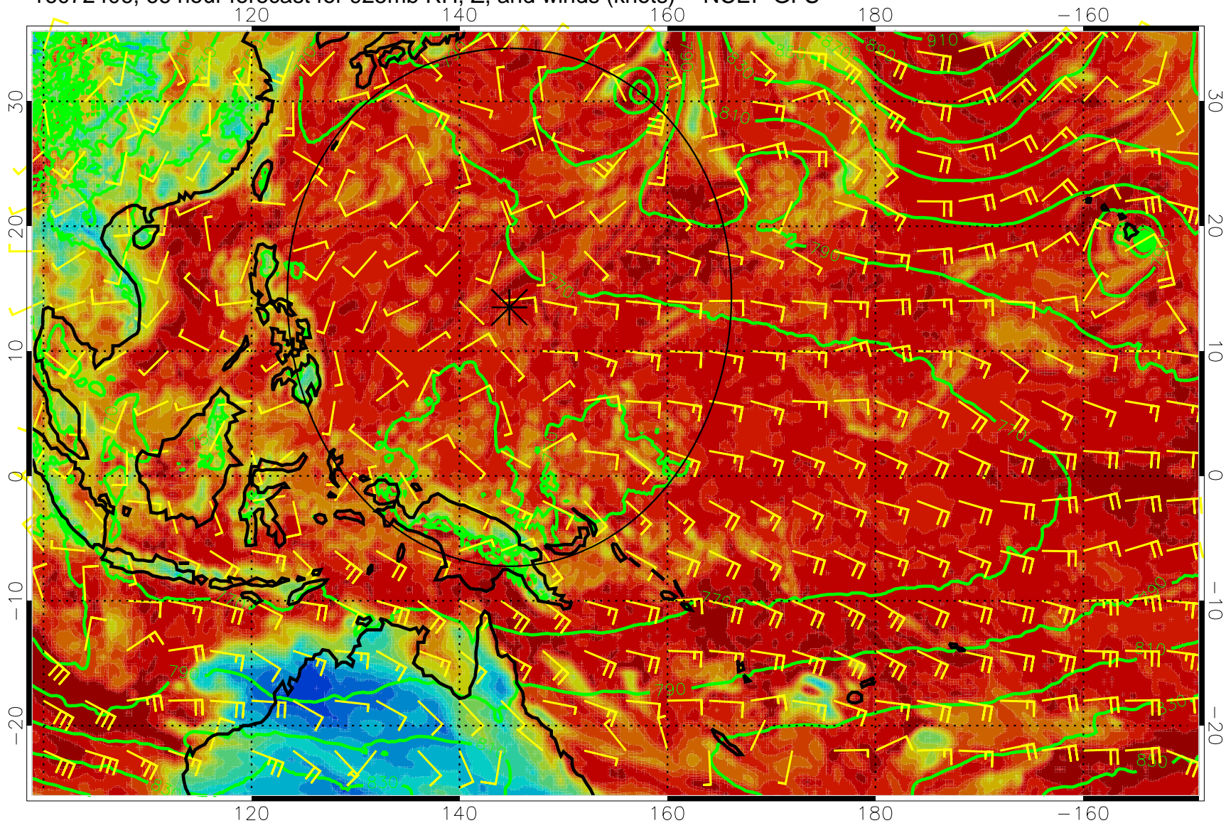
16072406, 66 hour forecast for 925mb RH, Z, and winds (knots) -- NCEP GFS
