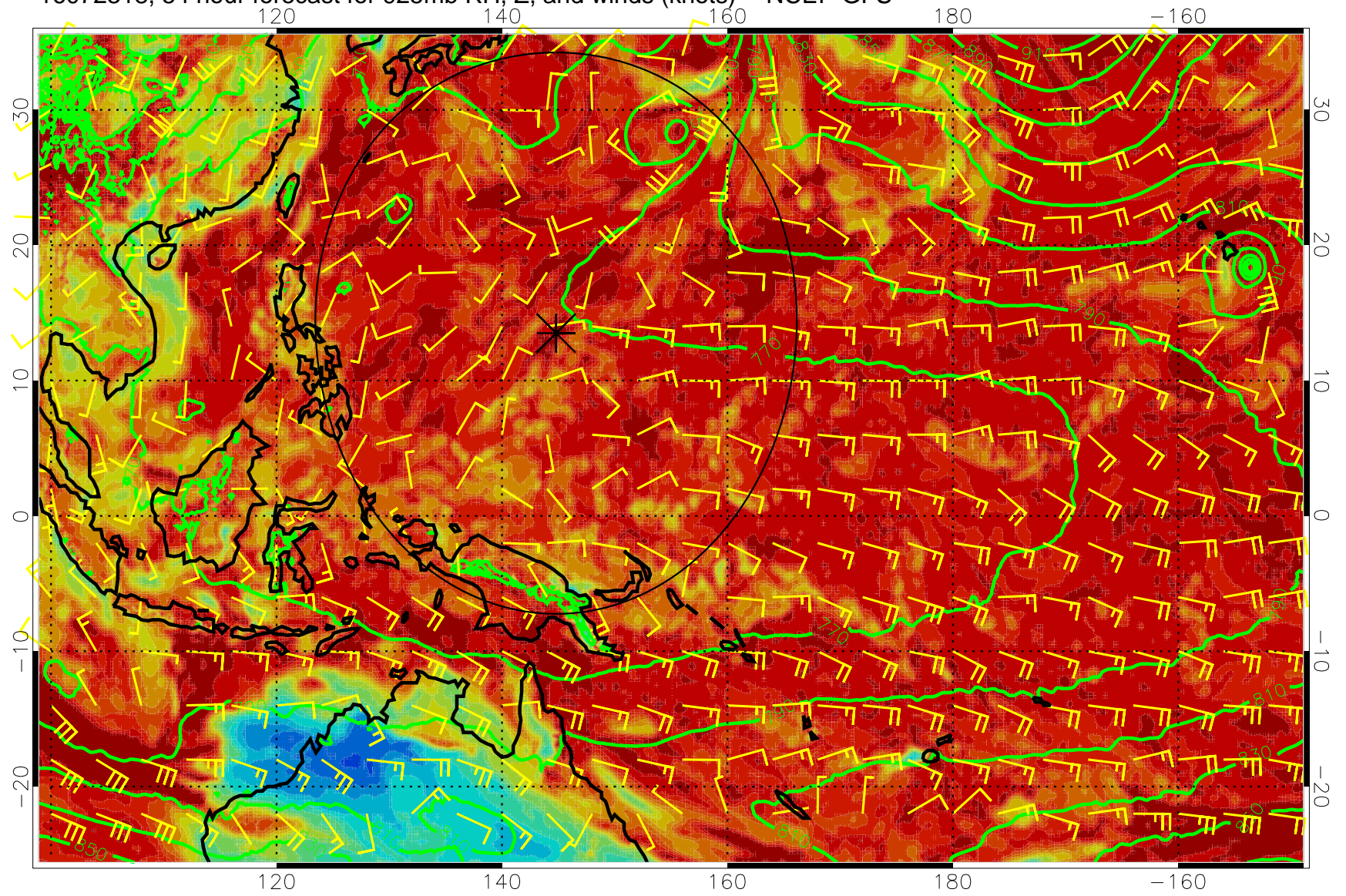
16072318, 54 hour forecast for 925mb RH, Z, and winds (knots) -- NCEP GFS
