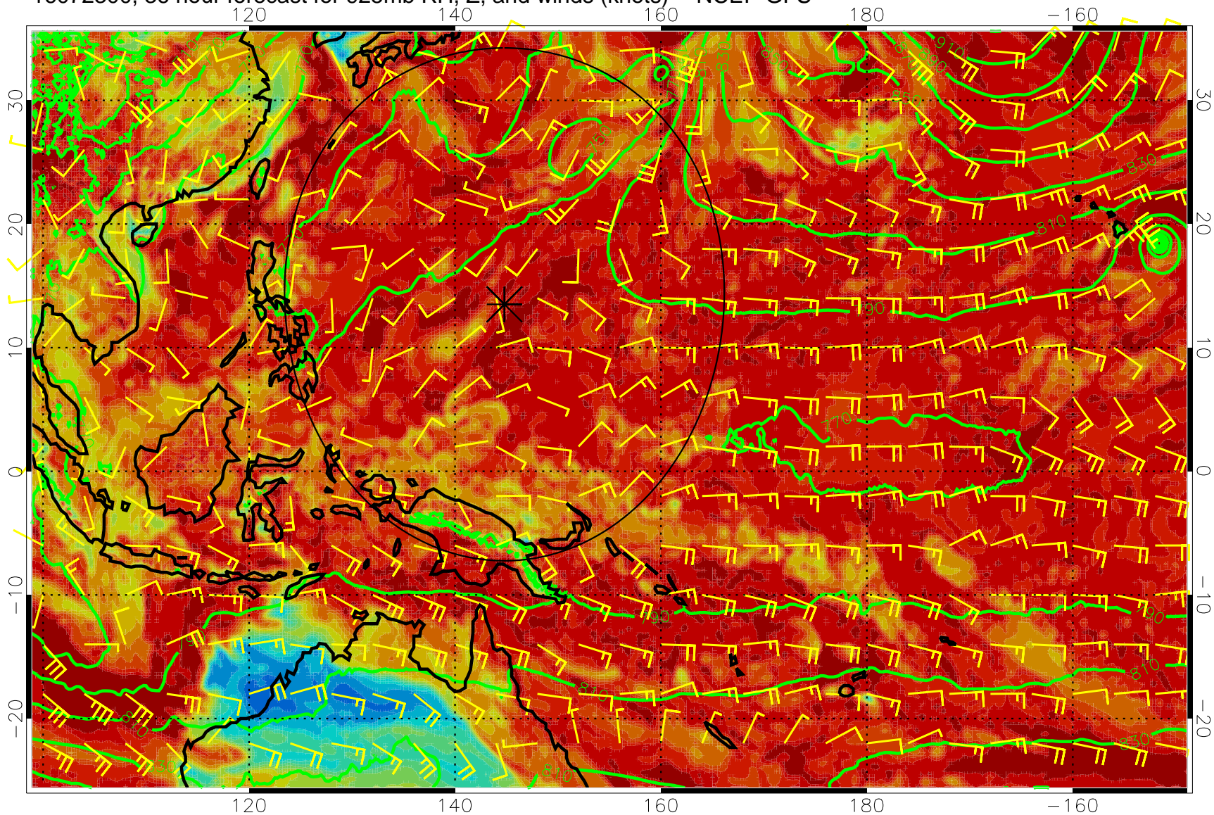
16072300, 36 hour forecast for 925mb RH, Z, and winds (knots) -- NCEP GFS
