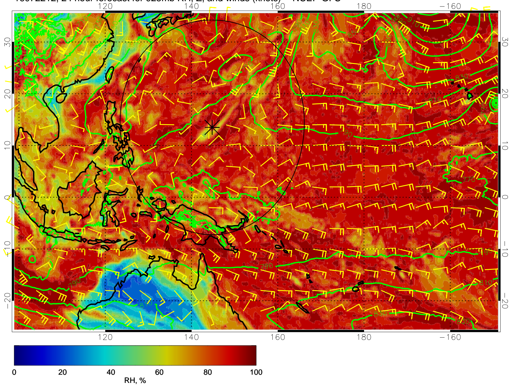
16072212, 24 hour forecast for 925mb RH, Z, and winds (knots) -- NCEP GFS
