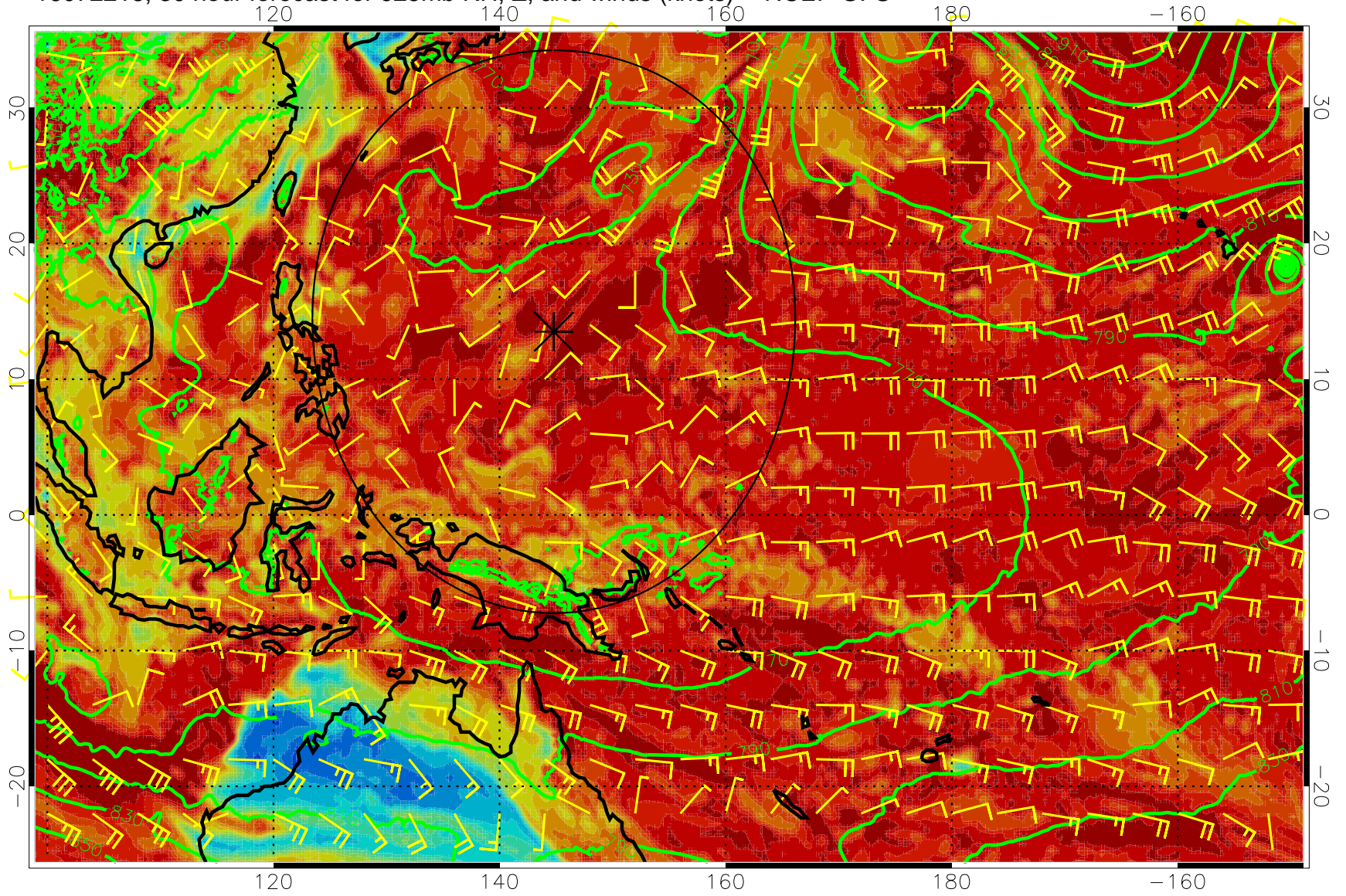
16072218, 30 hour forecast for 925mb RH, Z, and winds (knots) -- NCEP GFS
