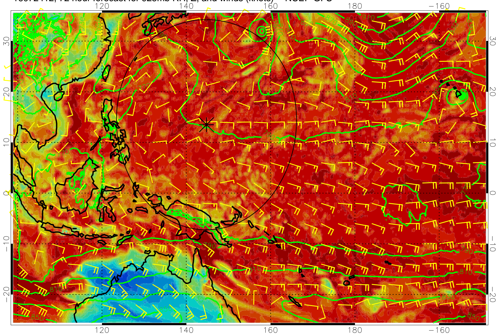
16072412, 72 hour forecast for 925mb RH, Z, and winds (knots) -- NCEP GFS
