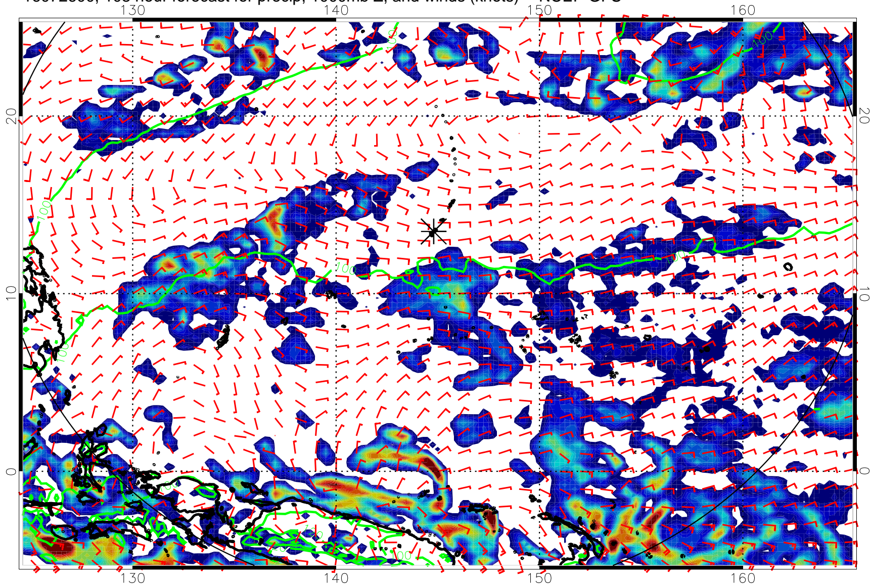
16072600, 108 hour forecast for precip, 1000mb Z, and winds (knots) -- NCEP GFS
