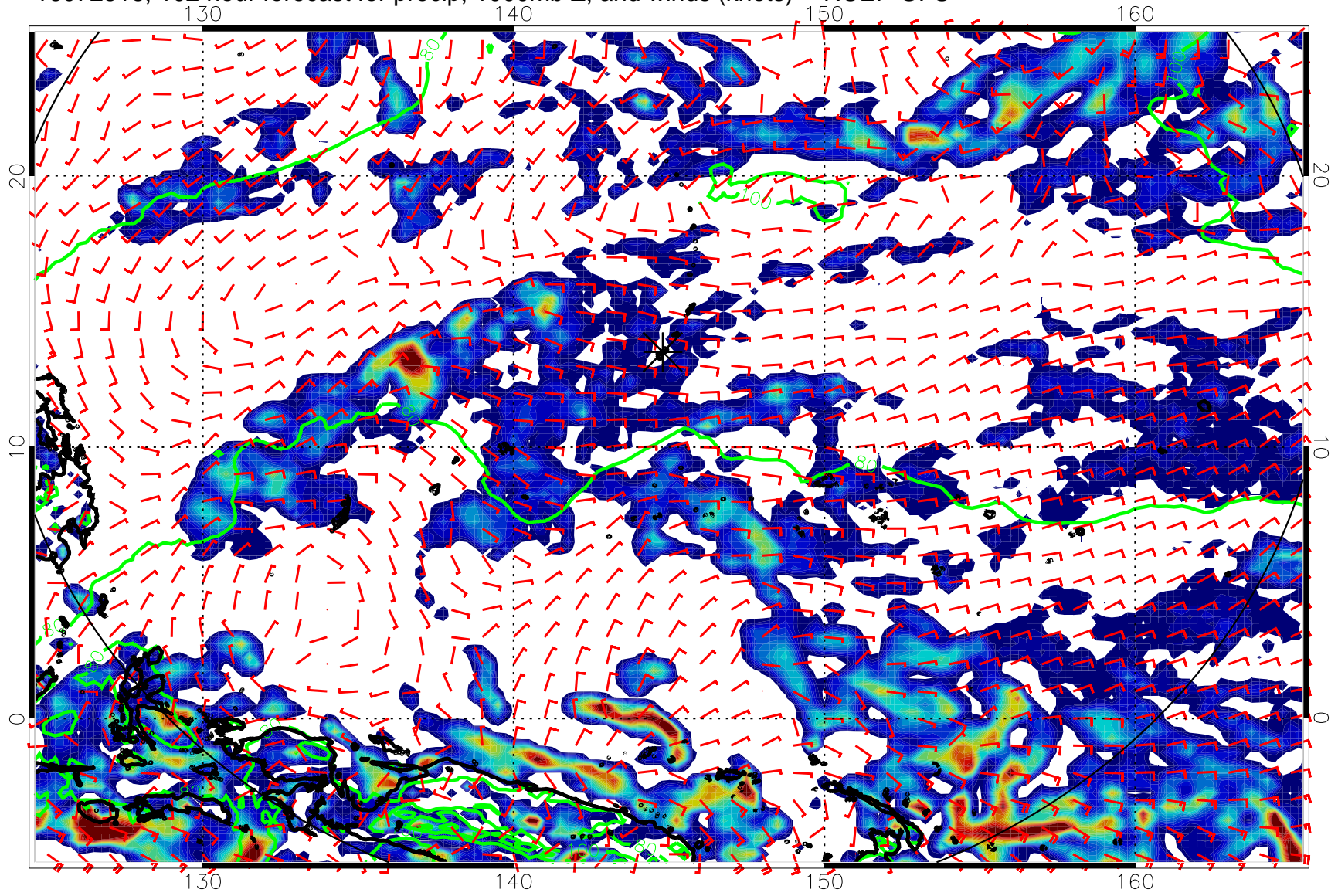
16072518, 102 hour forecast for precip, 1000mb Z, and winds (knots) -- NCEP GFS
