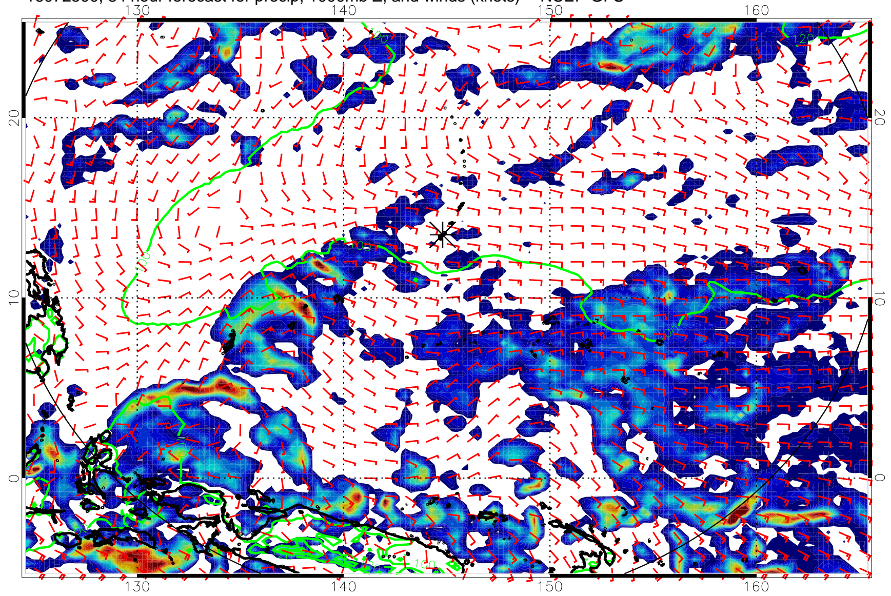
16072500, 84 hour forecast for precip, 1000mb Z, and winds (knots) -- NCEP GFS
