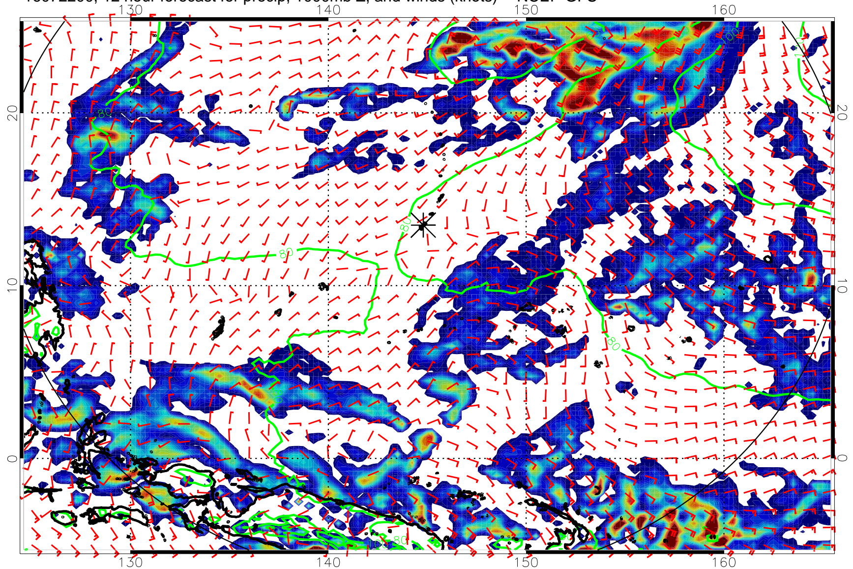
16072200, 12 hour forecast for precip, 1000mb Z, and winds (knots) -- NCEP GFS
