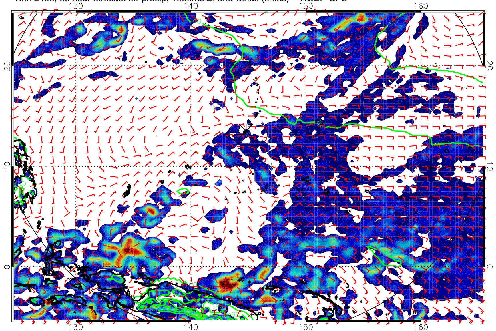
16072406, 66 hour forecast for precip, 1000mb Z, and winds (knots) -- NCEP GFS
