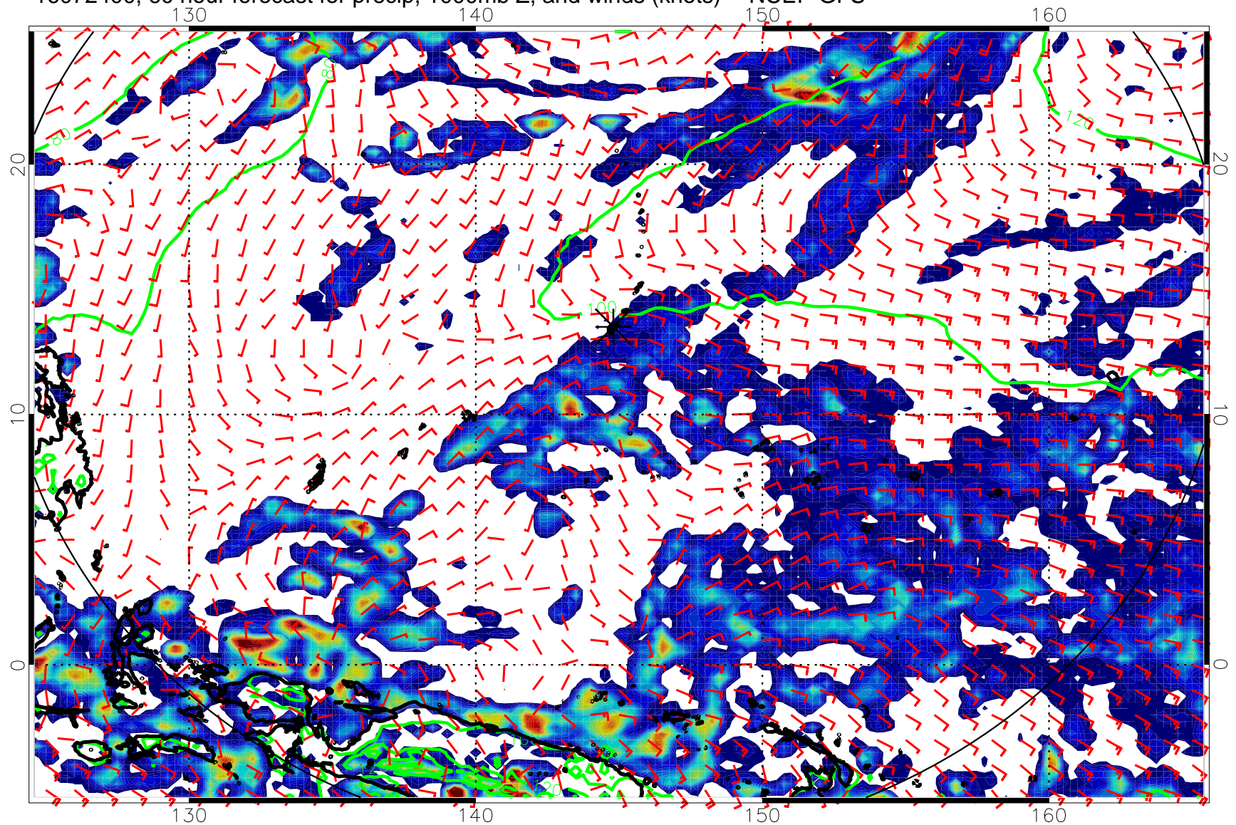
16072400, 60 hour forecast for precip, 1000mb Z, and winds (knots) -- NCEP GFS
