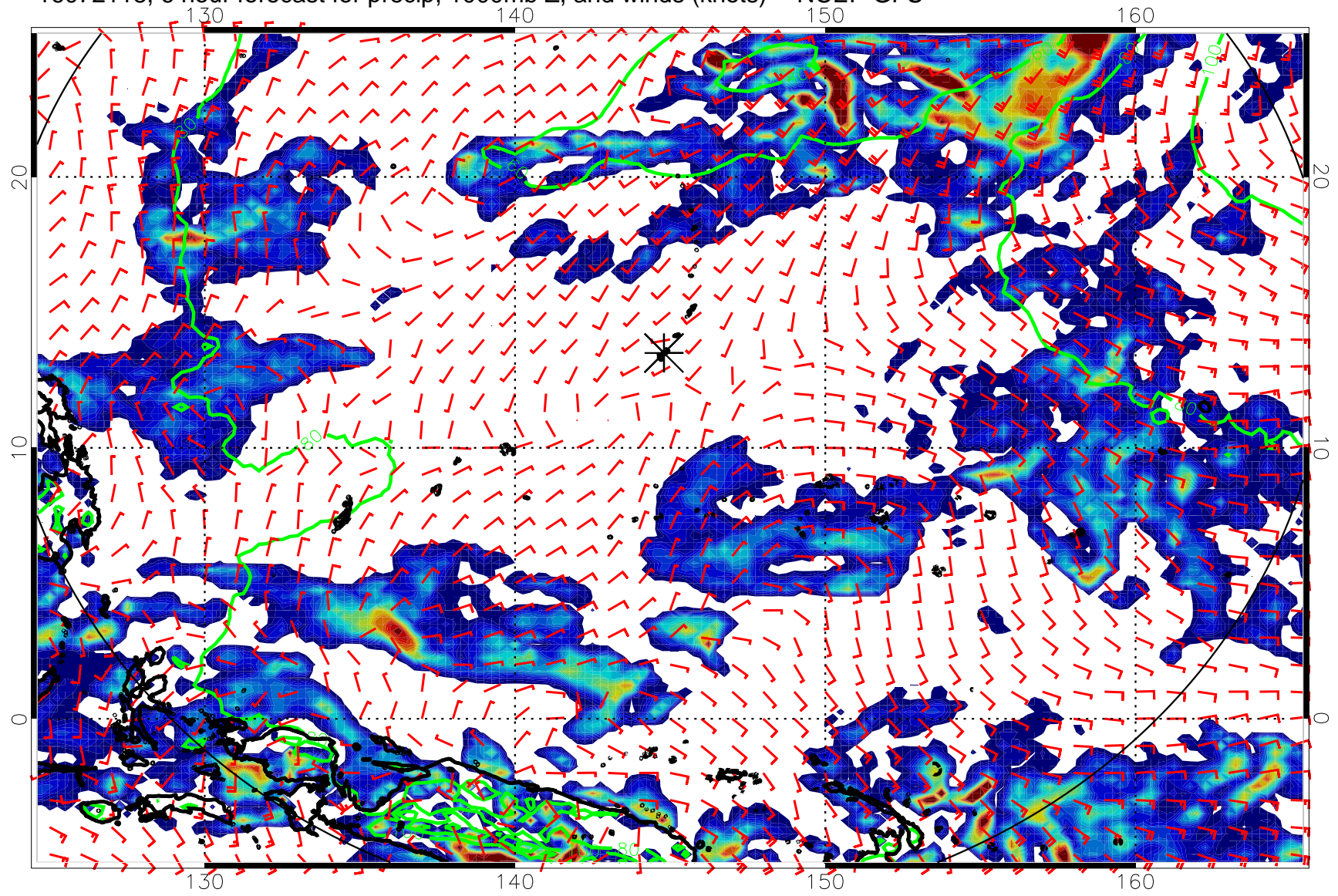
16072118, 6 hour forecast for precip, 1000mb Z, and winds (knots) -- NCEP GFS
