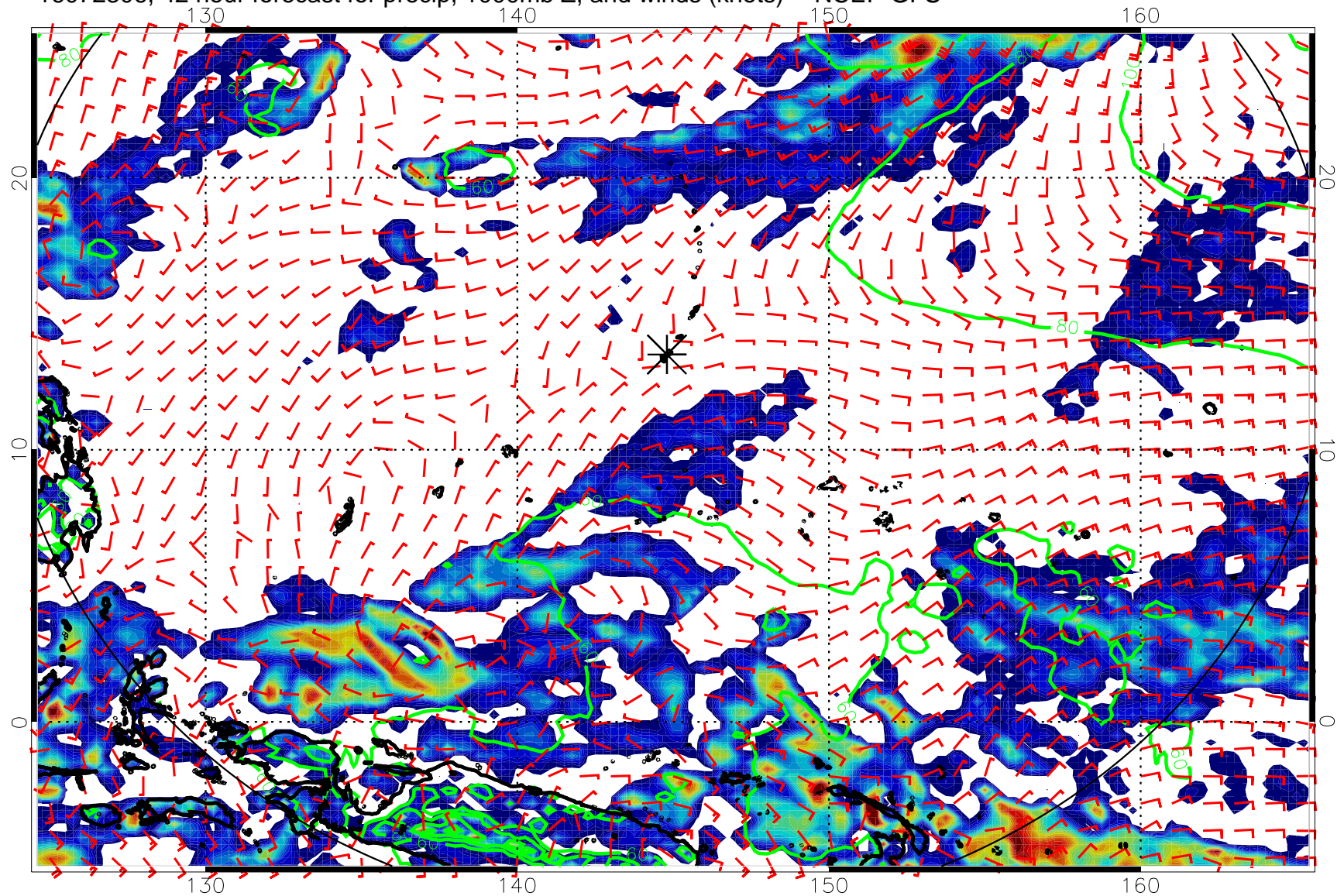
16072306, 42 hour forecast for precip, 1000mb Z, and winds (knots) -- NCEP GFS
