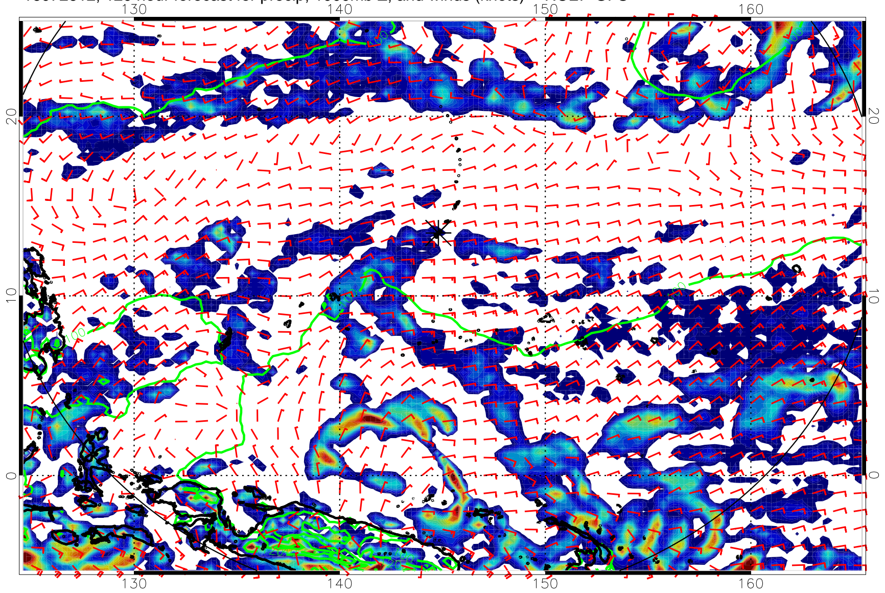
16072612, 120 hour forecast for precip, 1000mb Z, and winds (knots) -- NCEP GFS
