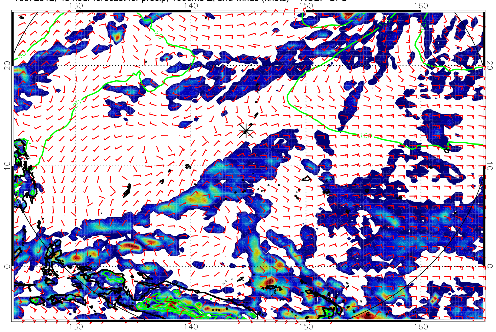
16072312, 48 hour forecast for precip, 1000mb Z, and winds (knots) -- NCEP GFS
