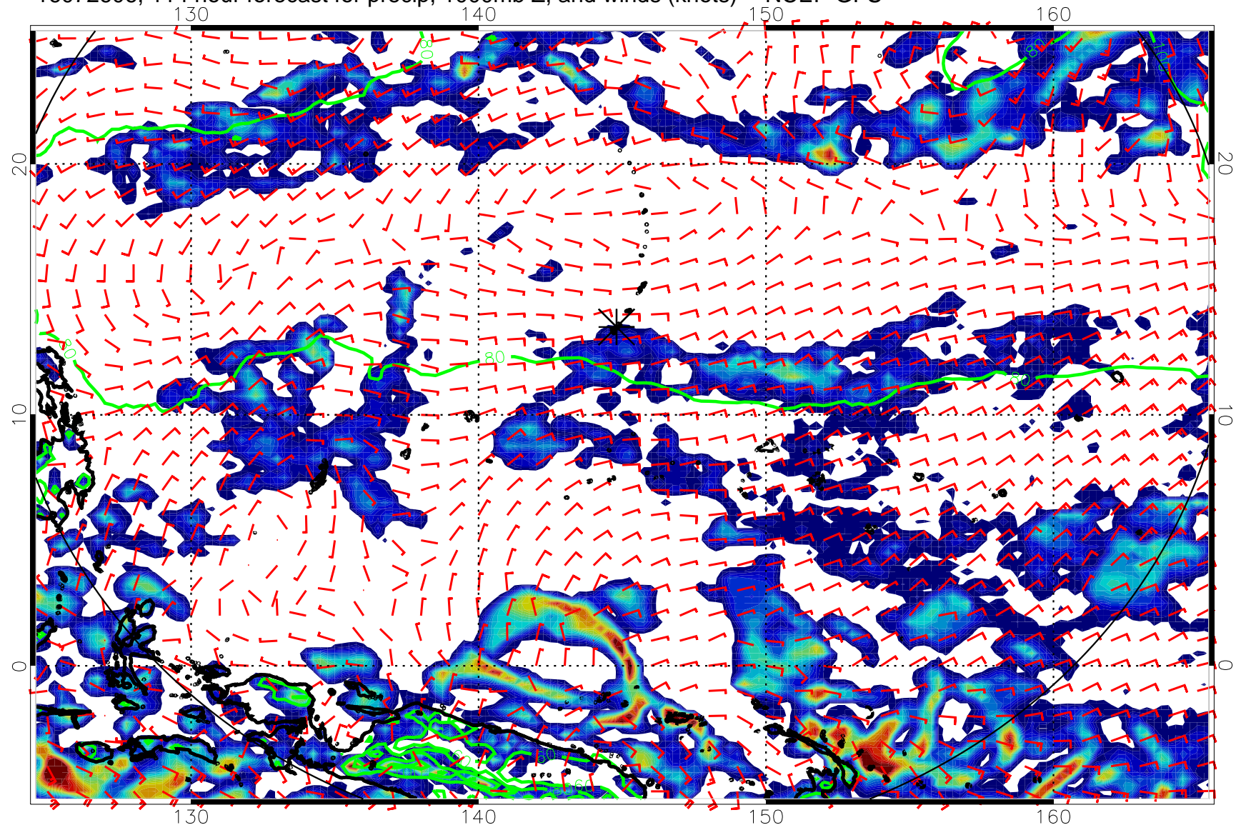
16072606, 114 hour forecast for precip, 1000mb Z, and winds (knots) -- NCEP GFS
