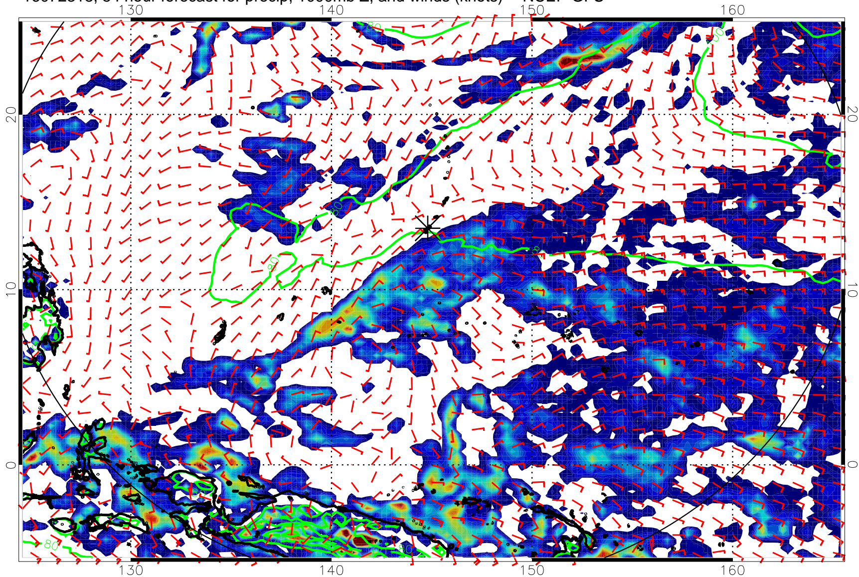
16072318, 54 hour forecast for precip, 1000mb Z, and winds (knots) -- NCEP GFS
