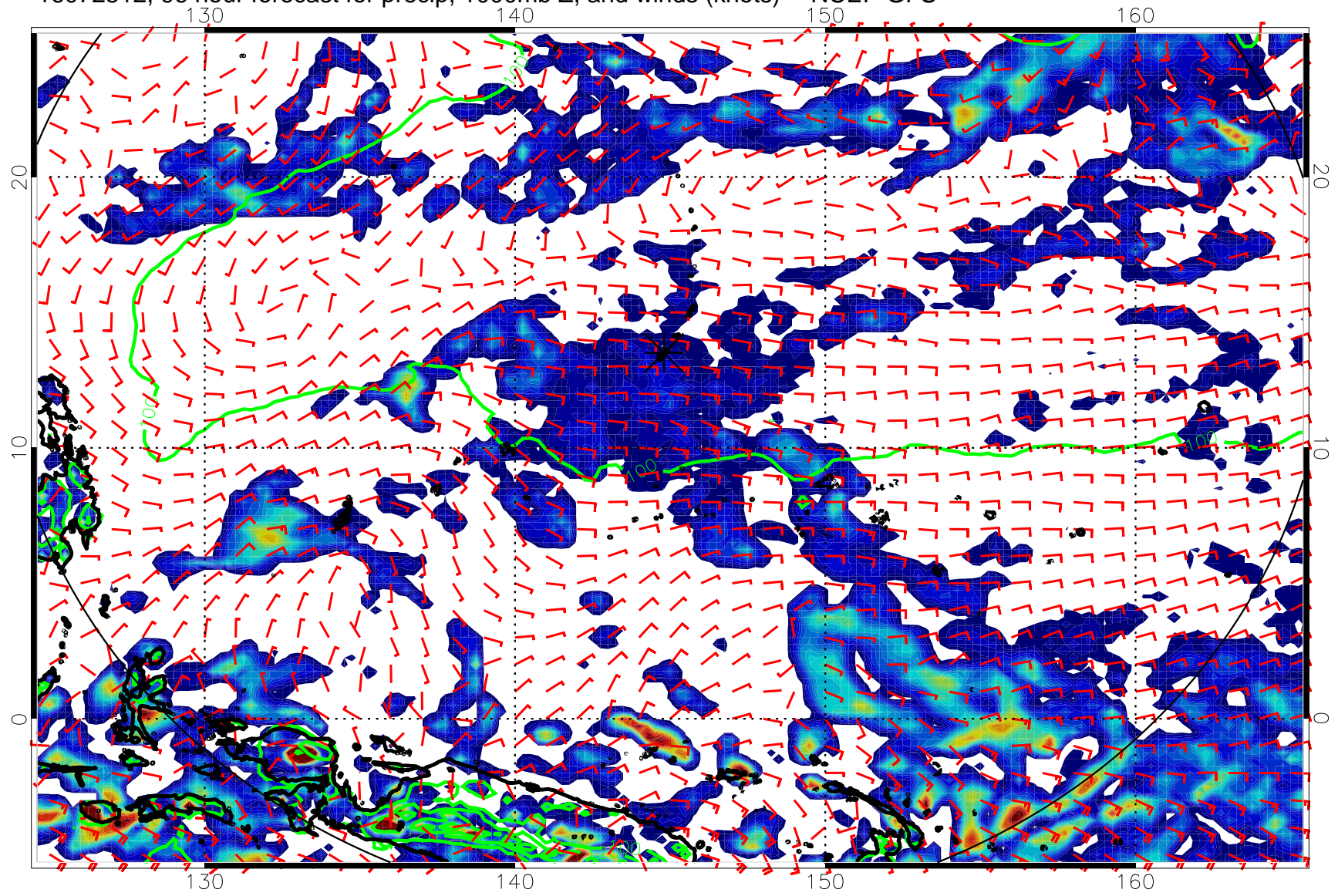
16072512, 96 hour forecast for precip, 1000mb Z, and winds (knots) -- NCEP GFS
