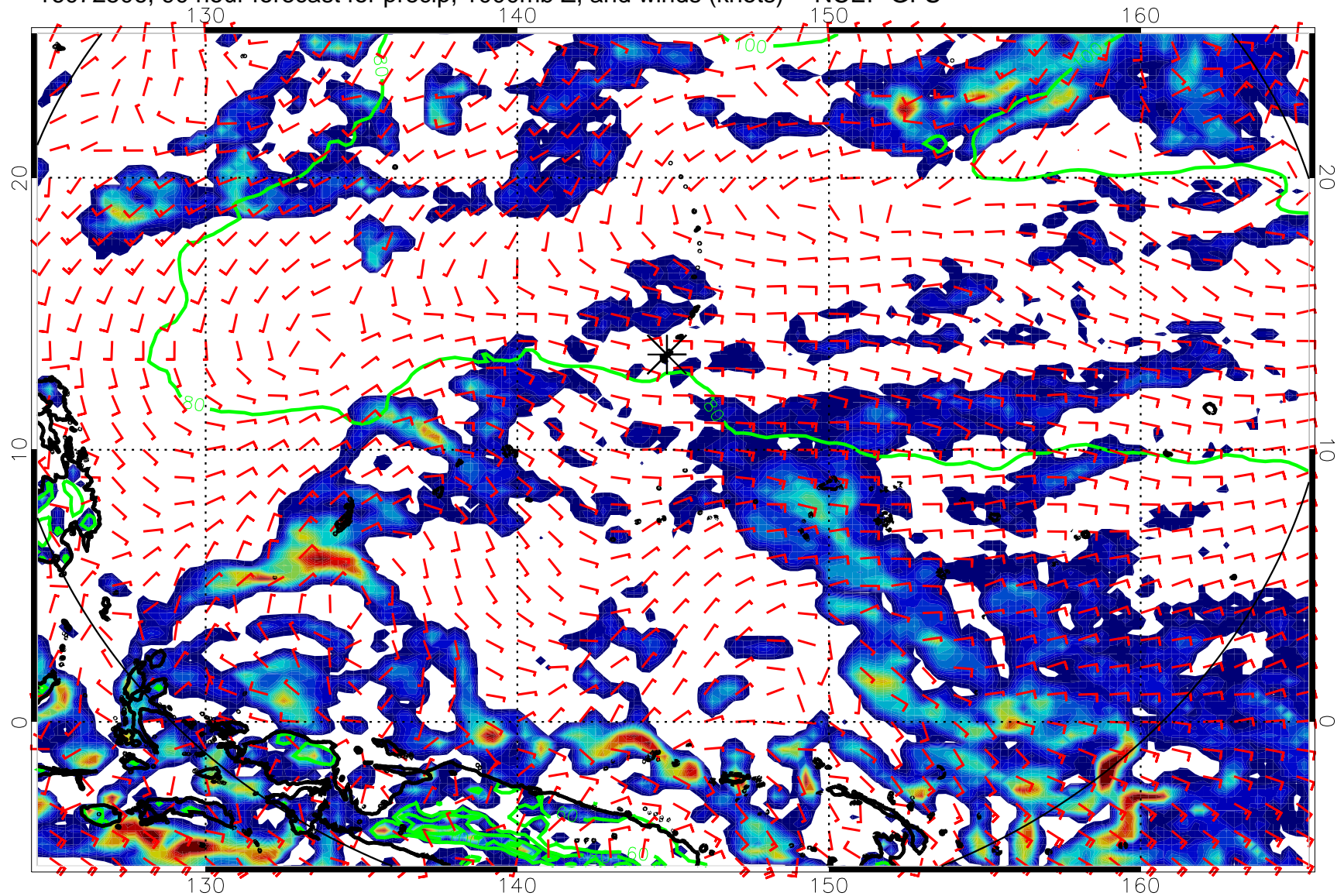
16072506, 90 hour forecast for precip, 1000mb Z, and winds (knots) -- NCEP GFS
