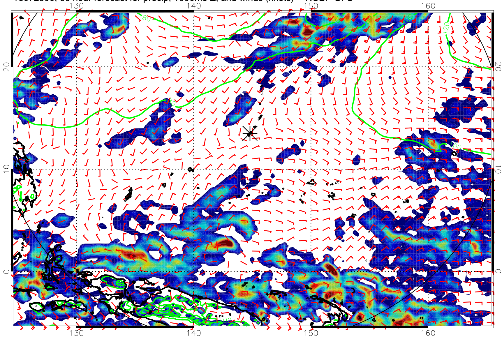
16072300, 36 hour forecast for precip, 1000mb Z, and winds (knots) -- NCEP GFS
