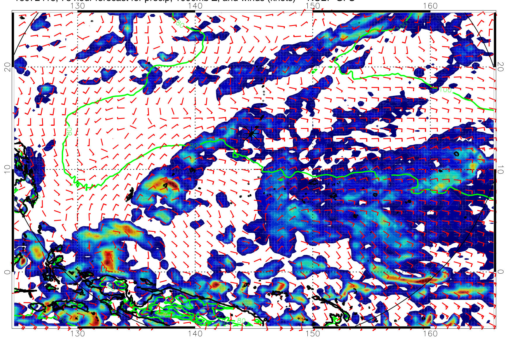
16072418, 78 hour forecast for precip, 1000mb Z, and winds (knots) -- NCEP GFS
