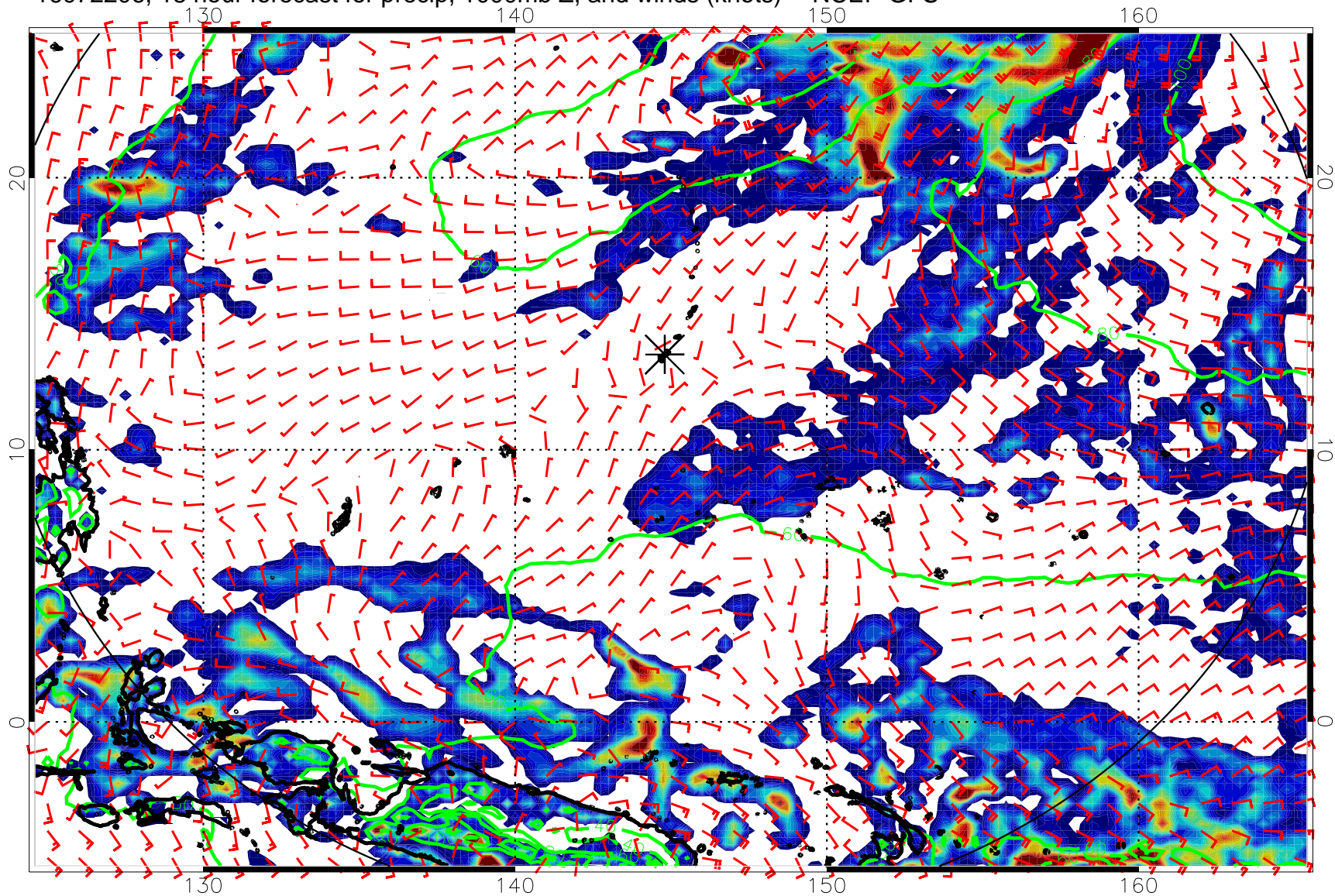
16072206, 18 hour forecast for precip, 1000mb Z, and winds (knots) -- NCEP GFS
