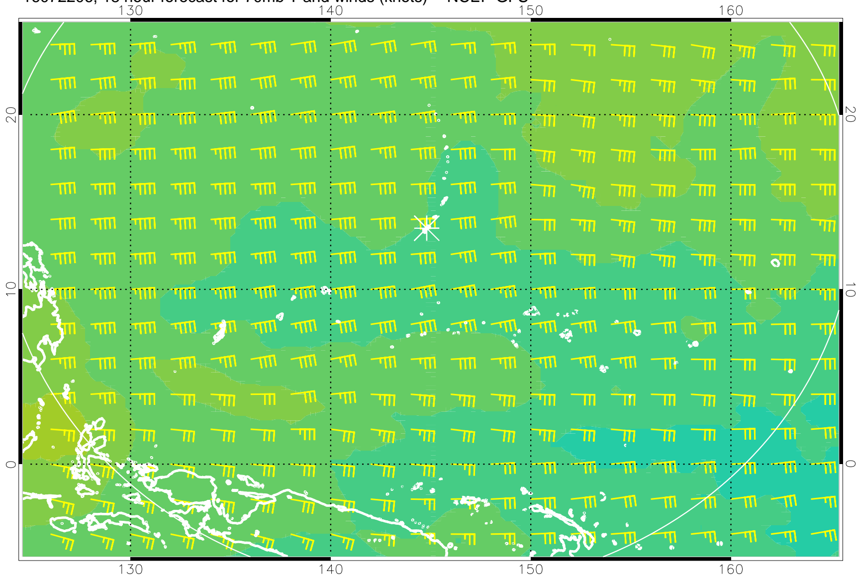
16072206, 18 hour forecast for 70mb T and winds (knots) -- NCEP GFS
