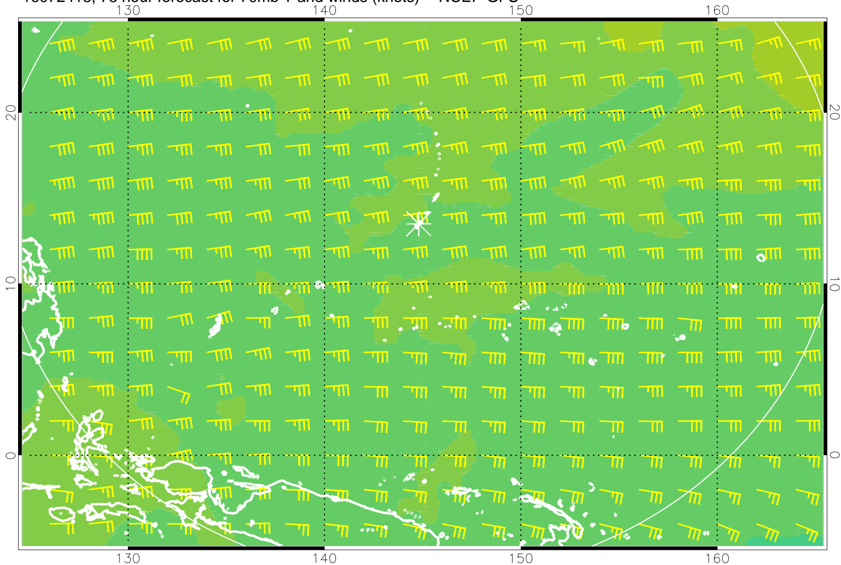
16072418, 78 hour forecast for 70mb T and winds (knots) -- NCEP GFS
