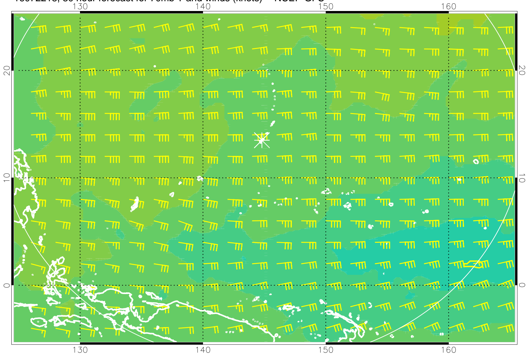
16072218, 30 hour forecast for 70mb T and winds (knots) -- NCEP GFS
