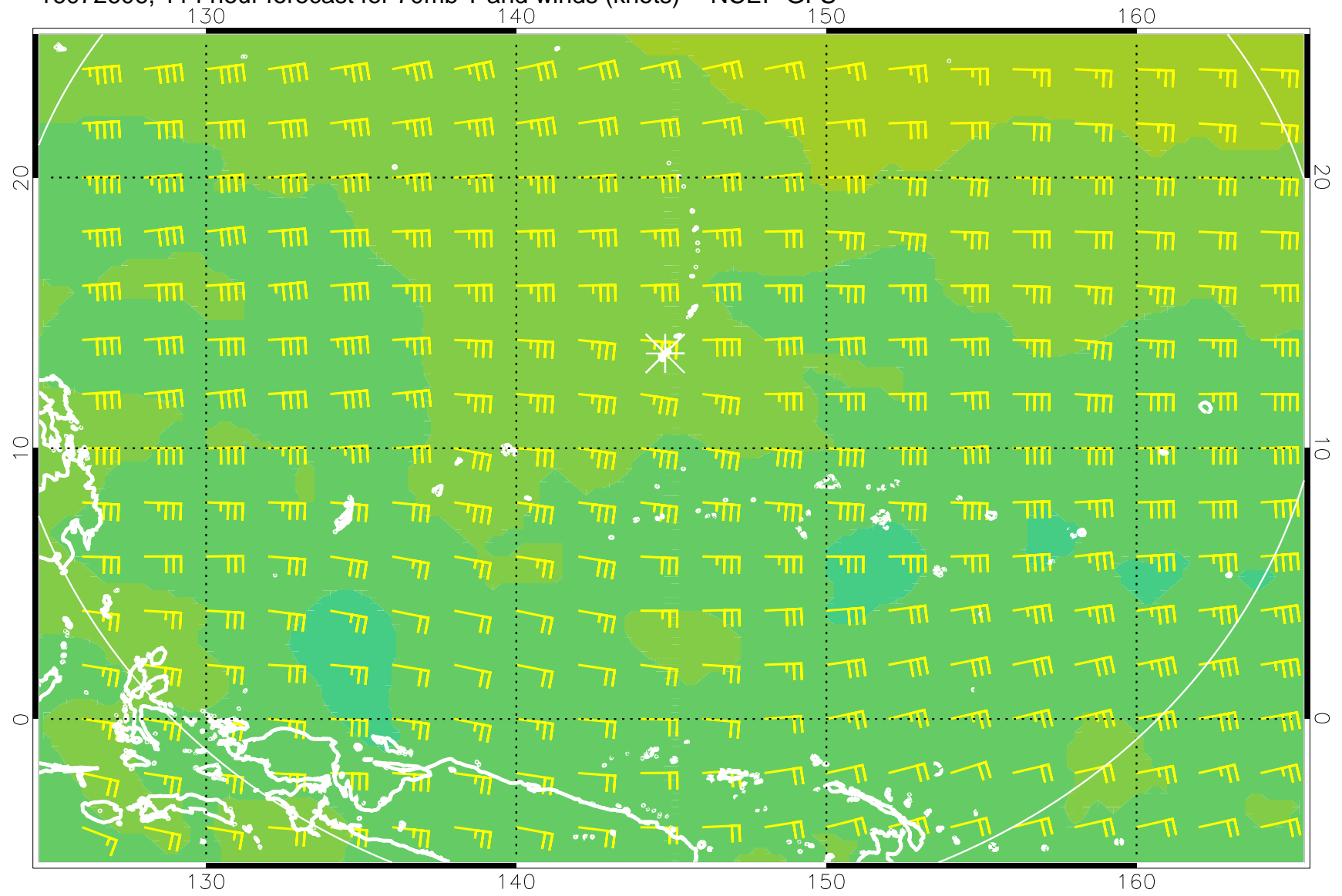
16072606, 114 hour forecast for 70mb T and winds (knots) -- NCEP GFS
