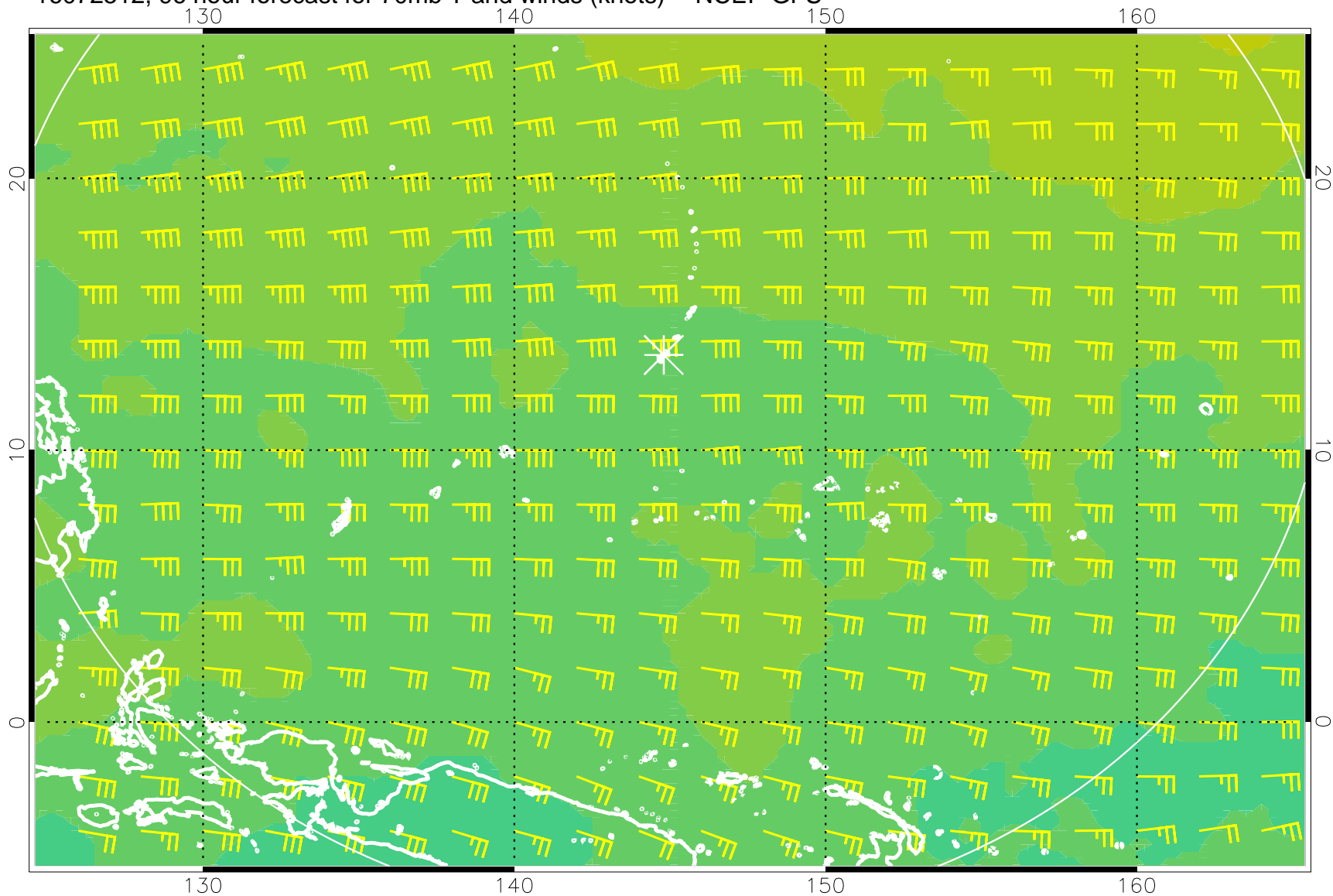
16072512, 96 hour forecast for 70mb T and winds (knots) -- NCEP GFS
