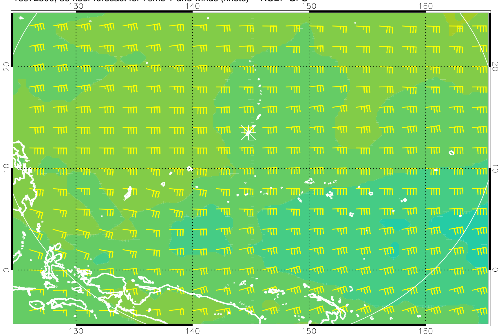
16072300, 36 hour forecast for 70mb T and winds (knots) -- NCEP GFS
