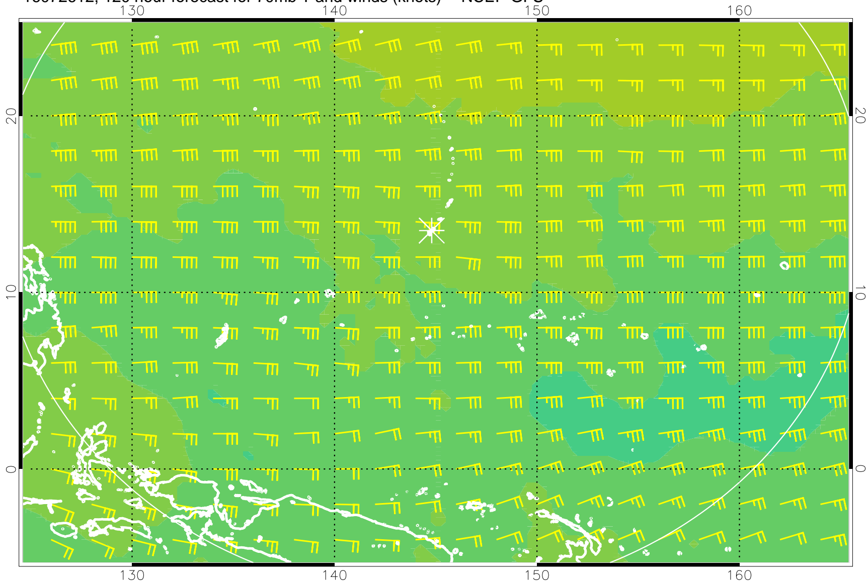
16072612, 120 hour forecast for 70mb T and winds (knots) -- NCEP GFS
