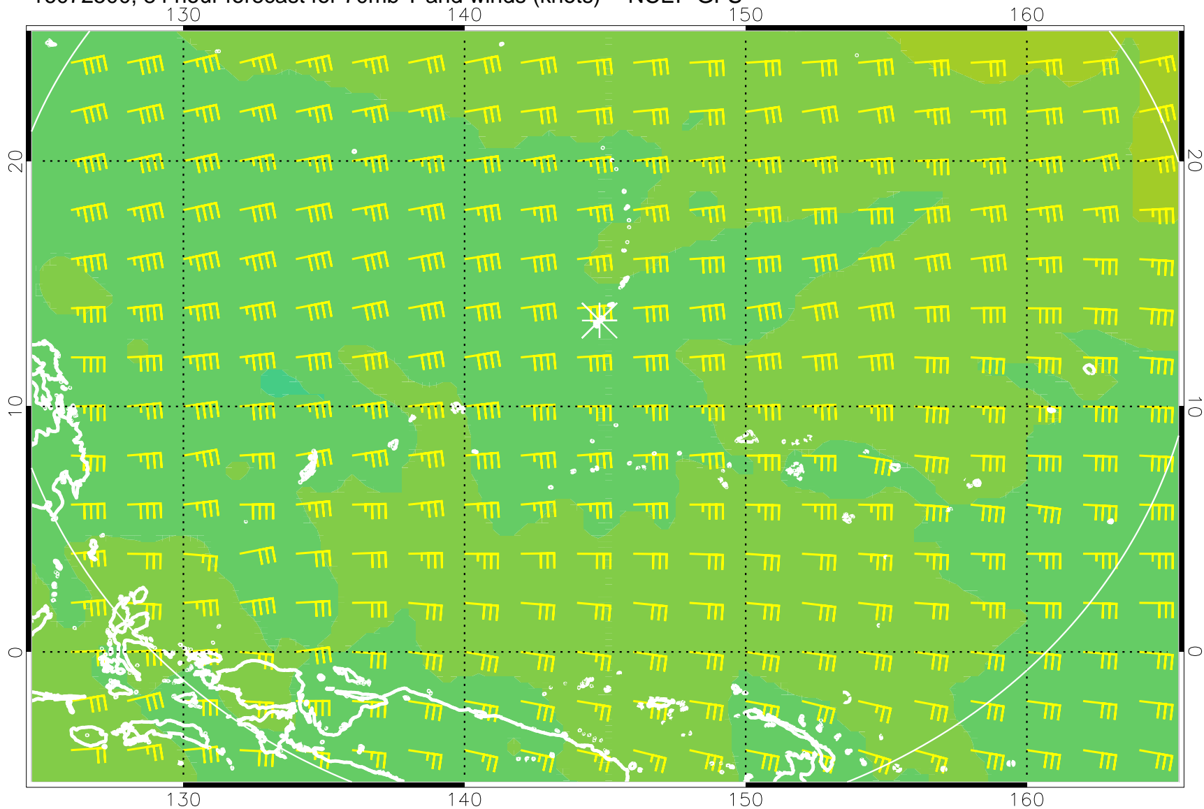
16072500, 84 hour forecast for 70mb T and winds (knots) -- NCEP GFS
