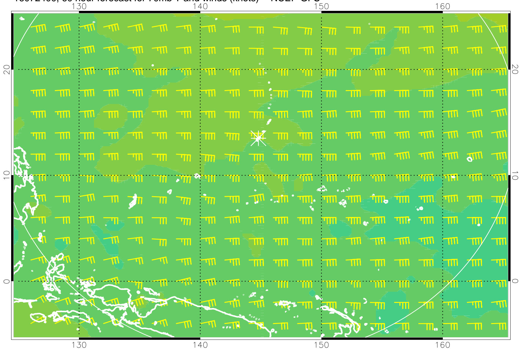
16072400, 60 hour forecast for 70mb T and winds (knots) -- NCEP GFS
