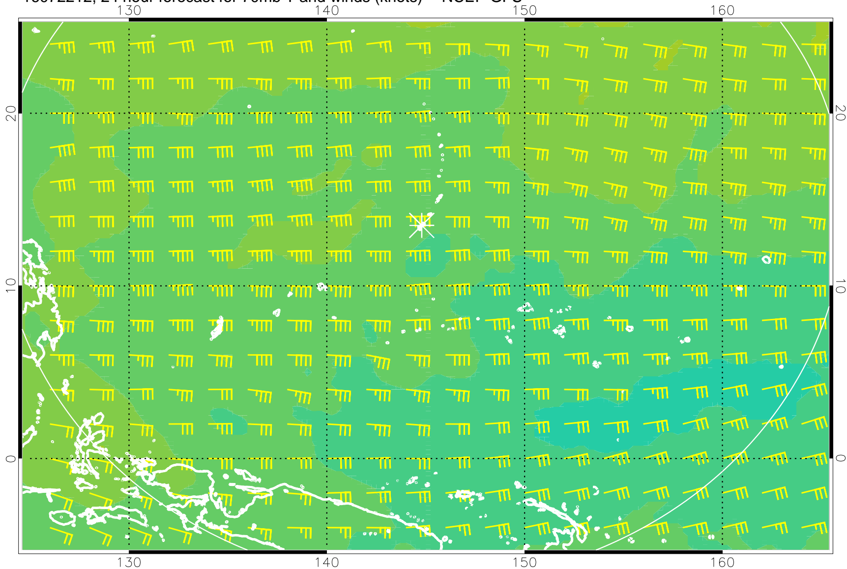
16072212, 24 hour forecast for 70mb T and winds (knots) -- NCEP GFS
