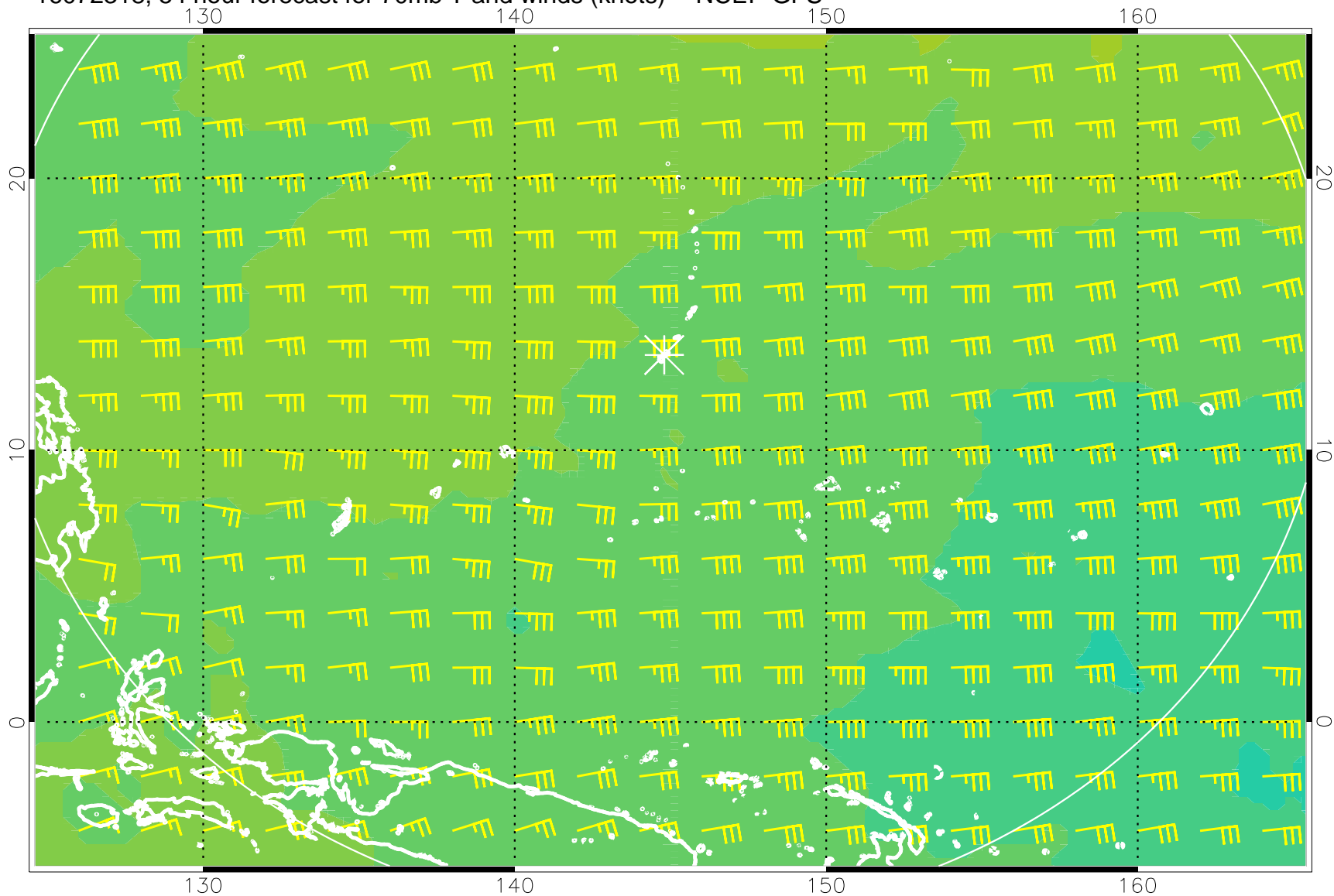
16072318, 54 hour forecast for 70mb T and winds (knots) -- NCEP GFS
