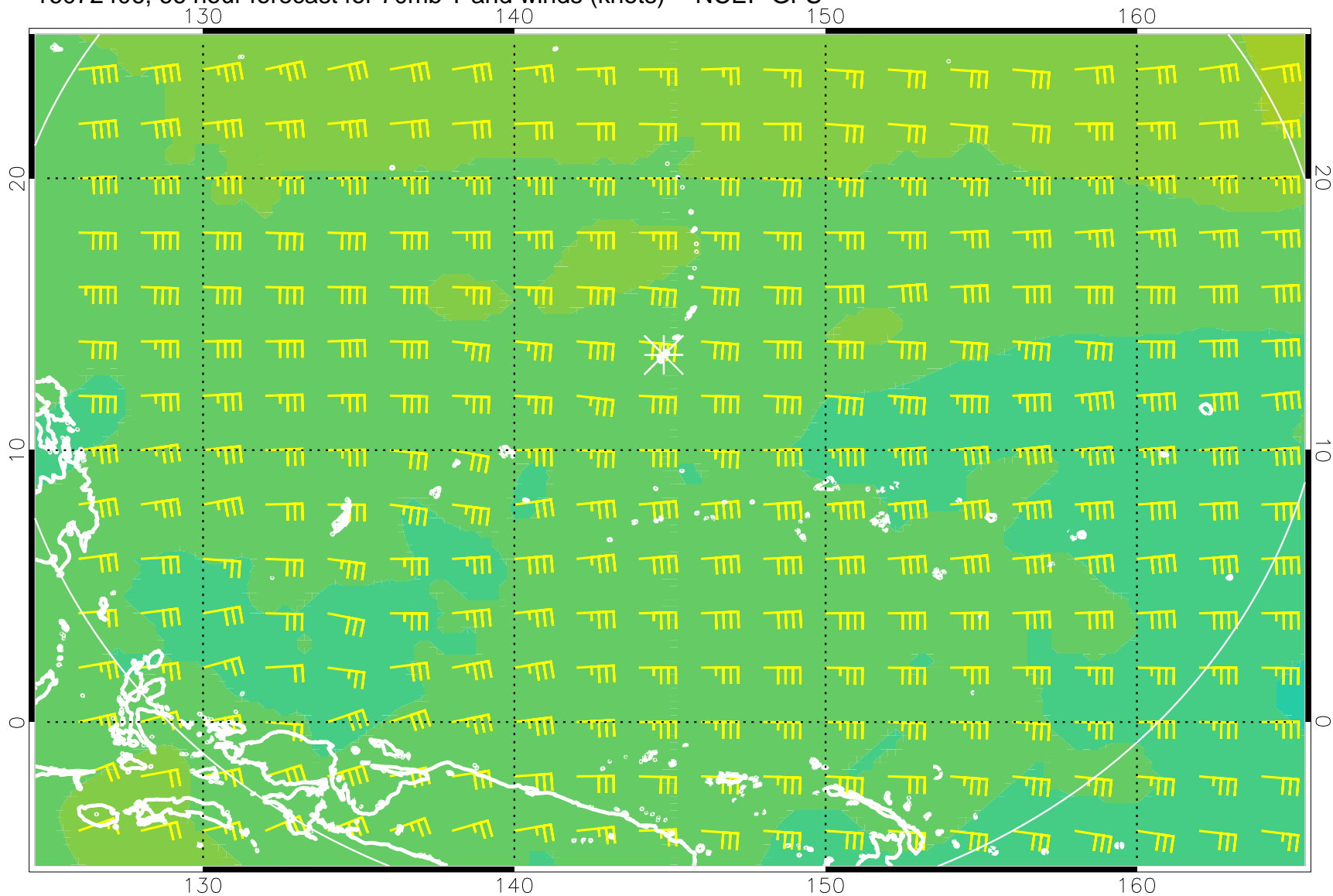
16072406, 66 hour forecast for 70mb T and winds (knots) -- NCEP GFS
