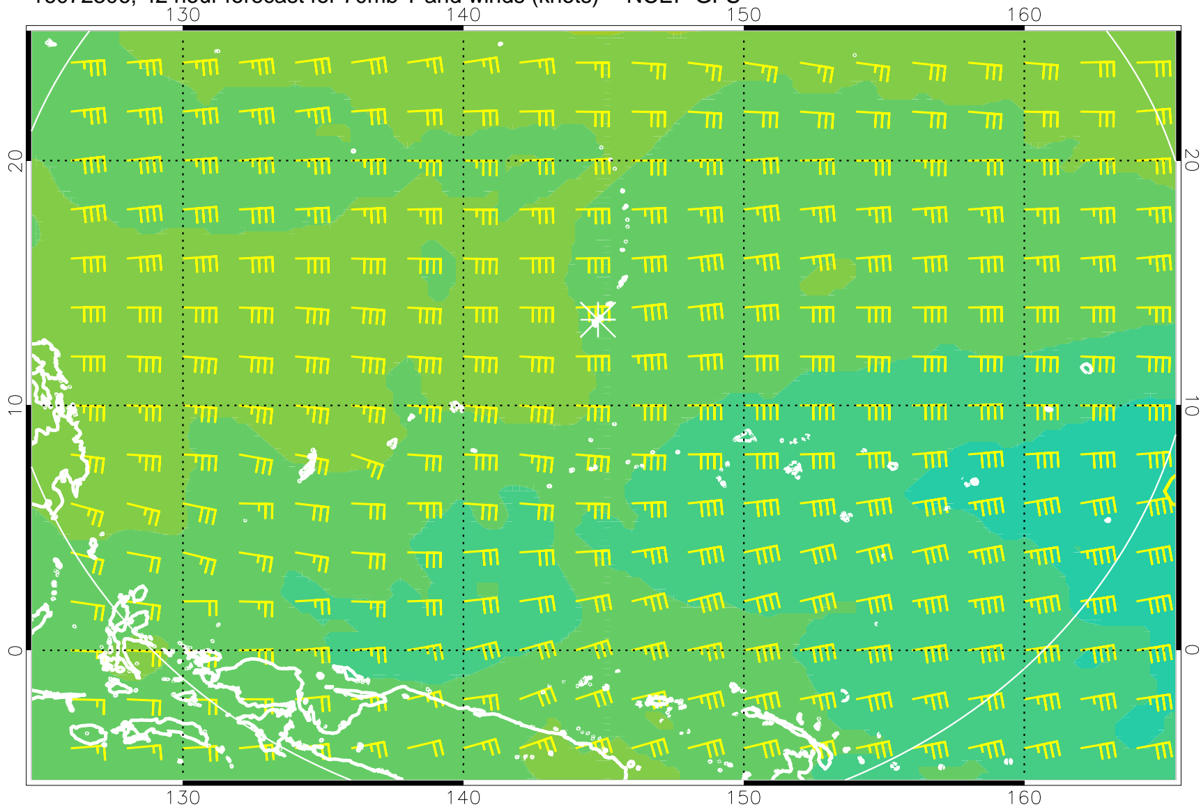
16072306, 42 hour forecast for 70mb T and winds (knots) -- NCEP GFS
