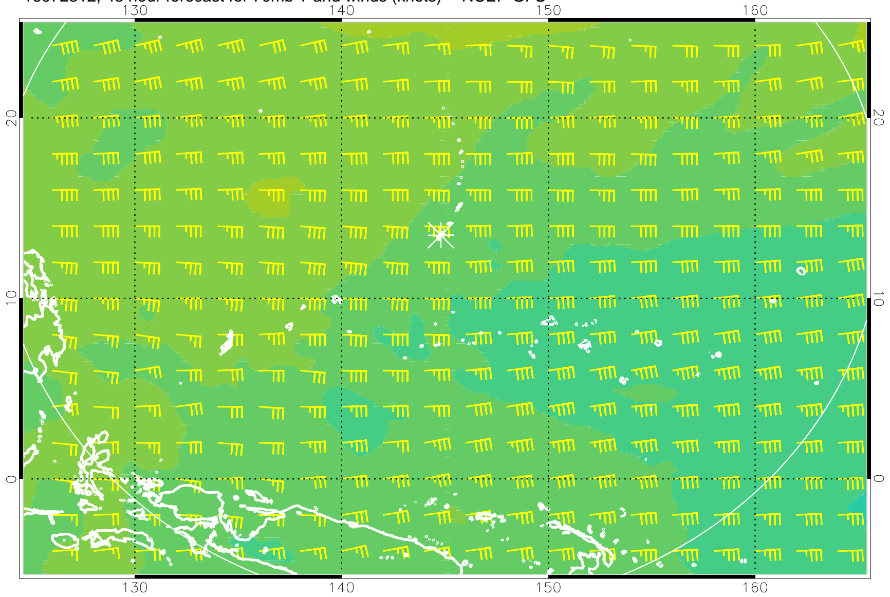
16072312, 48 hour forecast for 70mb T and winds (knots) -- NCEP GFS
