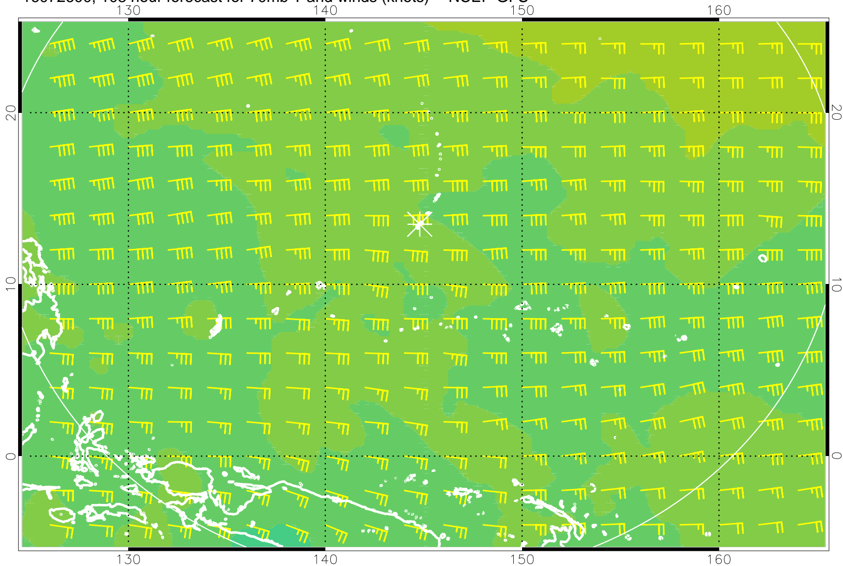
16072600, 108 hour forecast for 70mb T and winds (knots) -- NCEP GFS
