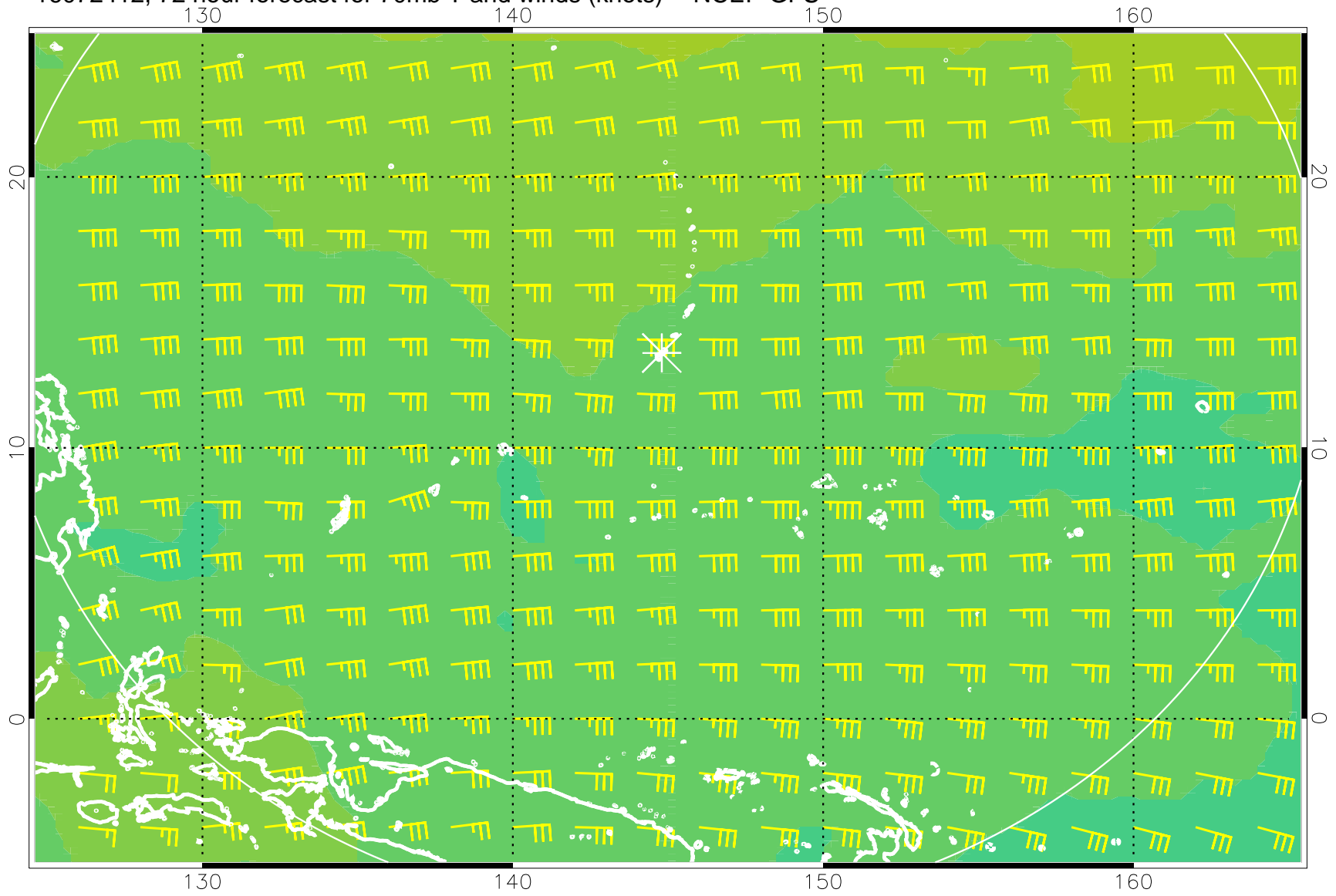
16072412, 72 hour forecast for 70mb T and winds (knots) -- NCEP GFS
