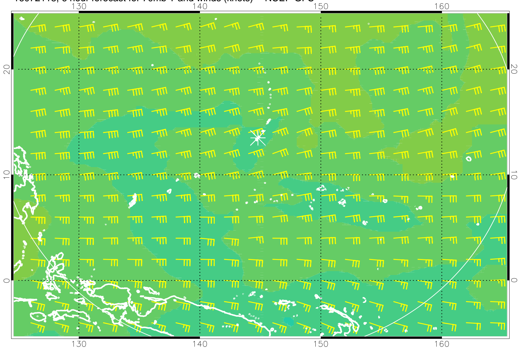
16072118, 6 hour forecast for 70mb T and winds (knots) -- NCEP GFS
