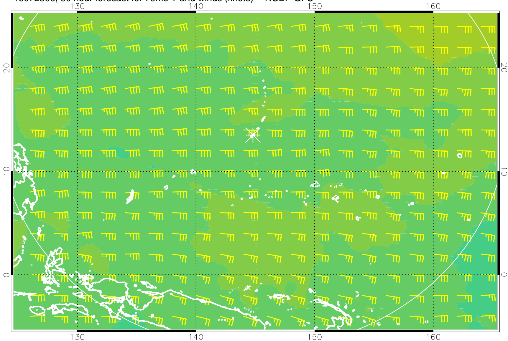
16072506, 90 hour forecast for 70mb T and winds (knots) -- NCEP GFS
