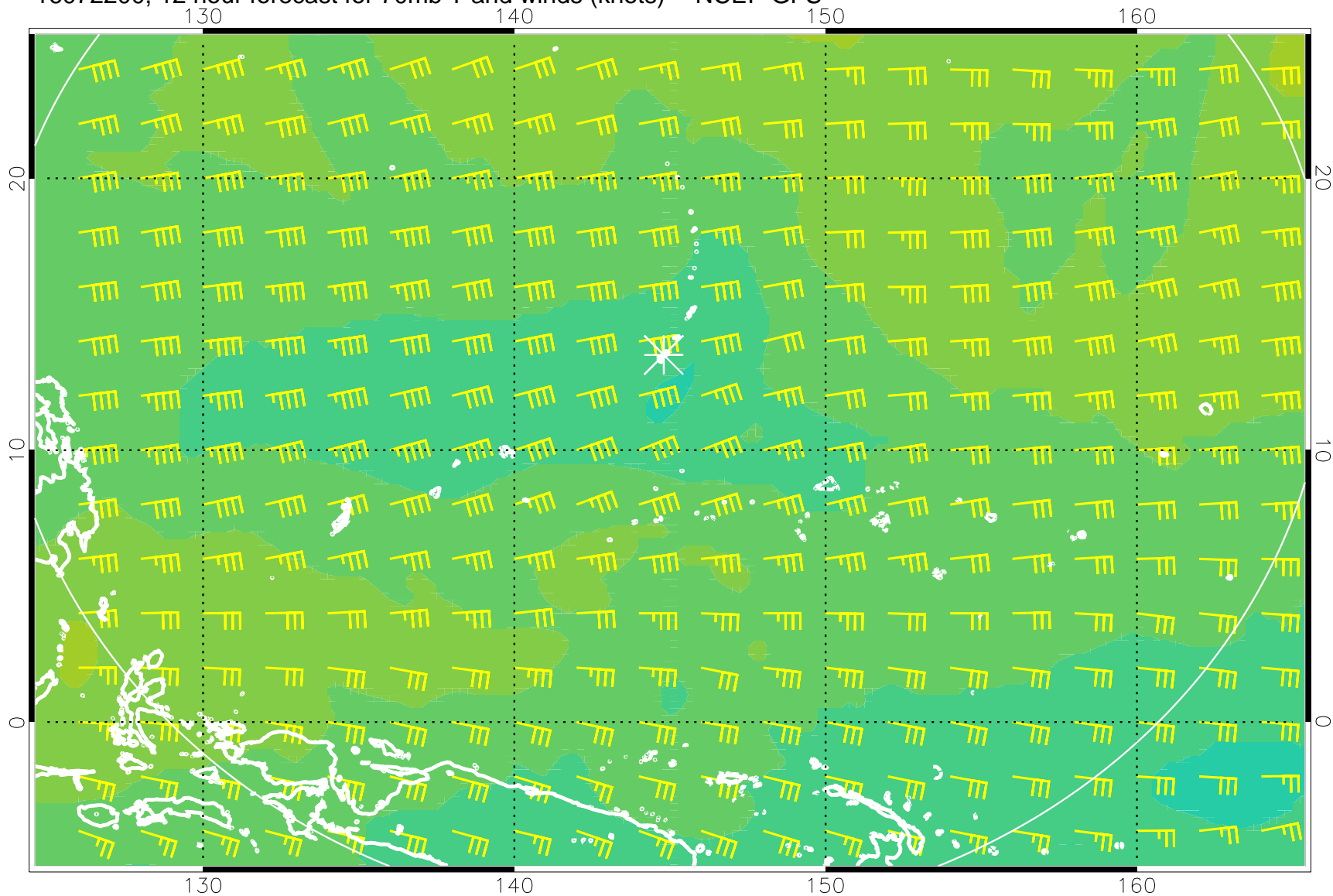
16072200, 12 hour forecast for 70mb T and winds (knots) -- NCEP GFS
