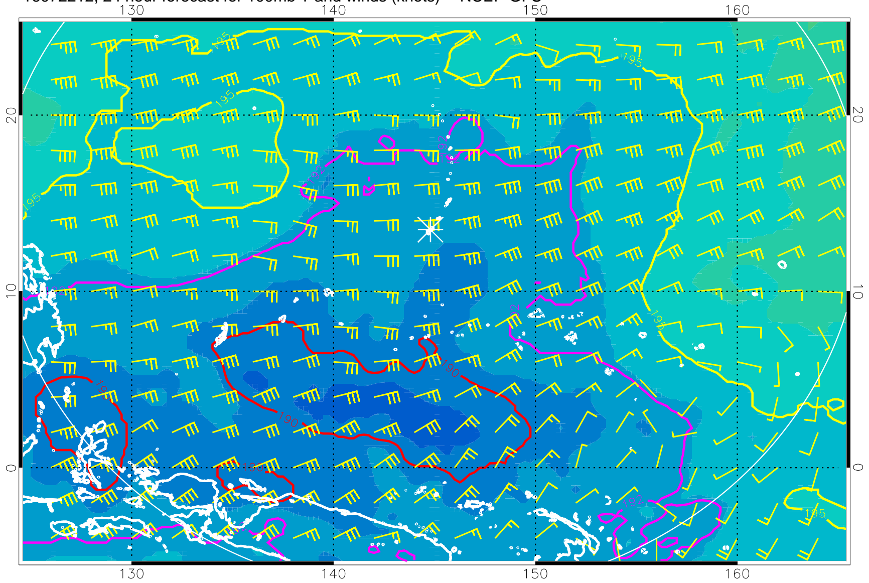
16072212, 24 hour forecast for 100mb T and winds (knots) -- NCEP GFS
