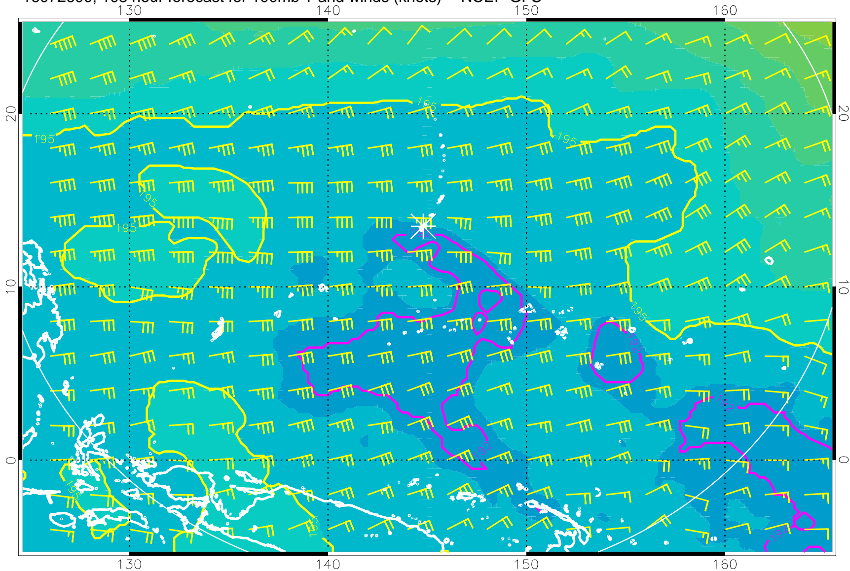
16072600, 108 hour forecast for 100mb T and winds (knots) -- NCEP GFS
