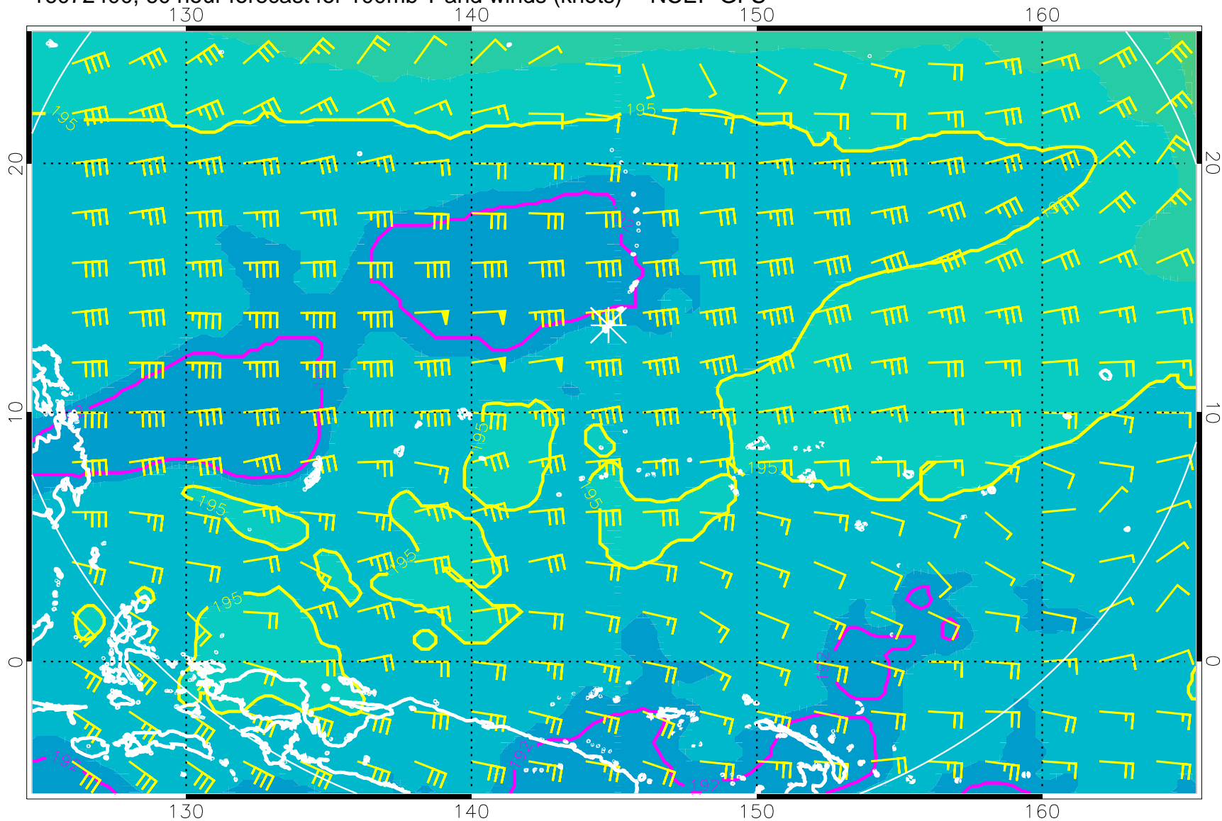
16072400, 60 hour forecast for 100mb T and winds (knots) -- NCEP GFS
