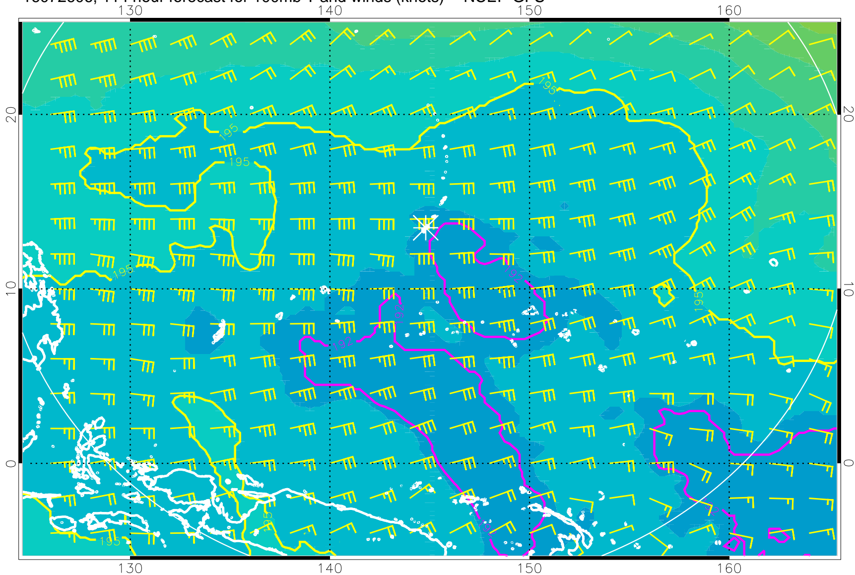
16072606, 114 hour forecast for 100mb T and winds (knots) -- NCEP GFS
