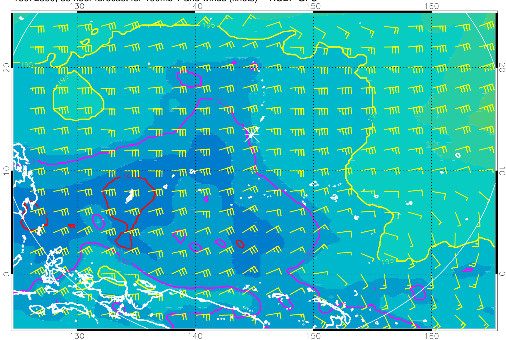
16072300, 36 hour forecast for 100mb T and winds (knots) -- NCEP GFS
