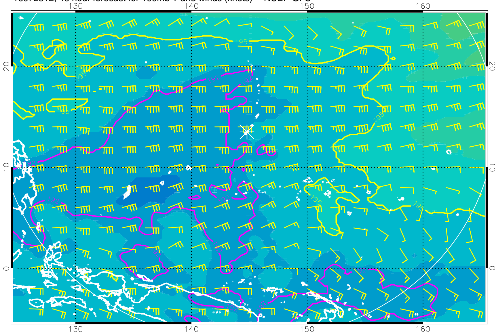
16072312, 48 hour forecast for 100mb T and winds (knots) -- NCEP GFS
