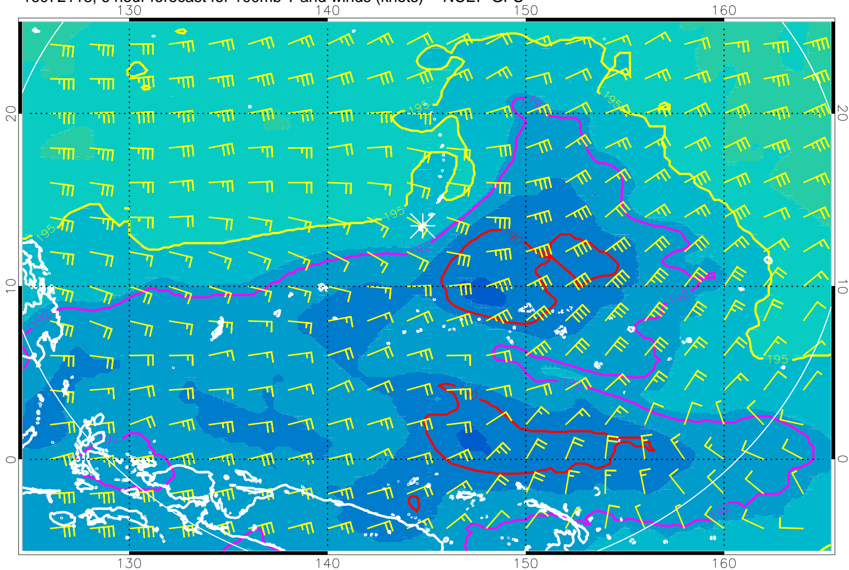
16072118, 6 hour forecast for 100mb T and winds (knots) -- NCEP GFS
