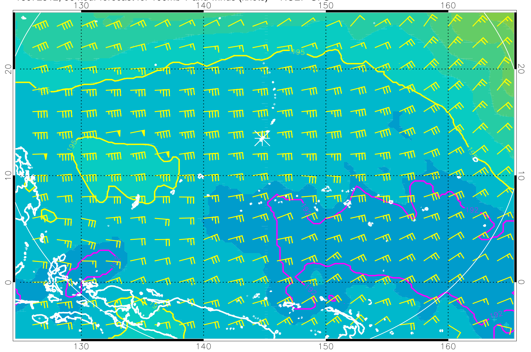
16072512, 96 hour forecast for 100mb T and winds (knots) -- NCEP GFS
