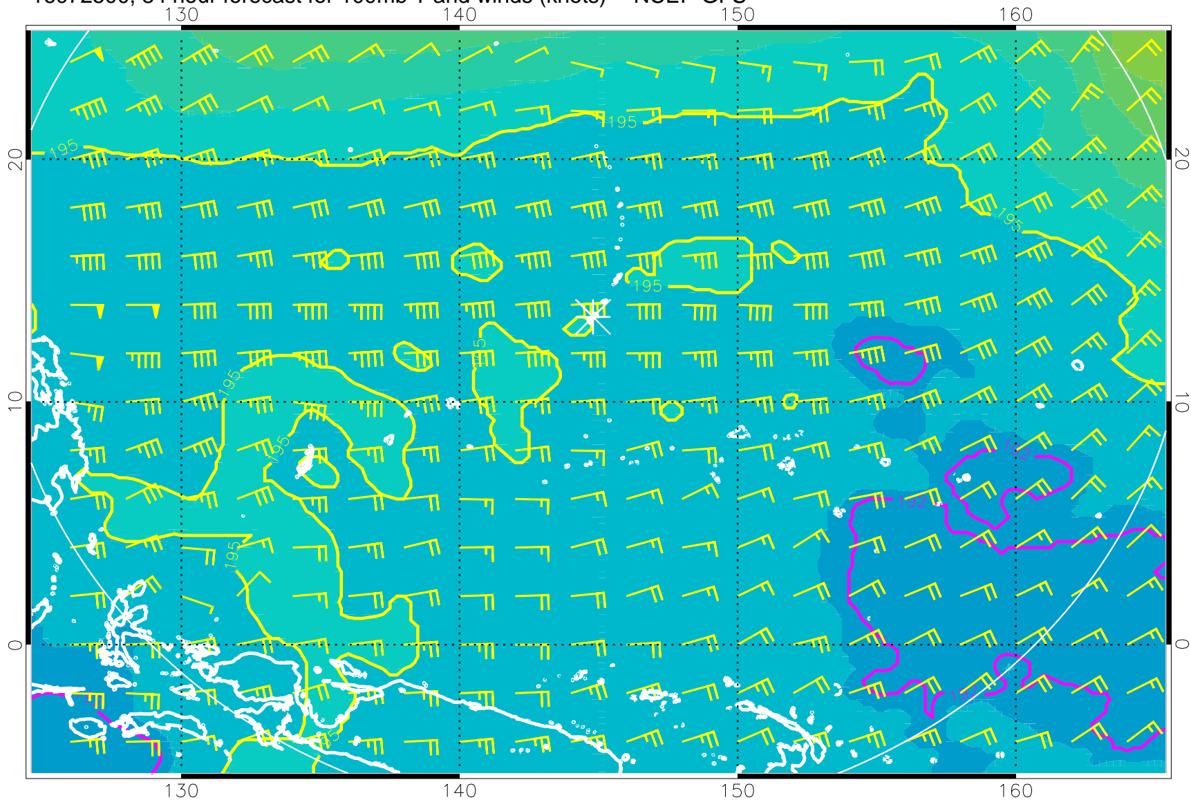
16072500, 84 hour forecast for 100mb T and winds (knots) -- NCEP GFS
