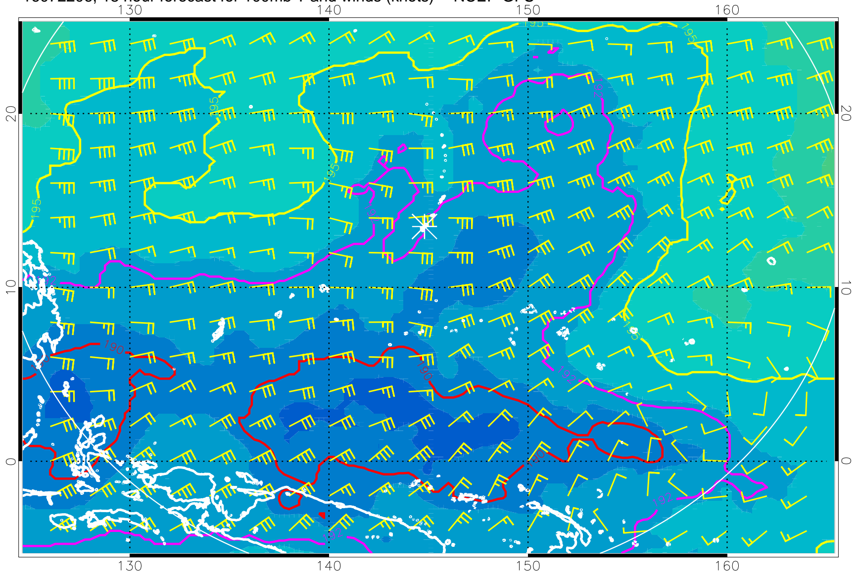
16072206, 18 hour forecast for 100mb T and winds (knots) -- NCEP GFS
