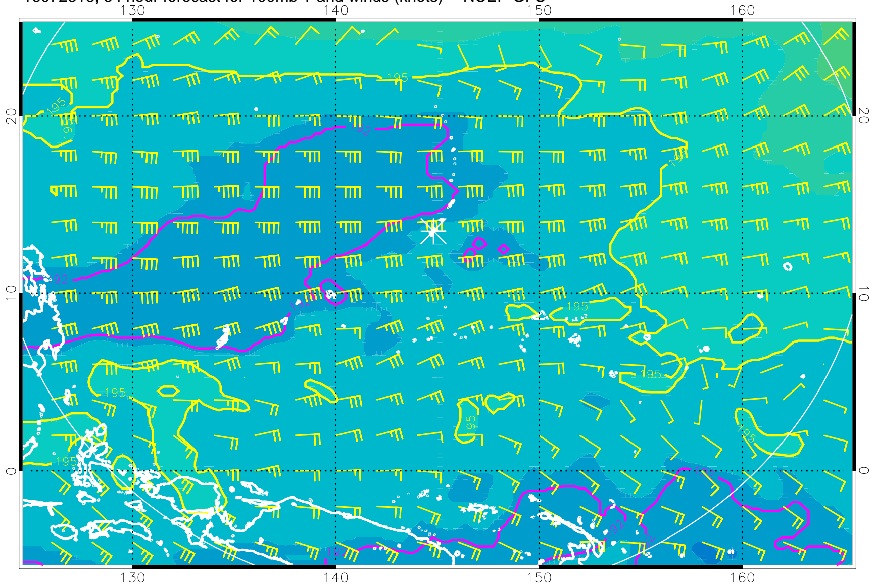
16072318, 54 hour forecast for 100mb T and winds (knots) -- NCEP GFS
