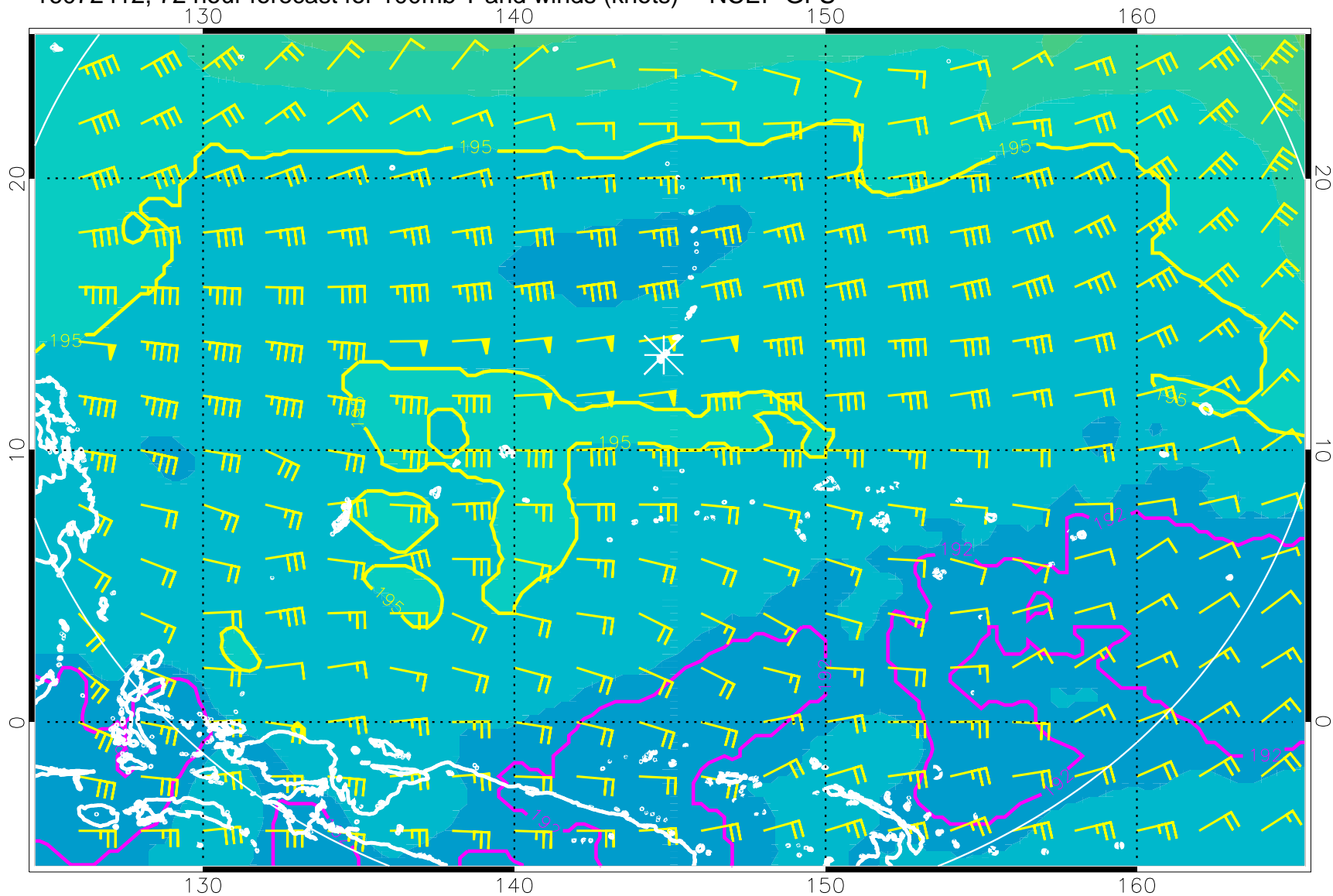
16072412, 72 hour forecast for 100mb T and winds (knots) -- NCEP GFS
