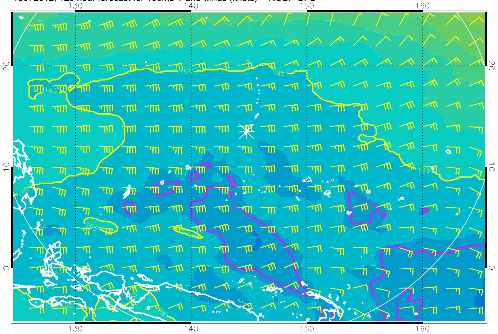
16072612, 120 hour forecast for 100mb T and winds (knots) -- NCEP GFS
