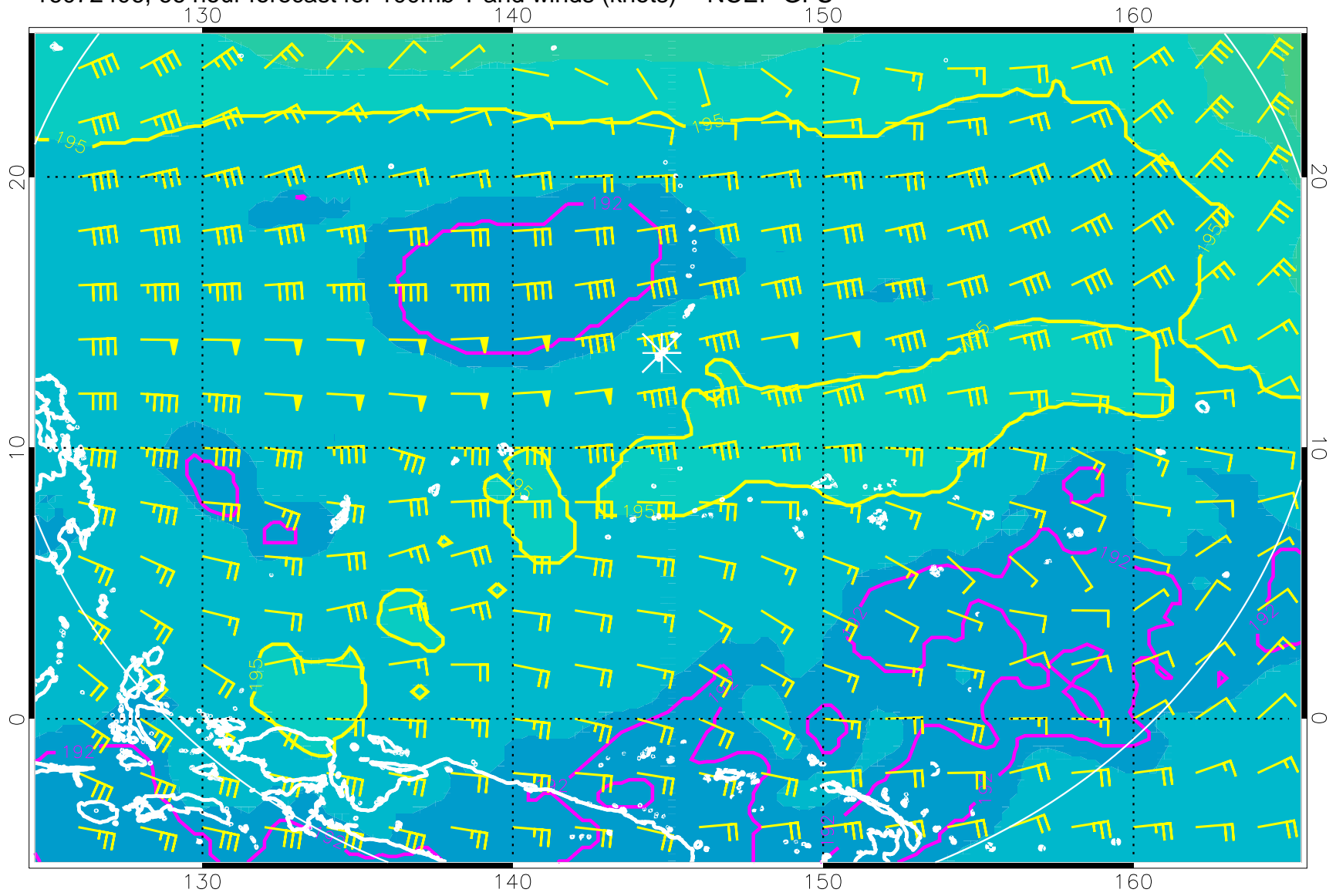
16072406, 66 hour forecast for 100mb T and winds (knots) -- NCEP GFS
