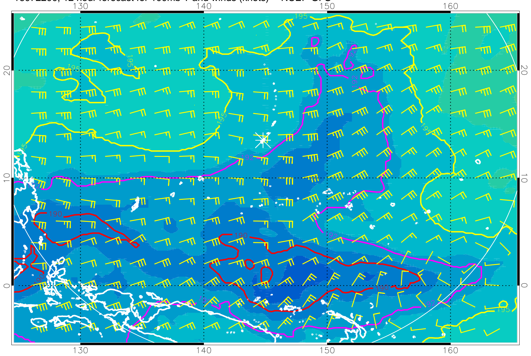
16072200, 12 hour forecast for 100mb T and winds (knots) -- NCEP GFS
