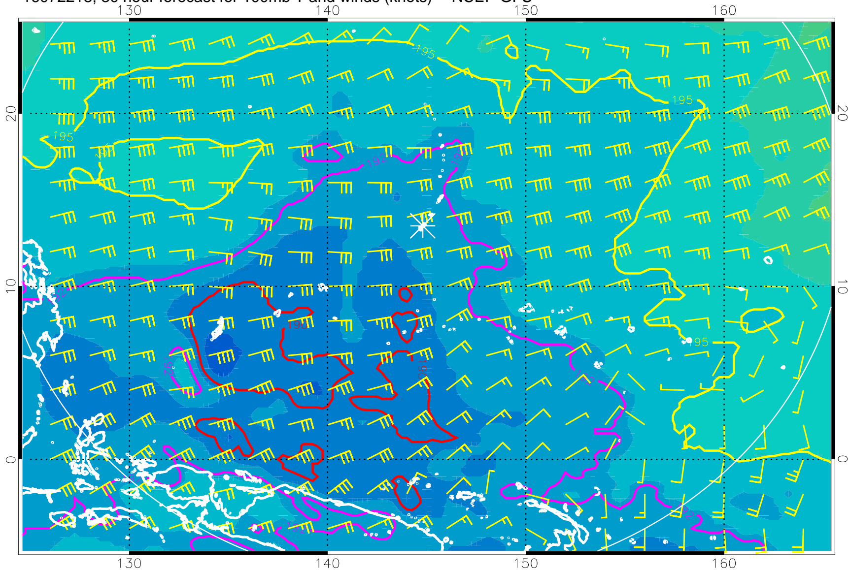
16072218, 30 hour forecast for 100mb T and winds (knots) -- NCEP GFS
