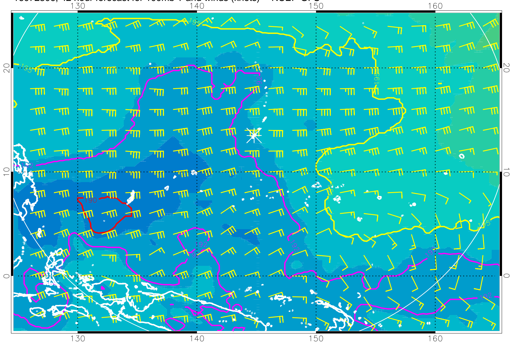
16072306, 42 hour forecast for 100mb T and winds (knots) -- NCEP GFS
