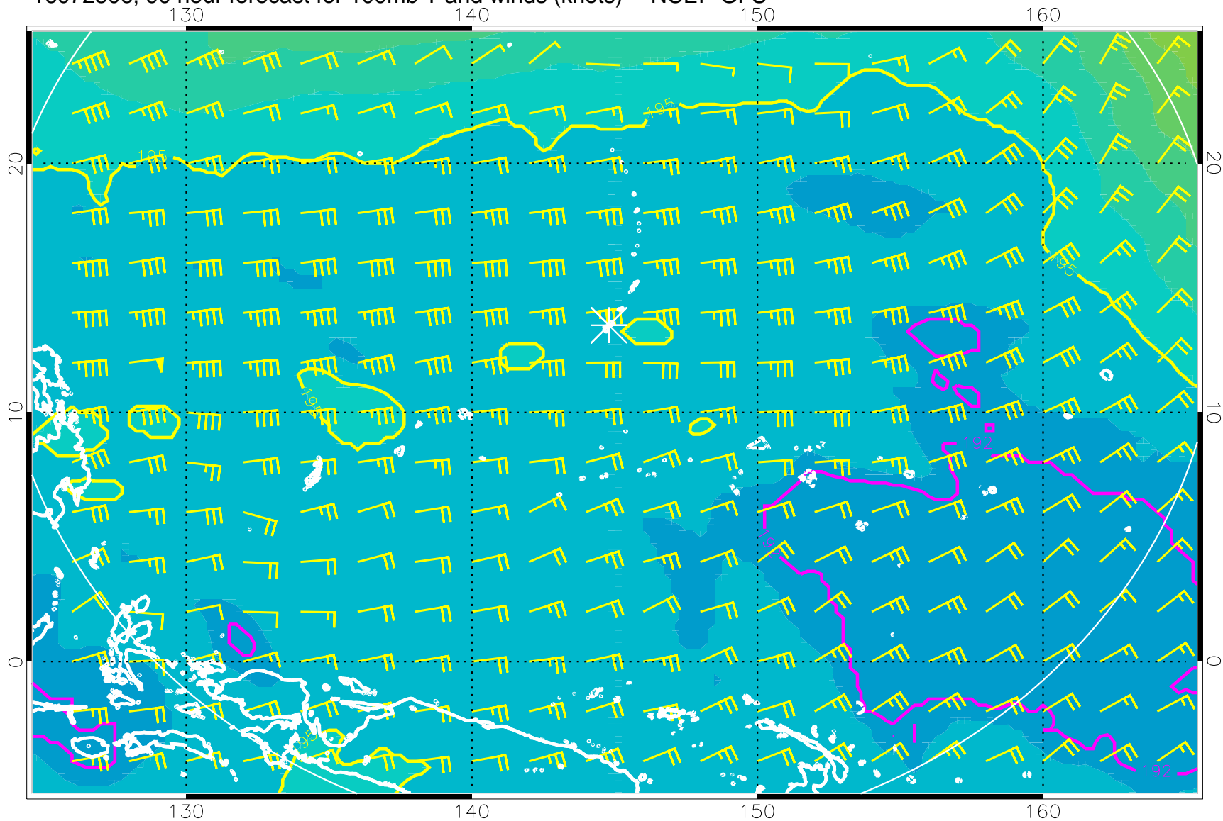
16072506, 90 hour forecast for 100mb T and winds (knots) -- NCEP GFS
