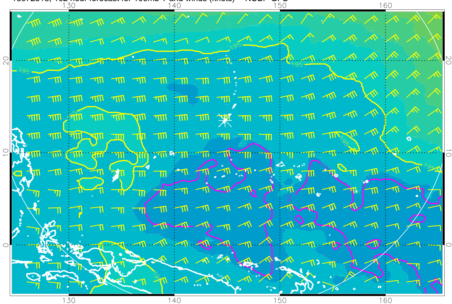
16072518, 102 hour forecast for 100mb T and winds (knots) -- NCEP GFS
