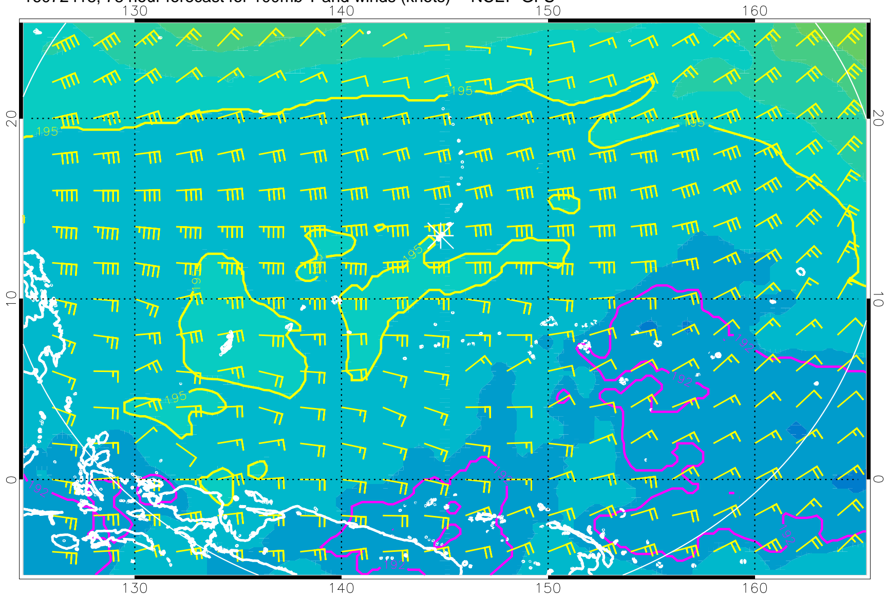
16072418, 78 hour forecast for 100mb T and winds (knots) -- NCEP GFS
