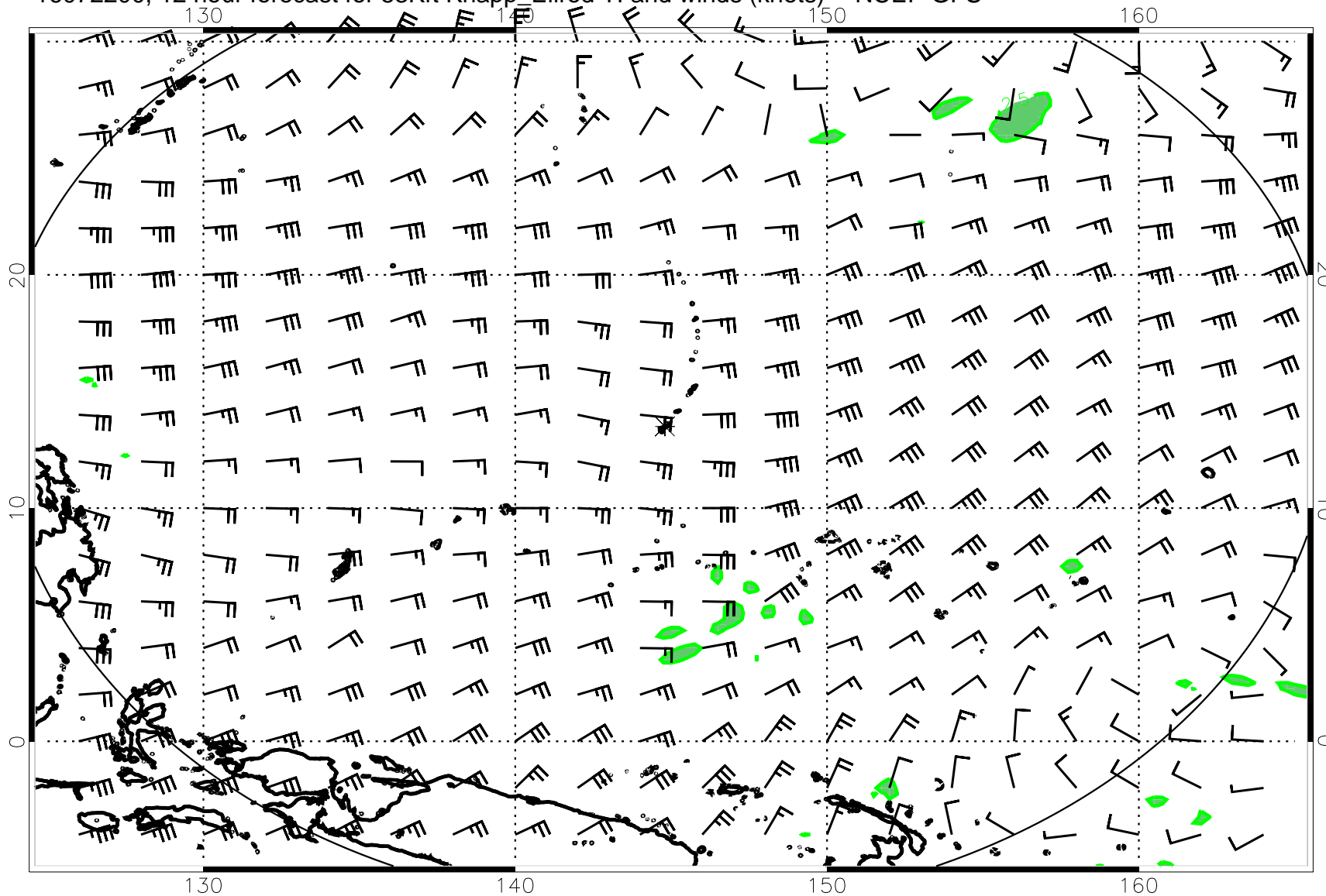
16072200, 12 hour forecast for 53Kft Knapp_Ellrod TI and winds (knots) -- NCEP GFS
