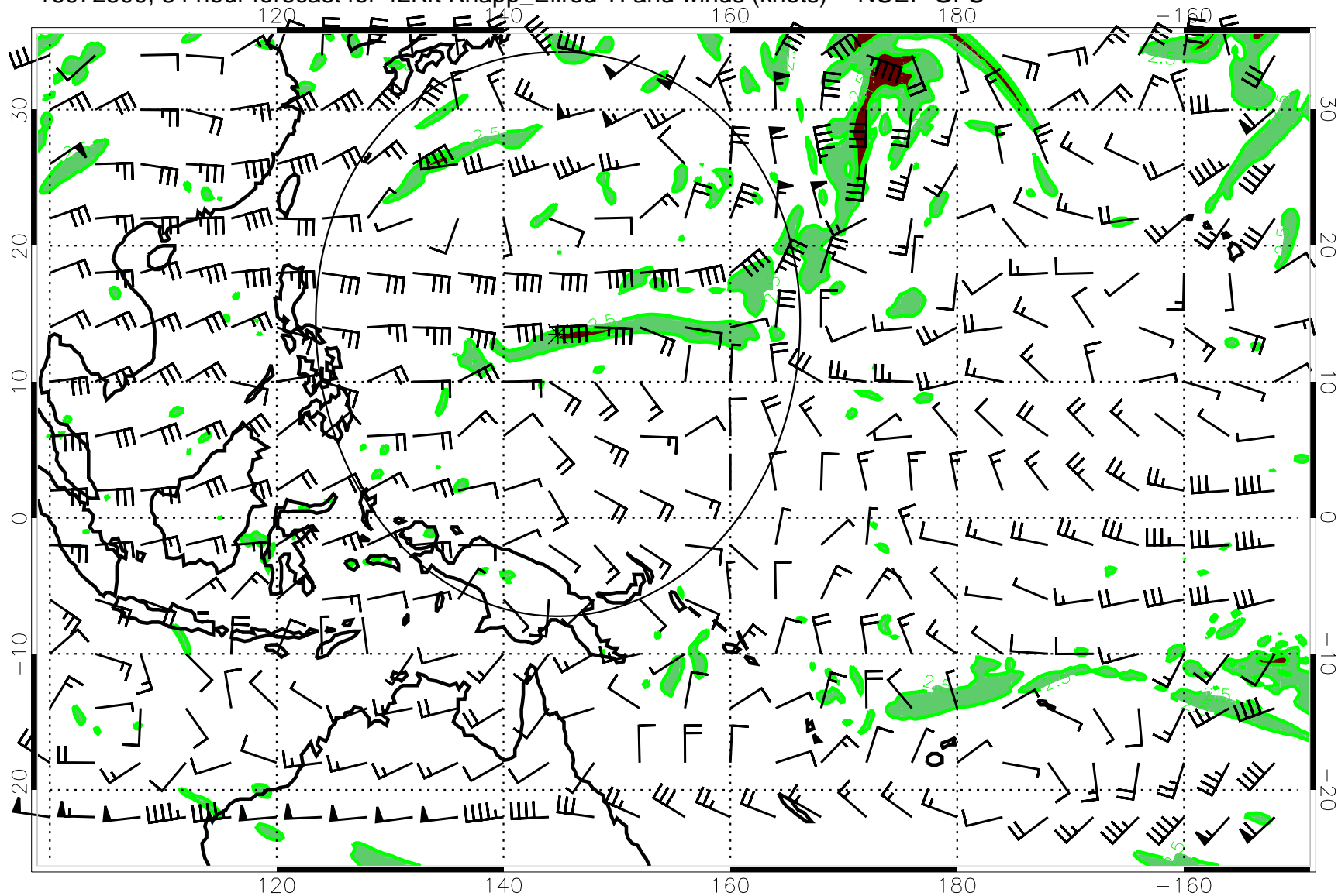
16072500, 84 hour forecast for 42Kft Knapp_Ellrod TI and winds (knots) -- NCEP GFS
