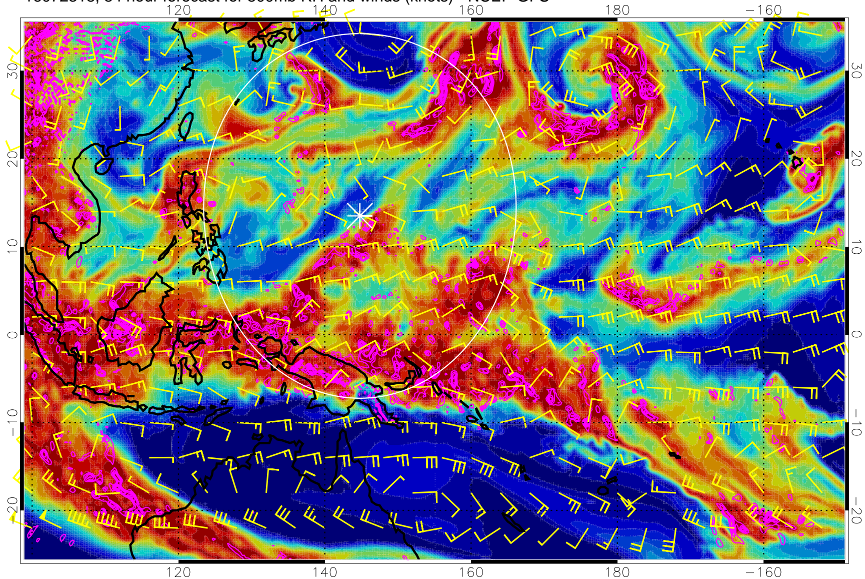
16072318, 54 hour forecast for 500mb RH and winds (knots) - NCEP GFS
