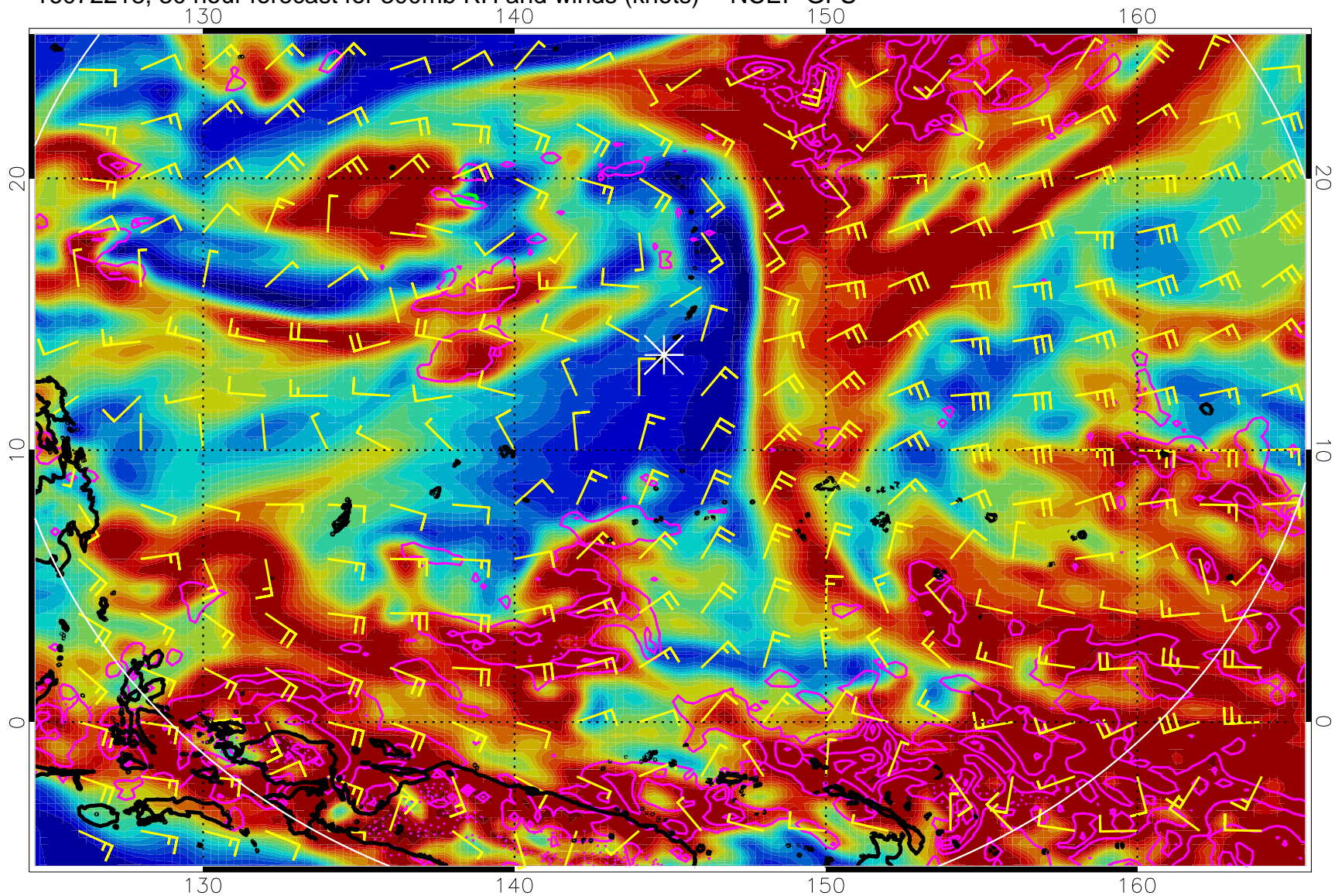
16072218, 30 hour forecast for 300mb RH and winds (knots) -- NCEP GFS
