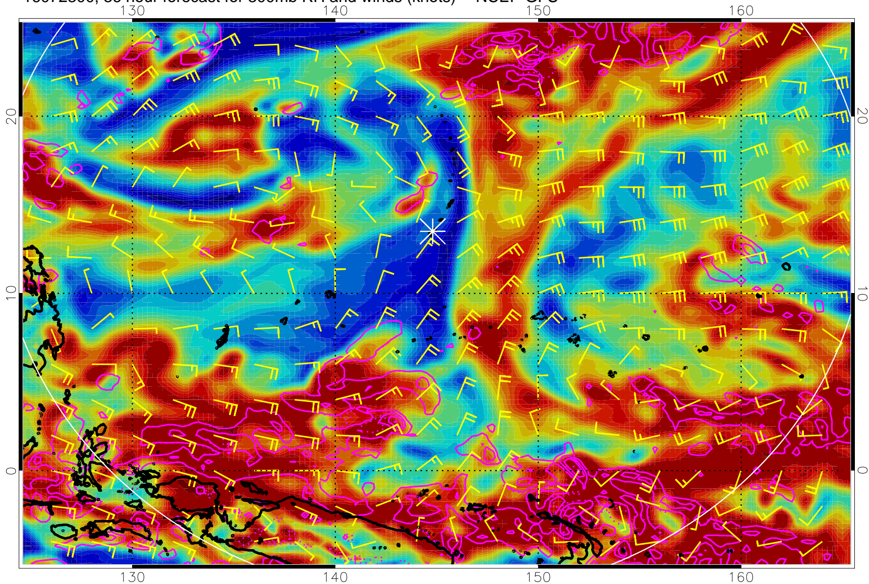
16072300, 36 hour forecast for 300mb RH and winds (knots) -- NCEP GFS
