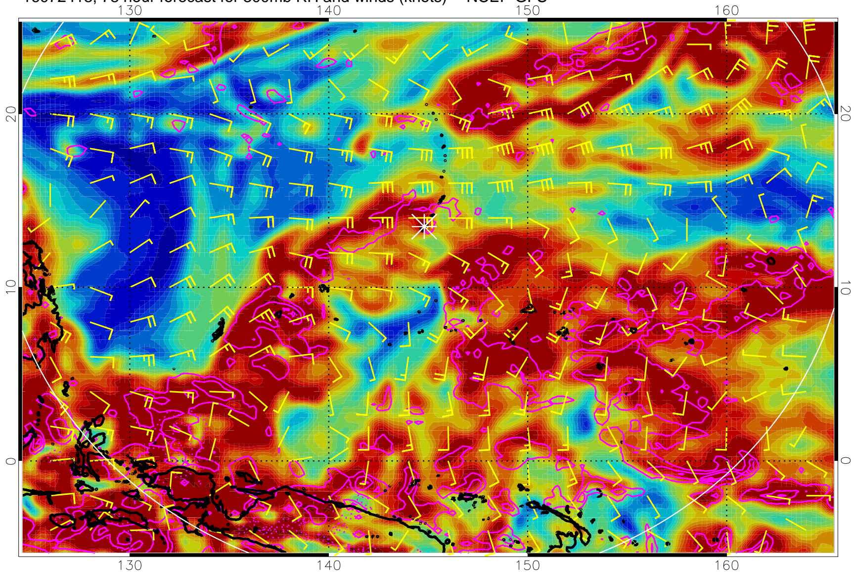
16072418, 78 hour forecast for 300mb RH and winds (knots) -- NCEP GFS
