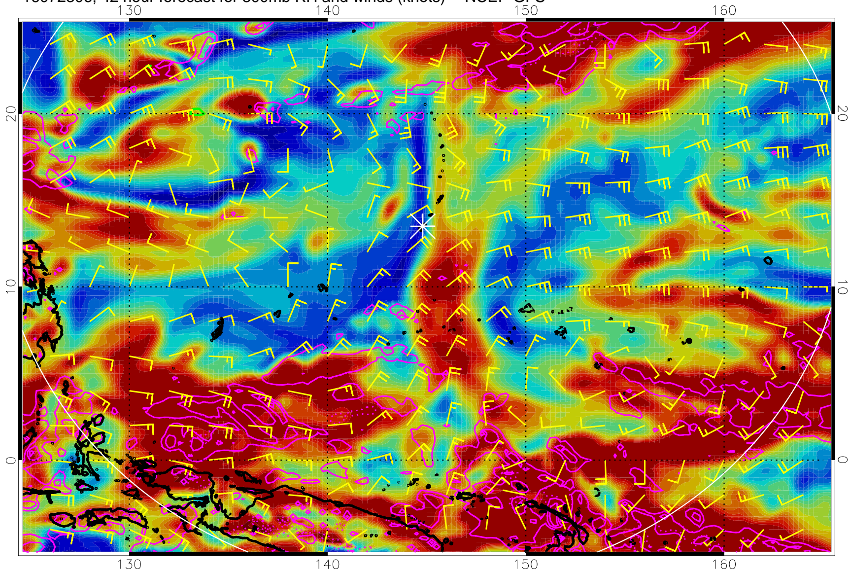
16072306, 42 hour forecast for 300mb RH and winds (knots) -- NCEP GFS
