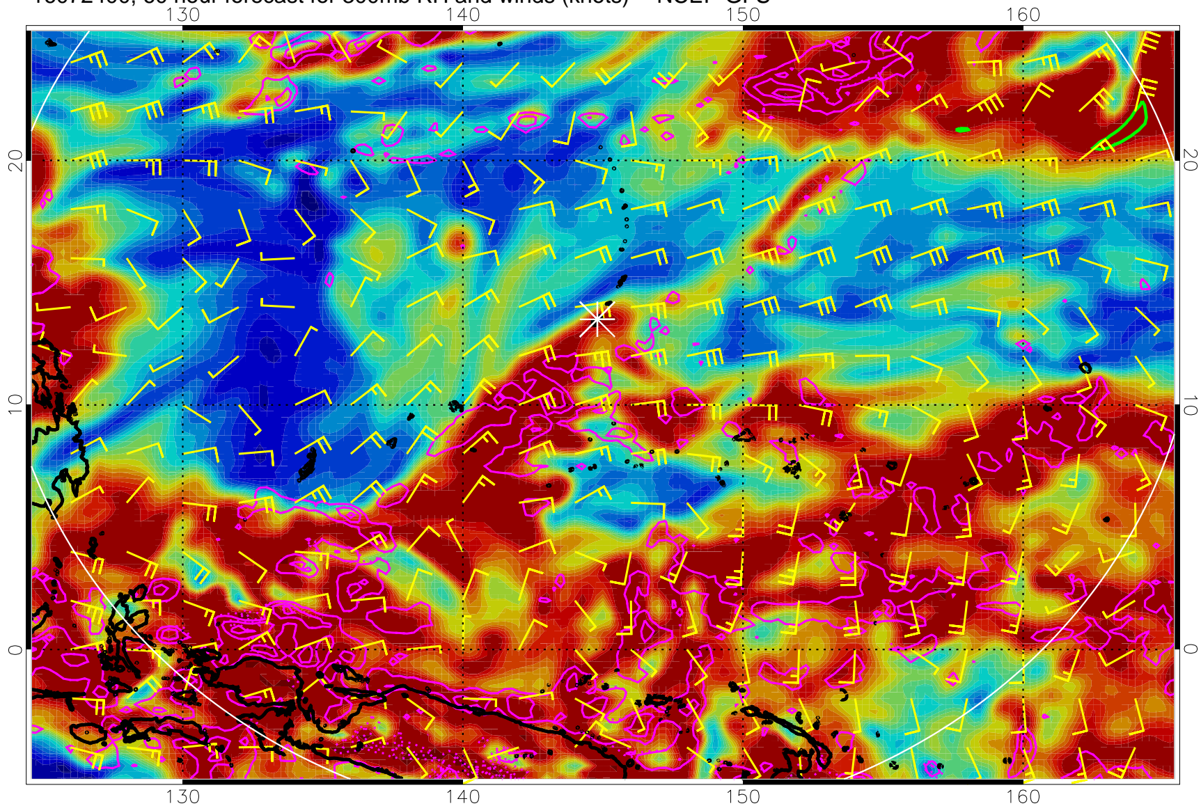
16072400, 60 hour forecast for 300mb RH and winds (knots) -- NCEP GFS
