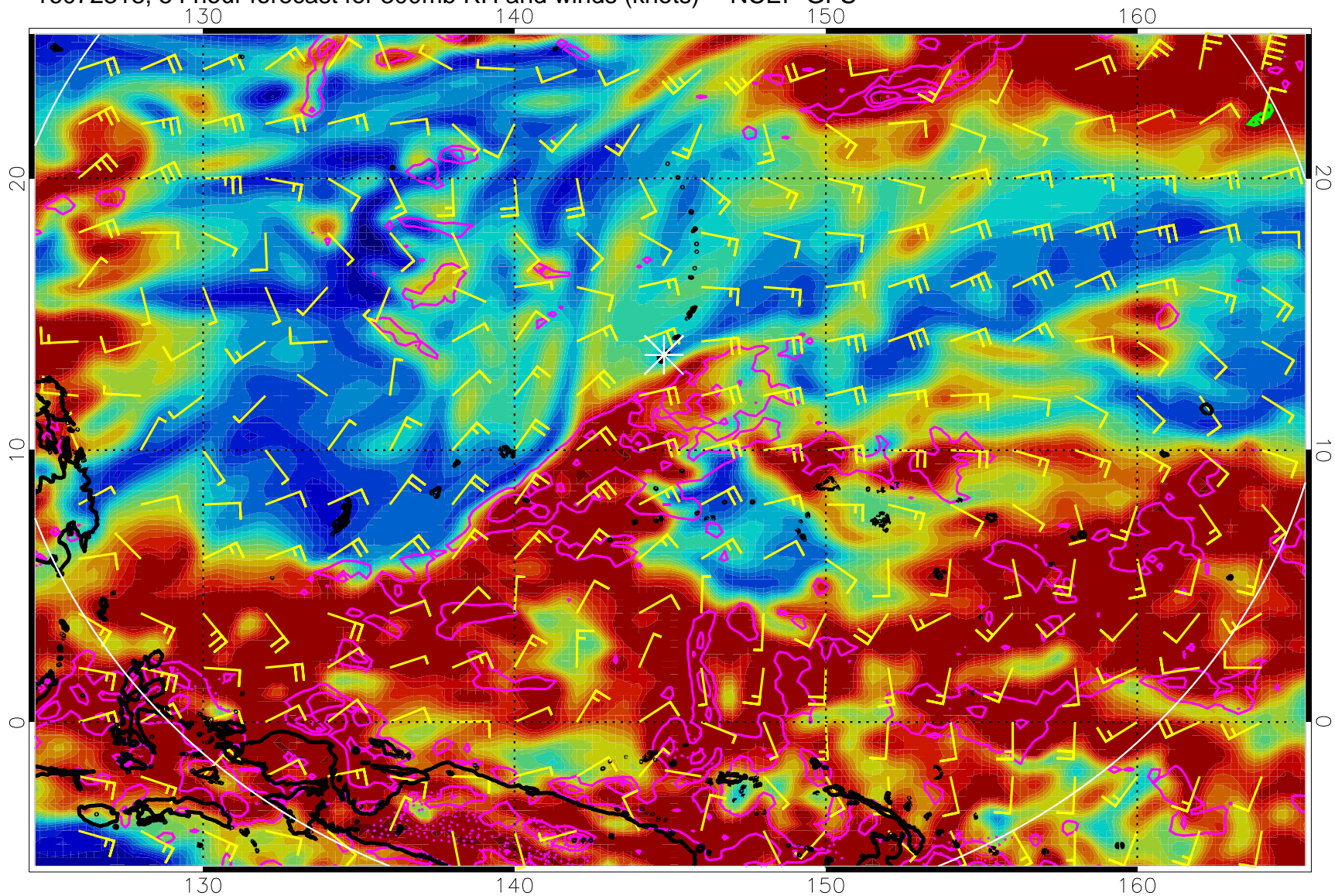
16072318, 54 hour forecast for 300mb RH and winds (knots) -- NCEP GFS
