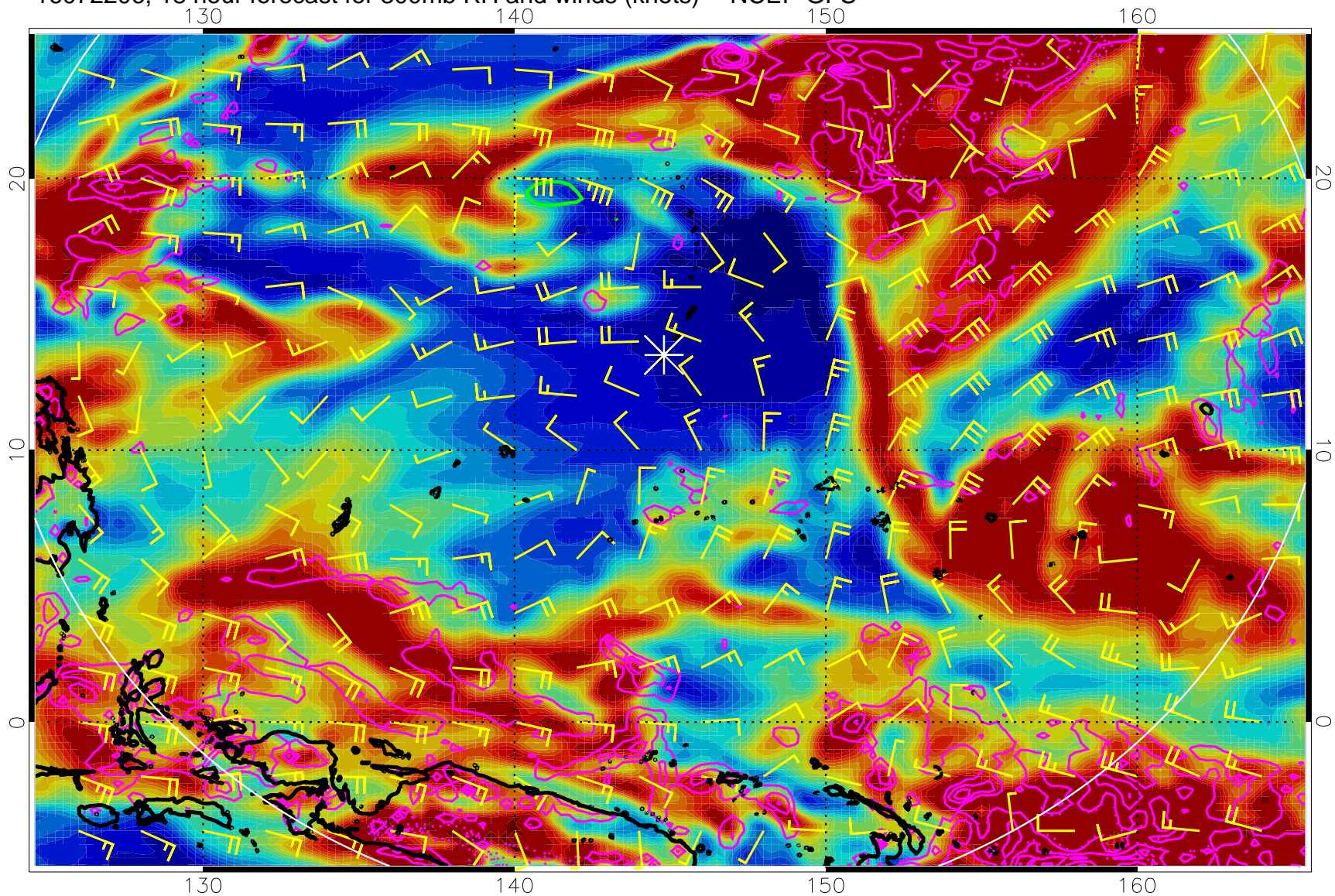
16072206, 18 hour forecast for 300mb RH and winds (knots) -- NCEP GFS
