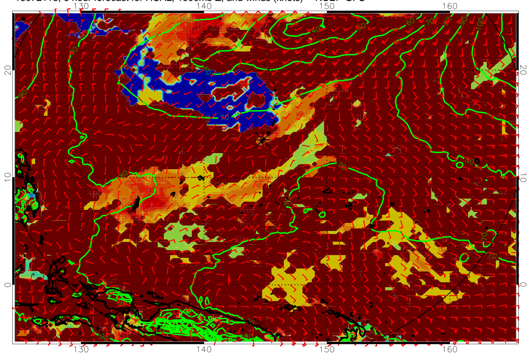
16072118, 6 hour forecast for HCAL, 1000mb Z, and winds (knots) -- NCEP GFS
