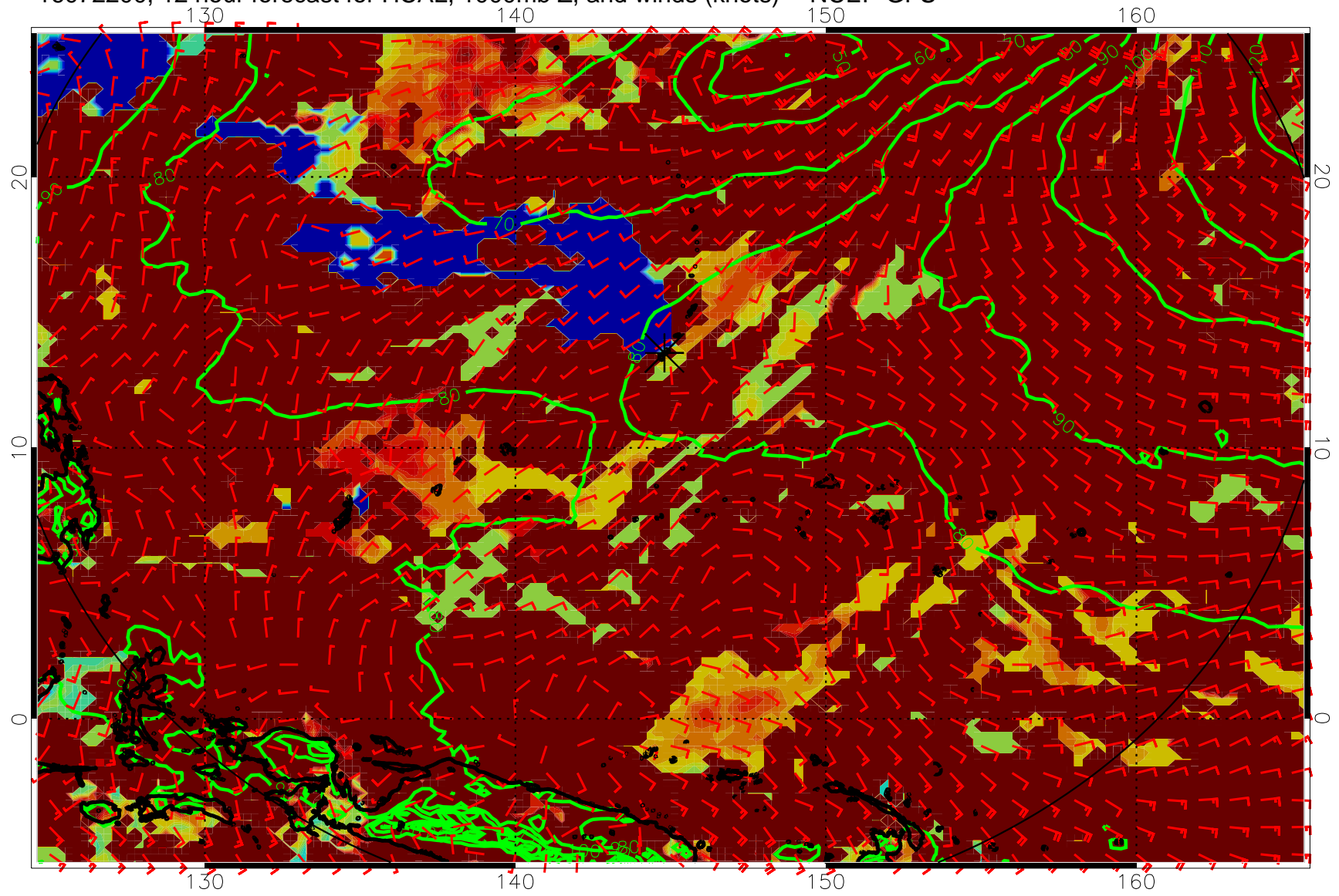
16072200, 12 hour forecast for HCAL, 1000mb Z, and winds (knots) -- NCEP GFS
