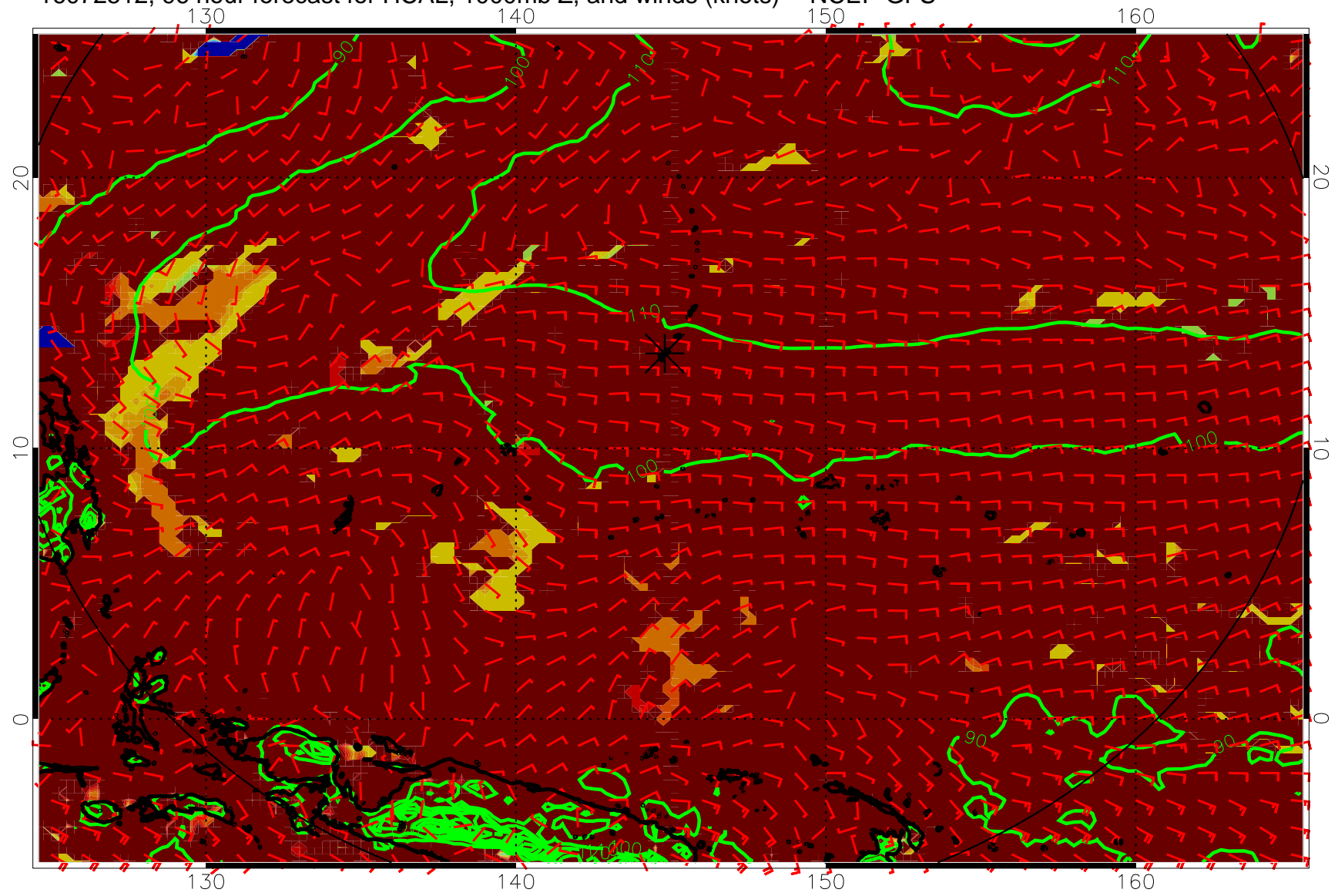
16072512, 96 hour forecast for HCAL, 1000mb Z, and winds (knots) -- NCEP GFS
