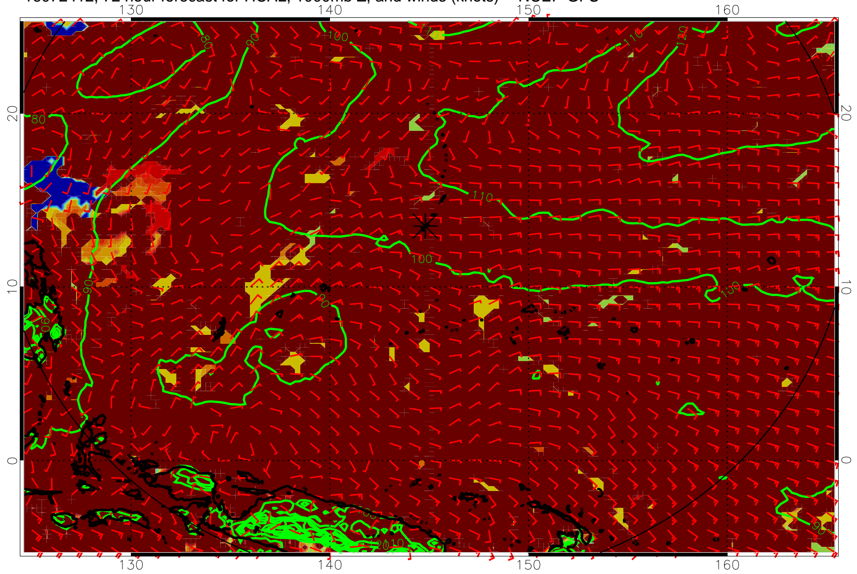
16072412, 72 hour forecast for HCAL, 1000mb Z, and winds (knots) -- NCEP GFS
