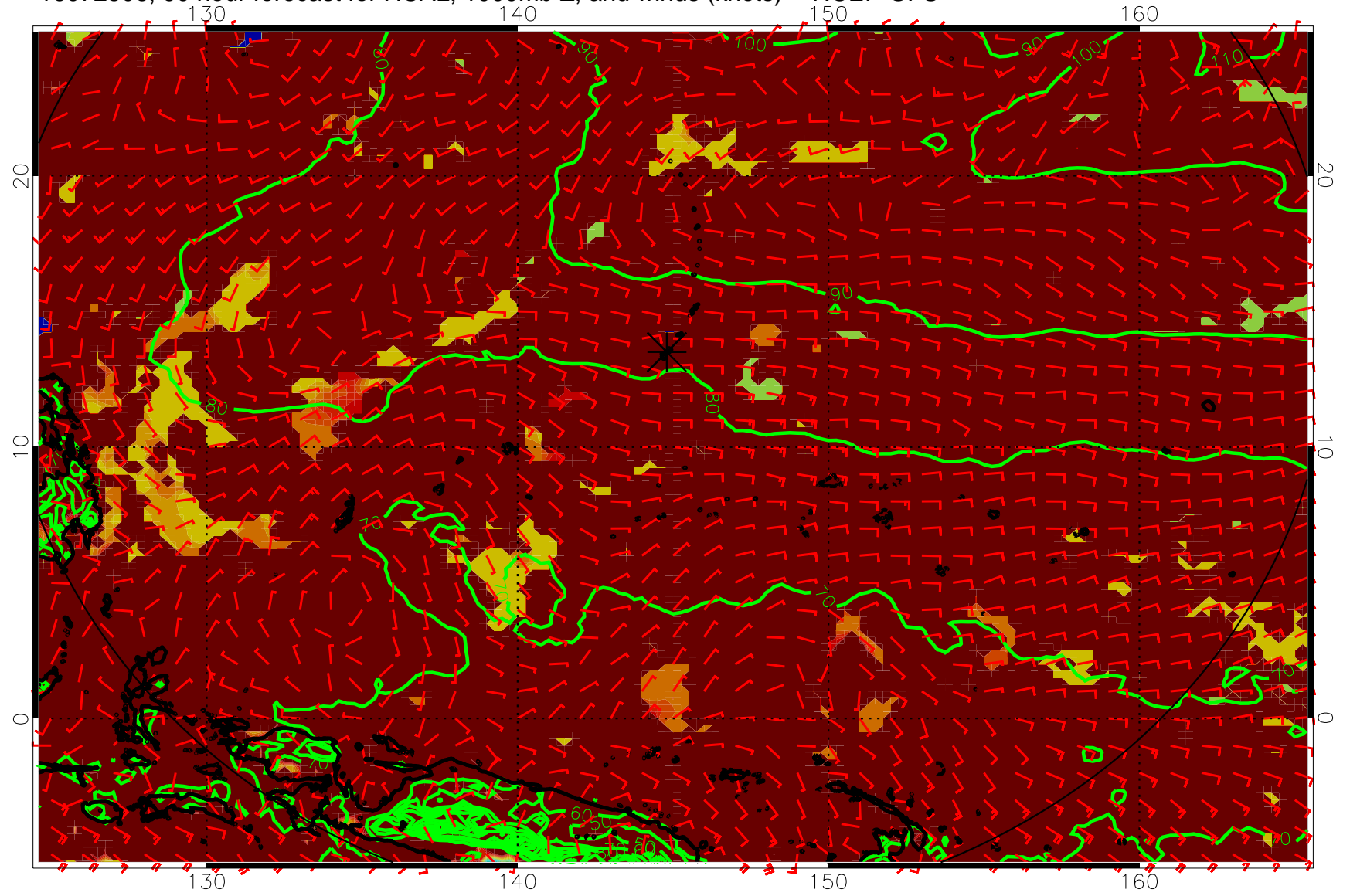
16072506, 90 hour forecast for HCAL, 1000mb Z, and winds (knots) -- NCEP GFS
