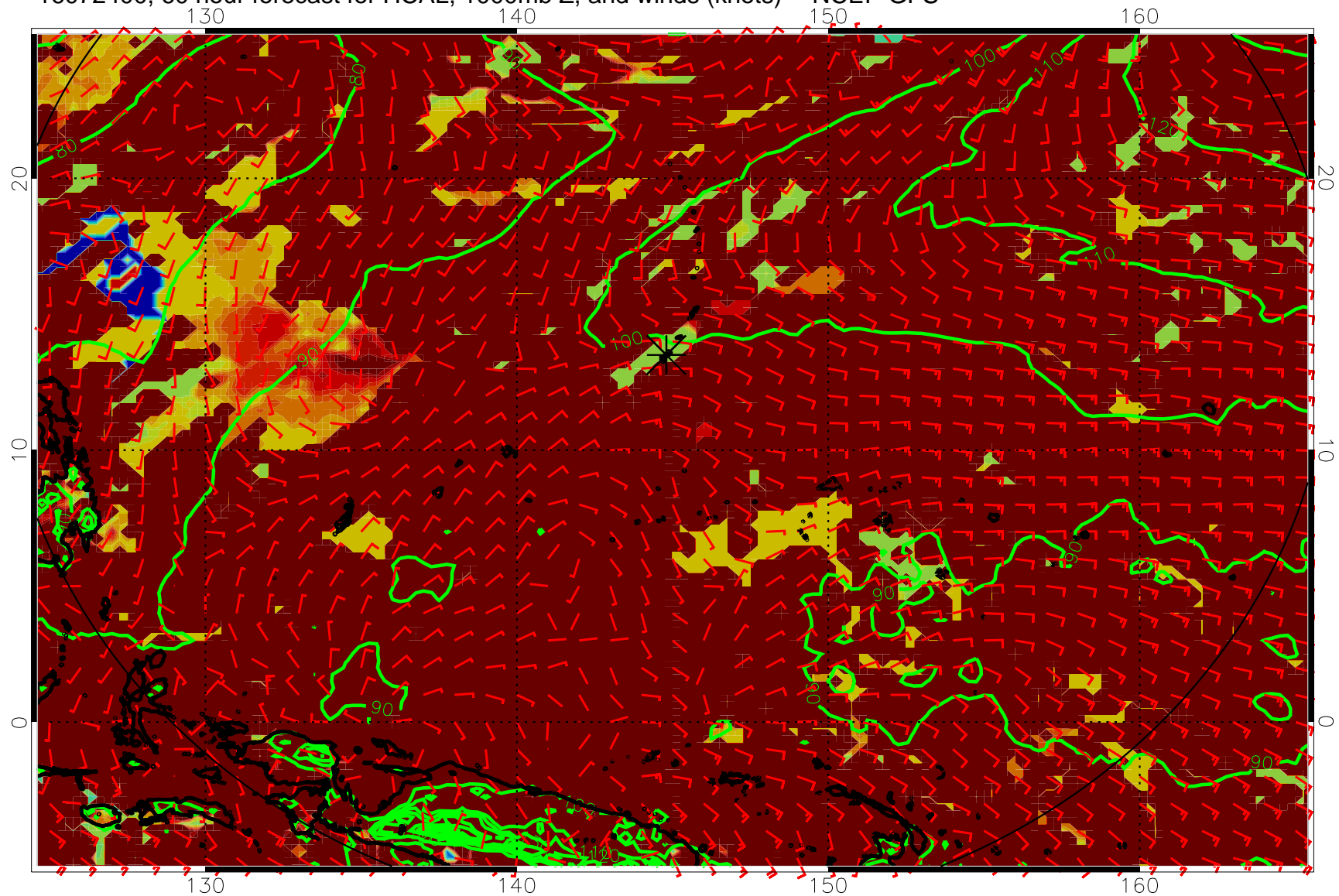
16072400, 60 hour forecast for HCAL, 1000mb Z, and winds (knots) -- NCEP GFS
