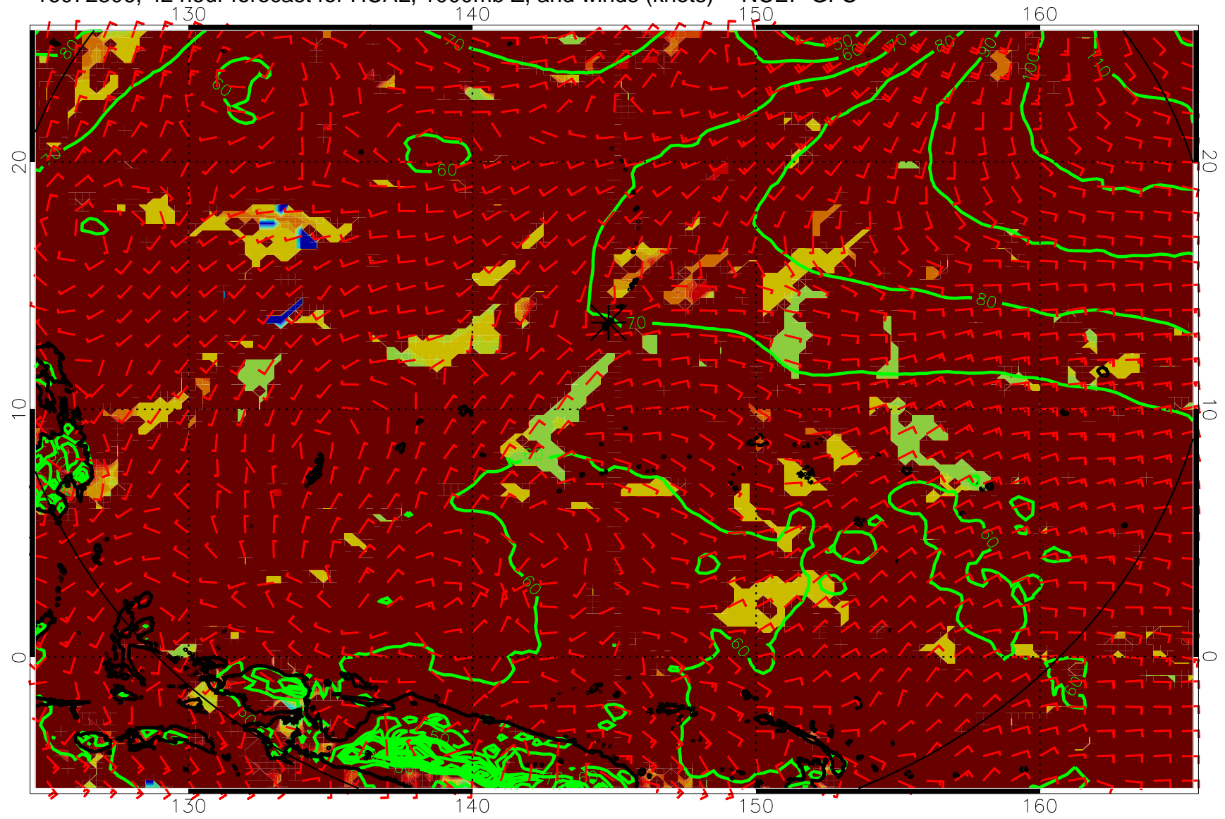
16072306, 42 hour forecast for HCAL, 1000mb Z, and winds (knots) -- NCEP GFS
