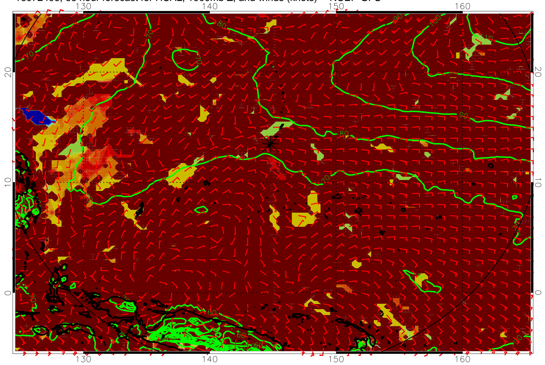
16072406, 66 hour forecast for HCAL, 1000mb Z, and winds (knots) -- NCEP GFS
