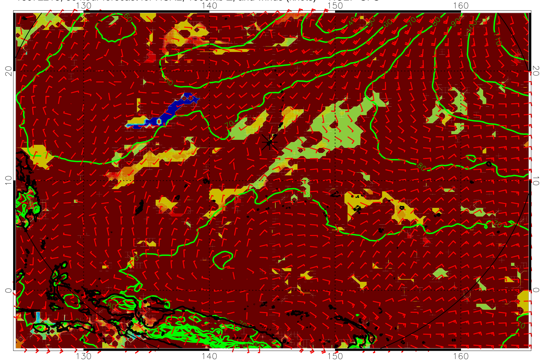
16072218, 30 hour forecast for HCAL, 1000mb Z, and winds (knots) -- NCEP GFS
