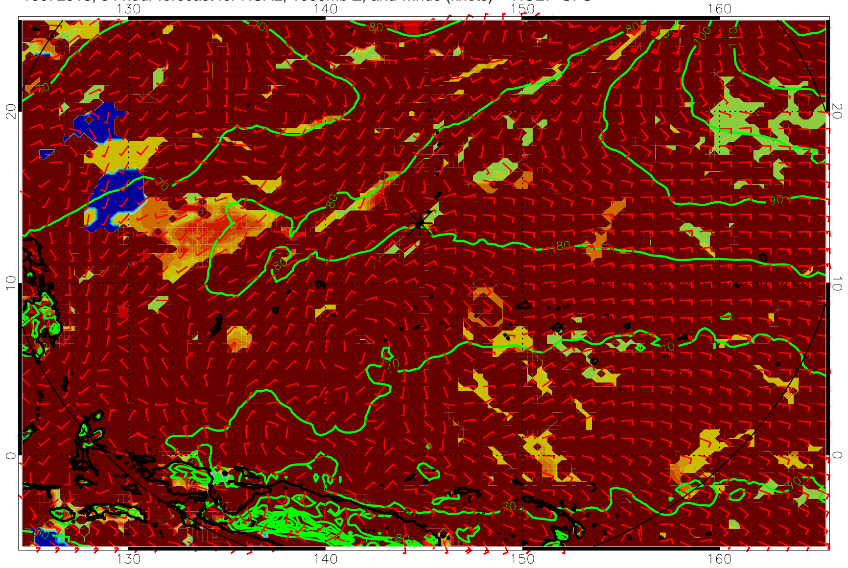
16072318, 54 hour forecast for HCAL, 1000mb Z, and winds (knots) -- NCEP GFS
