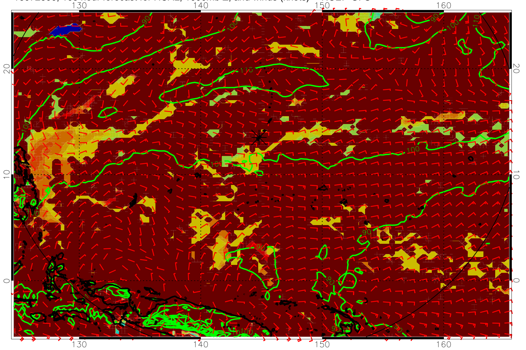
16072600, 108 hour forecast for HCAL, 1000mb Z, and winds (knots) -- NCEP GFS
