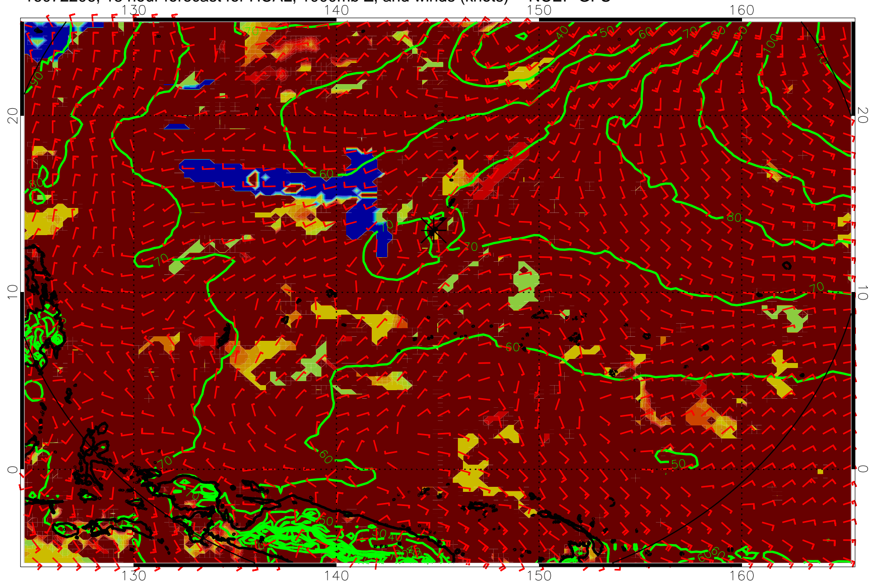
16072206, 18 hour forecast for HCAL, 1000mb Z, and winds (knots) -- NCEP GFS
