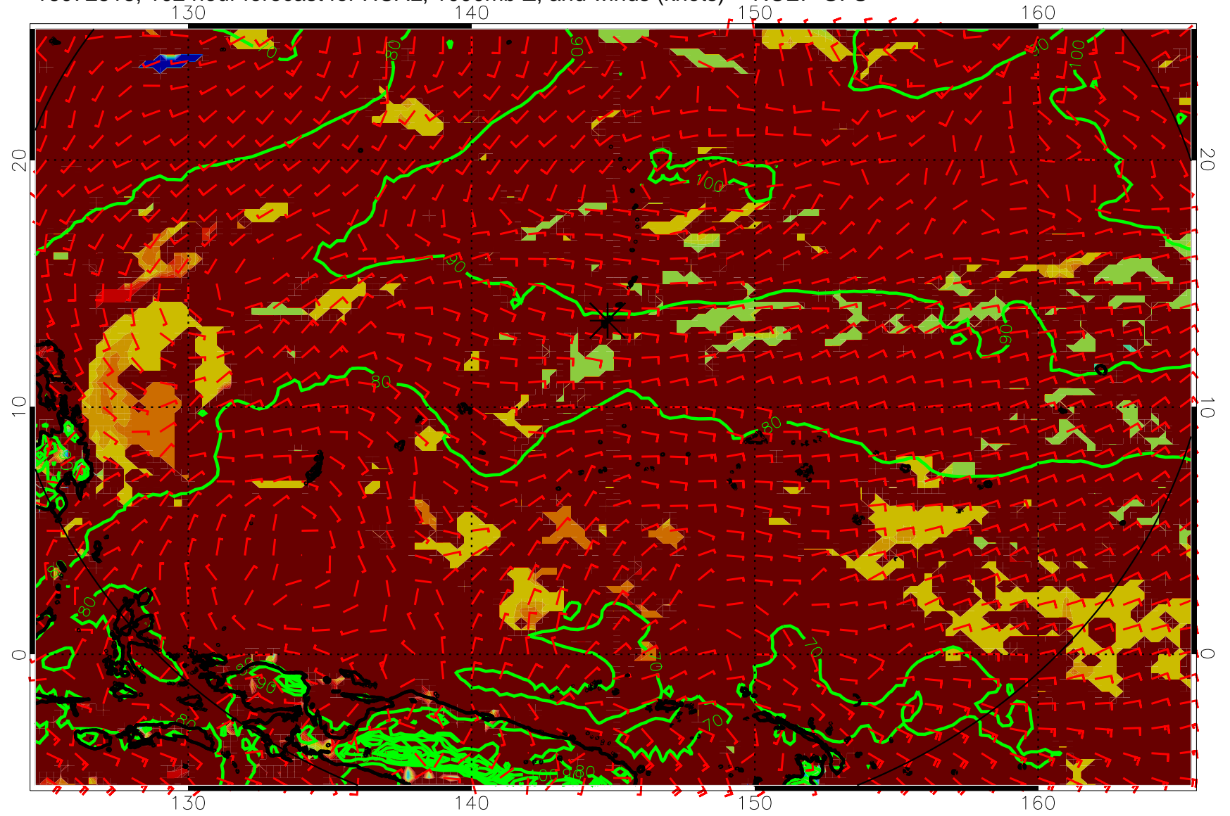
16072518, 102 hour forecast for HCAL, 1000mb Z, and winds (knots) -- NCEP GFS
