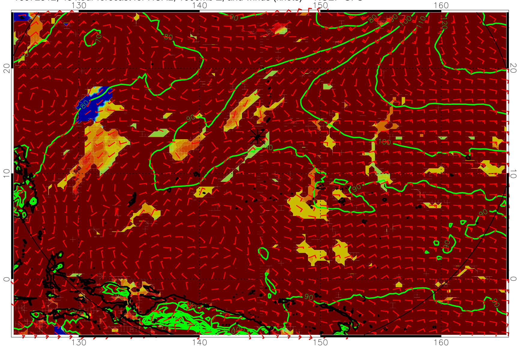
16072312, 48 hour forecast for HCAL, 1000mb Z, and winds (knots) -- NCEP GFS
