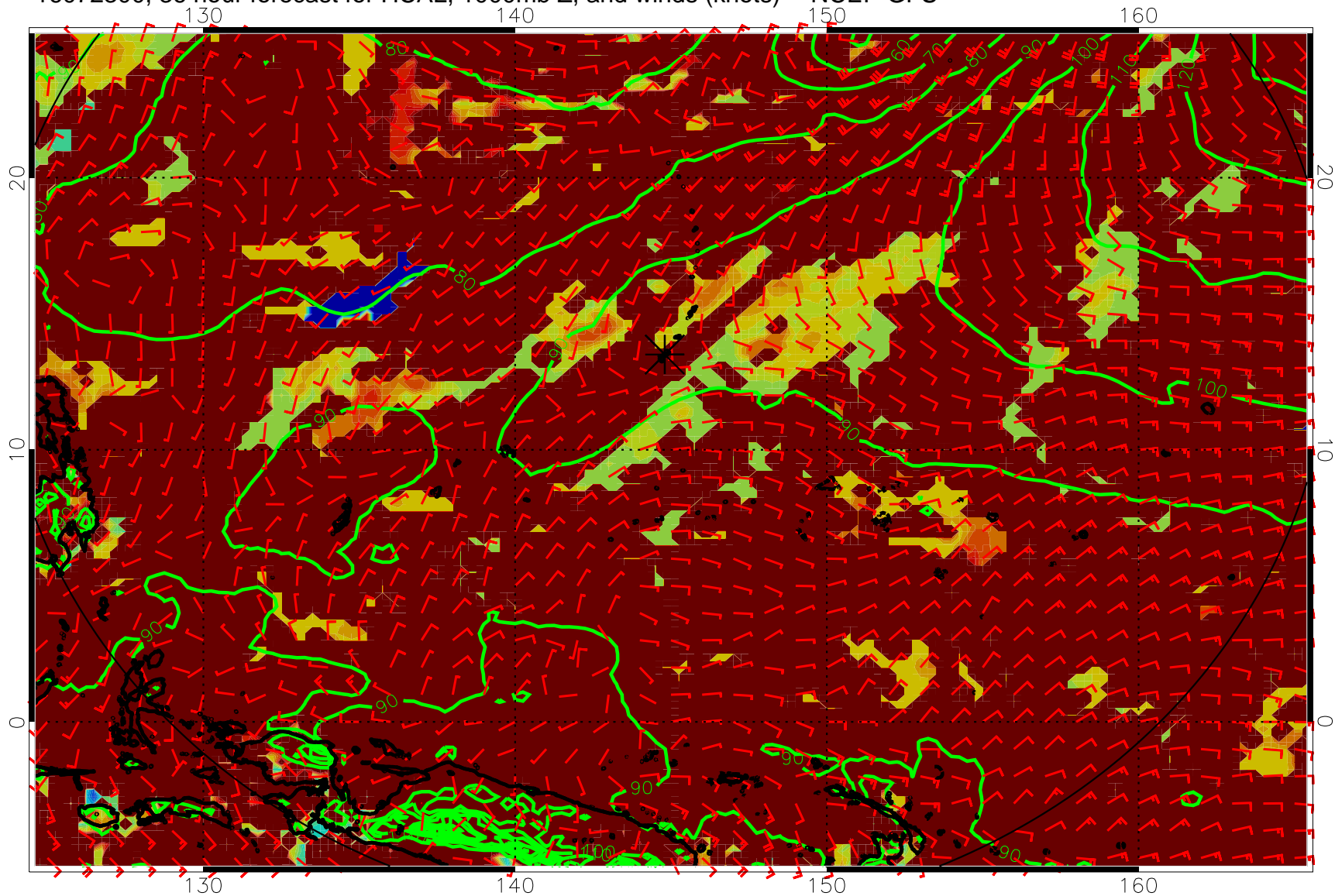
16072300, 36 hour forecast for HCAL, 1000mb Z, and winds (knots) -- NCEP GFS
