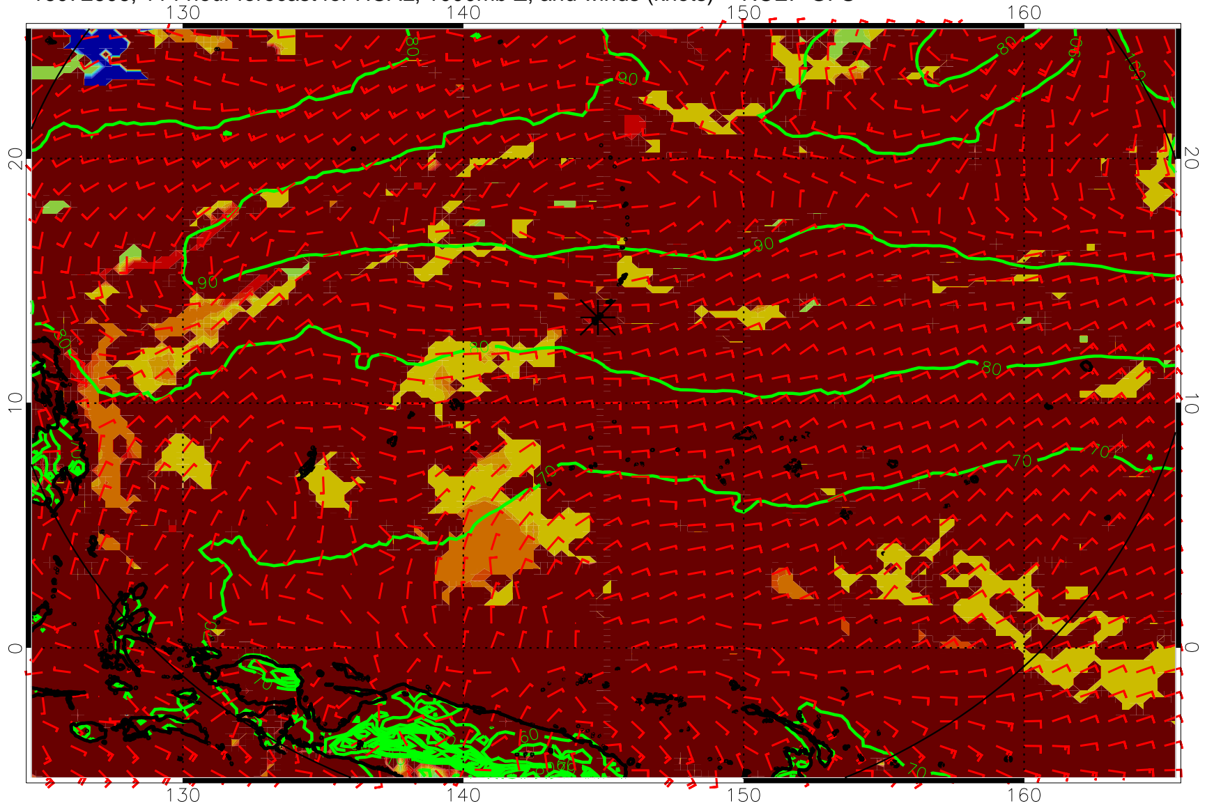
16072606, 114 hour forecast for HCAL, 1000mb Z, and winds (knots) -- NCEP GFS
