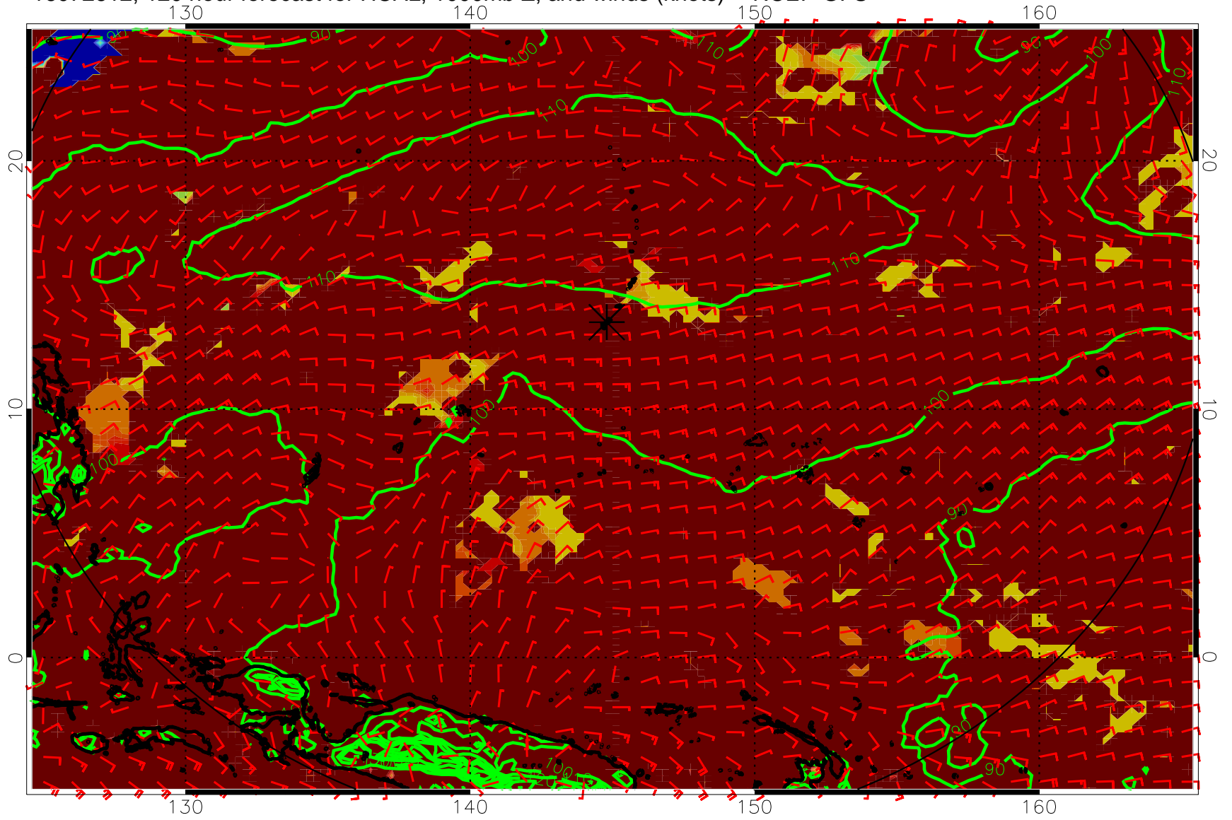
16072612, 120 hour forecast for HCAL, 1000mb Z, and winds (knots) -- NCEP GFS
