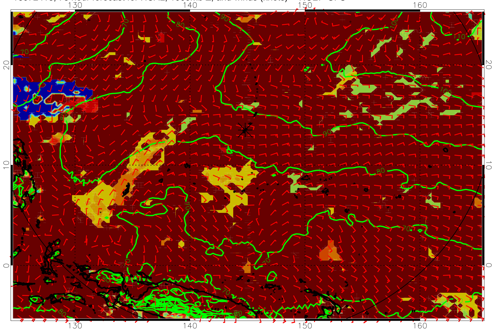
16072418, 78 hour forecast for HCAL, 1000mb Z, and winds (knots) -- NCEP GFS
