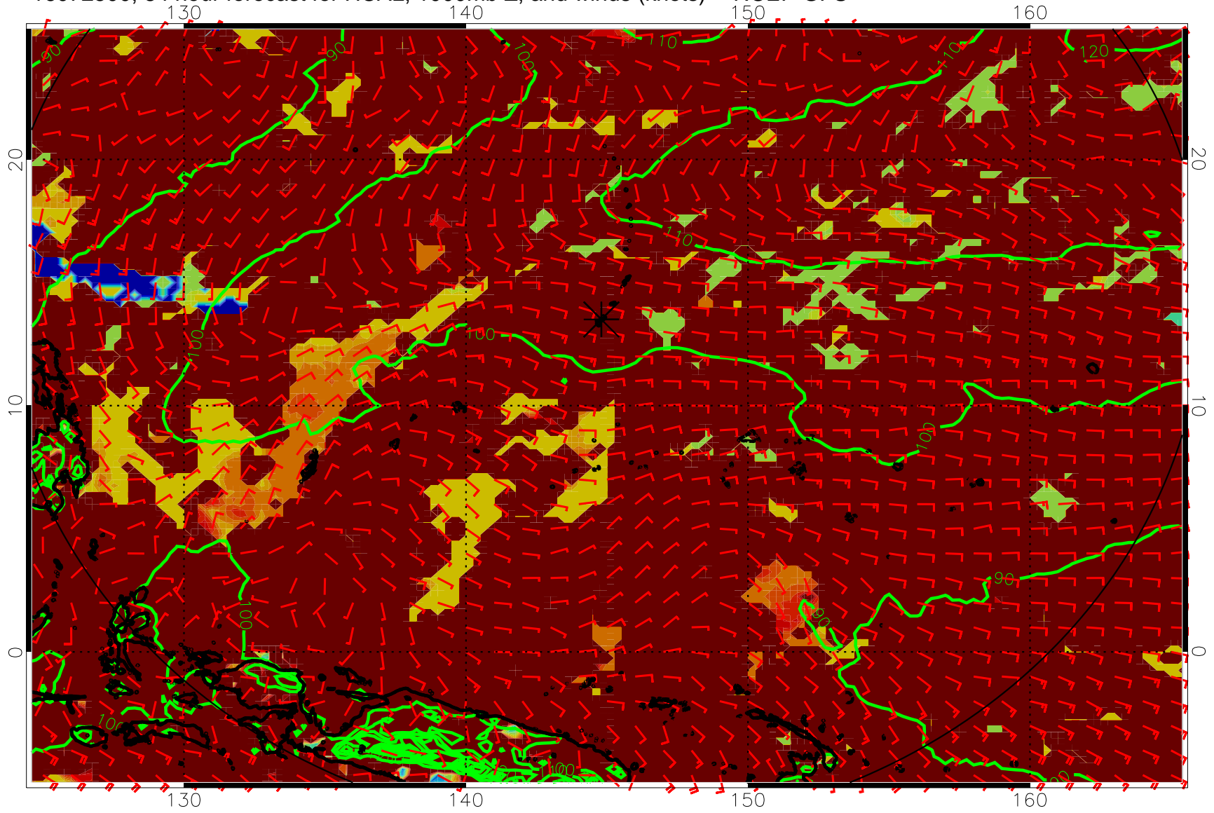
16072500, 84 hour forecast for HCAL, 1000mb Z, and winds (knots) -- NCEP GFS
