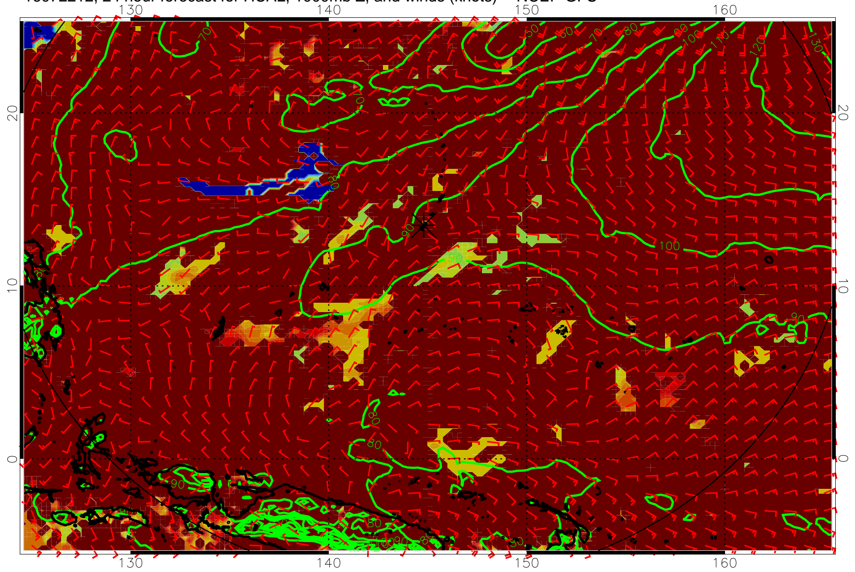
16072212, 24 hour forecast for HCAL, 1000mb Z, and winds (knots) -- NCEP GFS
