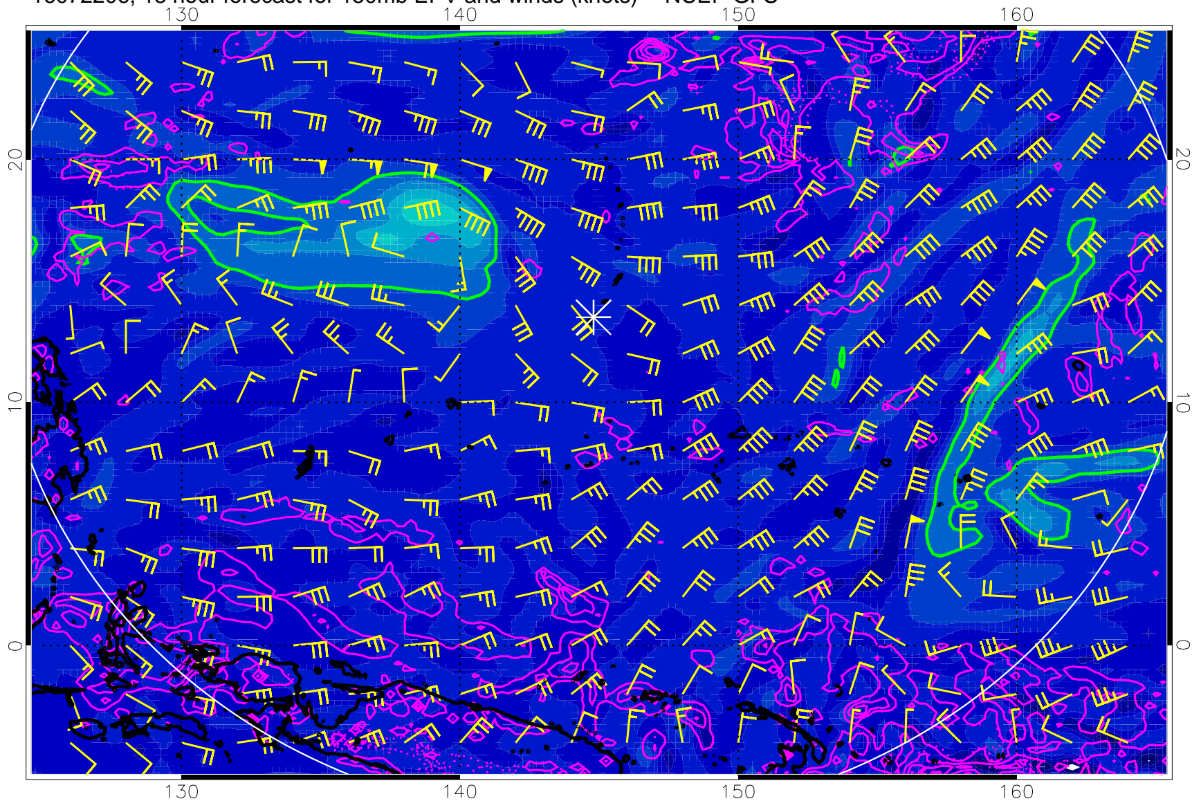
16072206, 18 hour forecast for 150mb EPV and winds (knots) -- NCEP GFS
