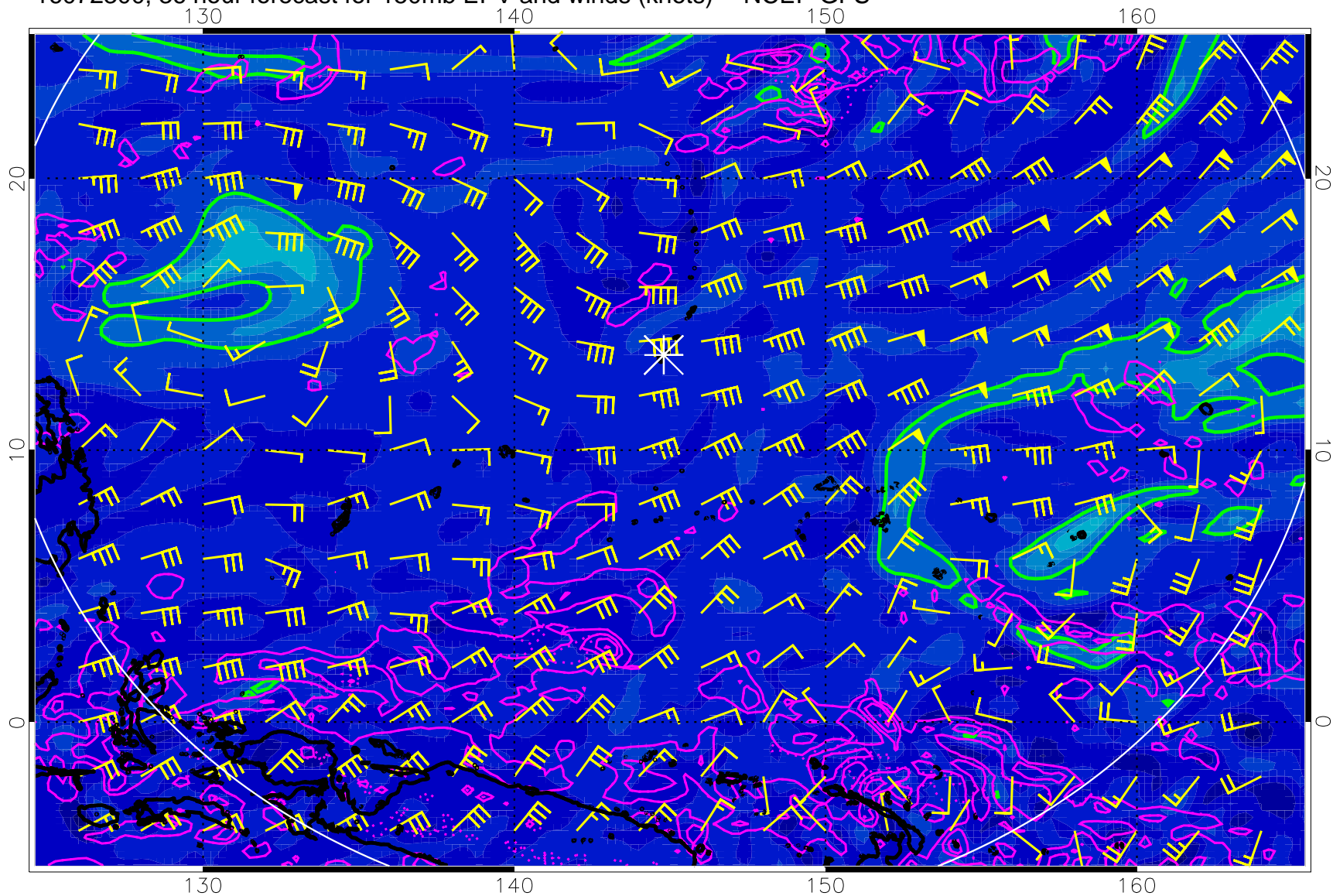
16072300, 36 hour forecast for 150mb EPV and winds (knots) -- NCEP GFS
