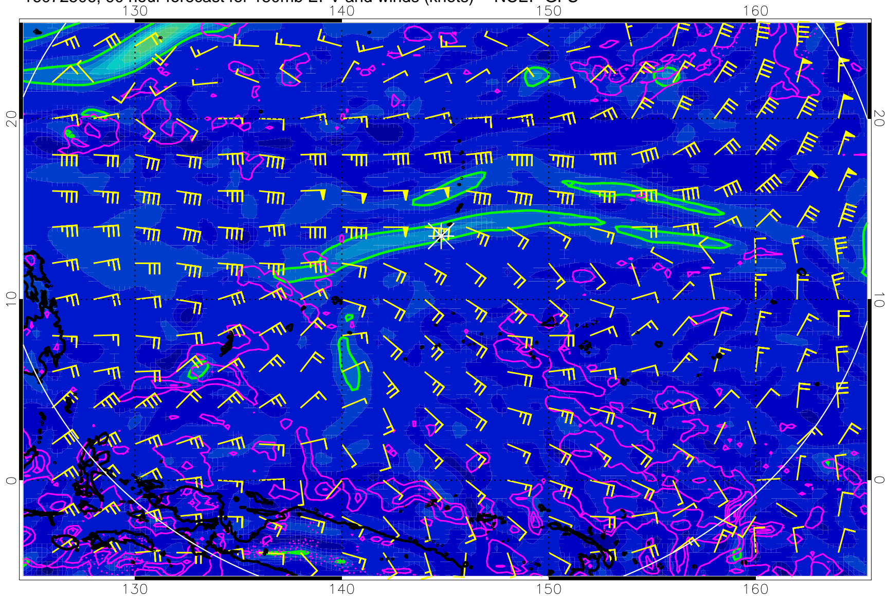
16072506, 90 hour forecast for 150mb EPV and winds (knots) -- NCEP GFS
