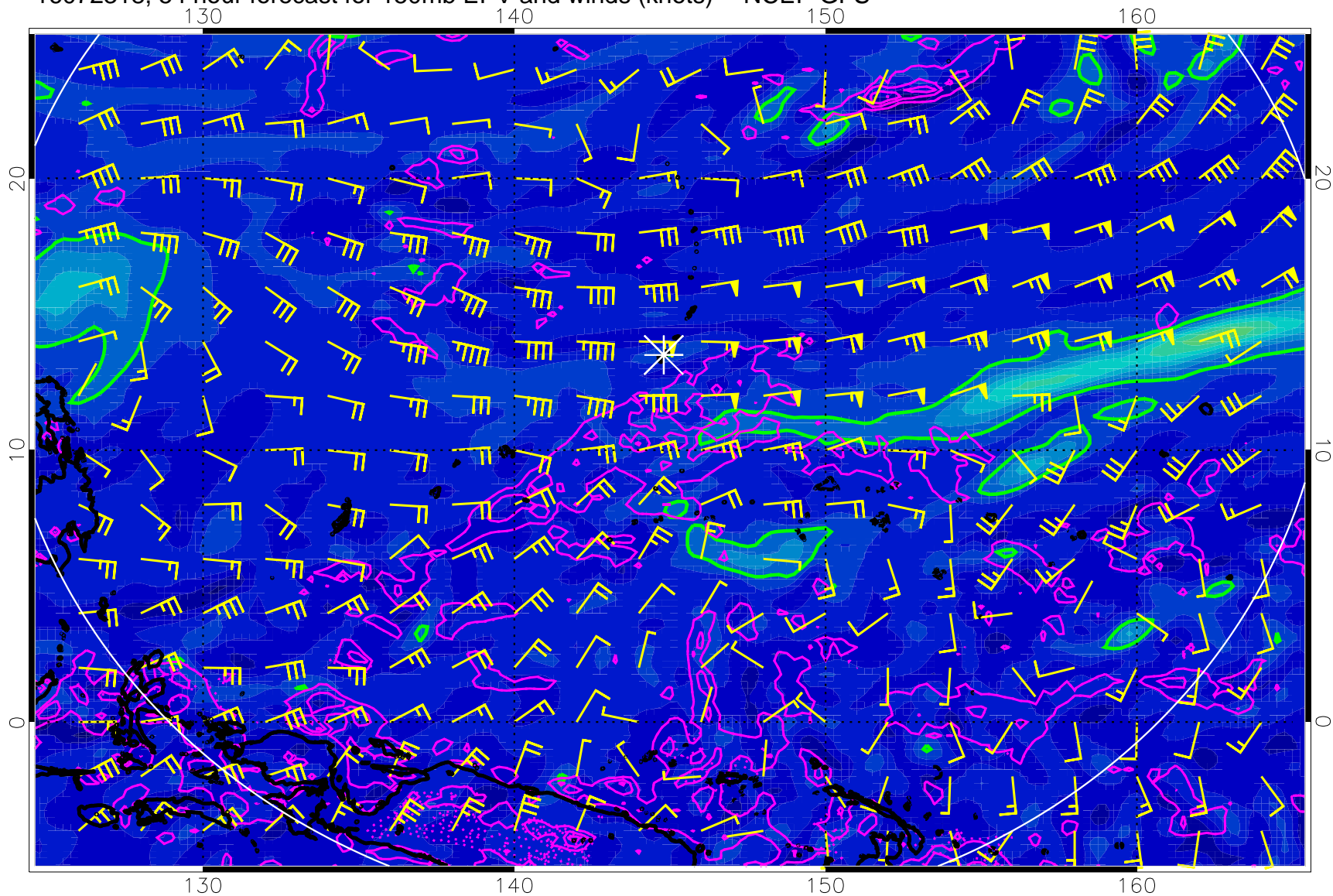
16072318, 54 hour forecast for 150mb EPV and winds (knots) -- NCEP GFS
