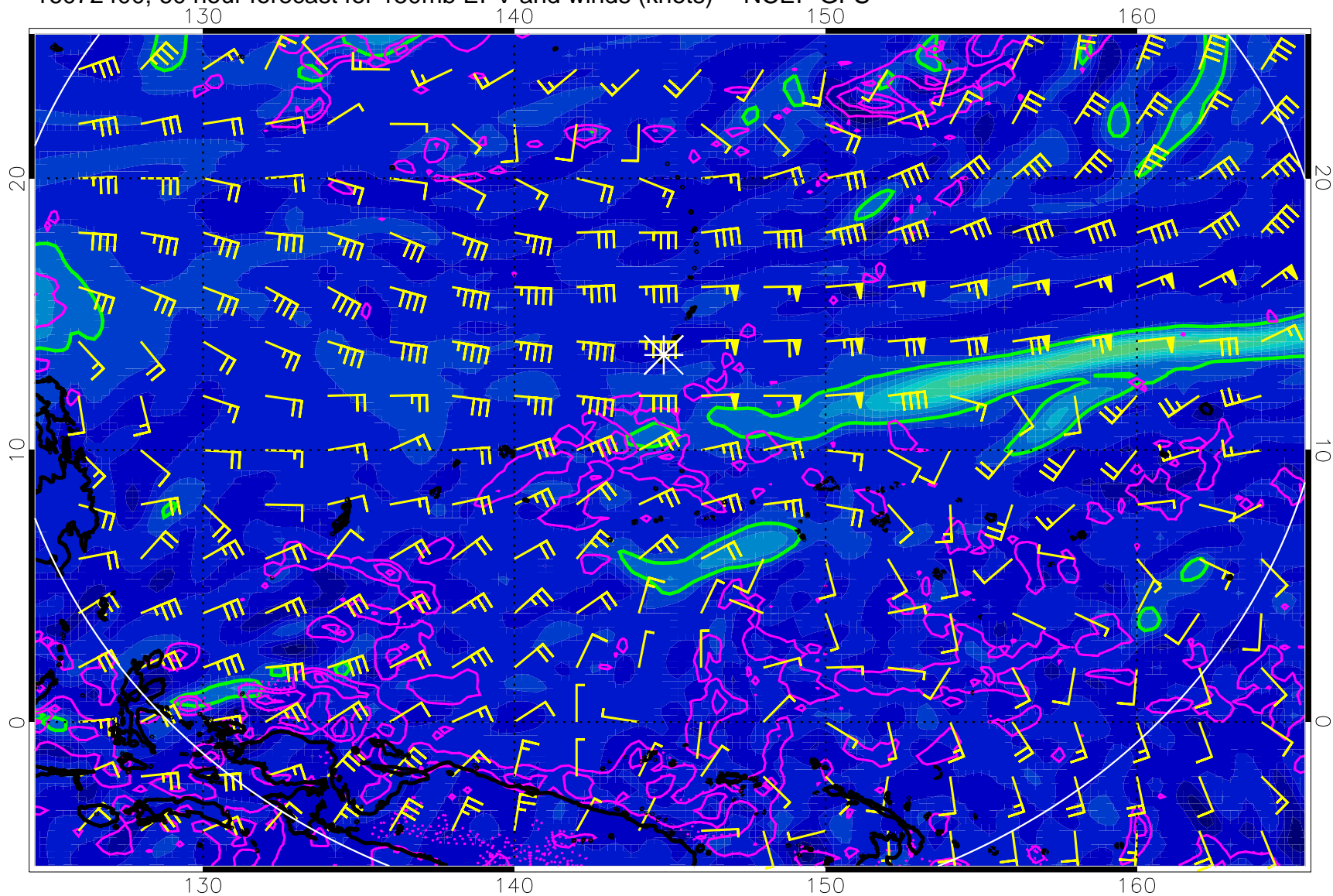
16072400, 60 hour forecast for 150mb EPV and winds (knots) -- NCEP GFS
