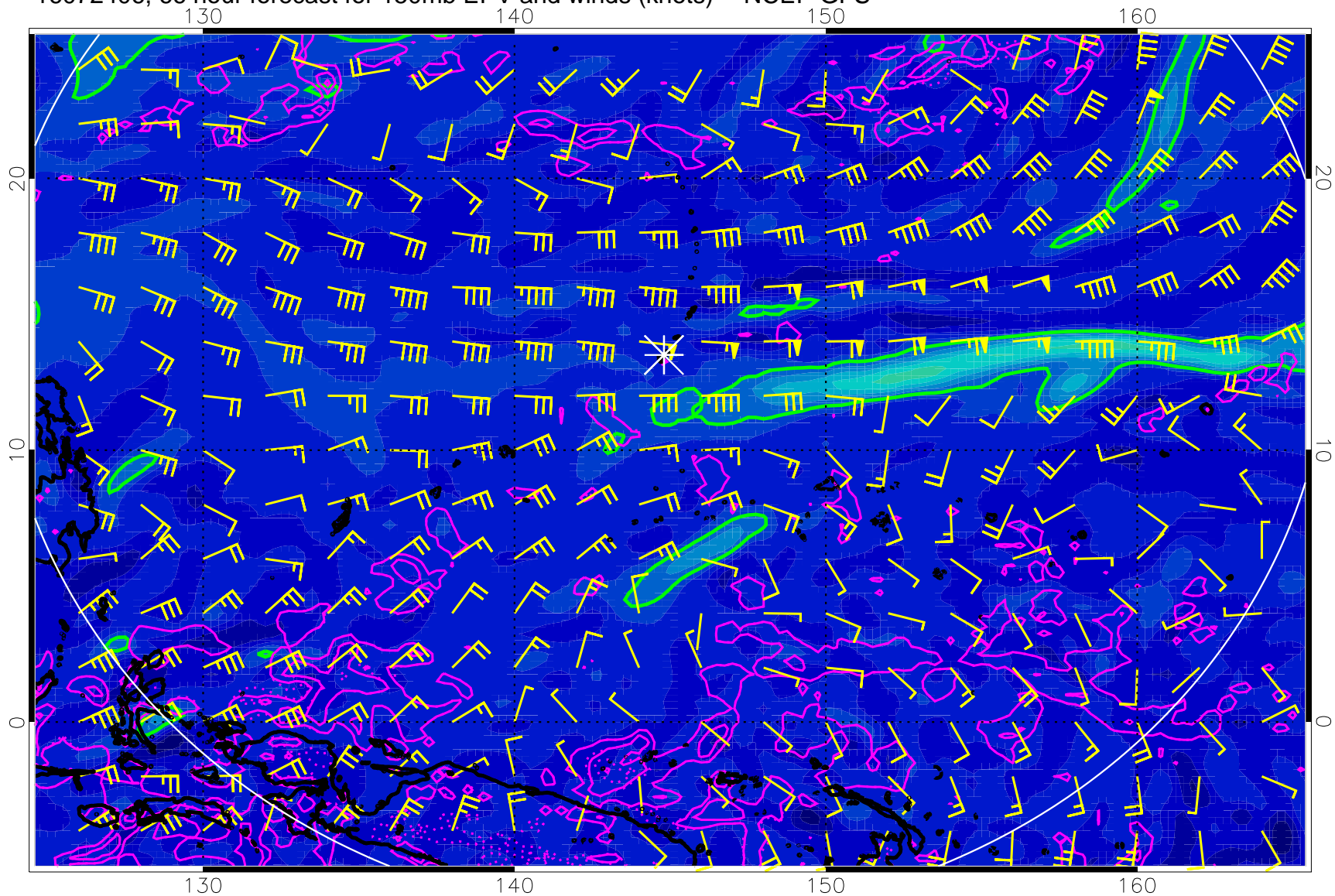
16072406, 66 hour forecast for 150mb EPV and winds (knots) -- NCEP GFS
