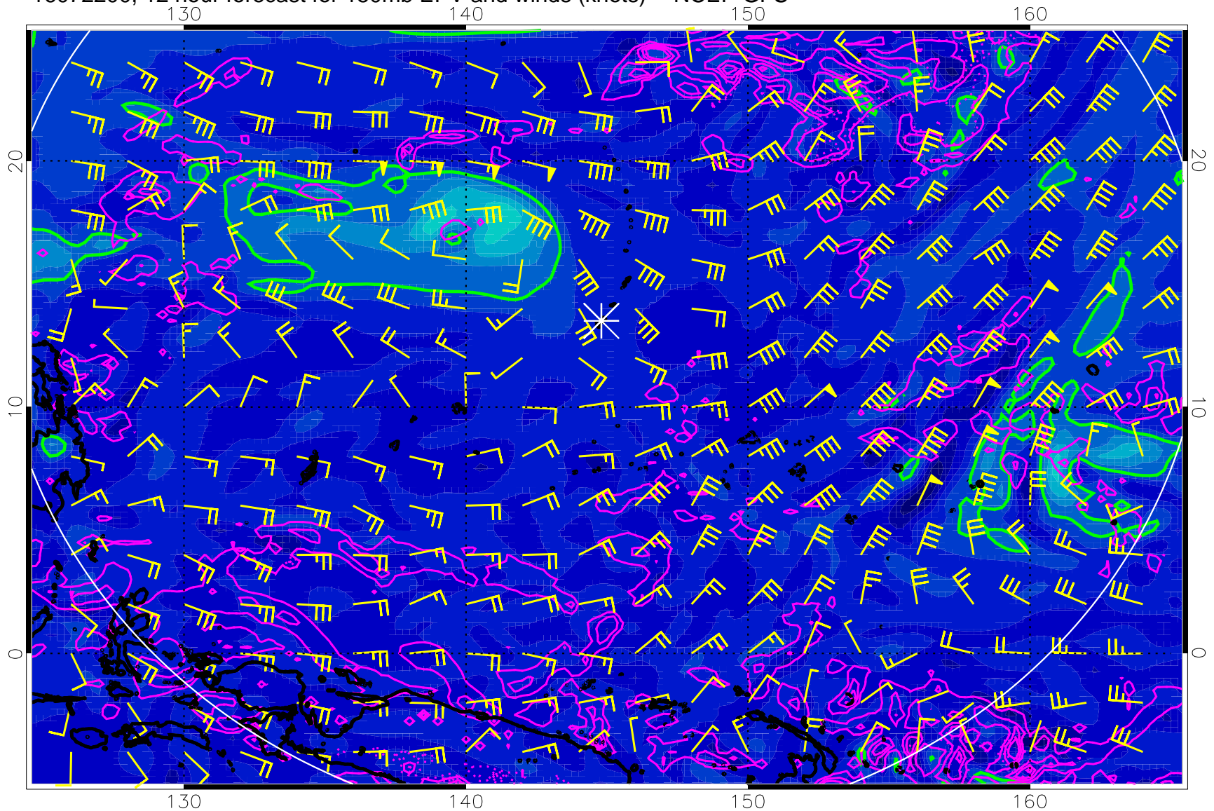
16072200, 12 hour forecast for 150mb EPV and winds (knots) -- NCEP GFS
