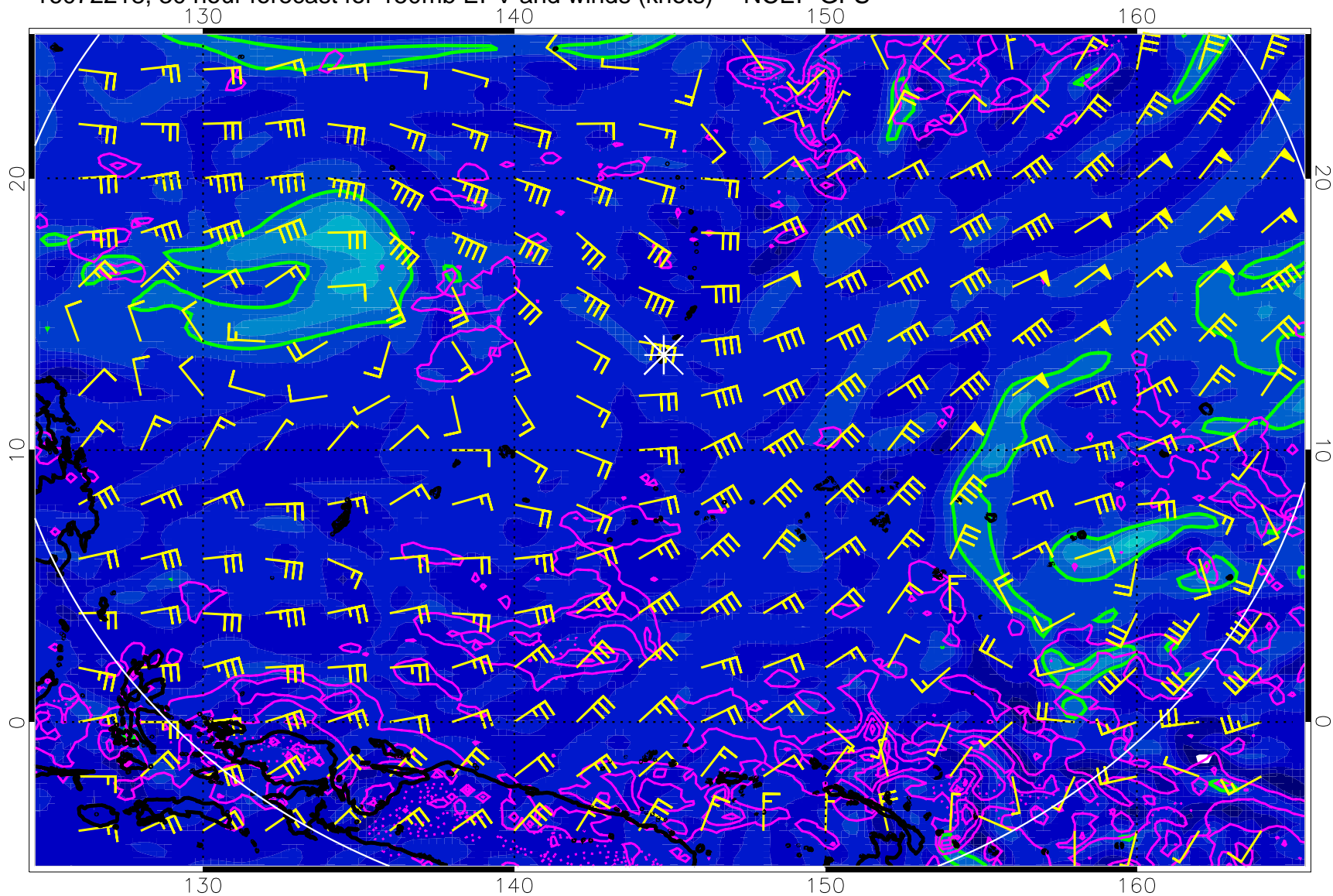
16072218, 30 hour forecast for 150mb EPV and winds (knots) -- NCEP GFS
