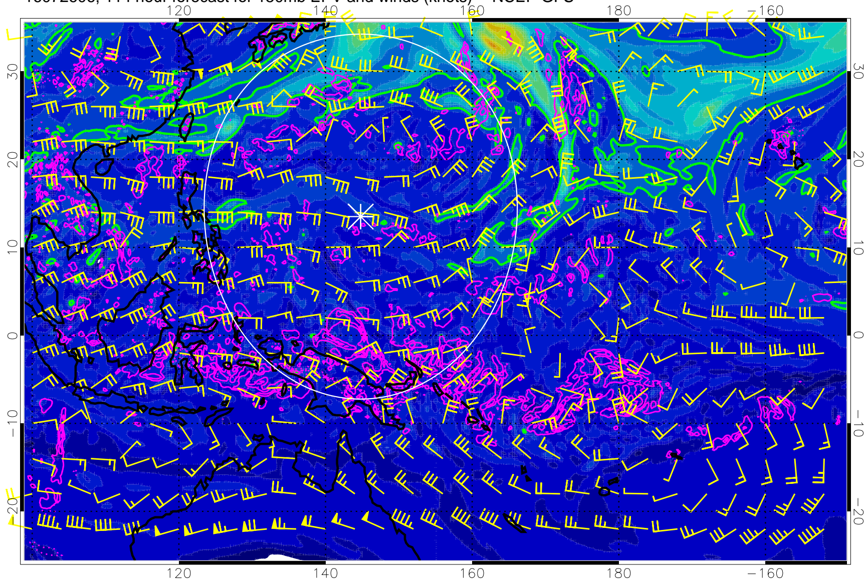
16072606, 114 hour forecast for 150mb EPV and winds (knots) -- NCEP GFS
