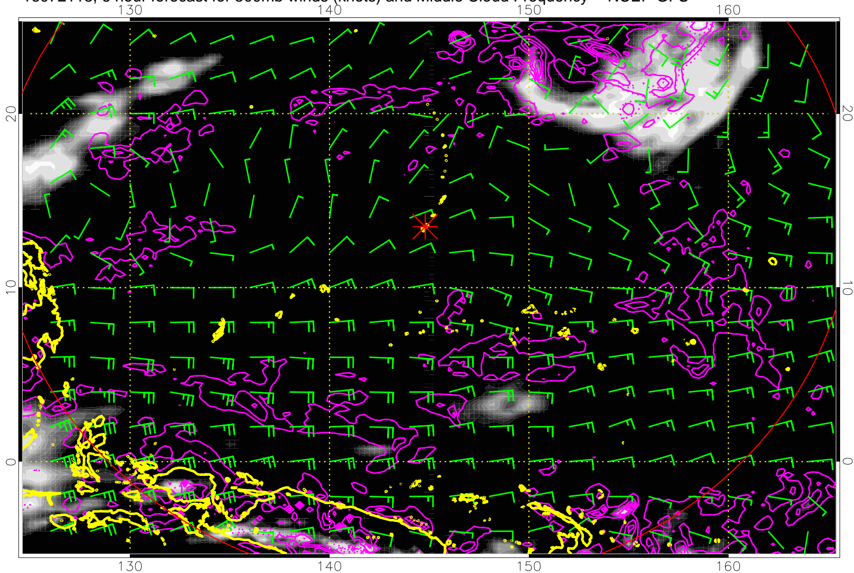
16072118, 6 hour forecast for 500mb winds (knots) and Middle Cloud Frequency -- NCEP GFS
