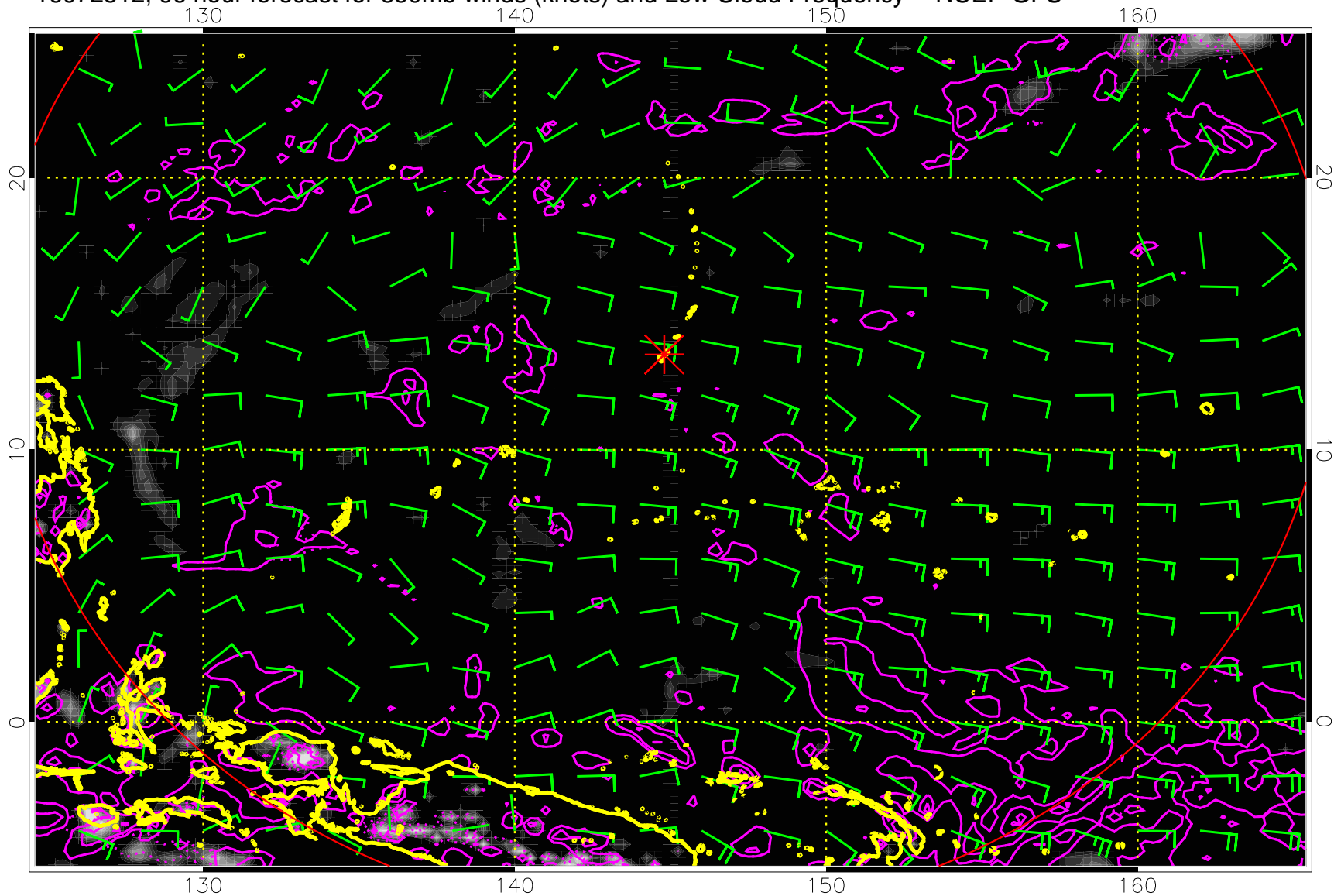
16072512, 96 hour forecast for 850mb winds (knots) and Low Cloud Frequency -- NCEP GFS
